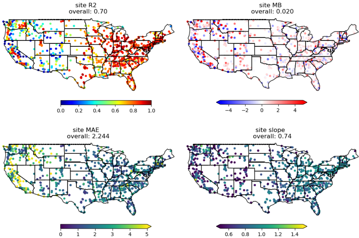
kriging stats 2006
