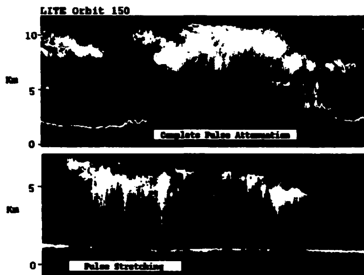
Figure 6.1: Examples of lidar pulse attenuation (Top) and pulse stretching (Bottom) caveats associated with some LITE cloud profiles.
