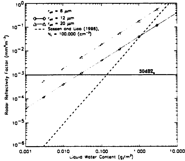
Figure 7.15: Z-LWC relationship corresponding to Equation 7.8 for varying effective radii. Shown for reference is the CloudSat -30 dBZ e sensitivity threshold. (Developed with the assistance of R. Austin)
