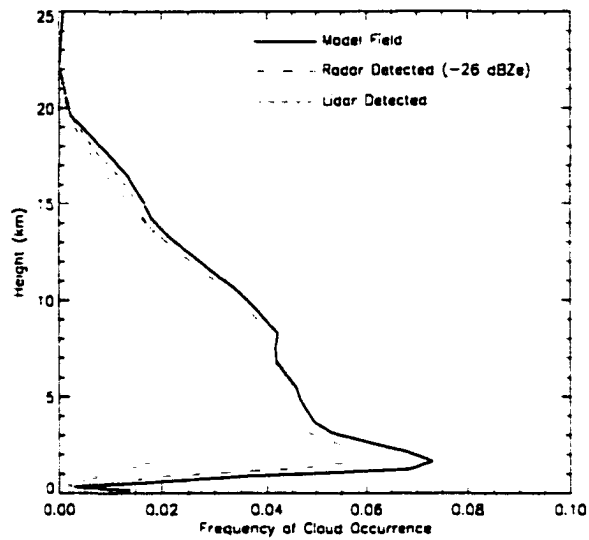
Figure 7.18: Frequency of lidar/radar cloud detection as a function of height for all 66 LITE night-time orbits using along-track ECMWF forecasts of cloud water and distribution fields.
