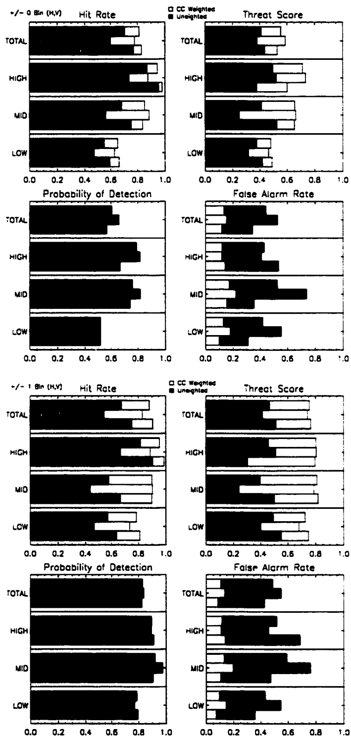
Figure B.98: LITE Orbit 124 Cloud Cover Statistics.
