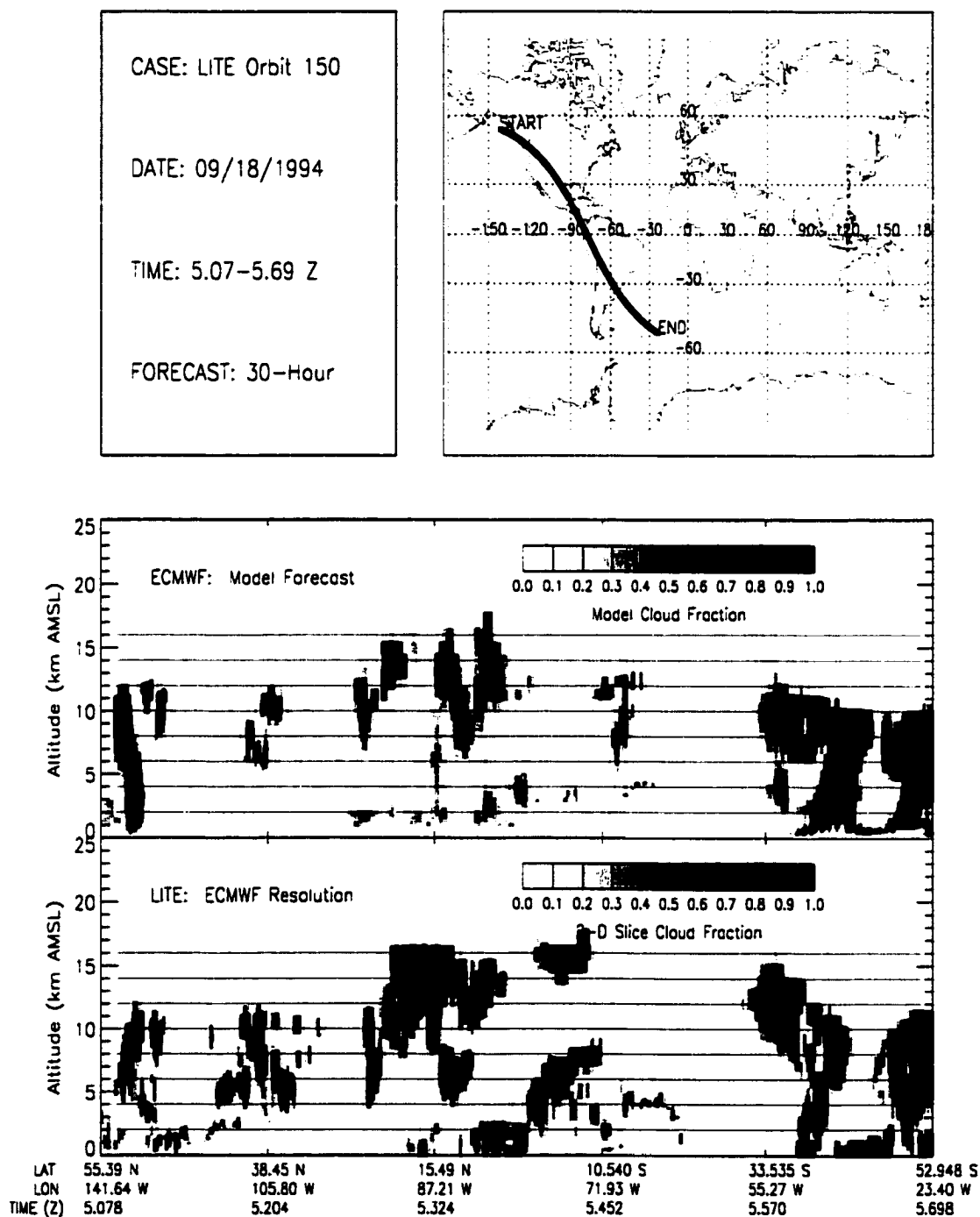
Figure B.129: LITE Orbit 150 Cloud Cover Comparison.
