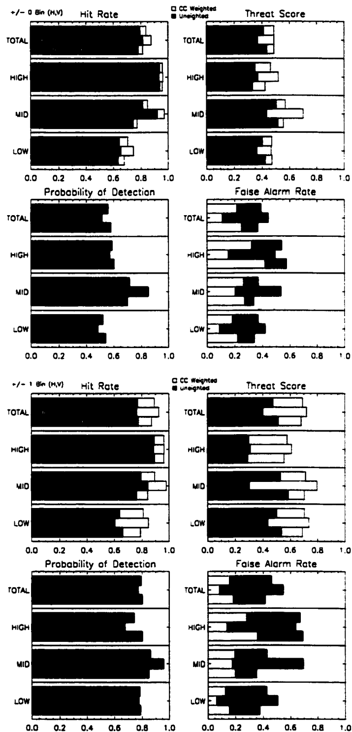
Figure B.80: LITE Orbit 104 Cloud Cover Statistics.
