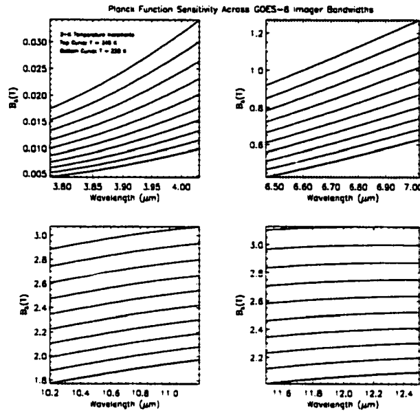
Figure 4.41: GOES-8 Channel 2-5 sensitivity to Planckian emission for typical upper-tropospheric cloud emitting temperatures.
