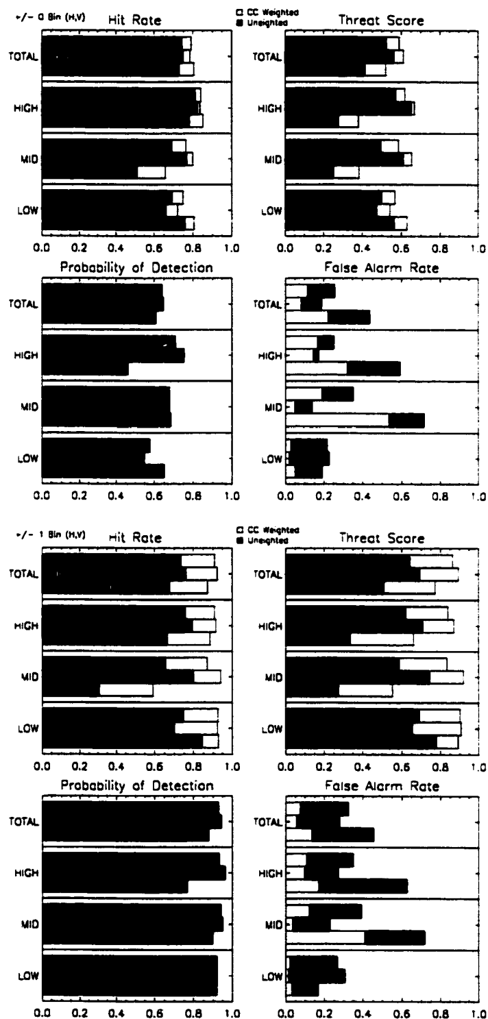
Figure B.10: LITE Orbit 015 Cloud Cover Statistics.
