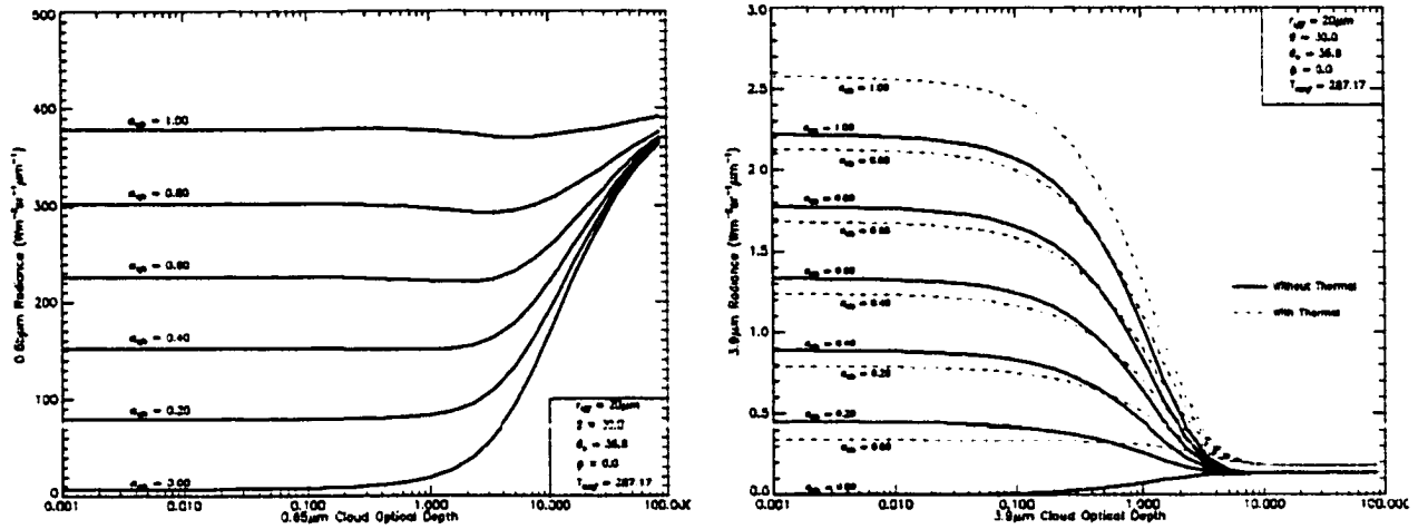
Figure 4.42: GOES Ch1 (0.65- \mu\text{m} , left panel) and Ch2 (3.9 \mu\text{m} , right panel) surface albedo sensitivities (Following Nakajima and Nakajima, 1995) for a 1km-thick water cloud with optical depth values as indicated. The 3.9 \mu\text{m} example shows full-scene (dashed) and solar-reflection only (solid) components for this case.
