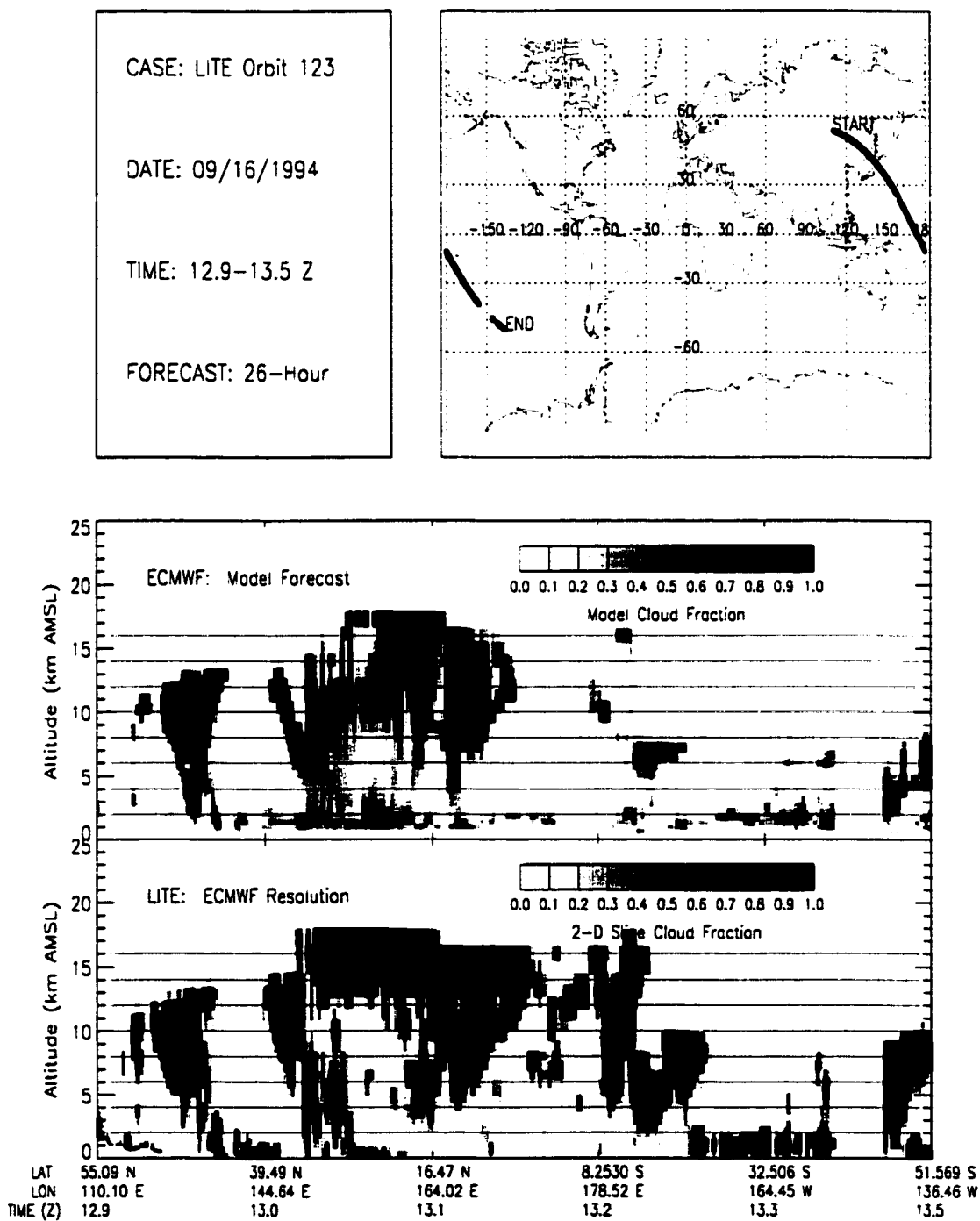
Figure B.95: LITE Orbit 123 Cloud Cover Comparison.
