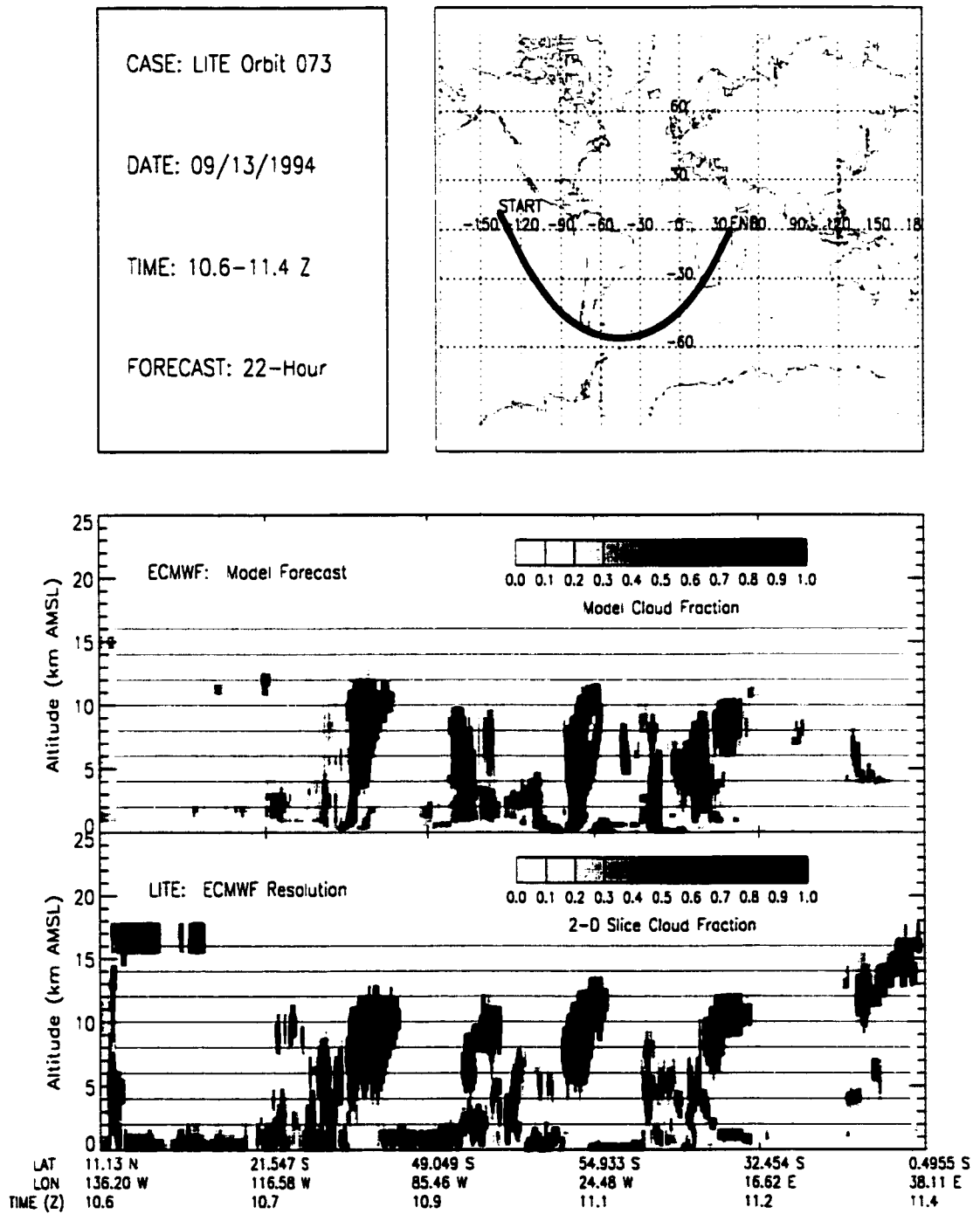
Figure B.53: LITE Orbit 073 Cloud Cover Comparison.
