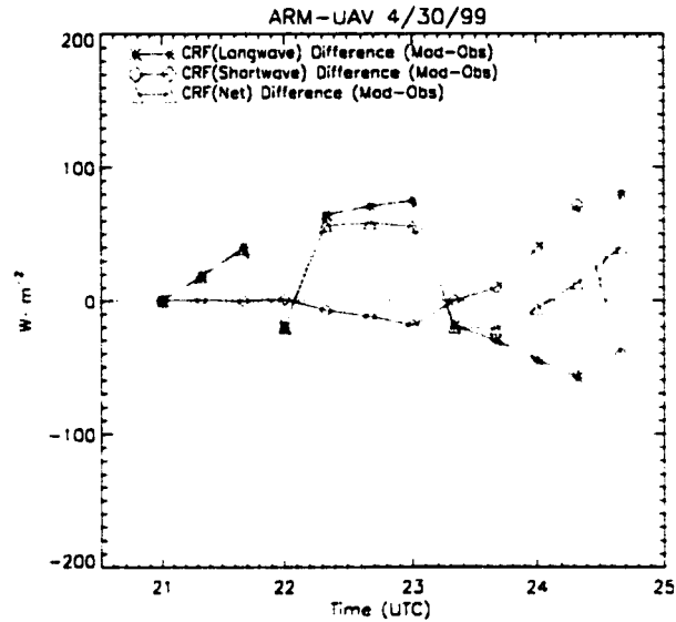
Figure 7.12: Differences between model and observed cloud radiative forcing derived from 2-stream TOA cloudy and clearsky flux results.
