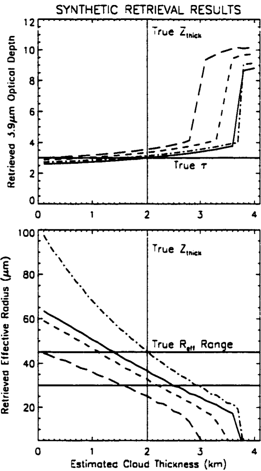
Figure 4.40: Analysis of IR-only retrieval uncertainty as a function of cloud physical thickness and vertical profile uncertainties. Sublayers are 0.5-km thick and listed from top down in the vertically inhomogeneous cases.
