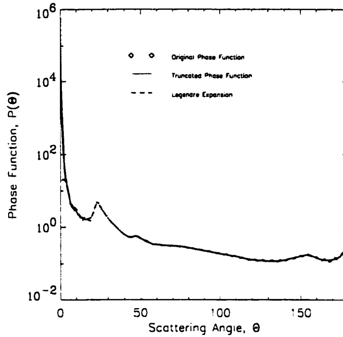
Figure 2.9: Legendre expansion of a tabulated ice crystal phase (Yang et al. , 1998) function from which \chi -expansion terms are computed.
