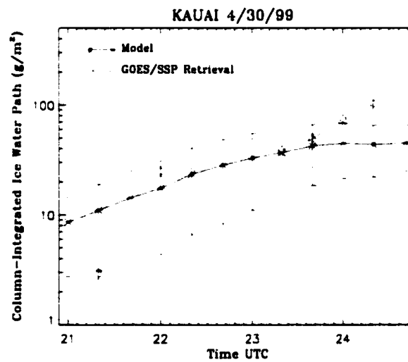
Figure 7.10: Comparison between water paths derived from GOES/SSP measurements and model forecasts for ARM-UAV 4/30/99.
