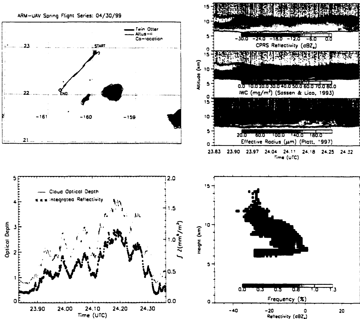
Figure 5.52: ACR results for 04/30/99 ARM-UAV flight track showing flight line (upper left), reflectivity derived products (upper right), column-integrated reflectivity and optical depth (lower left), and frequency distribution of reflectivity in space (lower right). See text for details.
