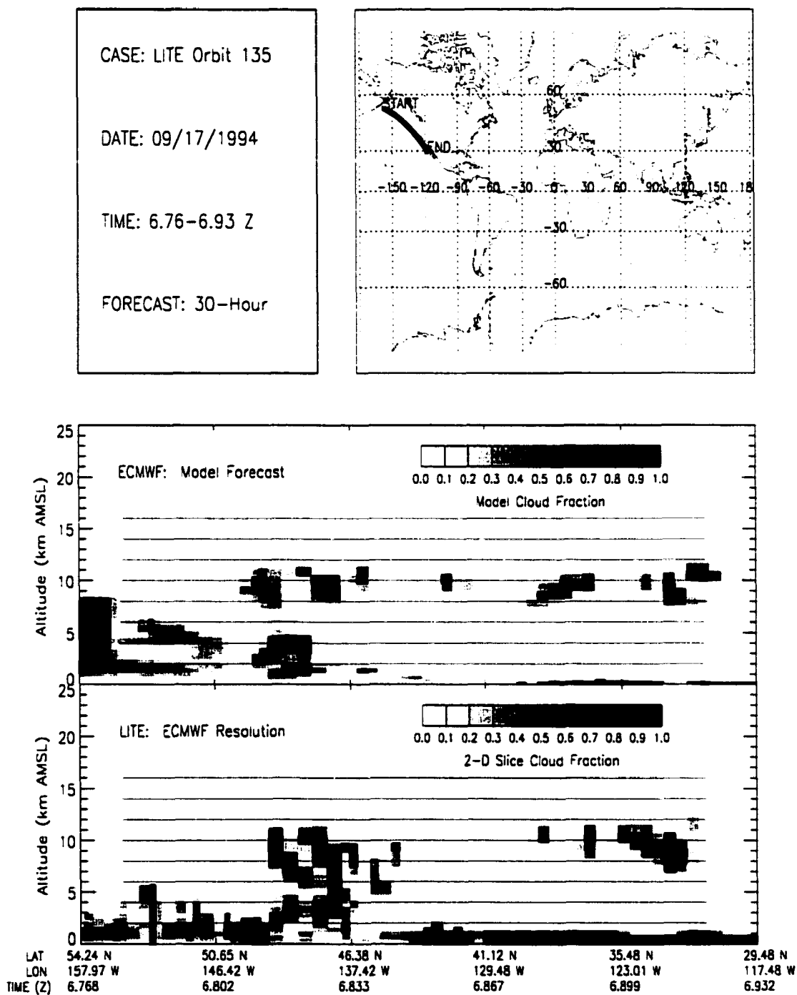
Figure B.111: LITE Orbit 135 Cloud Cover Comparison.
