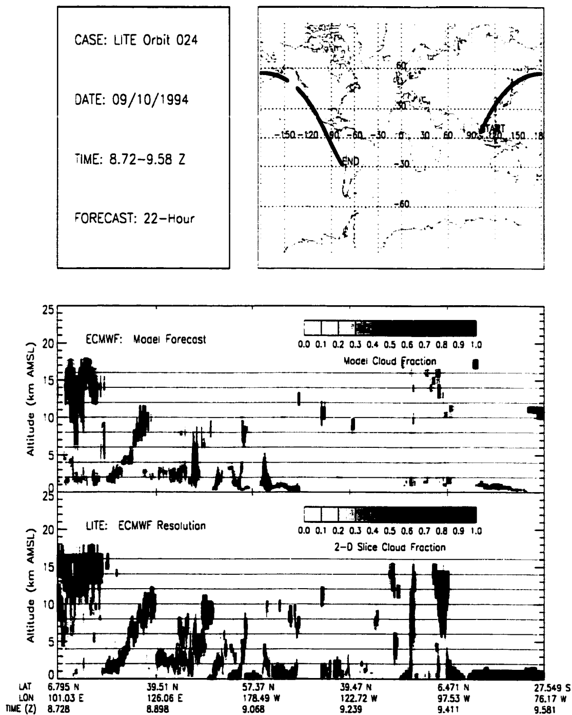
Figure B.15: LITE Orbit 024 Cloud Cover Comparison.
