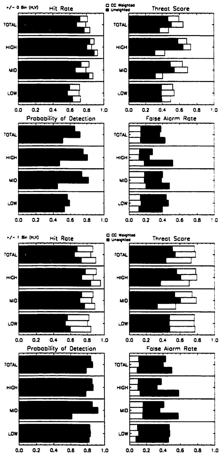
Figure B.6: LITE Orbit 013 Cloud Cover Statistics.
