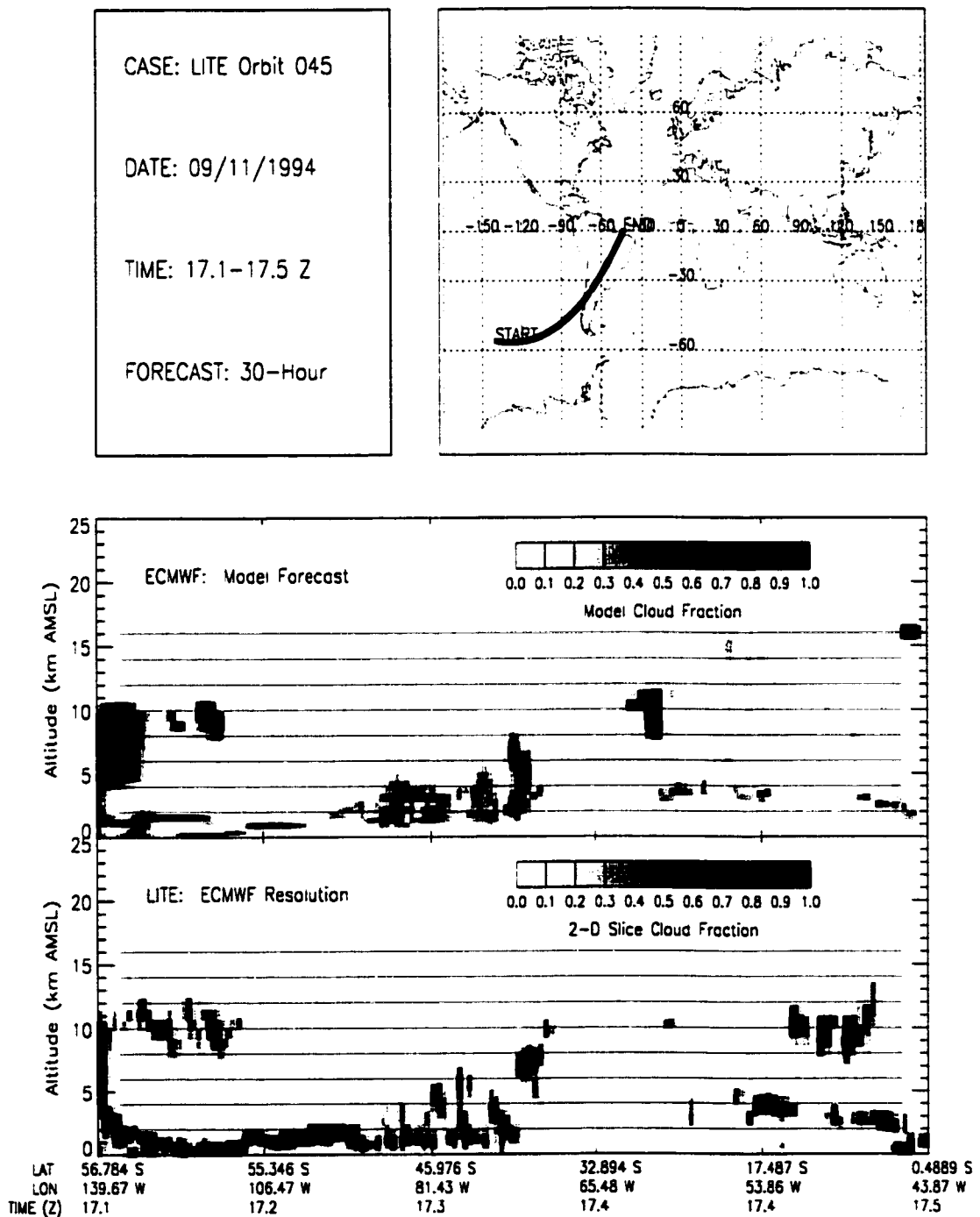
Figure B.29: LITE Orbit 045 Cloud Cover Comparison.
