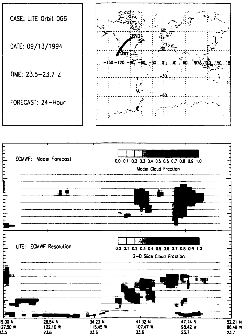
Figure B.47: LITE Orbit 066 Cloud Cover Comparison.
