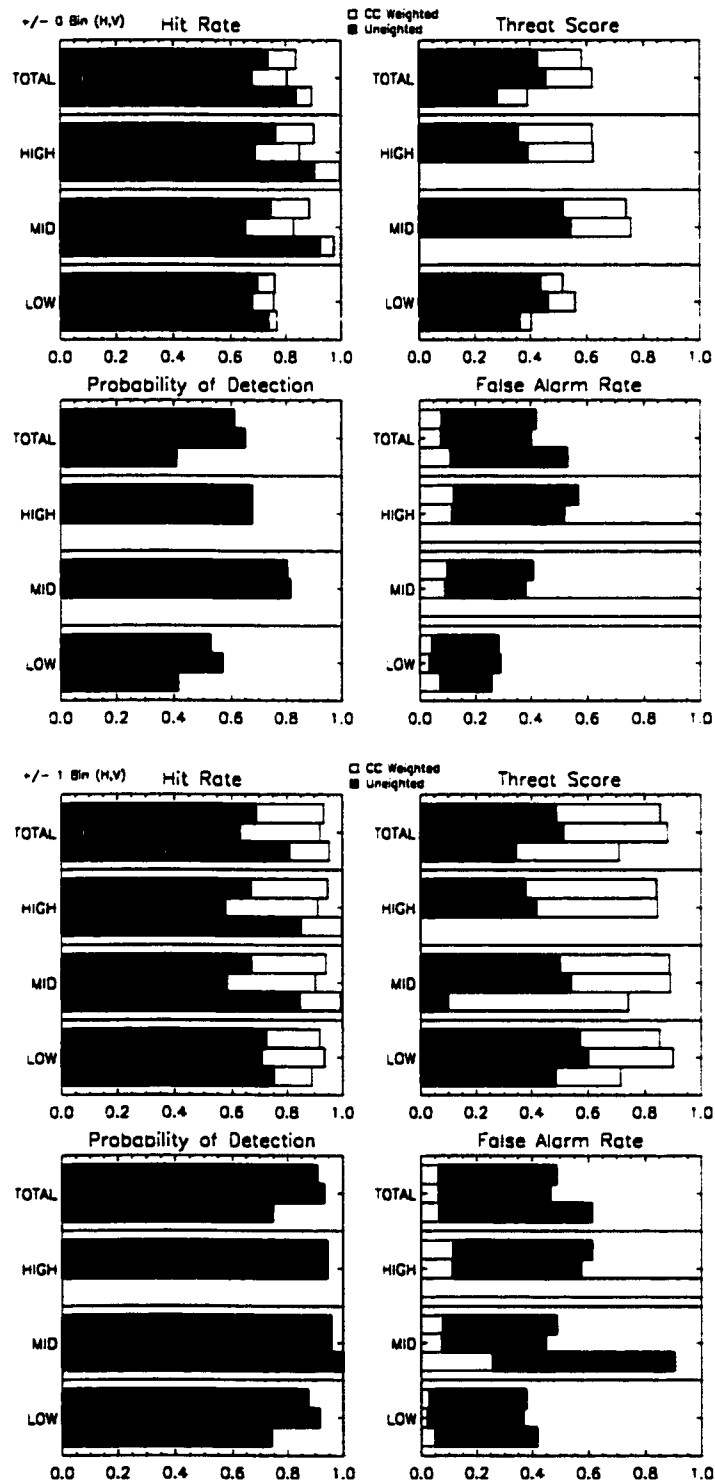
Figure B.70: LITE Orbit 083 Cloud Cover Statistics.
