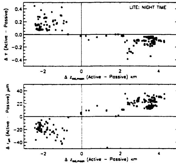
Figure 5.7: Comparison of retrieved parameter differences as a function of LITE-GOES estimated cloud heights.
