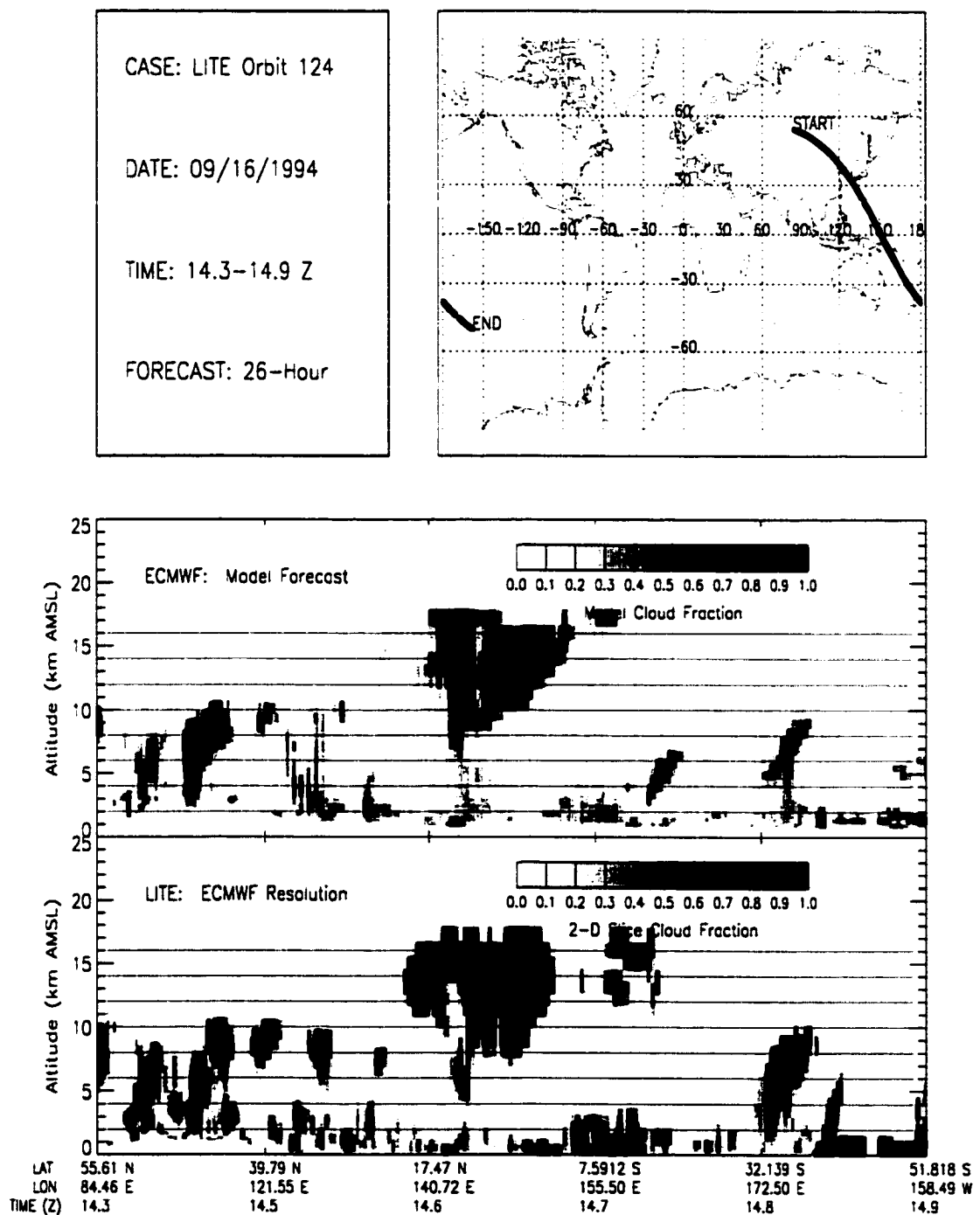
Figure B.97: LITE Orbit 124 Cloud Cover Comparison.
