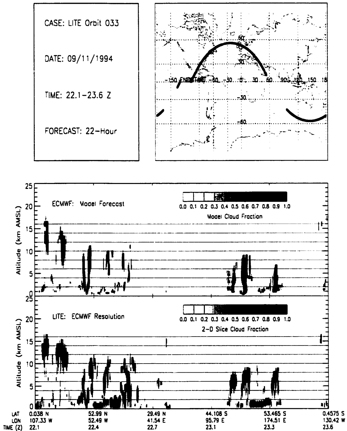
Figure B.21: LITE Orbit 033 Cloud Cover Comparison.
