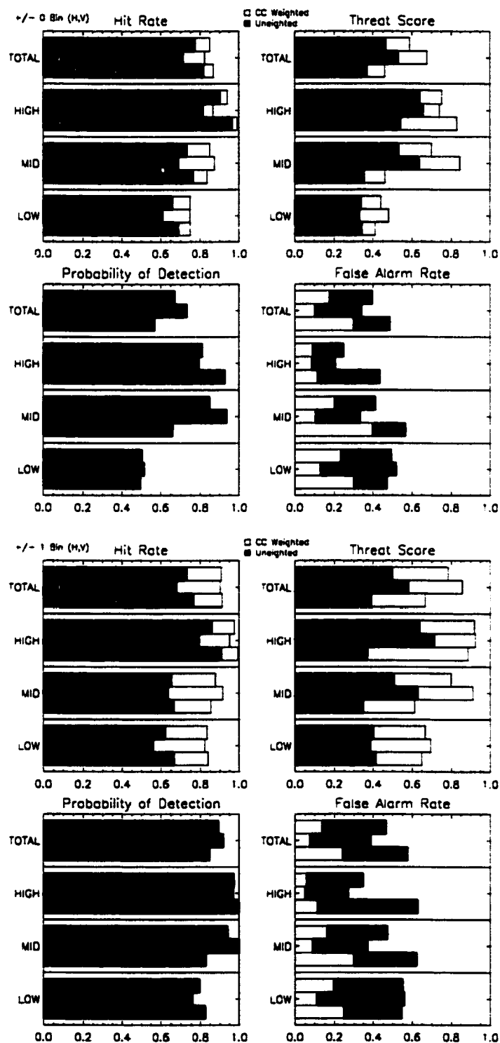
Figure B.122: LITE Orbit 146 Cloud Cover Statistics.
