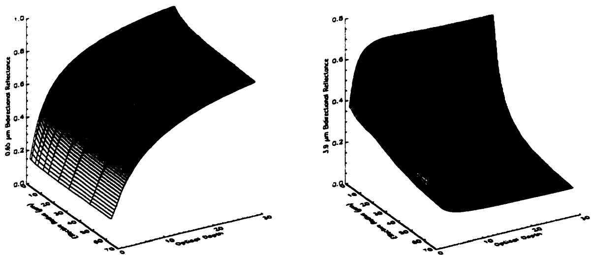
Figure 4.13: GOES Ch1 (0.65 \mu\text{m} ) and Ch2 (3.9 \mu\text{m} ) cloud parameter sensitivities for a 1km-thick water cloud ( \mu_0 = 0.6 , \mu = 0.707 , \phi - \phi_0 = 0.0 ).
