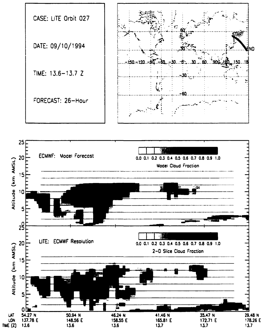
Figure B.17: LITE Orbit 027 Cloud Cover Comparison.
