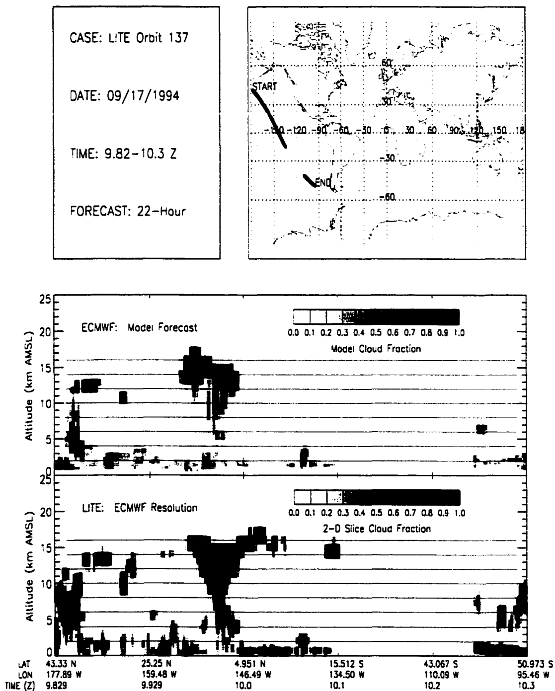
Figure B.115: LITE Orbit 137 Cloud Cover Comparison.
