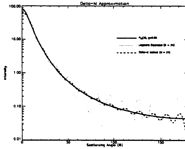
Figure 2.8: Legendre expansion of a Henyey-Greenstein phase function showing Delta-M improvement in approximation for the same order of expansion.
