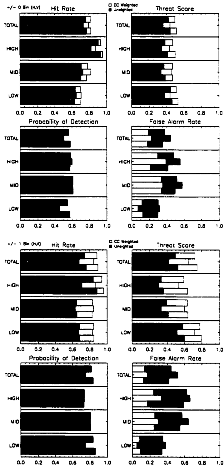
Figure B.56: LITE Orbit 074 Cloud Cover Statistics.
