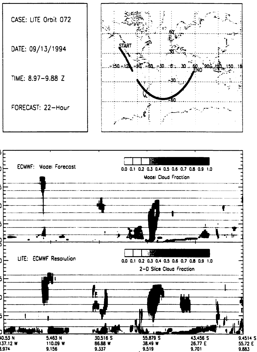
Figure B.51: LITE Orbit 072 Cloud Cover Comparison.
