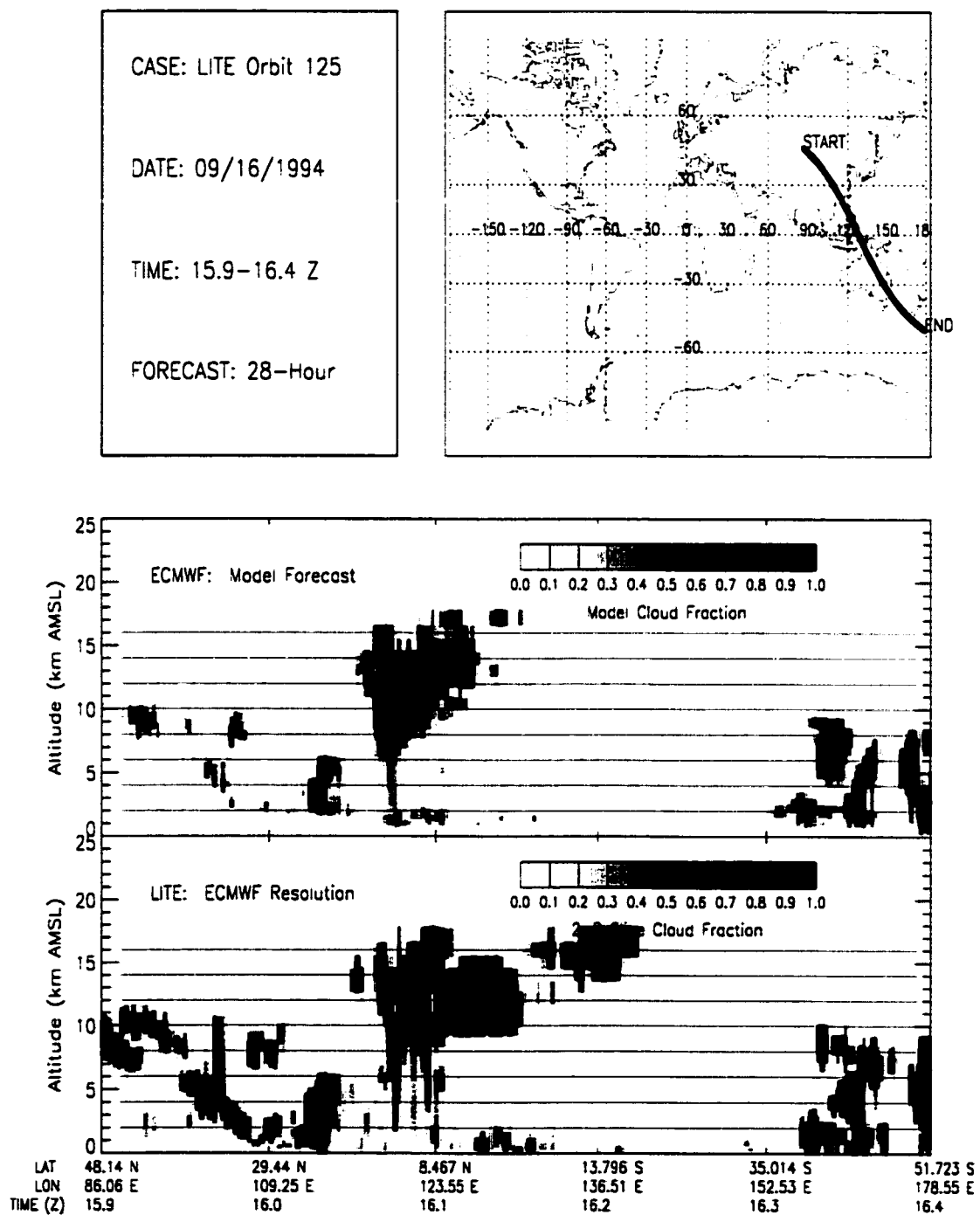
Figure B.99: LITE Orbit 125 Cloud Cover Comparison.
