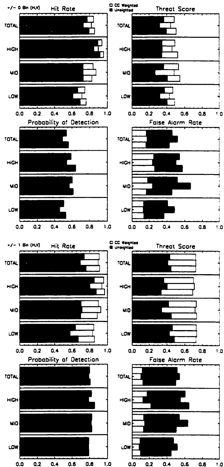
Figure B.24: LITE Orbit 034 Cloud Cover Statistics.
