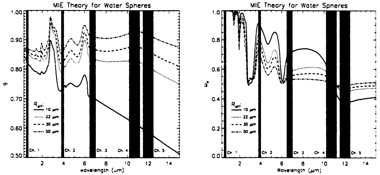
Figure 4.4: Spectral dependency of cloud optical parameters based on Mie theory for water spheres and a modified- \gamma size distribution. GOES imager channel bandwidths are indicated. Left panel: asymmetry parameter, Right panel: single-scatter albedo.
