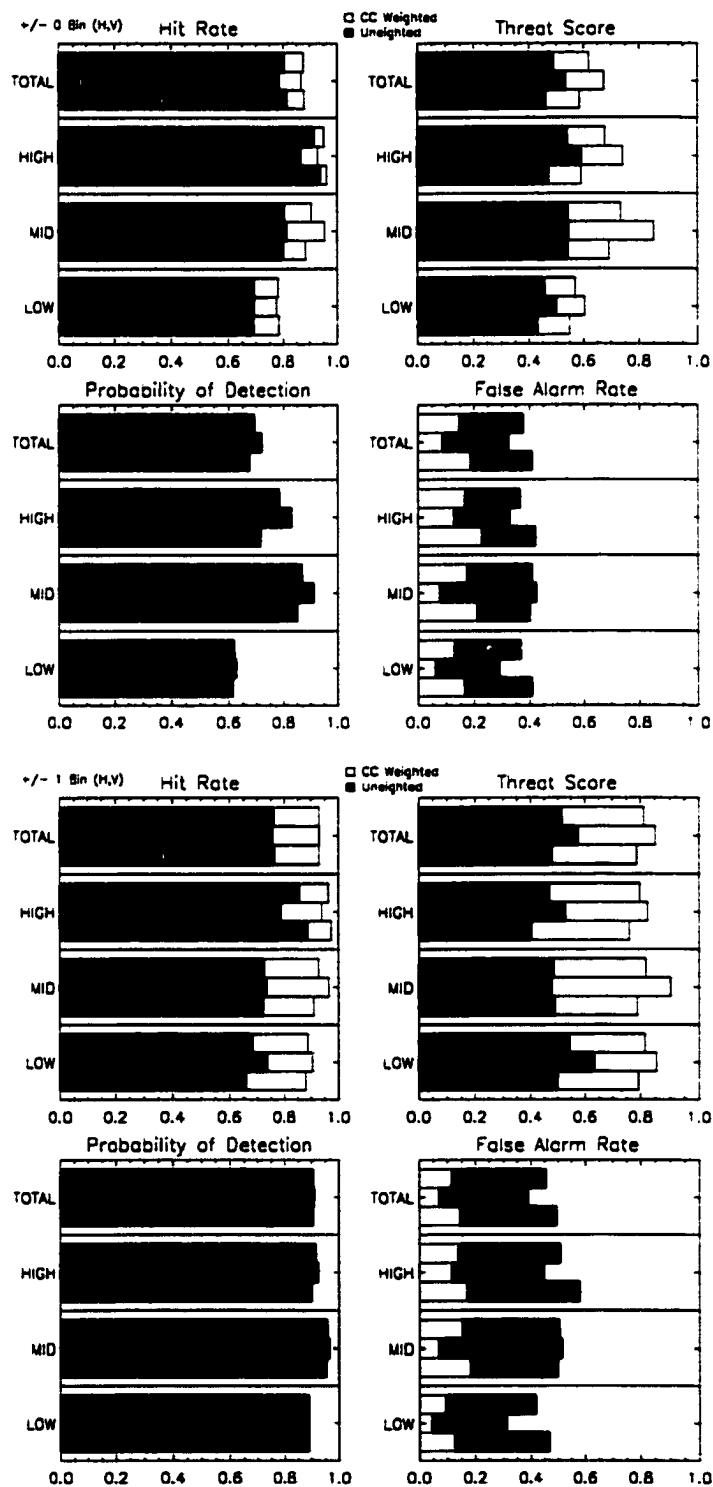
Figure B.34: LITE Orbit 047 Cloud Cover Statistics.
