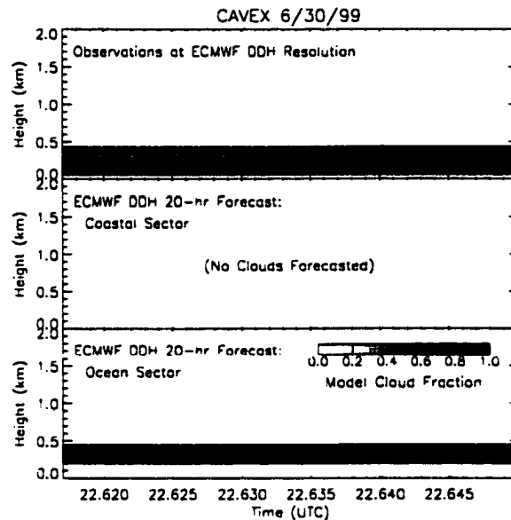
Figure 6.24: Comparison between radar (rebinbed to model resolution) and ECMWF cloud fraction forecast for CAVEX 6/30/99. See text for details of coastal and ocean sectors.
