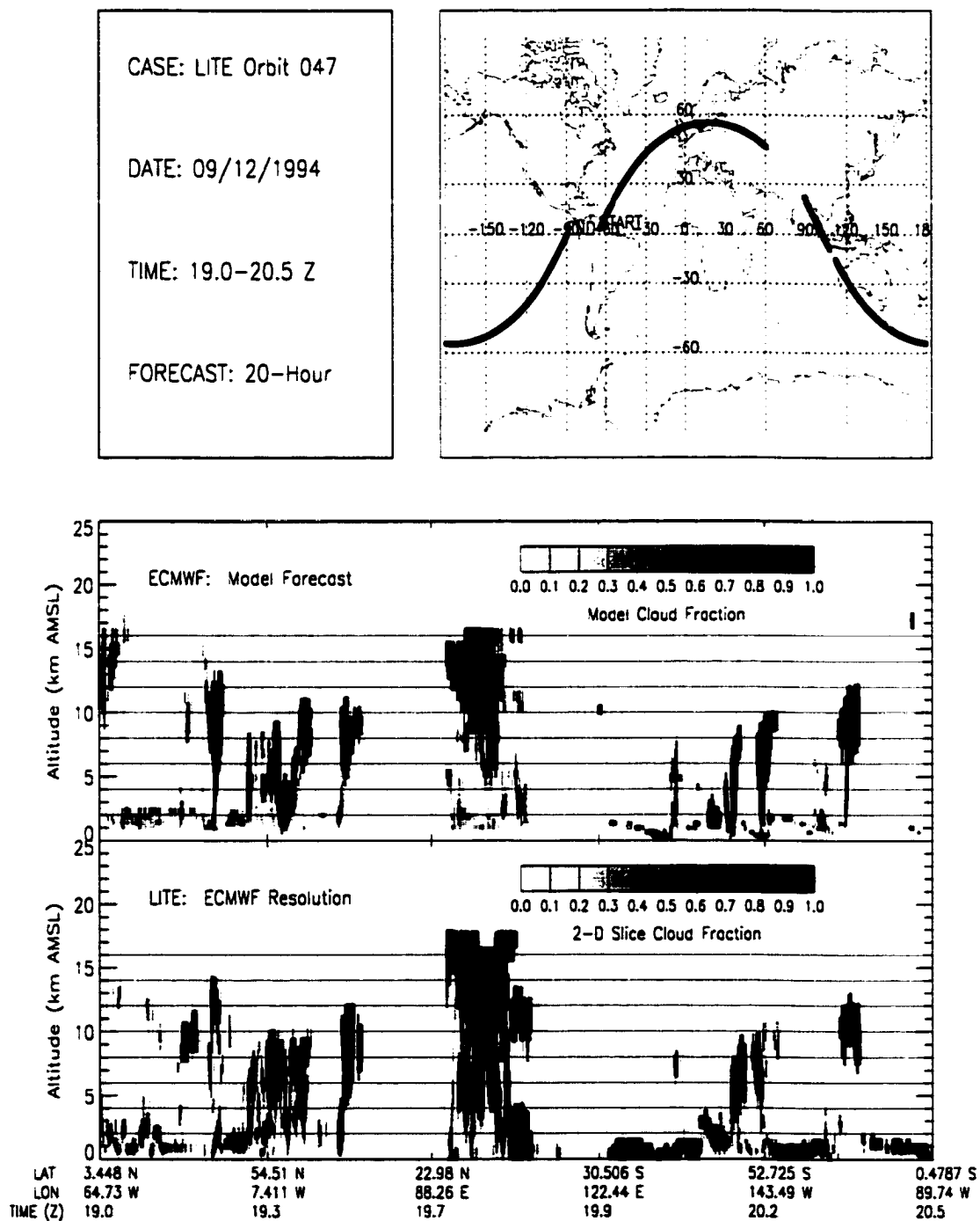
Figure B.33: LITE Orbit 047 Cloud Cover Comparison.
