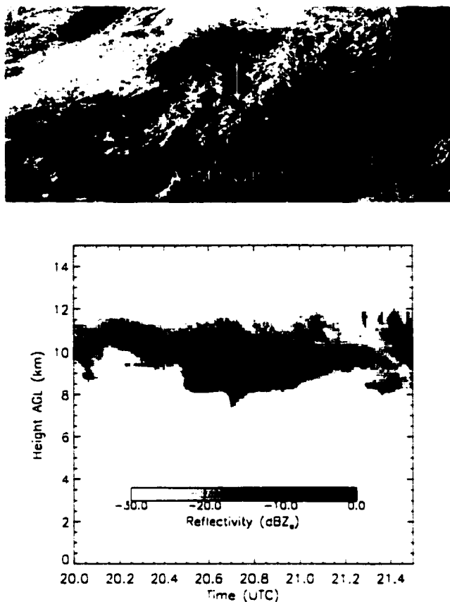
Figure 5.38: GOES-8 coverage of the ARM-SWIOF shown for the 3.9- \mu\text{m} imager channel (upper panel) and the surface-based cloud radar detected cirrus profile (lower panel).
