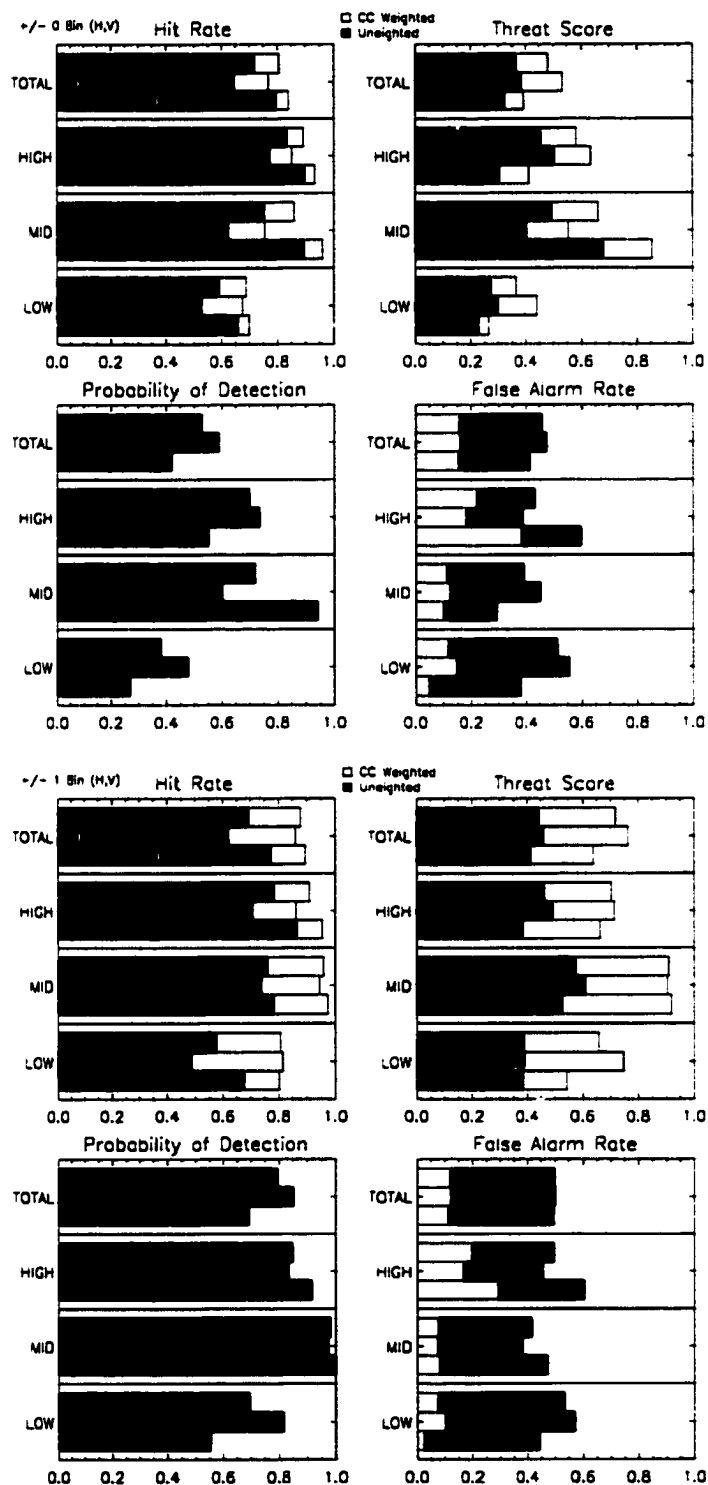
Figure B.8: LITE Orbit 014 Cloud Cover Statistics.
