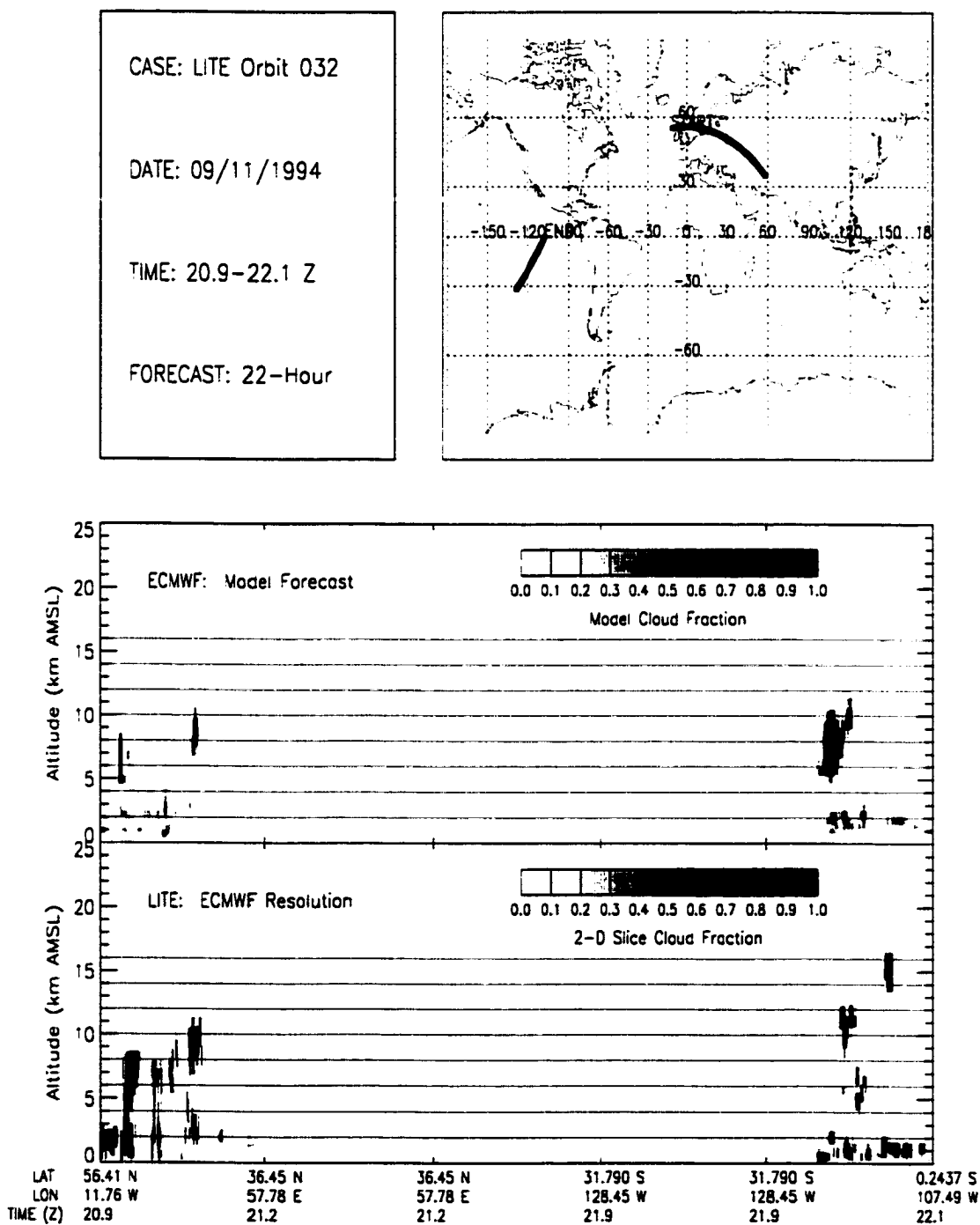
Figure B.19: LITE Orbit 032 Cloud Cover Comparison.
