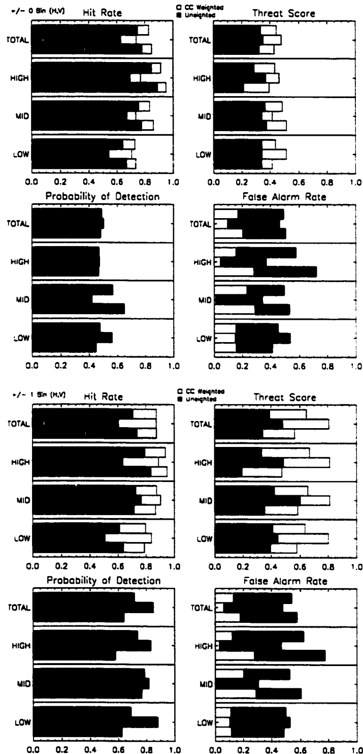
Figure B.68: LITE Orbit 082 Cloud Cover Statistics.
