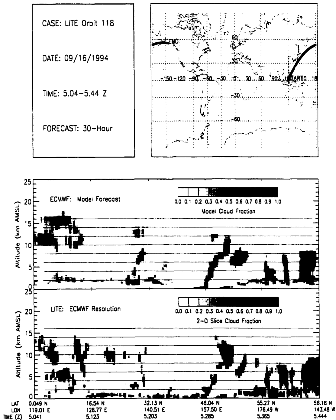
Figure B.89: LITE Orbit 118 Cloud Cover Comparison.
