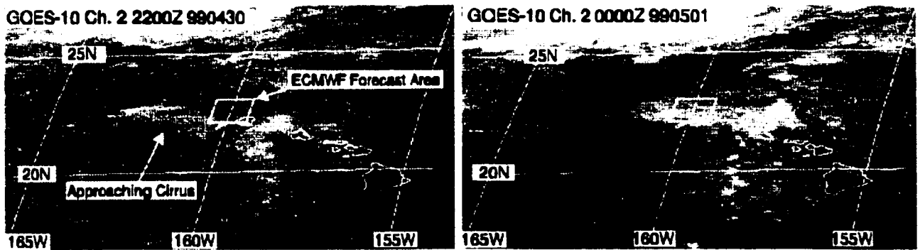
Figure 6.22: GOES-10 Ch. 2 ( 3.9\text{-}\mu\text{m} ) imagery of the Hawaiian archipelago during the ARM-UAV spring flight series 4/30/99 experiment. Two-hour interval imagery reveals an deck of cirrus that advected into the region over 2200-0000Z.
