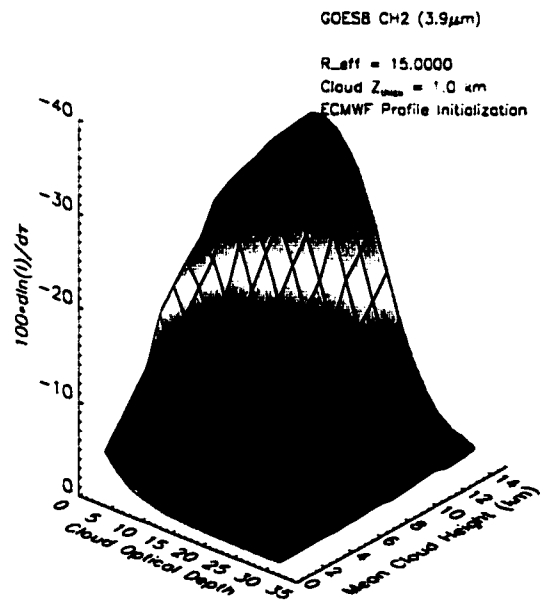
Figure 4.19: GOES Ch. 2 sensitivity to optical property perturbation as a function of cloud height: Nighttime case. Top panel: sensitivity to r_{\text{eff}} , Bottom Panel: sensitivity to \tau .
