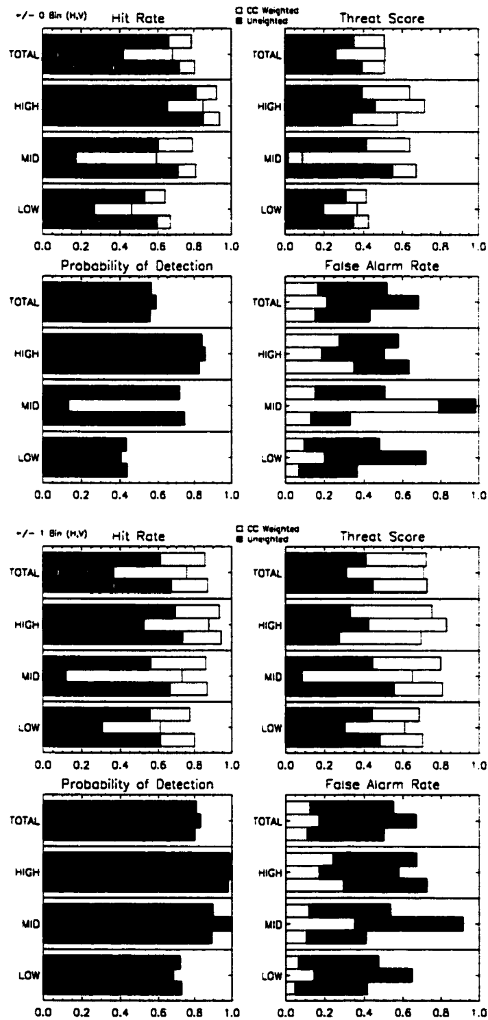
Figure B.14: LITE Orbit 023 Cloud Cover Statistics.
