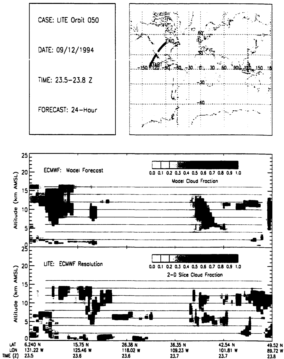
Figure B.37: LITE Orbit 050 Cloud Cover Comparison.
