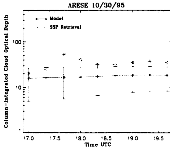
Figure 7.5: Comparison between optical depths derived from SSP measurements and those converted from model cloud water forecasts for ARESE 10/30/95.
