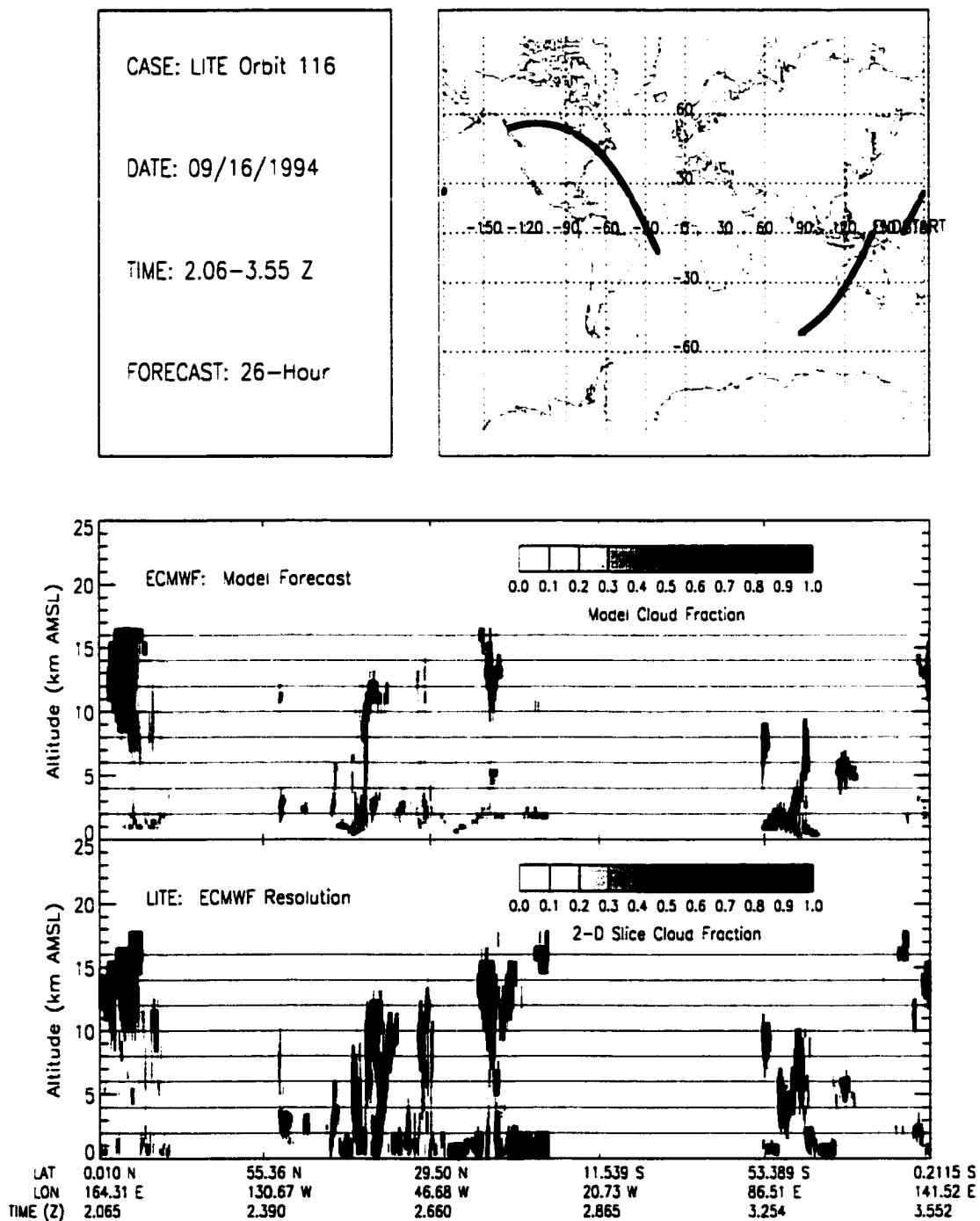
Figure B.87: LITE Orbit 116 Cloud Cover Comparison.
