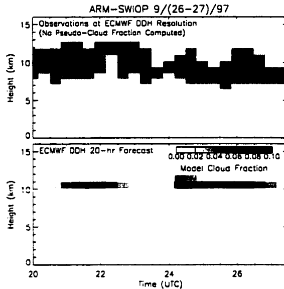
Figure 6.21: Comparison between CDL (rebinned to model resolution) and ECMWF cloud fraction forecast for ARM-SWIOP 9/(26-27)/97.
