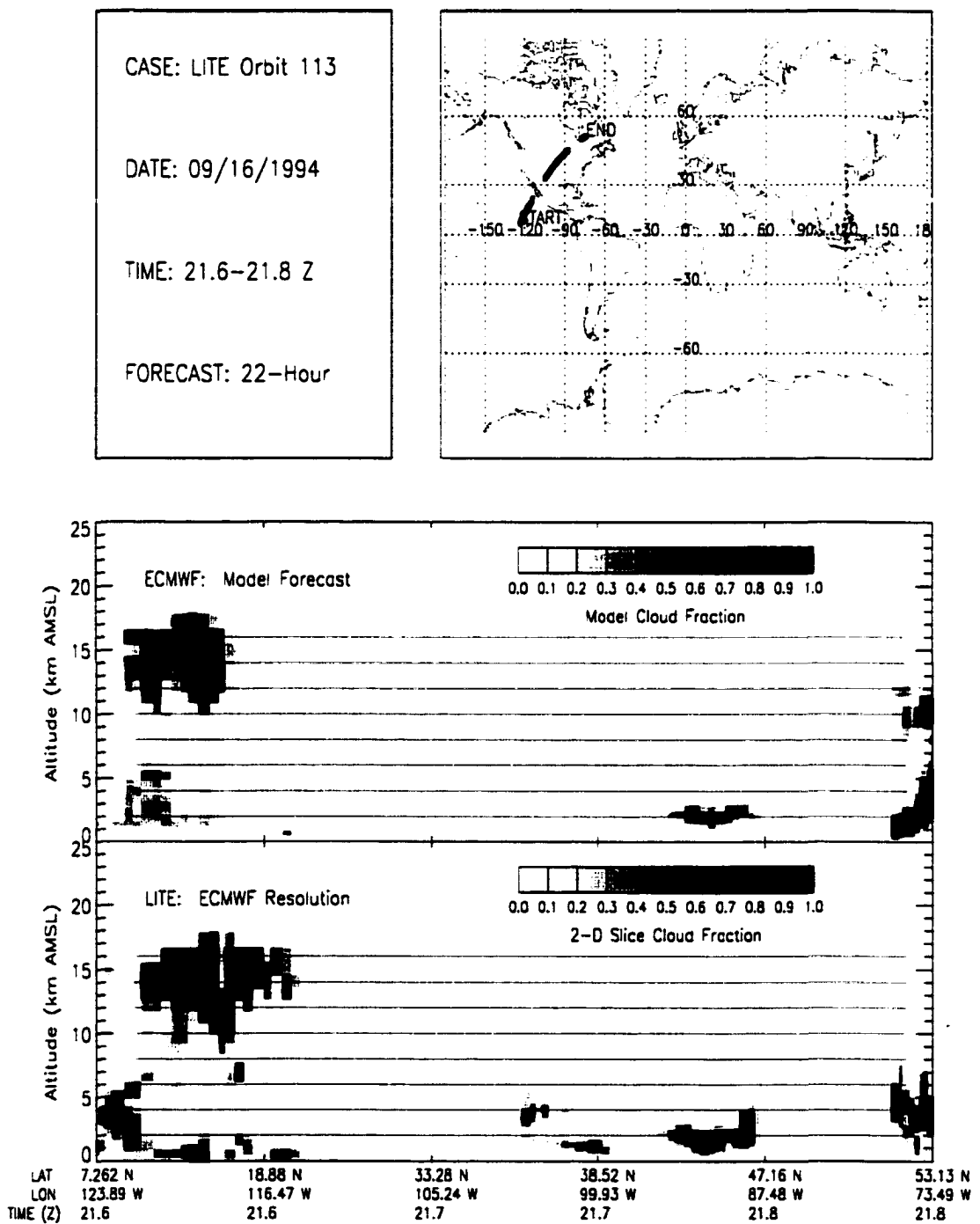
Figure B.83: LITE Orbit 113 Cloud Cover Comparison.
