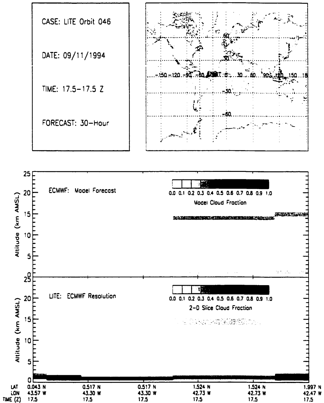
Figure B.31: LITE Orbit 046 Cloud Cover Comparison.
