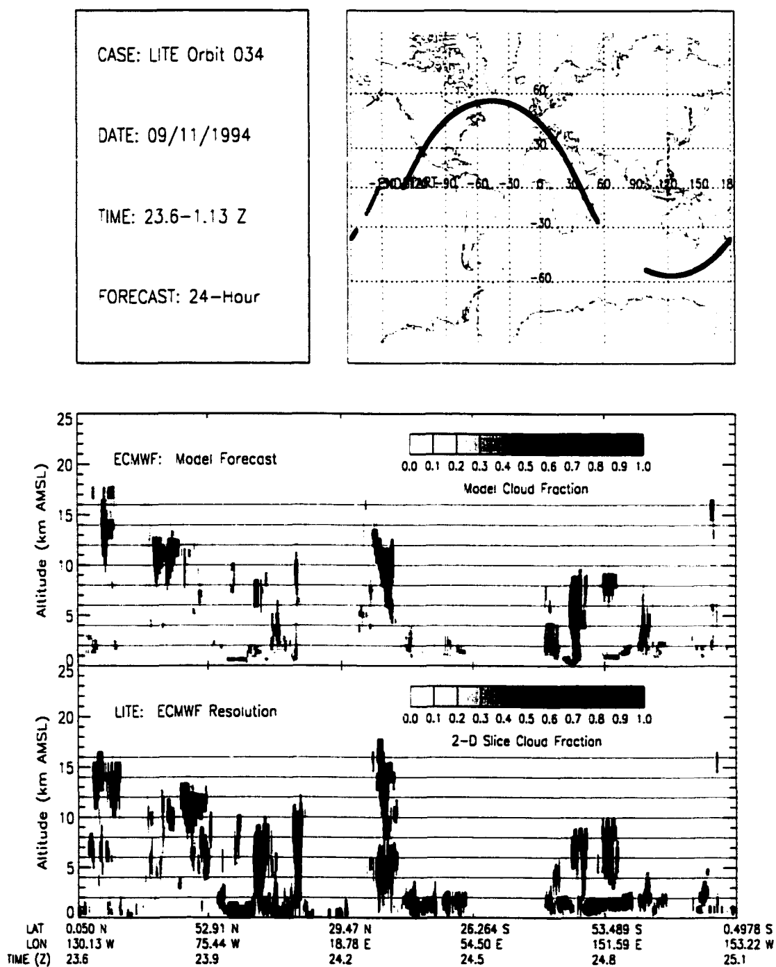
Figure B.23: LITE Orbit 034 Cloud Cover Comparison.
