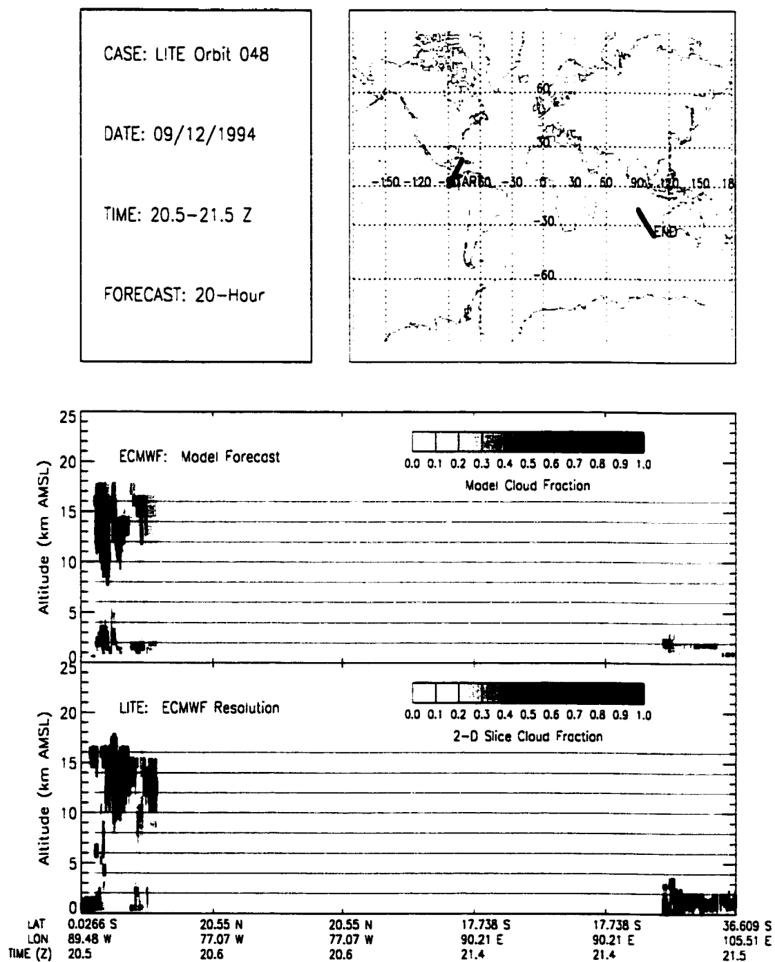
Figure B.35: LITE Orbit 048 Cloud Cover Comparison.
