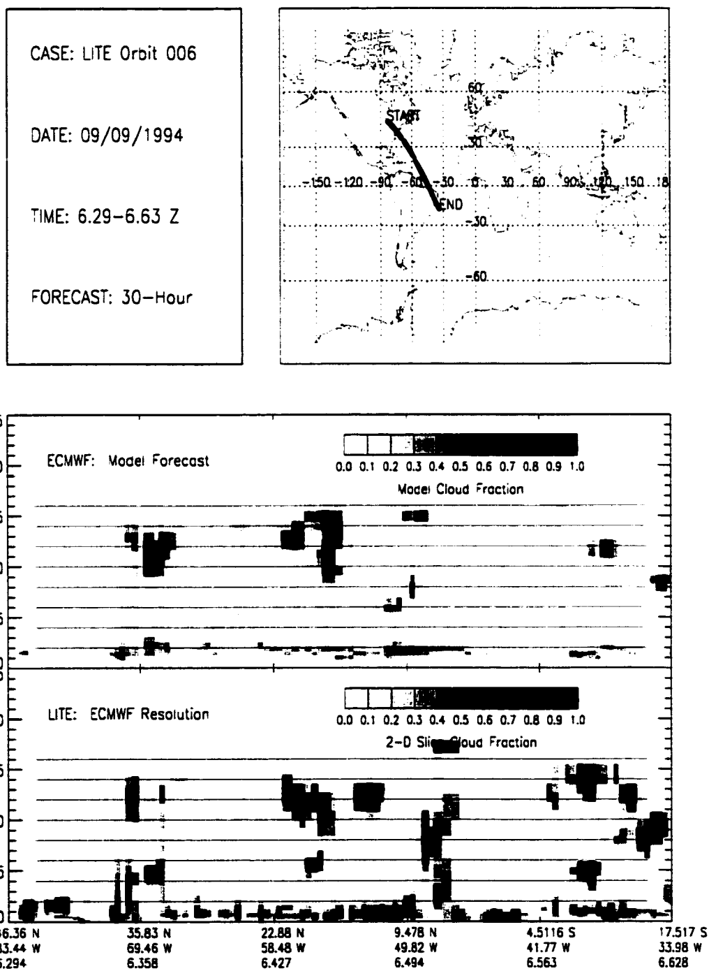
Figure B.3: LITE Orbit 006 Cloud Cover Comparison.
