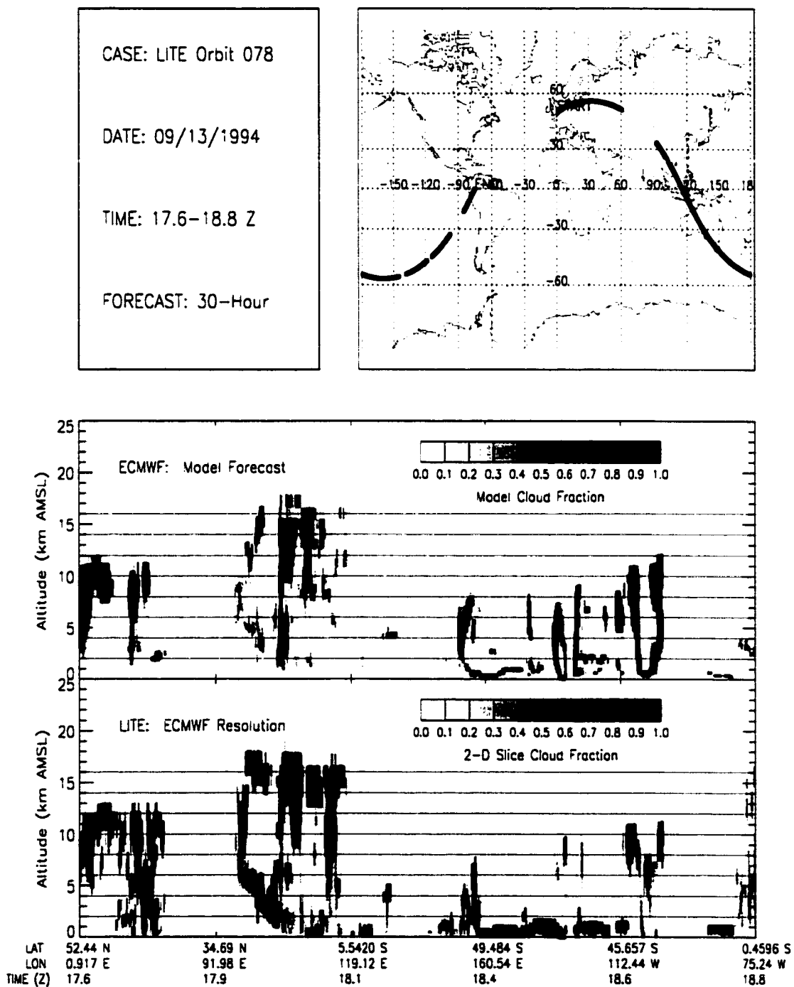
Figure B.59: LITE Orbit 078 Cloud Cover Comparison.
