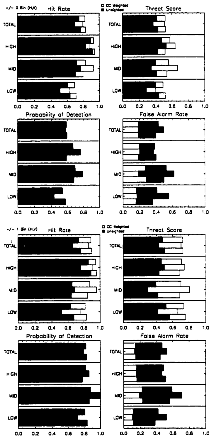
Figure B.62: LITE Orbit 079 Cloud Cover Statistics.
