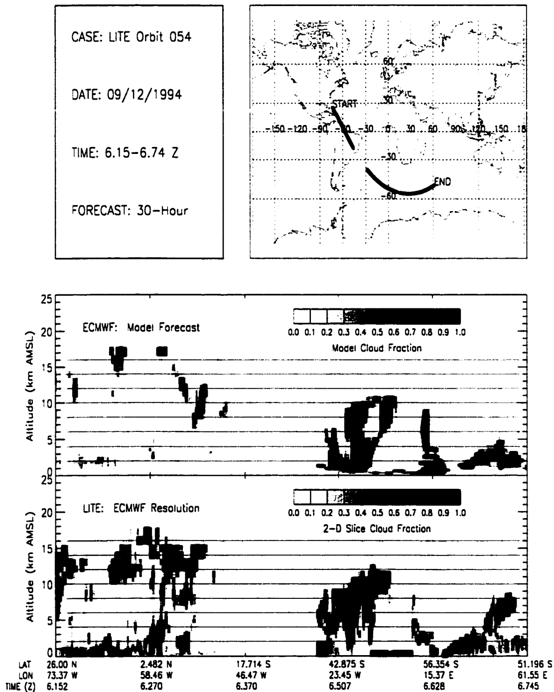
Figure B.41: LITE Orbit 054 Cloud Cover Comparison.
