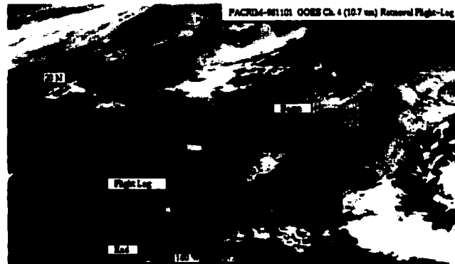
Figure 5.30: GOES-9 observations corresponding to the 11/01/96 PACRIM retrieval.
