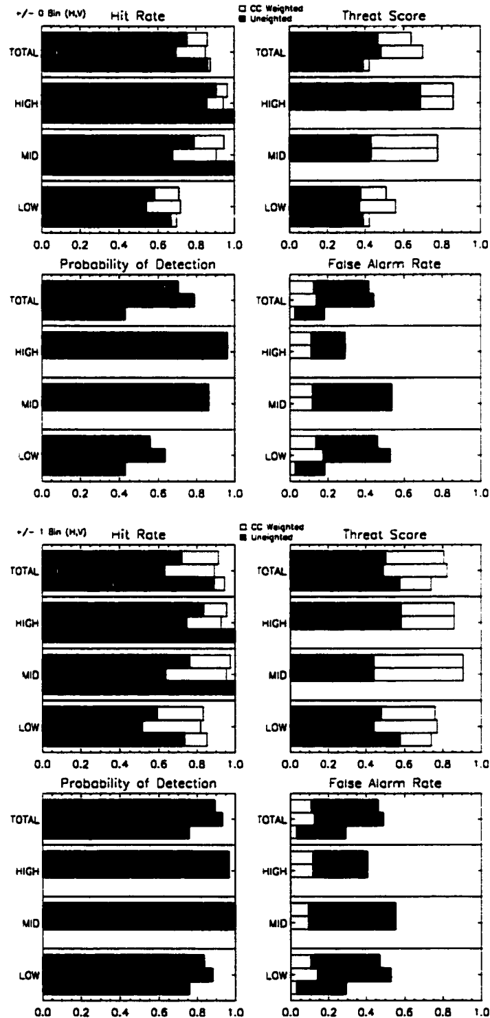
Figure B.36: LITE Orbit 048 Cloud Cover Statistics.
