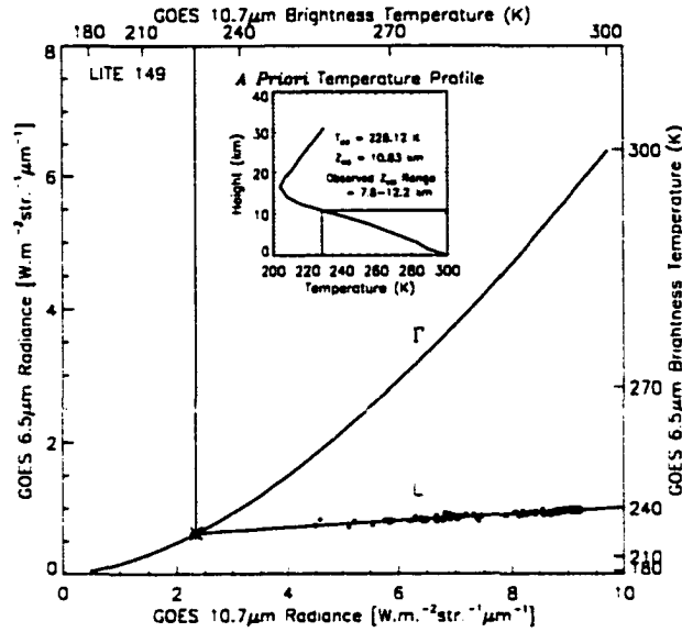
Figure 5.6: Passive sensor estimate of semi-transparent cirrus height for LITE Orbit 149 using GOES 6.5 \mu\text{m} water vapor and 10.7 \mu\text{m} IR window channels. Curve “ \Gamma ” is the theoretical blackbody relationship and line “ L ” is the linear fit to the observation set (following the method of Szejwach, 1982).
