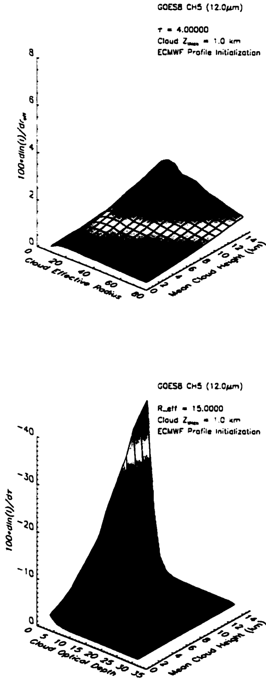
Figure 4.22: GOES Ch. 5 sensitivity to optical property perturbation as a function of cloud height. Top panel: sensitivity to r_{\text{eff}} , Bottom Panel: sensitivity to \tau .
