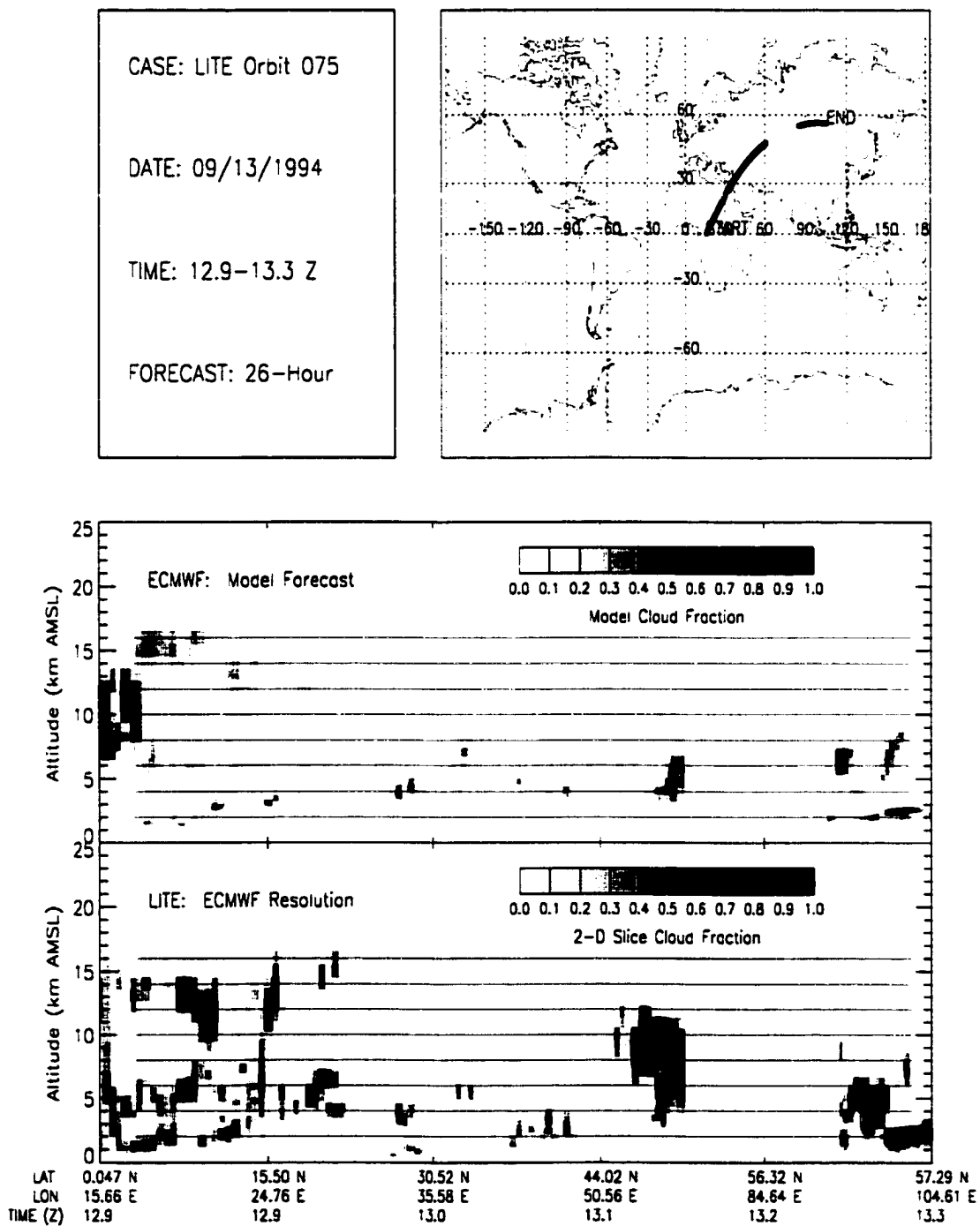
Figure B.57: LITE Orbit 075 Cloud Cover Comparison.
