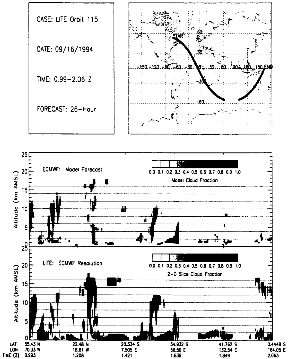
Figure B.85: LITE Orbit 115 Cloud Cover Comparison.
