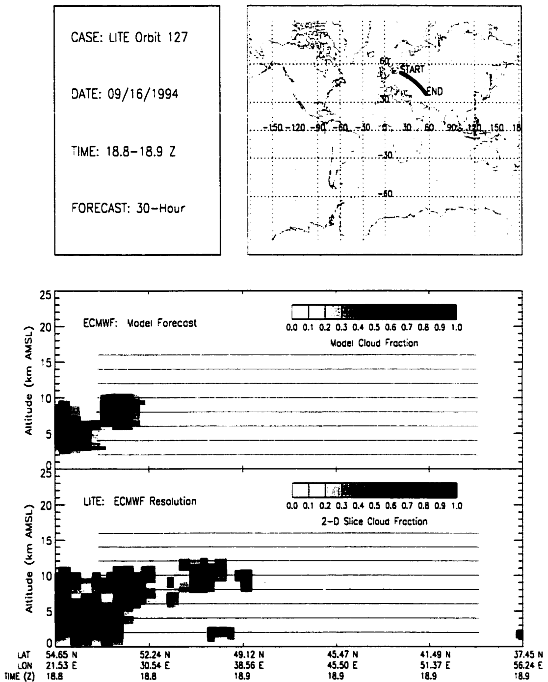
Figure B.101: LITE Orbit 127 Cloud Cover Comparison.
