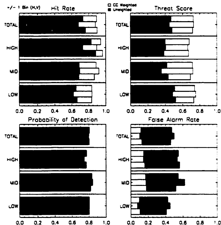
Figure 6.10: Ensemble-orbit statistics as defined in 6.9 for the ECMWF/LITE comparisons (Shown: \pm 1 bin H/V). Statistics are decomposed into Total-column, Low (0-4 km), Middle (4-8 km), and High (> 8 km) cloudiness for Tropics and Extra-Tropics.
