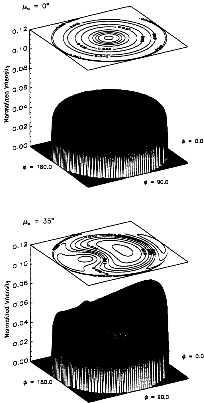
Figure 2.3: Upwelling intensity field with azimuthal structure modeled for a single cloud layer. Top panel: DHG phase function, \tau = 1.0 , g_1 = 0.85 , g_2 = -0.6 , g_{\text{eff}} = 0.70 , \omega_o = 1.0 , and \theta_o = 0^\circ only (equivalent to azimuthally averaged m = 0 structure). Lower panel: same optical properties as above azimuthal expansion m = 16 , \theta_o = 35^\circ .
