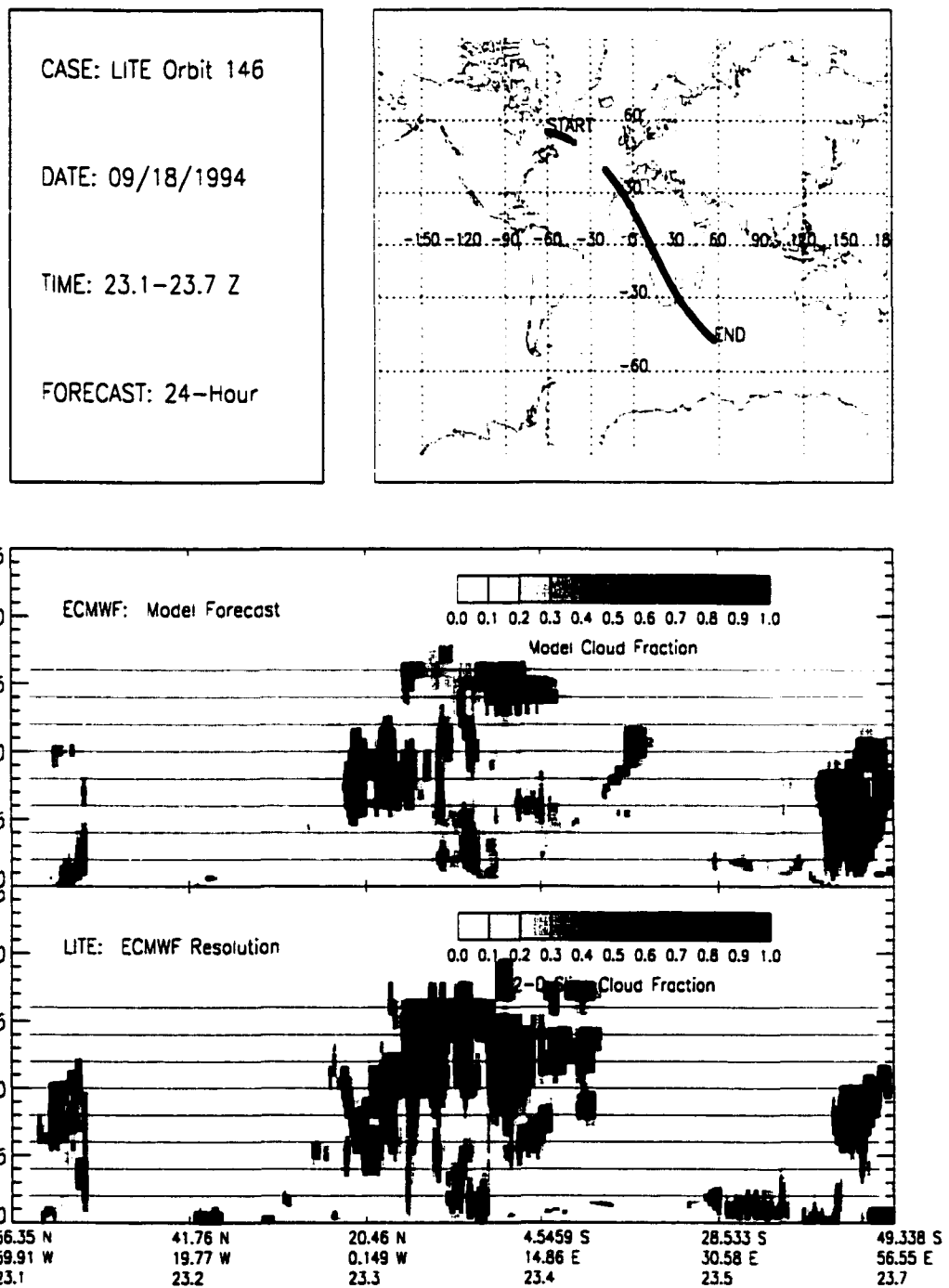
Figure B.121: LITE Orbit 146 Cloud Cover Comparison.
