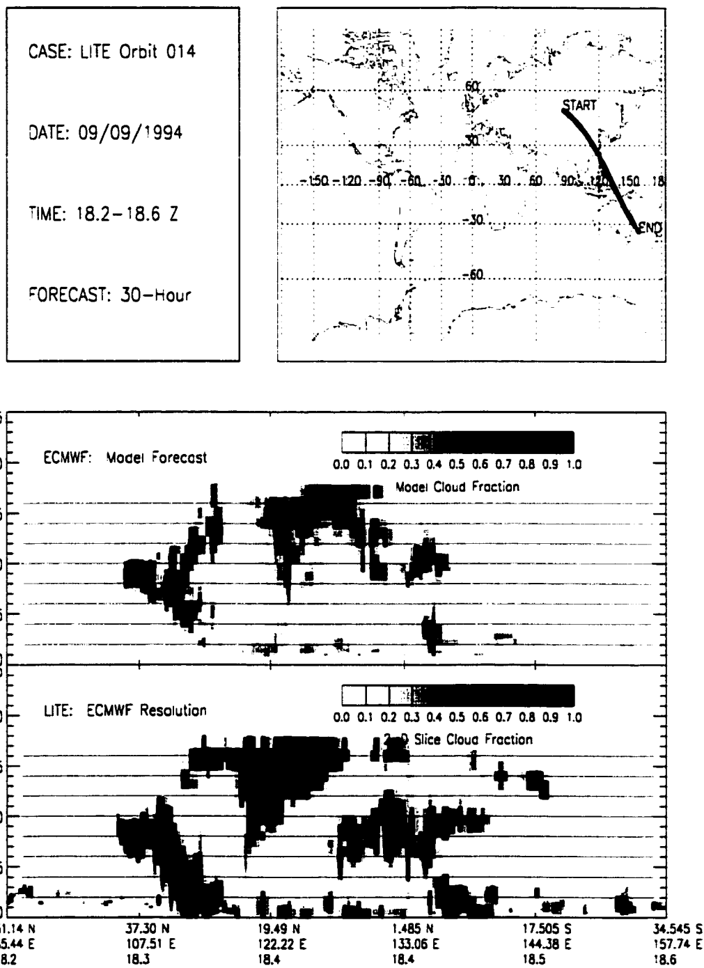
Figure B.7: LITE Orbit 014 Cloud Cover Comparison.
