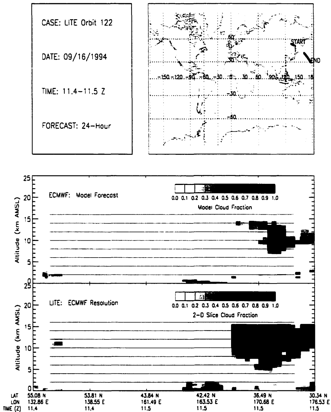
Figure B.93: LITE Orbit 122 Cloud Cover Comparison.
