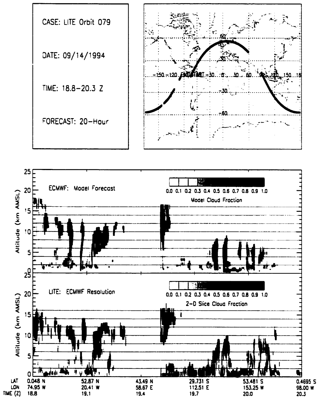
Figure B.61: LITE Orbit 079 Cloud Cover Comparison.
