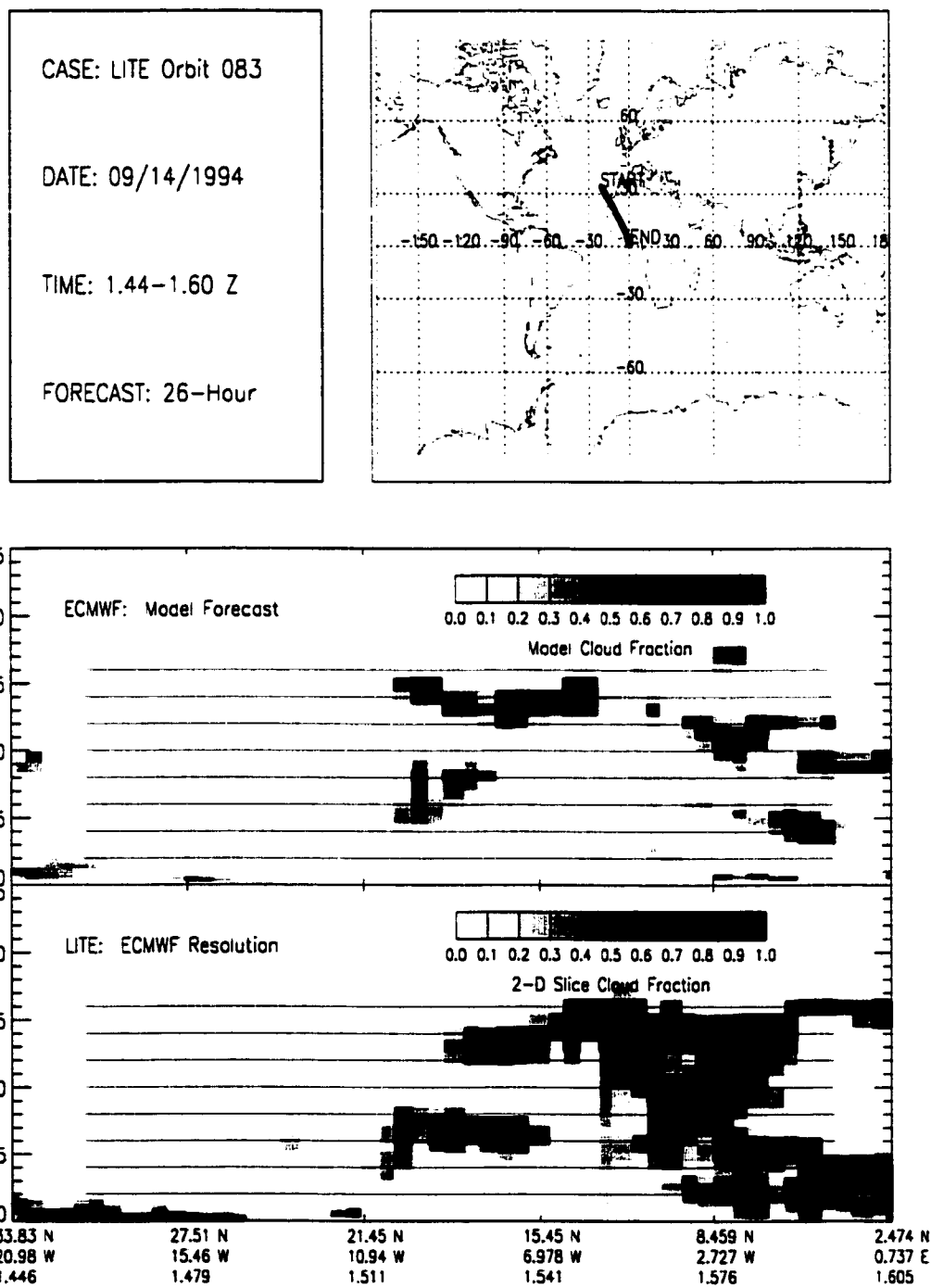
Figure B.69: LITE Orbit 083 Cloud Cover Comparison.
