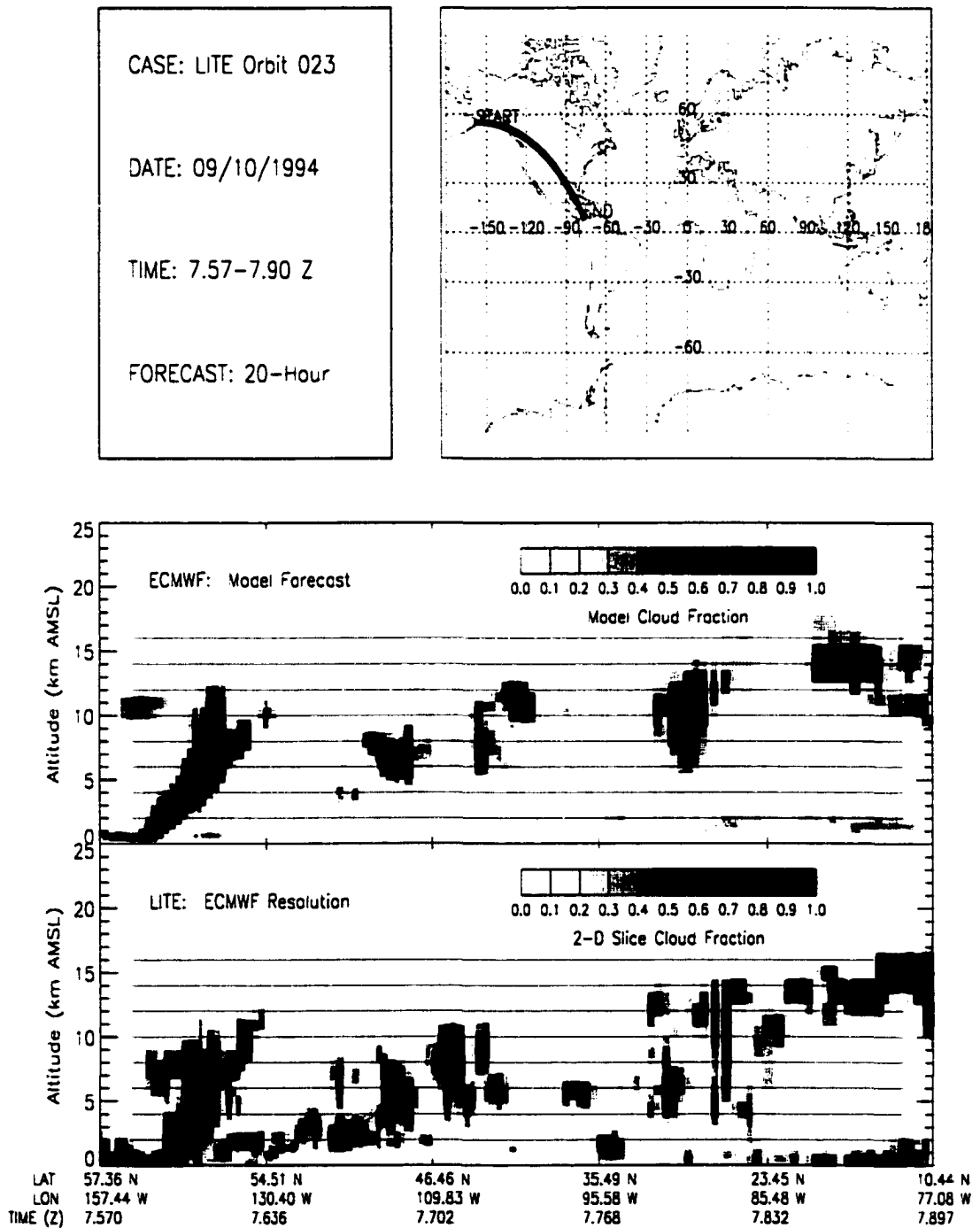
Figure B.13: LITE Orbit 023 Cloud Cover Comparison.
