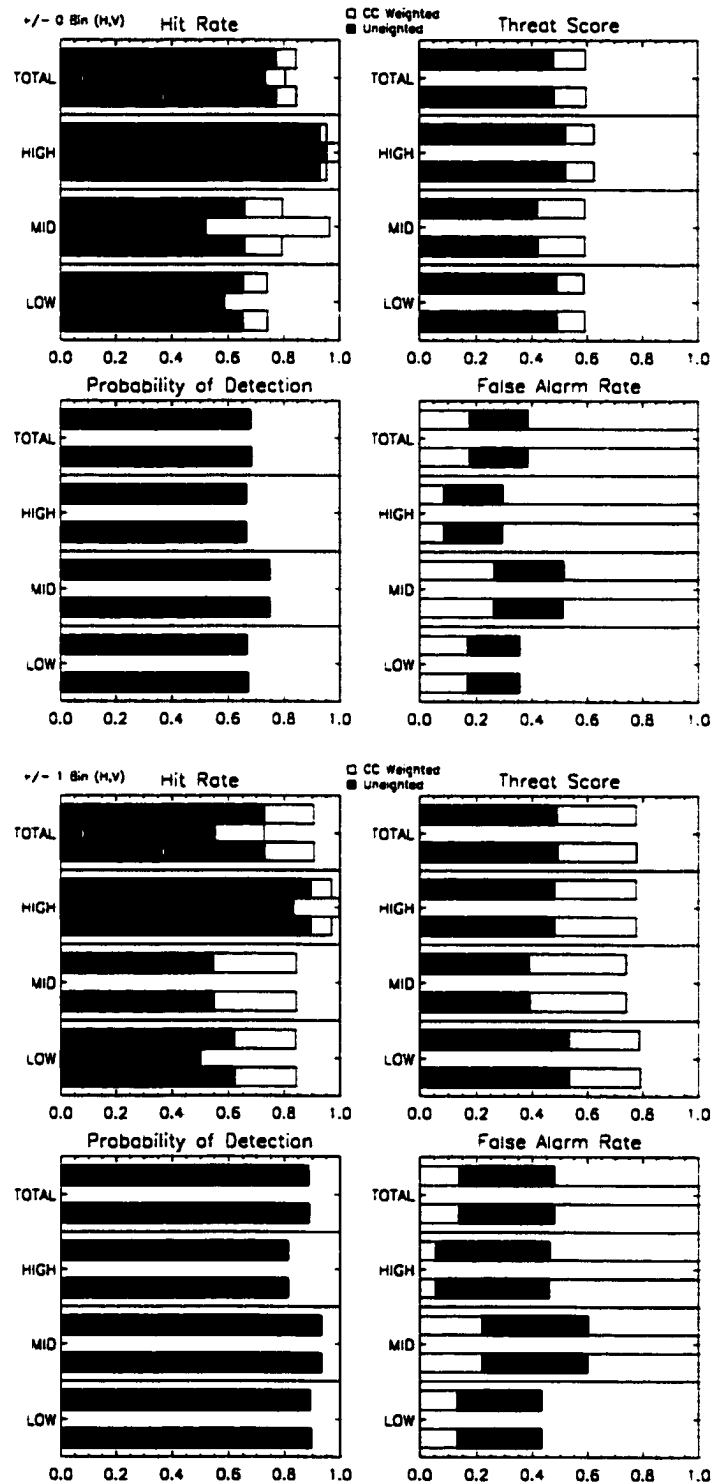
Figure B.44: LITE Orbit 055 Cloud Cover Statistics.
