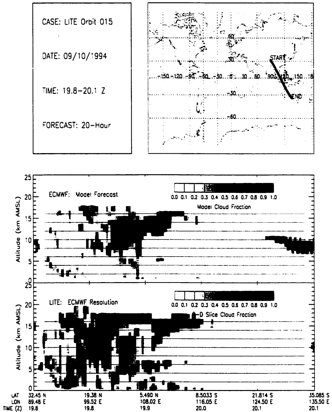
Figure B.9: LITE Orbit 015 Cloud Cover Comparison.
