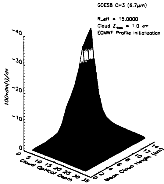
Figure 4.20: GOES Ch. 3 sensitivity to optical property perturbation as a function of cloud height. Top panel: sensitivity to r_{\text{eff}} , Bottom Panel: sensitivity to \tau .
