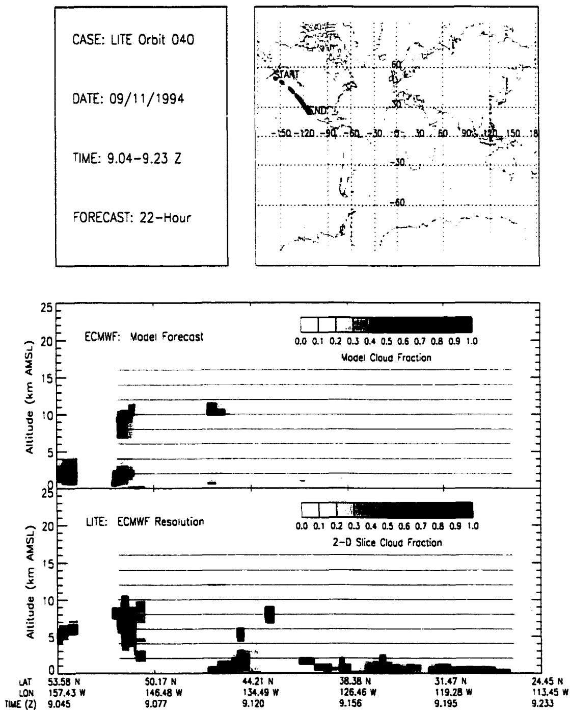
Figure B.27: LITE Orbit 040 Cloud Cover Comparison.
