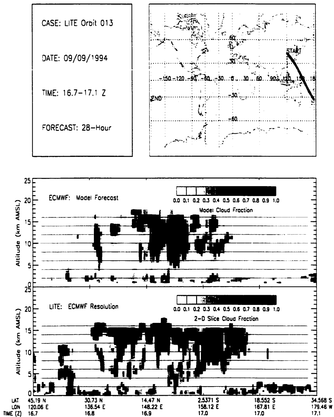
Figure B.5: LITE Orbit 013 Cloud Cover Comparison.
