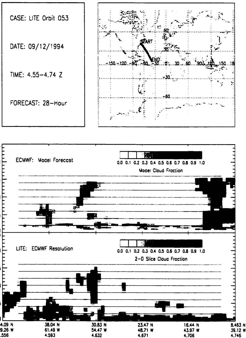
Figure B.39: LITE Orbit 053 Cloud Cover Comparison.
