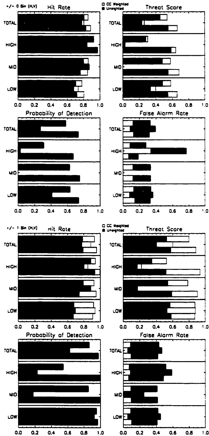
Figure B.66: LITE Orbit 081 Cloud Cover Statistics.
