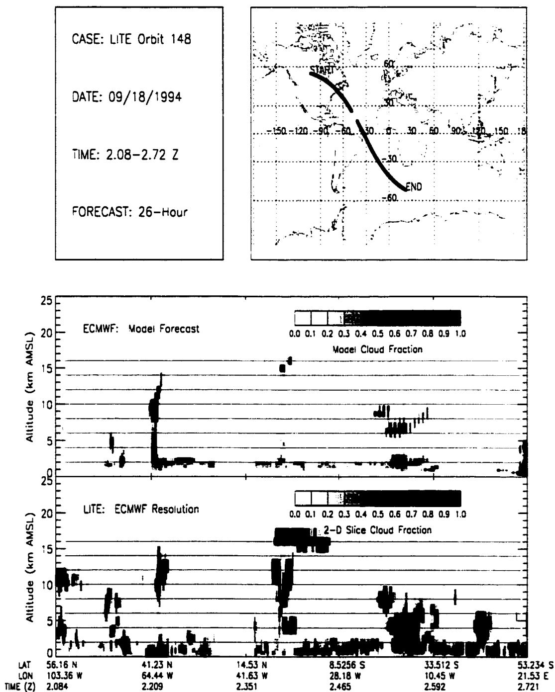
Figure B.125: LITE Orbit 148 Cloud Cover Comparison.
