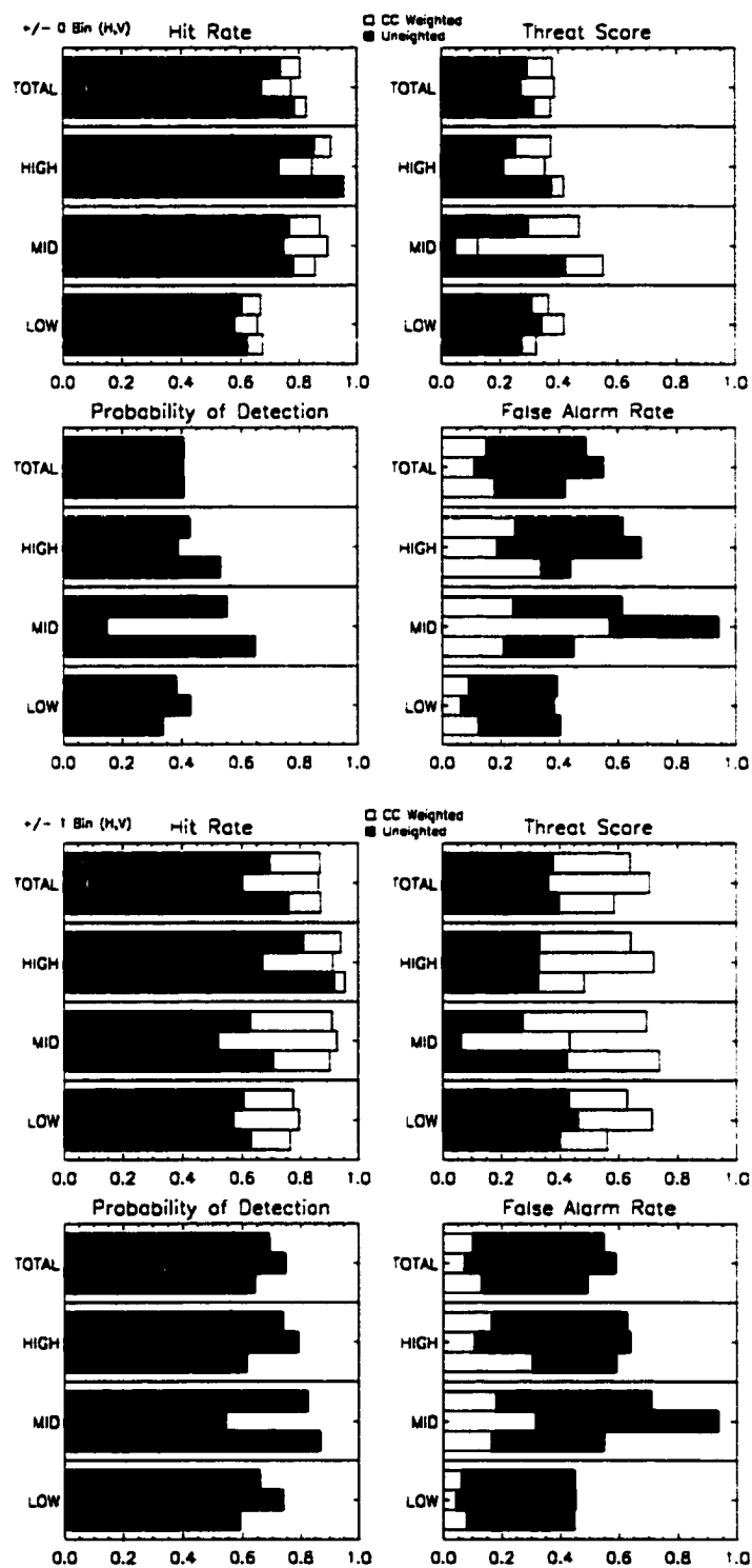
Figure B.12: LITE Orbit 022 Cloud Cover Statistics.
