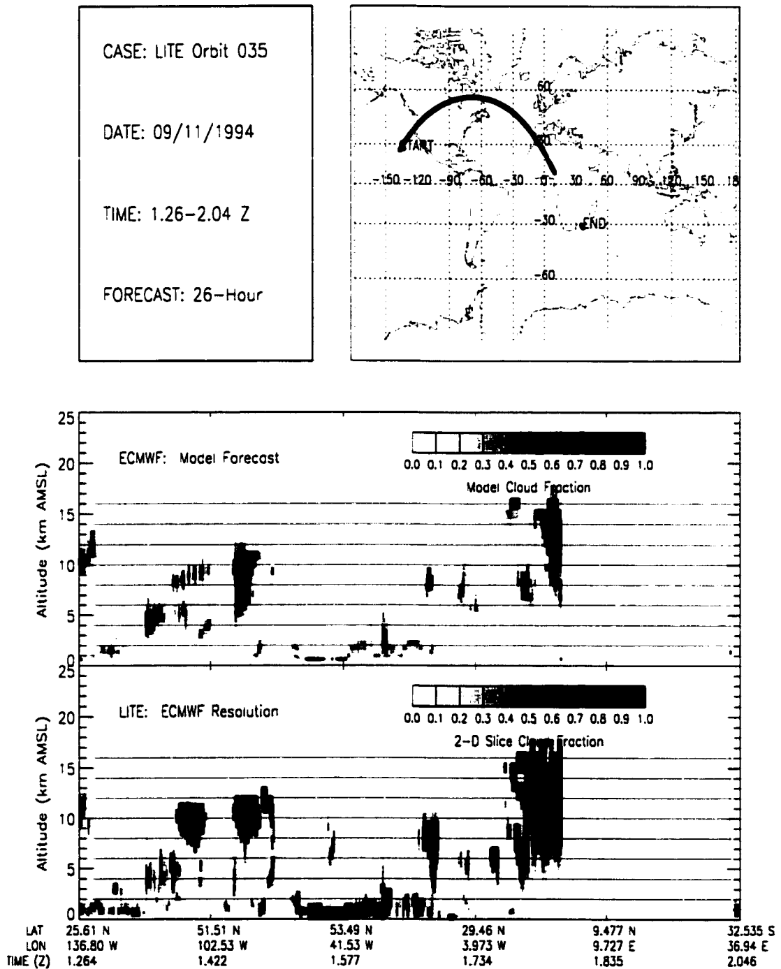
Figure B.25: LITE Orbit 035 Cloud Cover Comparison.
