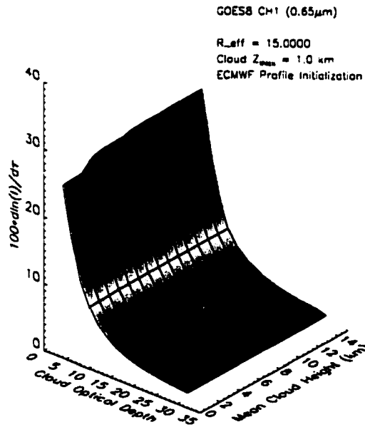
Figure 4.17: GOES Ch. 1 sensitivity to optical property perturbation as a function of cloud height. Top panel: sensitivity to r_{\text{eff}} , Bottom Panel: sensitivity to \tau .
