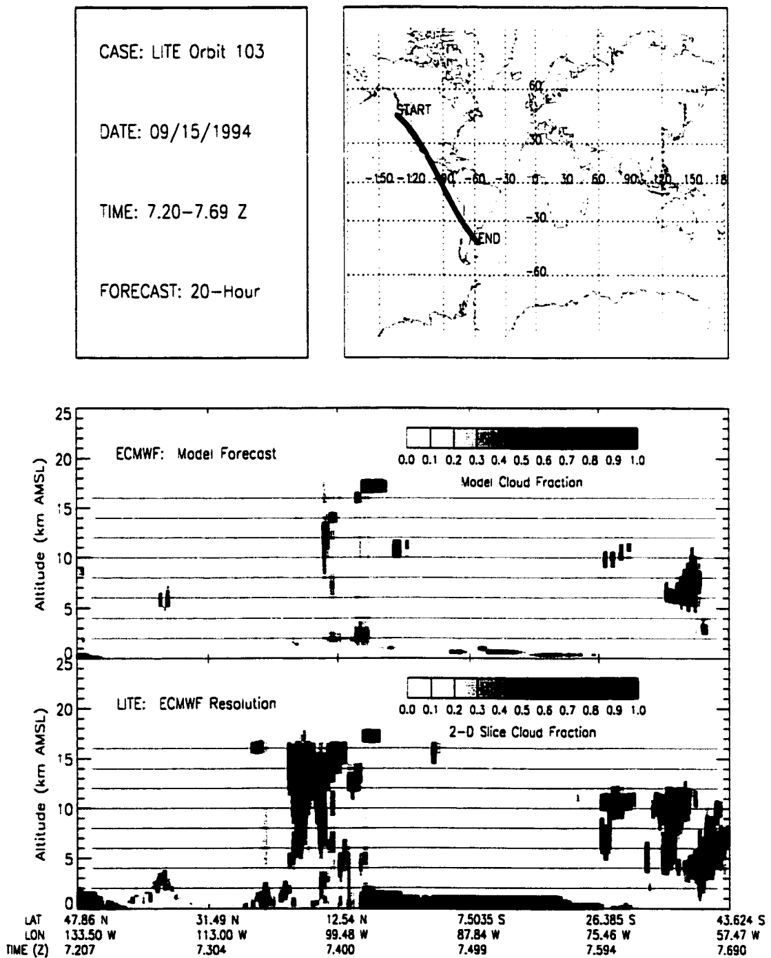
Figure B.77: LITE Orbit 103 Cloud Cover Comparison.
