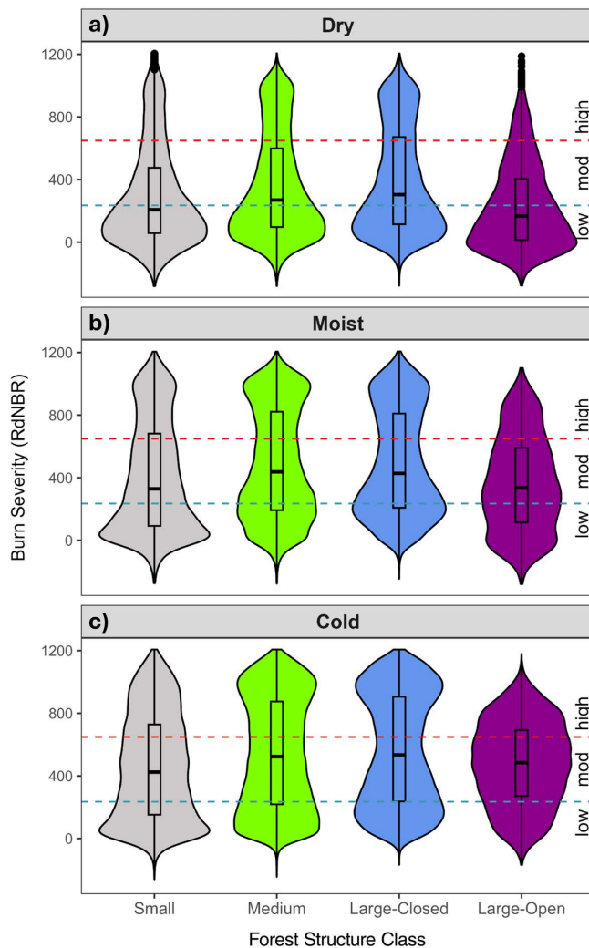
FIGURE 3 Observed burn severity across forest structure classes and forest types in the Schneider Springs Fire. The horizontal dashed lines correspond to thresholds between severity classes. See Figure 4 for predicted severity while accounting for primary fire drivers. See Appendix S1: Figure S2 for old-growth structural index and lidar-based northern spotted owl habitat suitability. Low-, moderate-, and high-severity classes correspond to basal area mortality values of <25%, 25%–75%, and >75%, and Relative differenced Normalized Burn Ratio (RdNBR) values of <235, 235–649, and >649, respectively, based on a regionally derived regression model (Reilly et al., 2017).
