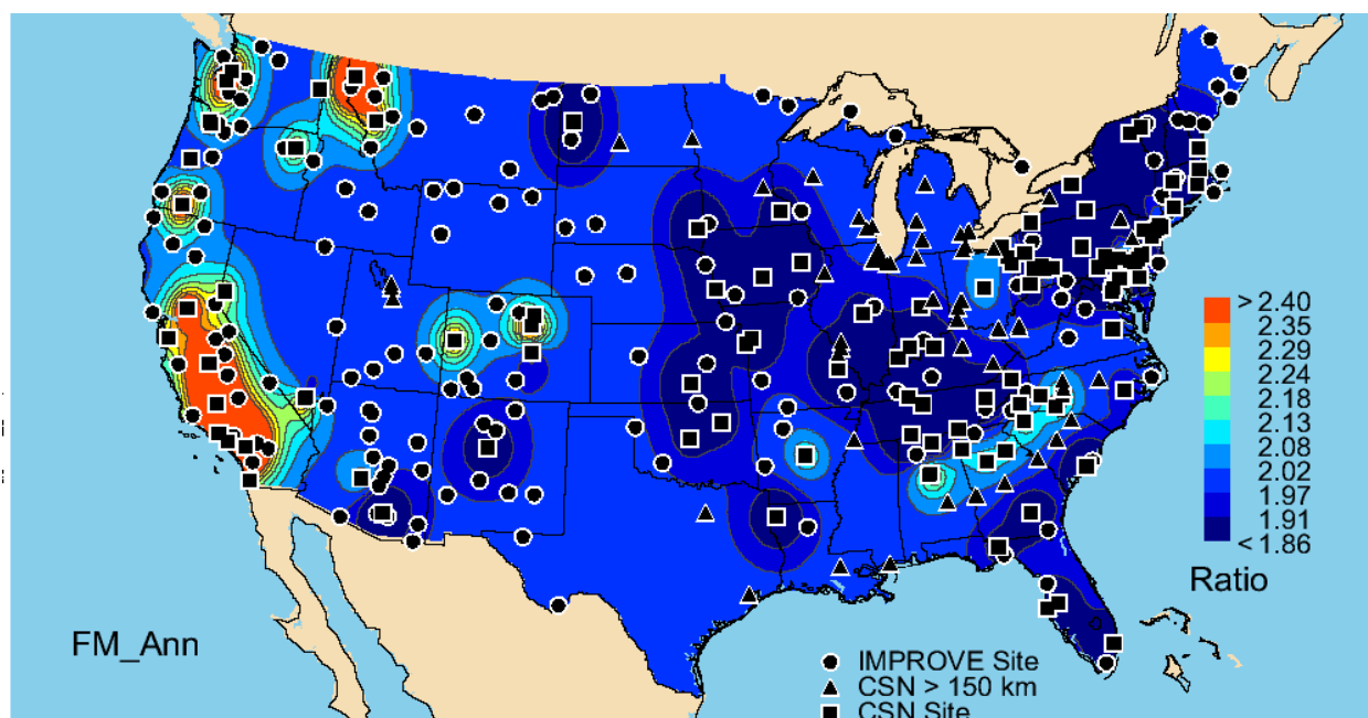
Figure 7.6.3. Interpolated ratios of urban (CSN) to rural (IMPROVE) annual mean PM 2.5 gravimetric fine mass (FM) concentrations for 2005–2008. IMPROVE sites are shown as circles, CSN sites with an IMPROVE monitor within 150 km are depicted as squares, and CSN sites not used in the analyses are shown as triangles.
