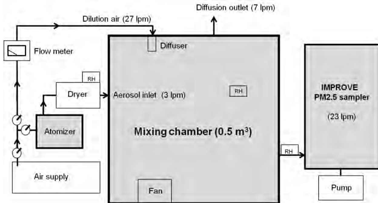
Figure 10.1. Schematic of the particle generation, mixing, and sampling system used to make reference materials. A solution is atomized and the resulting particles are dried and mixed with clean, dry air in the mixing chamber. The suspended particles are drawn through an IMPROVE PM 2.5 sampler and collected on 25 mm Teflon® filters. Relative humidity (RH) is measured in three locations to ensure that particles are anhydrous.
