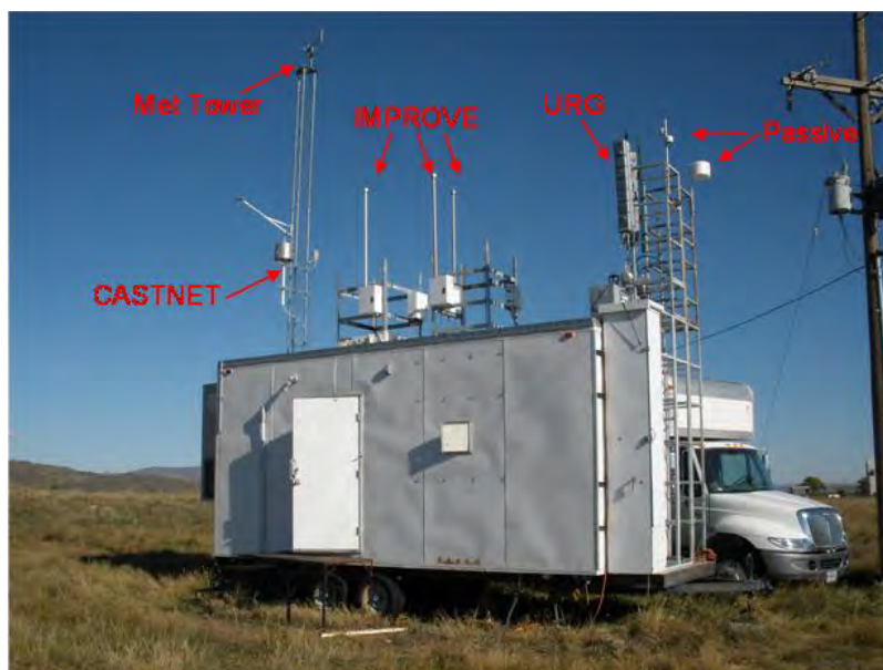
Figure 11.1. Study trailer showing aerosol sampling equipment. The CASTNET, Met tower, IMPROVE, URG, and passive samplers are shown from left to right.
