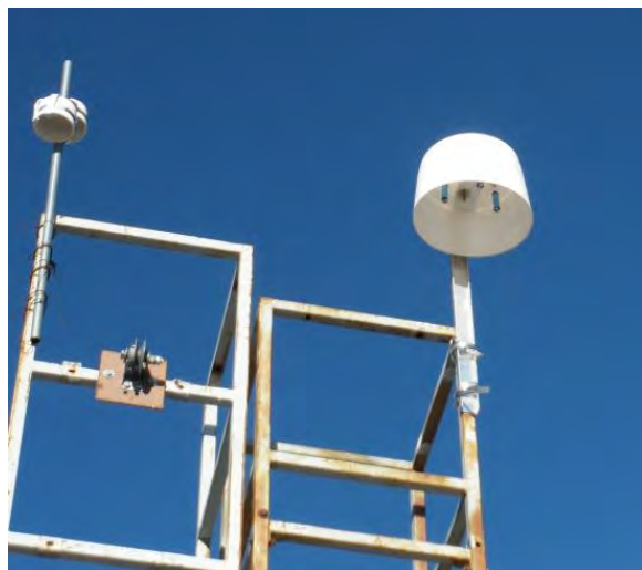
Figure 11.7. Passive samplers deployed in the field. The Ogawa sampler is on the left, and the Radiello sampler is on the right.
