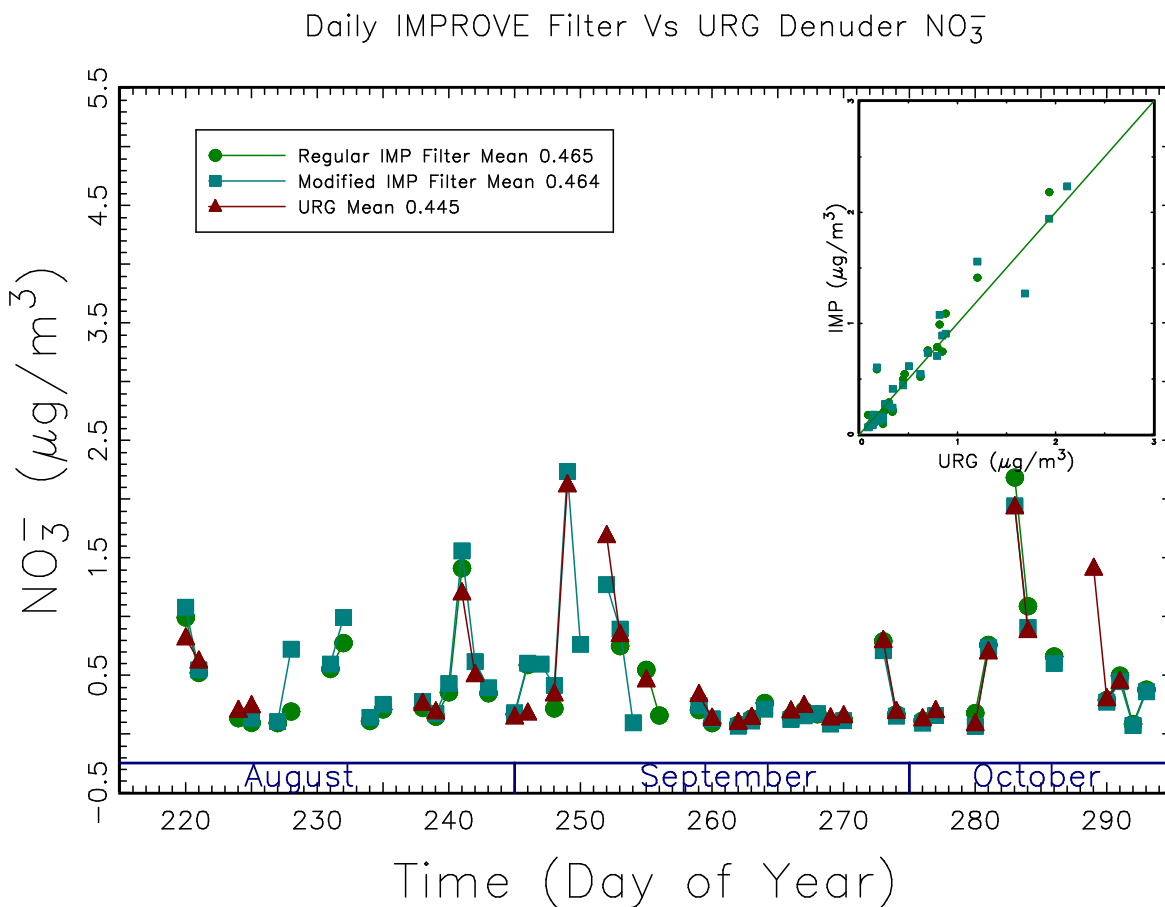
Figure 11.9. Comparisons of nitrate ion ( \text{NO}_3^- ) concentrations from the regular IMPROVE (RegIMP), modified IMPROVE (ModIMP), and URG samplers during fall 2008. Mean nitrate ion concentrations ( \mu\text{g m}^{-3} ) for each sampler are reported.
