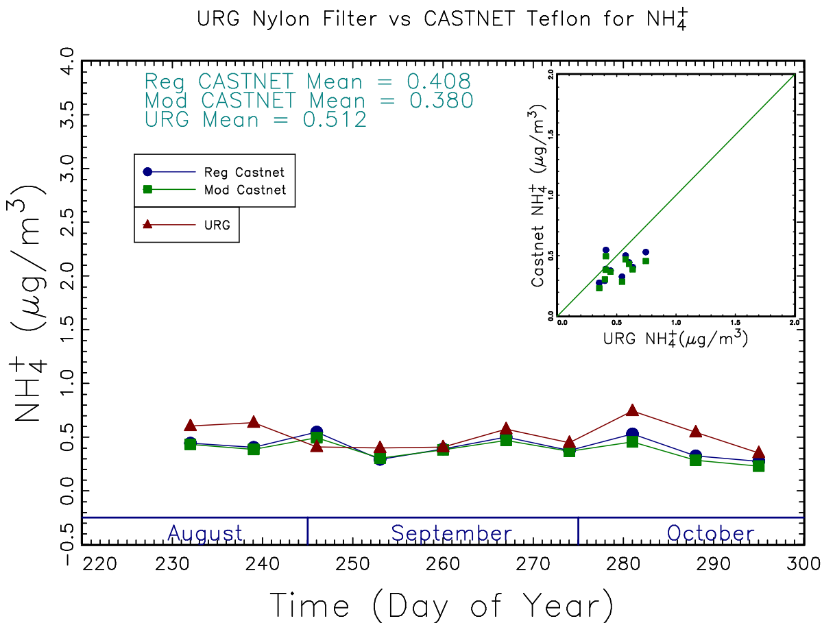
Figure 11.18. Comparisons of ammonium ion ( \text{NH}_4^+ ) concentrations from the modified CASTNET (Mod CASTNET), regular CASTNET (Reg CASTNET), and URG samplers during fall 2008. Ammonium concentrations ( \mu\text{g m}^{-3} ) for each sampler are reported.
