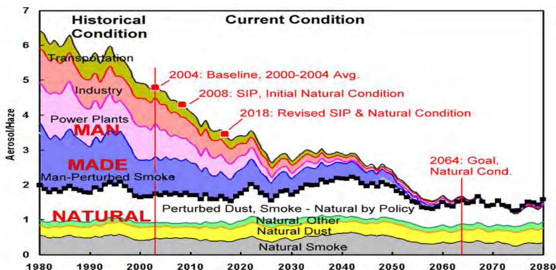
Figure 9.2.2. Depiction of realistic uniform rate of progress (URG) glide path (Husar, 2003).
