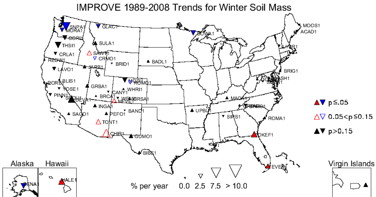
Figure 6.4.3. Long-term (1989–2008) trends (% yr -1 ) in average winter fine soil mass concentrations.
