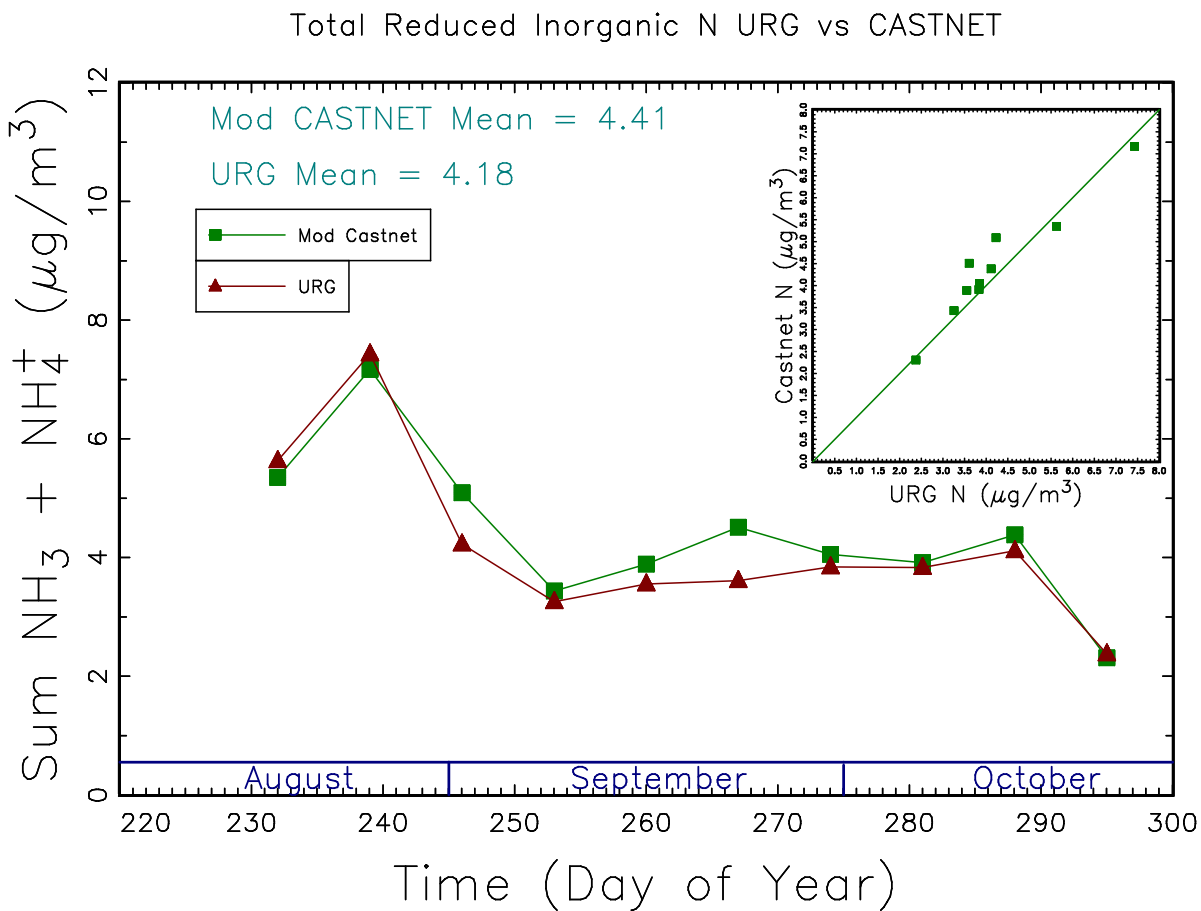
Figure 11.20. Comparisons of total reduced inorganic nitrogen ( \text{NH}_x = \text{NH}_3 + \text{NH}_4^+ ) concentrations from the modified CASTNET (Mod CASTNET) and URG samplers for 2008. \text{NH}_x ( \mu\text{g m}^{-3} ) for each sampler are reported.
