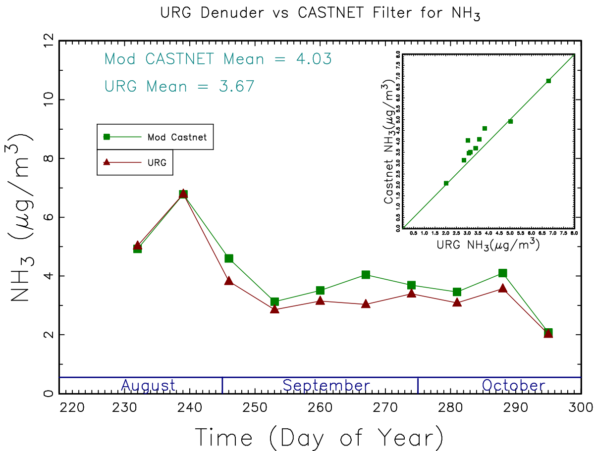
Figure 11.19. Comparisons of ammonia ( \text{NH}_3 ) concentrations from the modified CASTNET (Mod CASTNET), and URG samplers during fall 2008. Ammonia concentrations ( \mu\text{g m}^{-3} ) for each sampler are reported.
