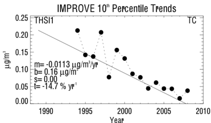
Figure 6.3.2. 10 th percentile total carbon (TC = organic carbon + light absorbing carbon) mass concentrations (µg m -3 ) for Three Sisters, Oregon (THSI1). Regression results, including Theil slope (m, µg m -3 yr -1 ), intercept (b, µg m -3 ), significance (s), and trend (t, % yr -1 ) are included. The trend line is plotted as a solid line. The intercept corresponds to the initial year of data.
