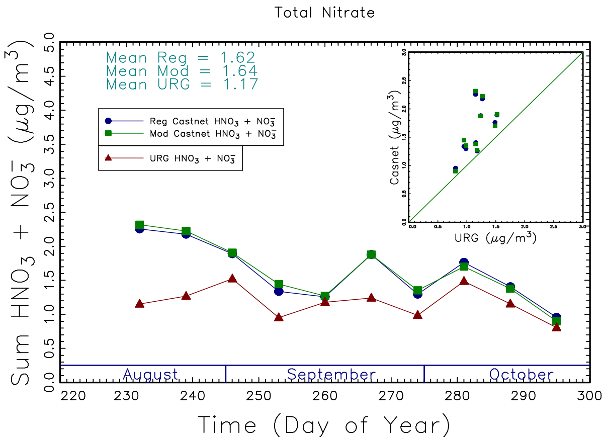
Figure 11.17. Comparisons of total oxidized nitrogen concentrations ( \text{NO}_3^- + \text{HNO}_3 ) from the modified CASTNET (Mod CASTNET), regular CASTNET (Reg CASTNET), and URG samplers during fall 2008. Total oxidized nitrogen concentrations ( \mu\text{g m}^{-3} ) for each sampler are reported.
