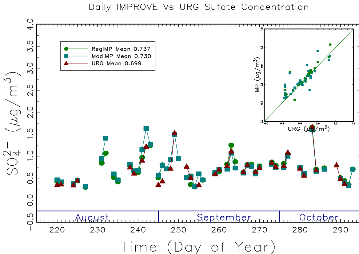
Figure 11.8. Comparisons of sulfate ion ( \text{SO}_4^{2-} ) concentrations from the regular IMPROVE (RegIMP), modified IMPROVE (ModIMP), and URG samplers during fall 2008. Mean sulfate ion concentrations ( \mu\text{g m}^{-3} ) for each sampler are reported.
