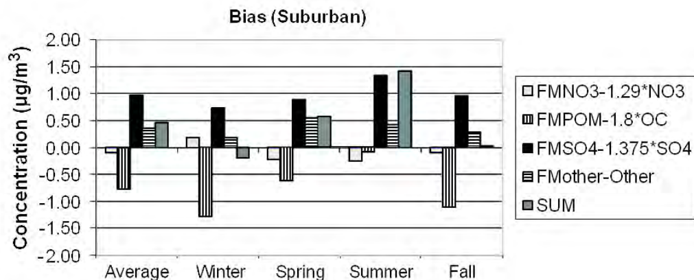
Figure 8.13. The estimated average difference between gravimetric and assumed forms of the various aerosol species contributing to PM_{2.5} for CSN suburban. The differences are estimated as 1.375*SO_4(a_1 - 1) , 1.29*NO_3(a_2 - 1) , OC*(a_3 - 1.8) , and Other*(a_4 - 1) for sulfates, nitrates, organics, and Other, respectively.
