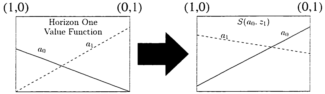
Figure 5.6: The value function can be transformed to give the value for the new belief state b' when taking action a_0 and observing z_1 from any initial belief state.
