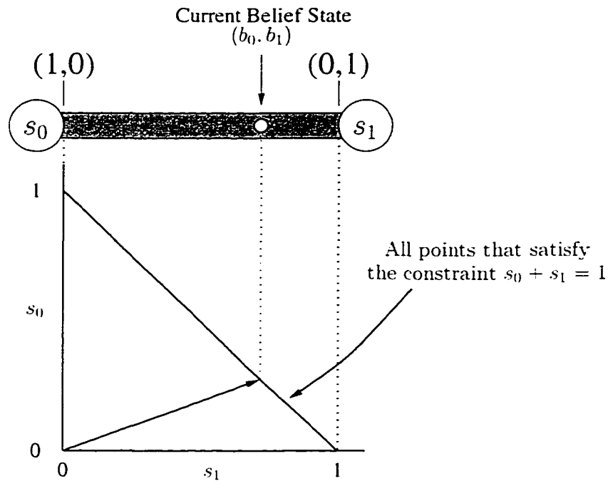
Figure 5.1: A graphical representation of belief state showing how the belief state for a two-state POMDP problem can be represented as a point on a line segment or as a dot in a bar connecting the two states.
