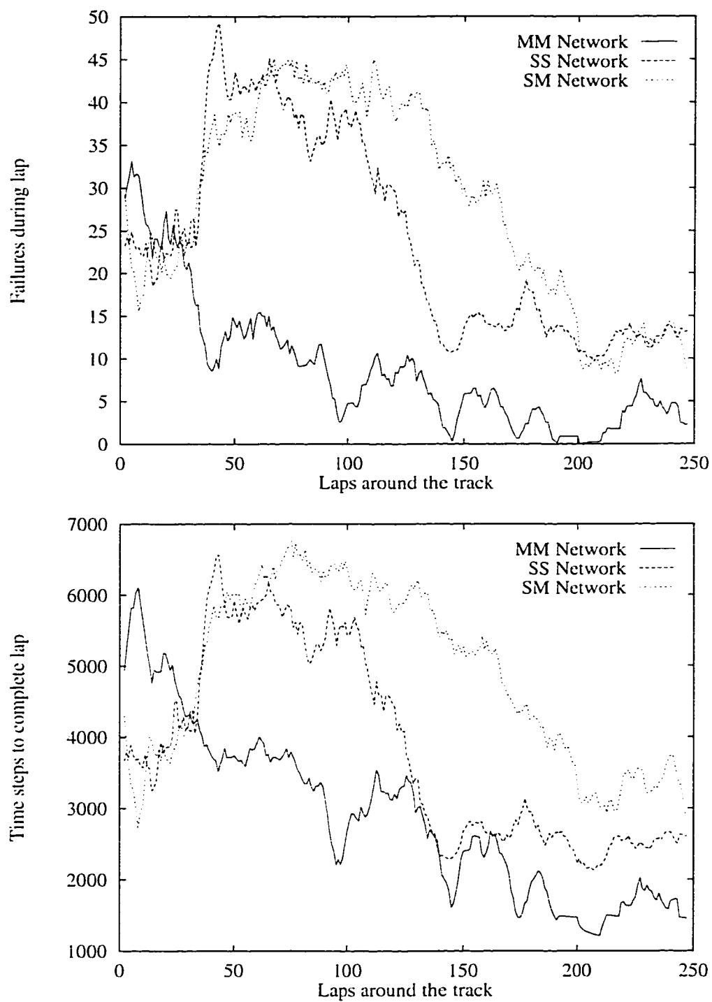
Figure 4.3: Comparison of three reinforcement learning networks to implement the race behavior.
