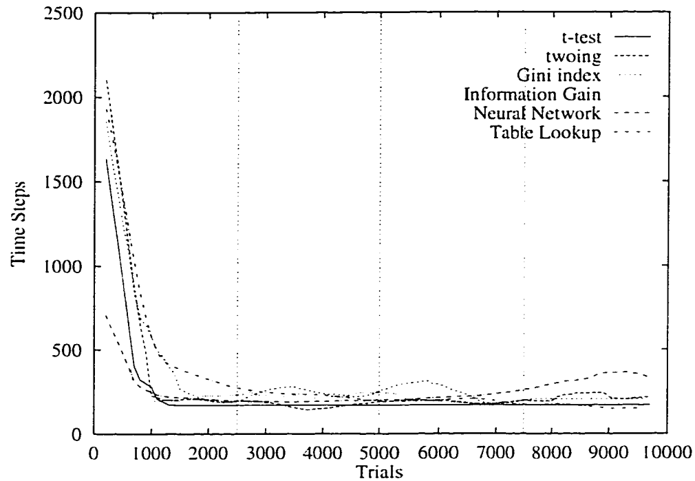
Figure 4.8: Smoothed learning performance on the mountain car problem.
