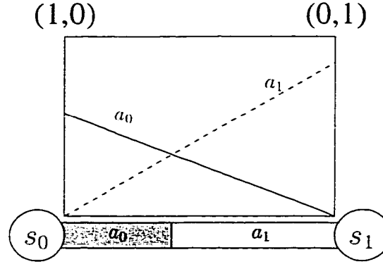
Figure 5.5: Value function at horizon one.
