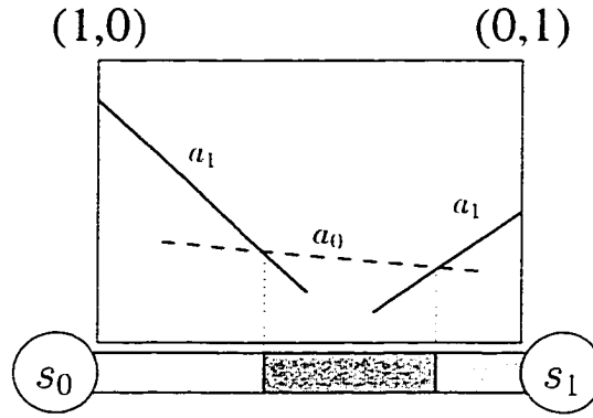
Figure 5.4: How the value function partitions belief space.
