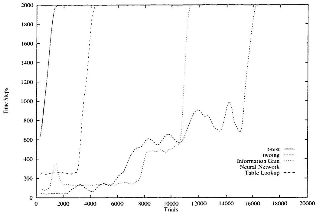
Figure 4.9: Smoothed learning performance on the pole balance problem. Gini index did not converge for this problem and is omitted from the graph.
