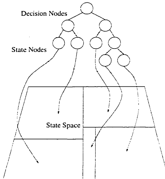
Figure 4.6: Dividing the state space with a decision tree.
