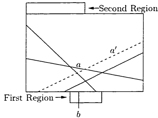
Figure 5.14: Sondik's second region.
