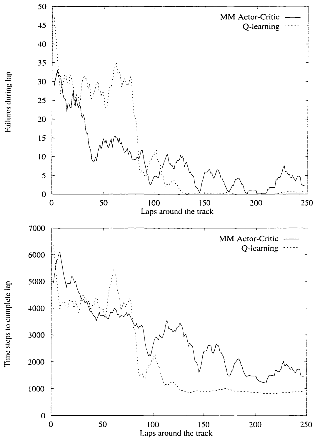
Figure 4.4: Learning performance for the improved learning strategy.
