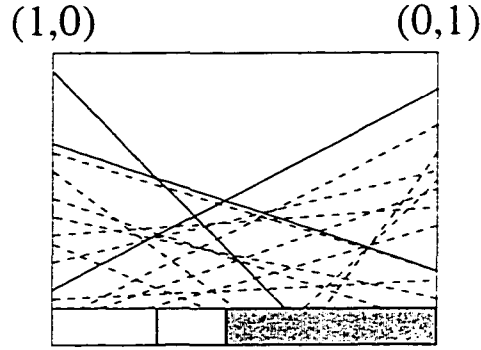
Figure 5.22: The set of vectors is checked to find out which ones are dominant.
