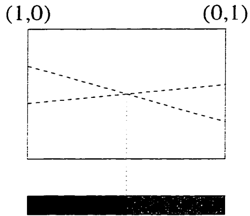
Figure 5.11: Partitions for the belief space given initial belief state b and action a_1 .
