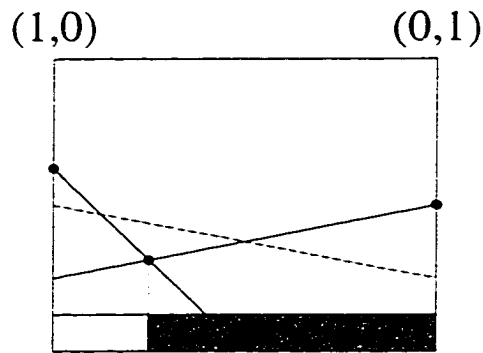
Figure 5.18: Second vector found by Cheng's algorithm.
