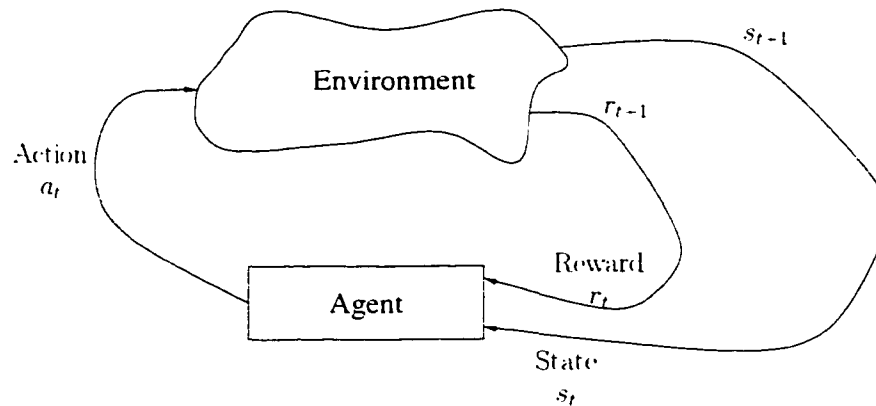
Figure 3.1: An agent using reinforcement learning interacts with its environment by receiving states and rewards from the environment, and generating actions that change the environment.
