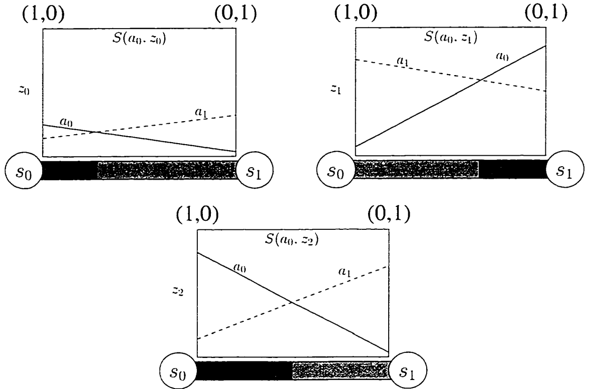
Figure 5.8: Each possible observation has a different transformation.
