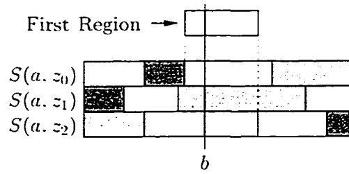
Figure 5.13: Sondik's first region.
