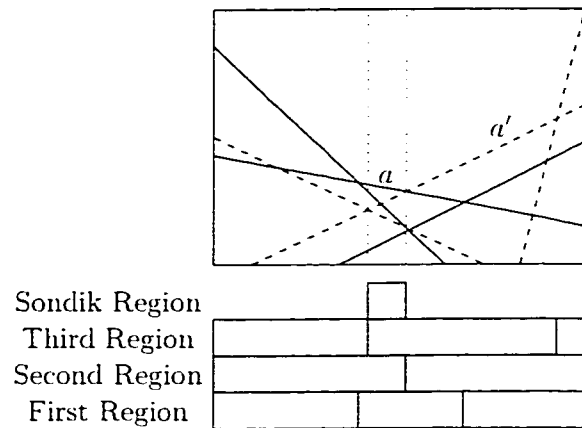
Figure 5.16: The complete Sondik region.
