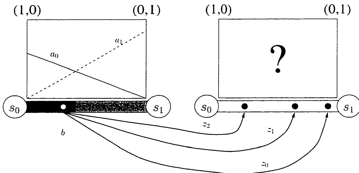
Figure 5.7: The transformed value function must account for all possible observations.
