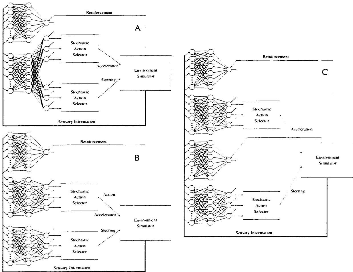
Figure 4.2: Three reinforcement learning networks to implement the race behavior. A) Single Utility Single Action. B) Single Utility Multiple Action. C) Multiple Utility Multiple Action.
