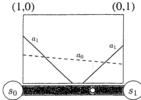
Figure 5.3: A graphical representation of a policy for a two state POMDP. The solid lines represent the value of taking action a_1 , while the dashed line represents the value of taking action a_0 . At the current belief state, represented by the dot, the value of action a_0 is greater than the value for action a_1 , so a_0 is the best action to take.
