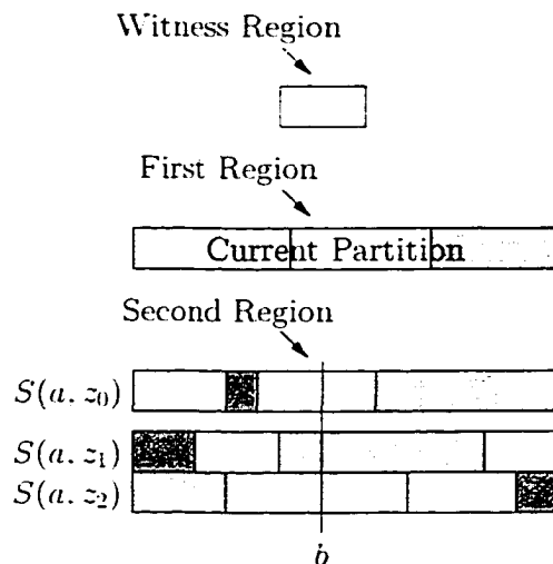
Figure 5.20: Regions defined in the Witness algorithm.
