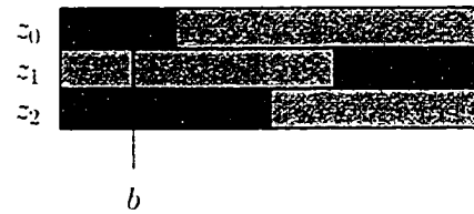
Figure 5.9: Partitions for the belief space given initial belief state b and action a_0 .
