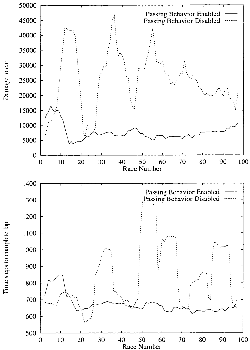
Figure 4.5: Using the passing behavior to improve performance.
