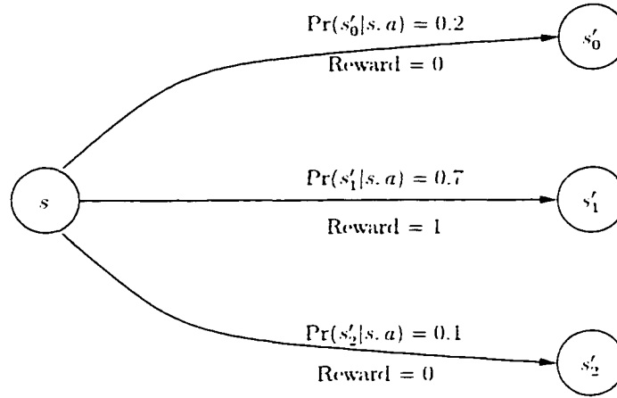
Figure 7.3: Rewards are assigned according to the most likely next state. In this case, the most likely state to follow s given action a is s'_1 . When the most likely state changes, a reward of one is produced only if the new most likely state is s'_1 .
