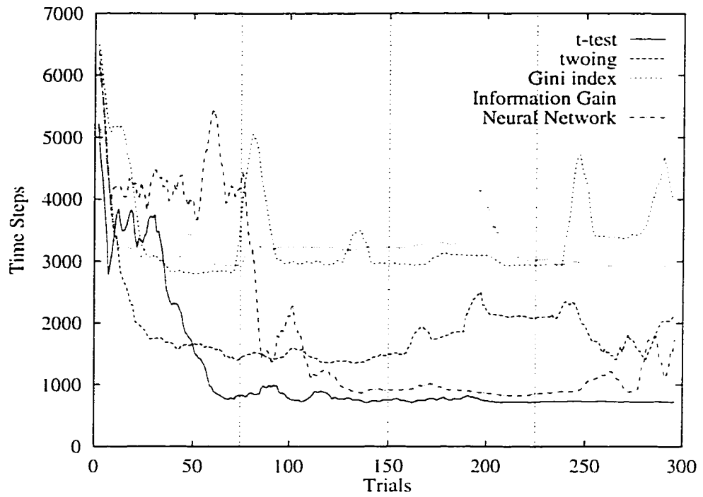
(a) time steps per lap.
