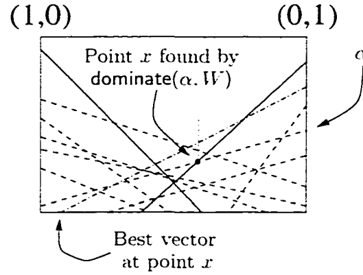
Figure 6.2: The two solid vectors are in the set W . All other vectors will be tested one at a time. For each vector \alpha , the dominate function finds the largest point x on \alpha that is not dominated by another vector in the set W , but this does not mean that \alpha should be added to W . The point x is only a witness to the fact that W does not contain the best vector at that point.
