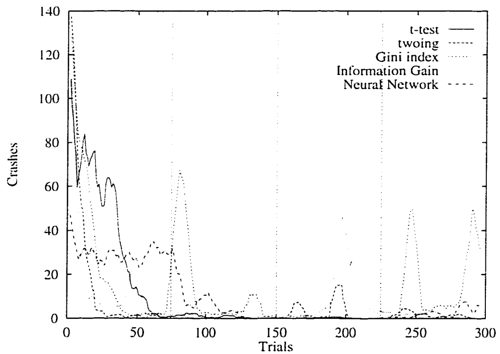
(b) number of crashes per lap.
