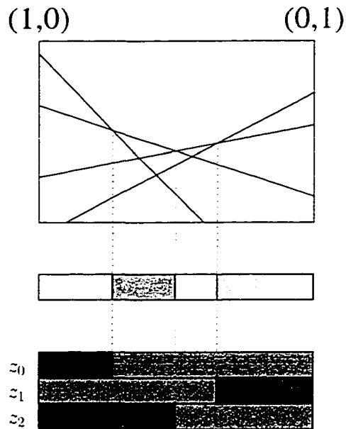
Figure 5.10: Partitions for the belief space as intersections in lines that form the value function.
