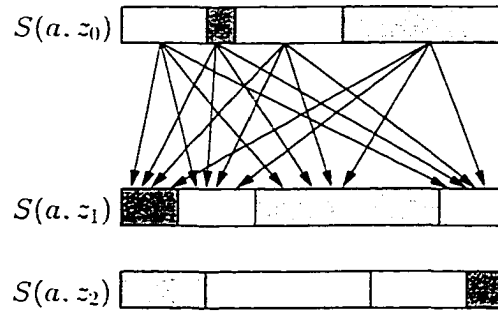
Figure 5.21: IP creates all combinations of vectors from the source sets.
