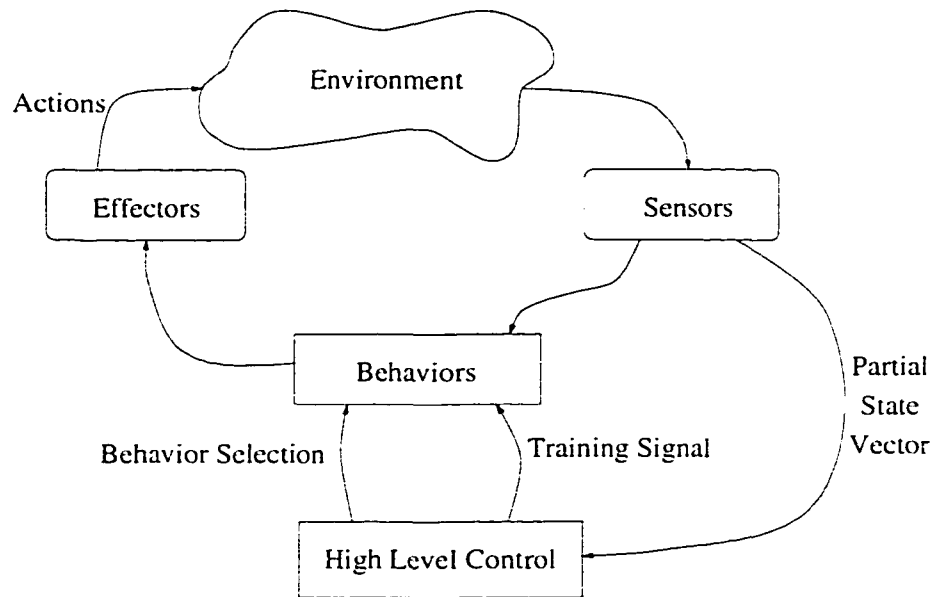
Figure 4.1: Simplified agent architecture for RARS experiments.
