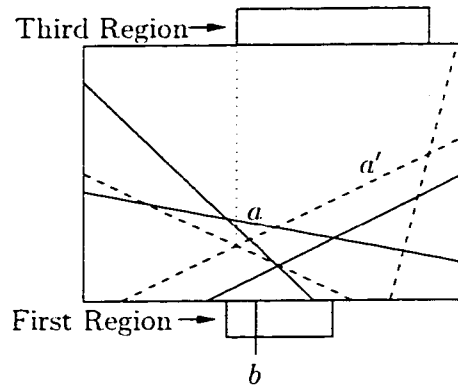
Figure 5.15: Sondik's third region.
