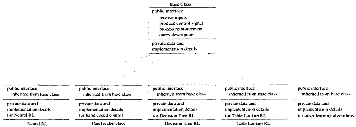
Figure 7.2: Low level actions are implemented as object classes.
