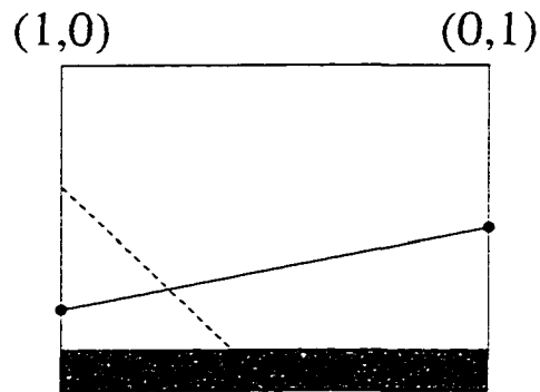
Figure 5.17: First vector found by Cheng's algorithm (solid line with dots at the endpoints) and second vector (dashed line).
