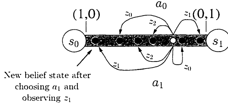
Figure 5.2: The new belief state depends on the action chosen and the observation received after executing that action. The three arcs at the top represent possible transitions when a_0 is chosen, while the arcs at the bottom represent possible transitions when a_1 is chosen.
