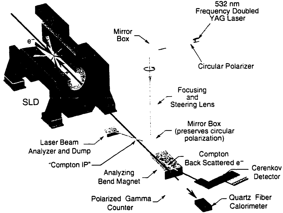
Figure 3.5: Schematic view of the Compton Polarimeter.
