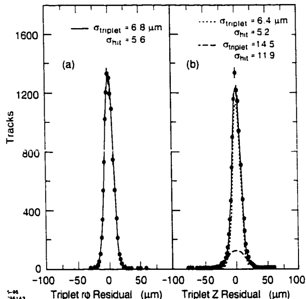
Figure 3.12: The VXD2 single hit resolution, determined from triplets, in (a) the r\phi plane and (b) the rz plane.
