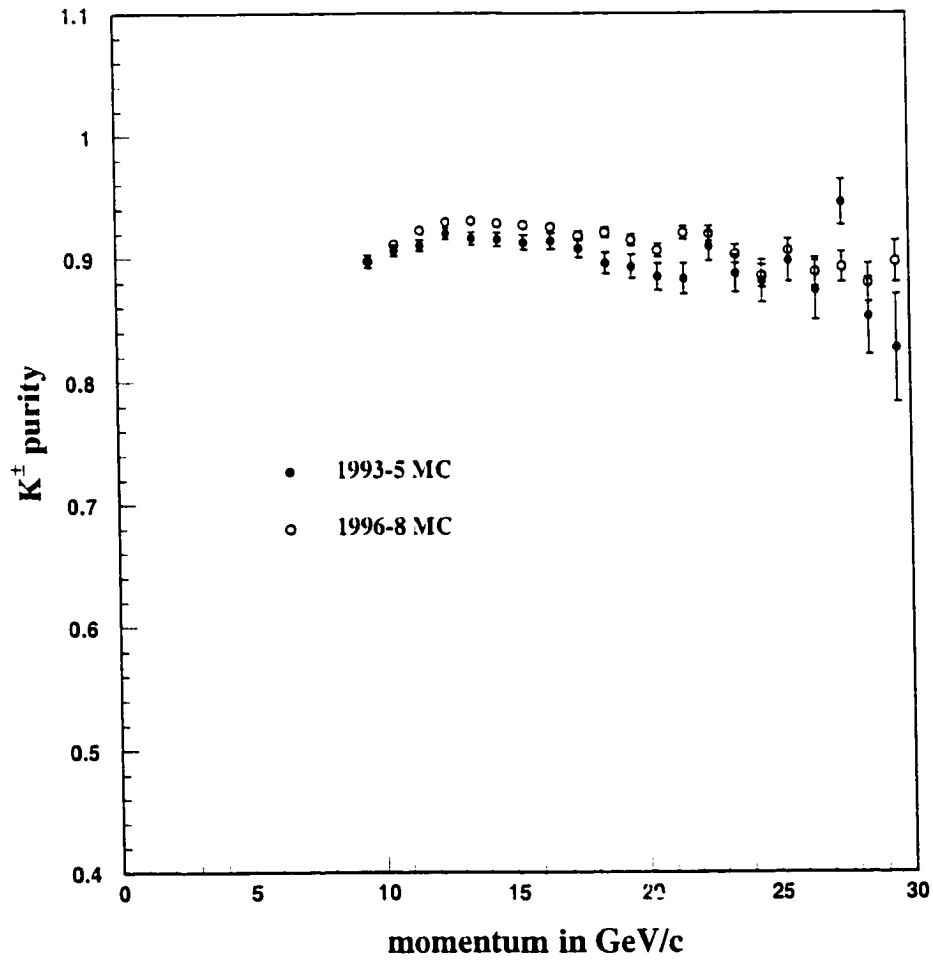
Figure 6.5: The purity of the identified K^\pm sample as a function of track momentum, as estimated from the Monte Carlo simulation. The uncertainties shown are statistical only.
