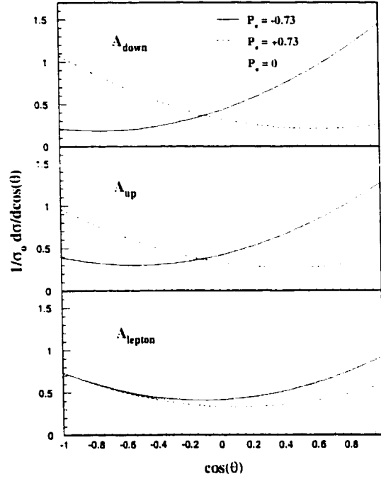
Figure 2.3: Polar angle dependence of the normalized production cross section for positive and negative electron beam polarization.
