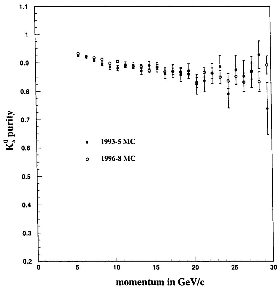
Figure 6.13: The purity of the selected K_s^0 candidate sample as a function of momentum, as estimated from the Monte Carlo simulation. The uncertainties shown are statistical only.
