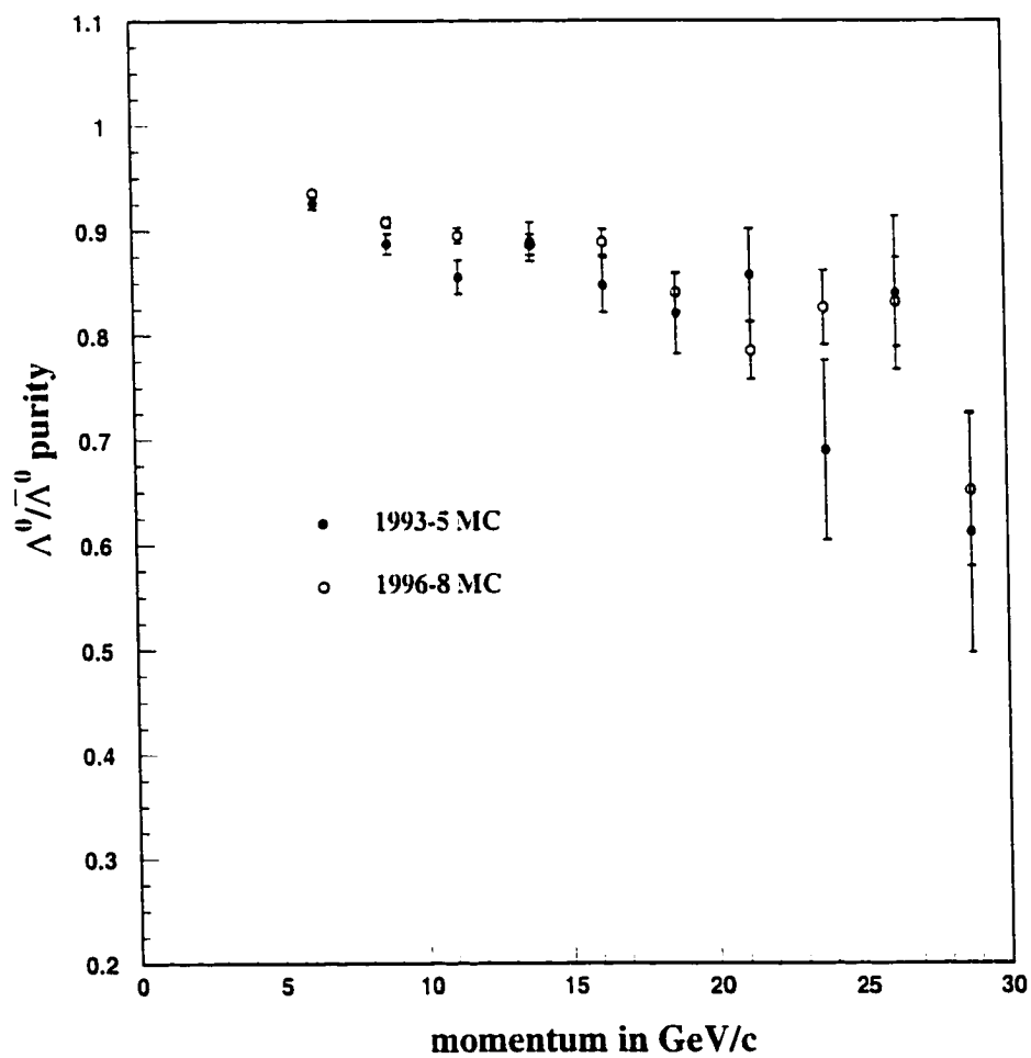
Figure 6.10: The purity of the selected \Lambda^0/\bar{\Lambda}^0 candidate sample as a function of momentum, as estimated from the Monte Carlo simulation. The uncertainties shown are statistical only.
