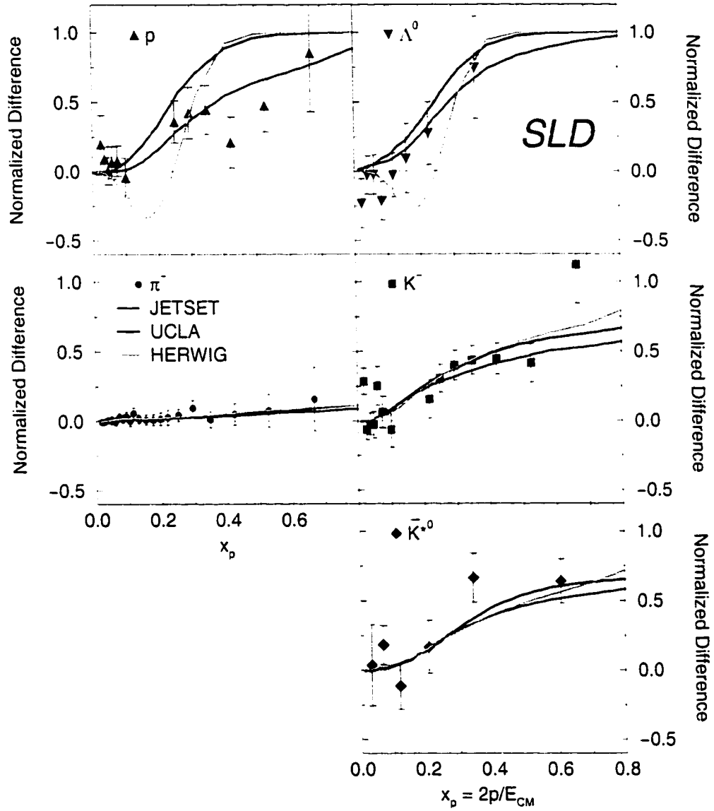
Figure 2.10: Normalized differences between hadron and anti-hadron production in light flavored jets. The data, represented by symbols, are compared to the predictions of three fragmentation models.
