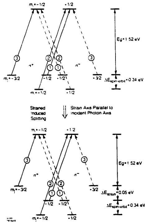
Figure 3.3: Energy state diagram for (top) bulk GaAs and (bottom) the strained GaAs lattice. The encircled numbers denote the relative intensities of the transitions. The strained lattice breaks the degeneracy and allows a theoretical polarization of 100%.
