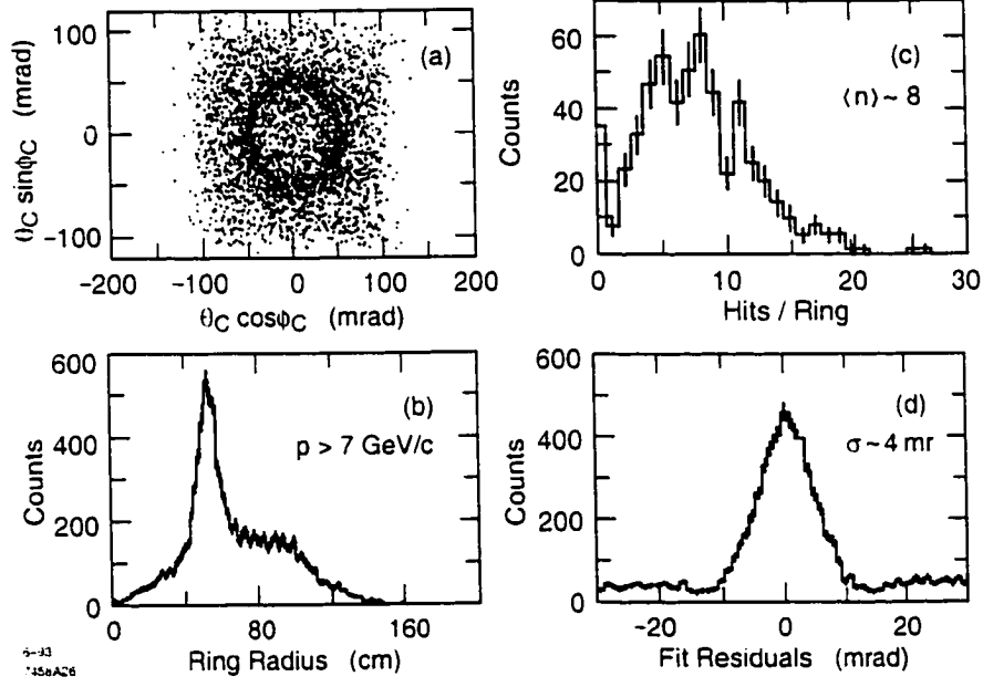
Figure 4.17: CRID gas rings: (a) in Cherenkov space, (b) radii, (c) number of photoelectrons per ring, (d) radii fit residuals.
