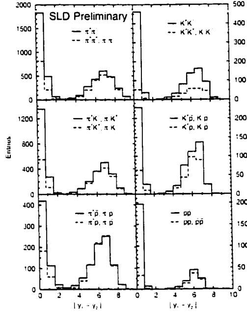
Figure 6.2: Rapidity differences for (solid) opposite charge pairs and (dashed) same charge pairs of identified \pi^\pm , K^\pm and p/\bar{p} with p > 9 GeV/c.
