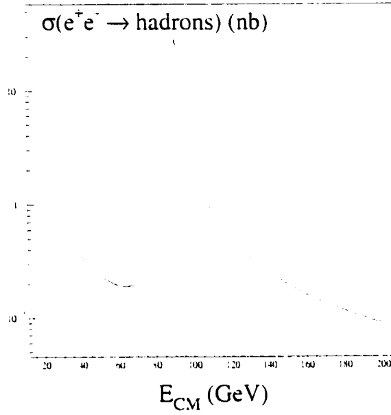
Figure 2.2: Energy dependence of the e^+e^- \rightarrow \text{hadrons} cross section.
