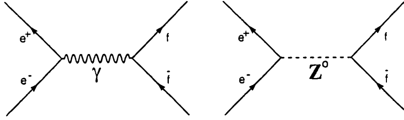
Figure 2.1: The s channel tree-level Feynman diagrams for the process e^+e^- \rightarrow Z^0/\gamma \rightarrow f\bar{f} .
