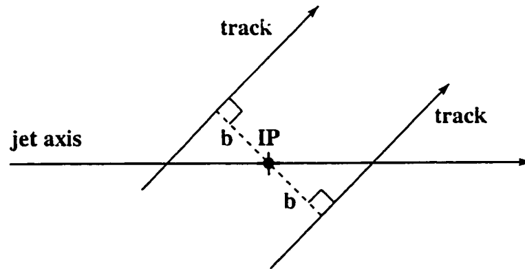
Figure 5.4: The impact parameter is assigned a positive (negative) sign if the charged track crosses the jet axis in front of (behind) the IP.
