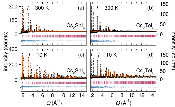
Figure 2.3: Rietveld refinements of high-resolution time-of-flight neutron scattering data of (a,c) \text{Cs}_2\text{SnI}_6 and (b,d) \text{Cs}_2\text{TeI}_6 collected from wavelength frame 2 on the POWGEN diffractometer at the Spallation Neutron Source, Oak Ridge National Laboratory. Data collected at T = 300 K are shown in panels (a) and (b) and data collected at T = 10 K are shown in panels (c) and (d). Refinements were performed using data collected from wavelength frames 2 and 4 of the POWGEN diffractometer. Black circles are the data, the orange line is the fit, and the blue line is the difference. The pink tick marks indicate the location of predicted Bragg reflections for the cubic structure.
