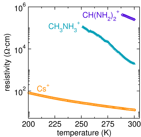
Figure 3.3: Electrical resistivity as a function of temperature for each member of the A_2\text{SnI}_6 series. Data were collected on cold-pressed polycrystalline pellets using a 4-wire configuration with Au paste for A = \text{Cs}^+ and \text{CH}_3\text{NH}_3^+ and Ag paste for \text{CH}(\text{NH}_2)_2^+ .
