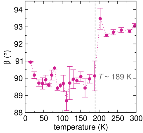
Figure 4.4: Monoclinic \beta angle plotted as a function of temperature extracted from sequential Rietveld refinements of the P2_1/n structural model of \text{Rb}_2\text{SnI}_6 against neutron diffraction data collected on the NOMAD instrument.
