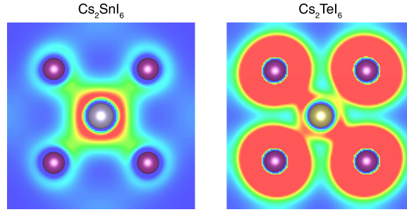
Figure 2.9: Charge density isosurfaces of the occupied ns^2 states in Cs_2SnI_6 and Cs_2TeI_6 . Sn, Te, and I atoms are denoted by grey, gold, and purple spheres, respectively. Contours shown from 0 (blue) to 0.002 \text{ eV } \text{\AA}^{-3} and 0.0034 \text{ eV } \text{\AA}^{-3} (red) for Cs_2SnI_6 and Cs_2TeI_6 , respectively.
