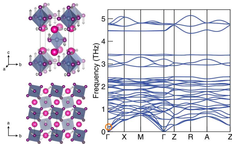
Figure 4.12: The phonon band structure of rubidium tin(IV) iodide in the tetragonal P4/mnc structure ( a^0a^0c^+ ). The lowest-frequency optic mode at 0.25 THz (1.03 meV, 8.27\text{ cm}^{-1} ) (denoted by the orange circle) corresponds to displacements of the rubidium and iodine atoms, as shown by the displacement vectors in the structural representations. Together, these displacements map to the octahedral tilting out of the ab plane coupled with \text{Rb}^+ displacements observed in the lower-symmetry monoclinic structure, ( a^-a^-c^+ ).
