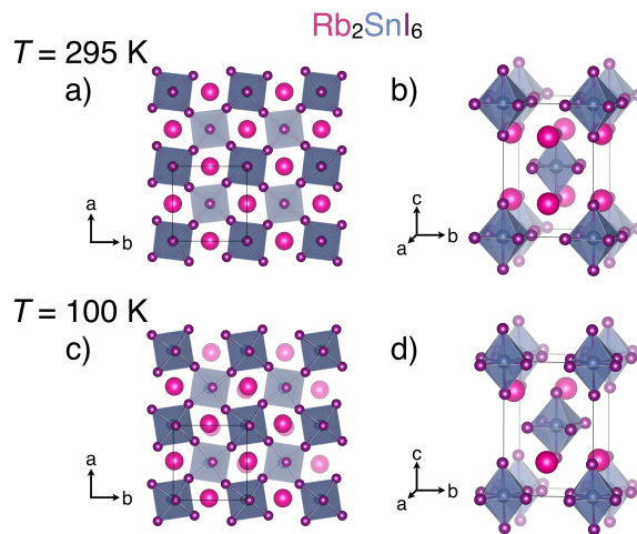
Figure 4.1: Crystal structures of \text{Rb}_2\text{SnI}_6 at T = 295\text{ K} and T = 100\text{ K} . In (a) and (c), the structures are projected down the c -axis to highlight the octahedral tilting and rotation, while unit cell descriptions are shown in b) and d). Rubidium atoms are shown in pink, tin atoms in blue, and iodine atoms are shown in purple.
