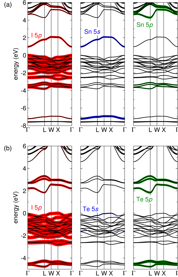
Figure 2.12: Band structures, including orbital projection analysis, of (a) \text{Cs}_2\text{SnI}_6 and (b) \text{Cs}_2\text{TeI}_6 , showing the contributions of: the I p states in red, the B 5s states in blue, and the B 5p states in green.
