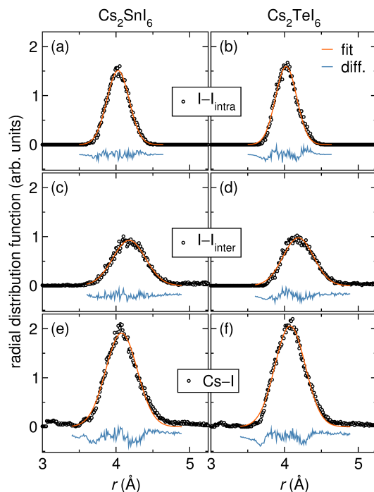
Figure 5.9: Partial radial distribution functions for \text{I-I}_{\text{intra}} (a,b), \text{I-I}_{\text{inter}} (c,d), and \text{Cs-I} (e,f) pair correlations in \text{Cs}_2\text{SnI}_6 and \text{Cs}_2\text{TeI}_6 obtained from pseudo-rigid-body Reverse Monte Carlo simulations (circles). The distributions are fit with Gaussian functions, shown by the orange line. The difference curves are shown in blue and reveal asymmetries in the \text{I-I}_{\text{inter}} and \text{Cs-I} RDFs.
