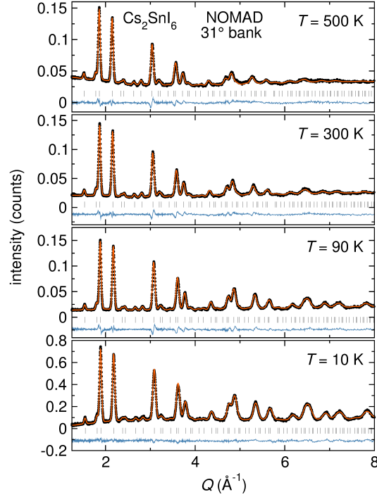
Figure 5.4: Rietveld refinements of temperature-dependent neutron diffraction of \text{Cs}_2\text{SnI}_6 at T = 10, 90, 300 , and T = 500 K from the 31^\circ bank (bank 2) of the NOMAD instrument at the Spallation Neutron Source, Oak Ridge National Laboratory. The data are modeled with the cubic vacancy-ordered double perovskite structure at all temperatures. Black circles are the data, the orange line is the fit, the blue line is the difference, and the grey tick marks represent positions of anticipated reflections for the Fm\bar{3}m vacancy-ordered double perovskite structure. The data at T = 10, 90 , and T = 300 K have been previously reported. 8
