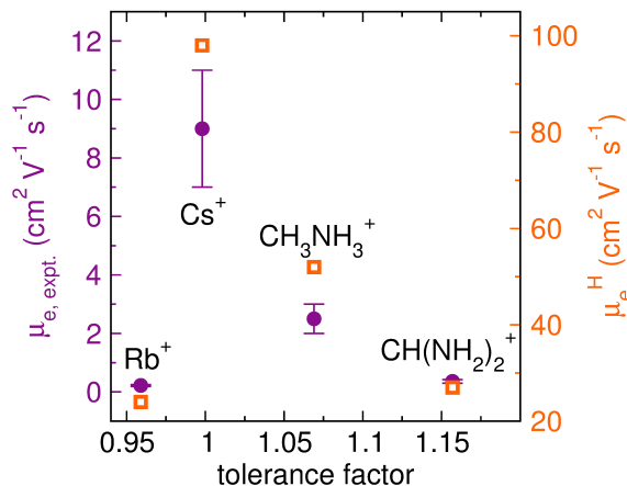
Figure 4.13: Experimentally- ( \mu_{e,\text{expt.}} ) and computationally-derived Hellwarth ( \mu_e^H ) electron mobilities of the \text{A}_2\text{SnI}_6 vacancy-ordered double perovskites plotted as a function of perovskite tolerance factor. Experimental electron mobilities are shown as filled purple circles on the left axis, while the calculated Hellwarth electron mobilities are denoted by open orange squares on the right axis. Values for the carrier mobilities of \text{Cs}_2\text{SnI}_6 , (\text{CH}_3\text{NH}_3)_2\text{SnI}_6 , and (\text{CH}(\text{NH}_2)_2)_2\text{SnI}_6 are taken from a previous study. 6 For \text{Rb}_2\text{SnI}_6 , the \mu_e^H value is calculated from the tetragonal structure.
