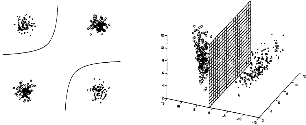
Figure 2.2: The Exclusive-Or Problem Revisited. On the left (a), the hyperbola xy = 1 separates X and Y . On the right (b), the same equation yields a plane which separates \Phi(X) and \Phi(Y) .
