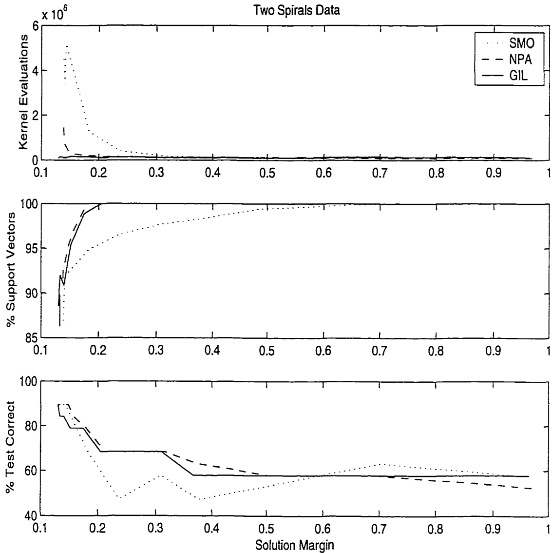
Figure 4.3: Two Spirals Data. Here we plot the performance statistics for SMO, NPA and Gilbert's Algorithm for SVMs on the Two Spirals Data. In each plot the horizontal axis gives the solution margin, dotted lines are used for SMO, dashed lines are used for NPA, and solid lines are used for Gilbert's Algorithm for SVMs. In the top plot (a) we see on the vertical axis the number of kernel evaluations performed, in the middle plot (b) we see the percentage of support vectors found, and in the bottom plot (c) we see the percentage of points in the test set correctly classified.
