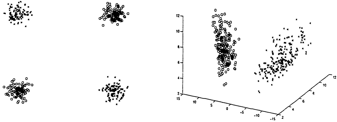
Figure 1.2: The Exclusive-Or Problem. On the left (a) we see that the exclusive-or problem is not linearly separable. On the right (b) the exclusive-or problem becomes linearly separable after nonlinear preprocessing by \Phi in Equation (1.2).
