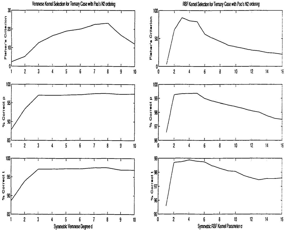
Figure 3.1: Symmetric Veronese and RBF Kernel Selection for Materials Design. Here we display kernel selection plots for the ternary case using Pao's N2 ordering. On the left are plots of Fisher's criterion, the percentage p of points correctly classified, and the percentage t of points correctly classified (from top to bottom) versus the symmetric Veronese degree d . Using these plots we selected d = 3 . On the right are plots of the same values versus the symmetric RBF kernel parameter \sigma . Using the RBF plots we selected \sigma = .25 .
