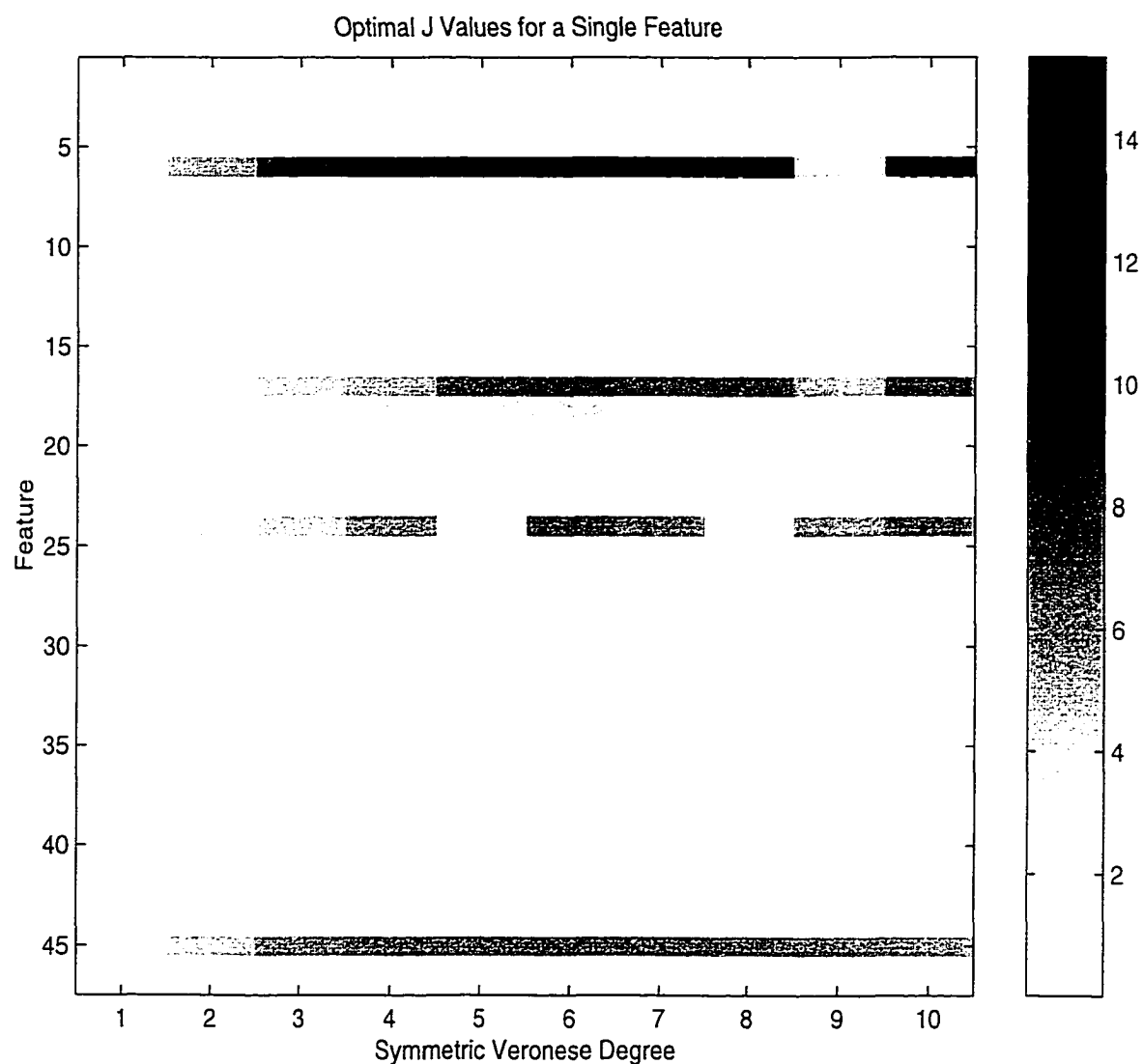
Figure 2.3: One Feature Test. This is an intensity plot of the optimal J value (whose range is given by the scale bar on the right) versus the symmetric Veronese degree for each feature. A dark horizontal bar indicates high optimal J values and thus identifies a good feature.
