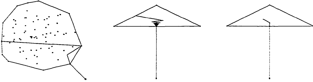
Figure 4.2: Convergence of Gilbert's Algorithm. Here we illustrate the behavior of Gilbert's Algorithm. On the left (a) s^* \in S , and the algorithm, whose progress is tracked by the jagged line, converges to s^* in a finite number of steps. In the middle (b), s^* \notin S and the algorithm converges only asymptotically to s^* . On the right (c), Gilbert's Algorithm for Support Vector Machines converges rapidly in angle to s^* .
