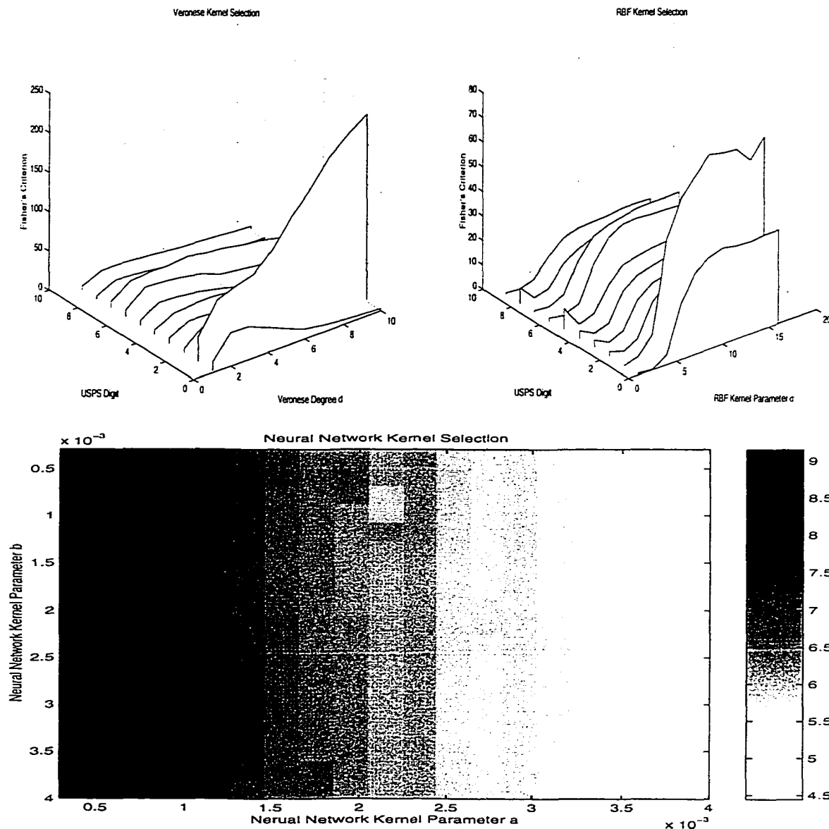
Figure 3.4: Entire USPS Problem. On the upper left is kernel selection information for the Veronese kernel for separating each of the USPS digits from the other nine. On the upper right is selection information for the RBF kernel. On the bottom is selection information for the neural network kernel for separating the digit 5 from the other nine digits. The neural network plot is an intensity plot with the values of Fisher's Criterion shown on the scale bar to the right.
