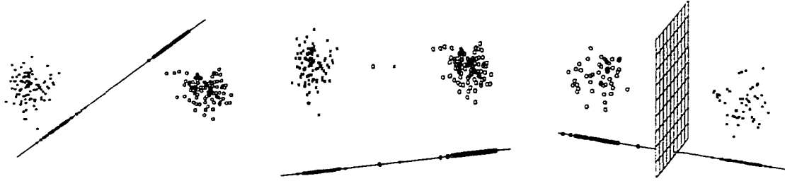
Figure 2.1: Fisher's Discriminant. On the left (a) is an example of Fisher's criterion. The two classes are represented by x's and o's, and the span of \mathbf{a} is shown as a line. In this example J(\mathbf{a}) = 77 . In the middle (b) is an example where J(\mathbf{a}) = 64.5 is a large number despite the fact that the two classes are not linearly separable. On the right (c) is the full version of Fisher's discriminant. In this case the line represents the span of \mathbf{a}^* in Equation (2.1) and the separating plane has Equation (2.2).
