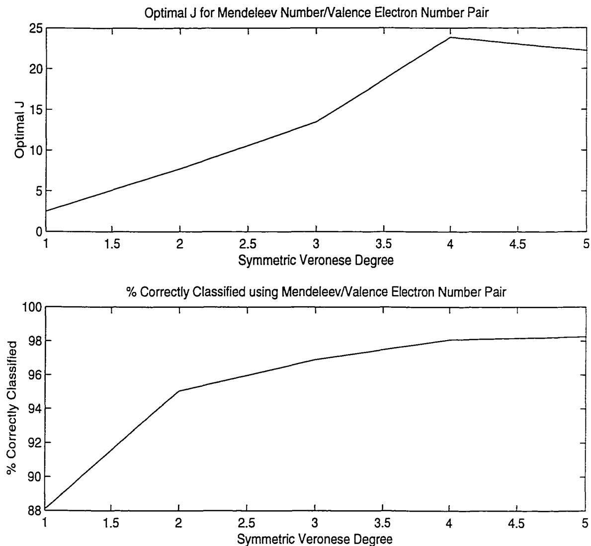
Figure 2.6: Mendeleev/valence electron numbers are the Best Feature Pair. On the top (a) we plot the optimal J value and on the bottom (b) the percentage correctly classified both versus the symmetric Veronese degree for the Mendeleev/valence electron number pair.
