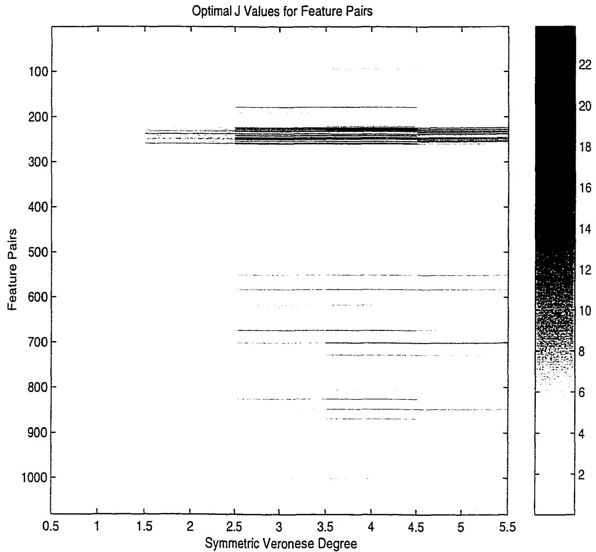
Figure 2.5: Two Feature Test. This is an intensity plot of optimal J versus the symmetric Veronese degree for every pair of features.
