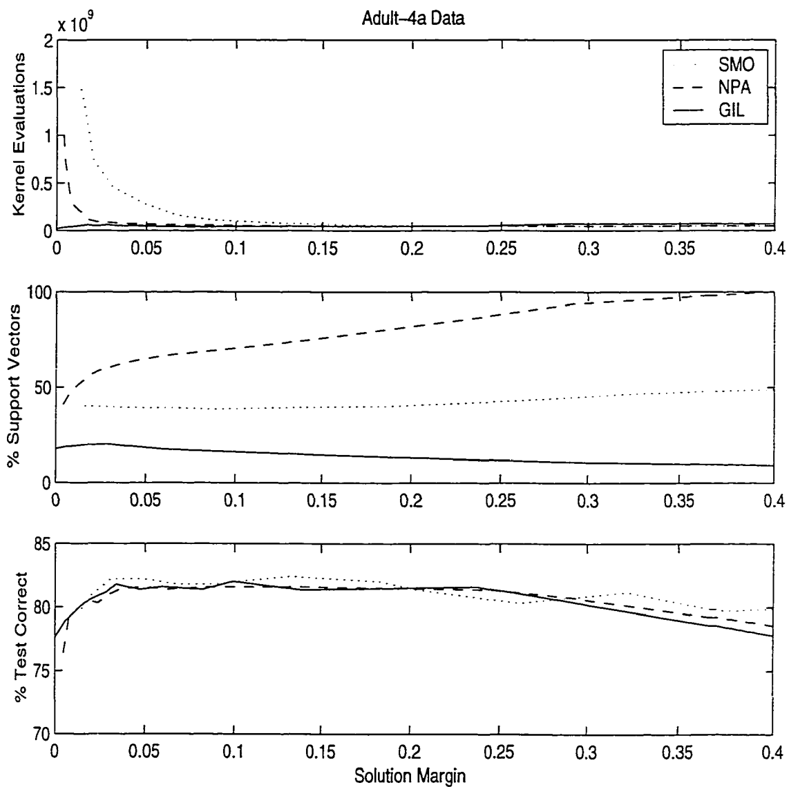
Figure 4.5: Adult-4a Data. Here we plot the performance statistics for SMO, NPA and Gilbert's Algorithm for SVMs on the Adult-4a Data.
