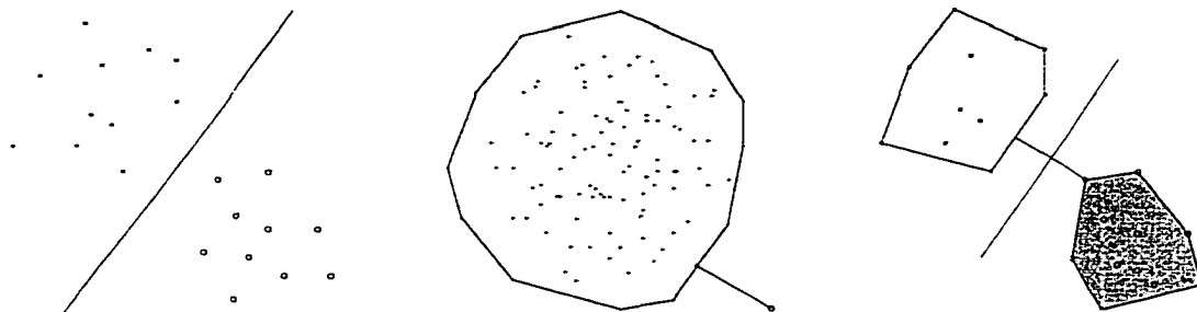
Figure 4.1: Pictorial summary of Theorem 4.2. On the left (a) is the typical illustration of a Support Vector Machine. The two classes X and Y are depicted using x 's and o 's, with the maximal margin hyperplane shown as a solid line separating them. The two dotted lines run through the support vectors and are separated by a distance equal to the margin. In the middle (b) is the corresponding secant hull with the origin marked by a circle, and with the point s^* in the secant hull closest to the origin marked by a star (and connected to the origin by a line segment). On the right (c) the maximal margin hyperplane is shown as the perpendicular bisector of a shortest line segment connecting the convex hulls of X and Y .
