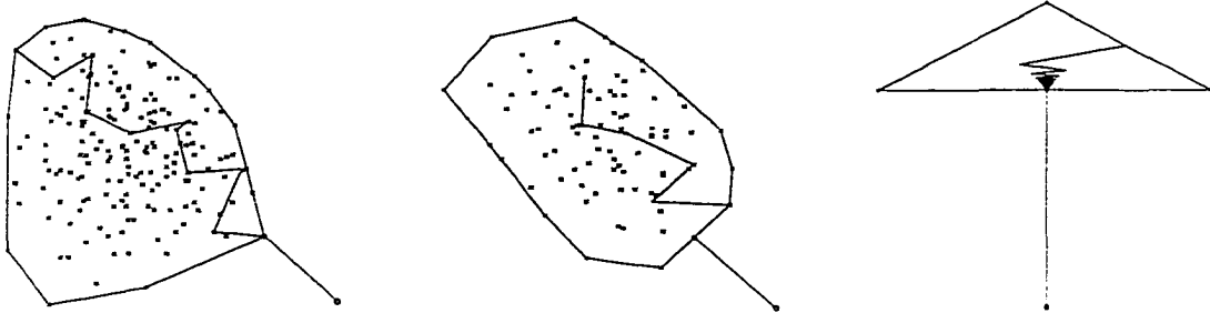
Figure A.1: Two Point Algorithm. Here we illustrate the behavior of the two point algorithm. On the left (a) s^* \in S , and the algorithm, whose progress is tracked by the jagged line, converges to s^* in at most p steps (guaranteed). In the middle (b). s^* \notin S but the algorithm still converges to s^* (in less than p steps for this example — not guaranteed). On the right (c), the algorithm converges only asymptotically to s^* .
