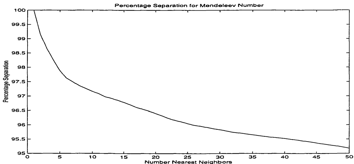
Figure 2.7: Percentage Separation Plot. Pierre Villars' percentage separation plot for the Mendeleev number.
