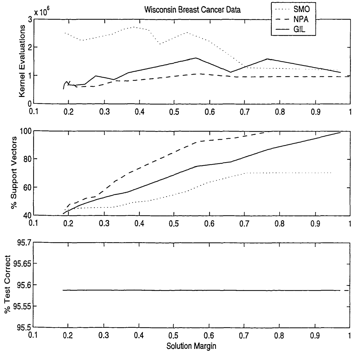
Figure 4.4: Wisconsin Breast Cancer Data. Here we plot the performance statistics for SMO, NPA and Gilbert's Algorithm for SVMs on the Wisconsin Breast Cancer Data. The data is presented as in Figure 4.3. The success rates on the test set are identical for all three algorithms.
