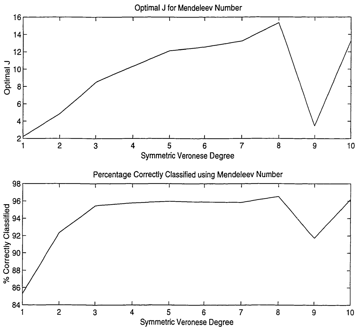
Figure 2.4: Mendeleeev Number is the Best Feature. On the top (a) we plot the optimal J value and on the bottom (b) the percentage correctly classified both versus the symmetric Veronese degree for the Mendeleeev number.
