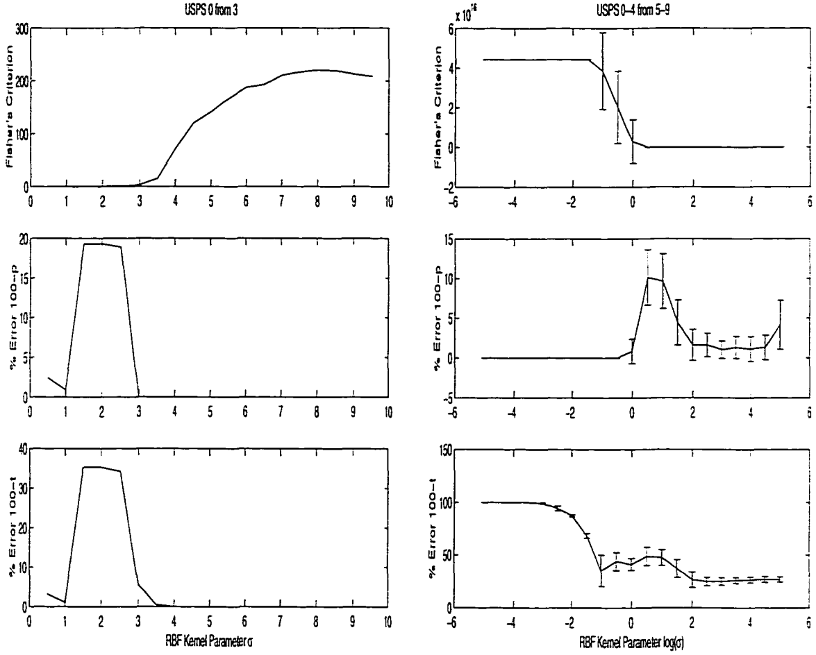
Figure 3.3: USPS Partial Problems. On the left are the plots of J(\mathbf{a}^*) , 100 - p , and 100 - t (from top to bottom) versus RBF kernel \sigma for the problem of separating 0 from 3 in the USPS data set. On the right are the plots of J(\mathbf{a}^*) , 100 - p , and 100 - t versus \log(\sigma) for the problem of separating the digits 0 to 4 from 5 to 9.
