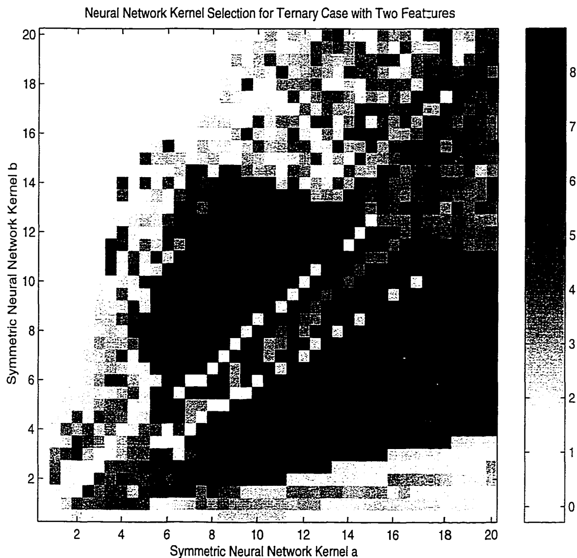
Figure 3.2: Symmetric Neural Network Kernel Selection for Materials Design. Here we display a kernel selection plot for the ternary case using Pao's N2 ordering and Pauling's Electronegativity (the third ranked feature pair). This is an intensity plot of the values of Fisher's criterion versus the symmetric neural network kernel parameters a and b . The values of Fisher's criterion are indicated by the scale bar on the right. Using this plot we selected a = 8.5 and b = 8 .
