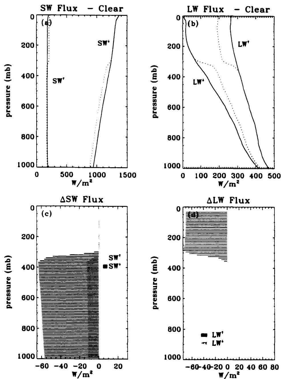
Figure 6.5: (Simulated) Clear sky computed fluxes and variations between cloudy and (simulated) clear sky: (a) SW fluxes: (b) LW fluxes: (c) \Delta SW fluxes: (d) \Delta LW fluxes. Nauru 1999 05 01 09:00 UTC.
