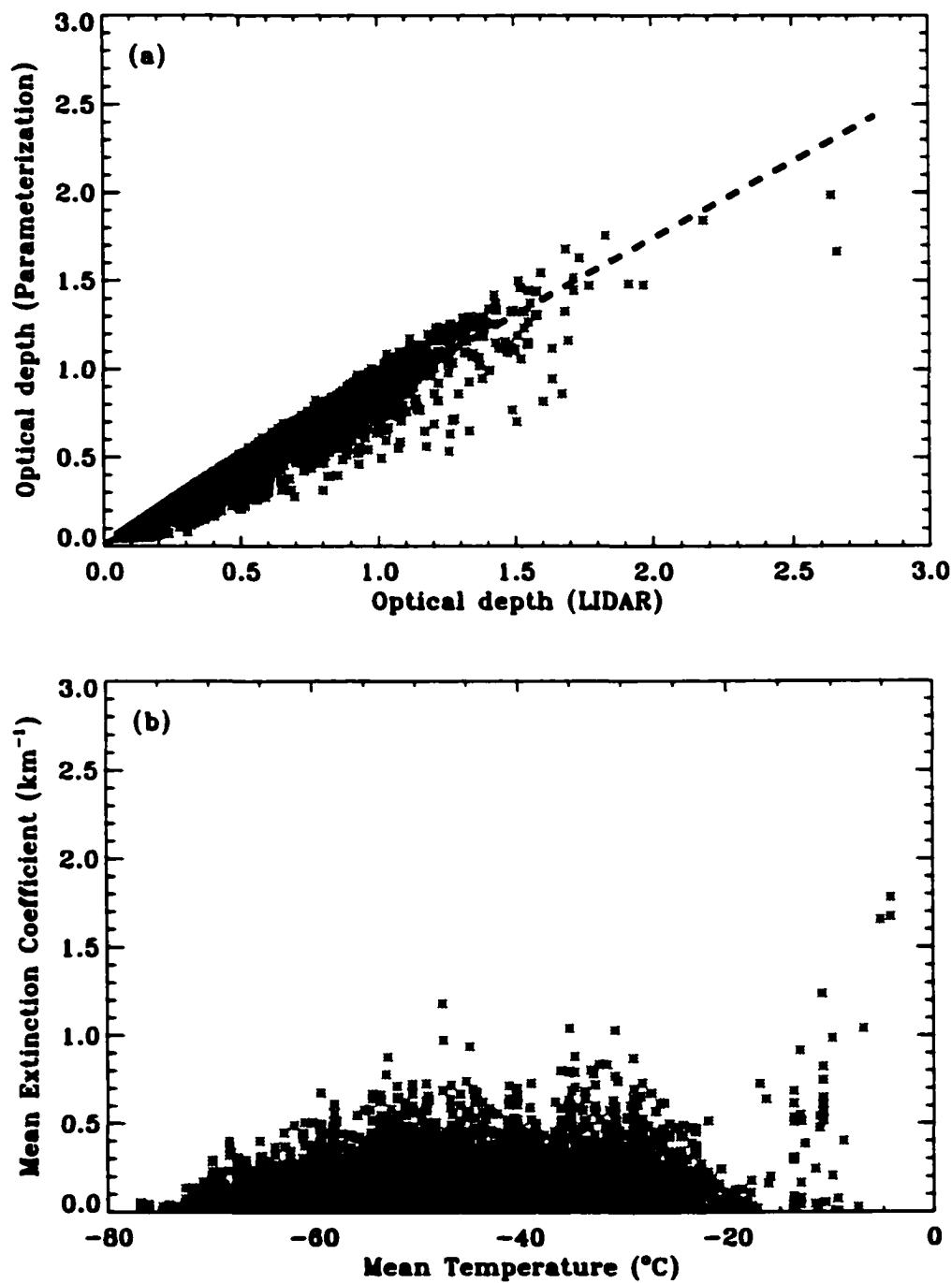
Figure 4.10: (a) Correlations between Optical Depths (stars). The slope for the linear correlation (dashed line) is 0.87; (b) Mean Extinction Coefficient vs. Layer mean Temperature. Nauru May-July 1999.
