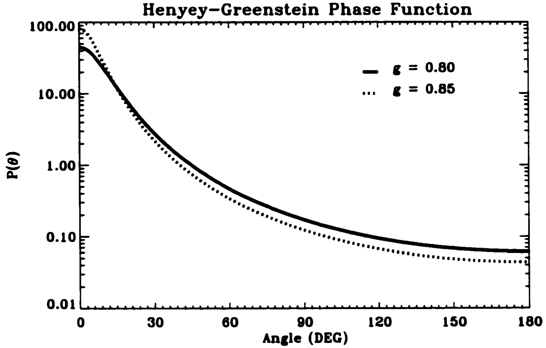
Figure 5.10: Henyey-Greenstein phase function for two asymmetry parameters: g=0.8 (solid line) and g=0.85 (dotted line).
