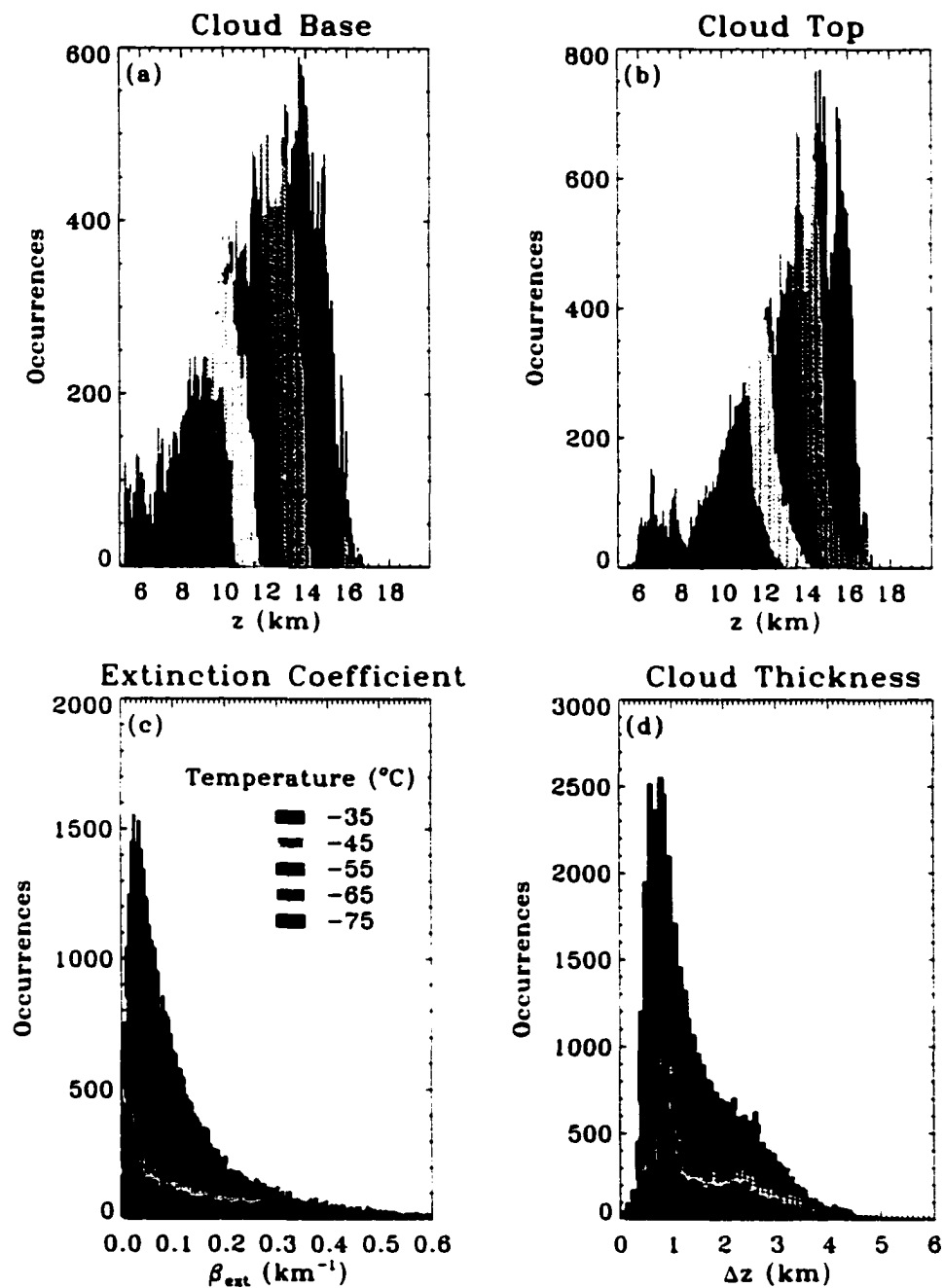
Figure 3.20: PDF for (a) Cloud base; (b) Cloud top; (c) Mean extinction coefficient; (d) Cloud thickness.
