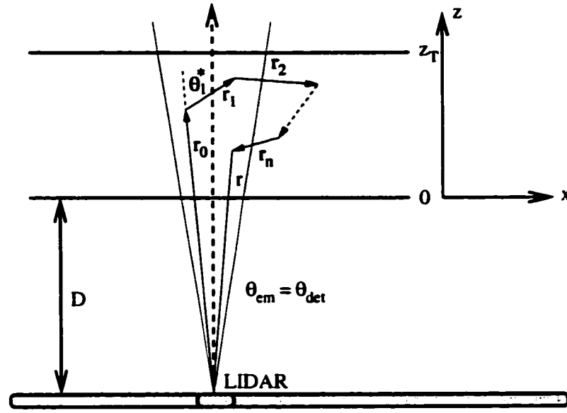
Figure 3.10: Multiple Scattering Geometry.
