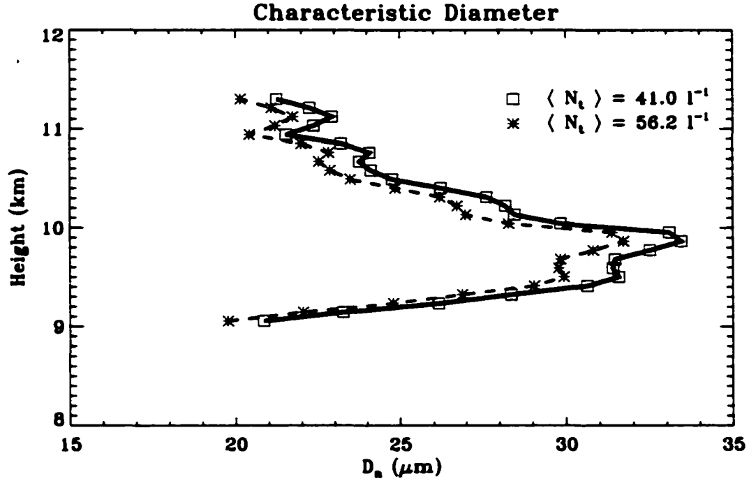
Figure 4.9: Profiles of Characteristic Diameter ( D_n ) using two radar-optical depth methods: optimal estimation approach (solid line and squares) compared with the present analytical method (dashed line and stars). Nauru 1999 05 21 08:22:09 UTC.
