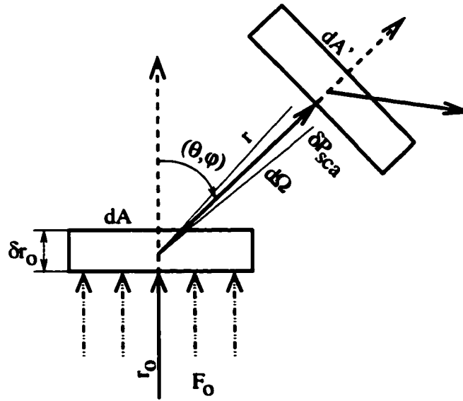
Figure 3.9: Scattering Geometry.
