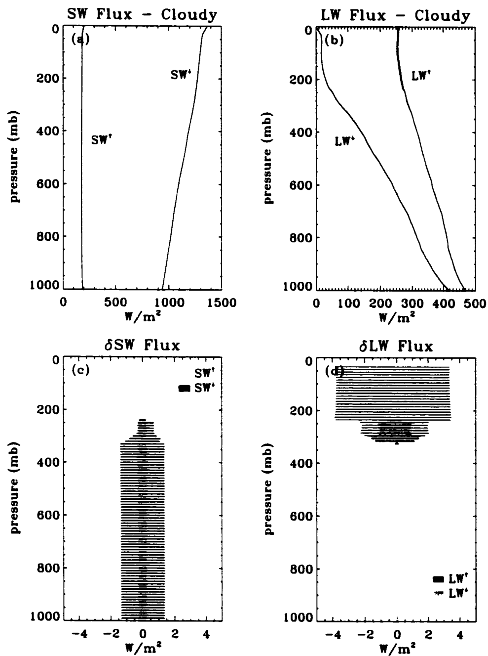
Figure 6.6: Cloudy sky computed fluxes and variations due to errors in mixing ratio: (a) SW fluxes; (b) LW fluxes; (c) \delta SW fluxes; (d) \delta LW fluxes. Nauru 1999 05 01 10:00 UTC.
