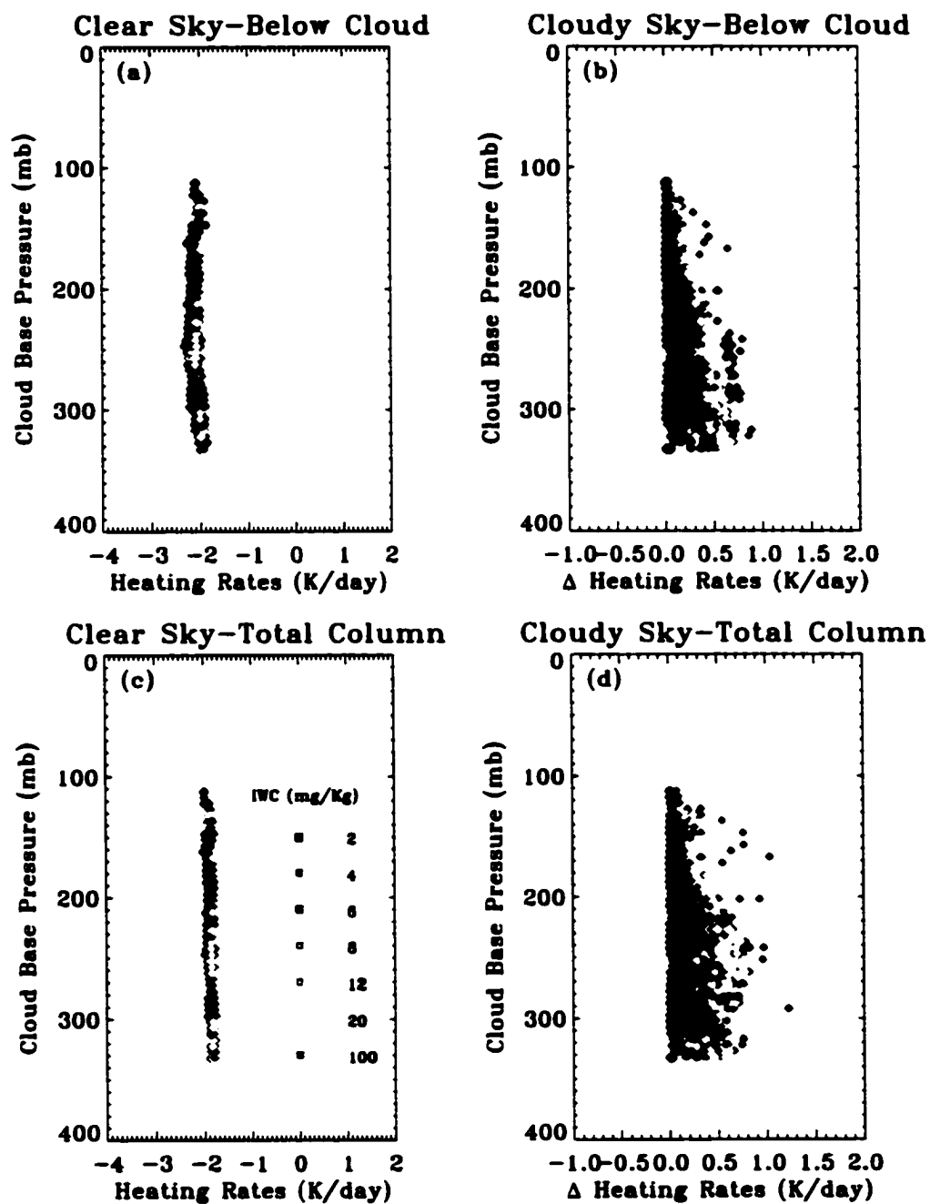
Figure 6.10: LW Heating rates for different atmospheric regions. Simulated clear sky (left panels): Differences between cloudy and clear sky (right panels). Colors represent mean IWC values. Nauru 1999.06.18–1999.07.15.
