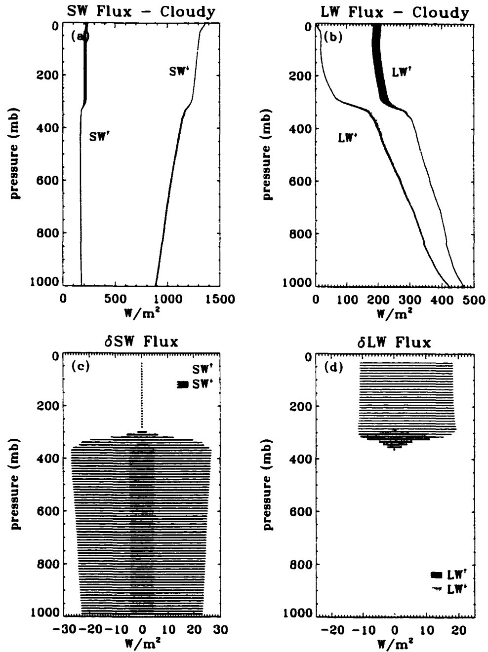
Figure 6.3: Cloudy sky computed fluxes and variations due to errors in mixing ratio: (a) SW fluxes: (b) LW fluxes: (c) \delta SW fluxes: (d) \delta LW fluxes. Nauru 1999 05 01 -- 09:00 UTC.
