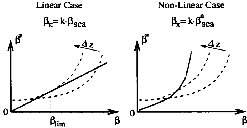
Figure 3.15: Inverse Method iteration procedure: Linear case: as the vertical resolution \Delta z increases, there is a limit in the retrieved scattering coefficient ( \beta_{lim} ). Non-linear case: a solution for the retrieved scattering coefficient exists for all possible vertical resolutions.
