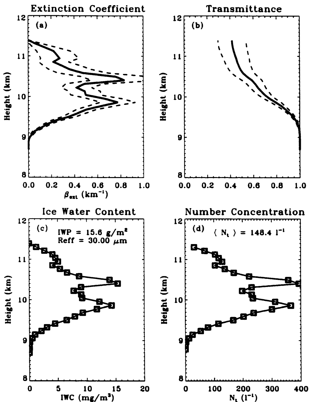
Figure 3.19: Retrieved quantities: (a) Extinction Coefficient (errors shown by dashed lines); (b) Transmittance (errors shown by dashed lines); (c) Ice Water Content; (d) Number Concentration. Nauru, 01 05 99 08:22:08 UTC.
