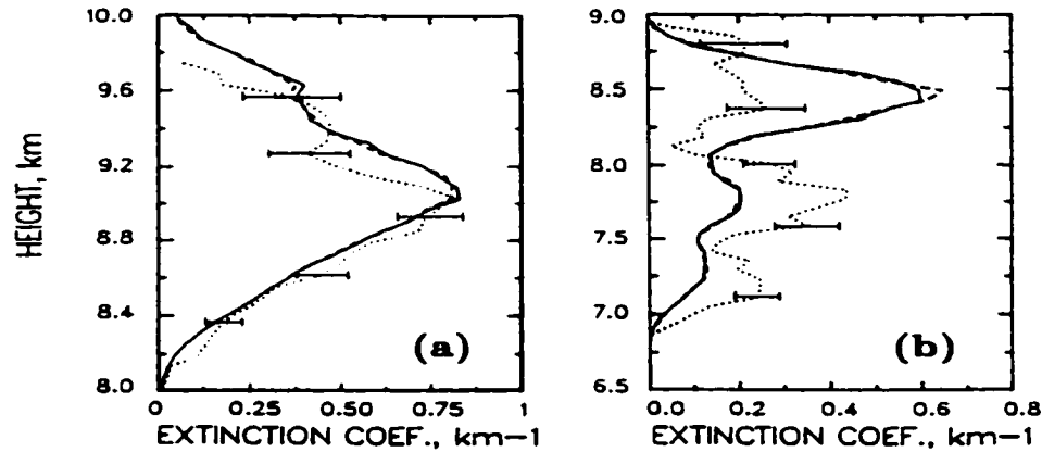
Figure 3.2: Aerosol extinction coefficient from a Raman lidar (dotted line) and from the same instrument used as an elastic-backscatter lidar (solid lines: Klett forward integration; dashed lines: Klett backward integration). (a) Lidar ratio = 15.7 sr; (b) Lidar ratio = 7.3 sr (From Ansmann et al., 1992a)
