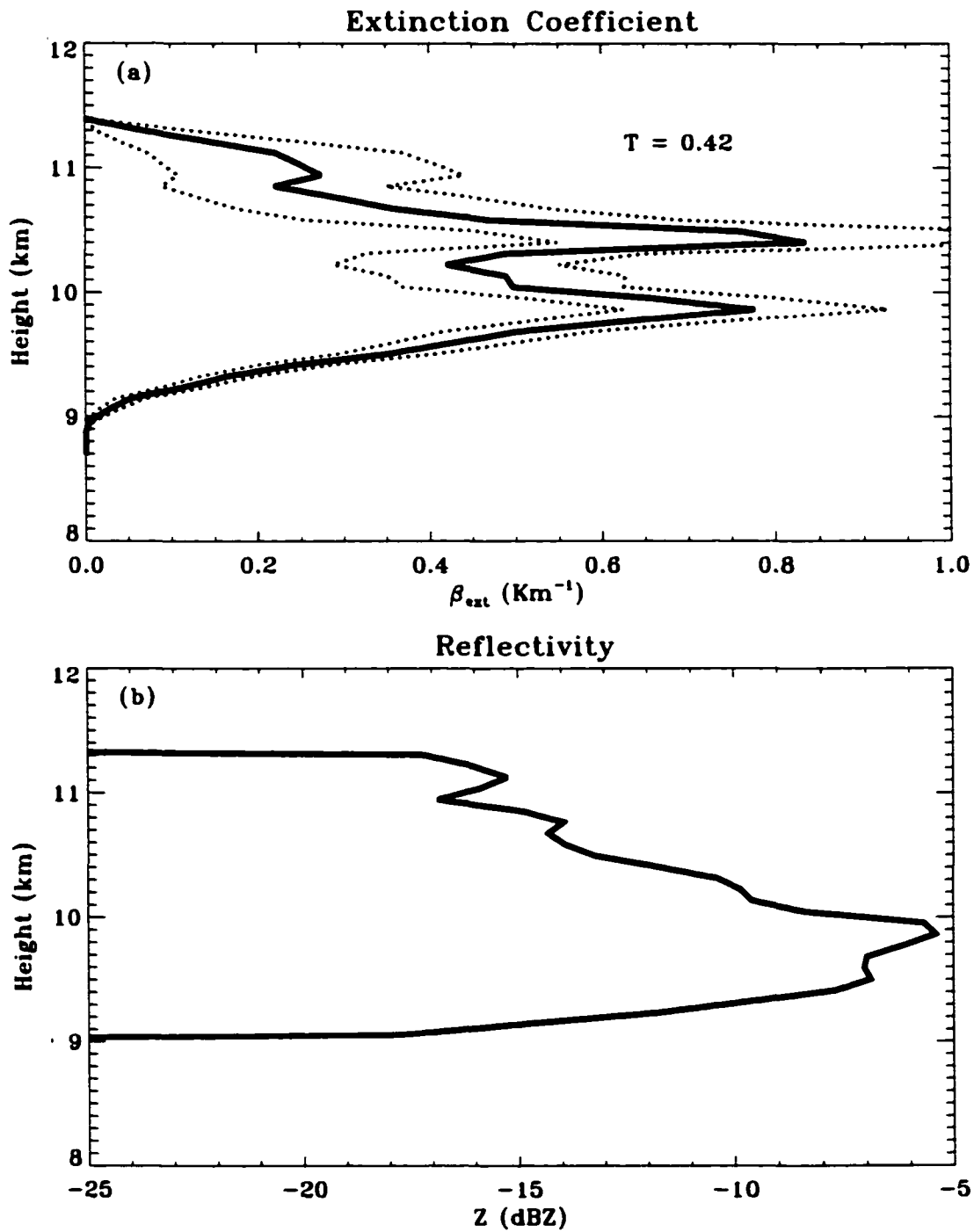
Figure 4.6: Profiles of (a) MPL Extinction Coefficient (transmittance of 0.42), and (b) MMCR Reflectivity. Uncertainties in profiles are shown by dots. Nauru 1999 05 21 08:22:09 UTC.
