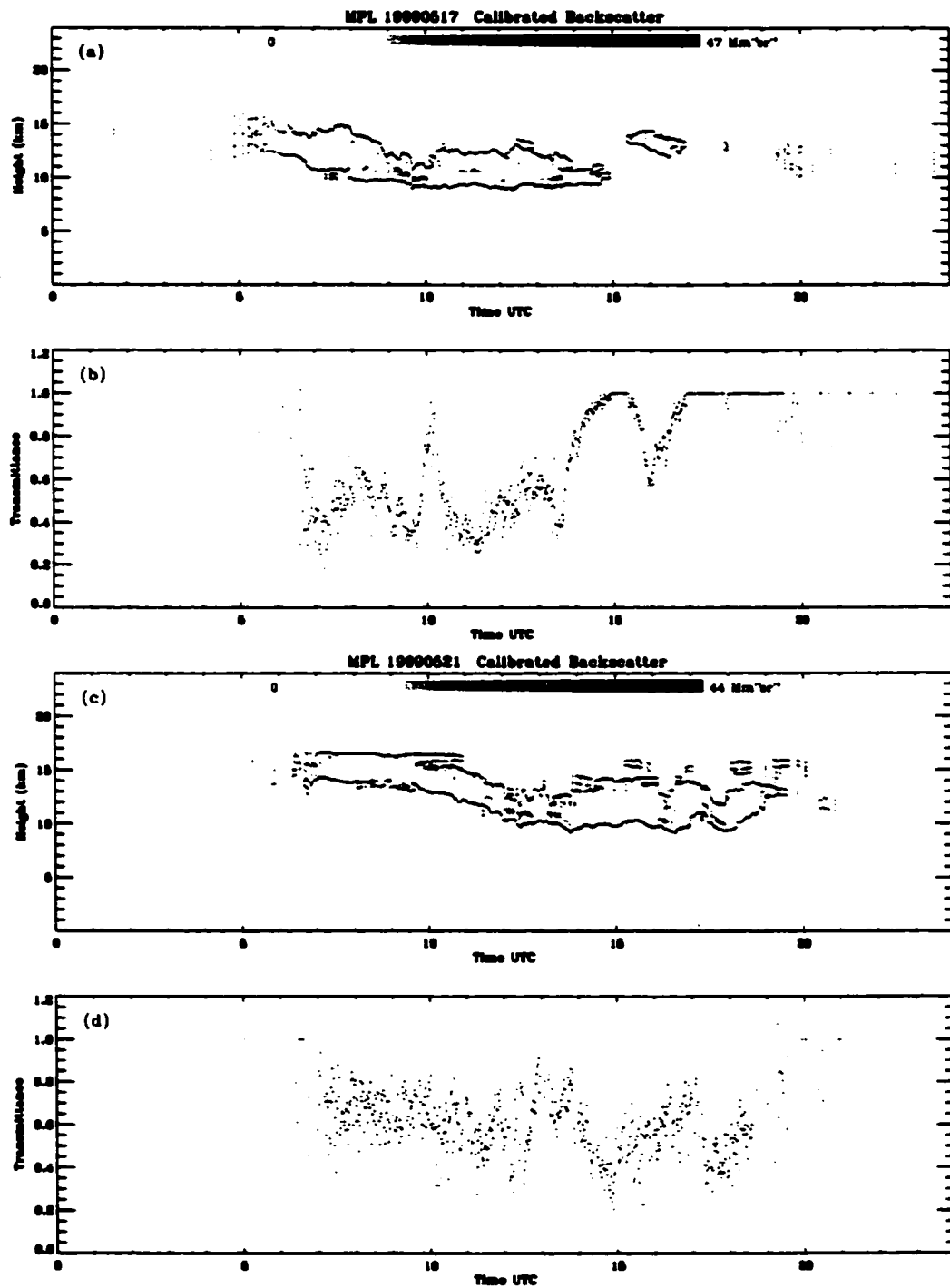
Figure 3.8: Time dependence of the MPL (a), (c) backscatter coefficient and (b), (d) transmittance for two days at Nauru: 1999/05/17 and 1999/05/21.
