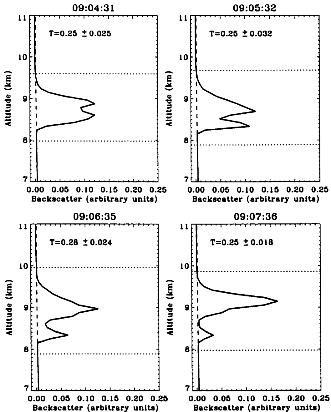
Figure 3.4: Raw backscatter signal (solid line), modeled signal (dashed line), and cloud boundaries (dotted line) at different times. Transmittance T for each profile is displayed. Nauru 1999 05 01.
