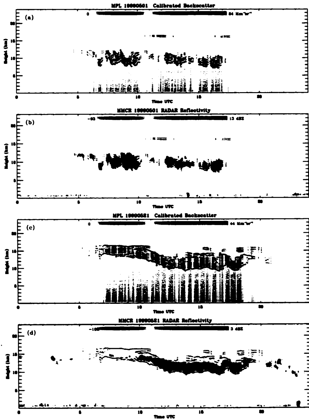
Figure 4.5: Time series of MPL and MMCR data at Nauru: (a), (b) 1999/05/01. (c), (d) 1999/05/21. Cloud boundaries shown by dots.
