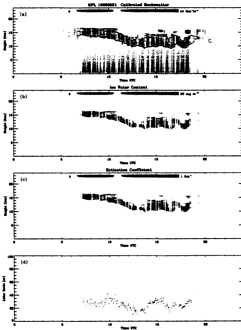
Figure 3.18: Time series for: (a) Backscatter coefficient (Cloud boundaries with dots); (b) Ice Water Content; (c) Extinction coefficient; (d) Lidar Ratio.
