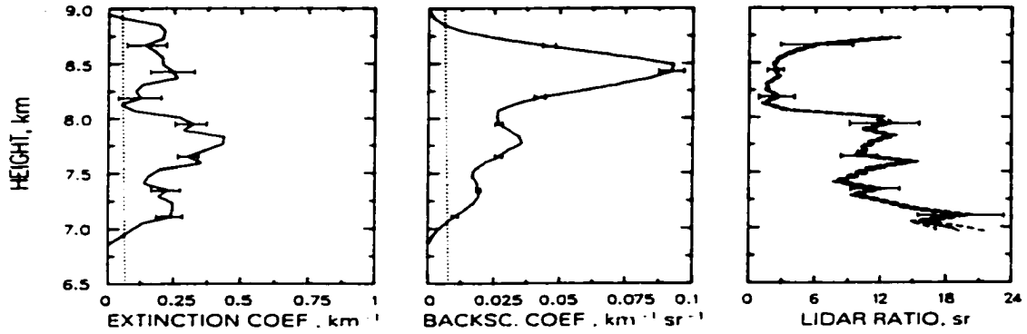
Figure 3.1: Raman lidar measurements of aerosol properties (From Ansmann et al., 1992a).
