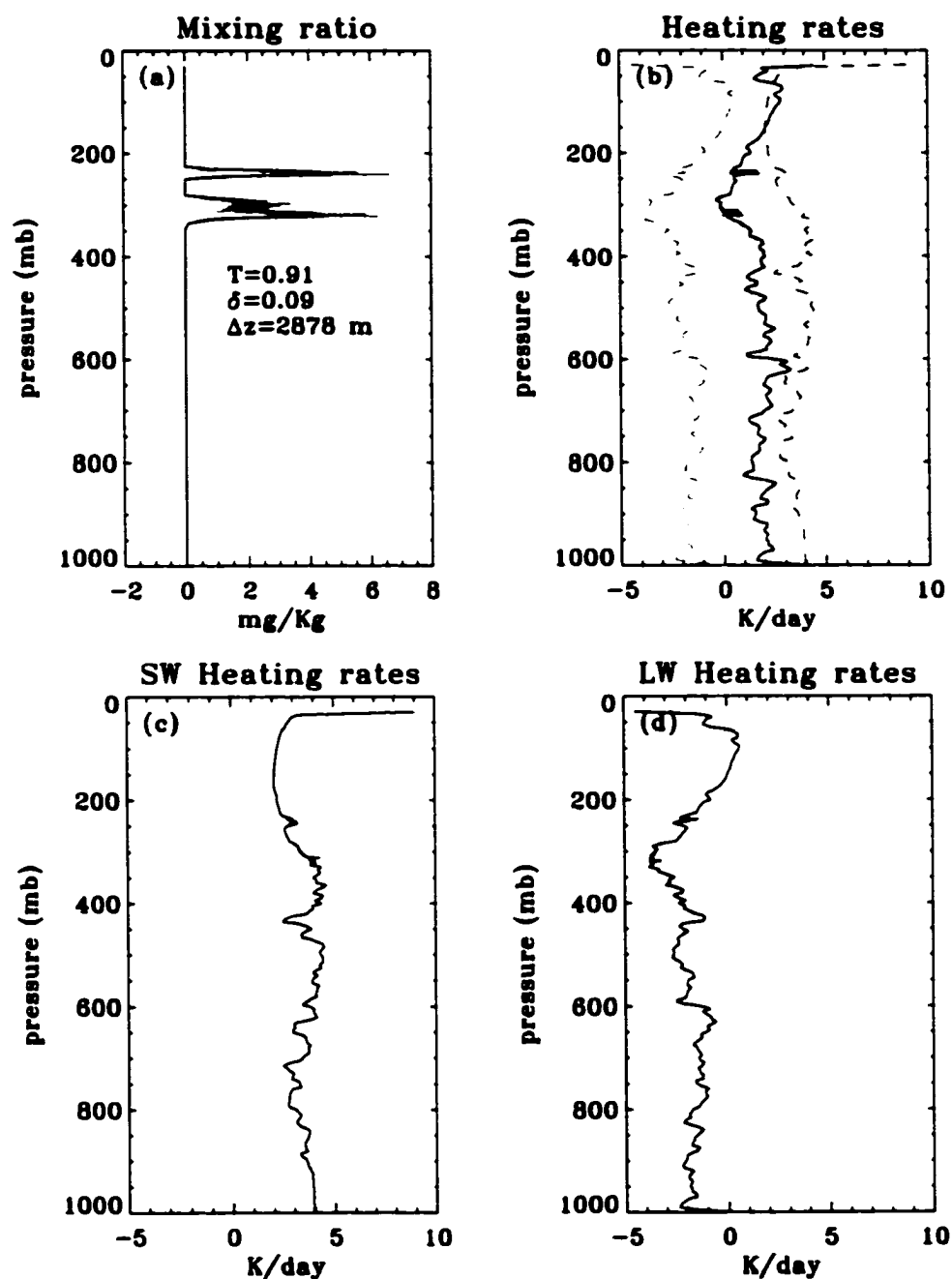
Figure 6.7: Cloudy sky heating rates and variations due to errors in mixing ratio: (a) Mixing ratio: (b) Total heating rate: (c) SW heating rate: (d) LW heating rate. In (a), cloud transmittance, optical depth and thickness are displayed. Nauru 1999 05 01 -- 10:00 UTC.
