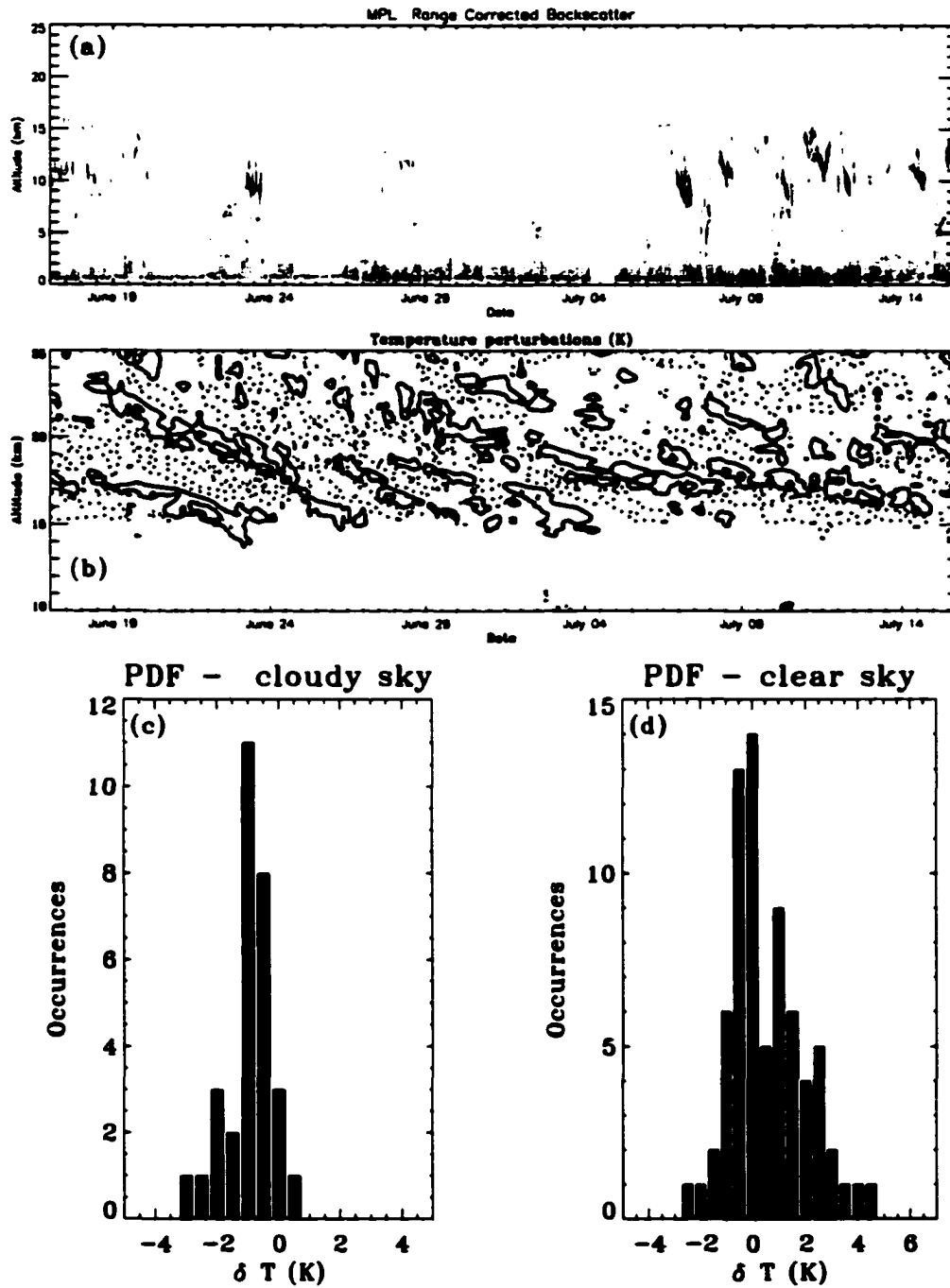
Figure 3.22: Waves interacting with cirrus clouds: (a) MPL time variation: (b) Temperature perturbations (2 K contours) time variation: (c) PDF: cloudy sky events vs. Temperature perturbations: (d) PDF: clear sky events vs. Temperature perturbations.
