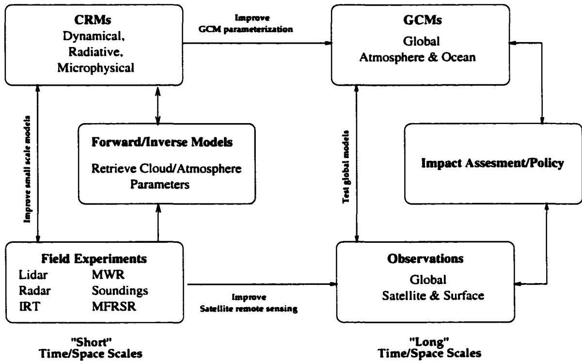
Figure 1.2: Observational strategy for the determination of the role of clouds and radiation in climate (After Wielicki et al., 1995)
