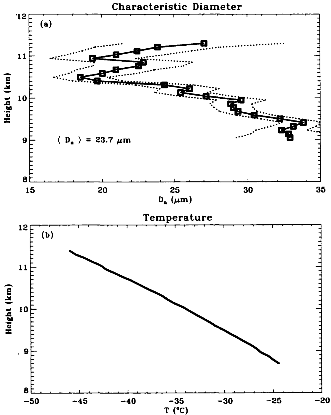
Figure 4.7: Profiles of (a) Characteristic Diameter ( D_n ), and (b) Temperature. Errors associated with the retrieval are shown by dots. Nauru 1999/05/21 08:22:09 UTC.
