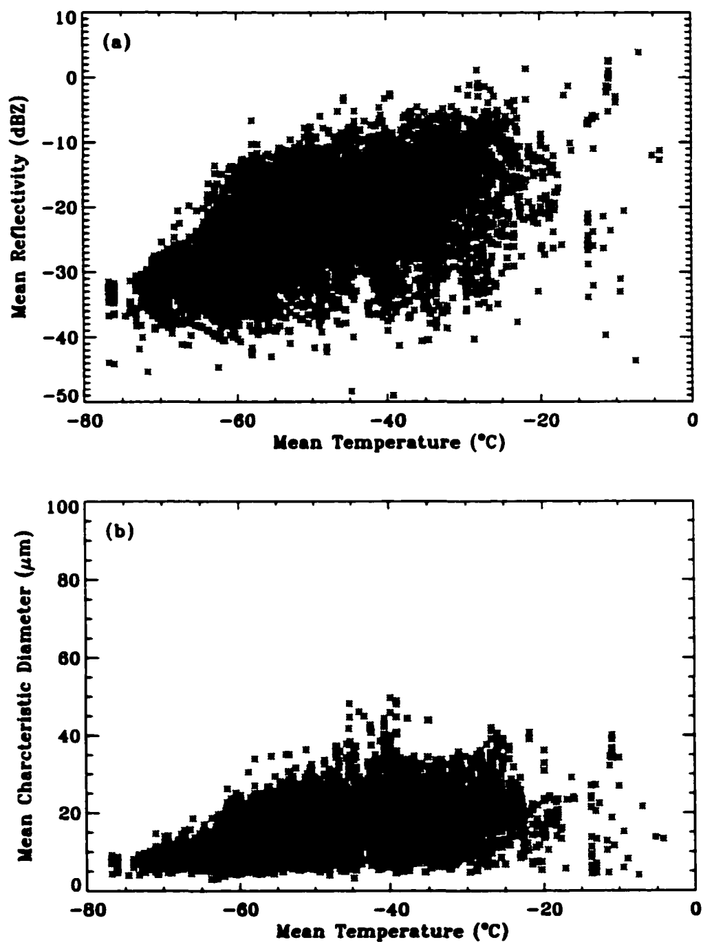
Figure 4.12: (a) Mean Radar Reflectivity vs. Temperature; (b) Mean Characteristic Diameter vs. Temperature. Nauru 1999 May-July.
