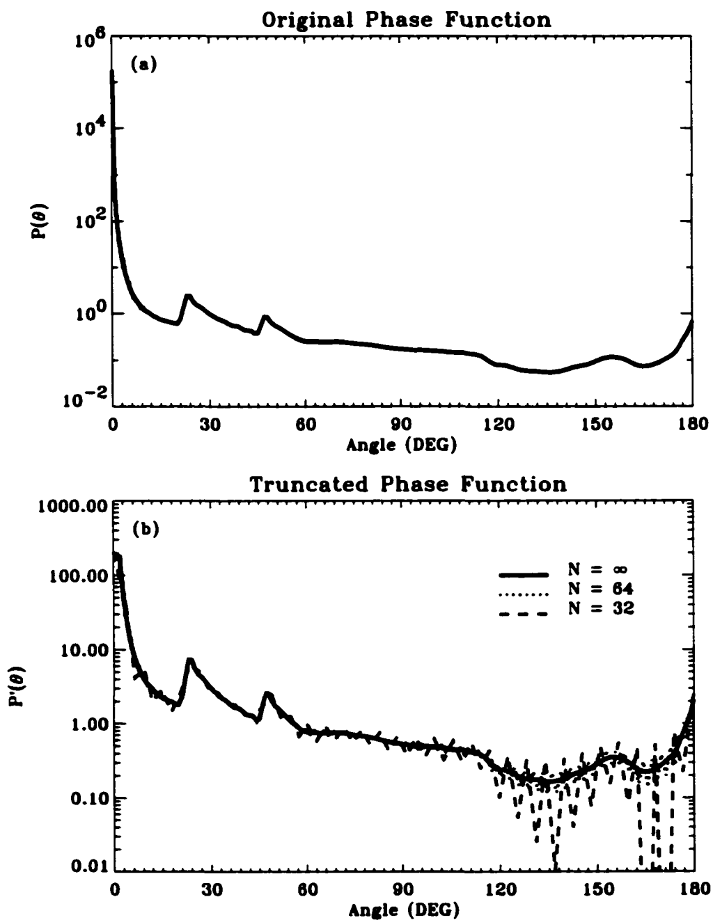
Figure 5.5: (a) Original Phase Function; (b) Truncated Phase Function (solid line). Approximation using Legendre Polynomials: dotted line for N = 64 ; dashed line for N = 32 .
