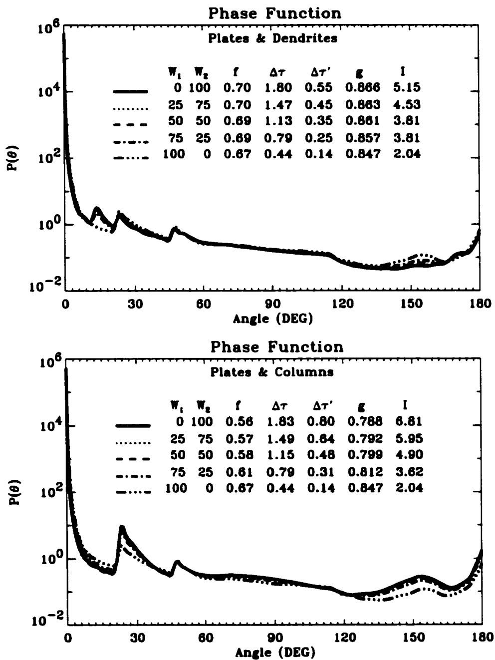
Figure 5.7: Sensitivity to particle habit and concentration: (a) Plates ( W_1 ) and Dendrites ( W_2 ); (b) Plates ( W_1 ) and Columns ( W_2 ). See text for explanations.
