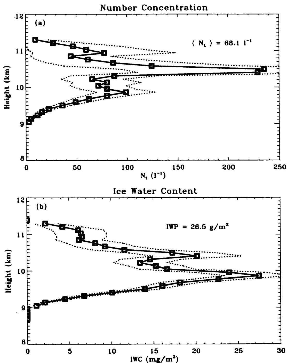
Figure 4.8: Profiles of (a) Number Concentration, and (b) Ice Water Content. Errors associated with the retrieval are shown by dots. Nauru 1999/05/21 08:22:09 UTC.
