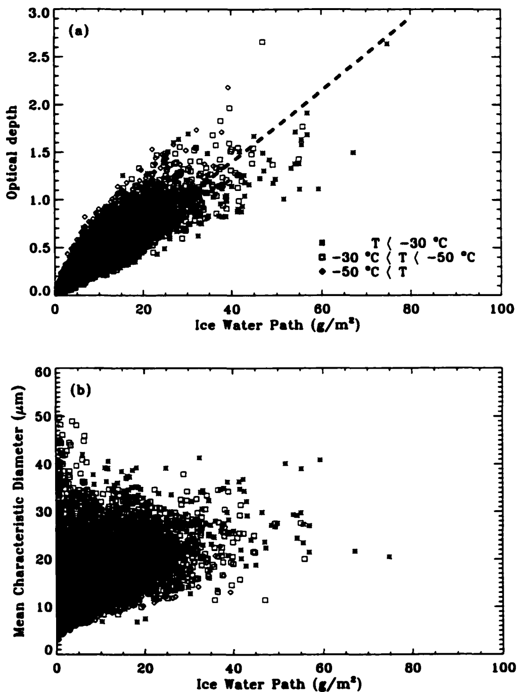
Figure 4.11: (a) Optical depth vs. Ice Water Path. With dashed line is the proposed parameterization (see text); (b) Mean Characteristic Diameter vs. Ice Water Path. Temperature dependence is according to Legend. Nauru 1999 May-July.
