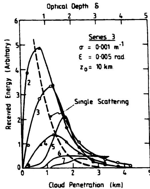
Figure 3.12: The relative received energies in different orders of scattering. (After Platt, 1981)
