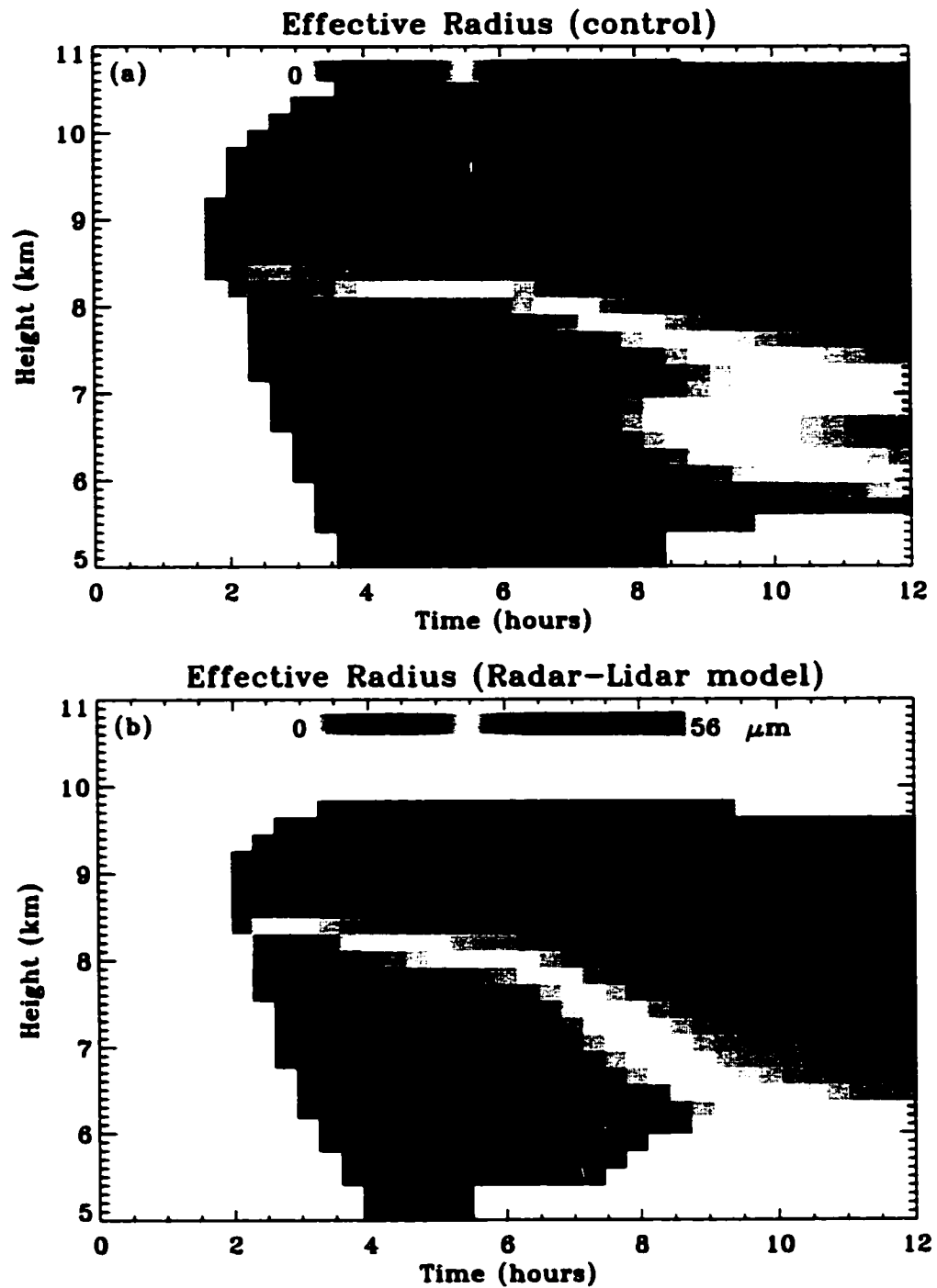
Figure 4.3: Comparison between (a) Control Effective Radius and (b) Retrieved Effective Radius.
