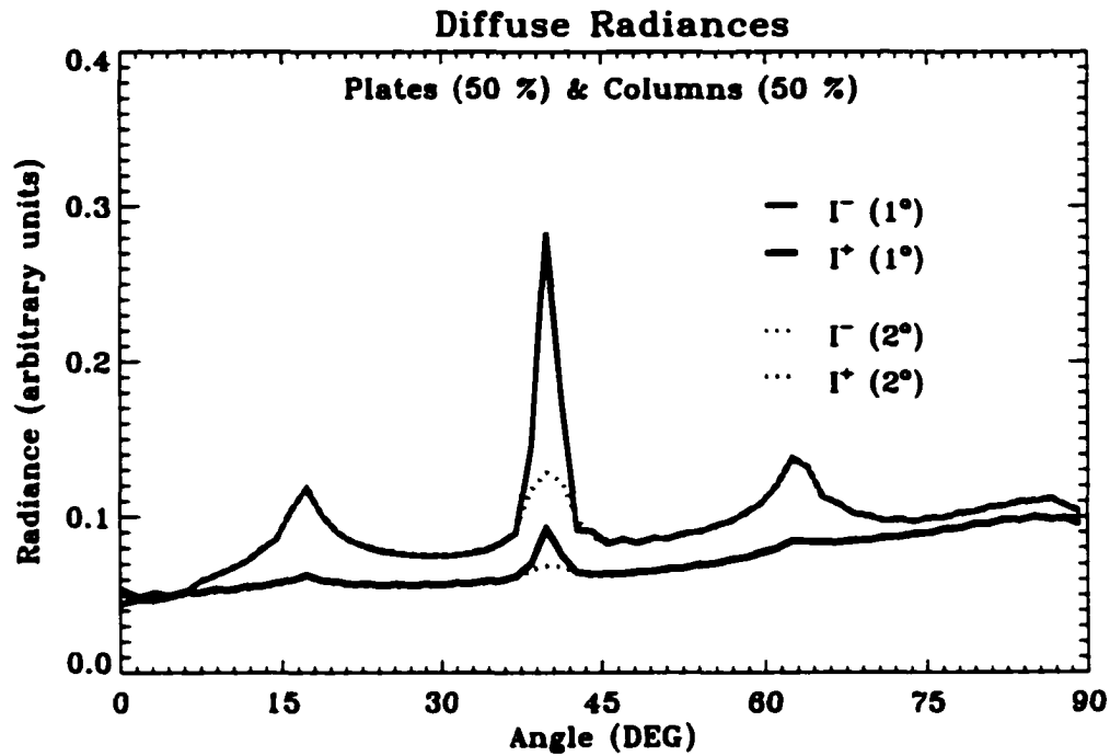
Figure 5.6: Diffuse radiances at top ( I^+ ) and base ( I^- ) of the cloud layer for two forward angles: \theta = 1^\circ and \theta = 2^\circ respectively.
