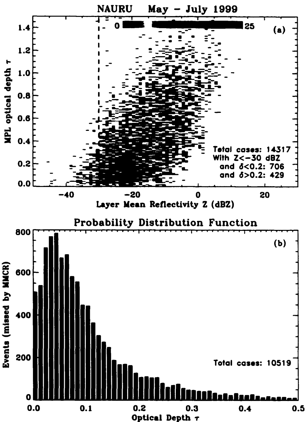
Figure 4.13: (a) Scatter plot of Layer Mean Reflectivity vs. MPL Optical Depth: (b) PDF of events missed by MMCR.
