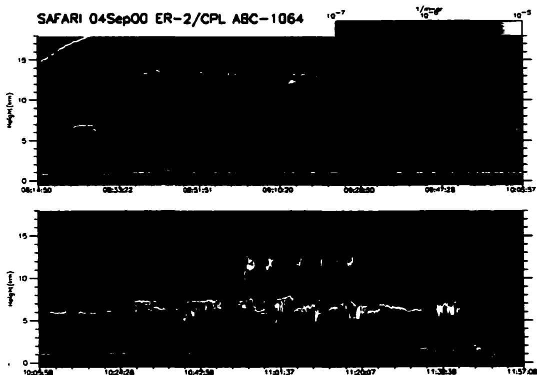
Figure 5.12: SAFARI 04 September 2000: CPL Data.
