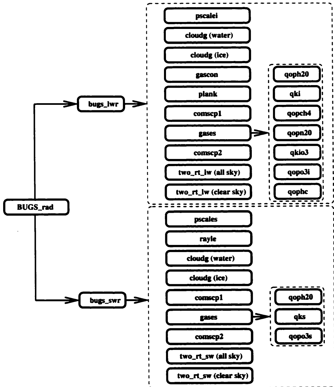
Figure 6.2: BUGS-Rad flow chart.
