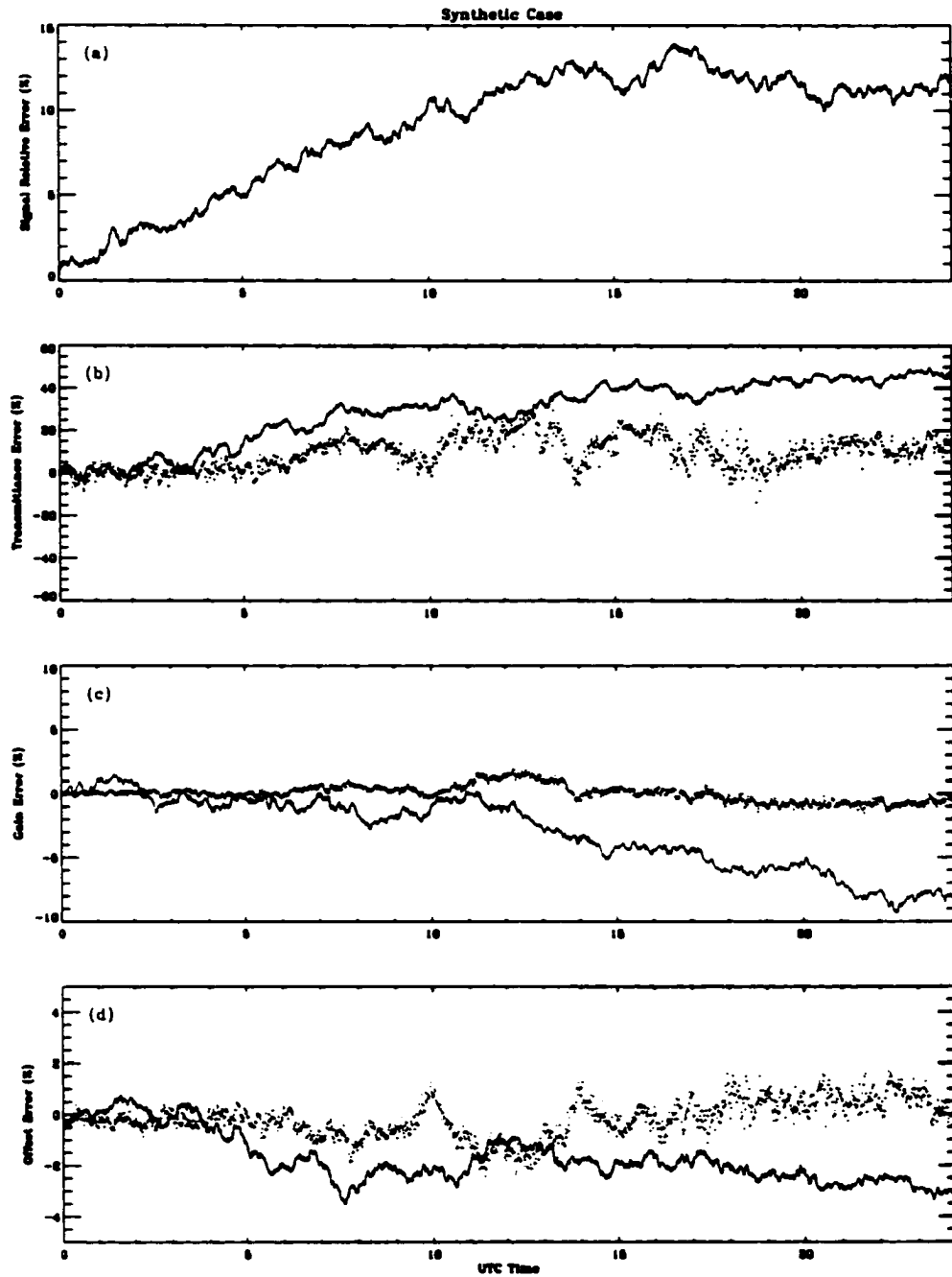
Figure 3.3: Synthetic Case: (a) Relative Error for the simulated signal; Errors in (b) Transmittance, (c) Gain and (d) Offset for the new method (dots) and old method (solid line). Shaded are the computed errors as explained in text for the new method.
