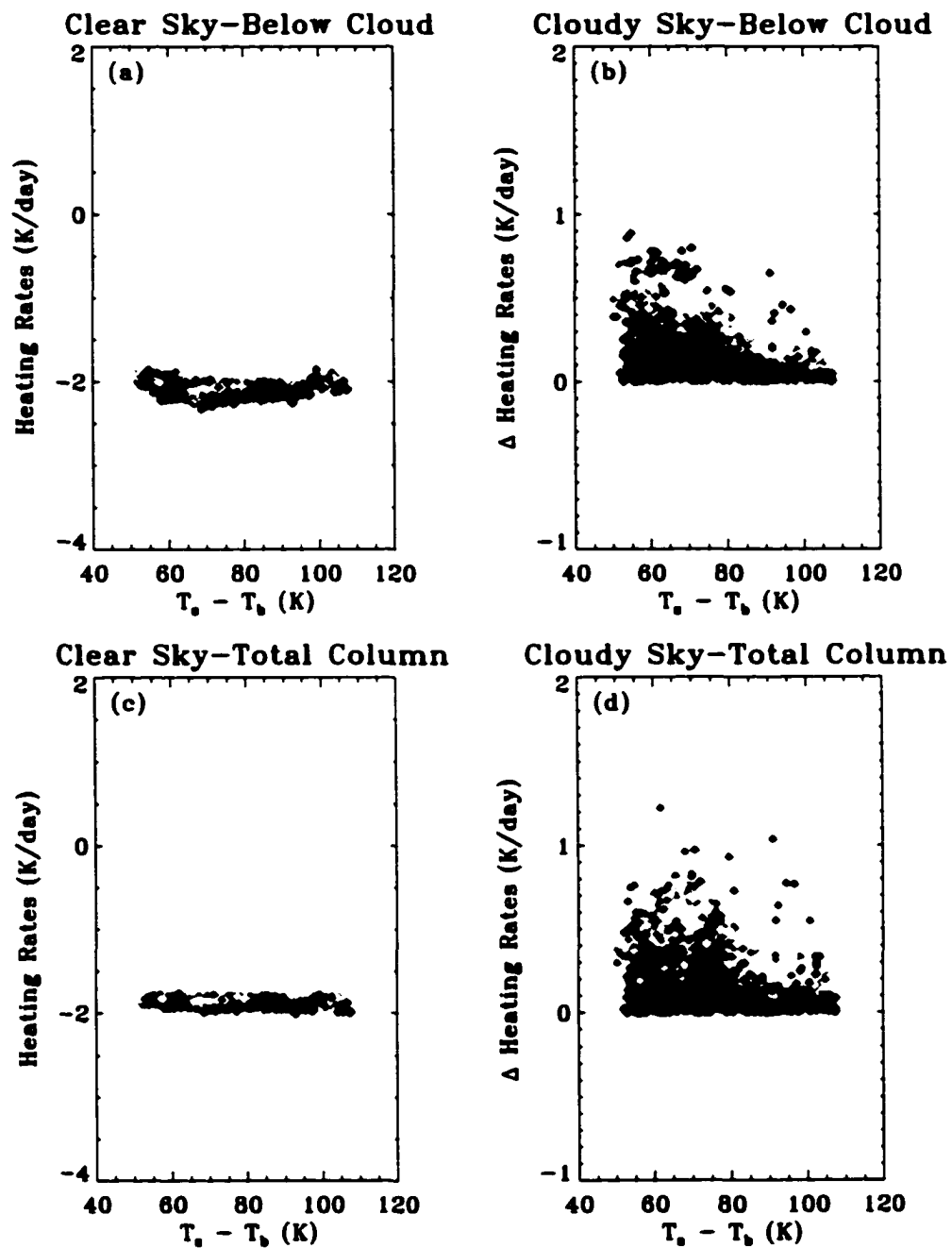
Figure 6.12: LW Heating rates vs. Temperature difference (surface - cloud) for different atmospheric regions. Simulated clear sky (left panels): Differences between cloudy and clear sky (right panels). Colors represent mean IWC values as in figure 6.10. Nauru 1999 06 18–1999 07 15.
