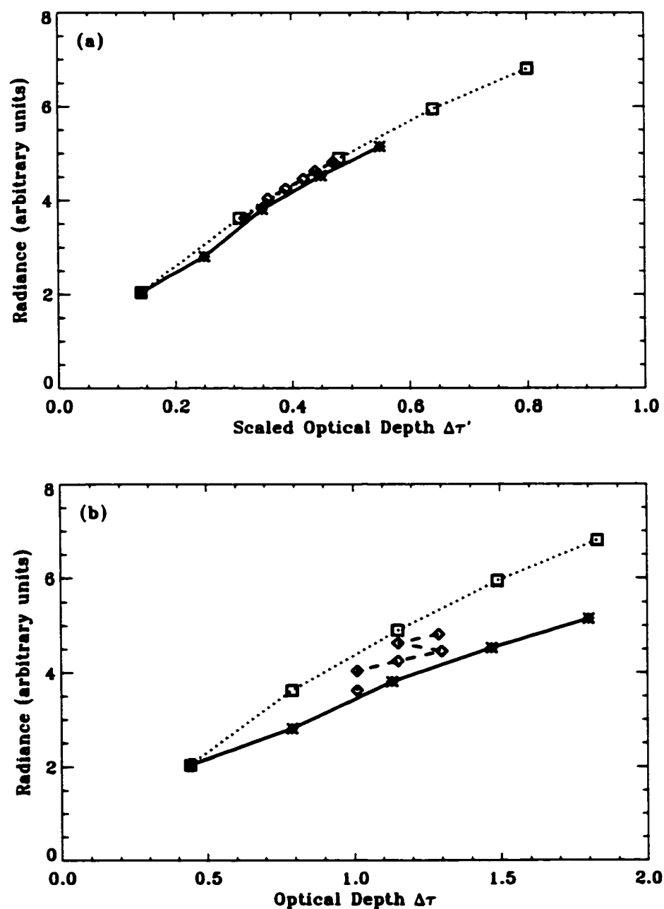
Figure 5.9: Radiances vs. (a) scaled optical depth or (b) optical depth for various ice crystals. Plates & Dendrites (solid line). Plates & Columns (dashed line). Plates & Columns & Aggregate (dotted line)
