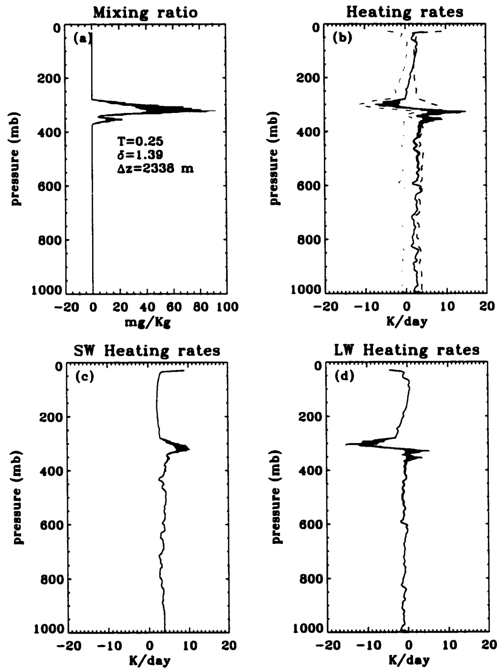
Figure 6.4: Cloudy sky heating rates and variations due to errors in mixing ratio: (a) Mixing ratio: (b) Total heating rate: (c) SW heating rate: (d) LW heating rate. In (a), cloud transmittance, optical depth and thickness are displayed. Nauru 1999 05 01 — 09:00 UTC.
