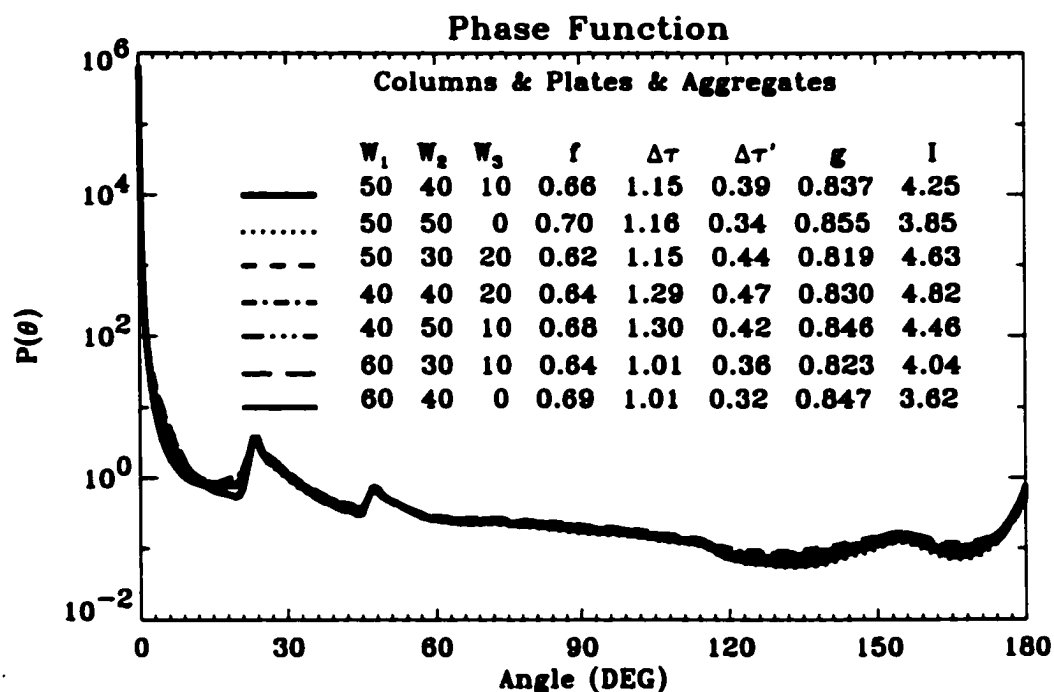
Figure 5.8: Sensitivity to particle habit and concentrations: Columns ( W_1 ), Plates ( W_2 ) and Aggregates ( W_3 ). See text for explanations.
