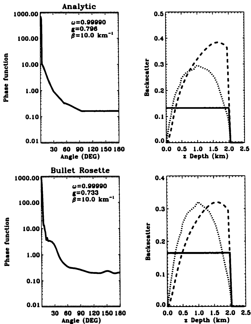
Figure 3.13: Multiple Scattering Contributions (right panels) to the Backscatter for a given Phase Function (left panels): first order (solid line), second order (dotted line), third order (dashed line).
