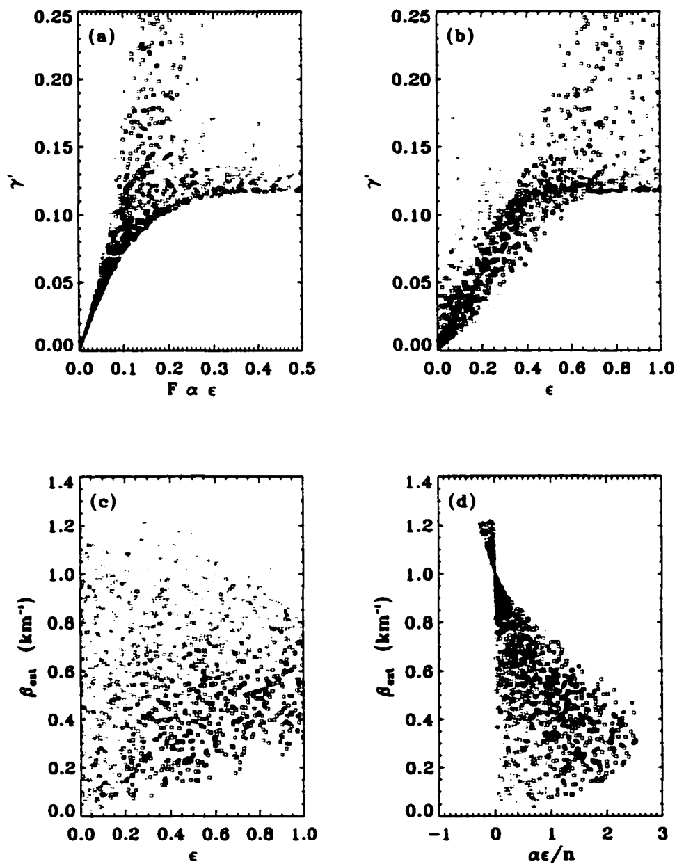
Figure 5.3: Synthetic data. (a), (b) Same as in figure 5.2 (a), (b). (c), (d) Domains of variations for the VIS extinction coefficient. Color coding as explained in text.
