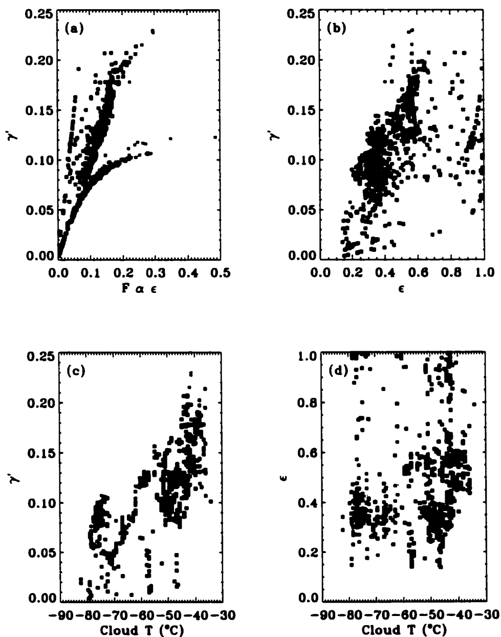
Figure 5.2: Observed data. (a) New representation: (b) Old representation: (c). (d) Variation of cloud properties with Mid-cloud Temperature. Color coding as explained in text. Nauru 1999 05 21
