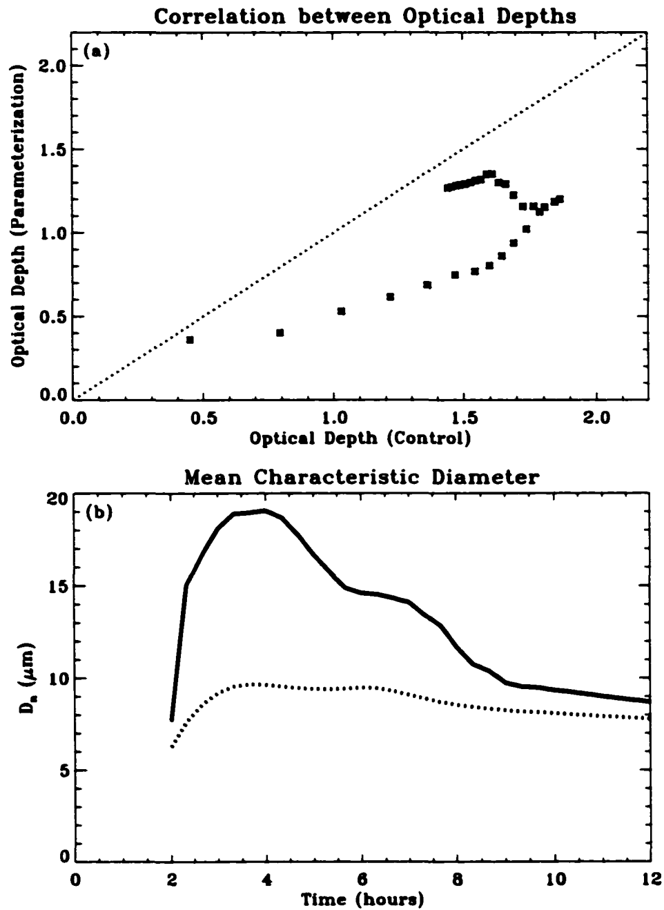
Figure 4.4: (a) Comparison between Control Optical Depth and Parameterized Optical Depth (with stars). Dotted line is the one-to-one relationship; (b) Time variation for Model Mean Characteristic Diameter (solid line) and Control Mean Characteristic Diameter (dotted line)
