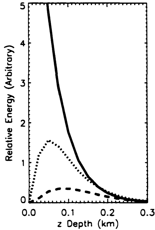
Figure 3.11: Relative energy from different orders of scattering for the “analytical” phase function: first order (solid line), second order (dotted line), third order (dashed line).
