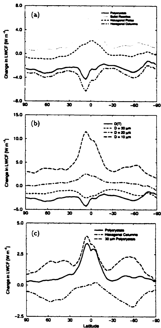
Figure 1.3: Change in the zonal mean LW cloud forcing due to a new ice optics scheme. (a) Effects of crystal shape and (b) of crystal size in CCM3. (c) Effect of shape and size in UKMO. (From Kristjansson et al., 2000)
