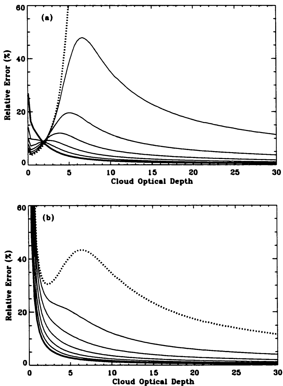
Figure 5.13: Best relative errors for retrieved cloud optical depth as function of albedo (5 % (thick solid line), 95 % (thick dotted line) in 15 % increments) in the presence of aerosol (b) or without aerosol (a). Aerosol optical depth was set to 0.8
