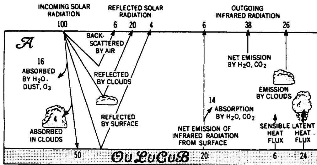
Figure 1.1: Schematic diagram of the global radiation budget in the climatic system. (From Peixoto and Oort, 1995)
