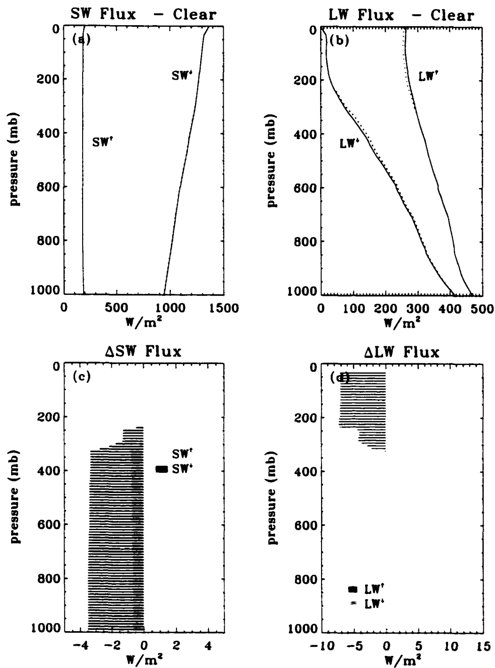
Figure 6.8: (Simulated) Clear sky computed fluxes and variations between cloudy and (simulated) clear sky: (a) SW fluxes: (b) LW fluxes: (c) \Delta SW fluxes: (d) \Delta LW fluxes. Nauru 1999 05 01 10:00 UTC.
