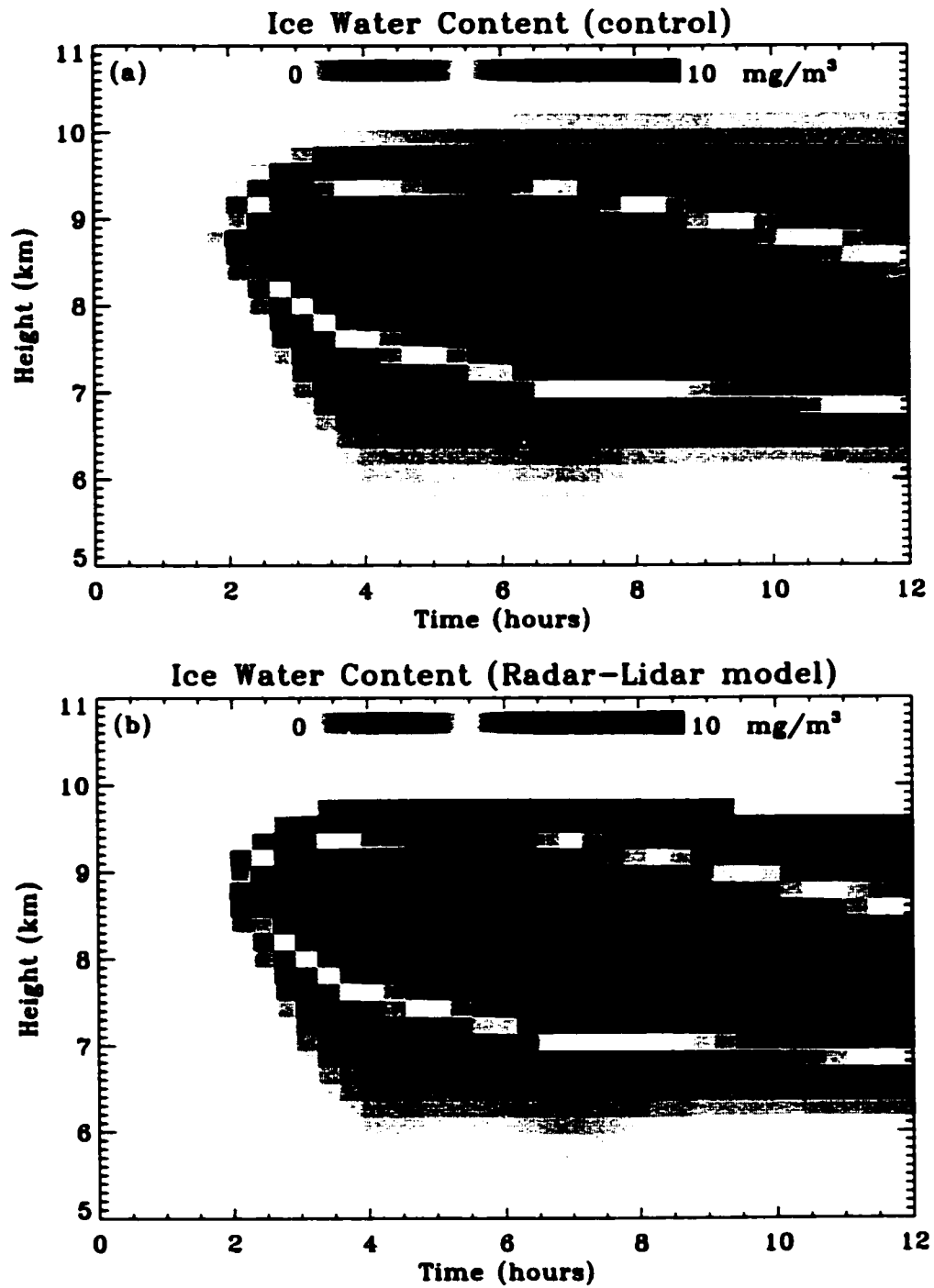
Figure 4.2: Comparison between (a) Control Ice Water Content and (b) Retrieved Ice Water Content.
