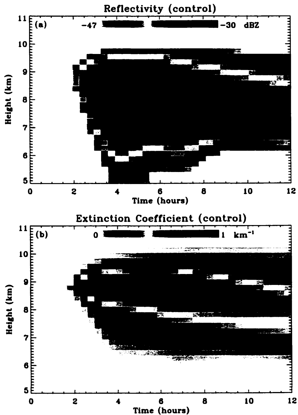
Figure 4.1: Input fields: (a) Radar Reflectivity; (b) Lidar Extinction Coefficient.
