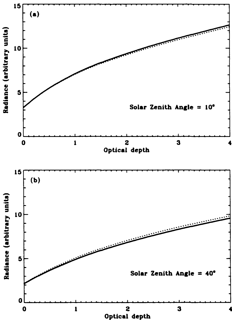
Figure 5.11: Two-layer cloud sensitivities for two solar zenith angles and two configurations: variable layer at base (solid line), and variable layer at top (dashed line). Optical depth for fixed layer is 0.5.
