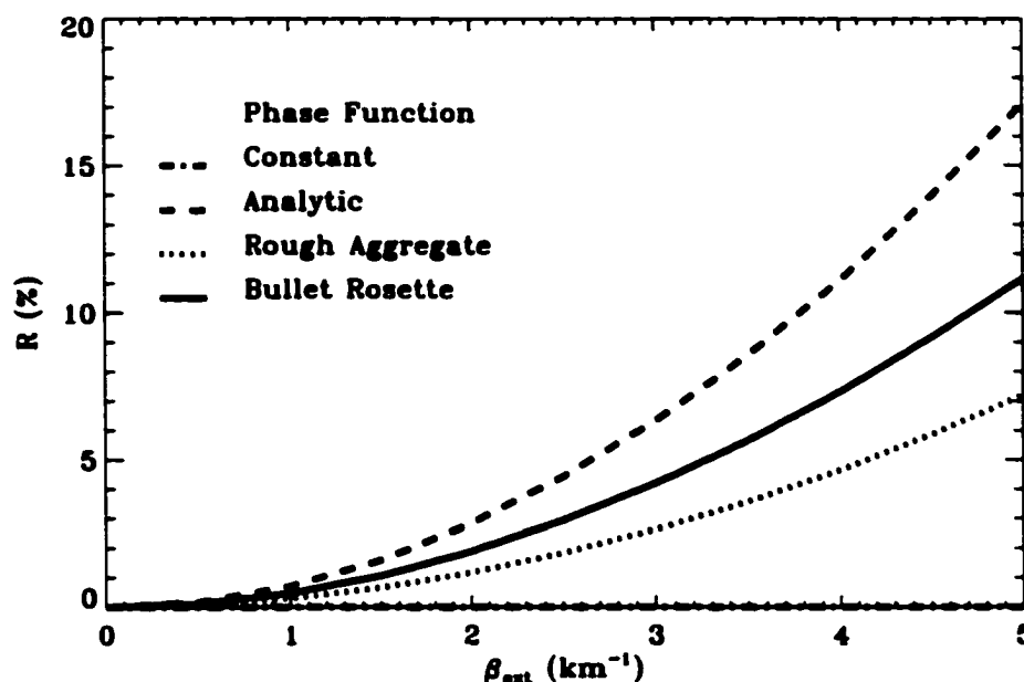
Figure 3.14: MS contributions to the received molecular backscatter signal from a region above the cloud as function of cloud extinction coefficient.
