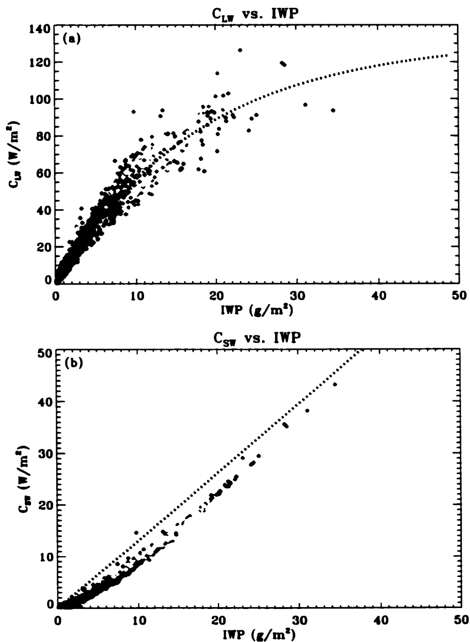
Figure 6.13: (a) LW and (b) SW cloud radiative forcing as function of IWP. Colors represent mean IWP values as in figure 6.10. With dotted lines are the proposed parameterizations as explained in text. Nauru 1999:06:18–1999:07:15.
