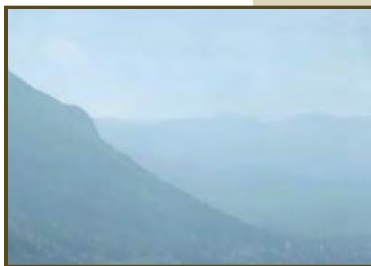
Figure 2. The same pollutants responsible for sulfur and nitrogen deposition also impair visibility, as shown in these photos from the IMPROVE network. In Rocky Mountain National Park, visibility is impaired to some degree 90% of the time. Viewing distance in the summer months averages 83 miles but can drop to 30 miles on high pollution days.
