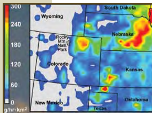
Figure 6. Regional ammonia emissions from livestock and agricultural sources.
