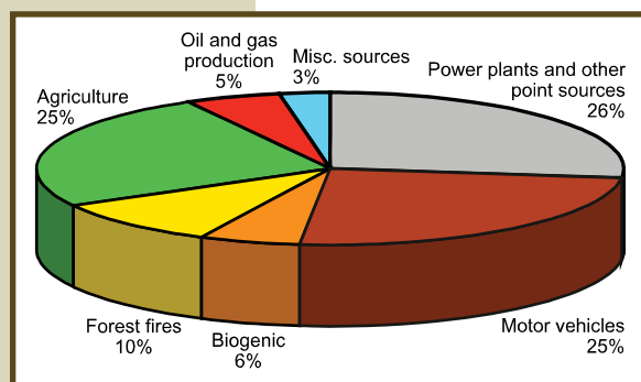
Figure 5. Nitrogen emissions from sources within Colorado, consisting primarily of contributions from power plants and other point sources (26%), agriculture (25%) and motor vehicles (25%).
