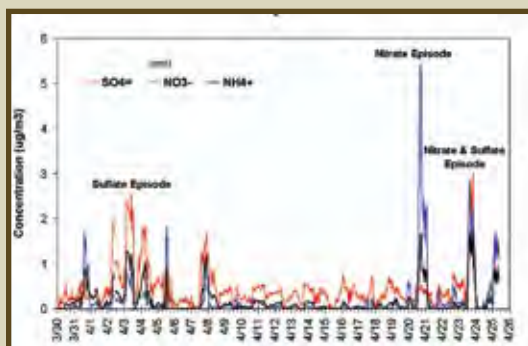
Figure 4. Measured sulfate ( \text{SO}_4 ), nitrate ( \text{NO}_3 ) and ammonium ( \text{NH}_4 ) concentrations at the core sampling site at RMNP during the spring field campaign. Understanding which emission sources contribute to these pollutant concentrations will be the primary goal of ROMANS.
