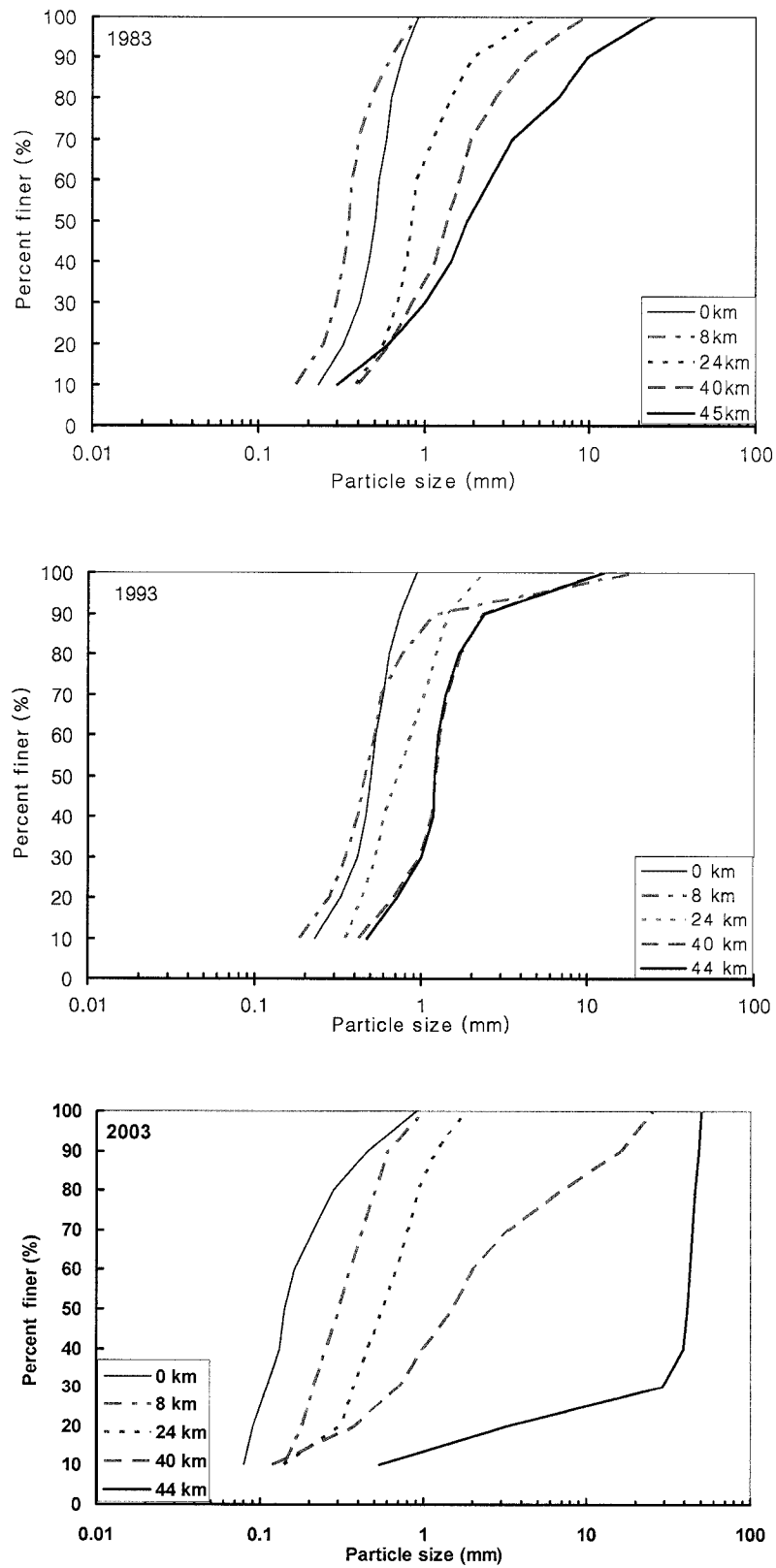
Figure 4-15. Particle size distributions along the study reach in 1983, 1993, and 2003
