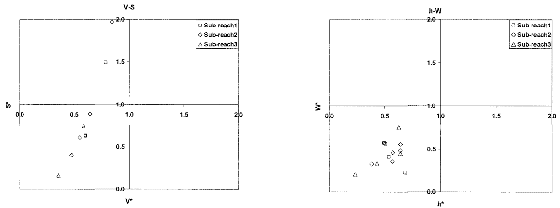
Figure D-4. Downstream change for the Hwang River below the Hapcheon Re-regulation Dam plotted on the response domain from Figure 7-2 for the V^* - S^* and h^* - W^* as function of dominant discharge, bed load discharge and grain diameter
