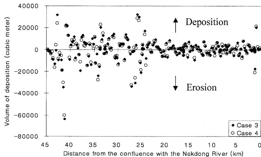
Figure 6-28. The cumulative volumes of erosion and deposition ( \text{m}^3 ) by the flood peak (case 3) and flood average (case 4) along the study reach
