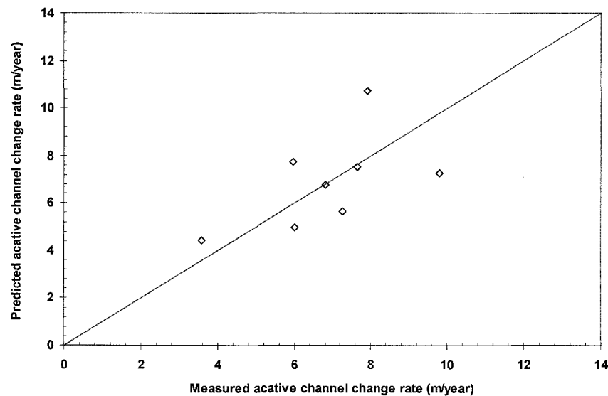
Figure C-1. Validation result of active channel width change rate for 1983~2003 of the sub-reach and entire reach by the equation (C-2)
