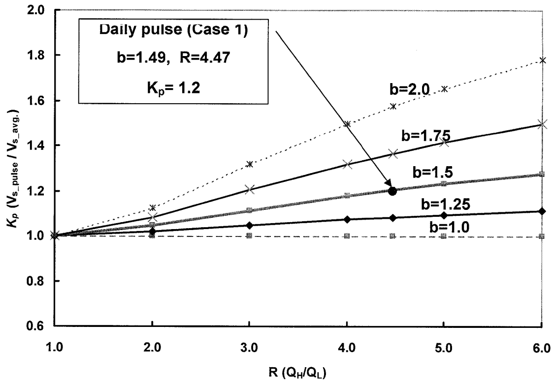
Figure 6-26. Variation of ratio the sediment volume by flow pulse to the sediment volume by average flow corresponding to the variation of b values
