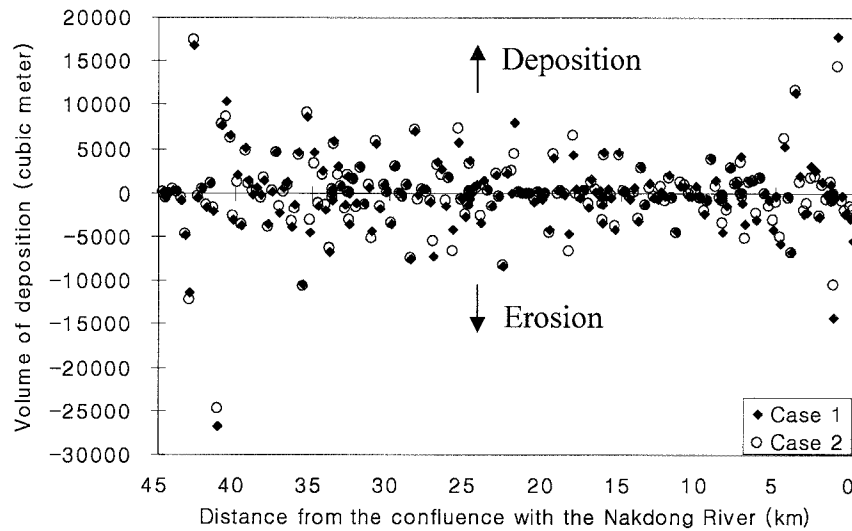
Figure 6-27. The cumulative volumes of erosion and deposition ( \text{m}^3 ) by the daily pulse (Case 1) and daily average (Case 2) along the study reach
