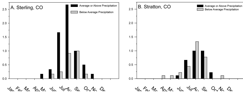
Figure 1.3. Monthly frequency of rainfall events \geq 13 \text{ mm hr}^{-1} for (A) Sterling and (B) Stratton. Frequency was determined separately for years with average or above average annual precipitation and years with below average precipitation.
