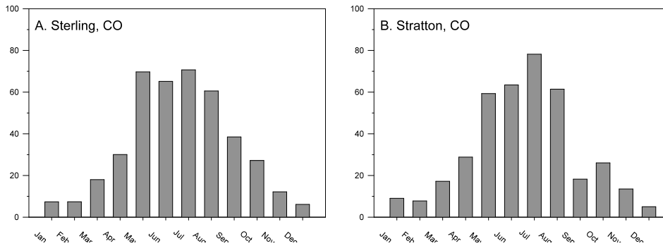
Figure 1.2. Average monthly precipitation in (A) Sterling and (B) Stratton, CO based on rainfall records from 1988 to 2006.
