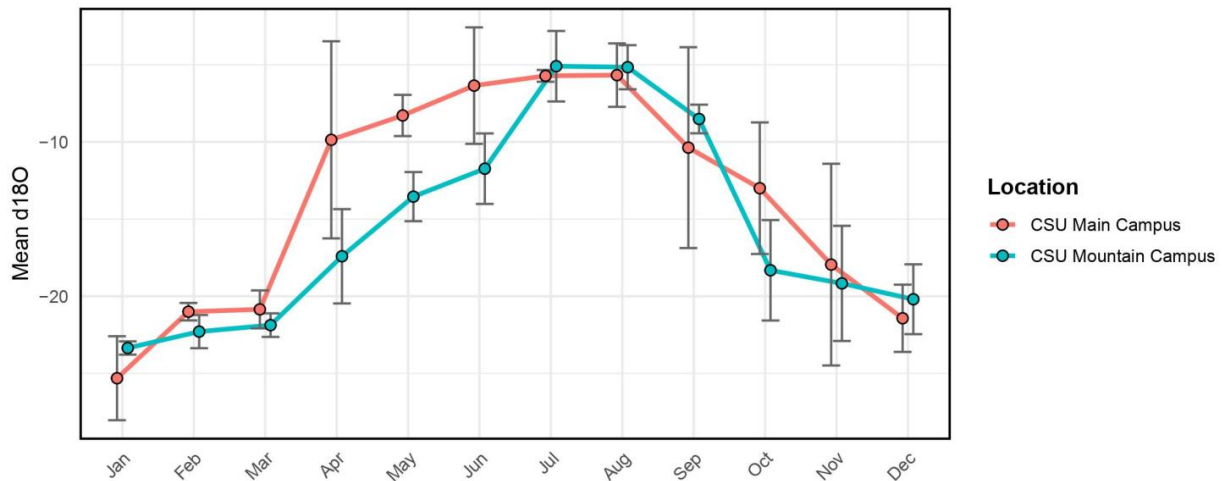
Figure 2-1. Monthly average precipitation \delta^{18}\text{O} values for the CSU Main Campus in Fort Collins and the CSU Mountain Campus in Pingree Park. Error bars show 1 S.D. from the mean.
