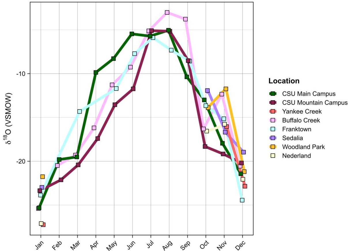
Figure 4-1. Precipitation mean \delta^{18}\text{O} values for all sampling locations. \delta^{18}\text{O} are highest in the summer and lower in the winter for all locations.
