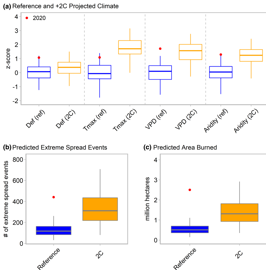
FIGURE 7 Reference period (1986–2015) versus future (+2°C) projections (a) for four climate variables [mean climatic water deficit (Def), mean maximum temperature (Tmax), mean vapour pressure deficit (VPD) and Aridity (defined in the main text as the average of the other three variables)]; (b) predicted number of extreme events >1,100 ha/day; and (c) annual area burned. Red dots represent observed climate and fire activity in 2020
