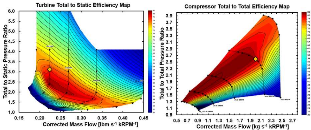
Figure 4-7 Turbine (Left) and compressor (Right) performance maps with reference conditions
