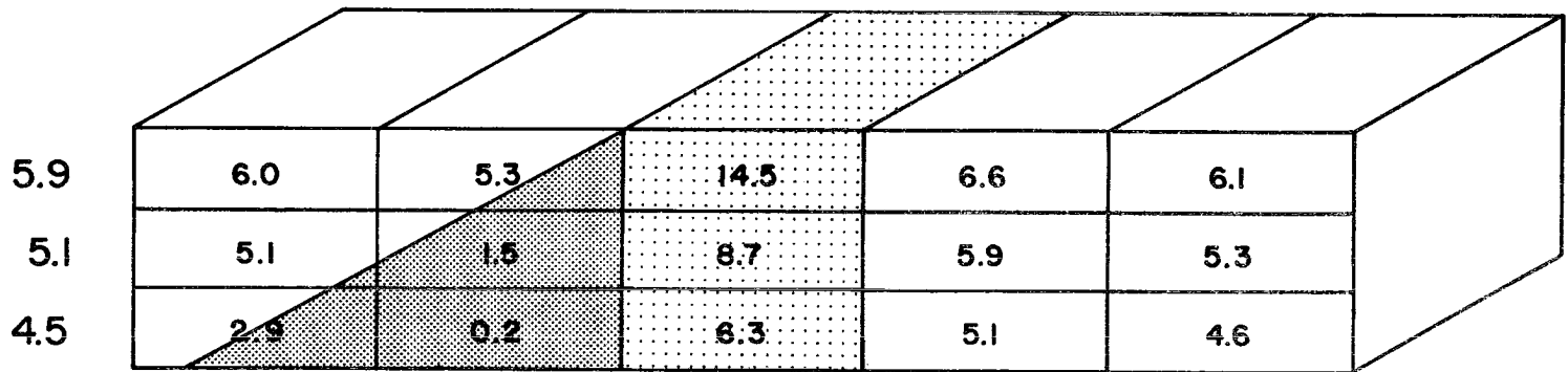
Figure 16. Solar absorption values in \text{watts}\cdot\text{m}^{-2} for the regions surrounding the 210 m (top) and 630 m thick (bottom) finite clouds for a 60^\circ zenith angle. Also given are cloud free layer values (left) and in cloud layer values (center).
