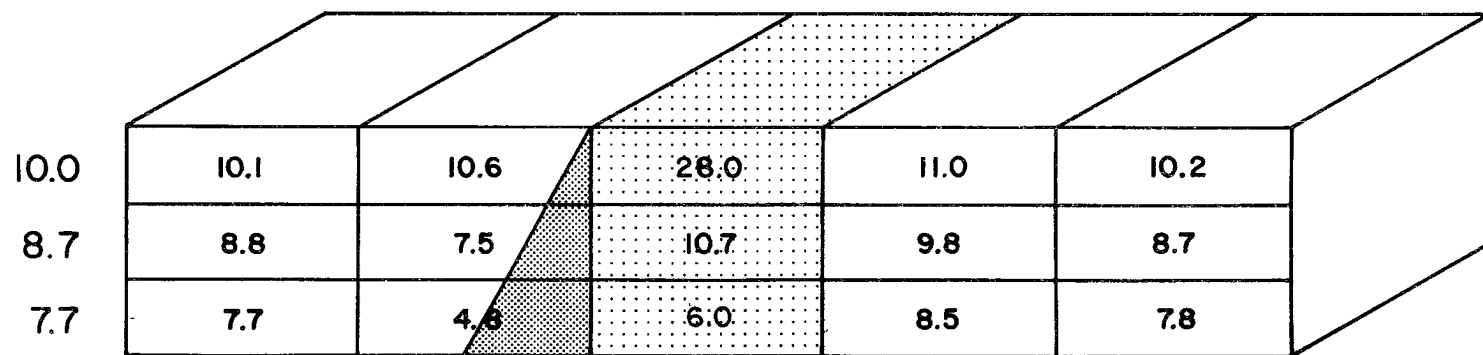
Figure 15. Solar absorption values in \text{watts}\cdot\text{m}^{-2} for the regions surrounding the 210 m (top) and 630 m thick (bottom) finite clouds for a 30^\circ zenith angle. Also given are cloud free layer values (left) and in cloud layer values (center).
