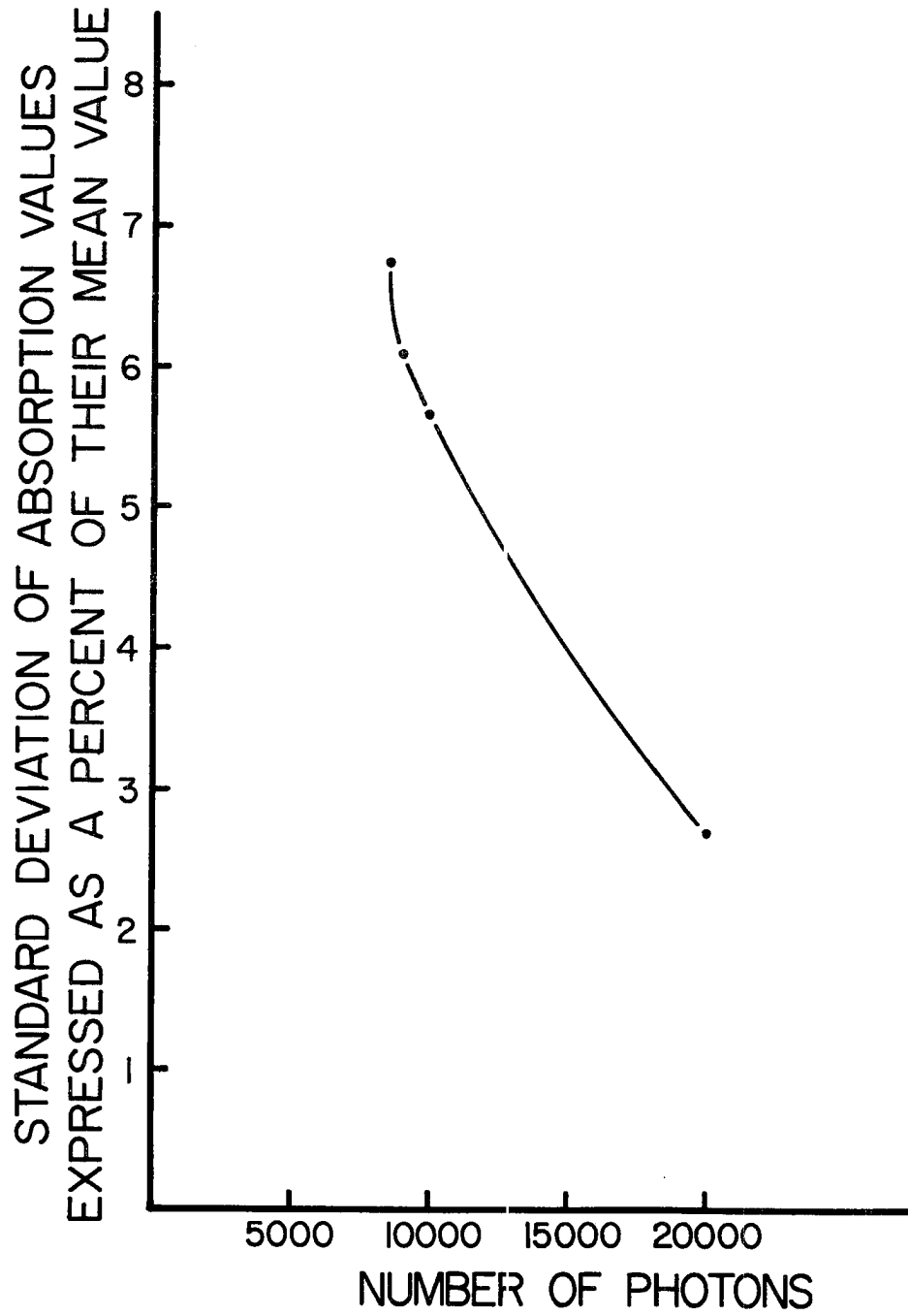
Figure 6. Standard deviation of absorption values expressed as a percent of their mean value vs. number of photons used in the calculation.
