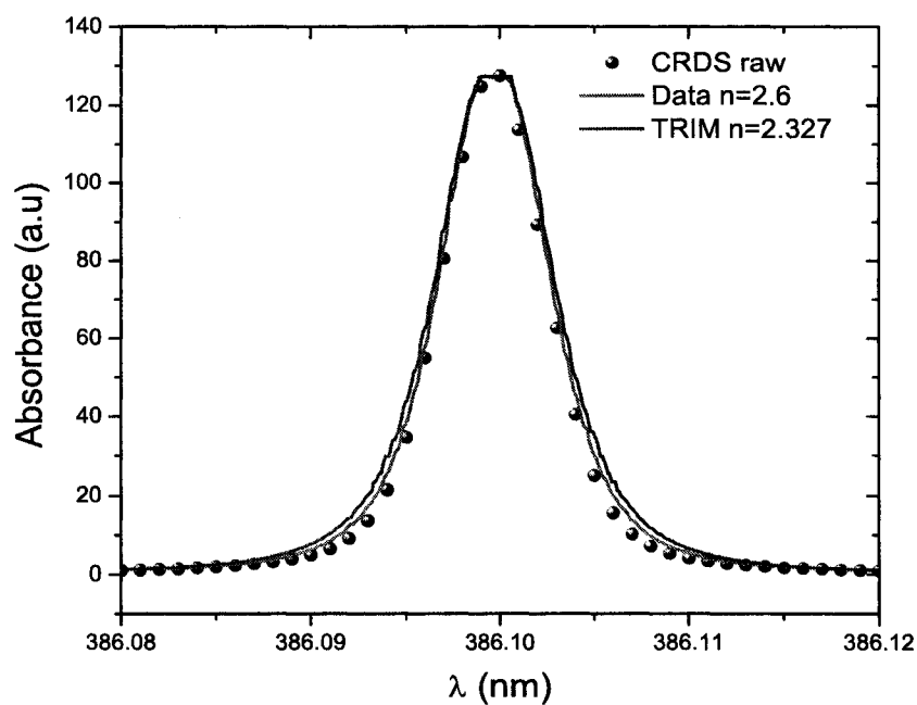
Figure 3.14: Comparison of CRDS measured lineshape with the sputter model predicted lineshape using LIF measured profile as the velocity distribution (instead of assuming the form of Eq.3.6)
