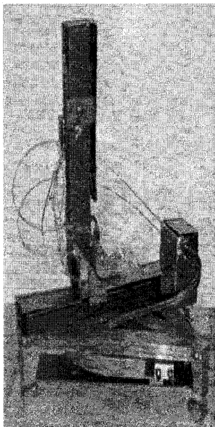
Figure A.1: Mechanical design of the system. Three stepper motors are used to position a Faraday probe in a three dimensional space.
