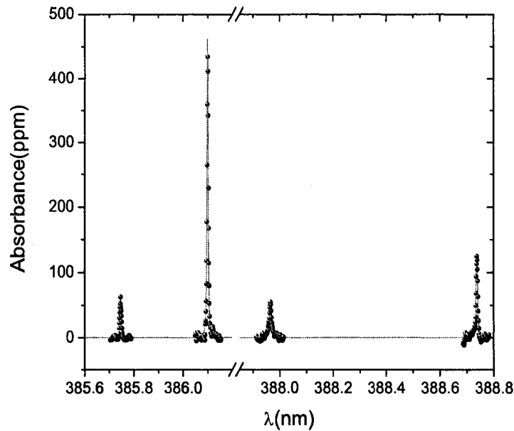
Figure 2.5: Iron absorbance spectrum recorded by CRDS.
