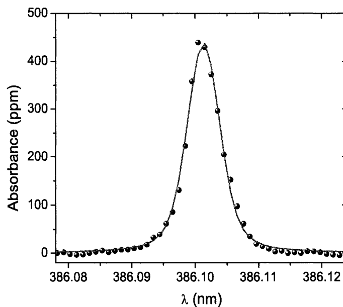
Figure 5.5: Iron absorbance spectrum from Fe-Mn target recorded by CRDS.
