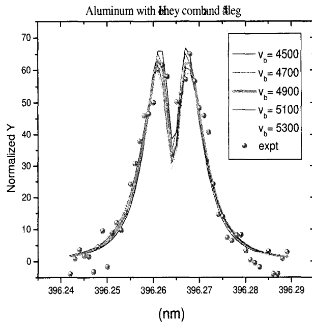
Figure 3.6: Al velocity measurements: Symbols - measured lineshape; Thick lines - modeled fit with V_b ranging from 4500 m/s to 5300 m/s
