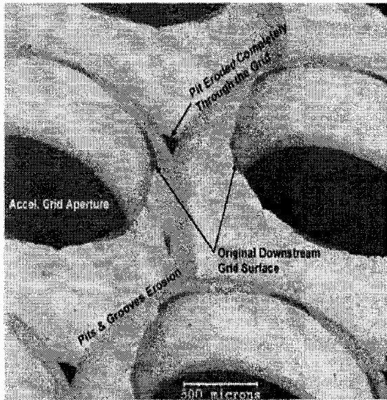
Figure 1.2: Accelerator grid from the NSTAR ELT thruster showing significant sputter erosion. In addition to limiting lifetime, the sputtered material can be re-deposited onto sensitive spacecraft surfaces causing contamination
