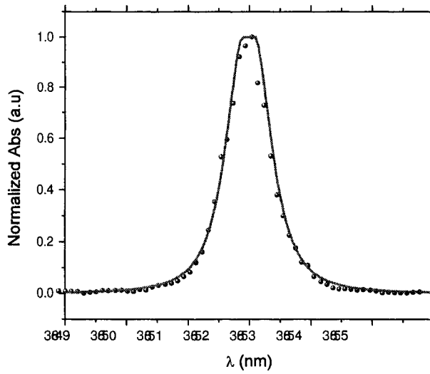
Figure 4.9: CRDS absorbance spectrum (symbols) of sputtered molybdenum at Y_b=0 , and Z=2 cm. Curve shows modeled lineshape for (best-fit value of) V_b = 3700 m/s.
