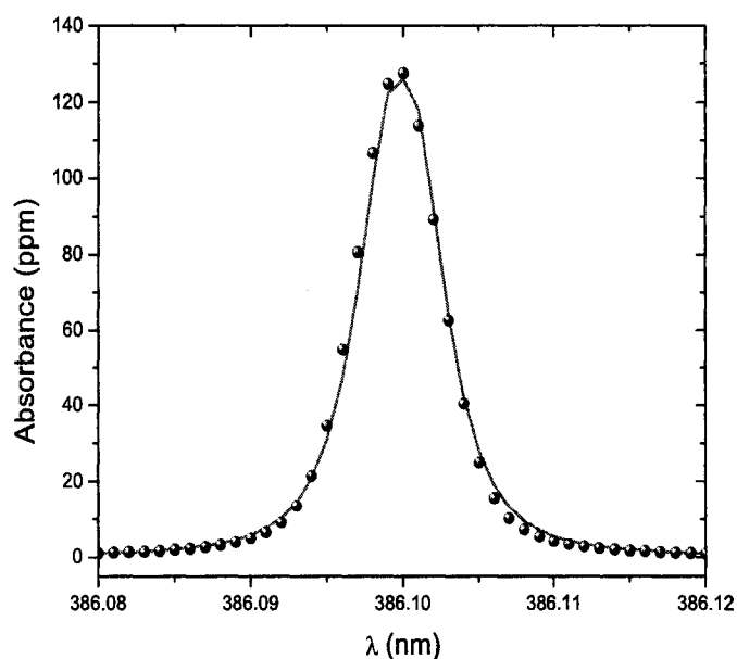
Figure 3.9: Fe absorbance lineshape: Symbols - measured lineshape; Thick line - modeled fits with V_b=2900 m/s;
