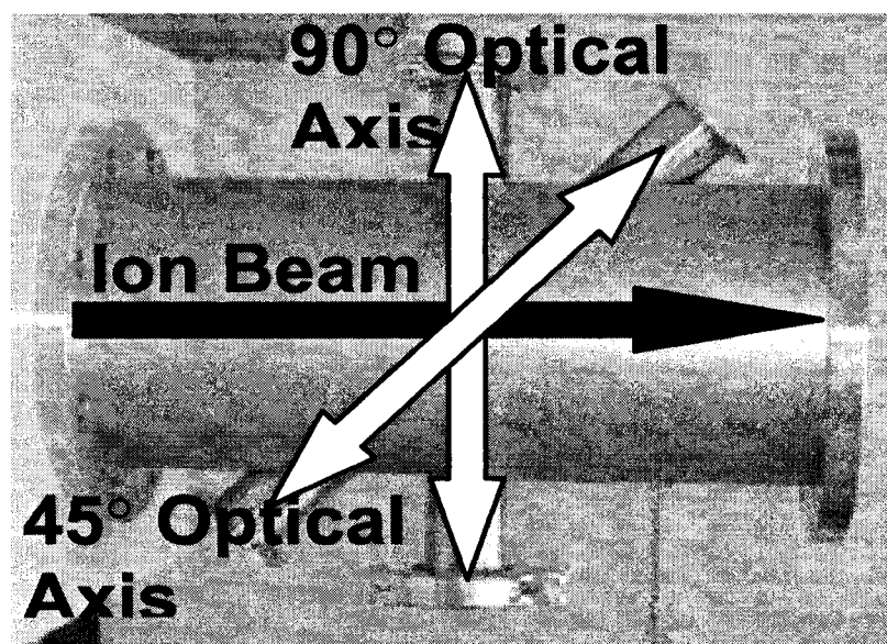
Figure 3.2: Vacuum chamber with arms for 2 optical axes with different angles.
