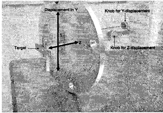
Figure 4.2: Photograph of the target mounting system. The target is in the X-Y plane and can be moved in the Y direction and in the Z-direction.
