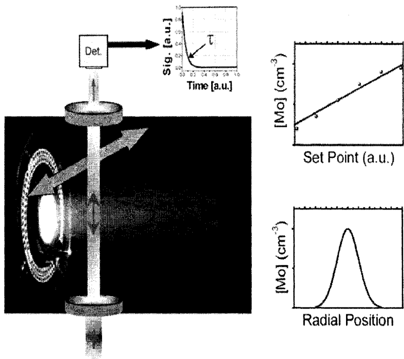
Figure 7.1: Approach to CRDS measurements in plume of a thruster. A CRDS cavity will surround the plume (actually with horizontal orientation), and measure Mo within the plume.
