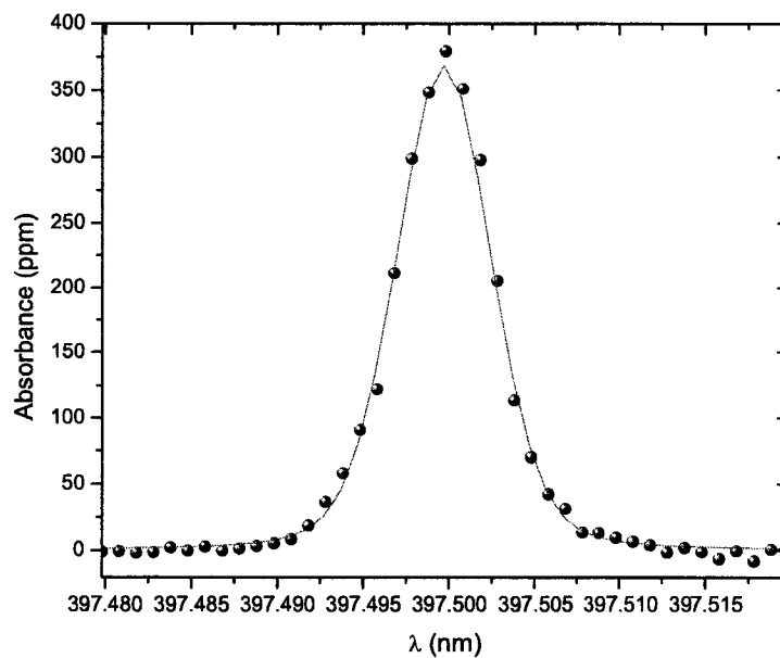
Figure 6.5: Sample absorbance spectrum collected with CRDS detection system at around 397.499 nm for probing the 0.938 eV level. Symbols: CRDS measurements. Solid line: fitted lienshape.
