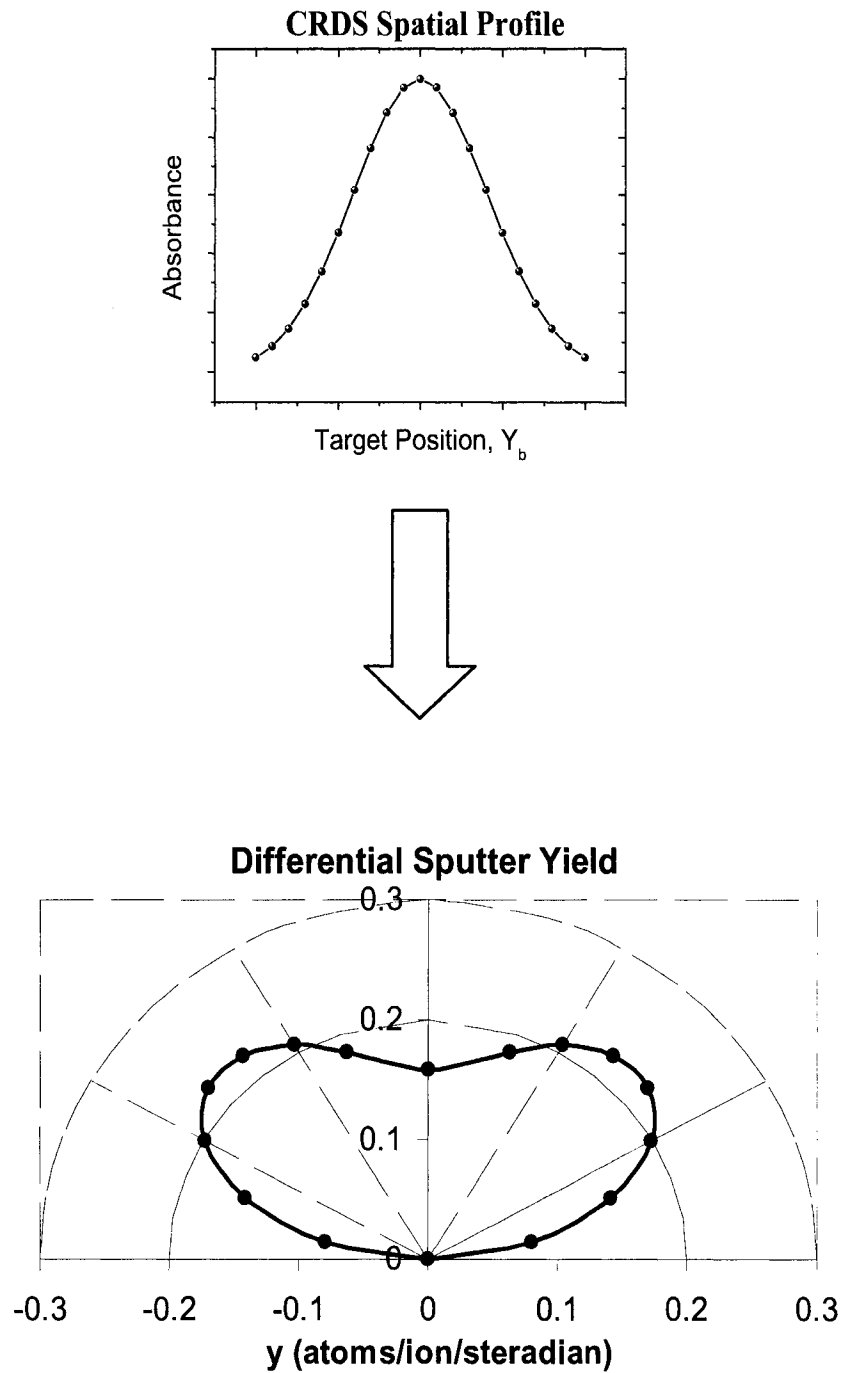
Figure 4.4: Left: The CRDS Spatial Profile is obtained by measuring the CRDS absorbance signal (Integral n \, dx ) at a series of displacements Y_b , between the target and optical axis. Right: The differential sputter yield, y(\alpha) , is inferred from the CRDS Spatial Profile.
