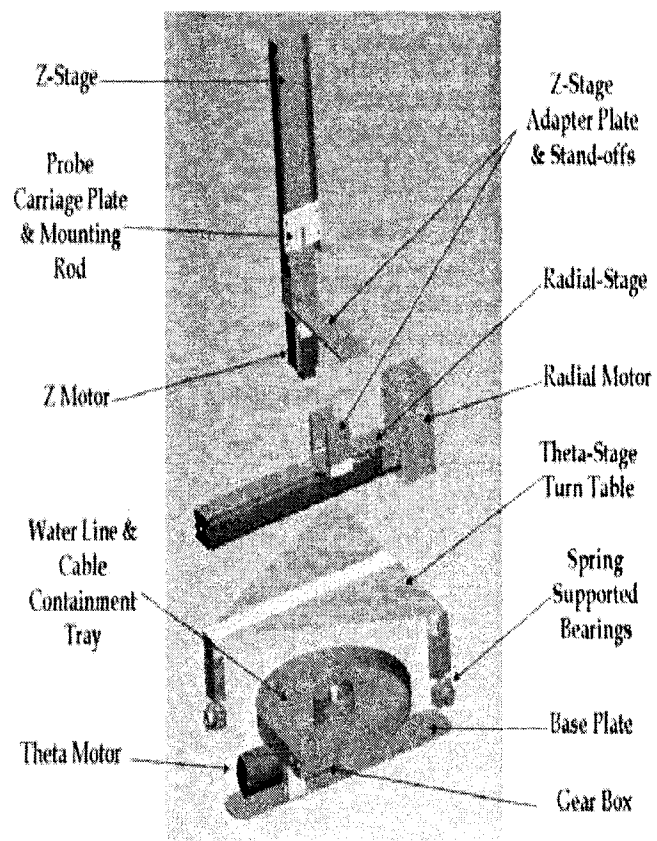
Figure A.1: Mechanical design of the system. Three stepper motors are used to position a Faraday probe in a three dimensional space.
