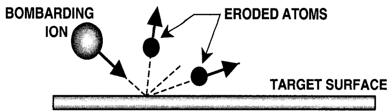
Figure 1.1: Schematic diagram of sputter erosion process. Ions bombard a target surface, and their impact causes atoms (and other particles) to be ejected due to sputtering.
