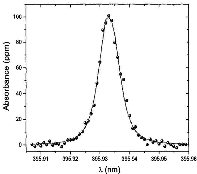
Figure 3.10: Ti absorbance lineshape: Symbols - measured lineshape; Thick line - modeled fits with V_b=4200 m/s;
