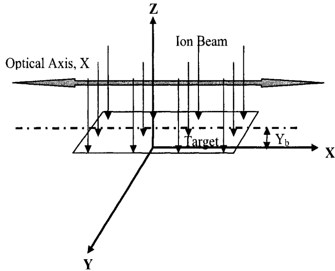
Figure 4.3: Definition of co-ordinate system used. The target is in the X-Y plane. The optical axis is at height Z above the target. The target can be moved in the Y direction and its position is denoted as Y_b .
