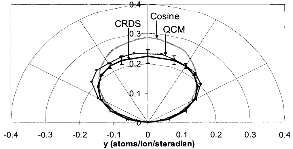
Figure 4.11: Comparison of differential yield profiles obtained at different Z 's for molybdenum with that of a regular cosine distribution and the actual QCM measured profile. One can clearly see the under cosine behavior of Mo.
