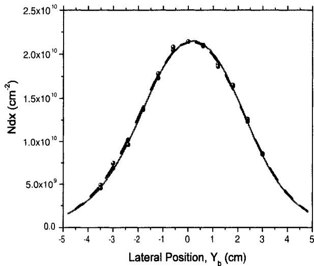
Figure 4.10: CRDS spatial profile of Mo: Symbols represent the experimentally measured points, solid line represents the best fit curve obtained from the model, and dashed line represents the curve obtained from the model using QCM coefficients.
