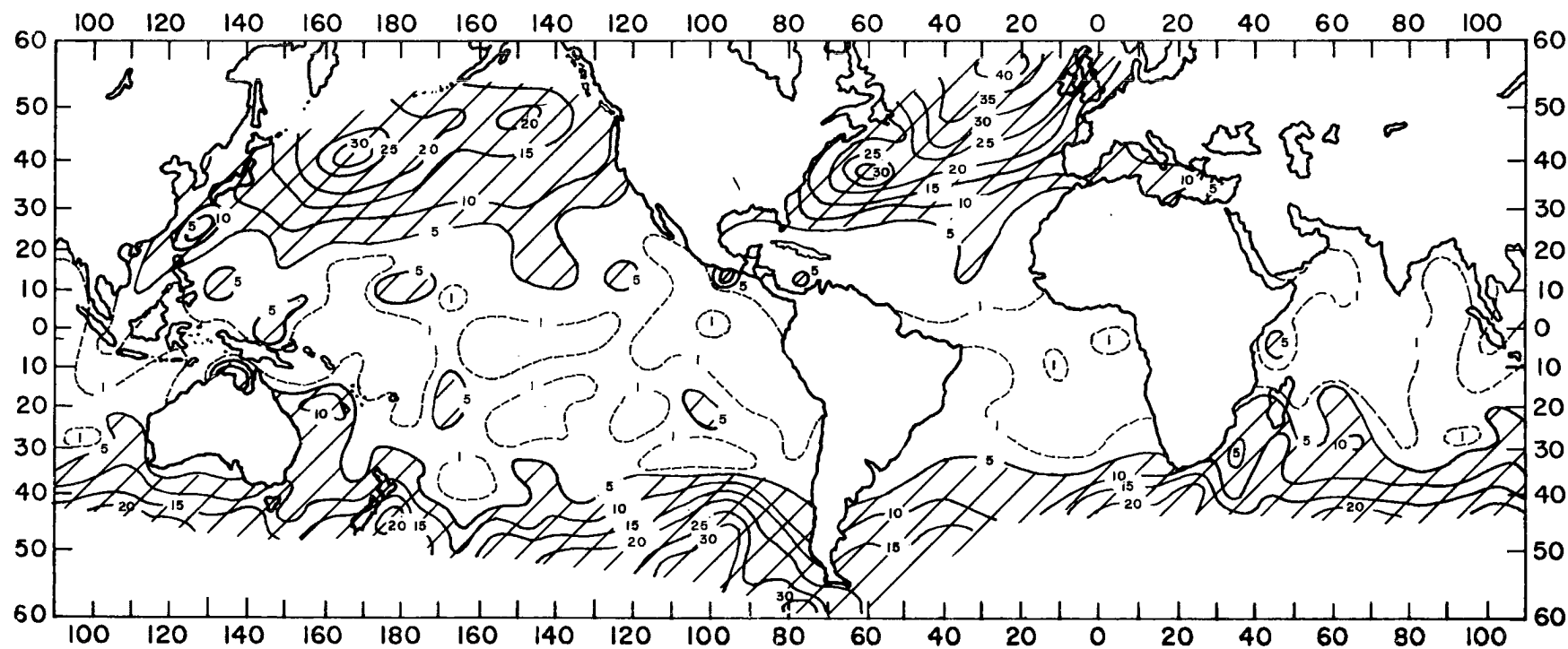
Figure 20. Frequency of Beaufort force 7 ( 15.5 \text{ m s}^{-1} ) or higher winds at Greenwich noon. (After McDonald, 1938).
