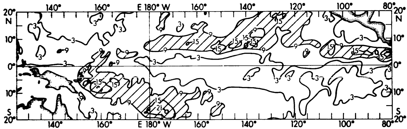
Figure 18. Frequency of highly reflective clouds for December 1971. (After Ramage, 1975)
