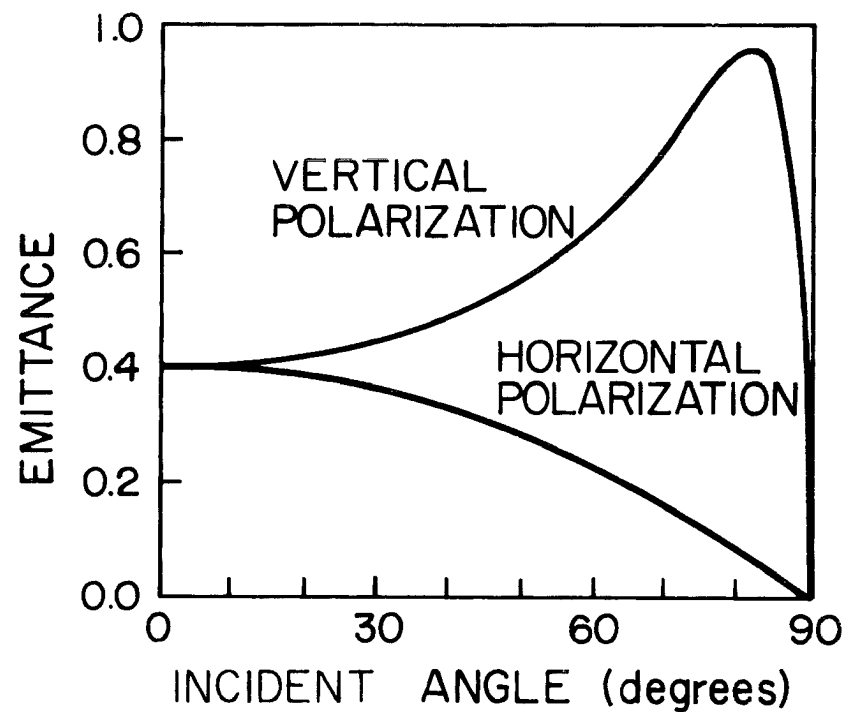
Figure 5. Emittance of a plane water surface versus angle of incidence for a wavelength of 1.55 cm and a surface temperature of 300 K.
