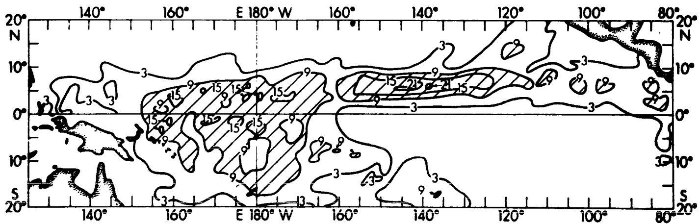
Figure 19. Frequency of highly reflective clouds for December 1972. (After Ramage, 1975)
