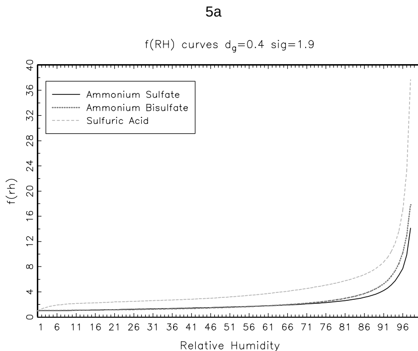
Figure 5. (a) f(RH) curves using the “no solids” method for ammonium sulfate, ammonium bisulfate, and sulfuric acid (assuming a size distribution with D_g = 0.4 \mu\text{m} and \sigma_g = 1.9 ). (b) Sulfate mass scattering efficiencies for ammonium sulfate, ammonium bisulfate, and sulfuric acid using the curves in part (a). (c) Ratios of ammonium bisulfate and sulfuric acid mass scattering efficiencies to the ammonium sulfate mass scattering efficiency shown in (b).
