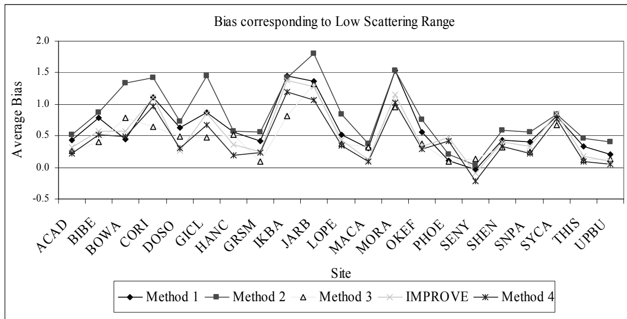
Figure 22. The average biases for each site corresponding to time periods with low measured scattering values (10–20%) (see Table 26).
