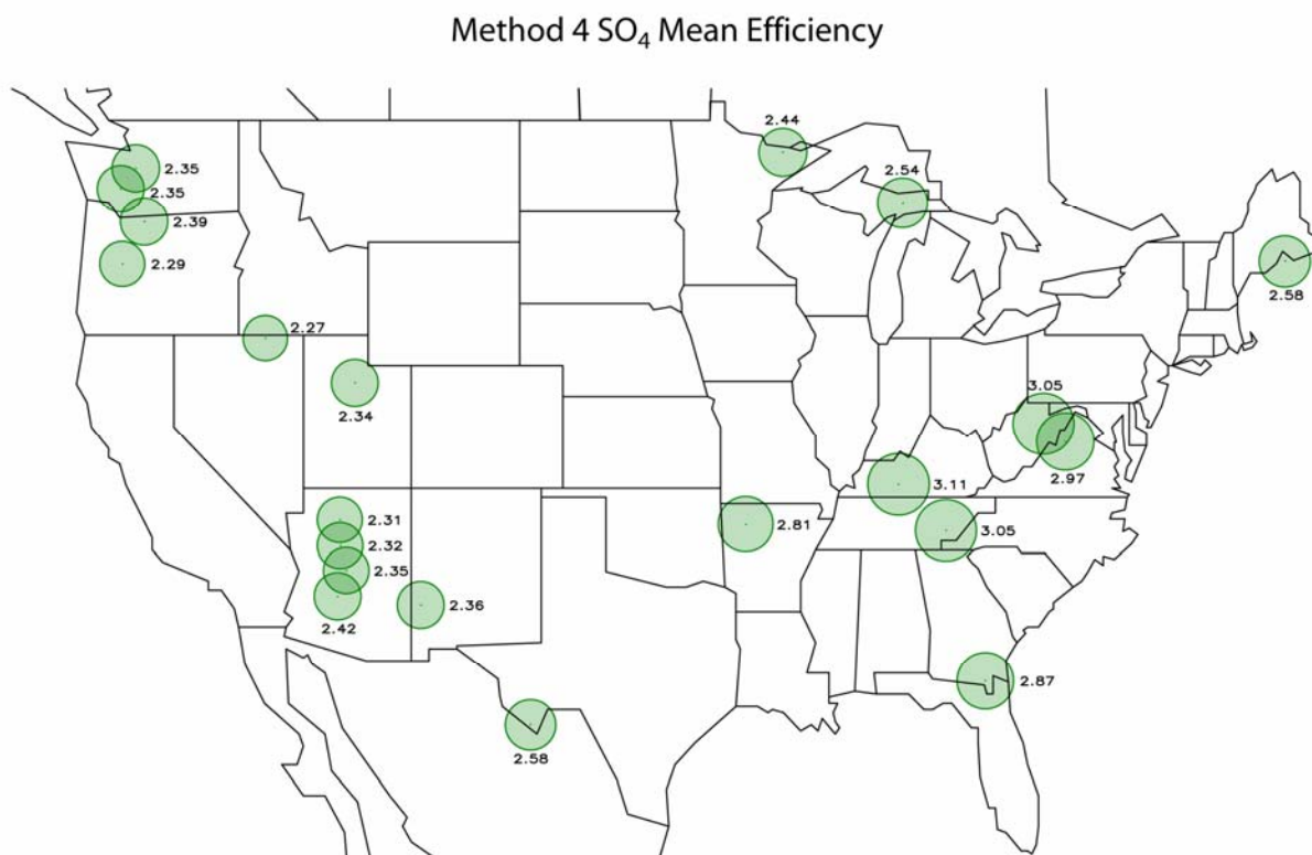
Figure 20. Map of the mean ammonium sulfate mass scattering efficiencies ( \alpha_{AS} , \text{m}^2 \text{g}^{-1} ) from method 4. The size of the circle reflects the magnitude of the efficiency, which is printed near the circle.
