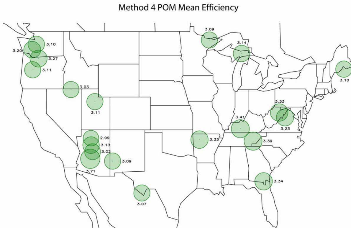
Figure 21. Map of mean POM mass scattering efficiencies ( \alpha_{POM} , \text{m}^2 \text{g}^{-1} ) from method 4. The size of the circle reflects the magnitude of the efficiency, which is printed near the circle.
