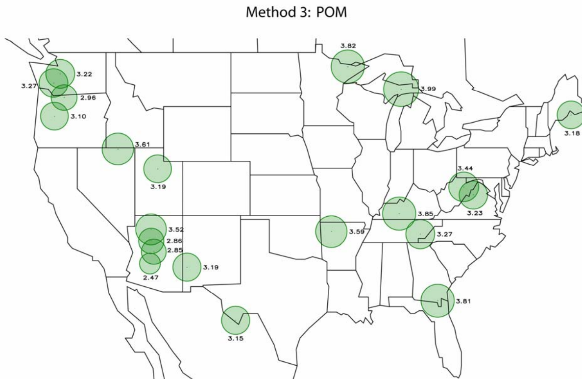
Figure 19. Map of organic mass scattering efficiencies ( \alpha_{org} , \text{m}^2 \text{g}^{-1} ) from method 3. The size of the circle reflects the magnitude of the efficiency, which is printed next to the circle..
