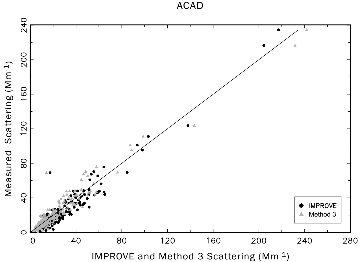
Figure 10. Comparisons of method 3 reconstructed mixed scattering ( b_{mix,esb} Mm^{-1} ) to measured mixed scattering ( b_{mix} Mm^{-1} ) for Acadia National Park.
