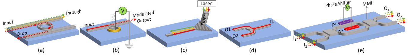
Figure 2: SiPh devices: (a) MRR add-drop filter, (b) MRR modulator, (c) grating coupler, (d) Y-splitter, and (e) the MZI-based switching element for TRINE’s tree-based network (MMI: Multi-Mode Interferometer).
