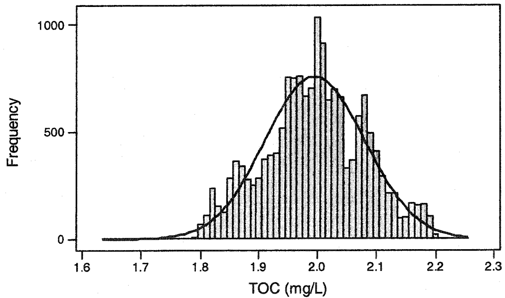
Figure B-2 Histogram of TOC with Normal Curve.
