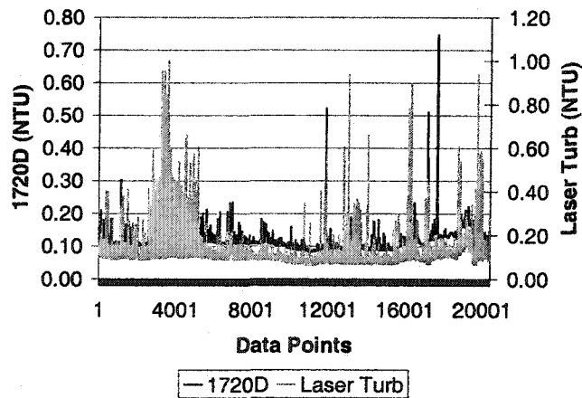
Figure 4-2 Baseline water quality time series plots
