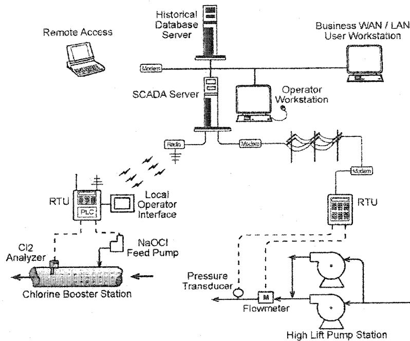
Figure 2-3 SCADA system with typical components (AWWARF, 2002)
