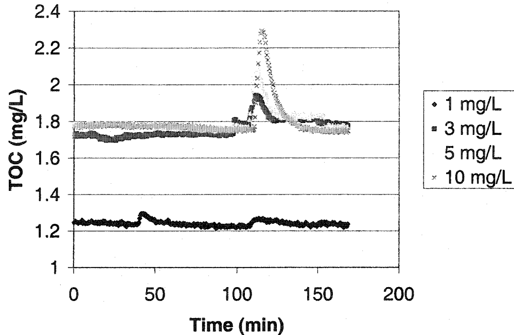
Figure 4-9 Time series plot of on-line instrument response for aldicarb and TOC.
