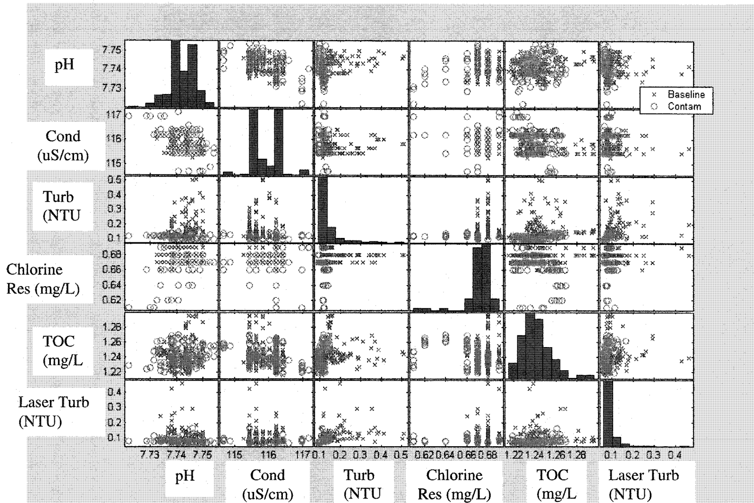
Figure 5-5 Bivariate plot of instrument response after 1 mg/L of aldicarb was added to tap water
