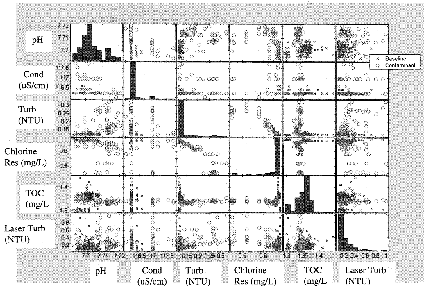
Figure 5-7 Bivariate plot of instrument response after 1 mg/L of sodium cyanide was added to tap water
