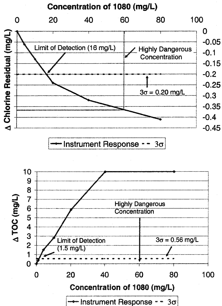
Figure 4-3 Concentration-instrument response for sodium fluoroacetate (1080), chlorine residual, and TOC
