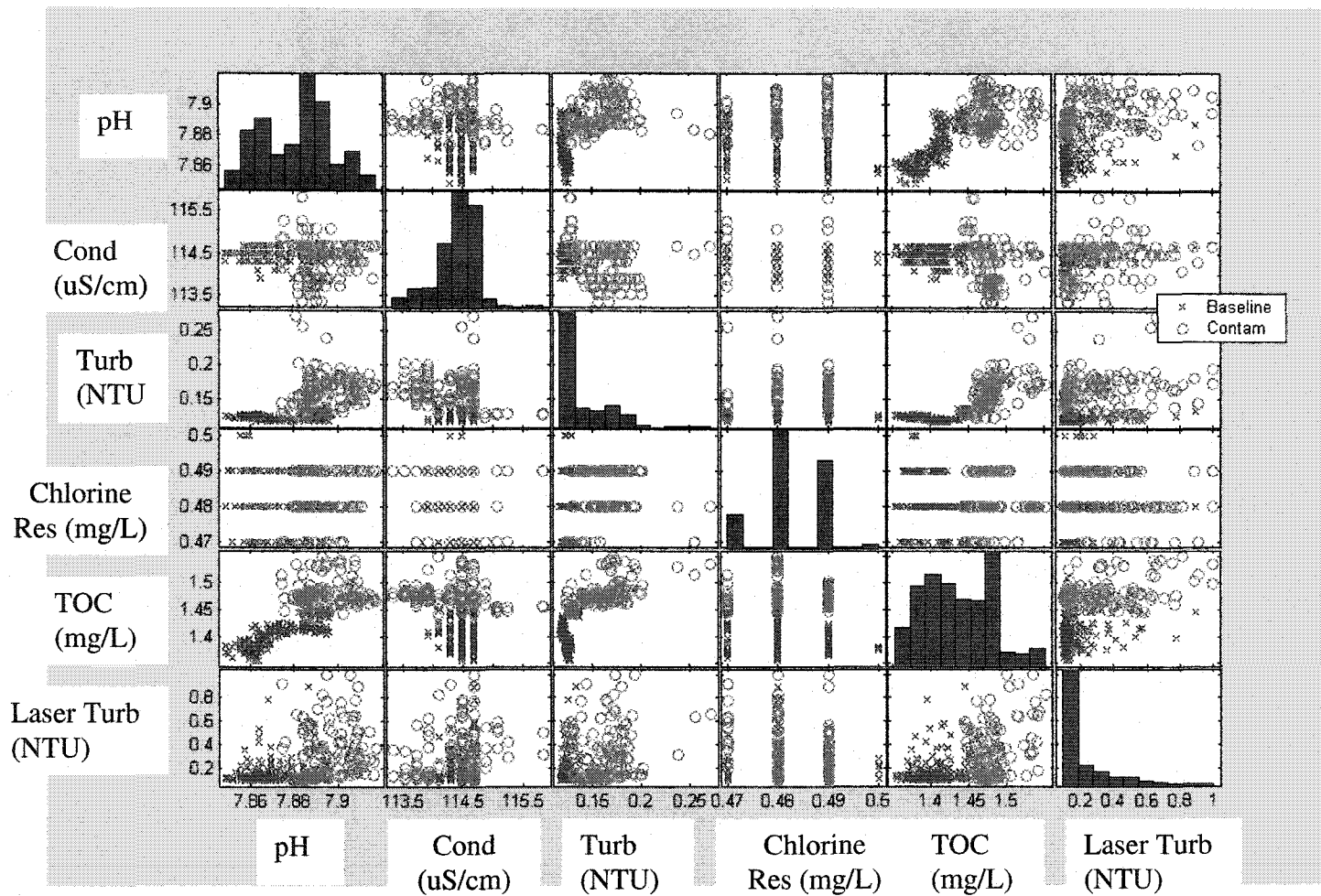
Figure 5-4 Bivariate plot of instrument response after 3 mg/L of sodium fluoroacetate was added to tap water
