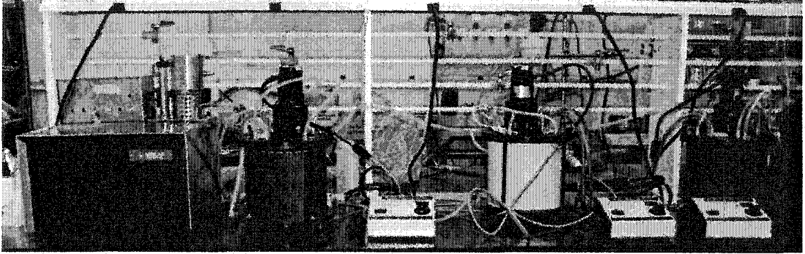
Figure D-4 Covered bioreactors and heat exchanger setup
