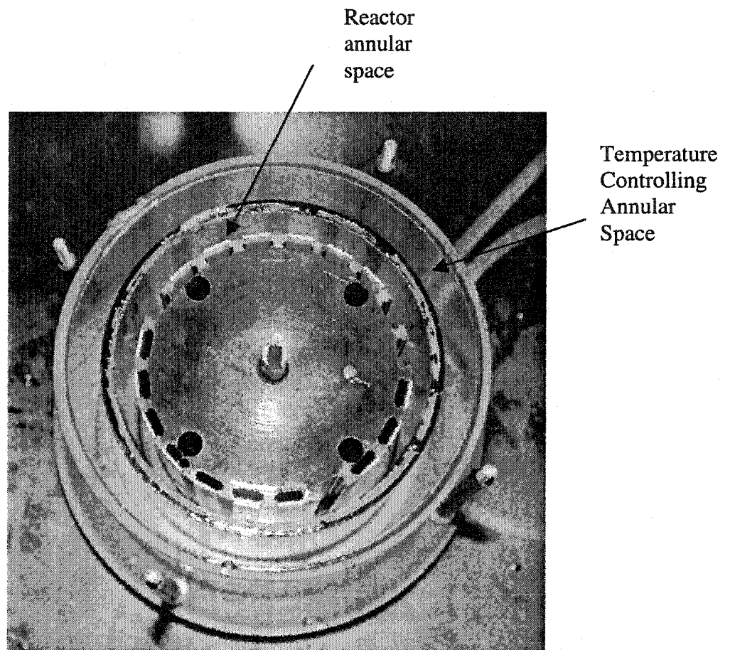
Figure D-1 Top view of open bioreactor
