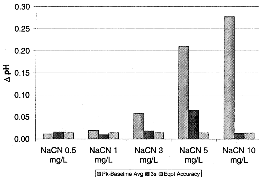
Figure B-7 Comparison of instrument response, 3\sigma , and equipment accuracy
