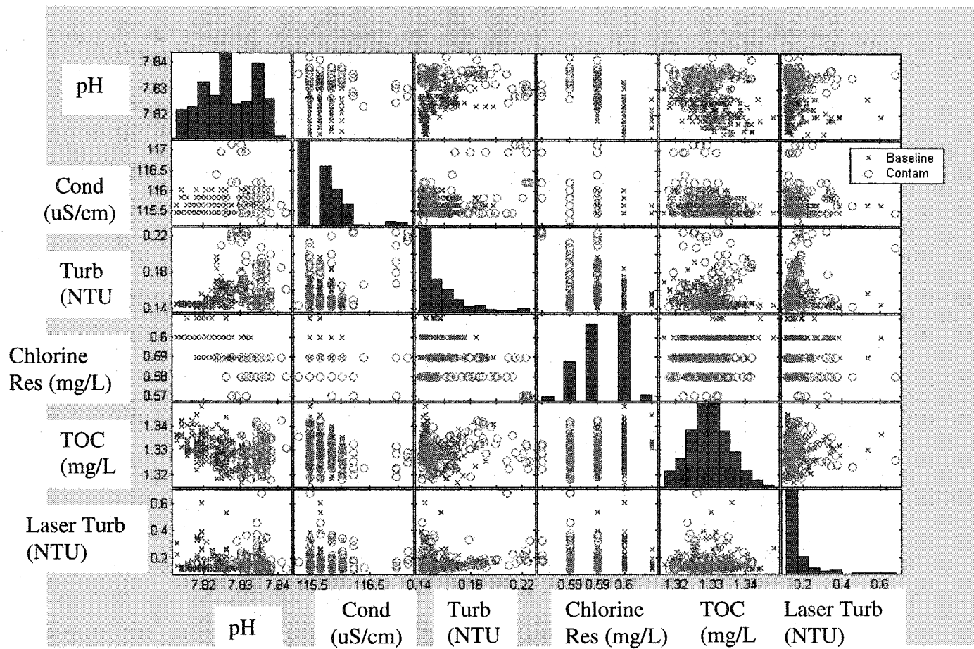
Figure 5-6 Bivariate plot of instrument response after 15 mg/L of sodium arsenate was added to tap water
