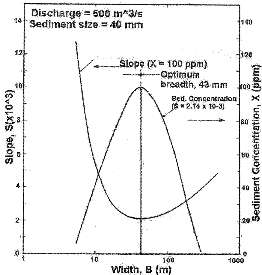
Figure 2.1: Sediment load, slope and channel width relationships (After White et al. 1982).
