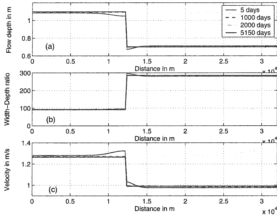
Figure 4.10: Results of the hydraulic component of the numerical model with constant discharge . (a) Flow depth along the channel, (b) Width-depth ratio along the channel, (c) Flow velocity along the channel.
