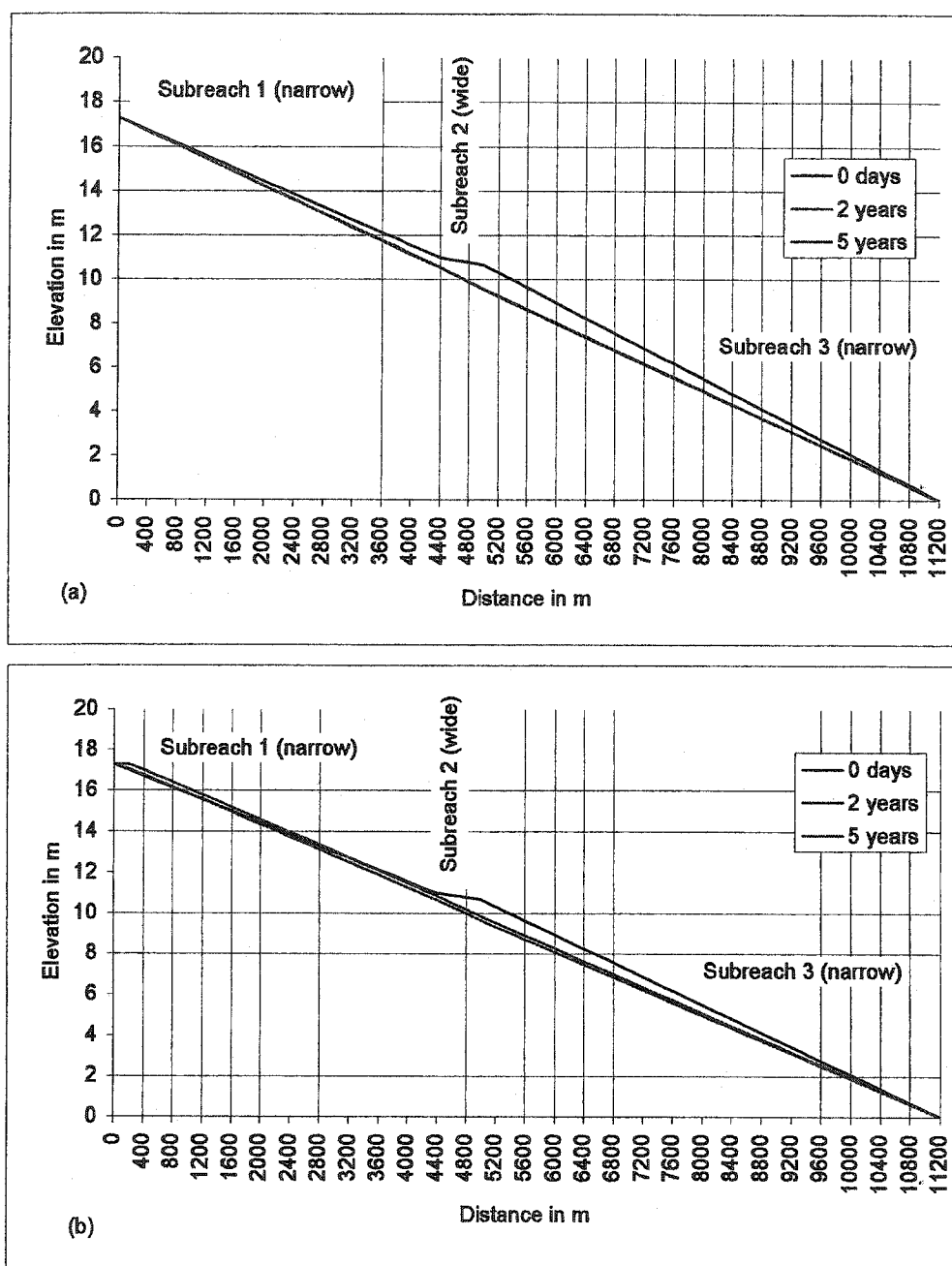
Figure D.1: Bed elevation profiles of the temporarily channel (a) Elevation profiles for case A. (b) Elevation profiles for case B.
