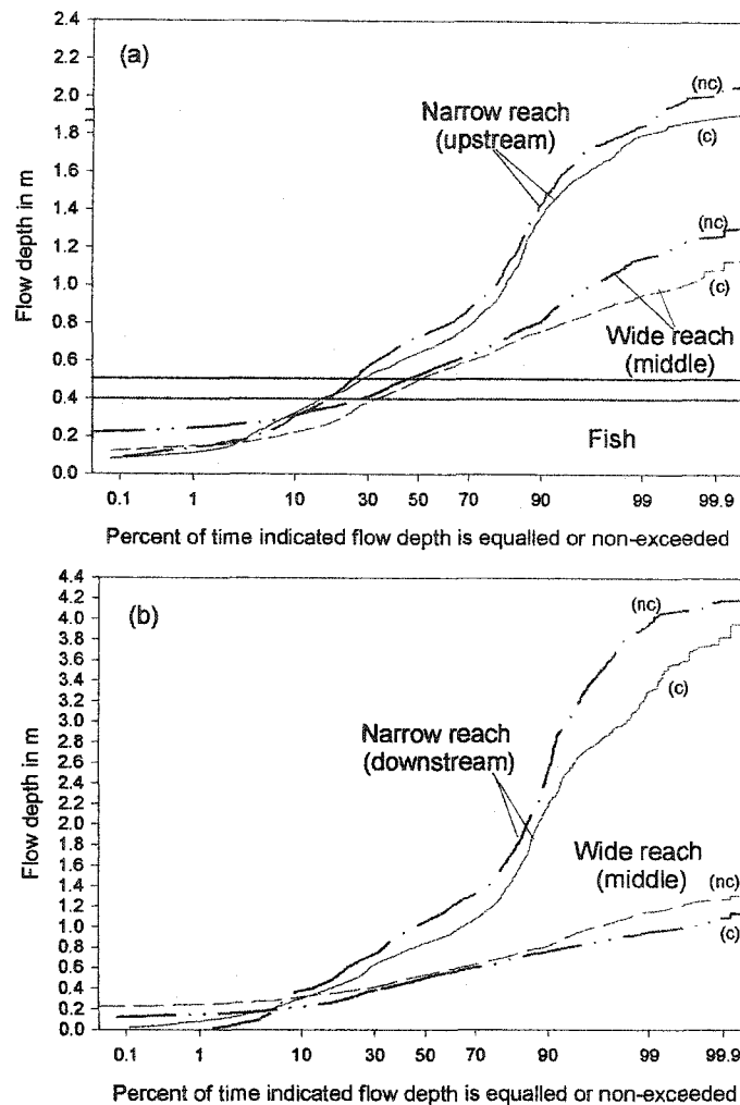
Figure 6.19: Flow depth duration curves. (a) Comparison of the curves at the narrow (upstream) and wide (middle) reaches. (b) Comparison of the curves at the wide (middle) and narrow (downstream) reaches. nc = no controlling degradation along the entire channel; c = controlling degradation along the entire channel.
