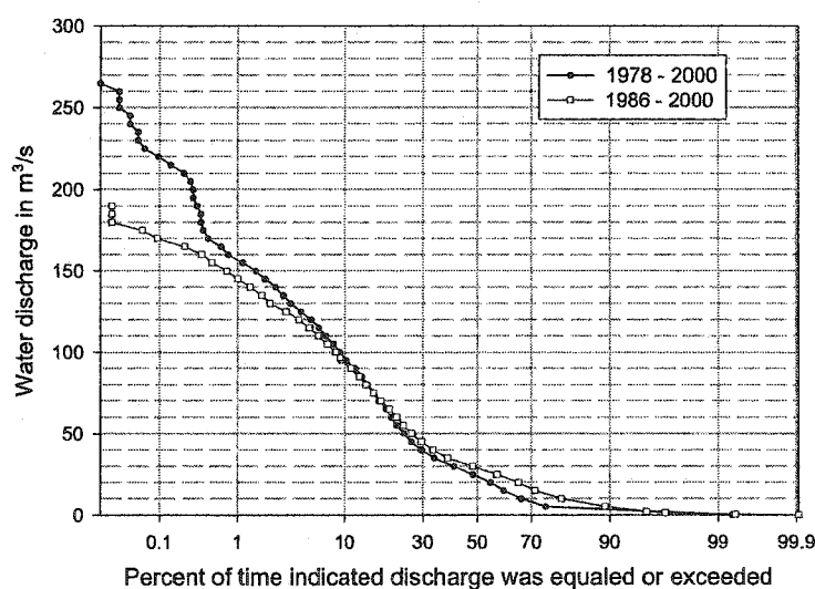
Figure E.1: Flow duration curves at the San Acacia gage for the 1978 to 2000 and 1986 to 2000 periods.
