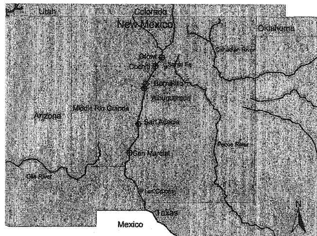
Figure 3.1: Location map of the Middle Rio Grande, NM. Large circles indicate the locations of USGS gage stations. Map not to scale.
