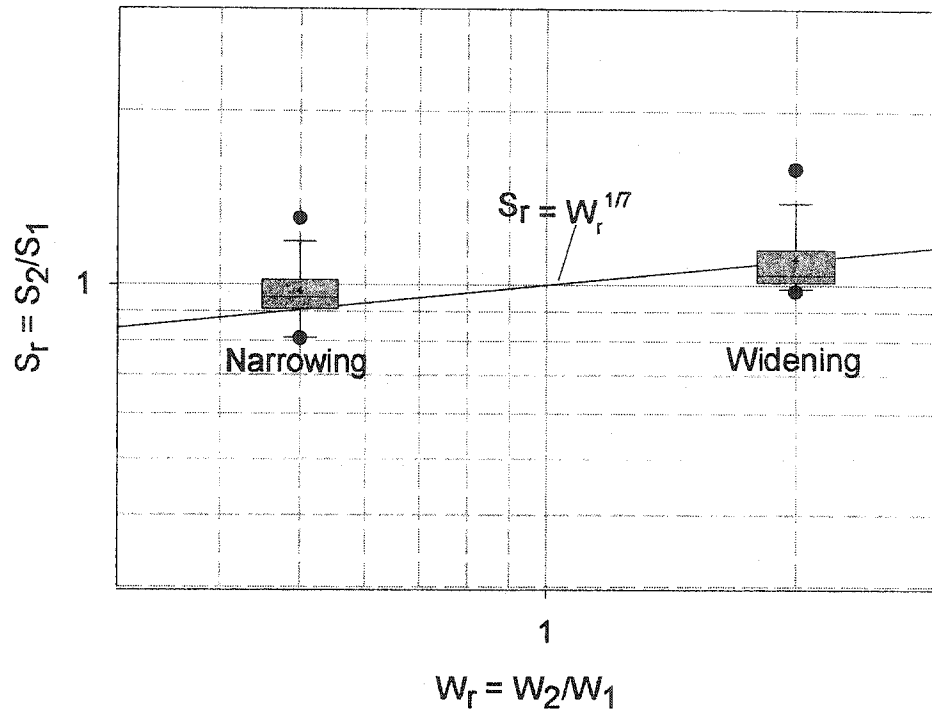
Figure 4.16: Comparison of the width ratio versus slope ratio relationship in equation 4.4 with the box plots for the results of the laboratory flume data of Bigillon (1997).
