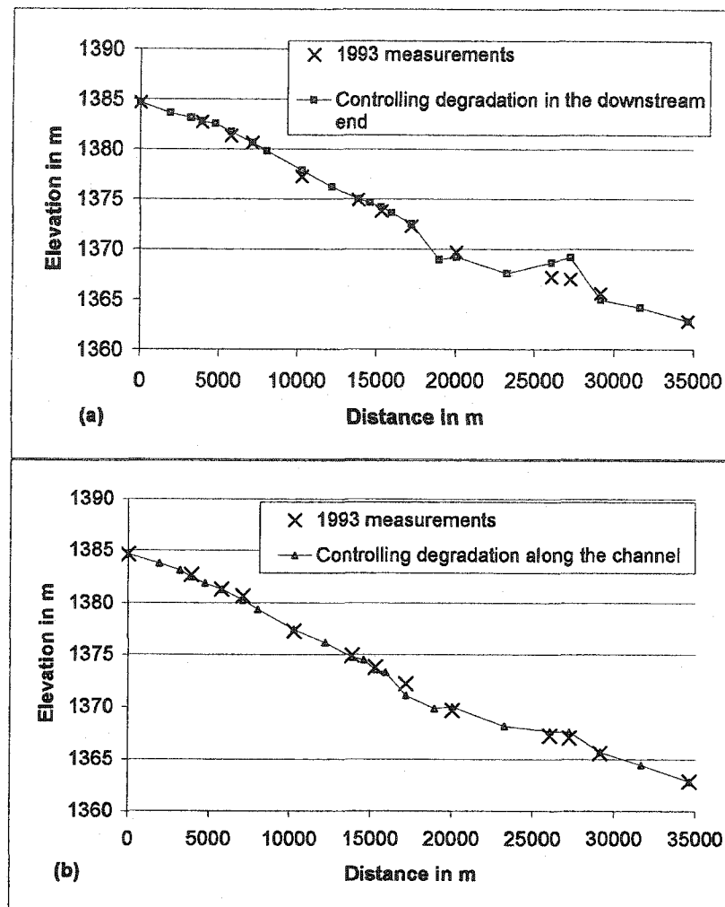
Figure I.4: Comparison of the resulting channel profile from the sediment transport model with the field data collected in 1993. (a) Channel degradation is controlled in the last two downstream nodes of the reach. (b) Channel degradation is controlled along the entire channel.
