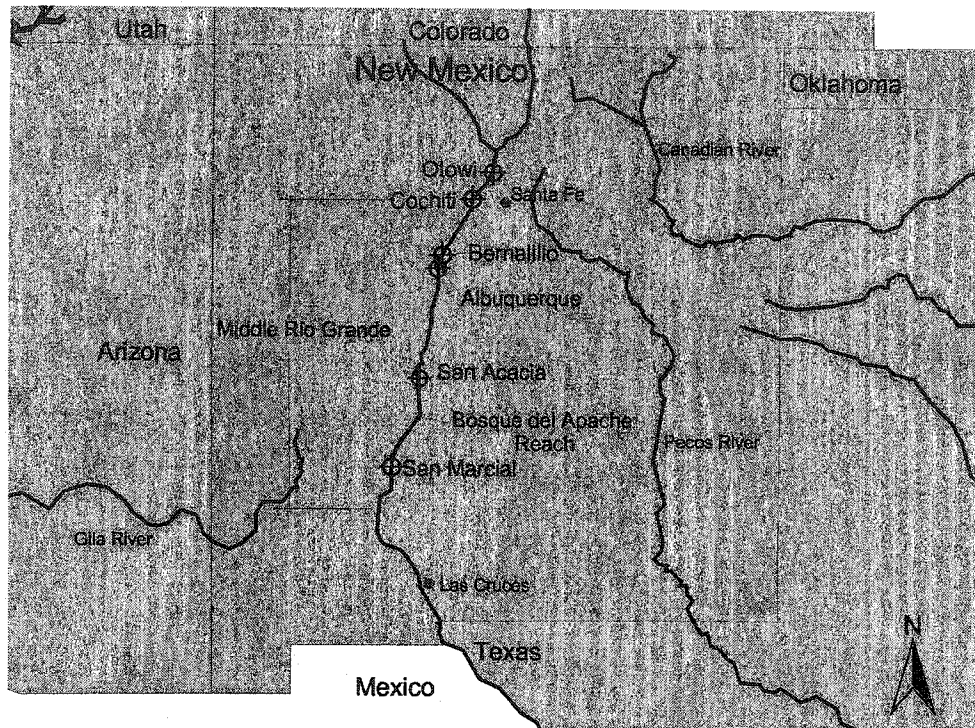
Figure 6.1: Approximate location of the Bosque del Apache reach in the middle Rio Grande. Map not to scale.
