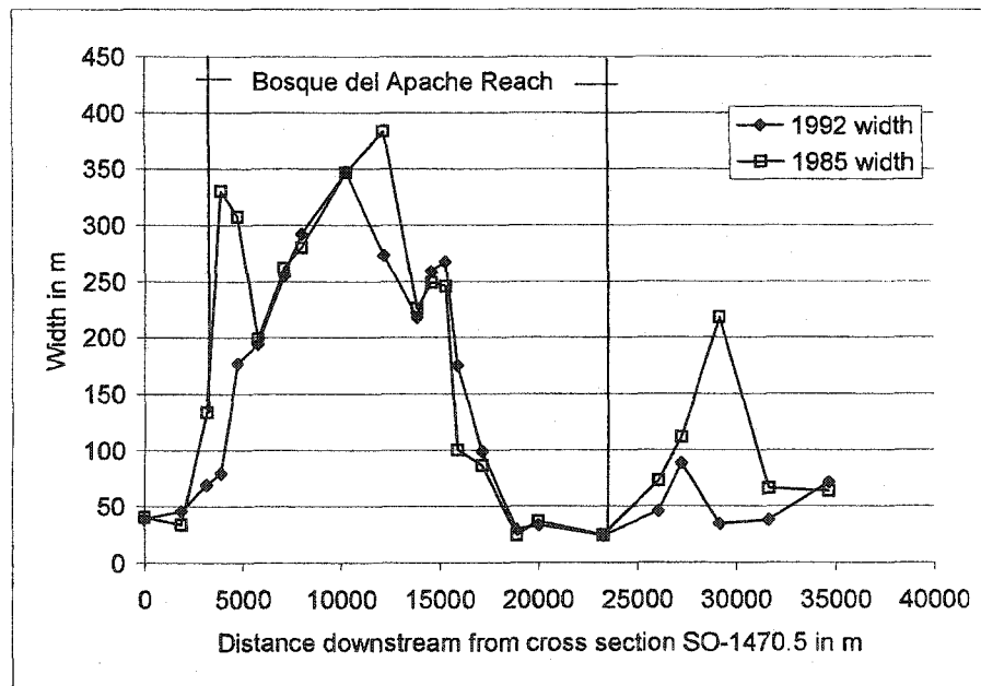
Figure 6.7: Non-vegetated channel width for 1985 and 1992.
