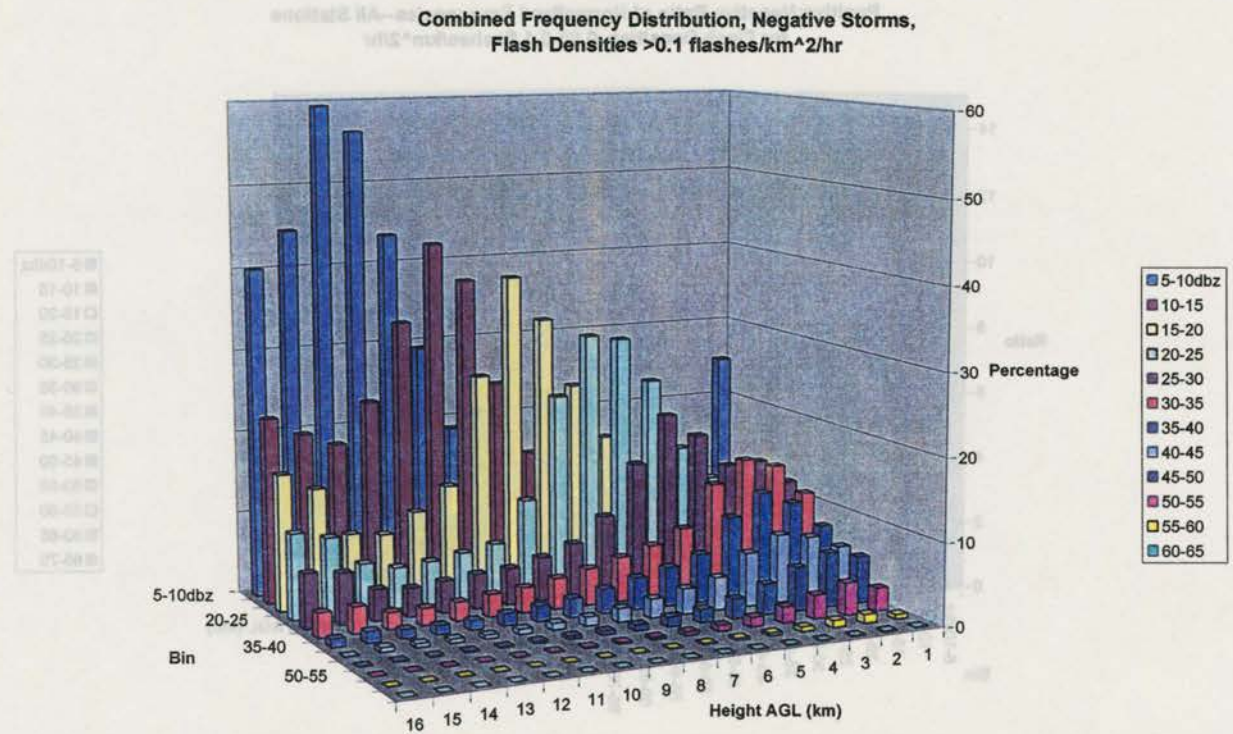
Figure 4.6: Combined Frequency Distribution with flash densities >0.1 flashes km -2 hr -1 for a) Positive storms, and b) Negative storms.
