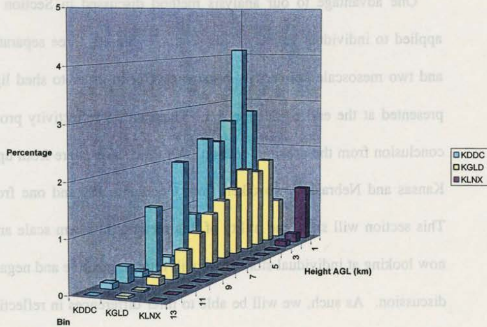
PPCG Station Comparison, Summed Frequencies >55 DBZ Flash Densities > 0.1 flashes/km 2 /hr
