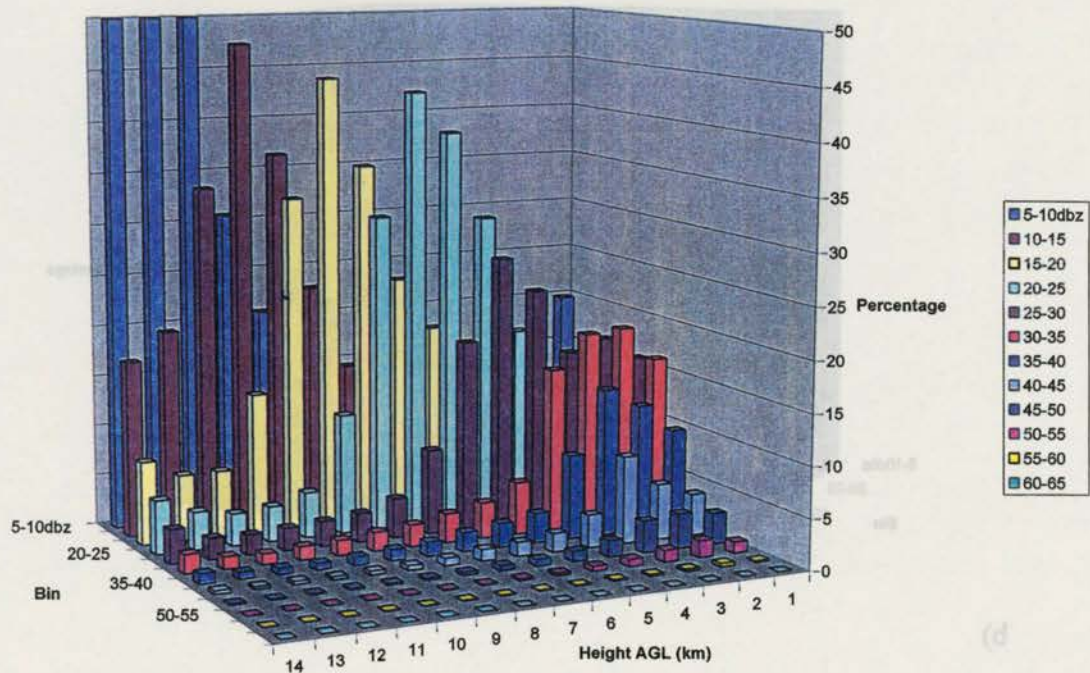
Dodge City, KS (KDDC) Combined Frequency Distribution All Positive Grids
