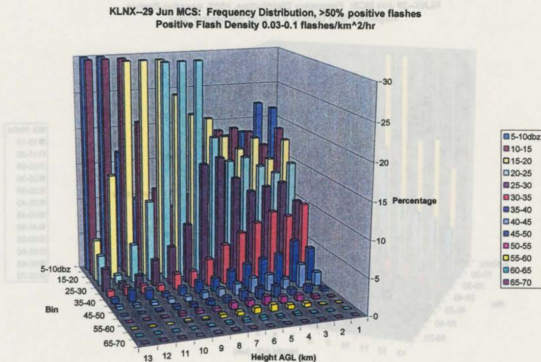
Figure 4.25: 29 Jun MCS frequency distribution for positive flash densities between 0.03-0.1 flashes km -2 hr -1 for a) positive grids and b) negative grids.
