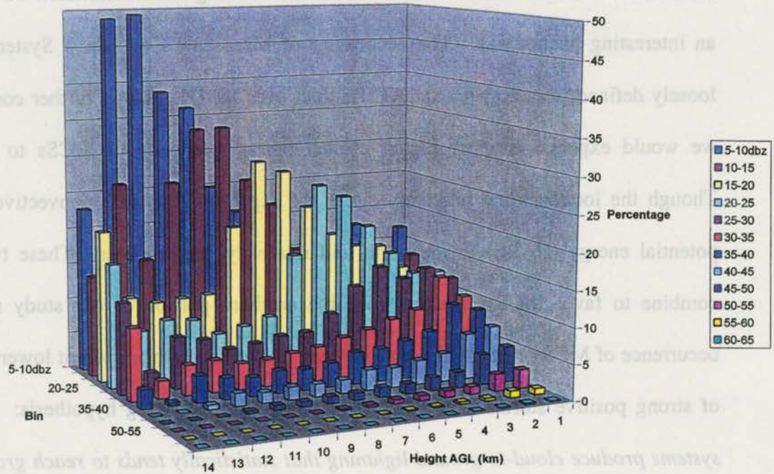
Cheyenne, WY (KCYS) Combined Frequency Distribution All Positive Grids
