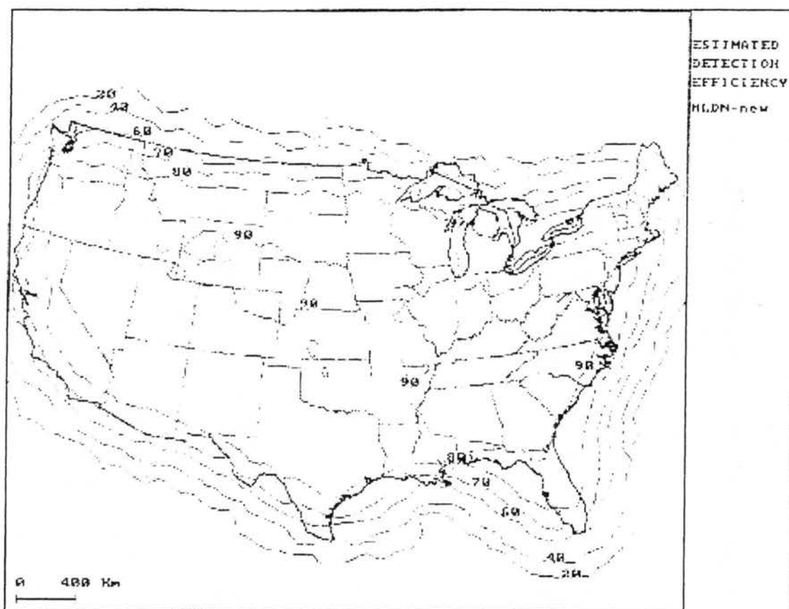
Figure . Projected NLDN Detection Efficiency (After Upgrade).
