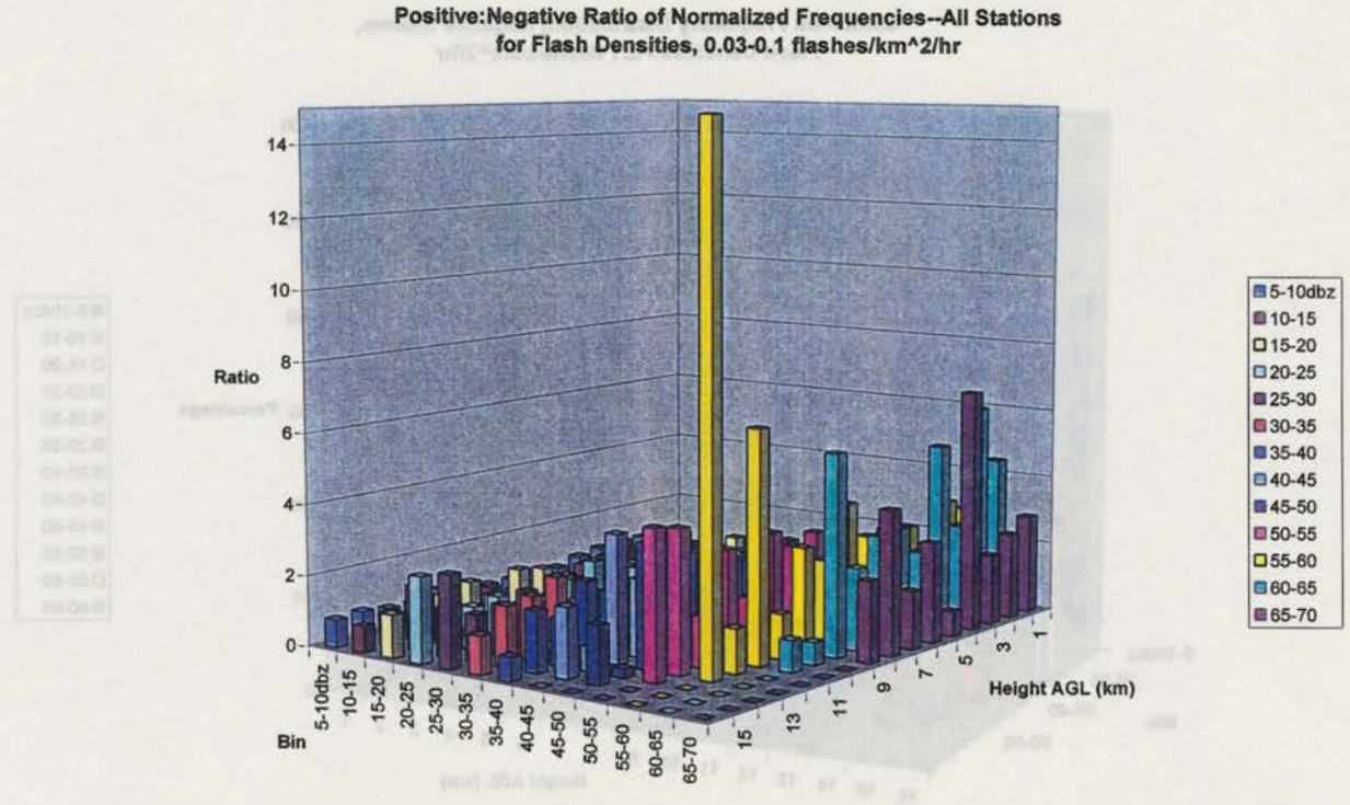
Figure 4.7: Positive to negative frequency ratios for storms with flash densities from a) >0.1 flashes \text{km}^{-2} \text{hr}^{-1} and b) 0.03-0.1 flashes \text{km}^{-2} \text{hr}^{-1} .
