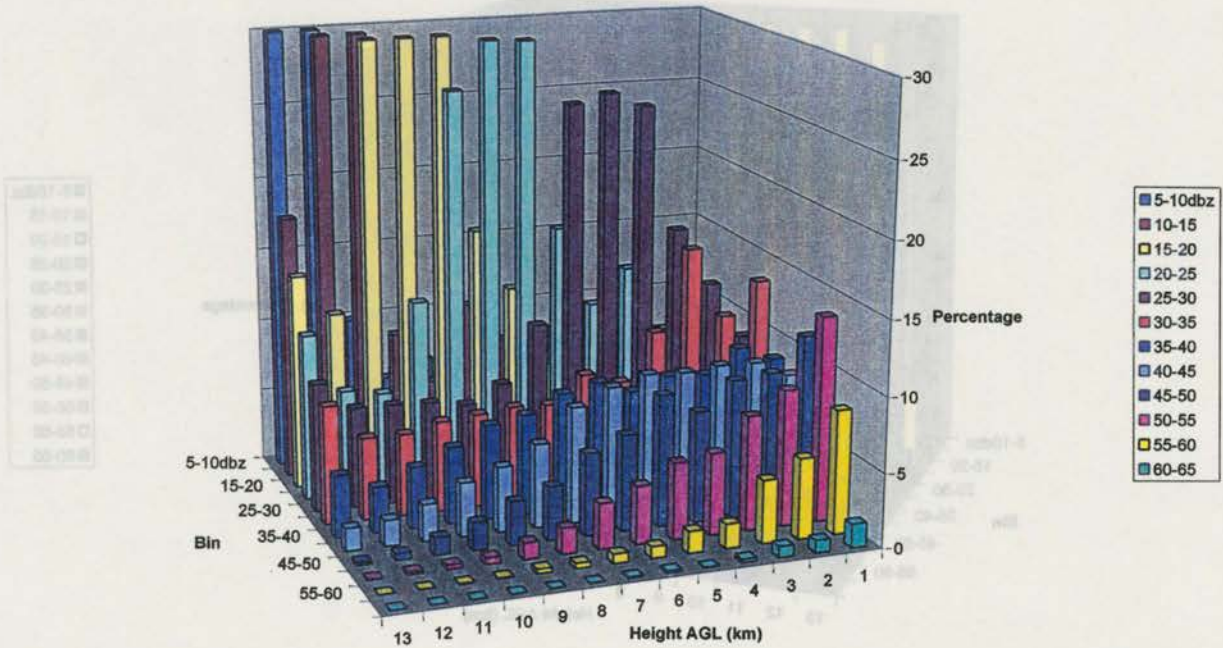
KGLD--22 Jun Frequency Distribution, >50% positive flashes Positive Flash Density 0.01-0.03 flashes/km 2 /hr
