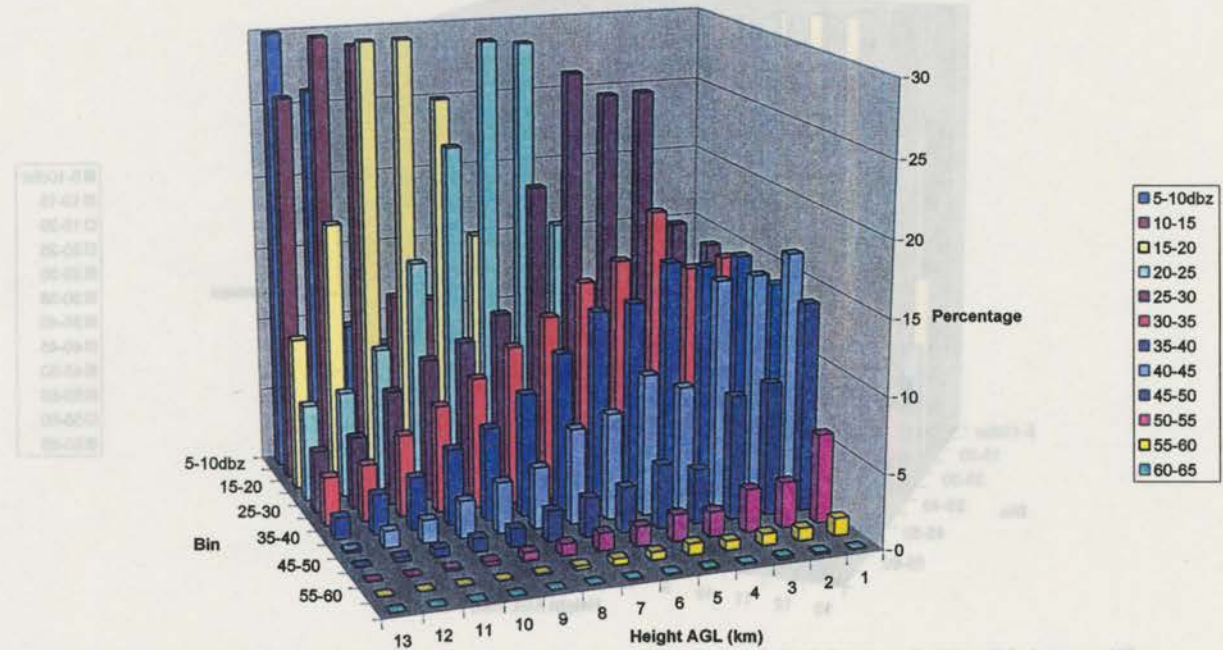
Figure 4.29: 22 Jun MCS frequency distribution for positive flash densities a) 0.01-0.03 flashes km -2 hr -1 and b) 0.0-0.01 flashes km -2 hr -1 .
