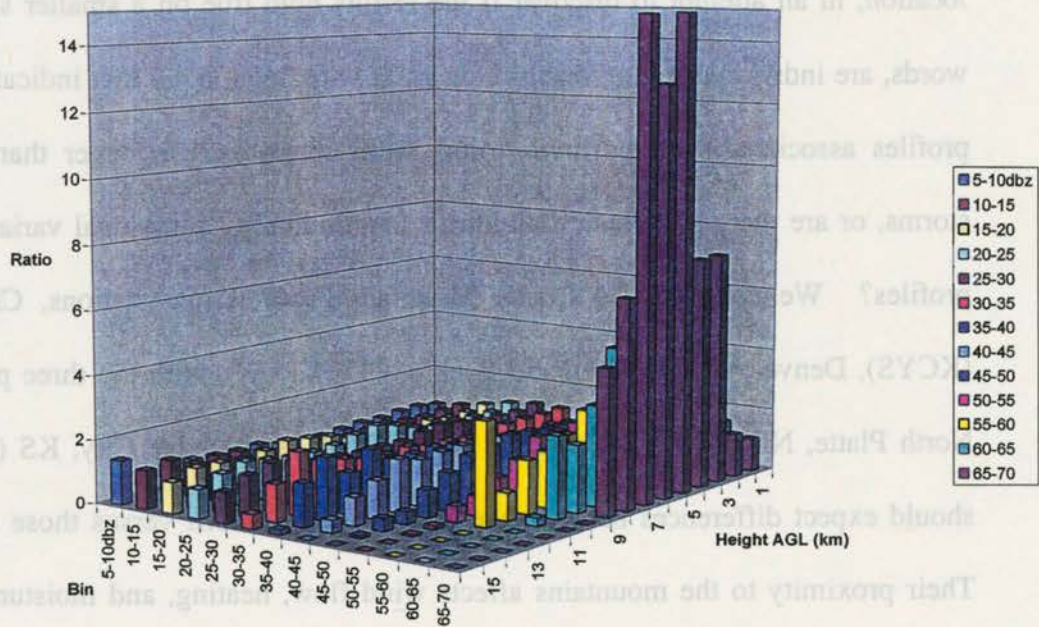
Positive:Negative Ratio of Normalized Frequencies--All Stations for Flash Densities, 0.01-0.03 flashes/km 2 /hr
