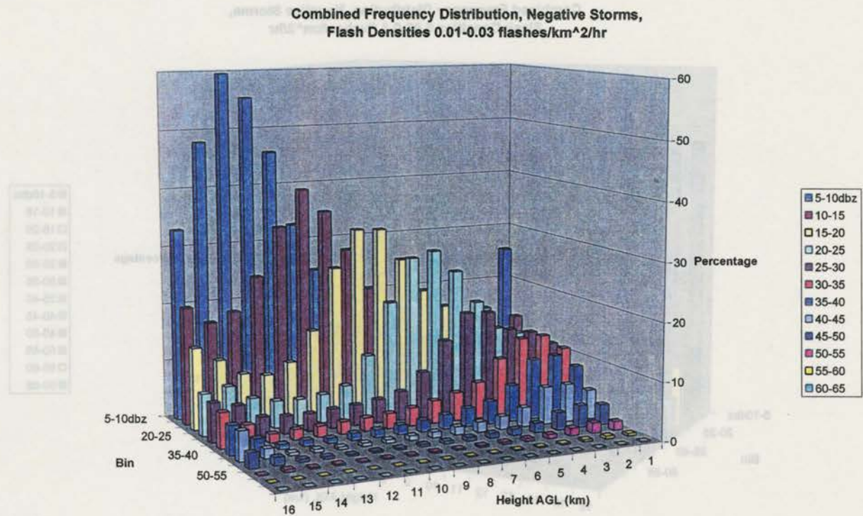
Figure 4.4: Combined Frequency Distribution with flash densities 0.01-0.03 flashes km -2 hr -1 for a) Positive storms, and b) Negative storms.
