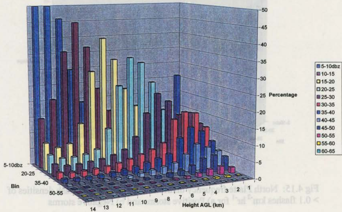
Fig 4.14: Dodge City, KS frequency distribution for a) Positive storms and b) Negative storms.
