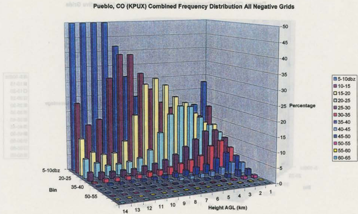
Fig 4.11: Pueblo, CO frequency distribution for a) Positive storms and b) Negative storms.
