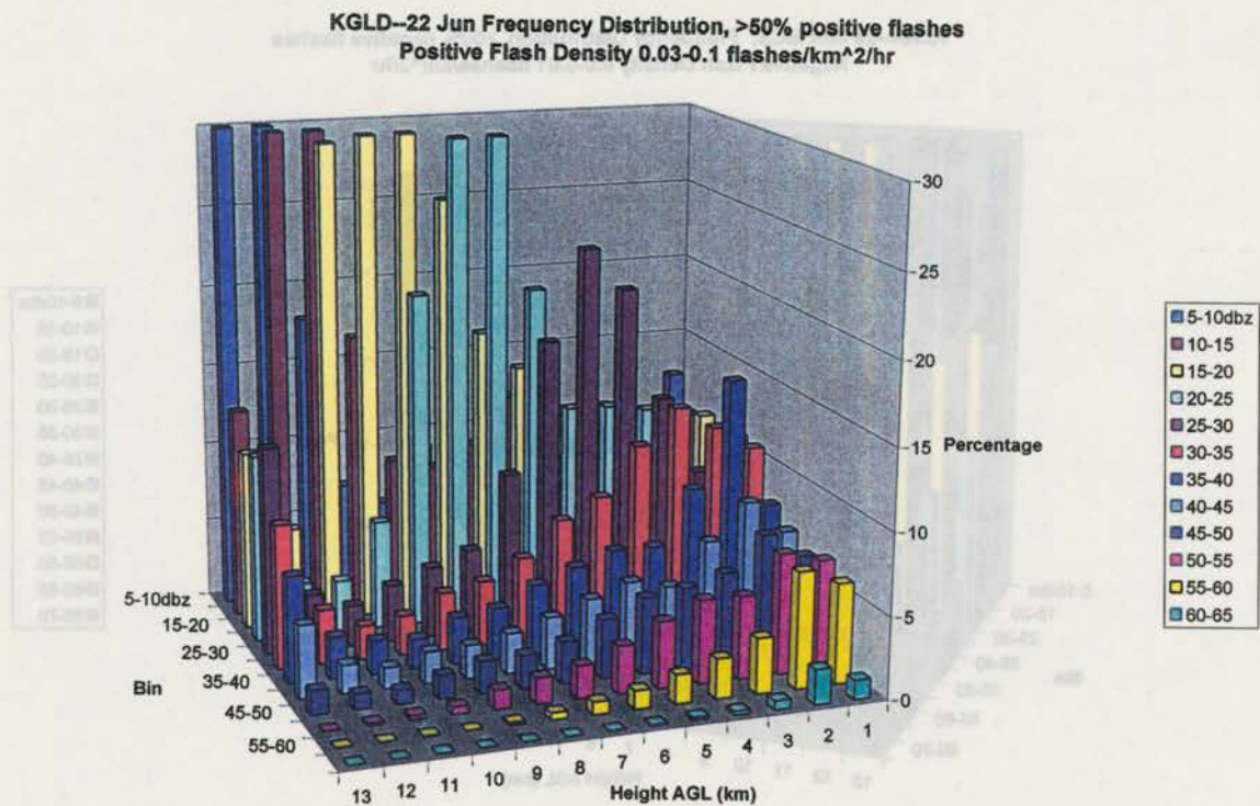
Figure 4.28: 22 Jun MCS frequency distribution for positive flash densities a) > 0.1 flashes km -2 hr -1 and b) 0.03-0.1 flashes km -2 hr -1 .
