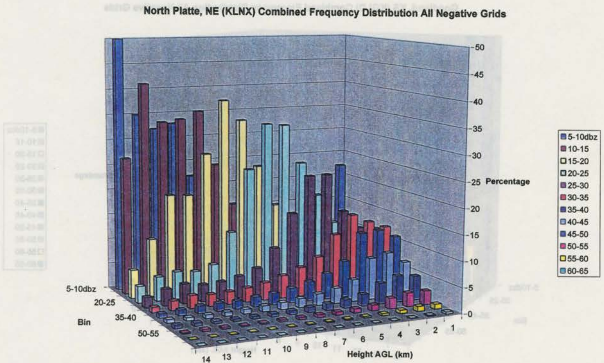
Fig 4.12: North Platte, NE frequency distribution for a) Positive storms and b) Negative storms.
