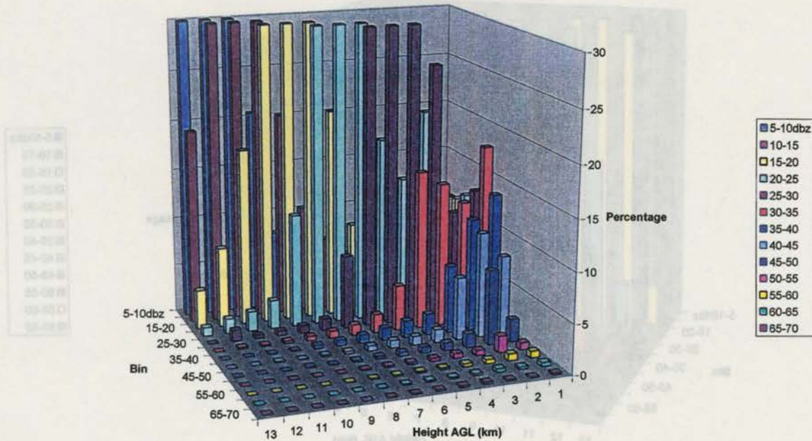
KLNX--29 Jun MCS: Frequency Distribution, >50% positive flashes Positive Flash Density 0.0-0.01 flashes/km 2 /hr
