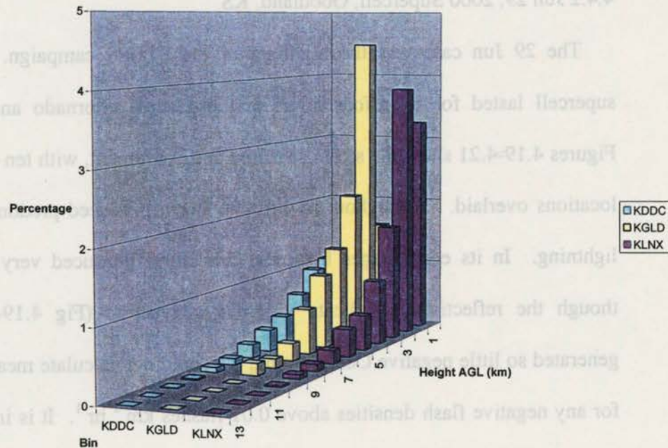
Figure 4.18: Latitudinal comparison of High Plains stations, Dodge City, Goodland, KS, and North Platte, NE for a) Positive storms and b) Negative storms.
