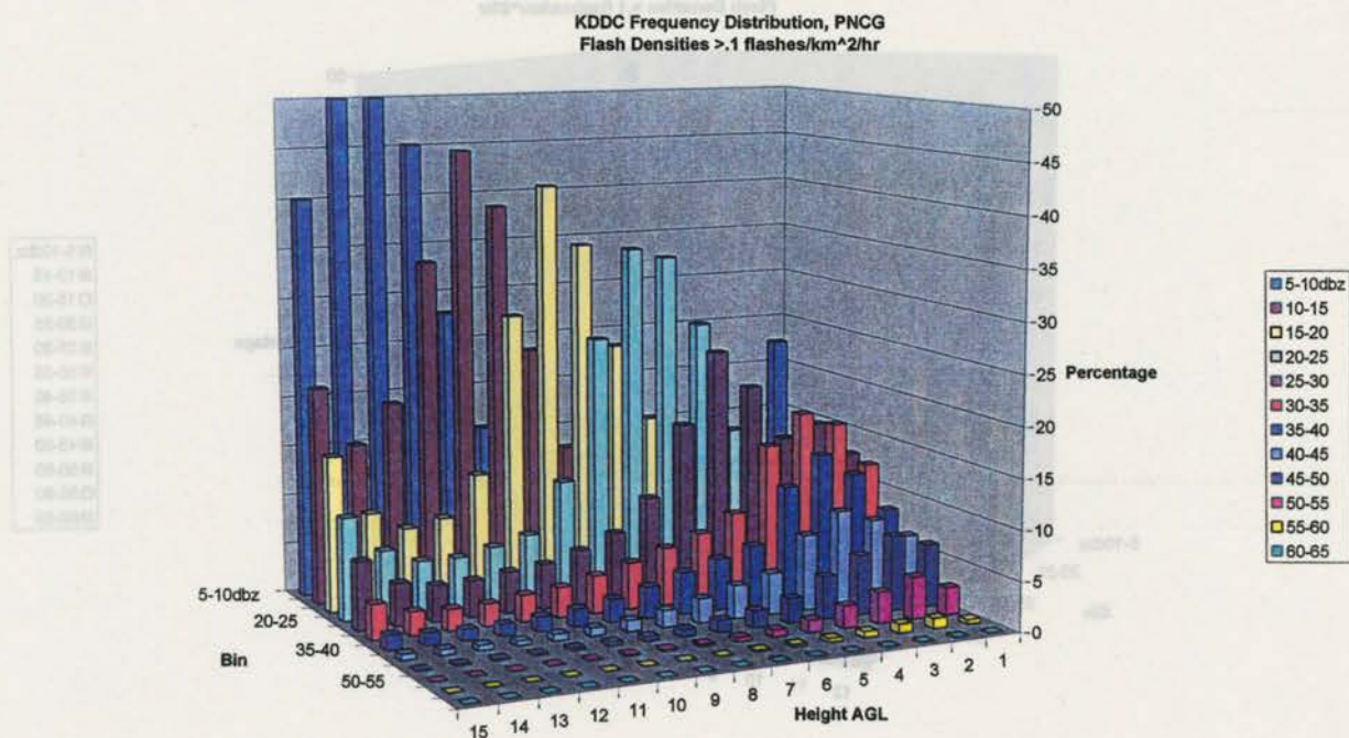
Figure 4.17: Dodge City frequency distribution of storms with flash densities of > 0.1 flashes km -2 hr -1 for a) Positive storms and b) Negative storms
