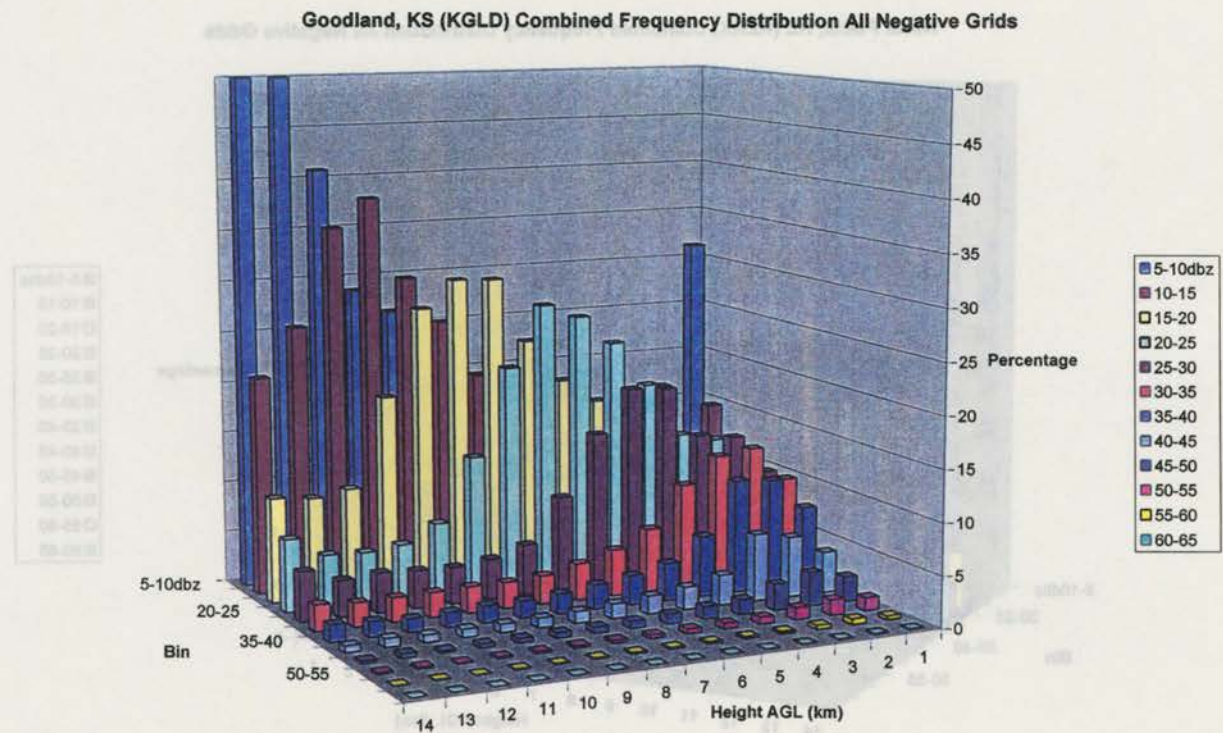
Fig 4.13: Goodland, KS frequency distribution for a) Positive storms and b) Negative storms.
