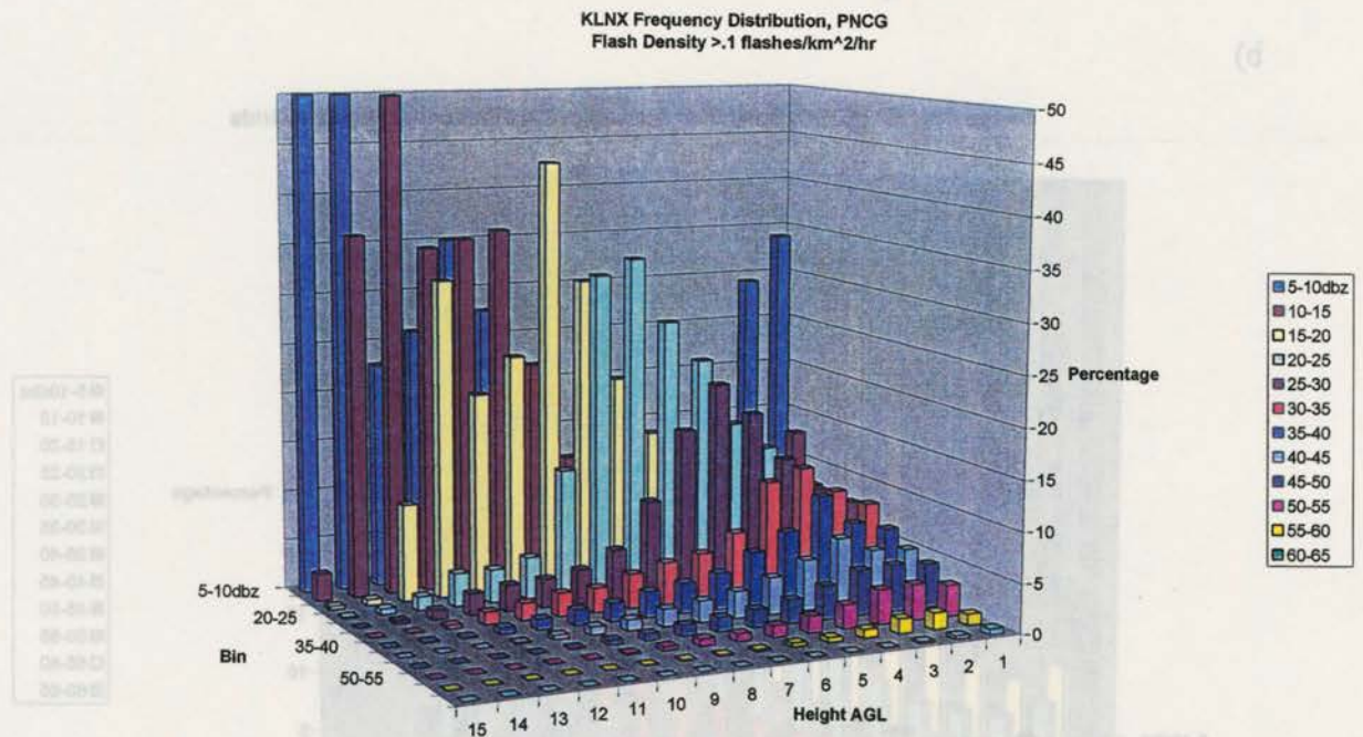
Fig 4.15: North Platte frequency distribution of storms with flash densities of > 0.1 flashes km -2 hr -1 for a) Positive storms and b) Negative storms
