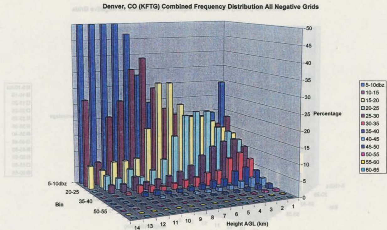
Fig 4.10: Denver, CO frequency distribution for a) Positive storms and b) Negative storms.
