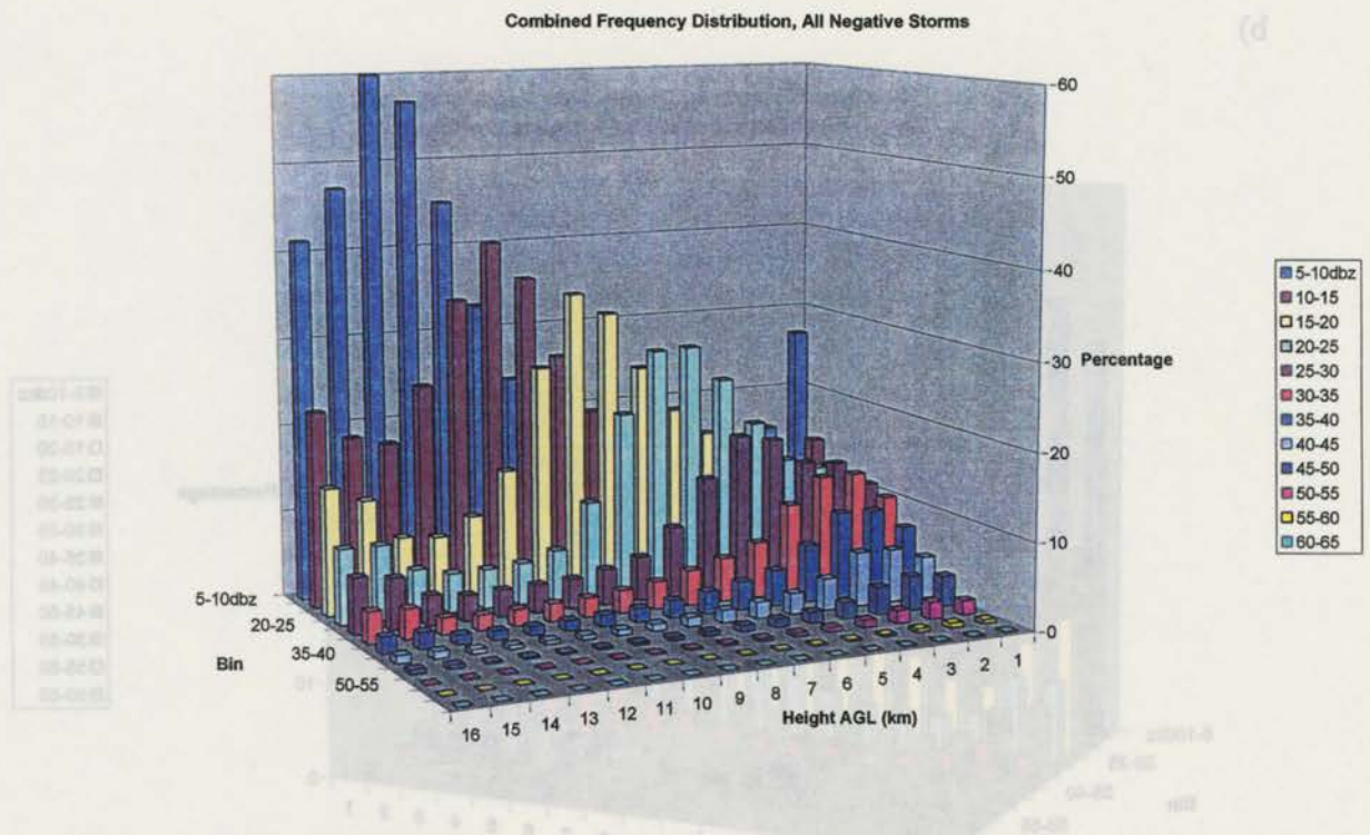
Figure 4.2: Combined Frequency Distribution for a) All positive storms, and b) All negative storms.
