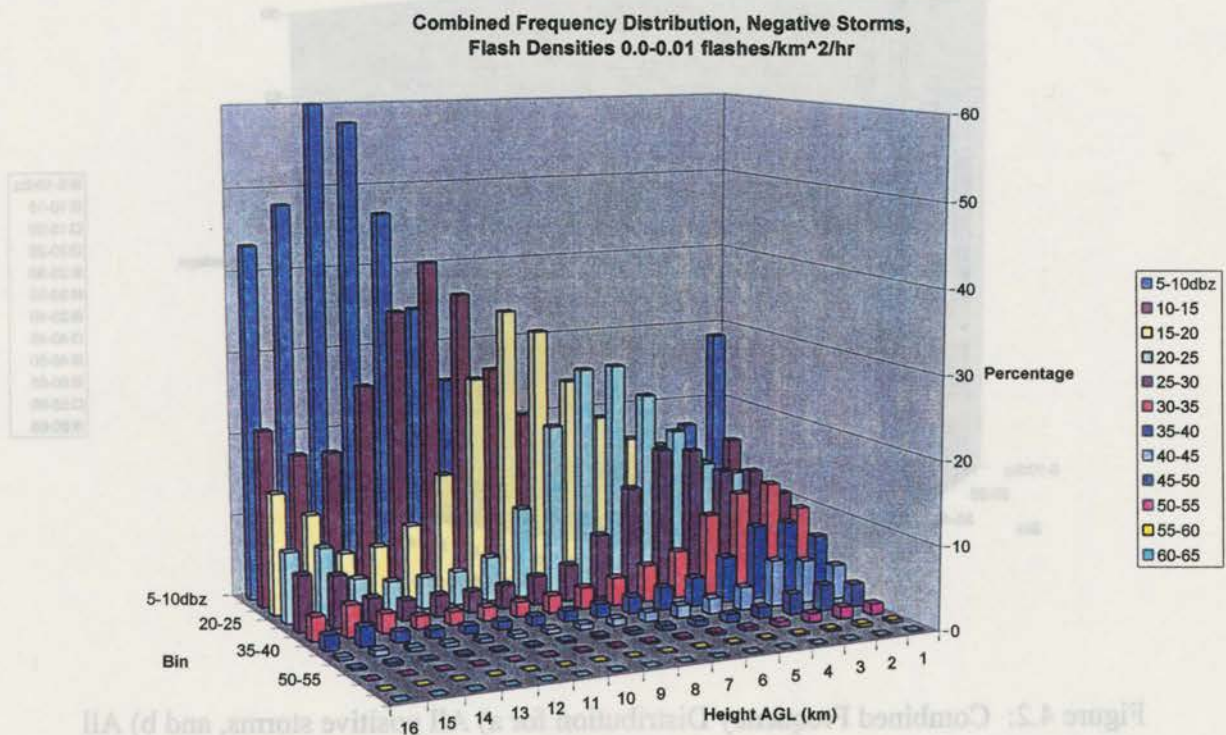
Figure 4.3: Combined Frequency Distribution with flash densities 0.0-0.01 flashes km -2 hr -1 for a) Positive storms, and b) Negative storms.
