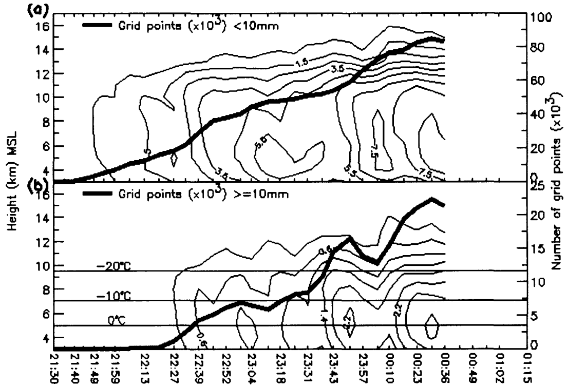
Figure 15. Time-height cross sections of the gridded particle growth model output to compare with Fig. 14. Contours represent the number of graupel-producing ( <10 mm) grid points in (a) and the number of hail-producing ( \geq 10 mm) grid points in (b) at each time and height. Contours in (a) begin at 0.5 \times 10^3 and have a contour interval of 1.0 \times 10^3 , and in (b) they begin at 0.2 \times 10^3 and have a contour interval of 0.4 \times 10^3 . The thick black lines overlaid are the same as those in panels (a) and (b) of Fig. 14. Isotherms are overlaid in (b) to highlight the 0^\circ\text{C} , -10^\circ\text{C} , and -20^\circ\text{C} levels.
