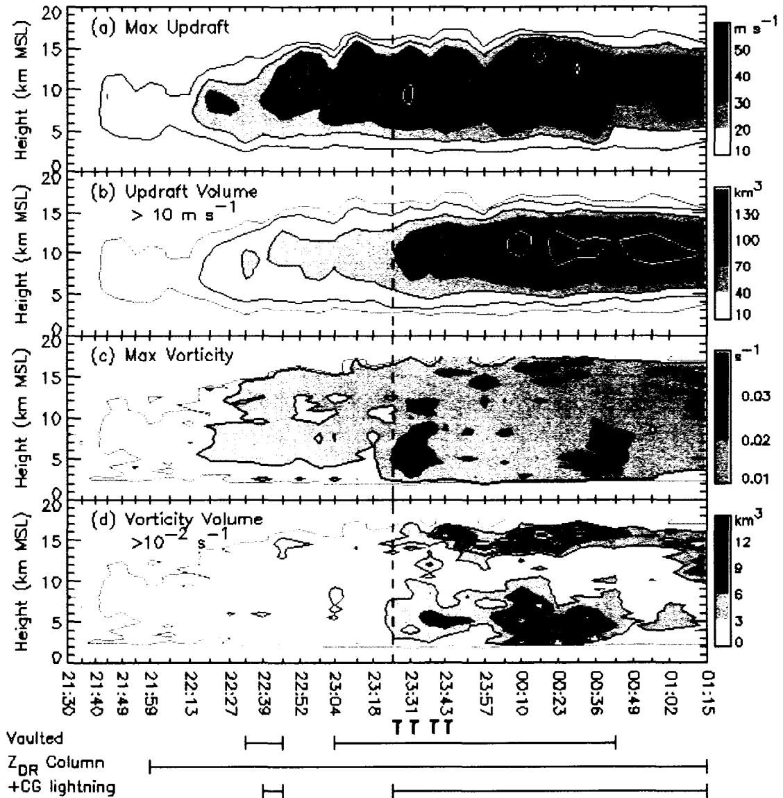
Figure 12. Time-height cross-sections of (a) maximum updraft ( \text{m s}^{-1} ), (b) updraft volume ( \text{km}^3 ) greater than 10 \text{ m s}^{-1} , (c) maximum vertical vorticity ( \text{s}^{-1} ), and (d) vertical vorticity volume ( \text{km}^3 ) greater than 10^{-2} \text{ s}^{-1} . A thick black line indicating the 10 \text{ m s}^{-1} maximum updraft contour is overlaid in (b), and the 5 \times 10^{-3} \text{ s}^{-1} maximum vertical vorticity contour is overlaid in (c) and (d) for reference. The 'T' indicates the tornado was on ground at that time, and bars across the bottom of the plot indicate the times when the storm had a vaulted reflectivity structure, a Z_{\text{dr}} column of at least 2 dB in magnitude, and positive cloud-to-ground lightning. The vertical dashed line represents the time when the storm made its right turn.
