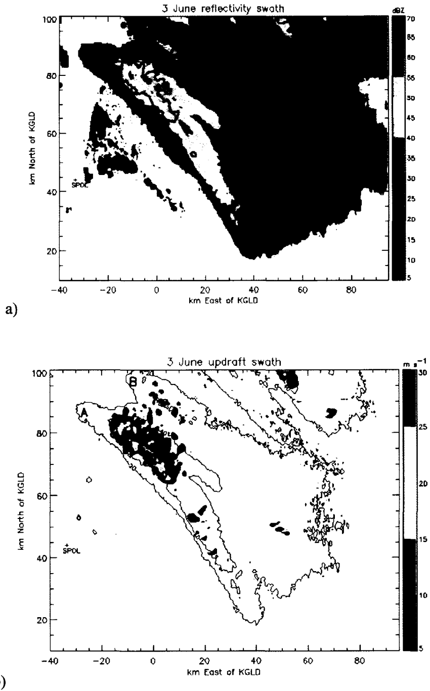
Figure 2. Swath of (a) KGLD composite reflectivity (dBZ) color contours for the period 2210-0121 UTC with a black contour overlaid indicating the regions with updrafts greater than 10 \text{ m s}^{-1} , and (b) maximum updraft color contours during the dual-Doppler analysis period with a thick black contour overlaid indicating the regions with vertical vorticity greater than 10^{-2} \text{ s}^{-1} . Thin black contours at 20 and 40 dBZ from (a) are overlaid (b) for reference. Radar locations are denoted with a '+' symbol.
