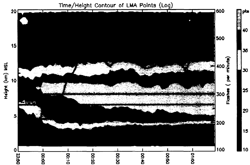
Figure 11. Time-height contours of the total number of LMA sources (color-shaded in logarithmic units) with the total flash rate time series overlaid in black for 22 June 2000.
