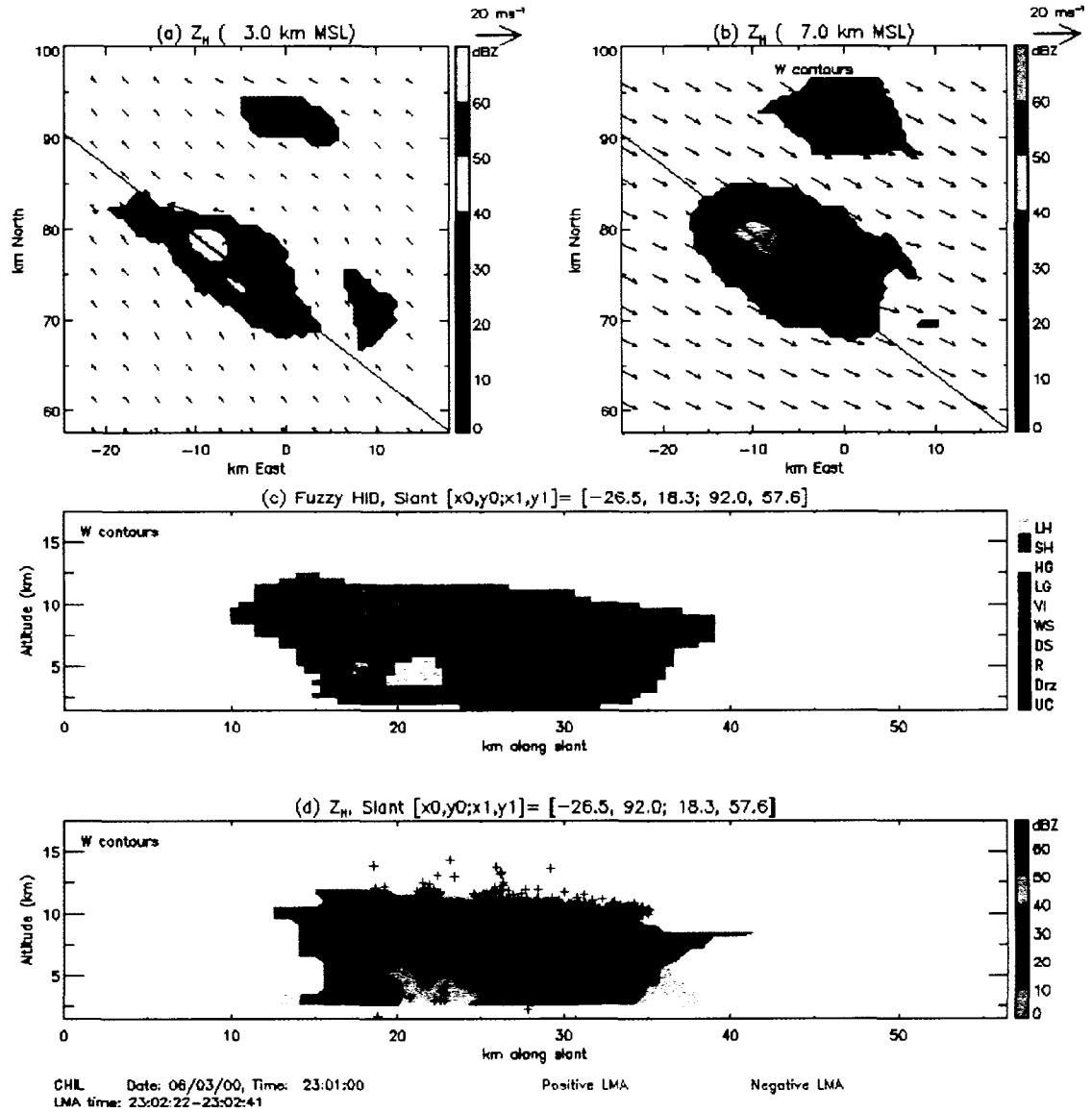
Figure 7. KGLD horizontal radar reflectivity ( Z_h ) at 2301 at (a) z = 3 km and (b) z = 7 km; fuzzy logic hydrometeor classification (FHC; using polarimetric data from CHILL along slanted black line in (a) and (b) is in (c), and grayscale contours of KGLD Z_h along slanted black line in (a) and (b) is in (d). Updraft velocity contours beginning at 10 \text{ m s}^{-1} (with a 10 \text{ m s}^{-1} contour interval) are overlaid in black in (b) and (c) and in pink in (d). LMA data of four representative flashes between 23:02:22-23:02:41 has been overlaid as small plus symbols onto (d) by inferred charge (red = positive, green = negative). Storm relative wind vectors have been overlaid onto (a) and (b). FHC categories are: large hail (LH), small hail (SH), high-density graupel (HG), low-density graupel (LG), vertically oriented ice crystals (VI), wet snow (WS), dry snow (DS), rain (R), drizzle (Drz), and unclassified (UC). Note: the LMA sources atop the storm appear to not be within reflectivity echo, but the 0 and 10 dBZ contours around the periphery of the storm are partially missing, either due to scanning/gridding geometry or the editing algorithms deleting echo in low signal-to-noise regions.
