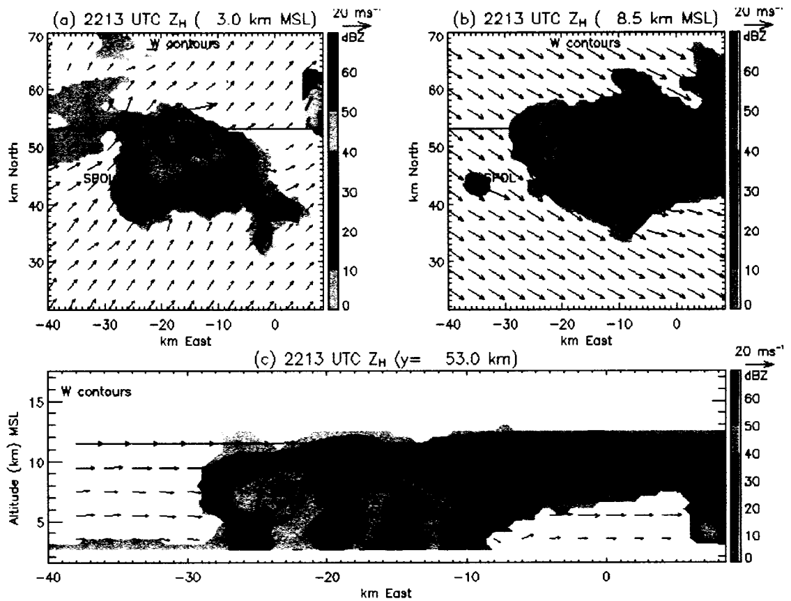
Figure 7. Winds and storm structure illustrating the temporal boundary between the early developing and ordinary mature phases at 2213: (a) horizontal cross-section of grayscale reflectivity at z = 3 km and bold black updraft contours beginning at 5 \text{ m s}^{-1} with a contour interval of 10 \text{ m s}^{-1} (due to the weak updrafts at this synthesis time no contours are evident in this frame), (b) horizontal cross-section of grayscale reflectivity at z = 8.5 km with bold black updraft contours beginning at 15 \text{ m s}^{-1} with a contour interval of 15 \text{ m s}^{-1} (again, no contours are evident in this frame due to the weak updrafts at this time), and (c) vertical cross-section of grayscale reflectivity at y = 53 km with bold black updraft contours beginning at 5 \text{ m s}^{-1} with a contour interval of 10 \text{ m s}^{-1} . All plots have storm-relative wind vectors overlaid.
