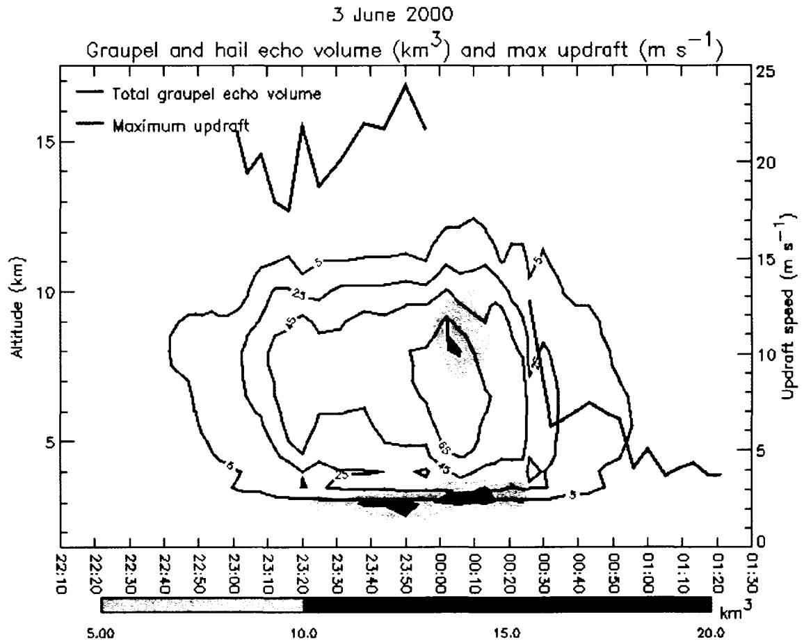
Figure 3. Time-height contours of total graupel echo volume and total hail echo volume (gray shaded contours), and maximum updraft time series (values on right axis) for 3 June 2000.
