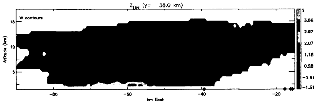
Figure 15. Vertical cross-section at y = 38 km (same as in Fig. 13) of differential reflectivity ( Z_{dr} ) at 0015 on 23 June 2000, with black updraft contours every 10 \text{ m s}^{-1} , beginning with 10 \text{ m s}^{-1} .
