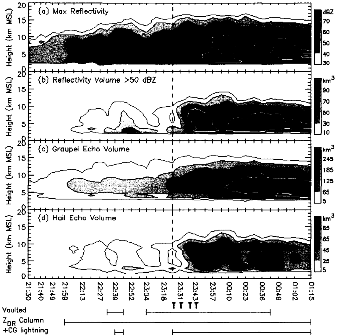
Figure 13. Same as Figure 12, except (a) maximum reflectivity (dBZ), (b) reflectivity volume (km 3 ) greater than 50 dBZ, (c) FHC total graupel (low-density + high-density) echo volume (km 3 ), contours beginning at 5 km 3 with a contour interval of 60 km 3 , and (d) FHC total hail (small + large) echo volume (km 3 ), contours beginning at 5 km 3 with a contour interval of 20 km 3 .
