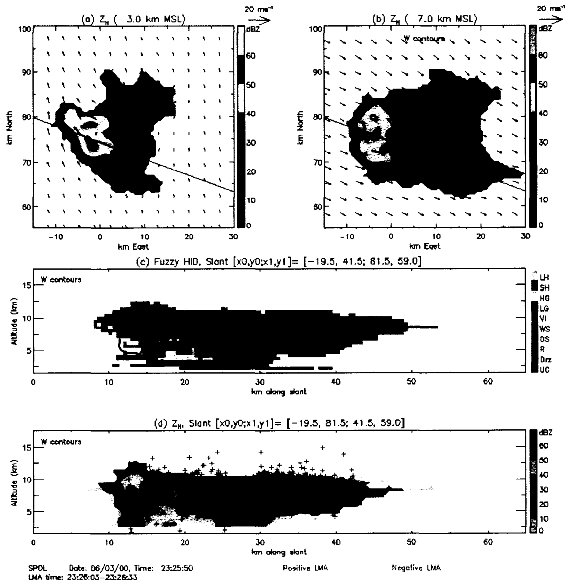
Figure 8. Same as Fig. 7, except for at 2325, the vertical cross-sections in (c) and (d) are at a slanted line shown in (a) and (b), and the FHC used polarimetric data from SPOL. LMA data of four representative flashes from 23:26:03-23:26:33 is overlaid in (d).
