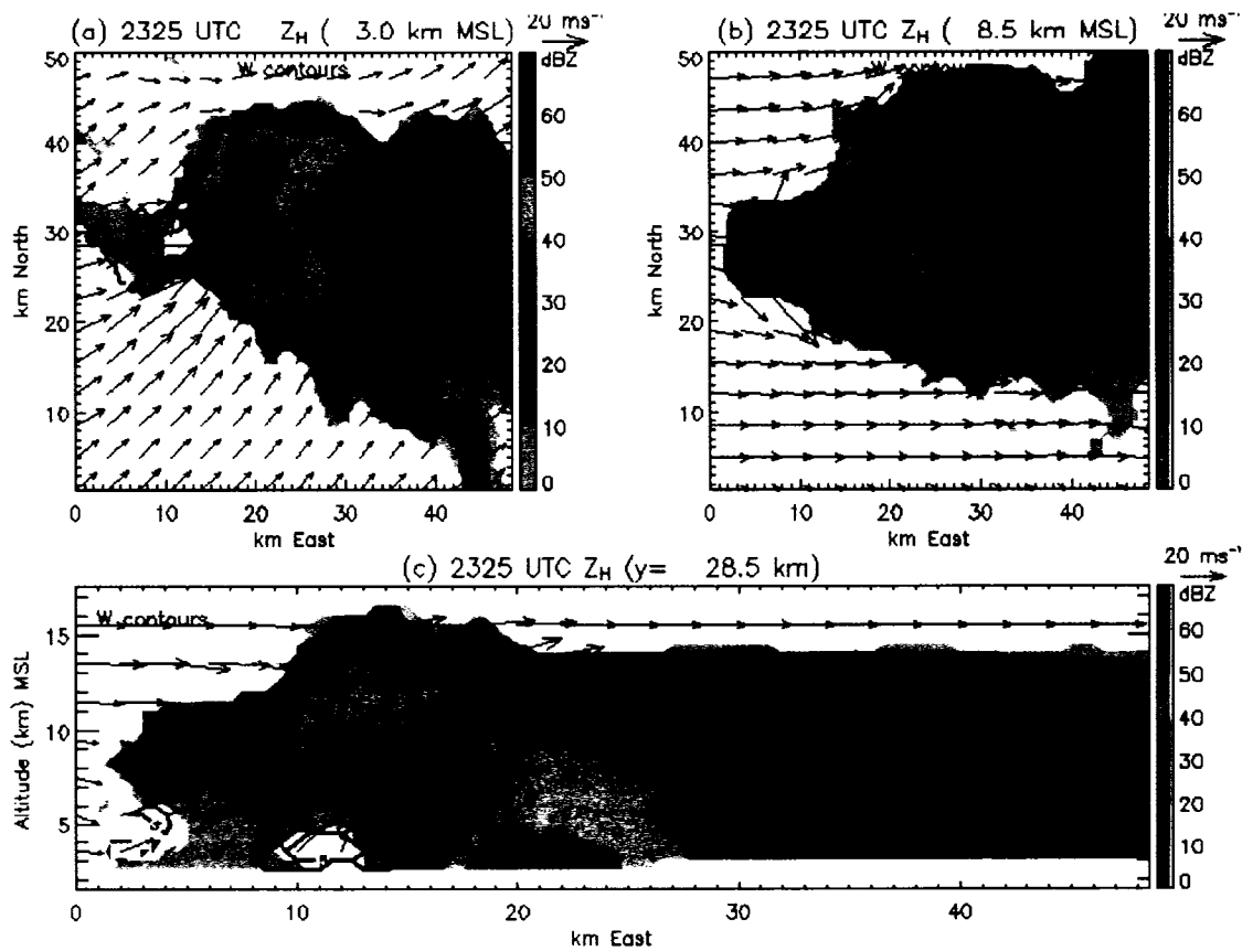
Figure 9. Same as Figure 7, except for synthesis representing the beginning of the tornadic period within the SR mature phase at 2325 and (c) y = 28.5 km.
