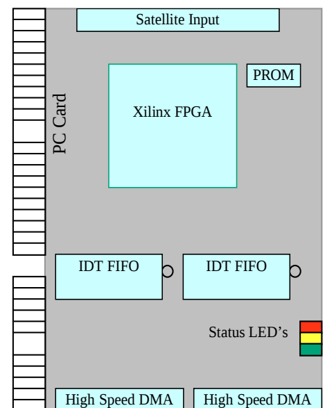
Figure 2. Hardware Processor Layout
