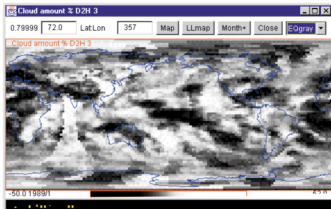
Figure 4. Significant cloud anomalies occurred in the 1989 El Nino areas in the central Pacific. Also there were large changes in cloud cover over Europe in the 1989 winter. This picture shows an example month: January 1989 ISCCP cloudiness anomaly from the January mean.
