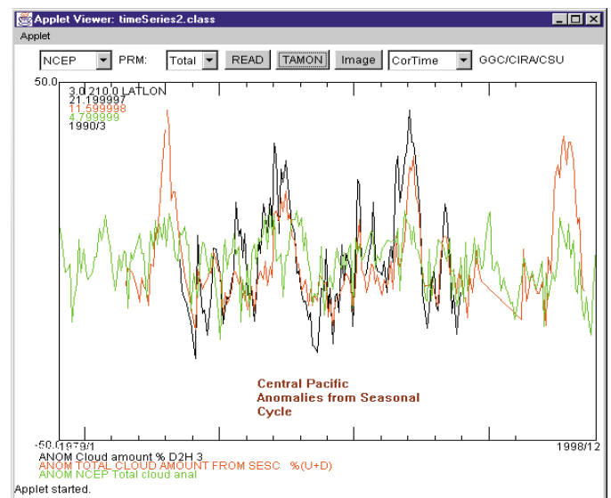
Figure 2. Time series of monthly anomalies : ISCCP, AVHRR Pathfinder, and NCEP Reanalysis
