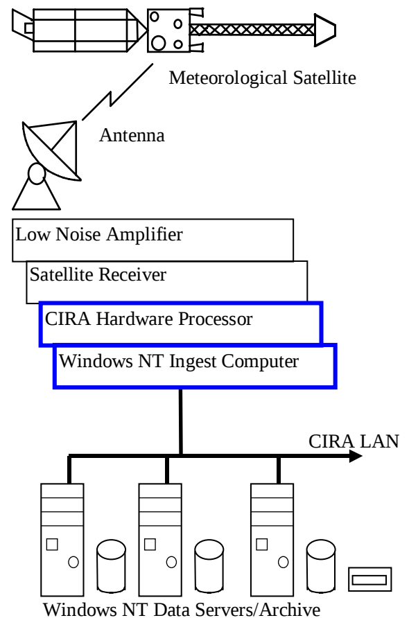
Figure 1. CIRA Earthstation Topology
