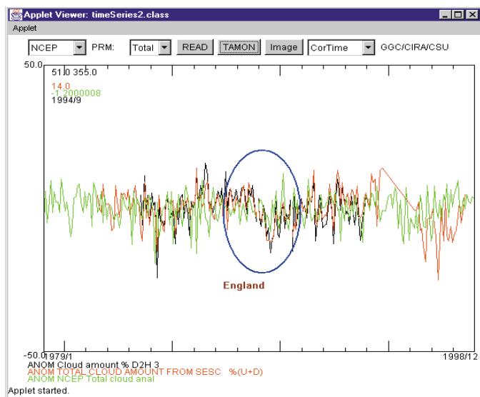
Figure 3. Time series of monthly anomalies for England: ISCCP, AVHRR Pathfinder, and NCEP Reanalysis
