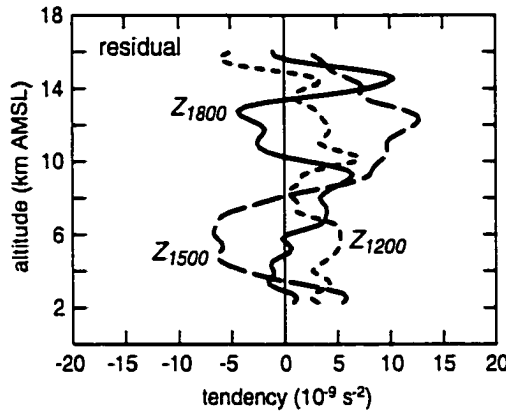
Figure 4.16: Residuals in the vorticity budget of observed wind. Contributions to the vorticity tendency are at 1200 UTC (short dashed), 1500 UTC (long dashed), and 1800 UTC (solid). Profiles are for a 2^\circ \times 2^\circ area centered on the MCV in the middle troposphere, averaged over 3 h ending at the time labeled on 1 August 1996.
