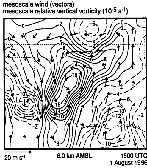
Figure 2.4: Mesoscale wind ( \text{m s}^{-1} ) and vorticity ( 10^{-5} \text{ s}^{-1} ) at 6.0 km AMSL at 1500 UTC on 1 August 1996.
