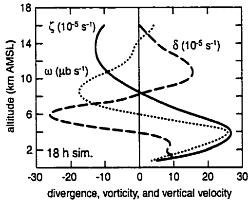
Figure 4.14: Kinematical averages in the numerically simulated MCV of 10–11 June 1985. Profiles are for the mature stage of the MCV and the decaying stage of the MCS. Relative vorticity ( 10^{-5} \text{ s}^{-1} ) is solid, divergence ( 10^{-5} \text{ s}^{-1} ) is dashed, and vertical velocity ( \mu\text{b s}^{-1} ) is dotted. Profiles are for a 100 \times 100 \text{ km} area centered on the MCV after an 18 h simulation. [Adapted from a figure by Zhang (1992).]
