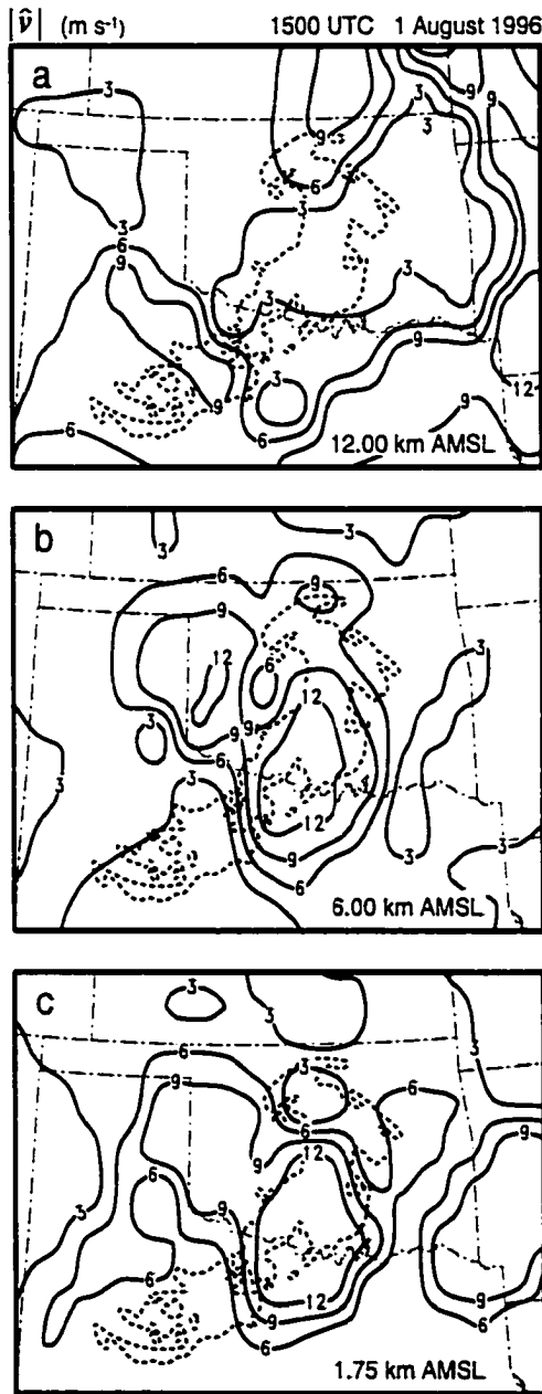
Figure 4.8: Speed of the mesoscale perturbation in wind at 1500 UTC on 1 August 1996. Contours are every 3 m s -1 at a) 12.00, b) 6.00, and c) 1.75 km AMSL. The contour of 15 dBZ reflectivity within the MCS is dashed.
