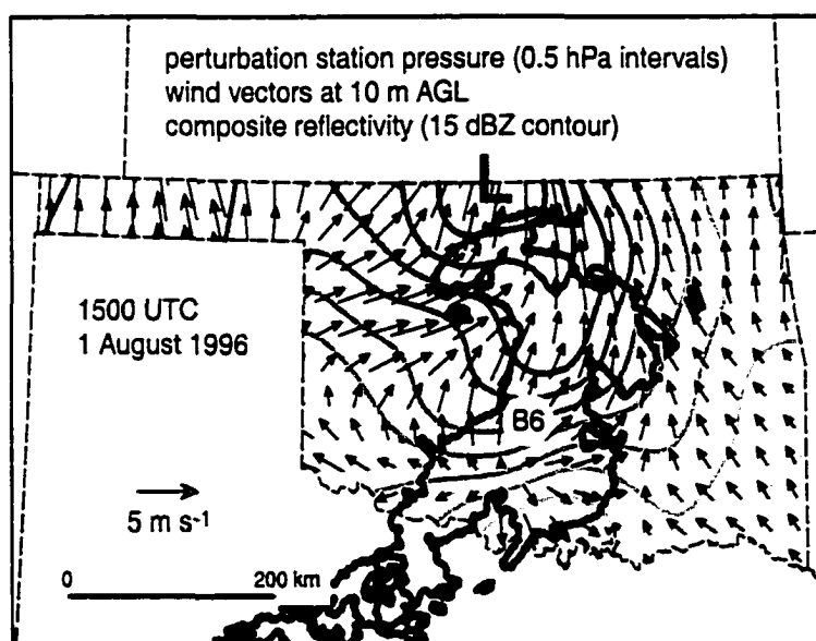
Figure 5.7: Radar reflectivity and surface conditions within the Oklahoma Mesonet at 1500 UTC on 1 August 1996. Surface pressure is contoured every 0.5 hPa in gray; values are deviations from a state-wide mean and darker grays indicate lower pressure. Vectors depict wind at 10 m AGL. The thick black contours outline reflectivity \geq 15 dBZ. The GCIP site at Purcell, OK is marked by "B6."
