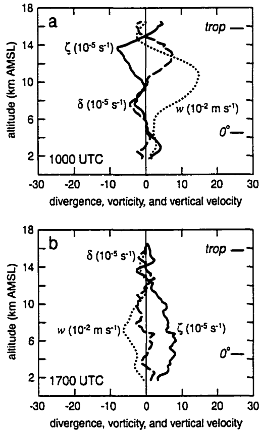
Figure 4.11: Kinematical averages in the MCV at 1000 and 1700 UTC on 1 August 1996. Relative vorticity ( 10^{-5} \text{ s}^{-1} ) of observed wind is solid, divergence ( 10^{-5} \text{ s}^{-1} ) is dashed, and vertical velocity ( 10^{-2} \text{ m s}^{-1} ) is dotted. Times are a) 1000 and b) 1700 UTC. Profiles are for a 2^\circ \times 2^\circ area centered on the MCV. Unlike in fig. 4.10, profiles are not for 3-h averages. The levels of 0^\circ\text{C} in the environment and the tropopause are marked along the right side of each panel.
