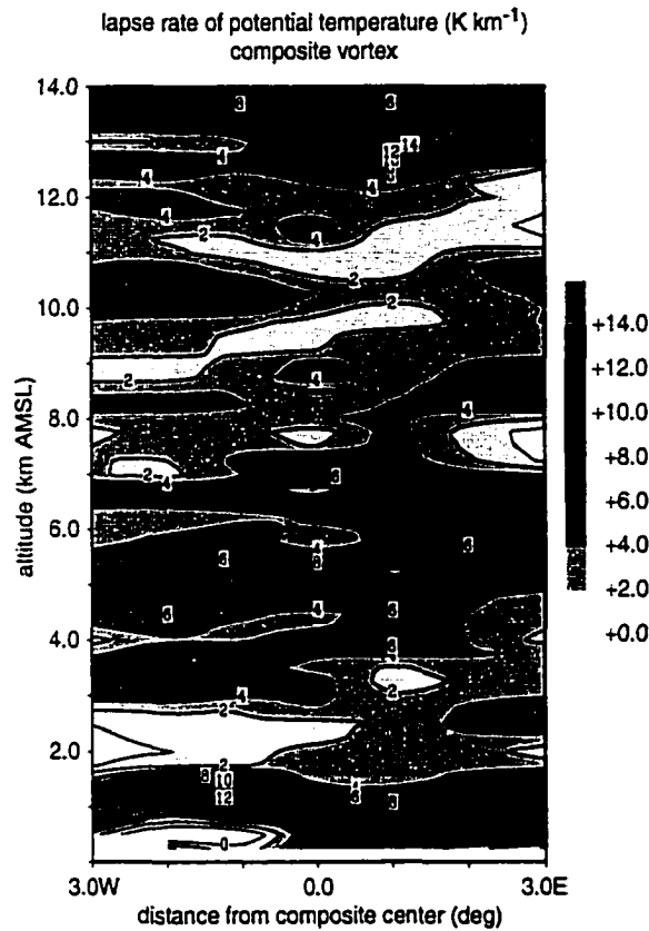
Figure 5.13: Lapse rate in potential temperature within the composite MCV. Contours and shading are every 2 \text{ K km}^{-1} .
