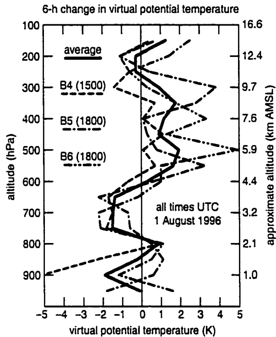
Figure 5.8: Changes in virtual potential temperature (K) within the MCSV over 6 h. Profiles are from soundings above Vici, OK (B4; dashed), Morris, OK (B5; dash-dot-dotted), and Purcell, OK (B6; dash-dot-dotted). The thick solid line shows the average profile. The 6-h intervals end at the times shown. The first of each sounding pair used to calculate the difference was taken ahead of the MCS and MCSV; the second of each was taken within the MCSV. Data are plotted every 50 hPa.
