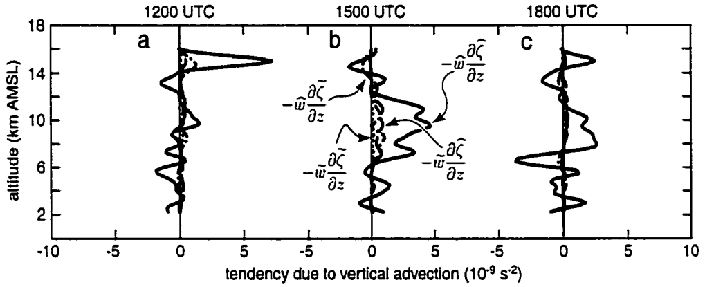
Figure 4.18: Components of vertical advection in the vorticity budget. Terms are: advection of mesoscale perturbation in vorticity by the mesoscale perturbation in wind (solid) and by the synoptic wind (dashed), and advection of synoptic vorticity by the mesoscale perturbation in wind (dashed-dotted) and by the synoptic wind (dotted). Profiles are for a 2^\circ \times 2^\circ area centered on the MCV in the middle troposphere, averaged over 3 h ending at the time labeled on 1 August 1996.
