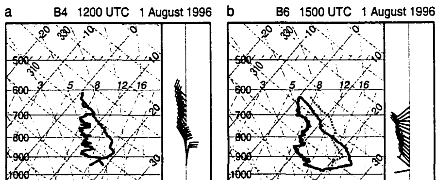
Figure 5.6: Temperature and dew point beneath the trailing anvil of the MCS on 1 August 1996. Profiles are plotted on a skew- T /log- p diagram. The soundings were above a) Vici, OK (B4) at 1200 UTC and b) Purcell, OK (B6) at 1500 UTC. Half and full wind barbs respectively represent 5 and 10 \text{m s}^{-1} . Both sondes stopped transmitting data at approximately the altitudes of 0°C.
