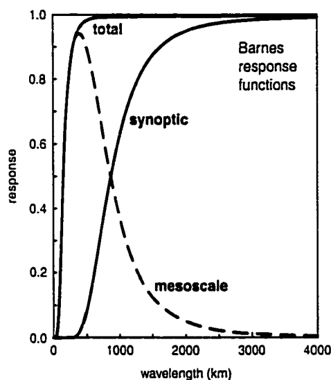
Figure 2.2: Response functions for the Barnes analyses.
