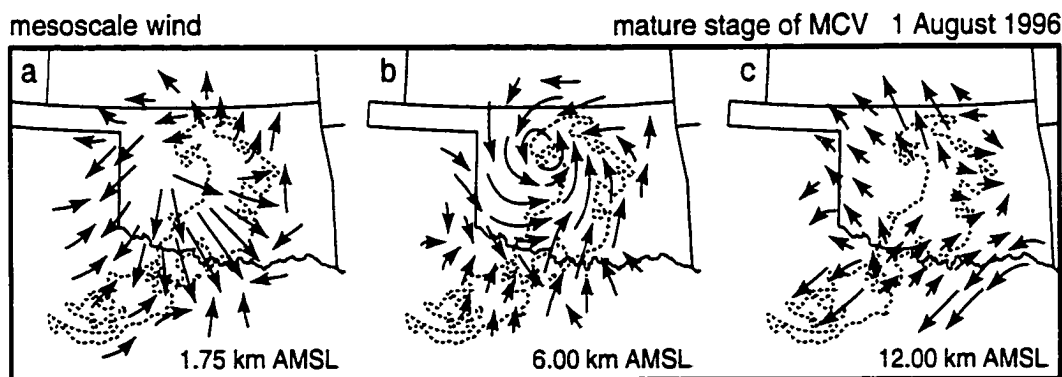
Figure 4.5: Schemata of the mesoscale perturbation in wind during the MCV's maturity on 1 August 1996. Horizontal wind is at altitudes of a) 1.75 km, b) 6.00 km, and c) 12.00 km AMSL. Arrows are a hybrid of vectors and streamlines, so their lengths roughly indicate relative wind speed. The contour of 15 dBZ reflectivity within the MCS is dashed.
