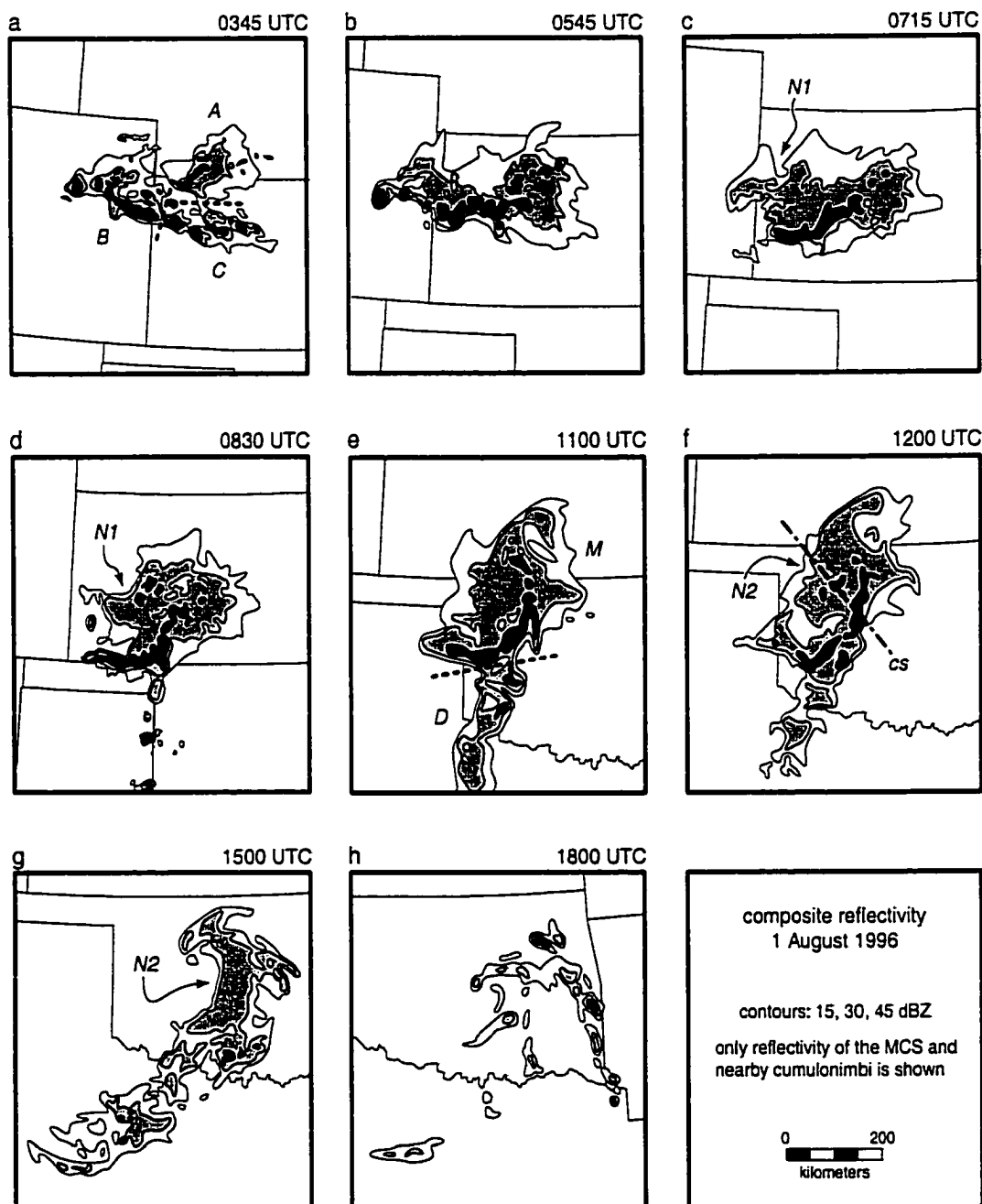
Figure 3.4: Composite base-scan reflectivity at eight times on 1 August 1996. Times are a) 0345, b) 0545, c) 0715, d) 0830, e) 1100, f) 1200, g) 1500, and h) 1800 UTC. Contours are at 15, 30, and 45 dBZ. Only reflectivity due to the MCS and nearby cumulonimbi is shown. Three clusters that merged to form the incipient MCS are separated by dashed lines and marked with A , B , and C . A band of cumulonimbi that was overtaken by the MCS, M , is marked by D . Notches are marked by N1 and N2 . The location of the cross section in fig. 4.4 is marked by cs .
