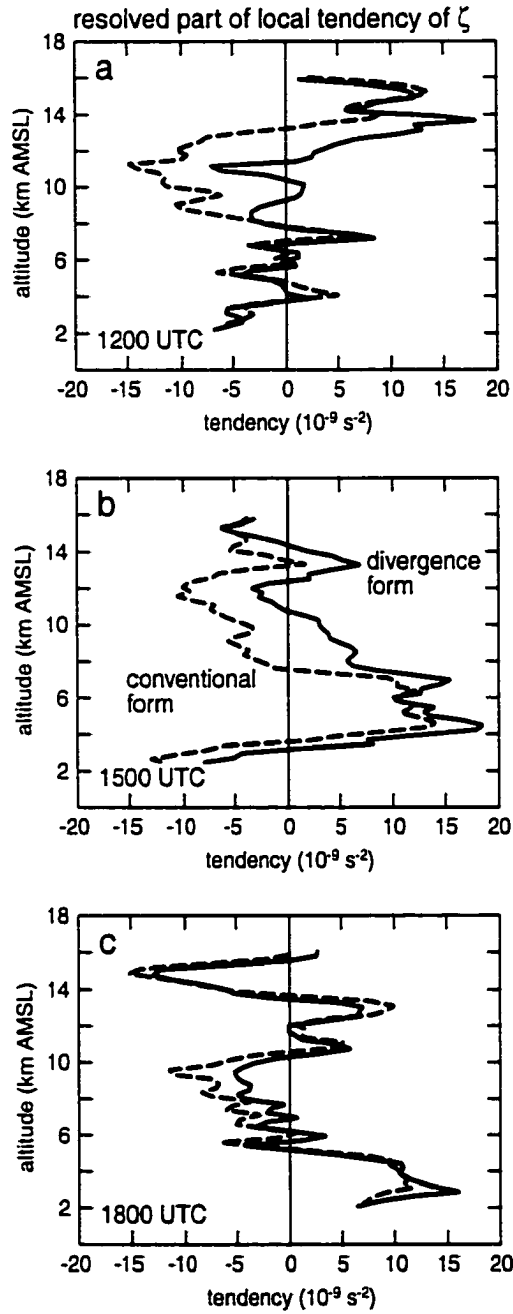
Figure 4.21: Resolved part of the local tendency of relative vorticity calculated according to the conventional (dashed) and divergence (solid) forms of the budget. Profiles are at a) 1200 UTC, b) 1500 UTC, and c) 1800 UTC on 1 August 1996 for a 2^\circ \times 2^\circ area centered on the MCV in the middle troposphere; the profiles have not been otherwise averaged or smoothed.
