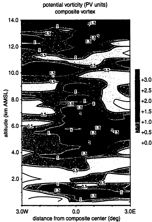
Figure 5.11: Potential vorticity within the composite MCV. Contours and shading are every 0.5 \times 10^{-7} \text{ m}^2 \text{ s}^{-1} \text{ K kg}^{-1} . Horizontal distance is from the center of the composite vortex.
