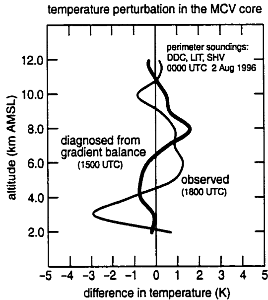
Figure 5.10: Balanced and observed temperature perturbations within the MCV. Both perturbations (K) are with respect to a far-field profile approximated with soundings above Dodge City, KS (DDC), Little Rock, AR (LIT), and Shreveport, LA (SHV) at 0000 UTC on 2 August 1996. The thin line is the observed profile from near the MCV's core above Purcell, OK (B6) at 1800 UTC on 1 August. The thick line is a retrieved profile in gradient balance with the MCV's wind field at 1500 UTC. Data are plotted every kilometer and smoothed.
