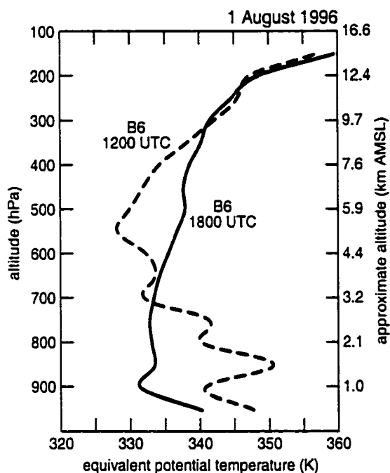
Figure 5.3: Equivalent potential temperature (K) above Purcell, OK (B6) on 1 August 1996. The sounding at 1200 UTC (dashed) was ahead of the MCS. The sounding at 1800 UTC (solid) was very near the center of the MCV. Data are plotted every 50 hPa and smoothed.
