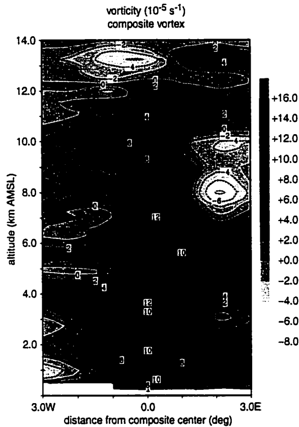
Figure 5.12: Relative vorticity within the composite MCV. Contours and shading are every 2 \times 10^{-5} \text{ s}^{-1} .
