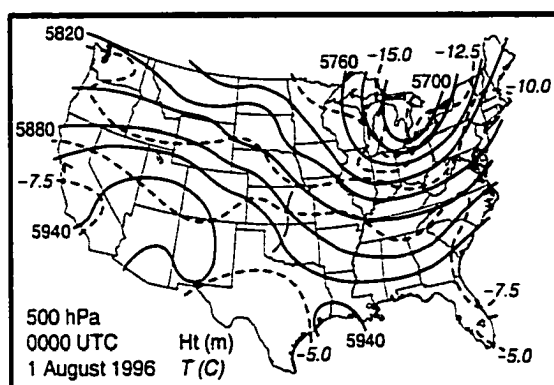
Figure 3.1: Height (m AMSL) and temperature (°C) at 500 hPa at 0000 UTC on 1 August 1996. The thin line with long dashes marks the axis of a short-wave trough.
