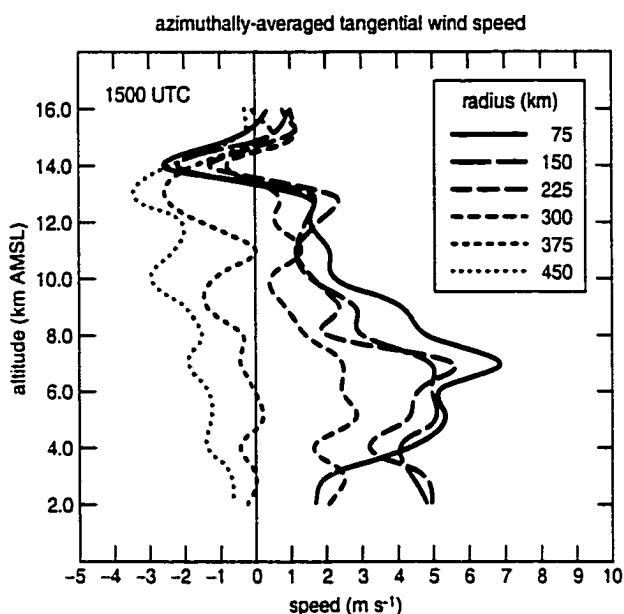
Figure 5.9: Azimuthally-averaged tangential wind speed ( \text{m s}^{-1} ) within the MCV at 1500 UTC on 1 August 1996. Radii are from 75 to 450 km at intervals of 75 km; the key indicates the lines for each radius. Data are plotted every kilometer and smoothed.
