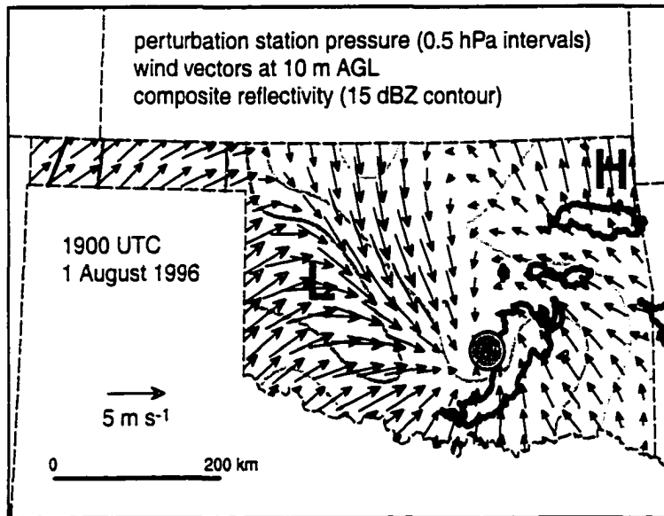
Figure 4.12: Radar reflectivity and surface conditions within the Oklahoma Mesonet at 1900 UTC on 1 August 1996. Surface pressure is contoured every 0.5 hPa in gray; values are deviations from a state-wide mean and darker grays indicate lower pressure. Vectors depict wind at 10 m AGL. The thick black contours outline reflectivity \geq 15 dBZ. The gray circle marks the middle-tropospheric center of the MCV.
