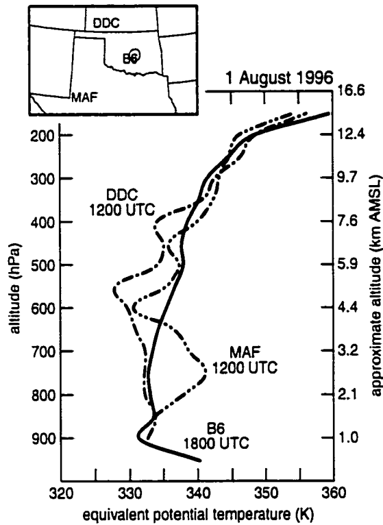
Figure 5.1: Equivalent potential temperature (K) in, and west of, the stratiform region of the MCS on 1 August 1996. Soundings were above Purcell, OK (B6), near the center of the MCV at 1800 UTC (solid), and west of the MCS at Dodge City, KS (DDC; dot-dashed) and Midland, TX (MAF; dot-dot-dashed) at 1200 UTC. The inset map shows the locations of the soundings and the center of the MCV at 1800 UTC (marked by the gray circle). Data are plotted every 50 hPa and smoothed.
