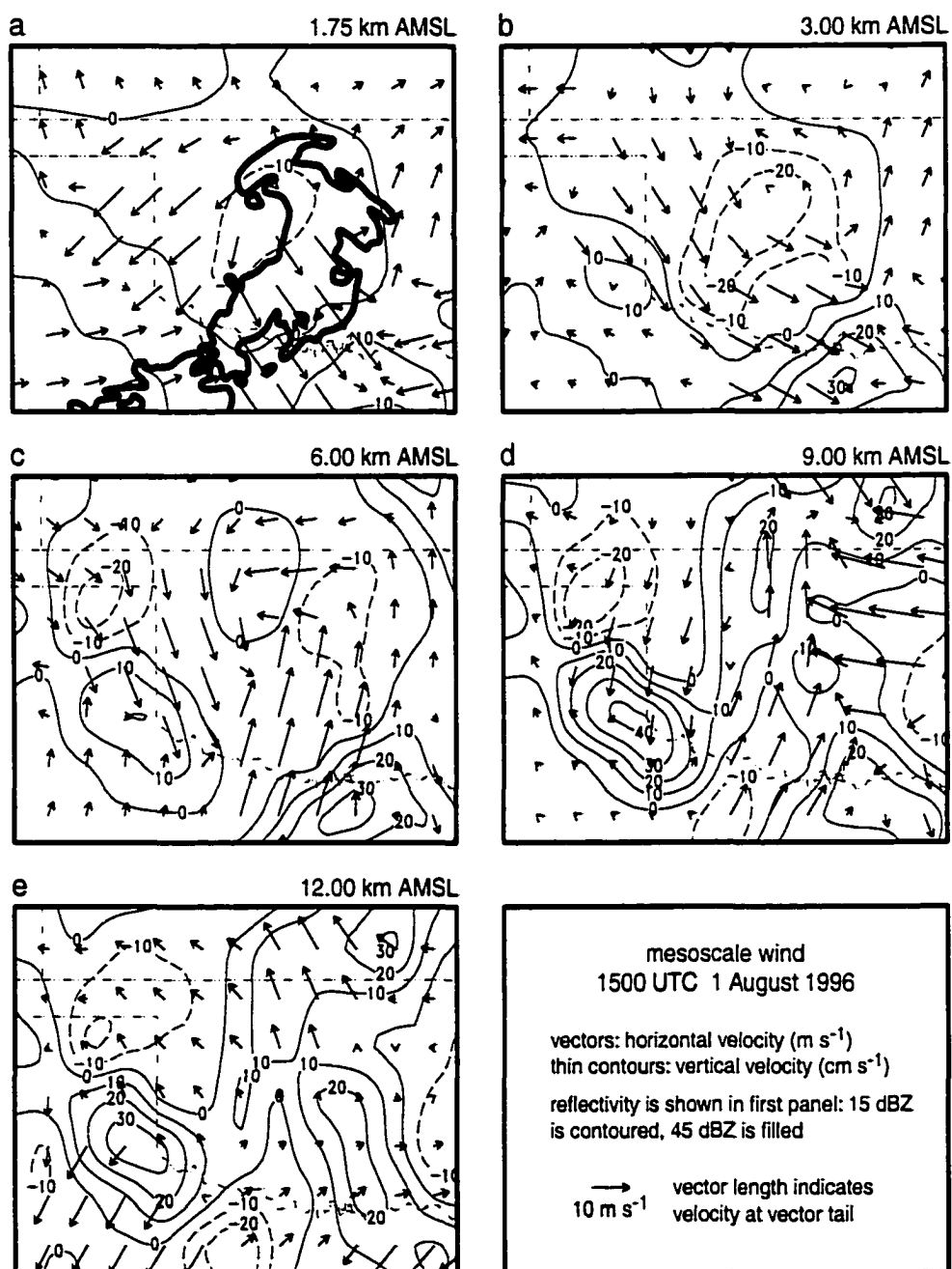
Figure 4.3: Three components of the mesoscale wind at 1500 UTC on 1 August 1996. The altitudes are a) 1.75 km, b) 3.00 km, c) 6.00 km, d) 9.00 km, and e) 12.00 km AMSL. Vectors represent horizontal velocity, and vertical velocity is contoured in thin lines every 10 \text{ cm s}^{-1} . In the first panel, reflectivity of 15 dBZ is contoured in the thick line and >45 \text{ dBZ} is filled.
