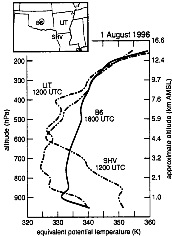
Figure 5.2: Equivalent potential temperature (K) in, and east of, the stratiform region of the MCS on 1 August 1996. Soundings were above Purcell, OK (B6), near the center of the MCV at 1800 UTC (solid), and east of the MCS at Little Rock, AR (LIT; dot-dashed) and Shreveport, LA (SHV; dot-dot-dashed) at 1200 UTC. The inset map shows the locations of the soundings and the center of the MCV at 1800 UTC (marked by the gray circle). Data are plotted every 50 hPa and smoothed.
