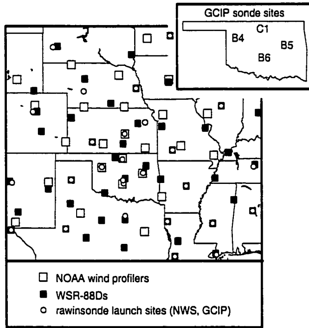
Figure 2.1: Sites of observations above the ground. NOAA wind profilers are marked by large open squares, WSR-88Ds by small solid squares, and radiosonde launch sites of the NWS and GCIP ESOP-96 by small open circles.
