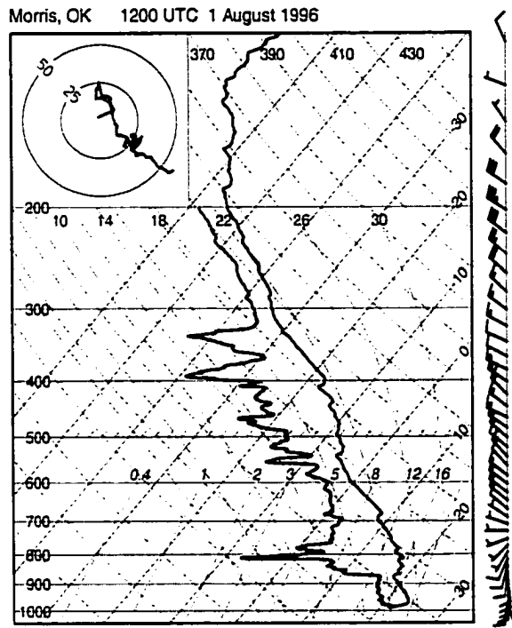
Figure 3.2: Sounding above Morris, OK (B4) at 1200 UTC on 1 August 1996. Half and full wind barbs respectively represent 2.5 and 5.0 \text{ m s}^{-1} . CAPE was 436 \text{ J kg}^{-1} and CIN was 198 \text{ J kg}^{-1} . This sounding is representative of those taken ahead of the MCS early on 1 August.
