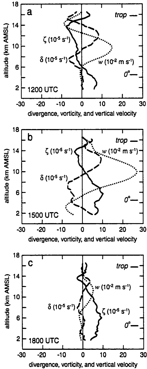
Figure 4.10: Kinematical averages in the MCV from 1200 to 1800 UTC on 1 August 1996. Relative vorticity ( 10^{-5} \text{ s}^{-1} ) of observed wind is solid, divergence ( 10^{-5} \text{ s}^{-1} ) is dashed, and vertical velocity ( 10^{-2} \text{ m s}^{-1} ) is dotted. Profiles are for a 2^\circ \times 2^\circ area centered on the MCV in the middle troposphere, averaged over 3 h ending at the time labeled. The levels of 0^\circ\text{C} in the environment and the tropopause are marked along the right side of each panel.
