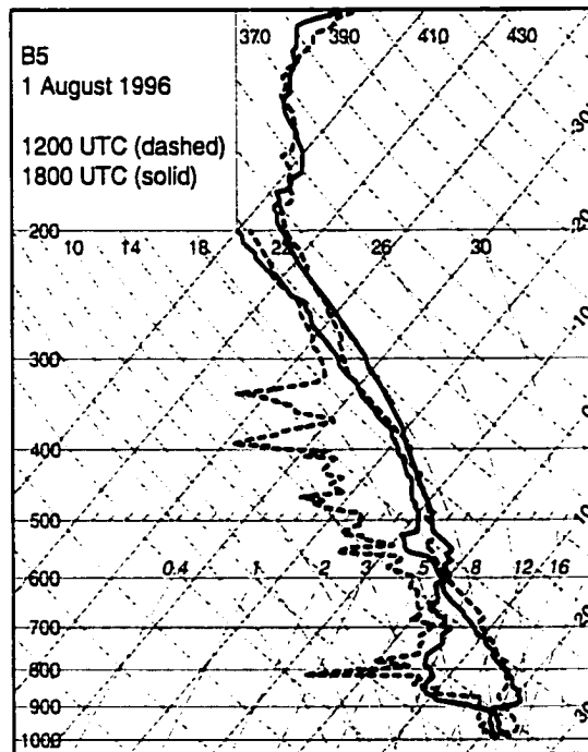
Figure 5.4: Soundings above Morris, OK (B5) plotted on a skew- T/\ln-p diagram. Traces are dew point (left pair of lines) and temperature (right pair of lines) at 1200 UTC (dashed) and 1800 UTC (solid) on 1 August 1996.
