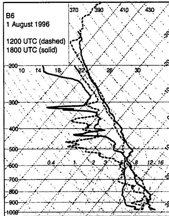
Figure 5.5: Soundings above Purcell, OK plotted on a skew- T/\ln-p diagram. Traces are dew point (left pair of lines) and temperature (right pair of lines) at 1200 UTC (dashed) and 1800 UTC (solid) on 1 August 1996.
