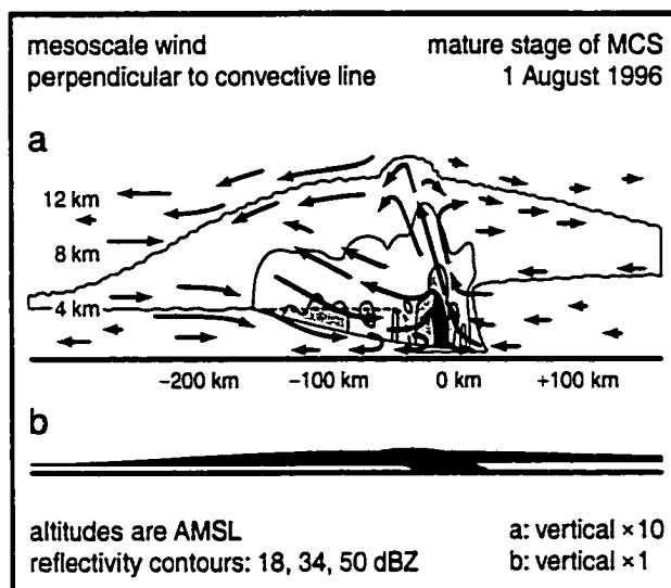
Figure 4.4: Schematic cross section of the mature MCS on 1 August 1996. Depicted are reflectivity and the cross-line component of the mesoscale perturbation in wind. Arrows are a hybrid of vectors and streamlines, so their lengths roughly indicate relative wind speed of consistently observed flows along various locations in the MCS as determined from the NPN at 1200 UTC and from cross sections of WSR-88D Doppler velocity from Oklahoma City, OK at 1233 to 1320 UTC. Contours, from outer to inner, are cloud edge and reflectivity of 18, 35, and 50 dBZ. Reflectivity is at 1233 UTC along the cross section shown in figure 3.4f. The bottom edge of the reflectivity cross section is due to the lower limit of the lowest radar scan. Cloud top is from a GOES 8 IR image at 1215 UTC along the same cross section; cloud bottom is estimated from GCIP soundings at 1200 UTC and from other studies of MCSs. Height is exaggerated by a factor of ten in the top schema; the bottom schema is an unexaggerated silhouette.
