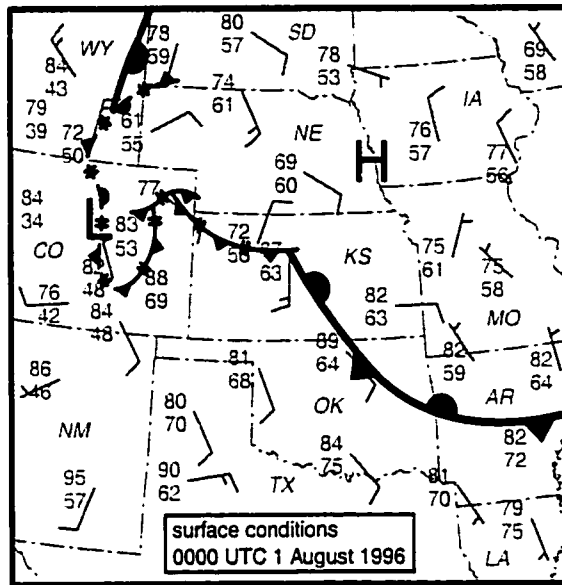
Figure 3.3: Synoptic and mesoscale fronts at 0000 UTC on 1 August 1996. Station models display temperature, dew point (both °F), and wind, for which full and half barbs respectively represent 2.5 and 5.0 m s -1 . An absent vector indicates a missing observation, not necessarily calm conditions. Regions of locally high and low pressure are respectively marked by Hs and Ls.
