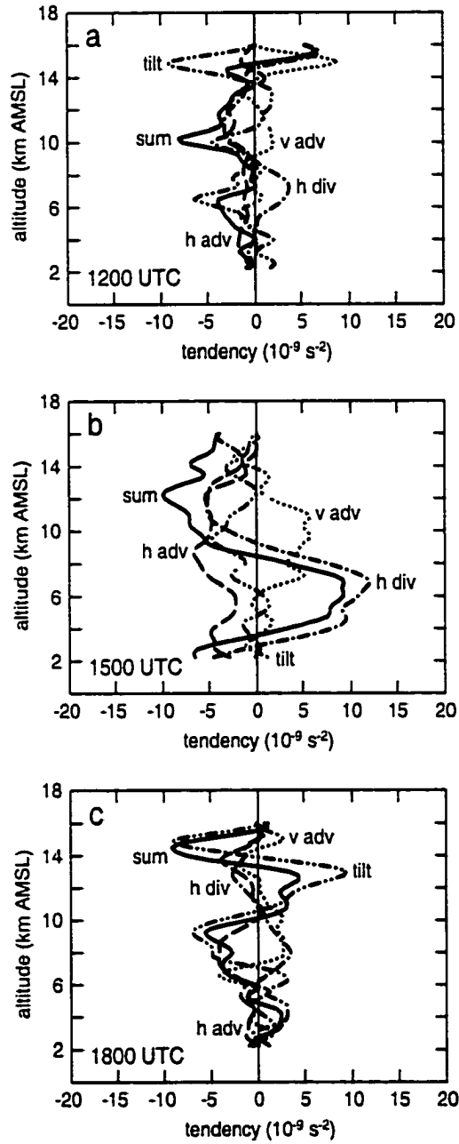
Figure 4.15: Resolved part of the vorticity budget for observed wind. Terms are: horizontal advection (dashed), vertical advection (dotted), divergence (dot-dashed), tilting (dot-dot-dashed), and the sum of terms (solid). Profiles are for a 2^\circ \times 2^\circ area centered on the MCV in the middle troposphere, averaged over 3 h ending at the time labeled on 1 August 1996.
