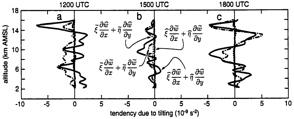
Figure 4.20: Components of tilting in the vorticity budget. Terms are: tilting of vertical shear of the mesoscale perturbation in wind by the horizontal gradient of mesoscale perturbation in vertical motion (solid) and by the horizontal gradient of synoptic vertical motion (dashed), and tilting of vertical shear of the synoptic wind by the horizontal gradient of mesoscale perturbation in vertical motion (dashed-dotted) and by the horizontal gradient of synoptic vertical motion (dotted). Profiles are for a 2^\circ \times 2^\circ area centered on the MCV in the middle troposphere, averaged over 3 h ending at the time labeled on 1 August 1996.
