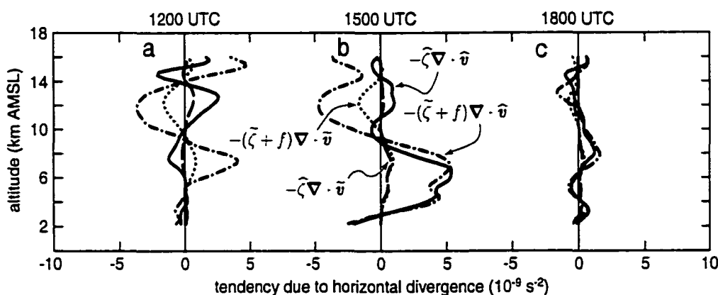
Figure 4.19: Components of horizontal convergence in the vorticity budget. Terms are: divergence of mesoscale perturbation in vorticity by the mesoscale perturbation in wind (solid) and by the synoptic wind (dashed), and divergence of synoptic vorticity by the mesoscale perturbation in wind (dashed-dotted) and by the synoptic wind (dotted). Profiles are for a 2^\circ \times 2^\circ area centered on the MCV in the middle troposphere, averaged over 3 h ending at the time labeled on 1 August 1996.
