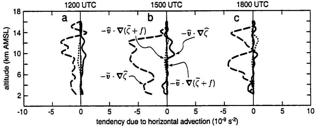
Figure 4.17: Components of horizontal advection in the vorticity budget. Terms are: advection of mesoscale perturbation in vorticity by the mesoscale perturbation in wind (solid) and by the synoptic wind (dashed), and advection of synoptic vorticity by the mesoscale perturbation in wind (dashed-dotted) and by the synoptic wind (dotted). Profiles are for a 2^\circ \times 2^\circ area centered on the MCV in the middle troposphere, averaged over 3 h ending at the time labeled on 1 August 1996.
