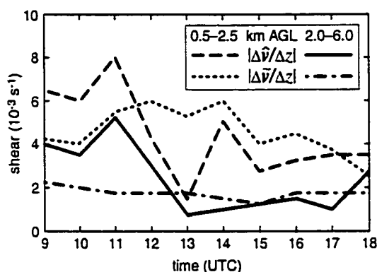
Figure 4.9: Vertical wind shear in the MCV from 0900 to 1800 UTC on 1 August 1996. Shears ( 10^{-3} \text{ s}^{-1} ) are at the MCV's center in the lower troposphere (0.5–2.5 km AGL) for the mesoscale perturbation in wind (dashed) and synoptic wind (dotted), and in the middle troposphere (2.0–6.0 km AGL) for the same components (solid and dash-dotted, respectively).
