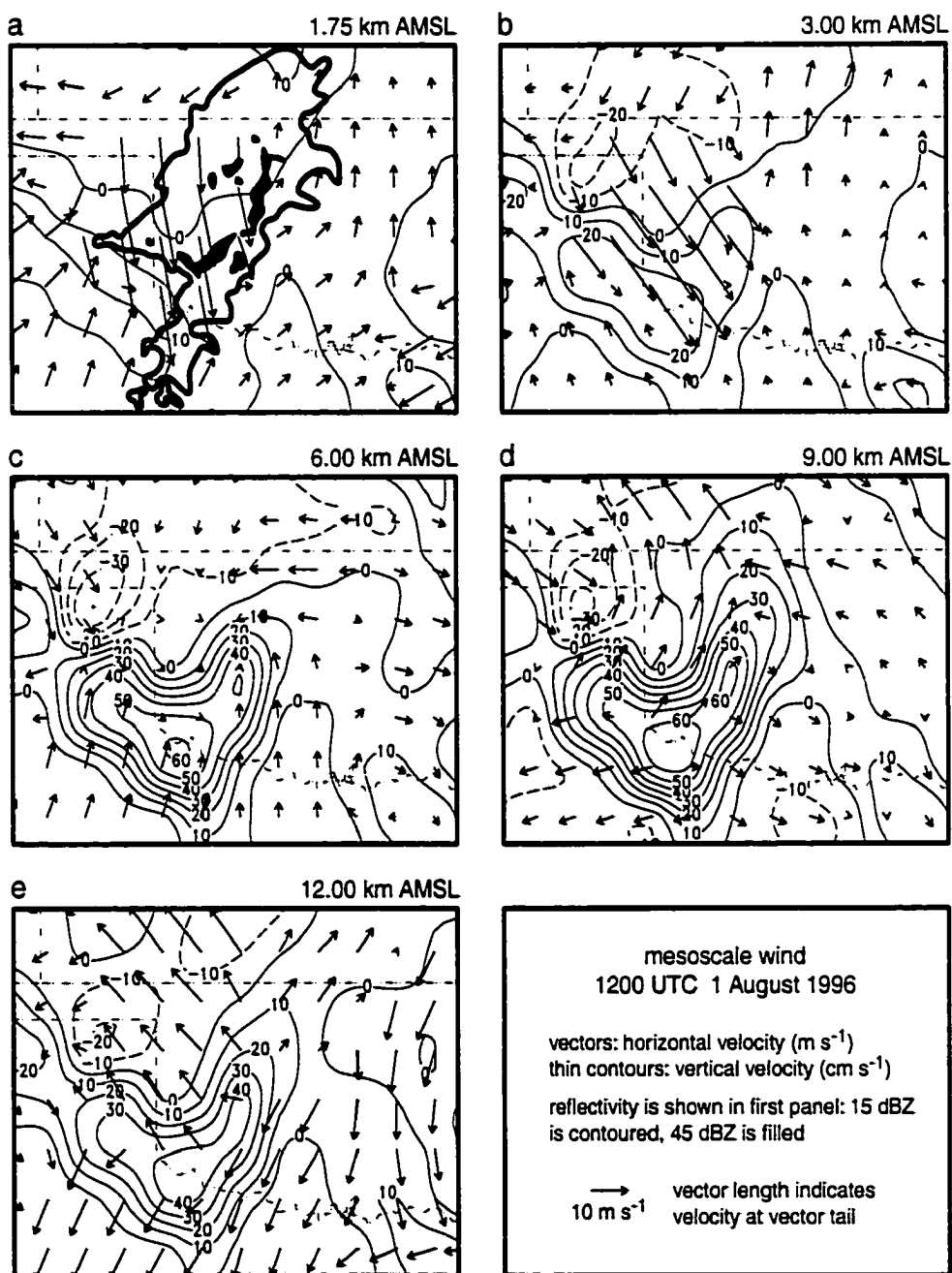
Figure 4.2: Three components of the mesoscale wind at 1200 UTC on 1 August 1996. The altitudes are a) 1.75 km, b) 3.00 km, c) 6.00 km, d) 9.00 km, and e) 12.00 km AMSL. Vectors represent horizontal velocity, and vertical velocity is contoured in thin lines every 10 \text{ cm s}^{-1} . In the first panel, reflectivity of 15 dBZ is contoured in the thick line and >45 \text{ dBZ} is filled.
