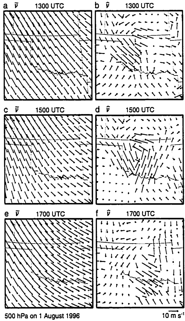
Figure 2.3: Synoptic and mesoscale winds at 500 hPa on 1 August 1996. The rows from top to bottom are for 1300, 1500, and 1700 UTC; the columns from left to right are the synoptic background wind and the mesoscale perturbation in wind.
