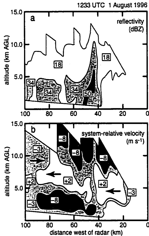
Figure 4.7: Cross section of level II data through the middle of the mature MCS at 1233 UTC on 1 August 1996. Panels show a) regions of reflectivity enclosed by contours of 18, 34, and 50 dBZ; and b) regions of system-relative radial wind enclosed by contours of 8 and 3 m s -1 toward the radar (westerlies), and 2 m s -1 away from the radar (easterlies). The section was taken along the 270° radian.
