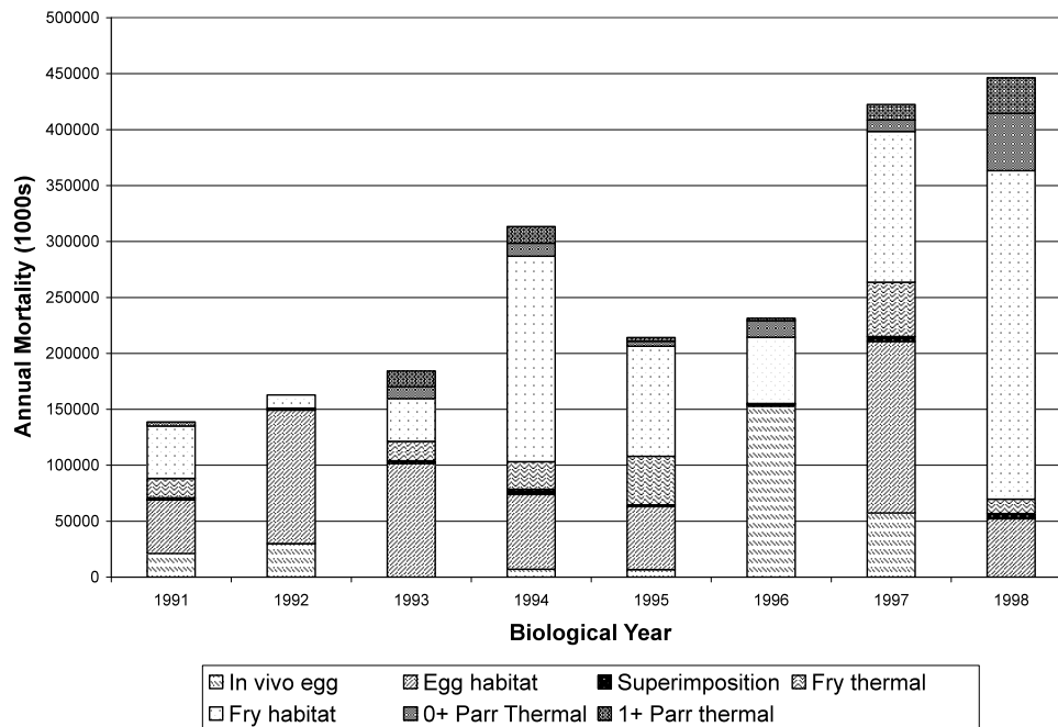
Figure 4. Example illustrating simulated annual variability in mortality for an Atlantic salmon population in the State of Maine. (Adapted from Bartholow et al. 2003).
