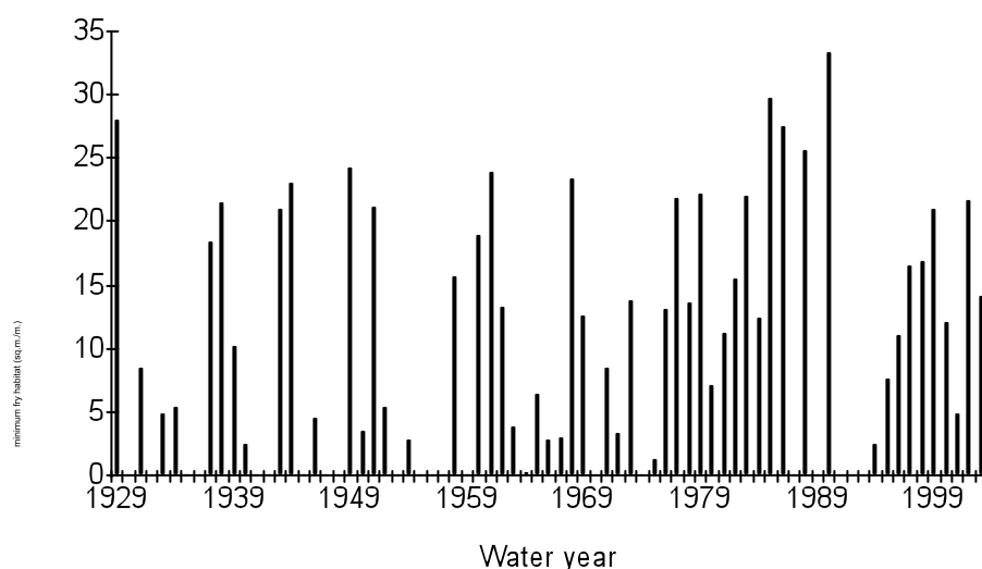
Figure 3. Annual minimum physical habitat for channel catfish fry in the Washita River near Dickson, OK. The annual minimum habitat is the physical habitat at the minimum 10-day average discharge. The streamflow data used was the daily discharge measured by USGS at the gage on the Washita River near Dickson, OK.
