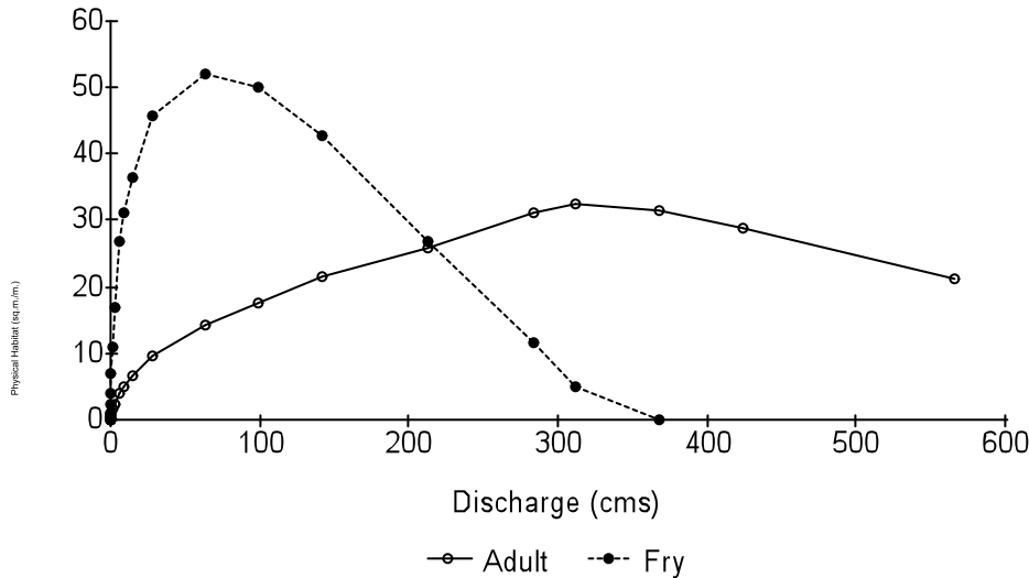
Figure 2. Physical habitat versus discharge relations for channel catfish in the Washita River near Dickson, OK. The velocity and depth data used in the analysis are from the discharge measurement summaries for the USGS gage at the site. The HABVD program in PHABSIM was used to calculate the relations.
