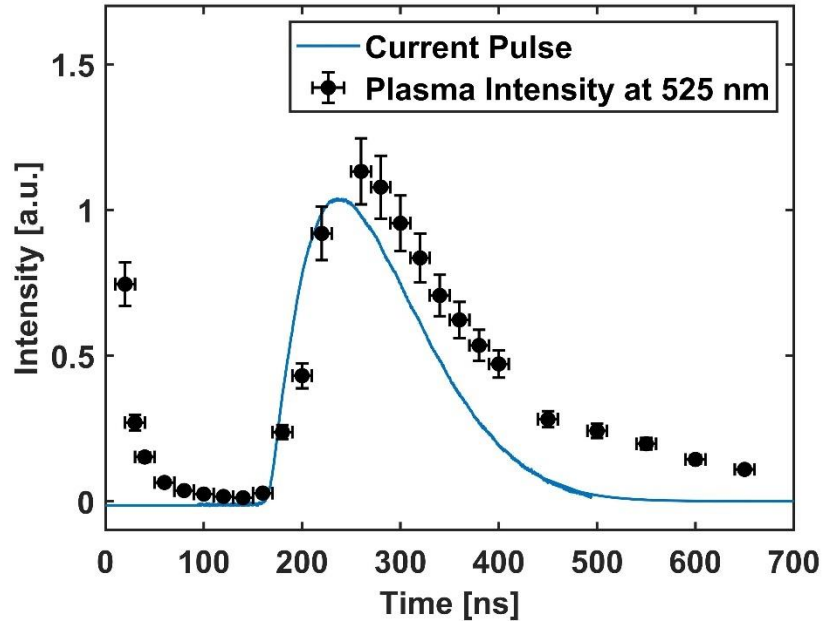
Figure 3-5 Plasma luminous intensity compared to the temporal evolution in current flow. Note that between t_0 and 180 ns, the laser induced plasma alone is present.
