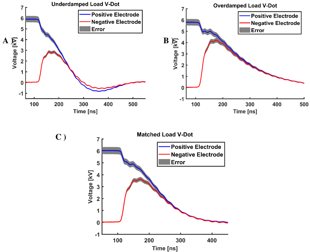
Figure 4-5 Calibrated V-Dot signals for corresponding to a 6 kV capacitor charge with a A) underdamped load, B) an overdamped load, and C) a matched load.
