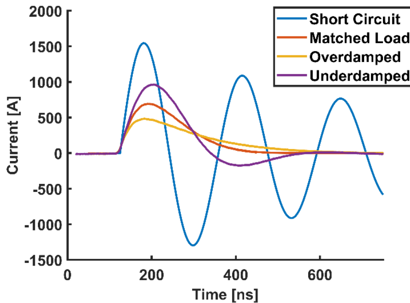
Figure 2-6 Current traces as measured by the current viewing resistor for several load configurations.
