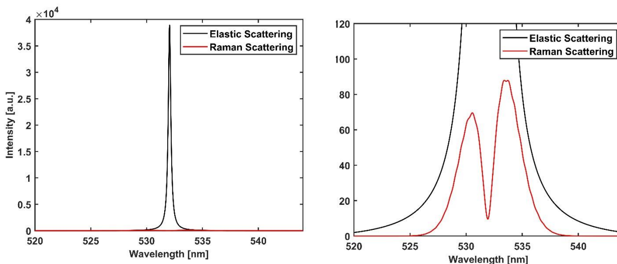
Figure 1-3 Left: Full scale comparison of elastic and Raman scattering. Right) Zoomed in version of left plot
