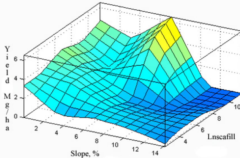
Figure 3. Yield-dependence on Slope and LnSCAfill computed using the two-input FIS.
