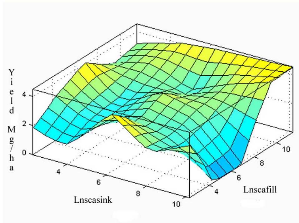
Figure 4. Yield-dependence on LnSCAsink and LnSCAfill computed using the two-input FIS.
