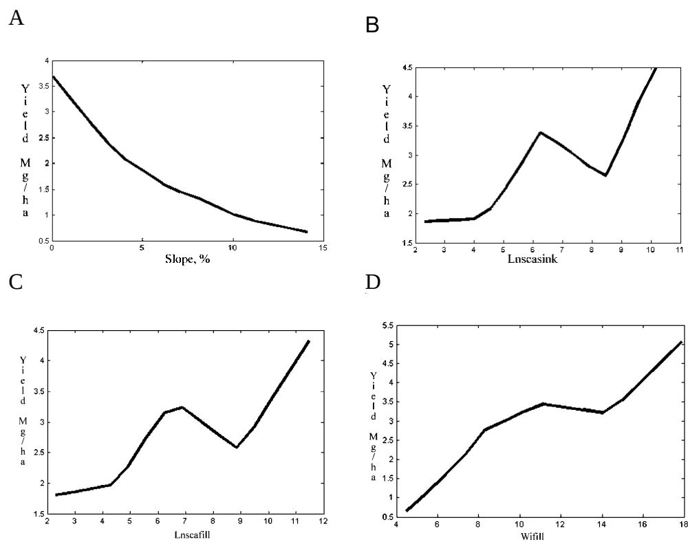
Figure 1. Yield-dependence of Slope (A), LnSCAsink (B), LnSCAfill (B), and Wifill (D) computed using the single-input FIS.
