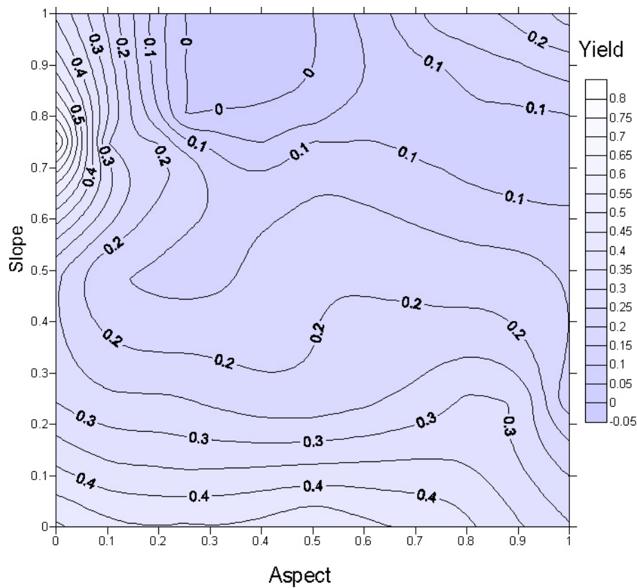
Figure 7. The yield-dependence on the slope and aspect computed using the two-input FIS. Here, Slope and Aspect were normalized to range from 0 to 1.
