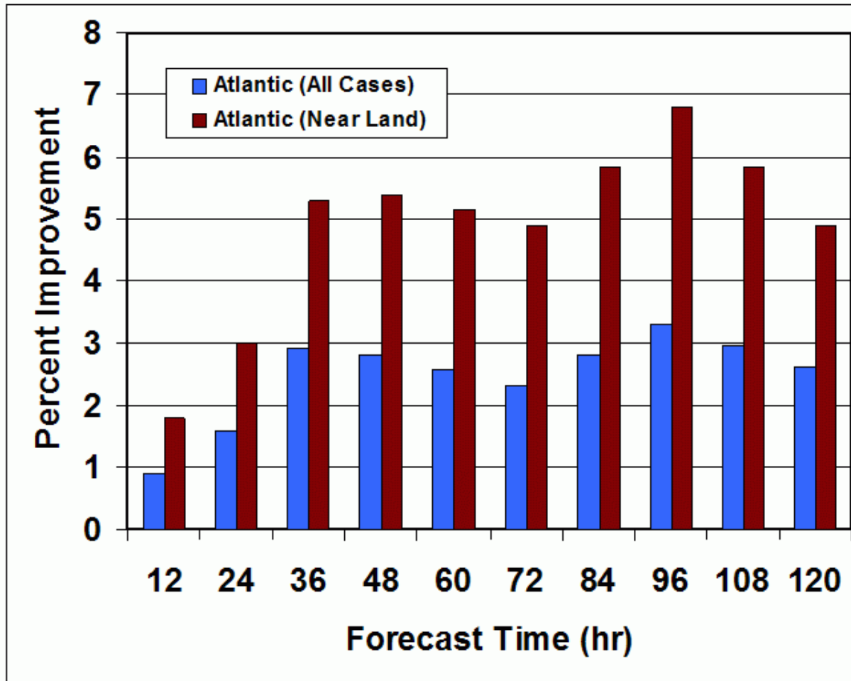
Figure 1. The percent improvement of the experimental SHIPS forecasts with the modified shear and GFS vortex variable in place of Z850 relative to the operational version of SHIPS. All cases from the 2006 season were included.
