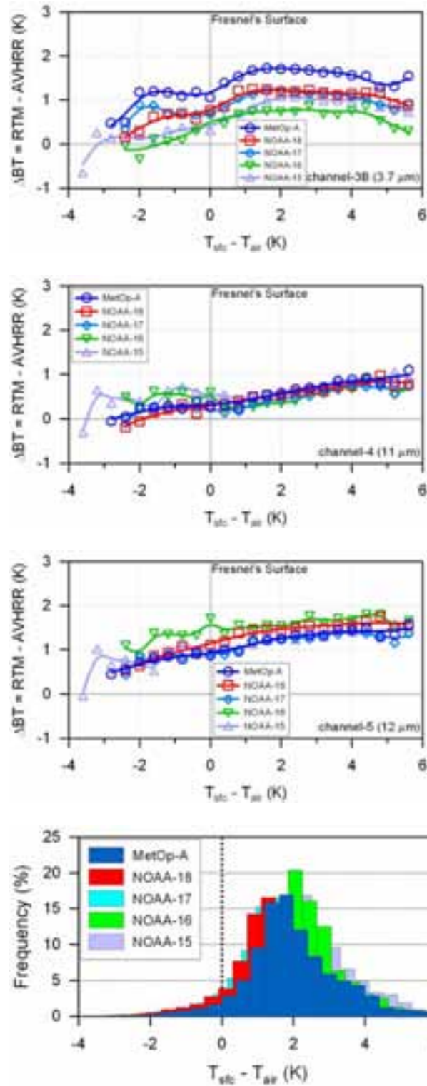
Figure 2. Bias (RTM brightness temperature – AVHRR brightness temperature) as a function of the sea-air temperature difference ( T_{sfc} - T_{air} ) binned at 0.4 K.
