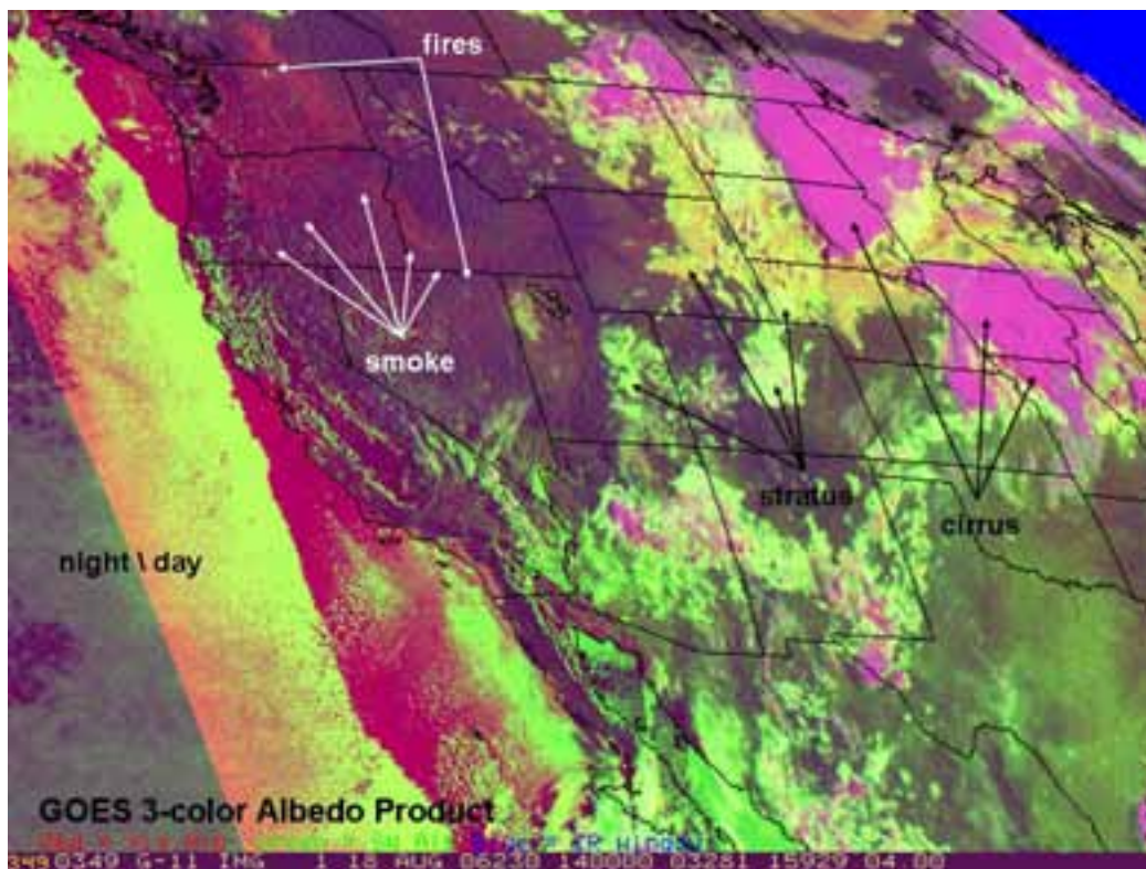
Figure 4. Three-color Albedo Product created by combining the GOES-West (GOES-11) Visible Albedo, Shortwave Albedo, and IR Window band ( 10.7 \mu\text{m} ) as the Red, Green, and Blue components, respectively. The new product shows both smoke and fires, as seen in this image at 1400 UTC on 18 August 2006. The smoke (red haze) appears best as a strongly-forward-scattered signal immediately after sunrise due to the visible albedo component of the image, but almost completely disappears when the solar zenith angle increases and vertical mixing of the atmosphere takes place with solar heating. Fire hot spots (white) are due to the excessive shortwave radiation in the shortwave “albedo” component, and are confirmed by temporal continuity of those spots in the image loop. There is also color discrimination between low-level water/stratus clouds (white to light green) and high-level ice/cirrus cloud (magenta) due to the shortwave albedo component. The product is indeterminate during the transition between day and night and is most useful during the day, although it can be generated day and night with appropriate substitute imagery at night in lieu of the visible band.
