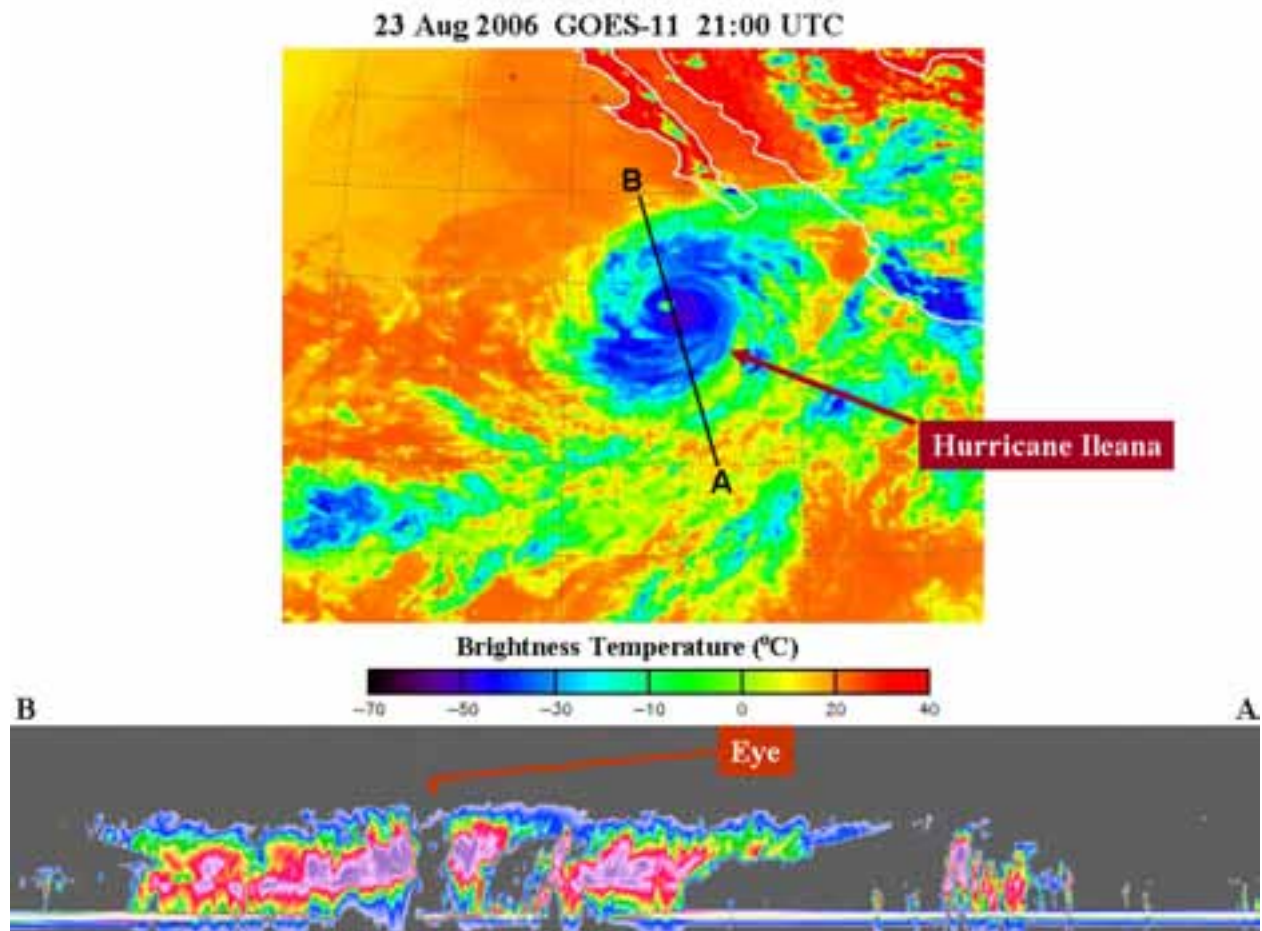
Figure 1. CloudSat Captures the Eye of Hurricane Ileana in August of 2006. This is an example of a CloudSat Case Study.
