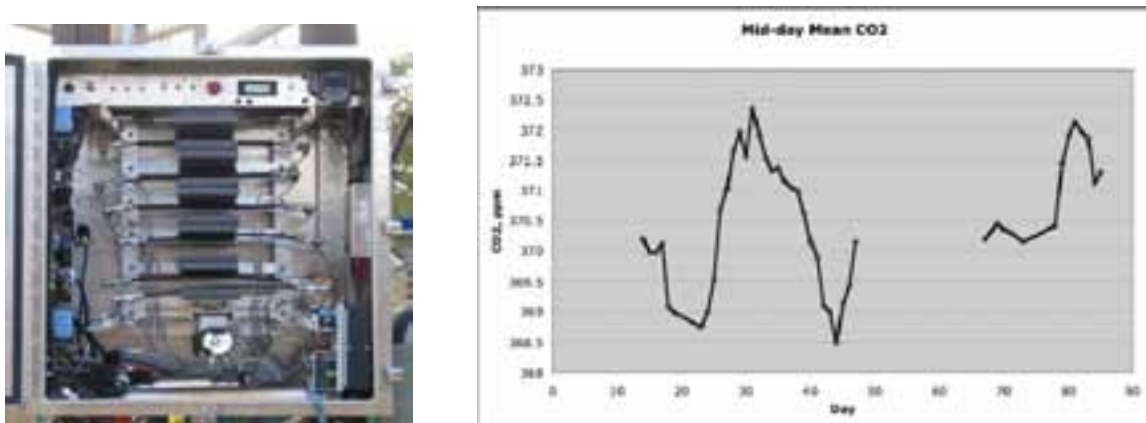
Figure 8. Precision carbon dioxide and flask sampling system (left) and midday atmospheric CO 2 concentration measurements (right) at the Skukuza eddy flux site in the Kruger National Park, South Africa. The system uses automatic calibration with WMO-traceable standards and a temperature controlled infrared gas analyzer to measure CO 2 concentration to an absolute precision of ~0.2 ppm.
