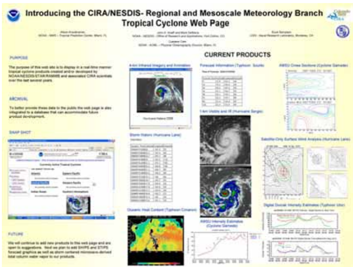
Figure 1. Poster describing the CIRA/AMMB real-time tropical cyclone page that was presented at the 61 st Interdepartmental Hurricane Conference in New Orleans, LA.
