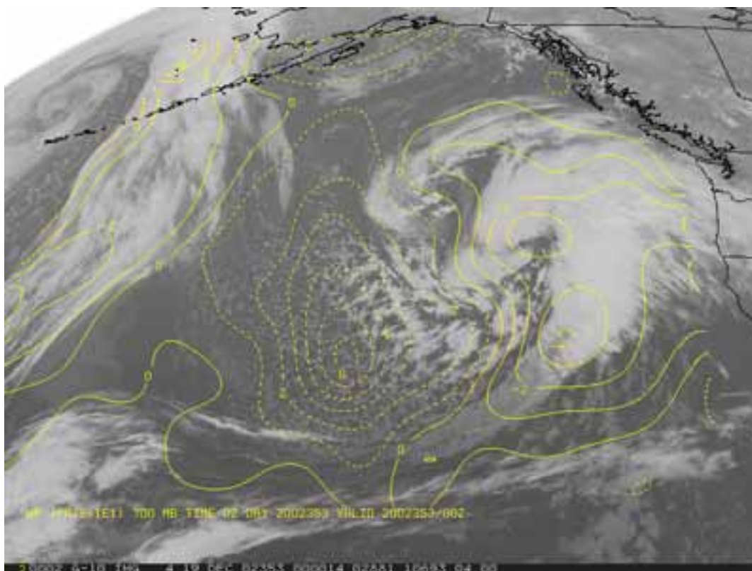
Figure 3. GOES-10 infrared image from 00 UTC 19 December 2002 with 700 hPa quasi-geostrophic \omega ( \mu\text{bar s}^{-1} ) overlaid. The vertical velocity field was derived using ATOVS data.
