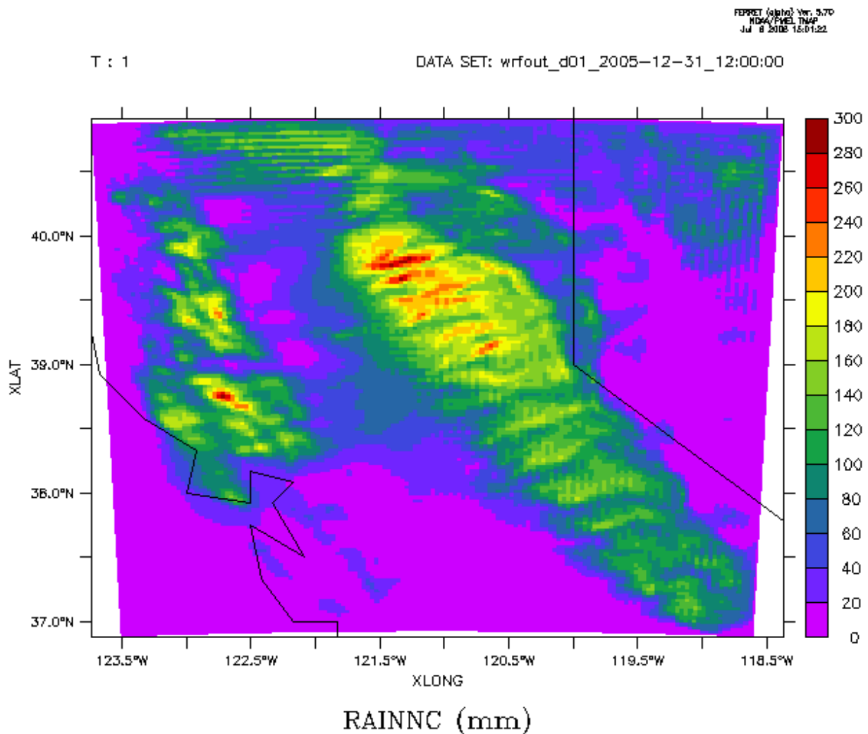
Fig 5a. Evident in this plot are narrow regions of 24-hour precipitation accumulation exceeding 200 mm (~7.9 inches).
