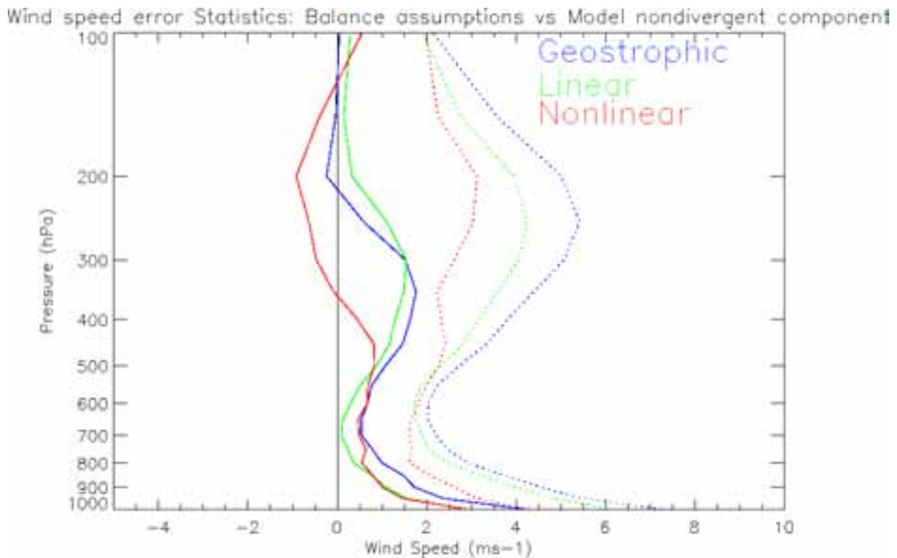
Figure 2. Using the height field from the GFS model, the winds associated with the geostrophic, linear, and nonlinear balance were compared to the model's nondivergent wind component.
