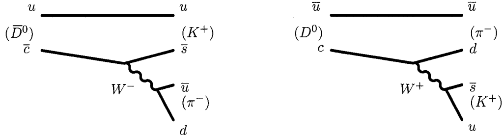
Figure 1.4: Cabibbo allowed \bar{D}^0 \rightarrow K^+\pi^- (left) and doubly Cabibbo suppressed (DCS) D^0 \rightarrow K^+\pi^- decay (right). The suppression is of order |V_{cd}V_{us}|^2/|V_{cs}V_{ud}|^2 \approx \lambda^4 .
