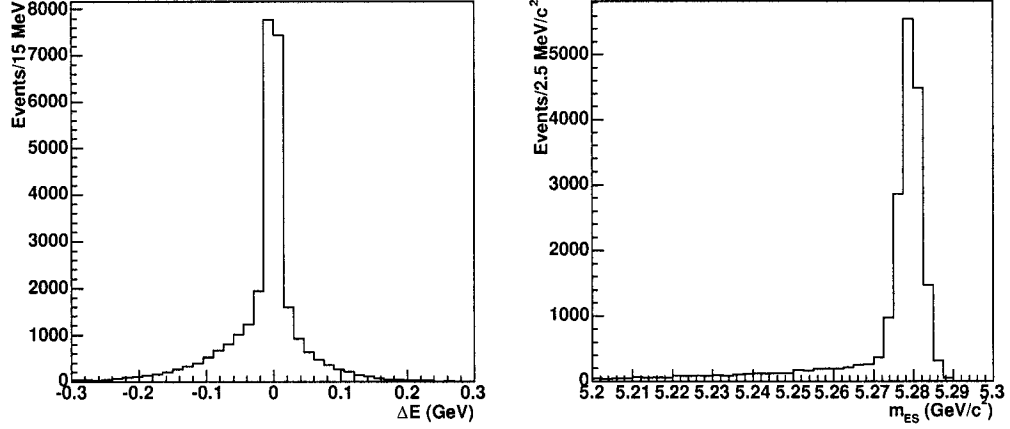
Figure 2.1: \Delta E (left) and m_{ES} (right) for B^- \rightarrow J/\psi \pi^+ \pi^- K^- signal Monte Carlo events.
