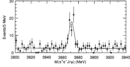
Figure 1.5: Distribution for J/\psi \pi^+ \pi^- invariant mass for the X(3872) region. The signal yield is 49.1 \pm 8.4 events
