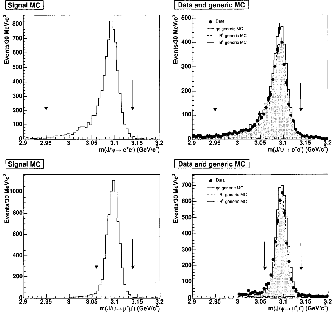
Figure 4.2: J/\psi \rightarrow e^+e^- (top) and J/\psi \rightarrow \mu^+\mu^- (bottom) in B^- \rightarrow J/\psi \pi^+ \pi^- K^- . One can see the longer tail in the electron mode because of the energy loss due to bremsstrahlung. The small arrows indicate our final cuts.
