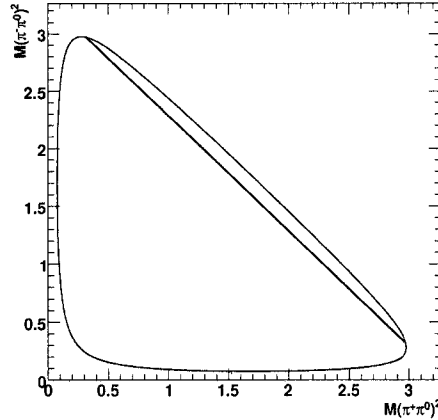
Figure 3.1: Schematic representation of the K_S^0 mass veto window applied to the Dalitz plot. Events within the diagonal line are rejected. The area within the boundary is the kinematic allowed region for D \rightarrow \pi^+ \pi^- \pi^0 decays.
