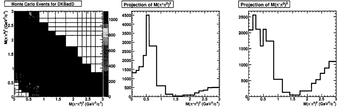
Figure 3.42: Dalitz distribution of DK_{\text{bgd}} events including the binning used for the histogram PDF (left). The two plots on the right show the projections of the PDF on s_{+0} and s_{-0} , respectively.
