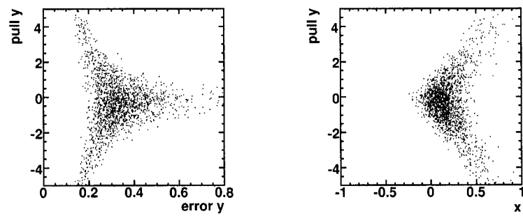
Figure 3.79: Scatter plots of the y -pull versus the error on y (left) and the fitted value of x .
