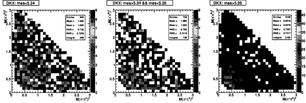
Figure 3.9: Dalitz distributions of m_{ES} for DKX events in the three bins used for the KS comparison shown in Table 3.16.
