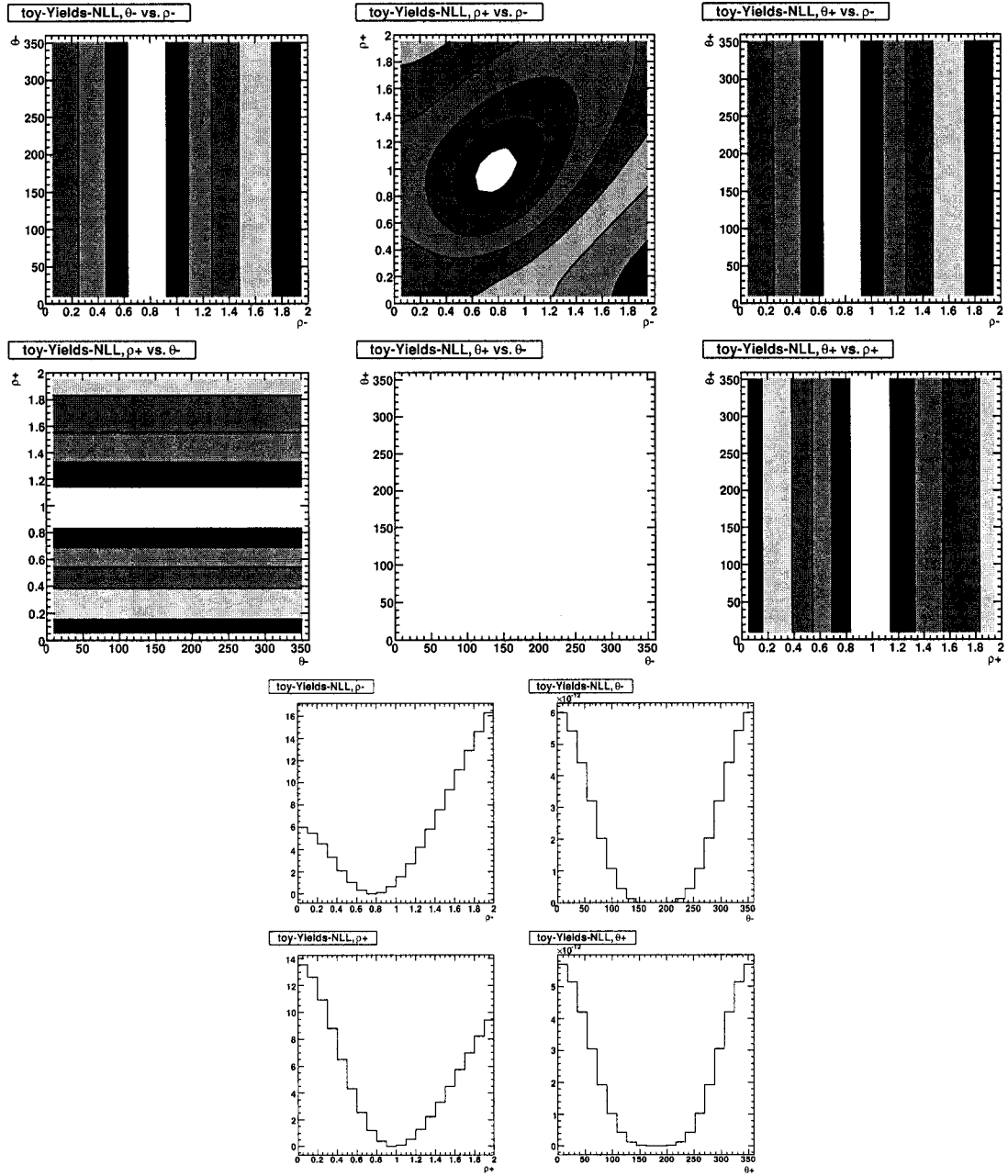
Figure 3.61: Dependence of \mathcal{L}_{\text{BA}} on all pair combinations of the parameters \rho_{\pm} , \theta_{\pm} (2D plots) with 1\sigma contours and the individual parameters in a toy experiment (1D plots).
