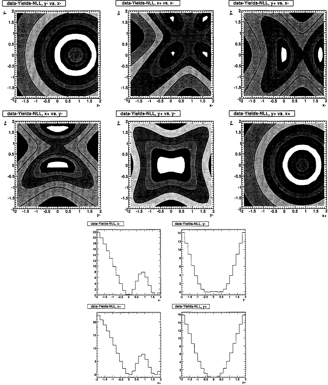
Figure 3.81: Dependence of \mathcal{L}_{\text{BA}} on all pair combinations of the parameters x_{\pm}, y_{\pm} (2D plots, 1\sigma contours) and on the individual parameters (1D plots), using the signal yield and asymmetry from the step-1 data fit.
