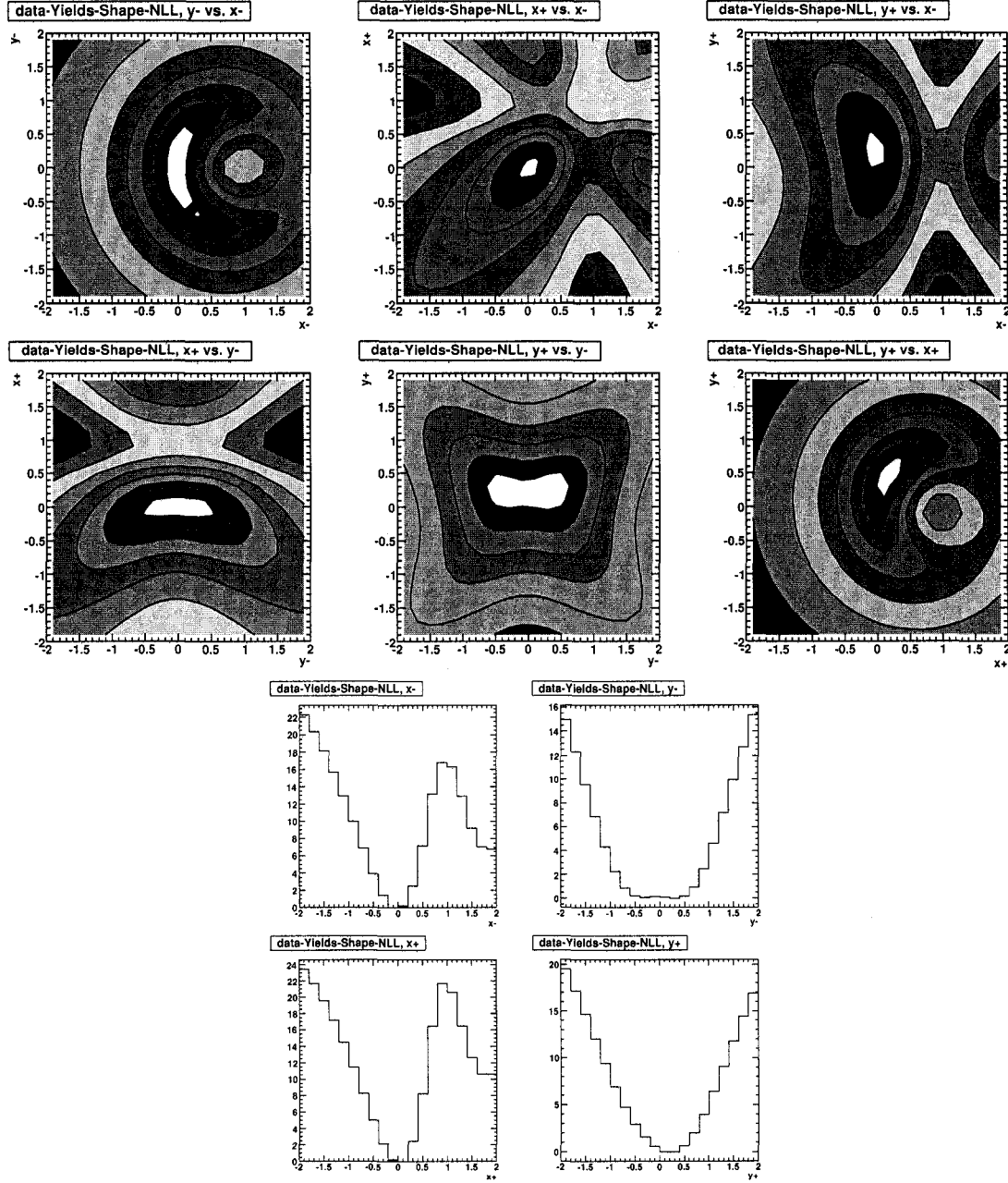
Figure 3.82: Dependence of \mathcal{L} = \mathcal{L}_{\text{DP}} + \mathcal{L}_{\text{BA}} on all pair combinations of the parameters x_{\pm}, y_{\pm} (2D plots, 1\sigma contours) and on the individual parameters (1D plots) for the data.
