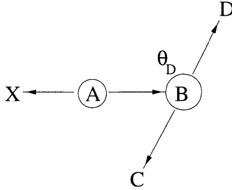
Figure 2.2: Definition of the helicity angle \theta_D in the two-body decay A \rightarrow B + X, B \rightarrow C + D . The angle is measured between the direction of D and A in the rest-frame of B .
