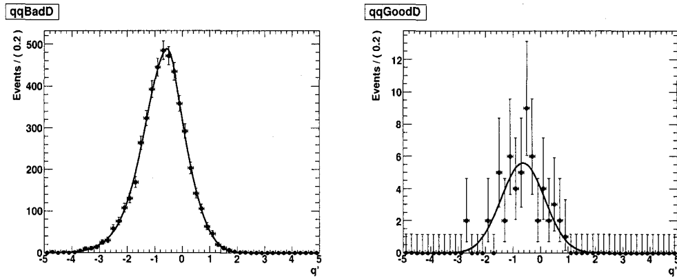
Figure 3.23: The distributions of q' for qq\bar{p} (left) and qq_D (right) obtained from MC.
