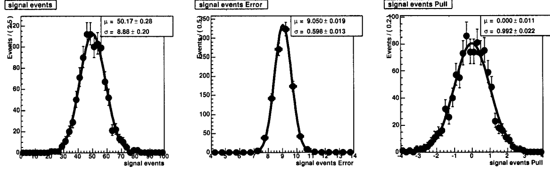
Figure 4.9: Result of 1000 toy-MC experiments for B^0 \rightarrow J/\psi \pi^+ \pi^- K_S^0 with n_{S,toy} = 50 . The left plot shows the number of signal events n_S returned by each fit, in the middle plot we can see the distribution of errors on n_S and the right plot shows the resulting pull distribution.
