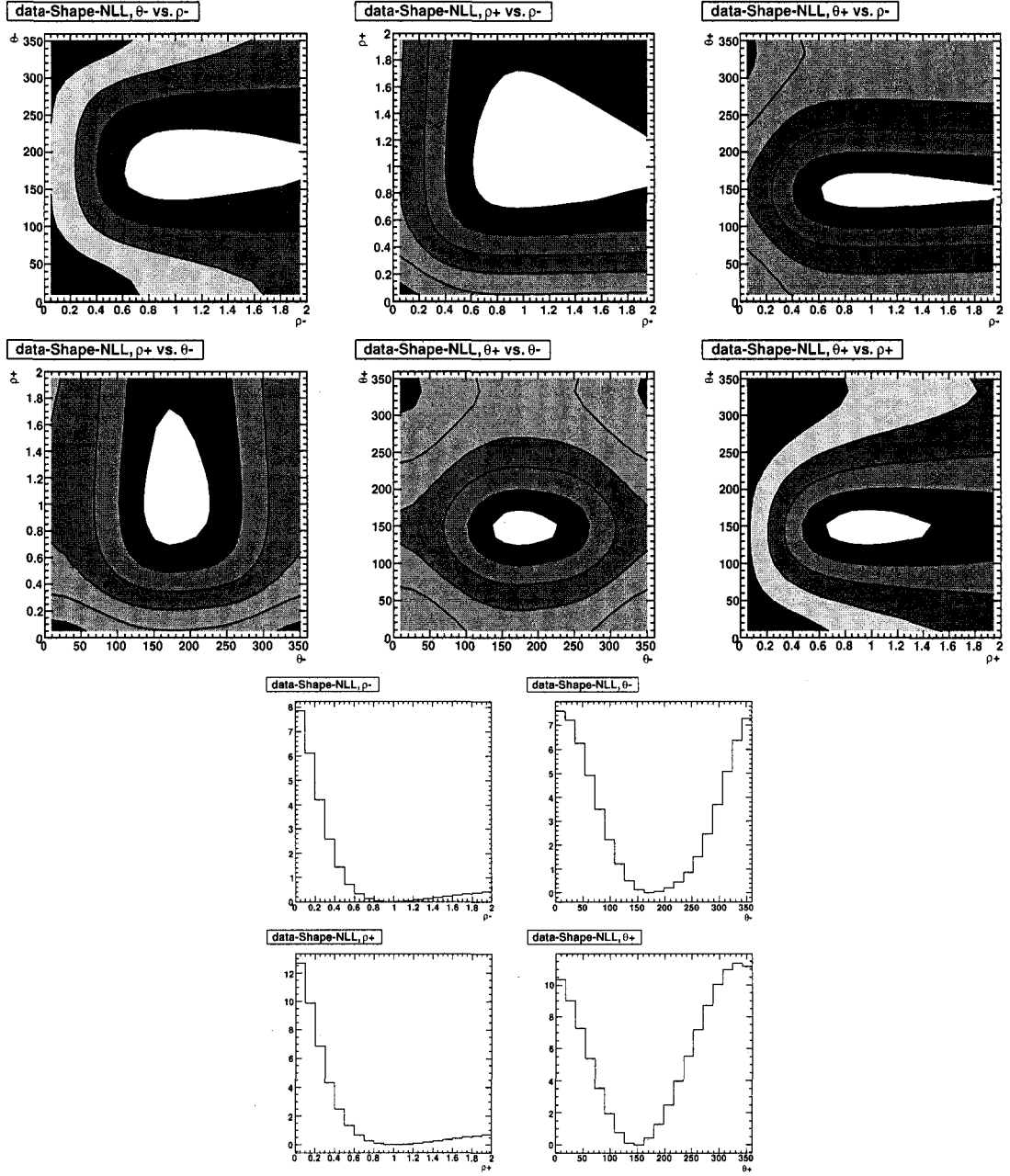
Figure 3.69: Dependence of \mathcal{L}_{\text{DP}} on all pair combinations of the parameters \rho_{\pm} , \theta_{\pm} (2D plots) with 1\sigma contours and the individual parameters (1D plots) for the data.
