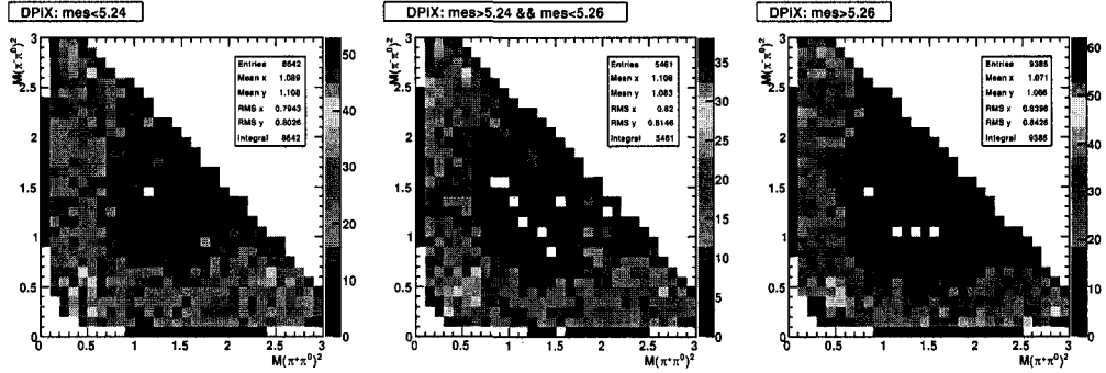
Figure 3.7: Dalitz distributions of m_{ES} for D\pi X events in the three bins used for the KS comparison shown in Table 3.15.
