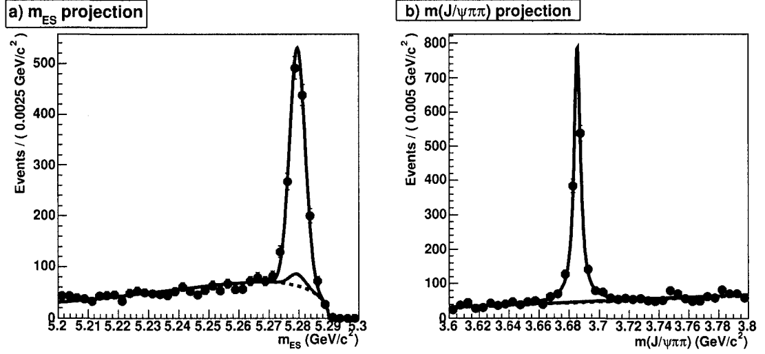
Figure 4.12: The fit result on 210.6 \text{ fb}^{-1} of data for the benchmark mode B^- \rightarrow \psi(2S)K^- . The lines represent (from bottom to top) combinatorial background (dotted, blue), peaking background (solid, red) and signal events (solid, blue).
