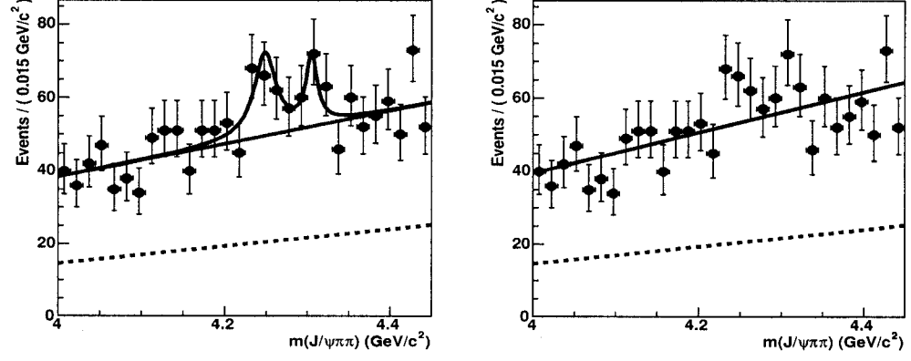
Figure 4.32: m_X projections of the fit result with K_1 veto but no lepton angle cut for the signal (left) and background (right) hypothesis. See Tab. 4.13 for the fit parameters.
