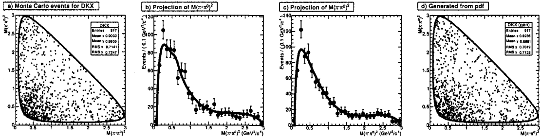
Figure 3.38: Fit to the Dalitz distribution of DKX events. a) shows the MC events used in the fit, b) and c) show the projections on s_{+0} and s_{-0} and d) shows the Dalitz distribution of events generated from the fitted PDF.
