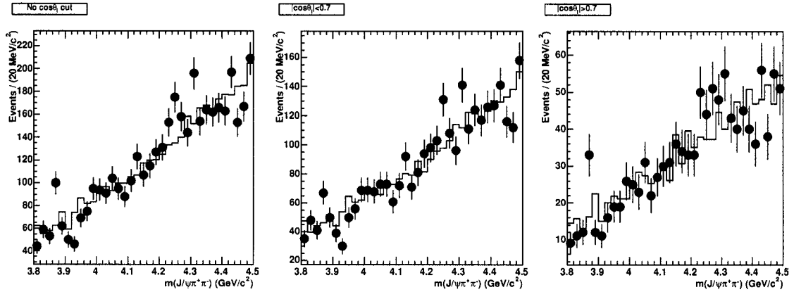
Figure 4.30: The J/\psi \pi^+ \pi^- invariant mass without \cos\theta_l cut (left), |\cos\theta_l| < 0.7 (middle) and |\cos\theta_l| > 0.7 (right). The dots are on-peak data and the solid line shows B\bar{B} generic MC scaled to the same number of events.
