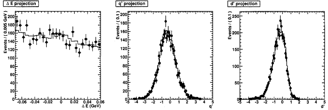
Figure 3.67: \Delta E (left), q' (center) and d' projection (right) of the data fit. The solid line shows the fitted PDF and the dots show the data.
