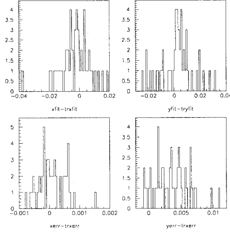
Figure 3.65: Top: Differences between the values of x (left) and y (right) when fitting the measured and the true Dalitz plot variables of “shaped” signal samples. Bottom: Differences between the fit errors on x (left) and y (right). The different entries in each plot, corresponding to different generated values of x and y , are highly correlated.
