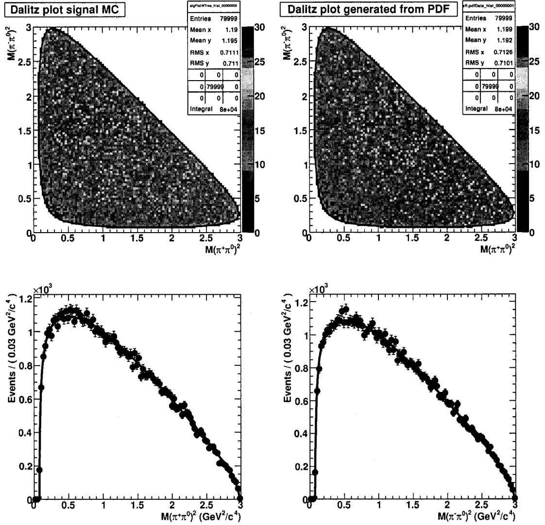
Figure 3.29: Fit of \text{Eff}_D on phase-space signal MC. Upper left: Efficiency map for correctly reconstructed MC B^- \rightarrow D_{\pi^+\pi^-\pi^0} K^- events. Upper right: The Dalitz plot distribution of events generated using the PDF used to fit the MC efficiency. Bottom: Projections onto the Dalitz plot axes of phase-space MC (data points) and the efficiency fit function (line).
