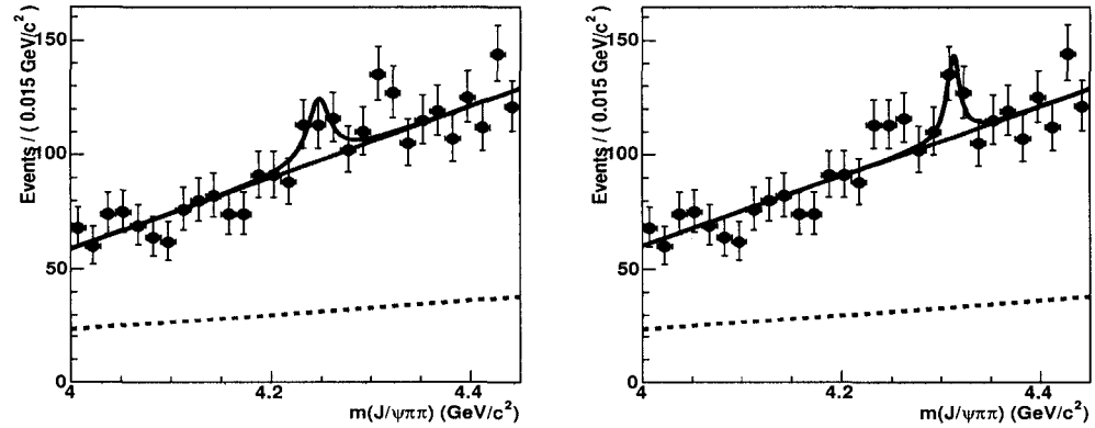
Figure 4.22: m_X projections of the fit result in configuration (III) (left) and (IV) (right). See Tab. 4.12 for the fit parameters.
