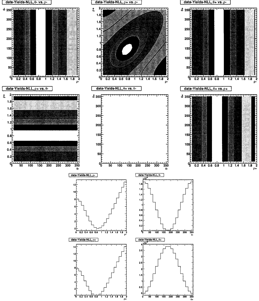
Figure 3.70: Dependence of \mathcal{L}_{BA} on all pair combinations of the parameters \rho_{\pm} , \theta_{\pm} (2D plots) with 1\sigma contours and the individual parameters (1D plots) for the data.
