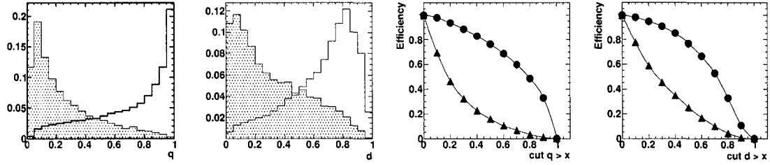
Figure 3.2: (left two plots) Distribution of the neural network variables q and d for background (hatched) and signal. (right two plots) The cut efficiencies to remove background (triangles) and signal (dots) when applying the selection q, d > x .
