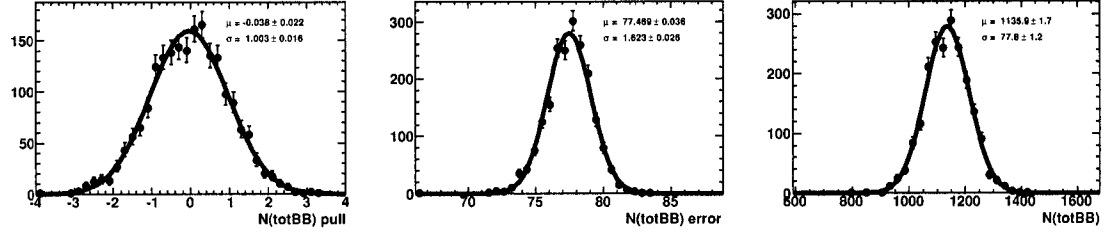
Figure 3.51: Results of 2000 toy MC experiments (signal and background, no systematic error in \mathcal{L}_{BA} ) for the pull (left), error (center) and fitted values (right) of N_{BB_D} .
