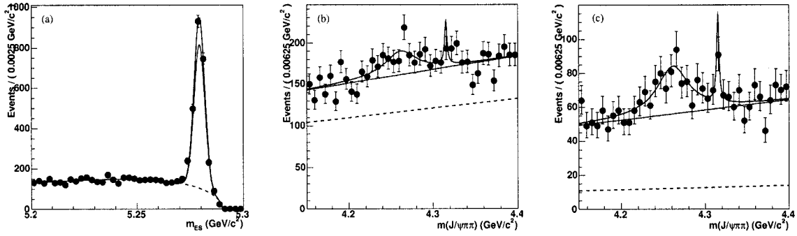
Figure 4.19: Fit to a MC cocktail of B\bar{B} generic MC, Y(4264) and Z(4315) . Plots a) and b) show the fit projections for m_{ES} and m_X whereas plot c) shows the m_X projection with a cut on the m_{ES} signal region applied.
