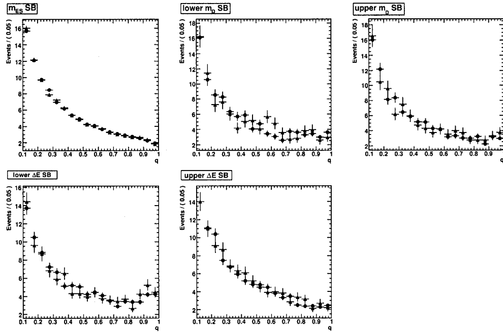
Figure 3.13: Comparison of q distributions in data (black triangles) and MC (blue circles) for different sidebands (see plot titles). The p-values of a \chi^2 -test between data and MC are listed in Table 3.23.
