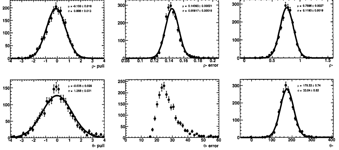
Figure 3.58: Results of 2000 toy MC experiments (signal and background, including systematic error in \mathcal{L}_{\text{BA}} ) for the pull (left), error (center) and fitted values (right) of \rho_- (top) and \theta_- (bottom). See Fig. 3.55 for the corresponding toy MC without systematic errors.
