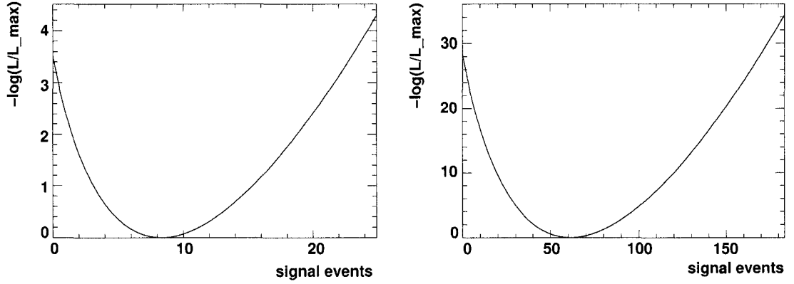
Figure 4.15: Projection of the negative log-likelihood of the data fit on the number of signal events n_S . The left plots shows B^0 \rightarrow X(3872)K_s^0 and the right plot shows the same for B^- \rightarrow X(3872)K^- .
