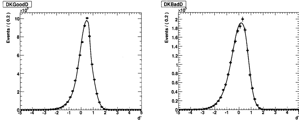
Figure 3.24: The distributions of d' for DK_{\text{sig}} (left) and DK_{\text{bgd}} (right) obtained from MC.
