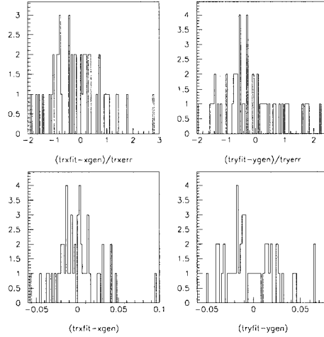
Figure 3.64: Top: Pull distributions for x (left) and y (right) when fitting the true Dalitz plot variables of “shaped” signal samples. Bottom: Differences between the generated and measured values of x (left) and y (right). The different entries in each plot, corresponding to different generated values of x and y , are highly correlated.
