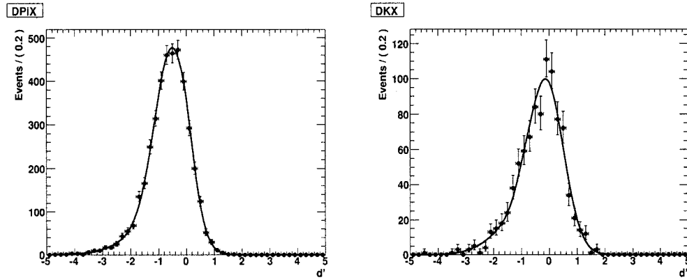
Figure 3.26: The distributions of d' for D\pi X (left) and DKX (right) obtained from MC.
