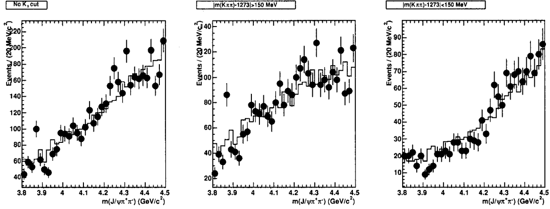
Figure 4.28: The J/\psi \pi^+ \pi^- invariant mass without K_1 cut (left), K_1 veto |m(K \pi^+ \pi^-) - 1273| > 150 \text{ MeV}/c^2 (middle) and |m(K \pi^+ \pi^-) - 1273| < 150 \text{ MeV}/c^2 (right). The dots are on-peak data and the solid line shows B\bar{B} generic MC scaled to the same number of events.
