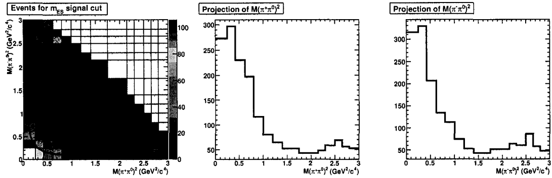
Figure 3.86: The histogram-based PDF used for the background shape (left), and the data (points) in the \Delta E sideband, from which the histogram was derived. The 1-D projections are also shown.
