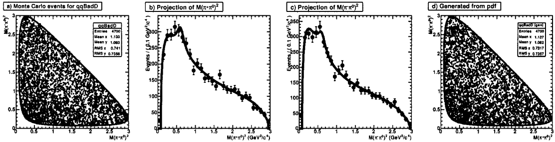
Figure 3.40: Fit to the Dalitz distribution of qqp events. a) shows the MC events used in the fit, b) and c) show the projections on s_{+0} and s_{-0} and d) shows the Dalitz distribution of events generated from the fitted PDF.
