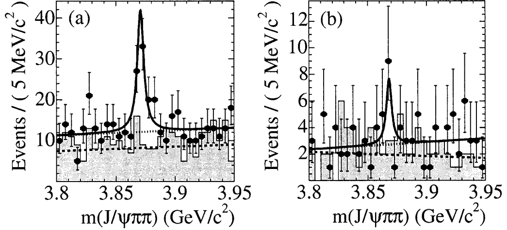
Figure 1.11: J/\psi \pi^+ \pi^- invariant mass for (a) B^- \rightarrow X(3872) K^- and (b) B^0 \rightarrow X(3872) K_s^0 . The dashed line represents the combinatorial background, the dotted line represents the sum of the combinatorial and peaking background and the solid line the sum of all background plus the signal. The shaded area shows events in the m_{ES} sideband region |m_{ES} - 5260 \text{ MeV}/c^2| < 6 \text{ MeV}/c^2 .
