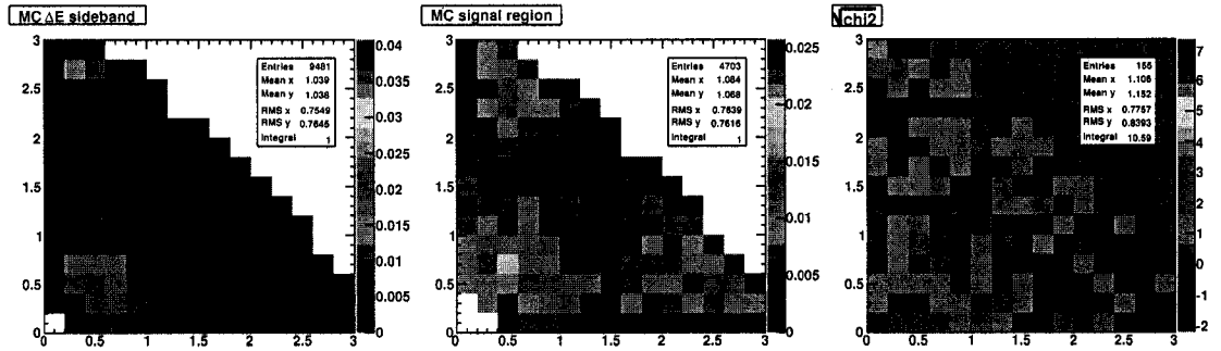
Figure 3.84: Comparison of MC Dalitz distributions for B^- \rightarrow D_{\pi^+\pi^-\pi^0\pi^-} in the \Delta E sideband (left) and \Delta E signal region (center) together with the signed \sqrt{\chi^2} distribution (right). The \chi^2 probability of the two histograms to be drawn from the same distribution is 0.4%.
