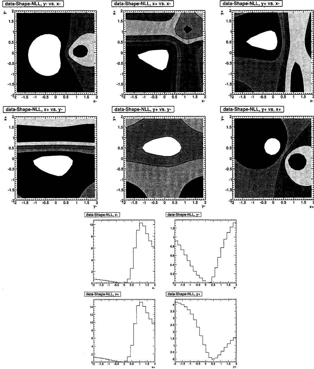
Figure 3.80: Dependence of \mathcal{L}_{DP} on all pair combinations of the parameters x_{\pm}, y_{\pm} (2D plots, 1\sigma contours) and on the individual parameters (1D plots) for the data.
