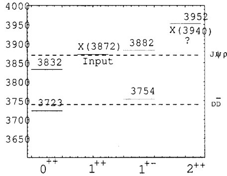
Figure 1.17: The full spectrum of X particles. The X(3872) J^{PC} = 1^{++} state is used as the input for the calculation of the other masses. The dashed lines indicate possible decay channel thresholds [36].
