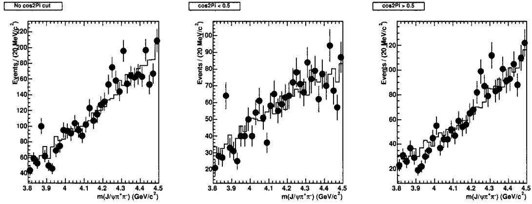
Figure 4.26: The J/\psi \pi^+ \pi^- invariant mass without \cos 2\pi_i cut (left), \cos 2\pi_i < 0.5 (middle) and \cos 2\pi_i > 0.5 (right). The dots are on-peak data and the solid line shows B\bar{B} generic MC scaled to the same number of events.
