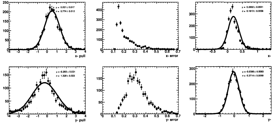
Figure 3.77: Results of 2000 toy MC experiments (signal and background) for the pull (left), error (center) and fitted values (right) of x_- (top) and y_- (bottom).
