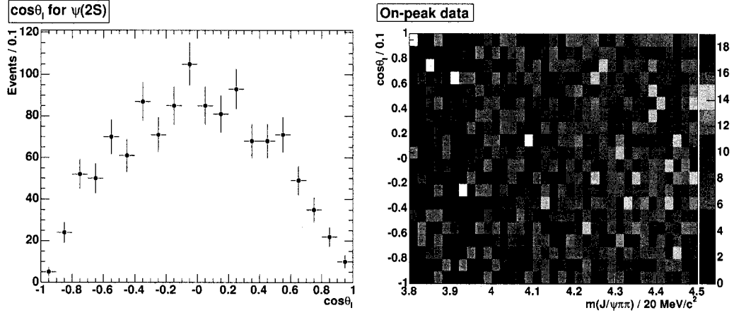
Figure 4.29: (left) \cos\theta_l distribution for the \psi(2S) as reference. (right) \cos\theta_l versus the J/\psi \pi^+ \pi^- invariant mass.
