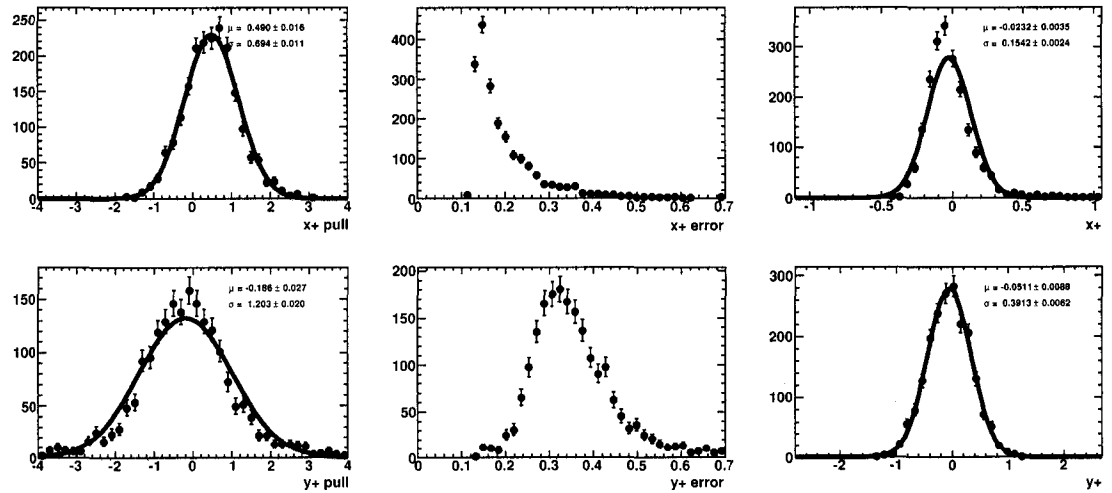
Figure 3.78: Results of 2000 toy MC experiments (signal and background) for the pull (left), error (center) and fitted values (right) of x_+ (top) and y_+ (bottom).
