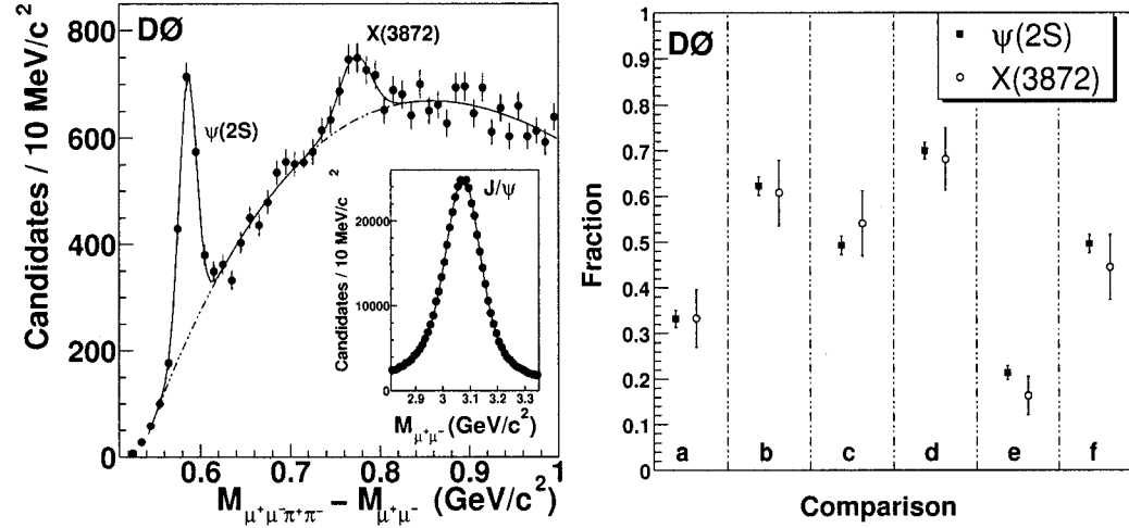
Figure 1.16: (left) The \mu^+ \mu^- \pi^+ \pi^- mass spectrum with the \psi(2S) and X(3872) . The insert shows the mass distribution of the J/\psi candidates used in the analysis. (right) Comparison of event-yield fractions for X(3872) and \psi(2S) in the regions: (a) p_T > 15 \text{ GeV}/c , (b) rapidity of J/\psi \pi^+ \pi^- < 1 , (c) \cos \theta_\pi < 0.4 , (d) effective proper decay length < 0.01 \text{ cm} , (e) isolation = 1, (f) \cos \theta_\mu < 0.4 .
