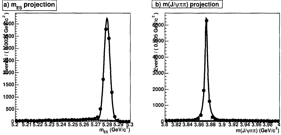
Figure 4.7: Result of the full 2D-UEML-fit (including all event types) for pure signal MC in B^0 \rightarrow X(3872)K_s^0 , X \rightarrow J/\psi \pi^+ \pi^- . The fit result is n_S = 10652 \pm 104 , n_P = 0.0 \pm 1.5 and n_C = 1904 \pm 46 . The number of signal events n_S is used to calculate our efficiency for reconstructing signal events (see Tab. 4.5).
