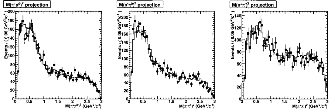
Figure 3.68: s_{+0} (left), s_{-0} (center) and s_{+-} projection (right) of the data fit. The solid line shows the fitted PDF and the dots show the data.
