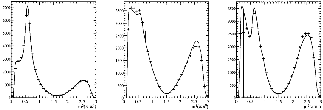
Figure 3.44: Projections of the data and PDF for the Dalitz fit to D^0 \rightarrow \pi^+\pi^-\pi^0 decays. From left to right, the invariant masses squared of \pi^+\pi^0 , \pi^-\pi^0 and \pi^+\pi^- are shown, respectively.
