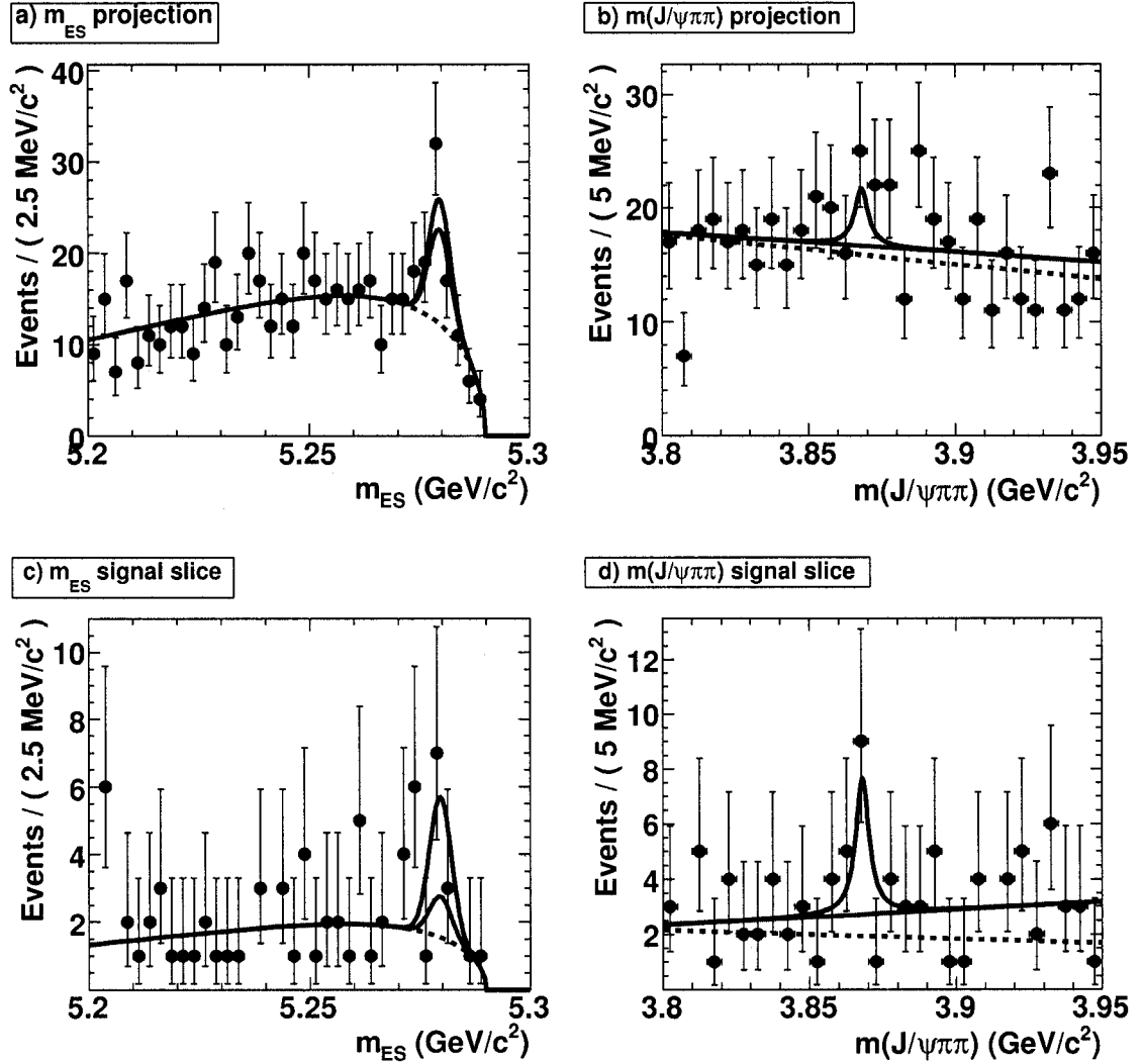
Figure 4.13: The fit result on 210.6 \text{ fb}^{-1} of data in B^0 \rightarrow X(3872)K_s^0 . The lines represent (from bottom to top) combinatorial background (dotted, blue), peaking background (solid, red) and signal events (solid, blue). a) and b) are projections on m_{ES} and m_X , respectively. Plots c) and d) show the signal band projection with an additional cut on the signal region of the variable not shown.
