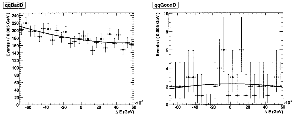
Figure 3.18: The distributions of \Delta E for qq_p (left) and qq_D (right) obtained from MC.
