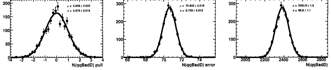
Figure 3.72: Results of 2000 toy MC experiments (signal and background) for the pull (left), error (center) and fitted values (right) of N_{qq\bar{p}} .
