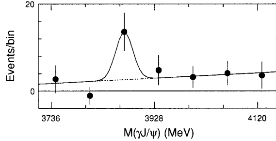
Figure 1.8: The signal yields from a fit to the m_{ES} and \Delta E distributions in bins of m(J/\psi\gamma) .
