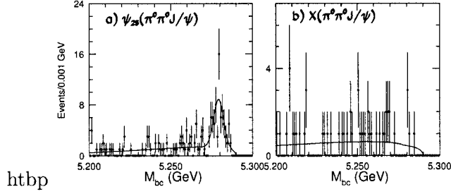
Figure 1.10: The m_{ES} distribution for (a) B \rightarrow \psi(2S)K, \psi(2S) \rightarrow J/\psi \pi^0 \pi^0 and (b) B \rightarrow X(3872)K, X(3872) \rightarrow J/\psi \pi^0 \pi^0 with a superimposed fit. The signal yield is 55 \pm 10 events for the \psi(2S) and 0.2 \pm 2.6 events for the X(3872) .
