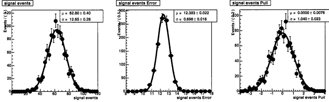
Figure 4.10: Result of 1000 toy-MC experiments for B^- \rightarrow J/\psi \pi^+ \pi^- K^- with n_{S,toy} = 63 . The left plot shows the number of signal events n_S returned by each fit, in the middle plot we can see the distribution of errors on n_S and the right plot shows the resulting pull distribution.
