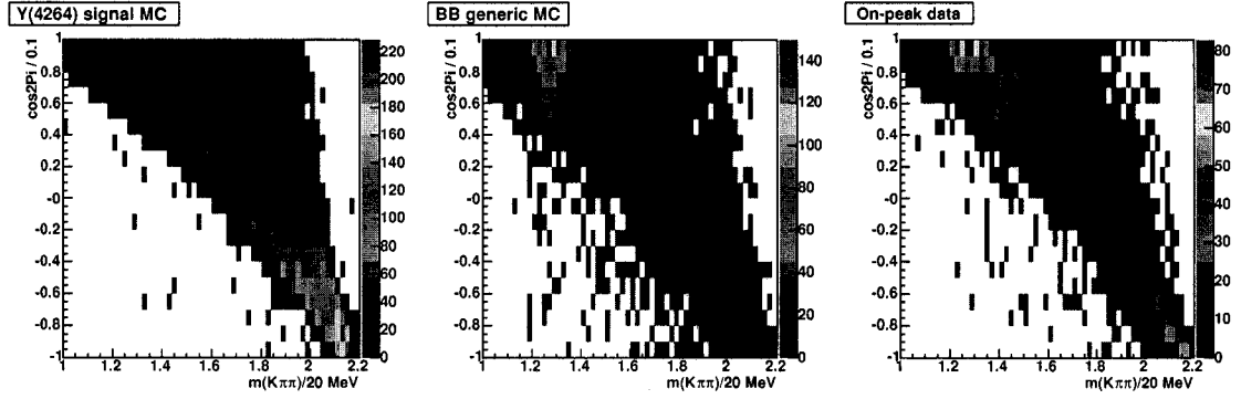
Figure 4.24: The angle \cos 2\pi_i versus the K\pi^+\pi^- invariant mass for signal MC (left), B\bar{B} generic MC (middle) and data (right) for events with 3.8 < m(J/\psi \pi^+\pi^-) < 4.5 \text{ GeV}/c^2 .
