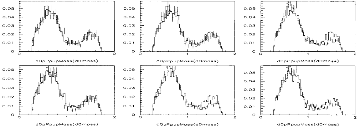
Figure 3.4: Comparison of s_{+0} in bins of m_D for D\pi X events corresponding to the KS probabilities of Table 3.9 (from left to right, top to bottom).
