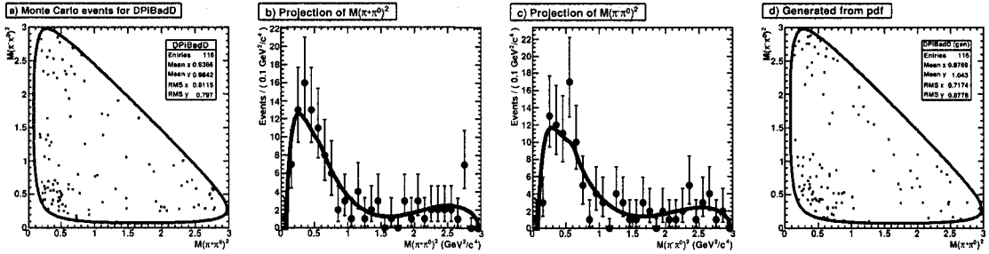
Figure 3.37: Fit to the Dalitz distribution of D\pi p events. a) shows the MC events used in the fit, b) and c) show the projections on s_{+0} and s_{-0} and d) shows the Dalitz distribution of events generated from the fitted PDF.
