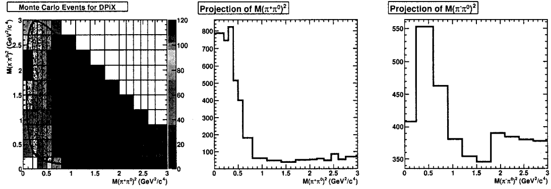
Figure 3.41: Dalitz distribution of D\pi X events including the binning used for the histogram PDF (left). The two plots on the right show the projections of the PDF on s_{+0} and s_{-0} , respectively.
