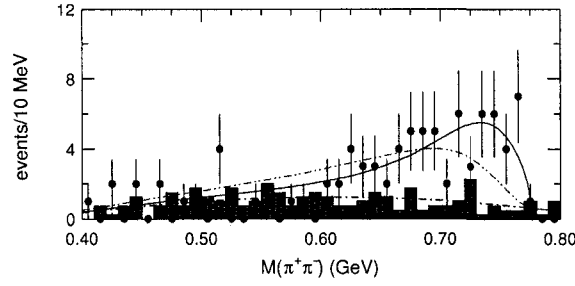
Figure 1.6: m(\pi^+\pi^-) distribution of events in the X(3872) signal region. The solid (dashed) curve shows the fit that uses a \rho Breit-Wigner line shape with the J/\psi and \rho in a relative S -wave ( P -wave). The histogram indicates the side-band determined background and the dot-dashed curve is a fit of this background.
