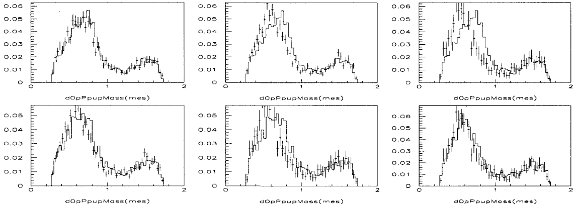
Figure 3.3: Comparison of s_{-0} in bins of m_{ES} for D\pi X events corresponding to the KS probabilities of Table 3.9 (from left to right, top to bottom).
