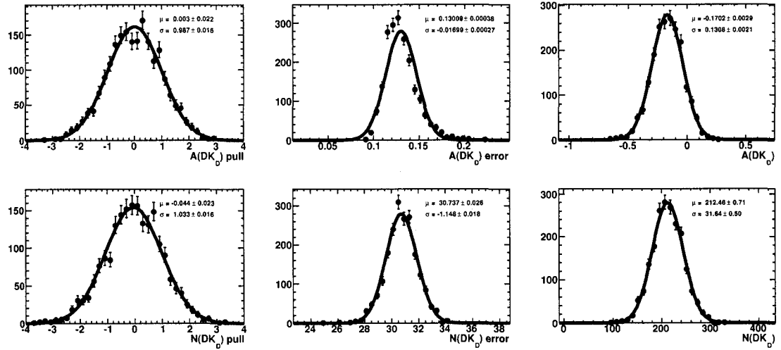
Figure 3.76: Results of 2000 toy MC experiments (signal and background) for the pull (left), error (center) and fitted values (right) of A_{DK_{sig}} (top) and N_{DK_{sig}} (bottom).
