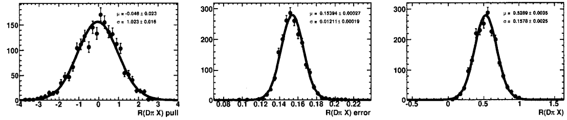
Figure 3.53: Results of 2000 toy MC experiments (signal and background, no systematic error in \mathcal{L}_{BA} ) for the pull (left), error (center) and fitted values (right) of R_{D\pi} .
