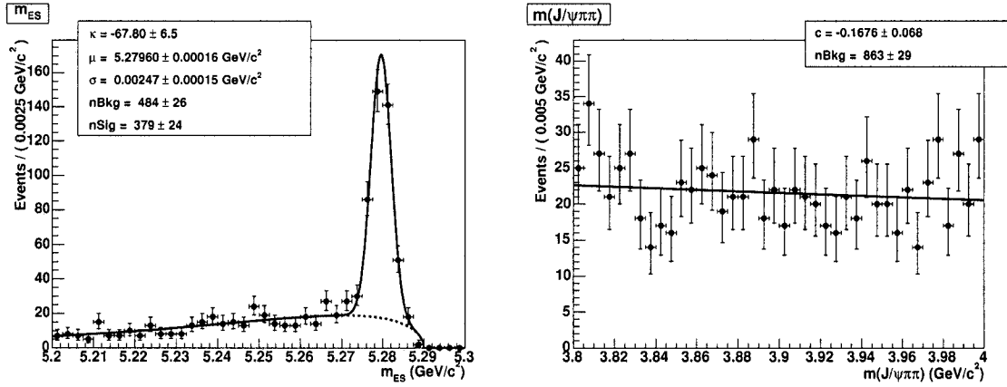
Figure 4.5: 1-dimensional UEML-fit to the m_{ES} (left) and m_X (right) distribution on generic MC for peaking background events in B^0 \rightarrow J/\psi \pi^+ \pi^- K_S^0 .
