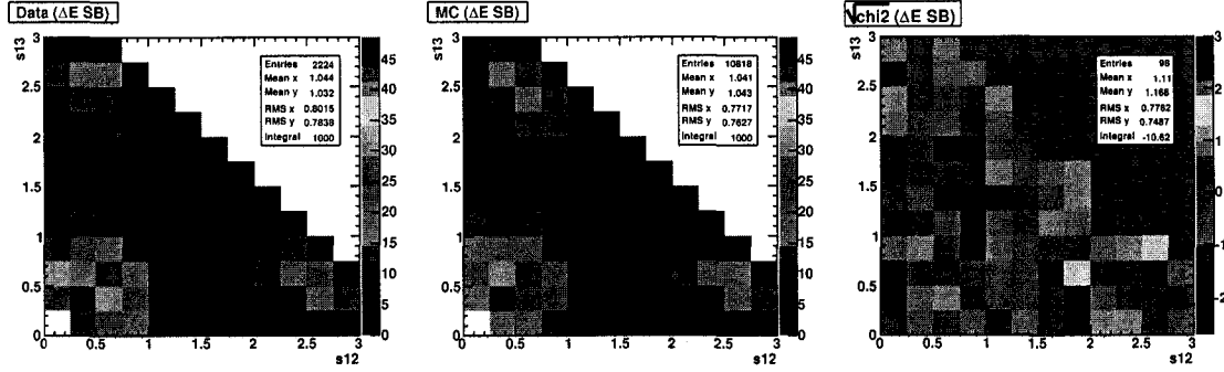
Figure 3.85: Comparison of data (left) and MC (center) Dalitz distributions for B^- \rightarrow D\pi^+\pi^-\pi^0\pi^- in the \Delta E sideband together with the signed \sqrt{\chi^2} distribution (right). The \chi^2 probability of the two histograms to be drawn from the same distribution is 16.0%.
