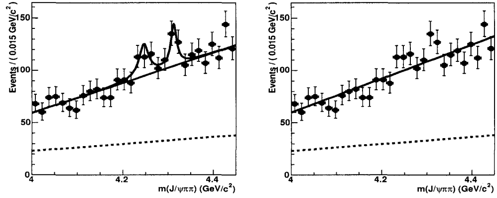
Figure 4.21: m_X projections of the fit result in configuration (I) (left) and the null hypothesis (II, right). See Tab. 4.12 for the fit parameters.
