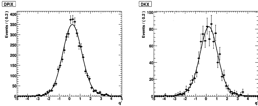
Figure 3.21: The distributions of q' for D\pi_X (left) and DK_X (right) obtained from MC.
