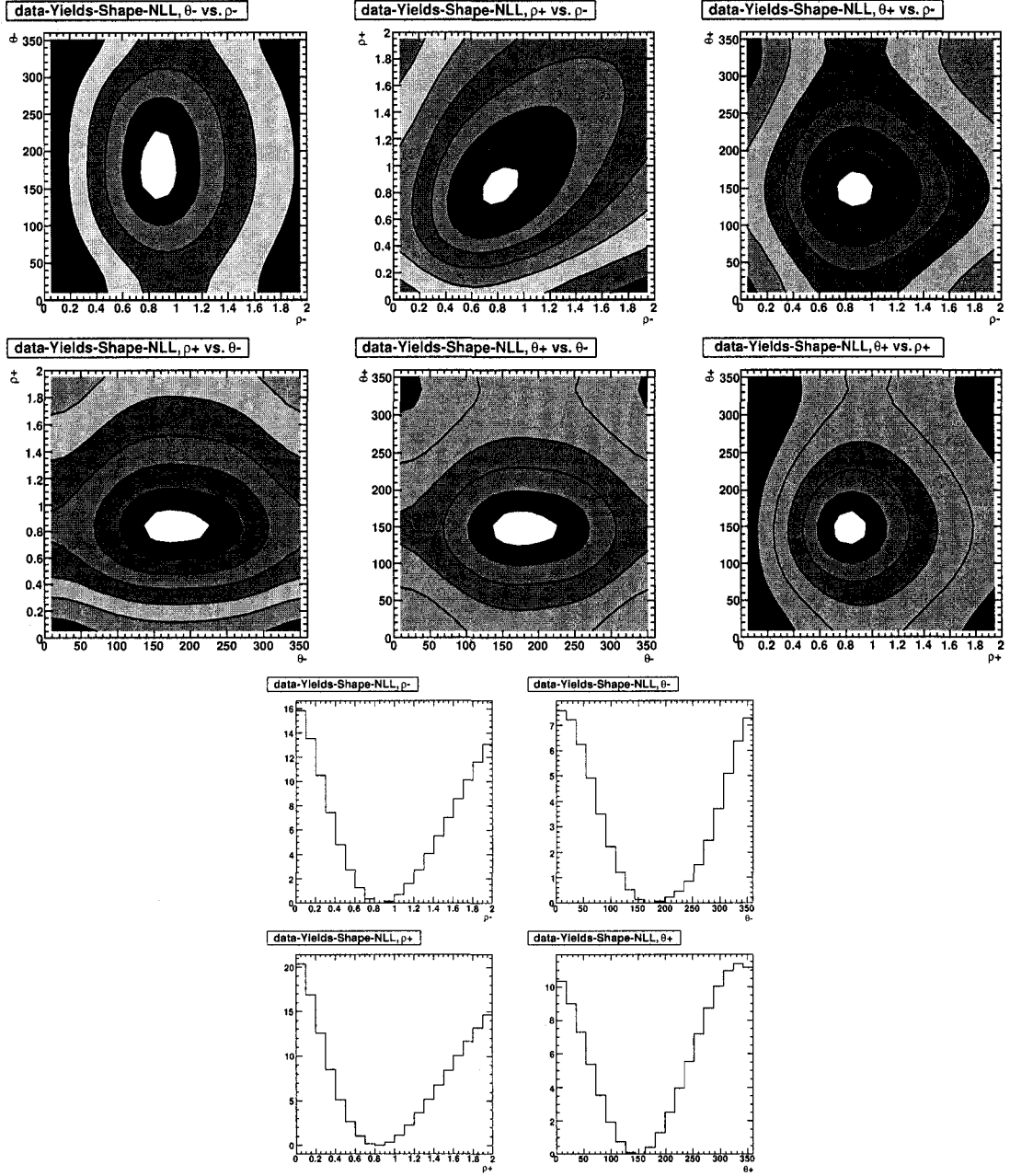
Figure 3.71: Dependence of \mathcal{L} = \mathcal{L}_{\text{DP}} + \mathcal{L}_{\text{BA}} on all pair combinations of the parameters \rho_{\pm} , \theta_{\pm} (2D plots) with 1\sigma contours and the individual parameters (1D plots) for the data.
