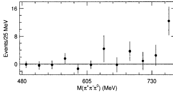
Figure 1.9: The signal yields from a fit to the m_{ES} and \Delta E distributions in bins of m(\pi^+ \pi^- \pi^0) .
