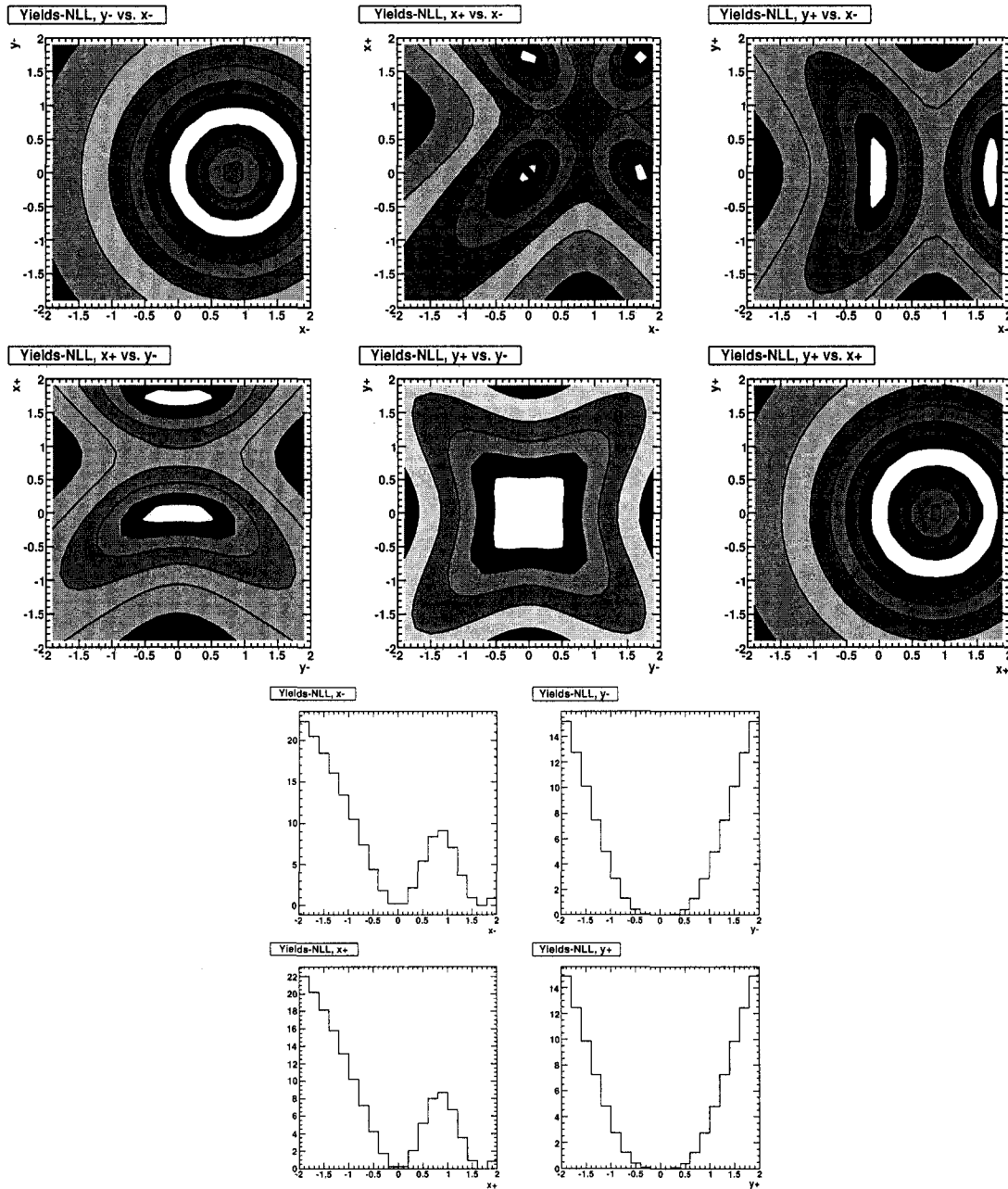
Figure 3.48: Dependence of \mathcal{L}_{BA} on all pair combinations of the parameters x_{\pm}, y_{\pm} (2D plots, 1\sigma contours) and on the individual parameters (1D plots) in a toy experiment. The true values of x_{\pm}, y_{\pm} are 0. The values of the parameters not shown in each plot are set to their true values.
