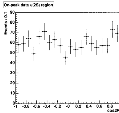
Figure 4.23: \cos 2\text{Pi} distribution for \psi(2S) events in on-peak data.
