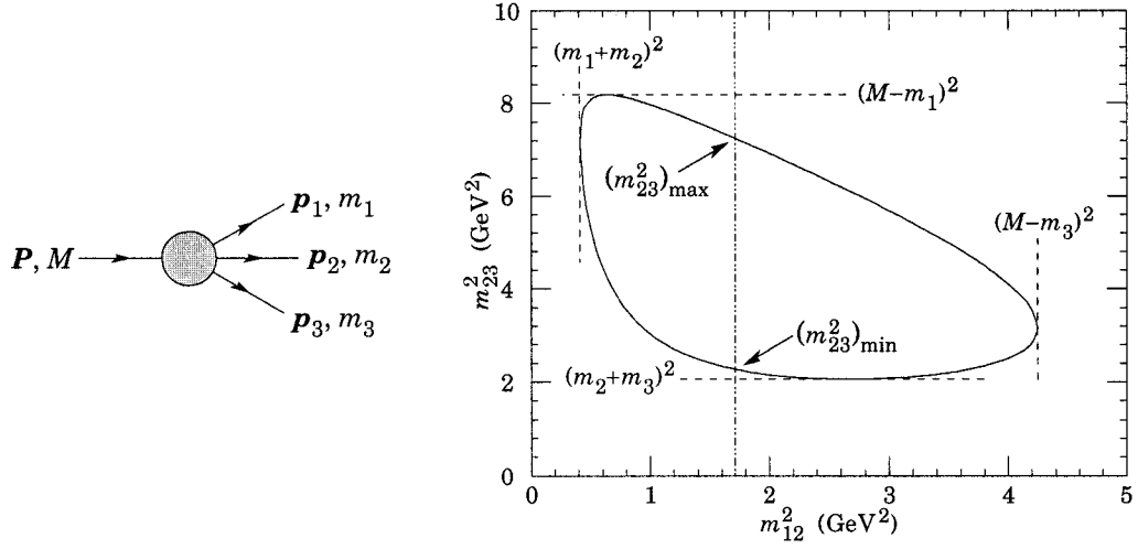
Figure 2.3: Left: A three-body decay of a parent particle with mass M and momentum P into three daughter particles with masses m_i and momenta p_i . Right: Kinematic allowed region for the three-body decay illustrated on the Dalitz plane.
