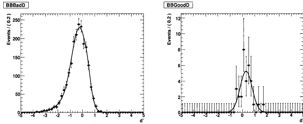
Figure 3.27: The distributions of d' for BBC_p (left) and BBC_D (right) obtained from MC.
