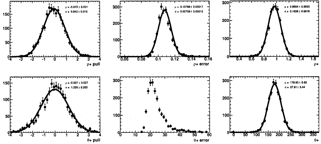
Figure 3.56: Results of 2000 toy MC experiments (signal and background, no systematic error in \mathcal{L}_{\text{BA}} ) for the pull (left), error (center) and fitted values (right) of \rho_+ (top) and \theta_+ (bottom). See Fig. 3.59 for the corresponding toy MC including systematic errors.
