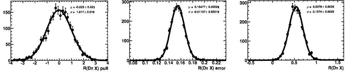
Figure 3.75: Results of 2000 toy MC experiments (signal and background) for the pull (left), error (center) and fitted values (right) of R_{D\pi} .
