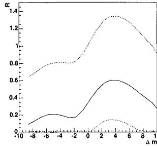
Figure 4.35: The solid line represent the central value of R for different values of \Delta m . The two dashed lines are the 90% CL interval on this value.
