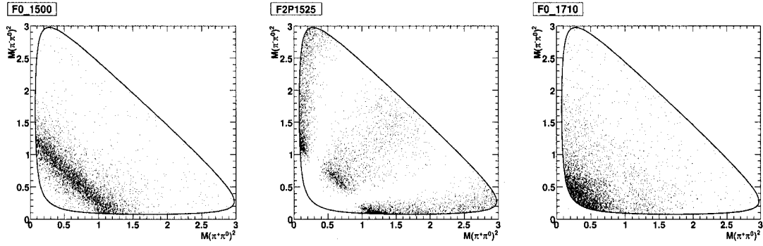
Figure 3.34: Dalitz plot distributions of f_0(1500)\pi^0 , f_2'(1525)\pi^0 , and f_0(1710)\pi^0 toy MC events.
