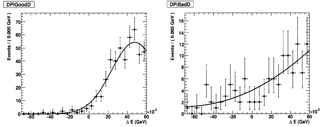
Figure 3.15: The distributions of \Delta E for D\pi_D (left) and D\pi_p (right) obtained from MC.
