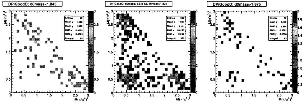
Figure 3.11: Dalitz distributions of m_D for D\pi_D events in the three bins used for the KS comparison shown in Table 3.17.
