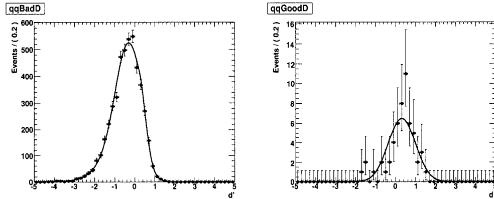
Figure 3.28: The distributions of d' for qq_p (left) and qq_D (right) obtained from MC.
