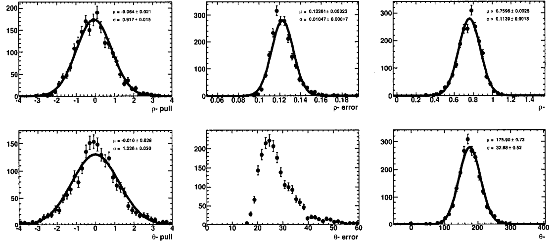
Figure 3.55: Results of 2000 toy MC experiments (signal and background, no systematic error in \mathcal{L}_{BA} ) for the pull (left), error (center) and fitted values (right) of \rho_- (top) and \theta_- (bottom). See Fig. 3.58 for the corresponding toy MC including systematic errors.
