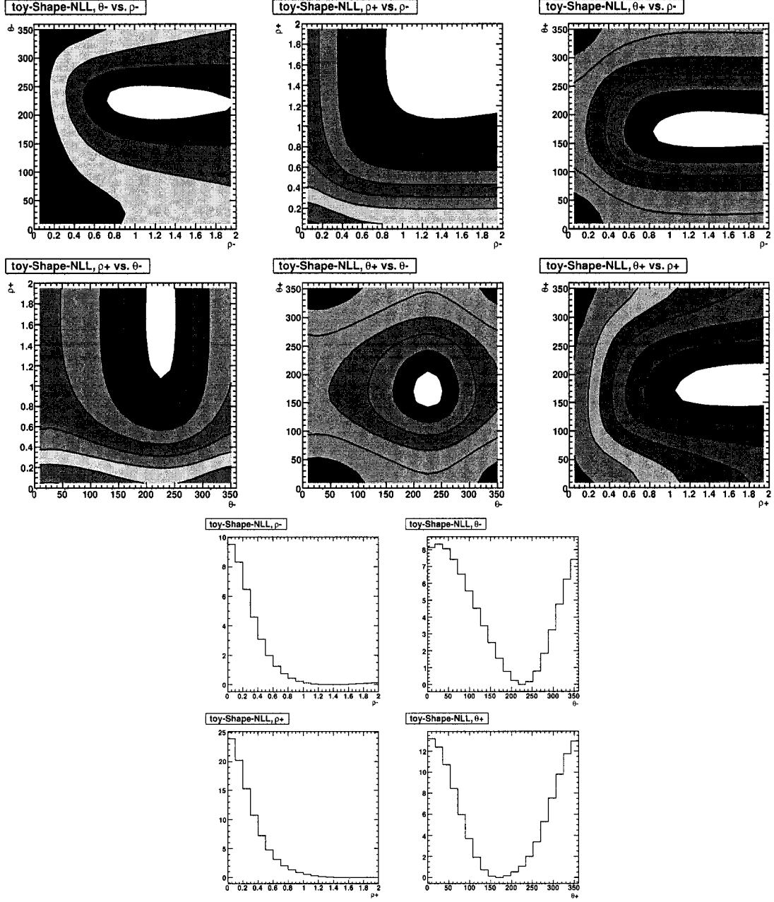
Figure 3.60: Dependence of \mathcal{L}_{\text{DP}} on all pair combinations of the parameters \rho_{\pm} , \theta_{\pm} (2D plots) with 1\sigma contours and the individual parameters in a toy experiment (1D plots).
