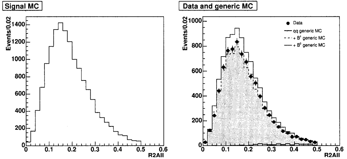
Figure 4.1: Fox-Wolfram moment R2 in B^- \rightarrow J/\psi \pi^+ \pi^- K^- for signal MC (left), generic MC and data (right).
