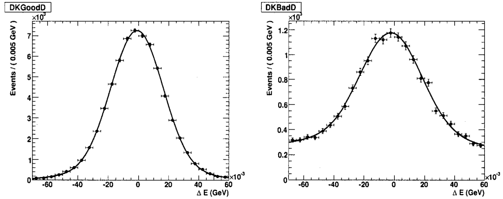
Figure 3.14: The distributions of \Delta E for DK_{\text{sig}} (left) and DK_{\text{bgd}} (right) obtained from MC.
