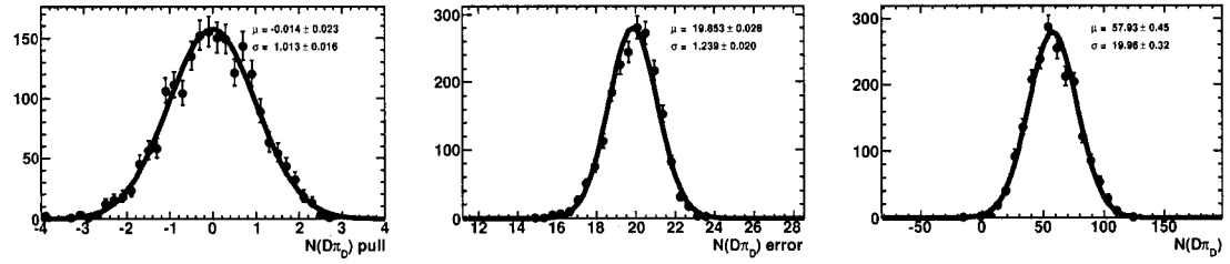
Figure 3.52: Results of 2000 toy MC experiments (signal and background, no systematic error in \mathcal{L}_{BA} ) for the pull (left), error (center) and fitted values (right) of N_{D\pi_D} .
