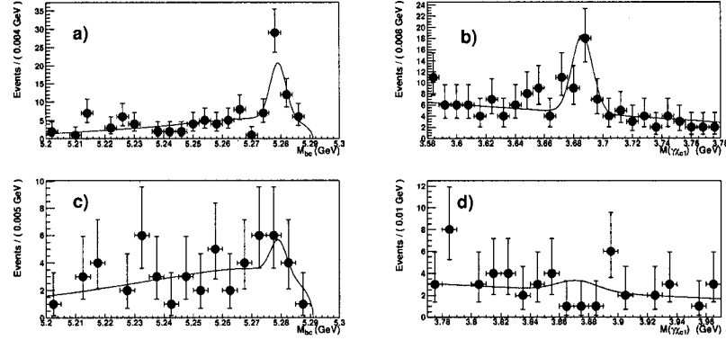
Figure 1.7: Signal-band projections of (a) m_{ES} and (b) m(\gamma\chi_{c1}) for the \psi(2S) region with the results of the unbinned fit superimposed from Belle. (c) and (d) are the corresponding results for the X(3872) region.
