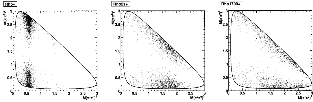
Figure 3.30: Dalitz plot distributions of \rho^+\pi^- , \rho(1450)^+\pi^- , and \rho(1700)^+\pi^- toy MC events.
