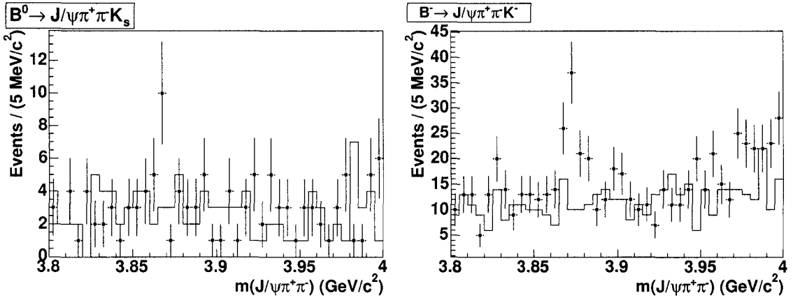
Figure 4.18: J/\psi \pi^+ \pi^- invariant mass spectrum between 3.8 and 4.0 \text{GeV}/c^2 in 5 \text{MeV}/c^2 bins. The dots represent the data and the solid line shows an m_{ES} sideband. The left plot shows B^0 \rightarrow J/\psi \pi^+ \pi^- K_s^0 and the right plot shows B^- \rightarrow J/\psi \pi^+ \pi^- K^- .
