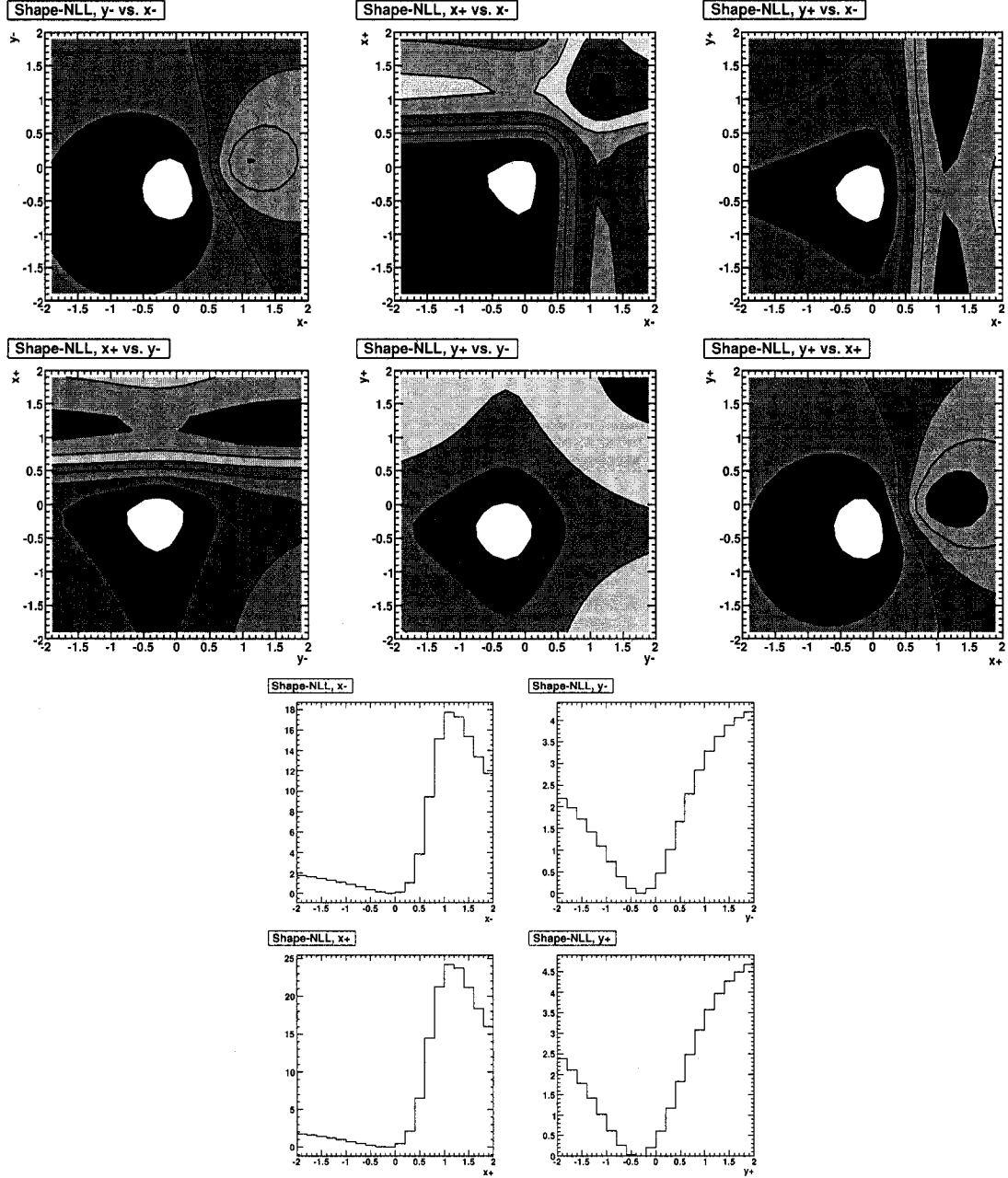
Figure 3.45: Dependence of the negative log likelihood \mathcal{L}_{DP} , computed with a single toy MC experiment containing both signal and background, on all pair combinations of the parameters x_{\pm}, y_{\pm} (2D plots, 1\sigma contours) and on the individual parameters (1D plots). The true values of x_{\pm}, y_{\pm} are 0. The values of the parameters not shown in each plot are set to their true values.
