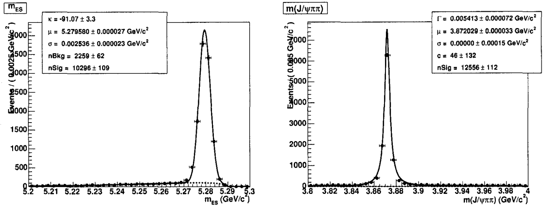
Figure 4.4: 1-dimensional UEML-fit to the m_{ES} (left) and m_X (right) distribution on signal MC for B^0 \rightarrow J/\psi \pi^+ \pi^- K_S^0 .
