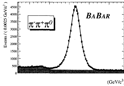
Figure 3.43: \pi^+\pi^-\pi^0 invariant mass of D^0 candidates obtained from D^{*+} \rightarrow D^0\pi_s^+ decays. The dots represent the data, the dashed line shows the combinatorial background and the shaded region represents the total background.
