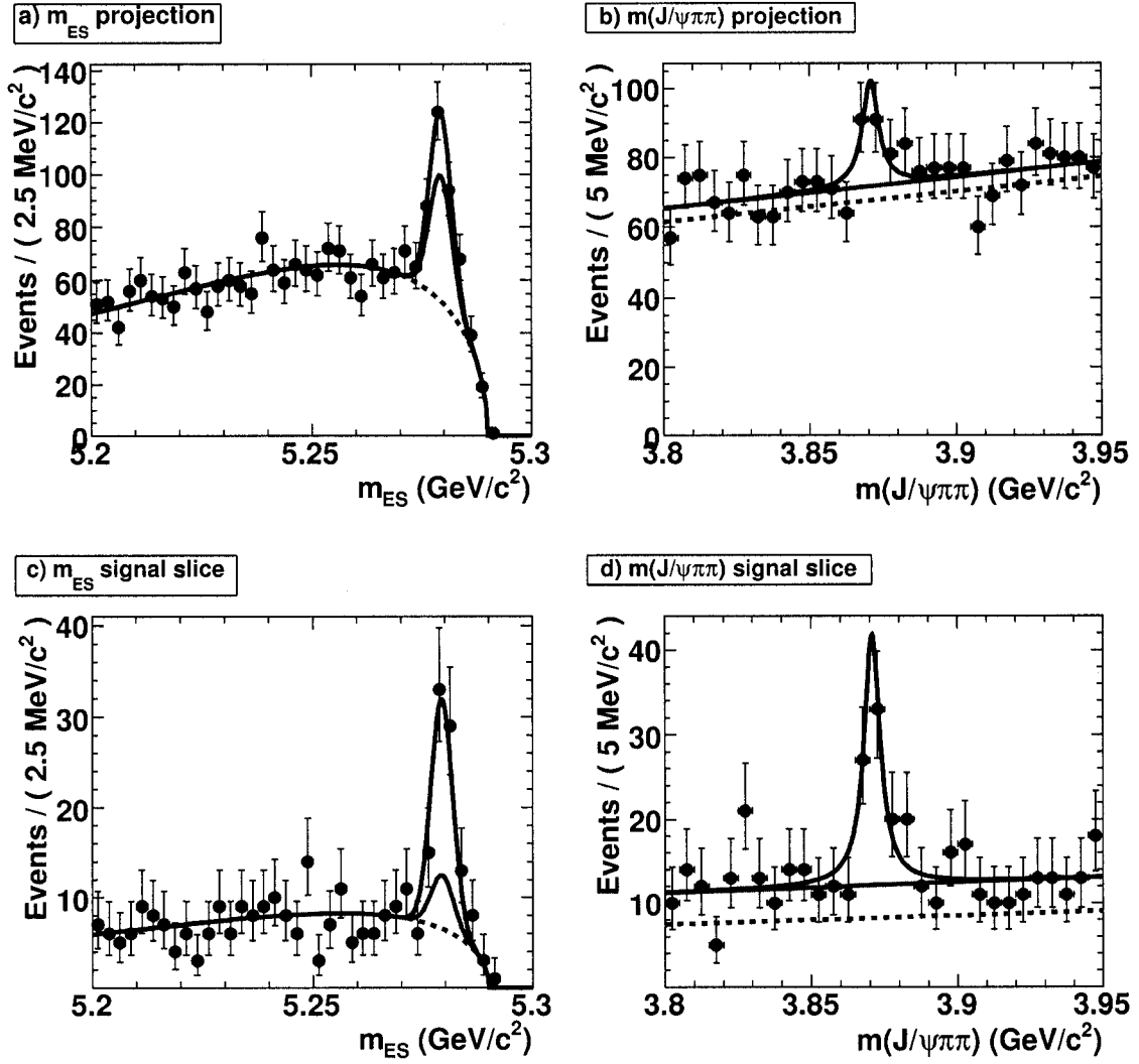
Figure 4.14: The fit result on 210.6 \text{ fb}^{-1} of data in B^- \rightarrow X(3872)K^- . The lines represent (from bottom to top) combinatorial background (dotted, blue), peaking background (solid, red) and signal events (solid, blue). a) and b) are projections on m_{ES} and m_X , respectively. Plots c) and d) show the signal band projection with an additional cut on the signal region of the variable not shown. Note the different bin size in m_X compared to Fig. 4.13.
