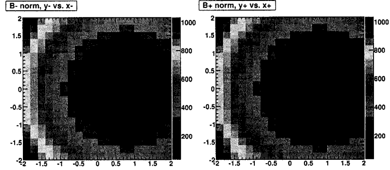
Figure 3.47: Dependence of the expected number of events N_{\text{exp}}^{\pm} on the true values of the CP parameters x_{\pm}, y_{\pm} in a toy experiment.
