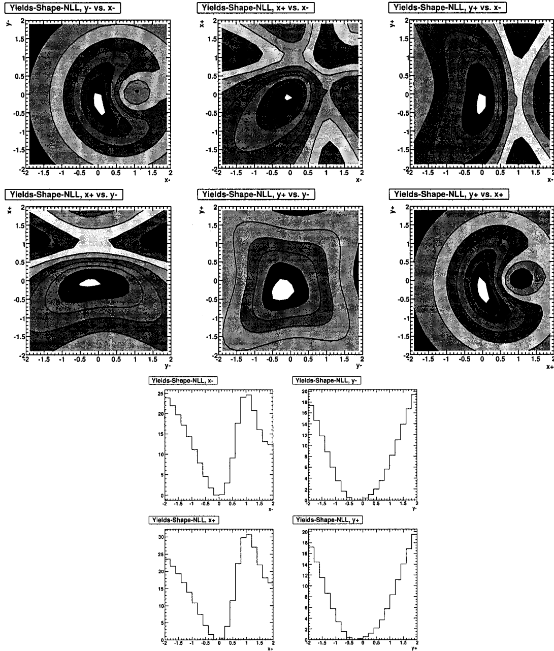
Figure 3.49: Dependence of \mathcal{L} on all pair combinations of the parameters x_{\pm}, y_{\pm} (2D plots, 1\sigma contours) and on the individual parameters (1D plots) in a toy experiment. The true values of x_{\pm}, y_{\pm} are 0. The values of the parameters not shown in each plot are set to their true values.
