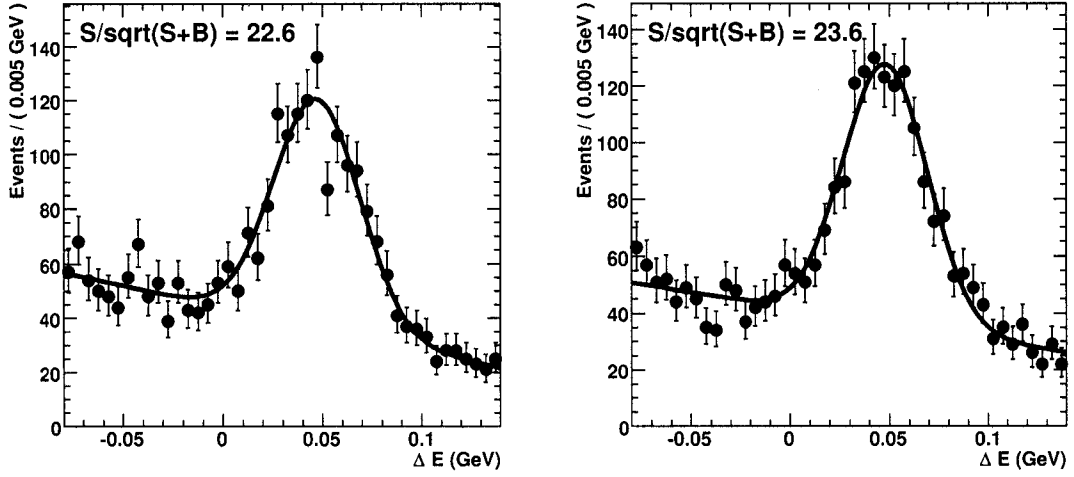
Figure 3.83: Fits to the \Delta E distribution of negative (left) and positive (right) B \rightarrow D_{\pi^+\pi^-\pi^0\pi^-} candidates in the data.
