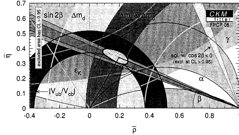
Figure 1.2: Experimental constraints [9] on the apex of the Unitarity Triangle. \bar{\rho} = \rho(1 - \lambda^2/2) and \bar{\eta} = \eta(1 - \lambda^2/2) are the rescaled Wolfenstein parameters. \epsilon_K is the CP violating parameter in the kaon system and \Delta m_{s,d} are measurements obtained from B_{s,d}^0 mixing.
