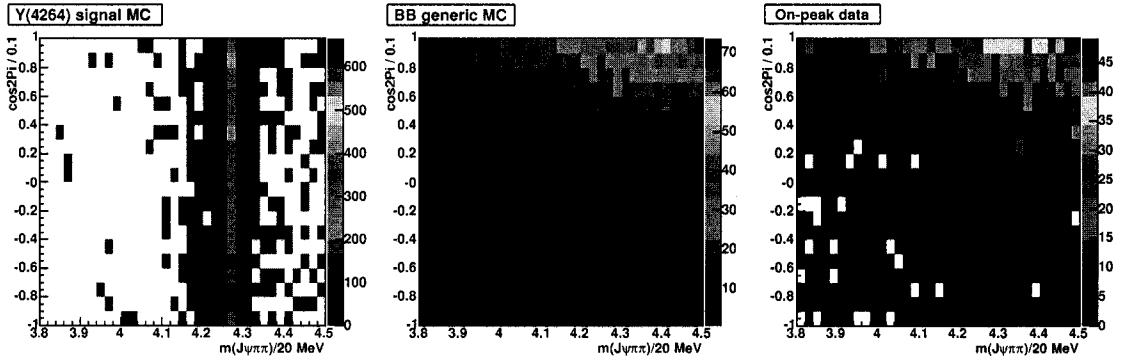
Figure 4.25: The angle \cos 2\pi_i versus the J/\psi \pi^+\pi^- invariant mass for signal MC (left), B\bar{B} generic MC (middle) and data (right)
