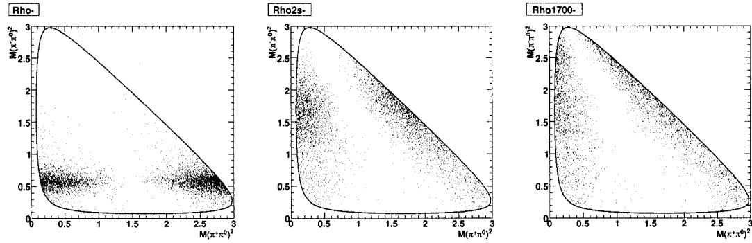
Figure 3.31: Dalitz plot distributions of \rho^-\pi^+ , \rho(1450)^-\pi^+ , and \rho(1700)^-\pi^+ MC events.
