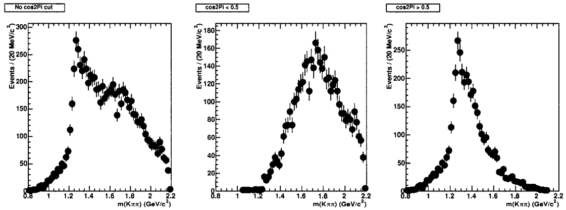
Figure 4.27: The K \pi^+ \pi^- invariant mass without \cos 2\pi_i cut (left), \cos 2\pi_i < 0.5 (middle) and \cos 2\pi_i > 0.5 (right) for on-peak data.
