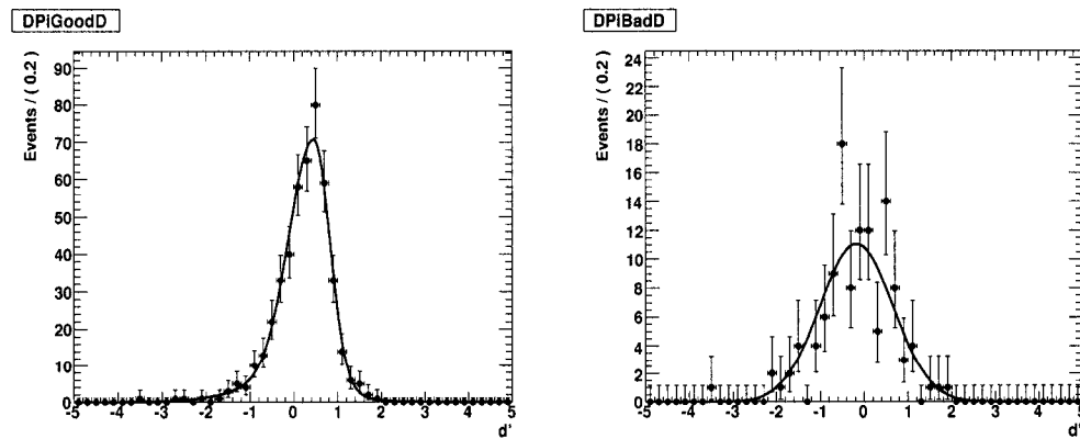
Figure 3.25: The distributions of d' for D\pi_D (left) and D\pi_p (right) obtained from MC.
