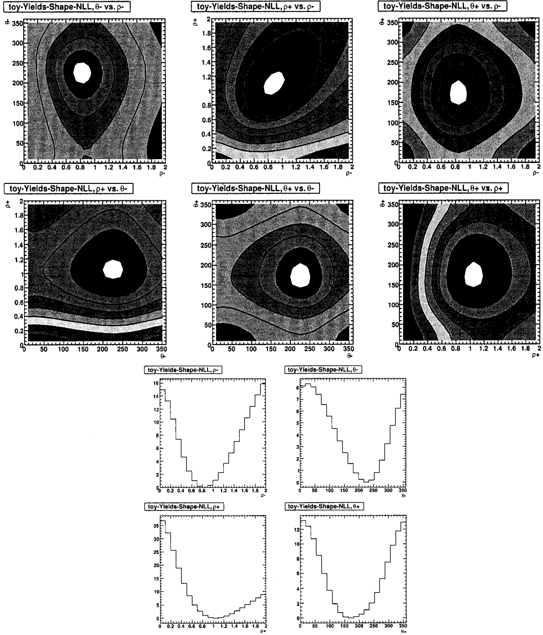
Figure 3.62: Dependence of \mathcal{L} = \mathcal{L}_{\text{DP}} + \mathcal{L}_{\text{BA}} on all pair combinations of the parameters \rho_{\pm} , \theta_{\pm} (2D plots) with 1\sigma contours and the individual parameters in a toy experiment (1D plots).
