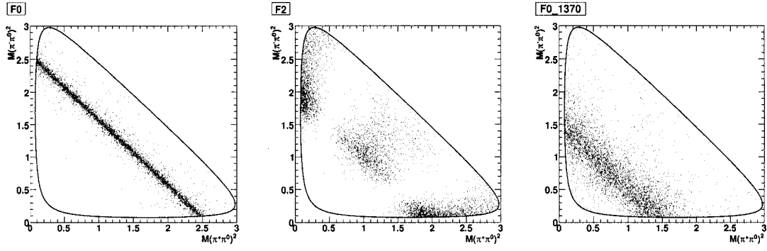
Figure 3.33: Dalitz plot distributions of f_0\pi^0 , f_2\pi^0 , and f_0(1370)\pi^0 toy MC events.
