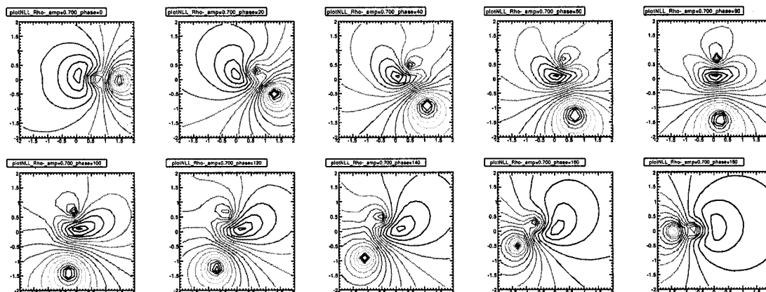
Figure 3.46: \mathcal{L}_{\text{DP}} of a signal-only B^- toy sample as a function of x_- and y_- if the Dalitz plot contains only \rho^+ and \rho^- . The phase difference between them varies from 0^\circ (top left) to 180^\circ (bottom right) in 20^\circ steps.
