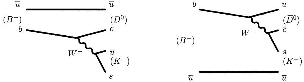
Figure 1.3: Color allowed B^- \rightarrow D^0 K^- (left) and color suppressed B^- \rightarrow \bar{D}^0 K^- decay (right). The b \rightarrow u transition in the right decay gives rise to the weak phase e^{-i\gamma} .
