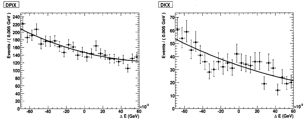
Figure 3.16: The distributions of \Delta E for D\pi X (left) and DKX (right) obtained from MC.
