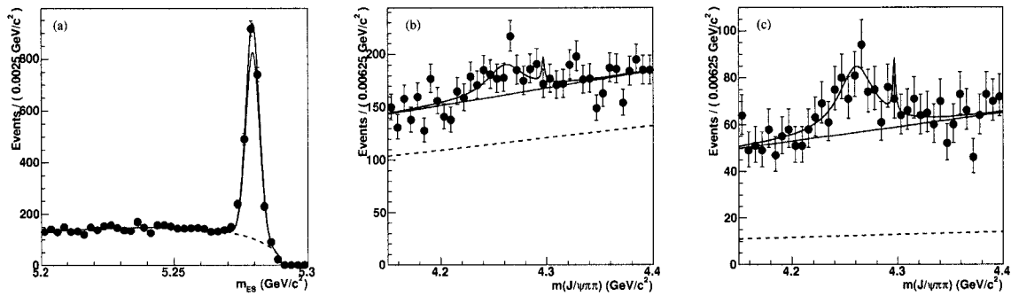
Figure 4.20: Fit to a MC cocktail of B\bar{B} generic MC and Y(4264) without the additional narrow resonance. Plots a) and b) show the fit projections for m_{ES} and m_X whereas plot c) shows the m_X projection with a cut on the m_{ES} signal region applied.
