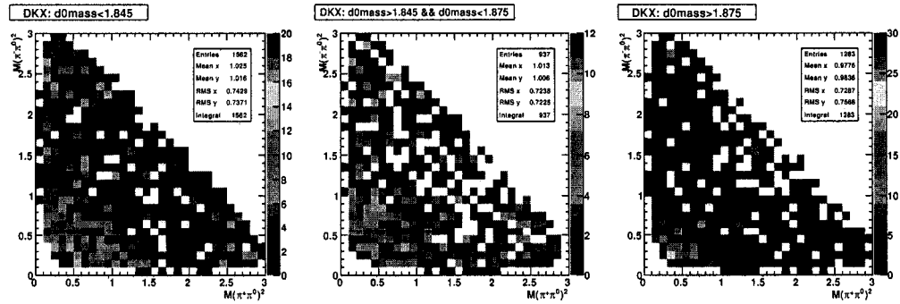
Figure 3.10: Dalitz distributions of m_D for DKX events in the three bins used for the KS comparison shown in Table 3.16.
