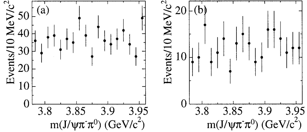
Figure 1.12: J/\psi\pi^-\pi^0 invariant mass for (a) B^0 \rightarrow J/\psi\pi^-\pi^0K^+ (b) and B^- \rightarrow J/\psi\pi^-\pi^0K_s^0 . No evidence for a charged partner of the X(3872) is found.
