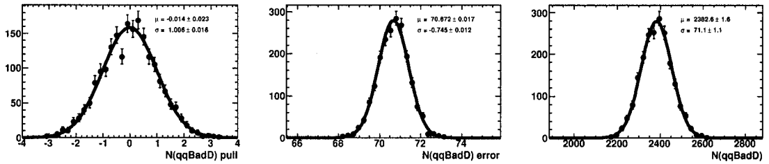
Figure 3.50: Results of 2000 toy MC experiments (signal and background, no systematic error in \mathcal{L}_{BA} ) for the pull (left), error (center) and fitted values (right) of N_{qq\bar{p}} .
