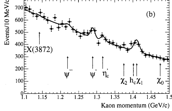
Figure 1.13: Kaon momentum spectrum for B^- \rightarrow X_{c\bar{c}} K^- in the X(3872) region. The arrows indicate the position of known charmonium states. No evidence for the X(3872) is found.
