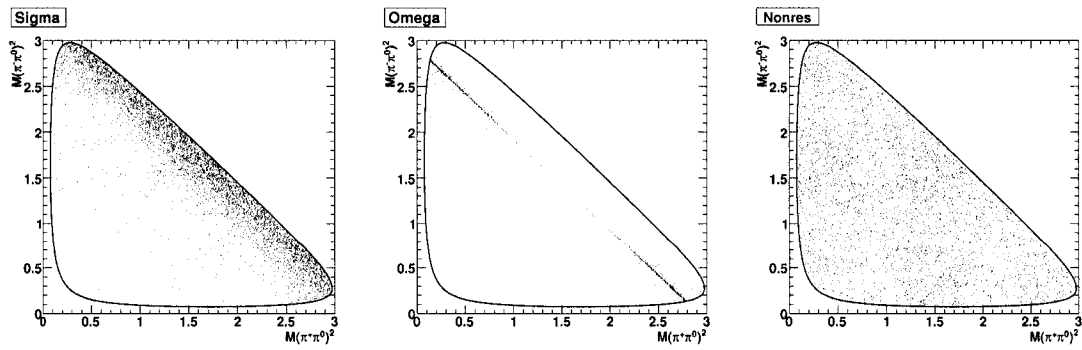
Figure 3.35: Dalitz plot distributions of \sigma\pi^0 , \omega\pi^0 , and nonresonant toy MC events.
