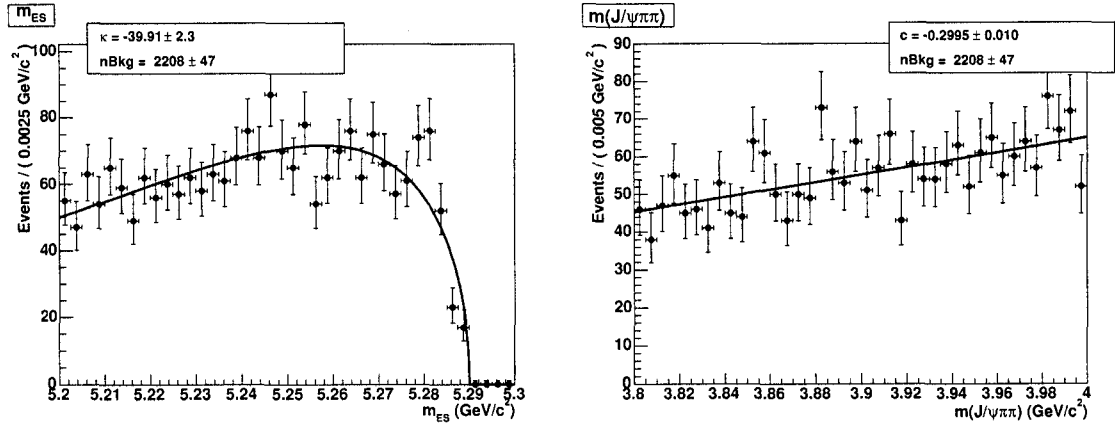
Figure 4.6: 1-dimensional UEML-fit to the m_{ES} (left) and m_X (right) distribution on generic MC for combinatorial background events in B^0 \rightarrow J/\psi \pi^+ \pi^- K_S^0 .
