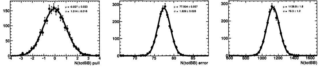
Figure 3.73: Results of 2000 toy MC experiments (signal and background) for the pull (left), error (center) and fitted values (right) of N_{BB\bar{p}} .
