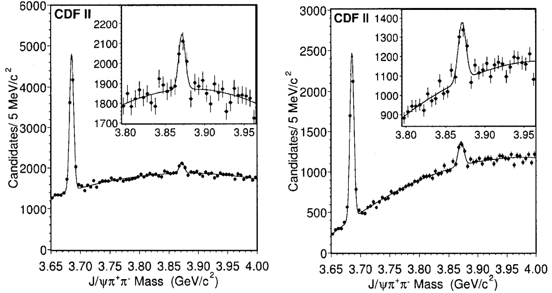
Figure 1.14: (left) The mass distribution of J/\psi \pi^+ \pi^- observed by CDF II in inclusive p \bar{p} collisions. A large peak for the \psi(2S) is seen and a signal near a mass of 3872 \text{ MeV}/c^2 is visible (enlargement shown in the inset). (right) shows the same requiring m(\pi^+ \pi^-) > 500 \text{ MeV}/c^2 .
