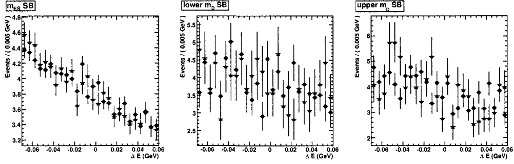
Figure 3.12: Comparison of \Delta E distributions in data (black triangles) and MC (blue circles) in the m_{ES} (left), lower m_D (middle) and upper m_D (right) sideband for 0.1 < q < 1.0 . The p-values of a \chi^2 -test are listed in Table 3.22.
