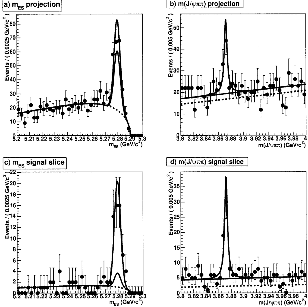
Figure 4.8: The fit result of an arbitrary experiment in B^0 \rightarrow J/\psi \pi^+ \pi^- K_S^0 . The lines represent (from bottom to top) combinatorial background (dotted, blue), peaking background (solid, red) and signal events (solid, blue). a) and b) are projections on m_{ES} and m_{\chi} , respectively. Plots c) and d) show the signal band projection with an additional cut on the signal region of the variable not shown.
