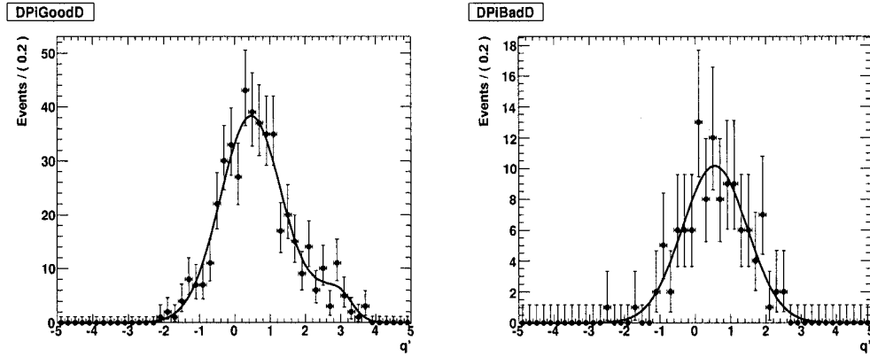
Figure 3.20: The distributions of q' for D\pi_D (left) and D\pi_p (right) obtained from MC.
