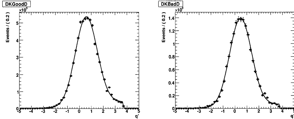
Figure 3.19: The distributions of q' for DK_{\text{sig}} (left) and DK_{\text{bgd}} (right) obtained from MC.
