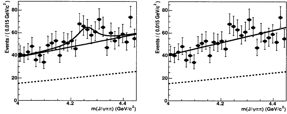
Figure 4.34: m_X projections of the fit result with K_1 veto and signal parameters fixed to the results in the ISR analysis for the signal (left) and background (right) hypothesis.
