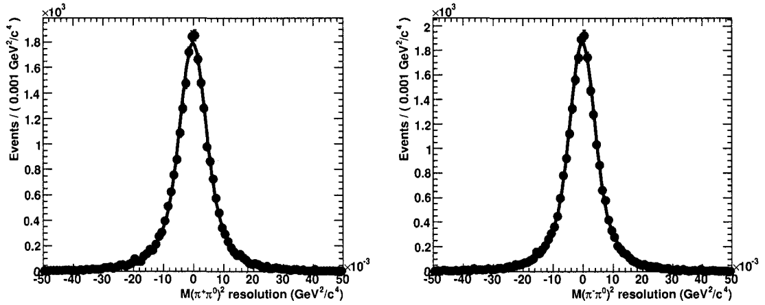
Figure 3.63: Resolution of the Dalitz variables s_{+0} (left) and s_{-0} (right) for DK_{\text{sig}} events. The superimposed curve shows a fit using the sum of three Gaussians with common mean.
