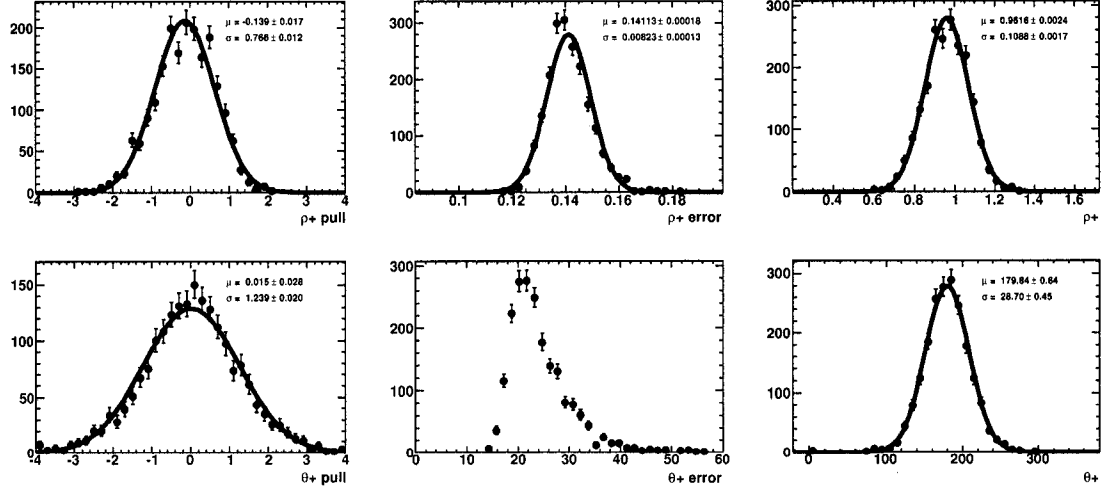
Figure 3.59: Results of 2000 toy MC experiments (signal and background, including systematic error in \mathcal{L}_{\text{BA}} ) for the pull (left), error (center) and fitted values (right) of \rho_+ (top) and \theta_+ (bottom). See Fig. 3.56 for the corresponding toy MC without systematic errors.
