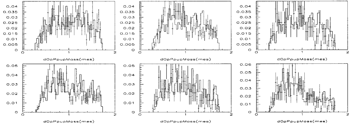
Figure 3.6: Comparison of s_{+0} in bins of m_{ES} for DKX events corresponding to the KS probabilities of Table 3.10 (from left to right, top to bottom).
