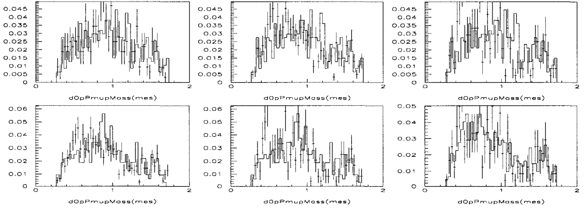
Figure 3.5: Comparison of s_{-0} in bins of m_{ES} for DKX events corresponding to the KS probabilities of Table 3.10 (from left to right, top to bottom).
