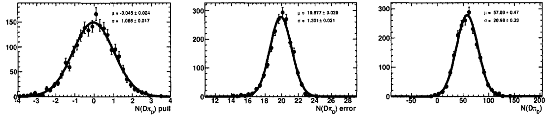
Figure 3.74: Results of 2000 toy MC experiments (signal and background) for the pull (left), error (center) and fitted values (right) of N_{D\pi_D} .
