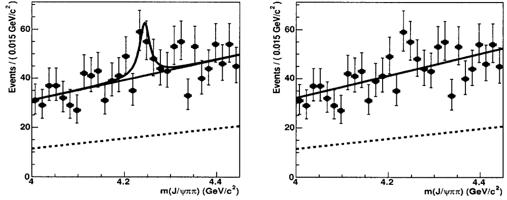
Figure 4.33: m_X projections of the fit result with K_1 veto and |\cos \theta_l| < 0.8 for the signal (left) and background (right) hypothesis. See Tab. 4.13 for the fit parameters.
