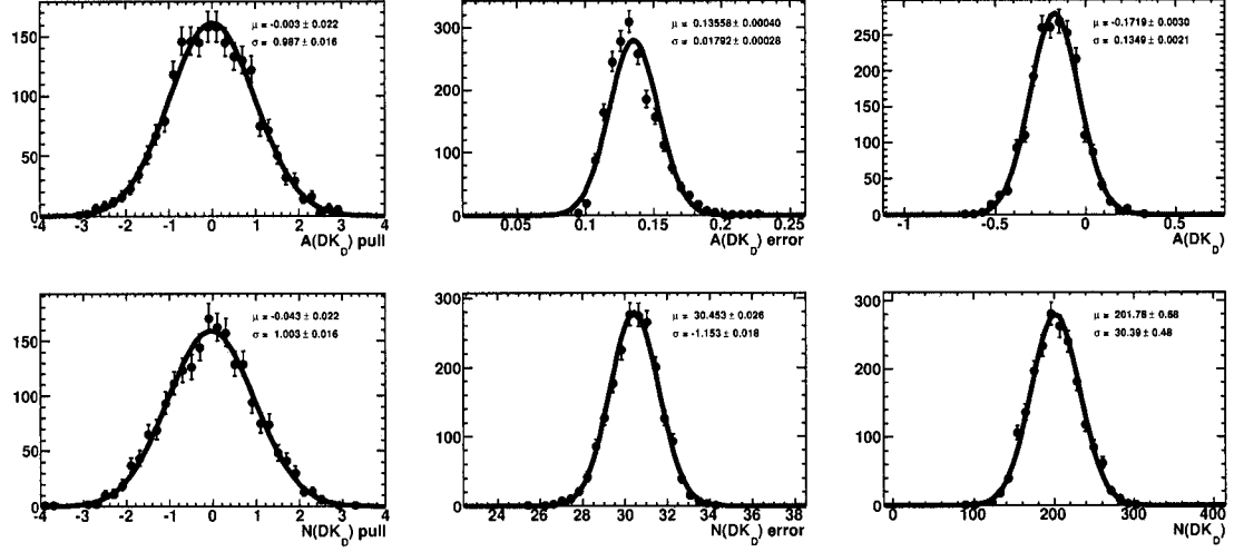
Figure 3.54: Results of 2000 toy MC experiments (signal and background, no systematic error in \mathcal{L}_{BA} ) for the pull (left), error (center) and fitted values (right) of A_{DK_{\text{sig}}} (top) and N_{DK_{\text{sig}}} (bottom).
