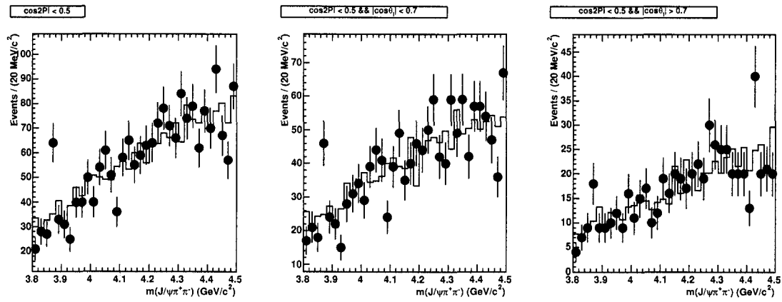
Figure 4.31: The J/\psi \pi^+ \pi^- invariant mass without \cos \theta_l cut (left), |\cos \theta_l| < 0.7 (middle) and |\cos \theta_l| > 0.7 (right) for events with \cos 2\text{Pi} < 0.5 . The dots are on-peak data and the solid line shows B\bar{B} generic MC scaled to the same number of events.
