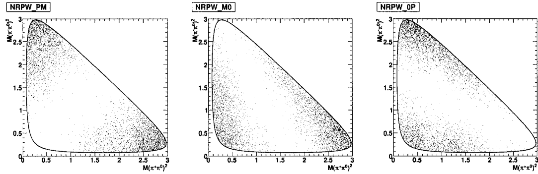
Figure 3.36: Dalitz plot distributions of nonresonant P -wave toy events, with the P -wave particles being the \pi^+\pi^- (left), \pi^-\pi^0 (center), or \pi^0\pi^+ (right).
