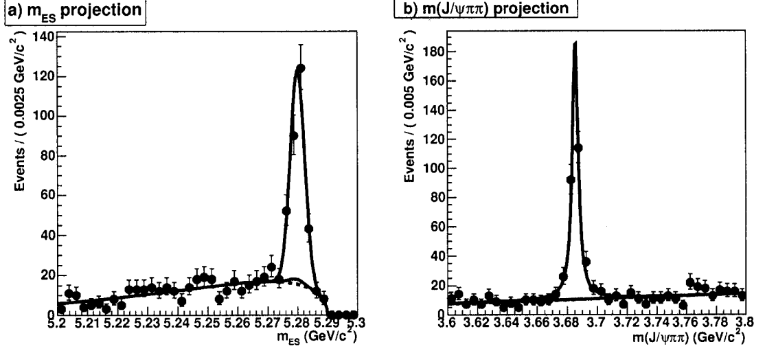
Figure 4.11: The fit result on 210.6 \text{ fb}^{-1} of data for the benchmark mode B^0 \rightarrow \psi(2S) K_S^0 . The lines represent (from bottom to top) combinatorial background (dotted, blue), peaking background (solid, red) and signal events (solid, blue).
