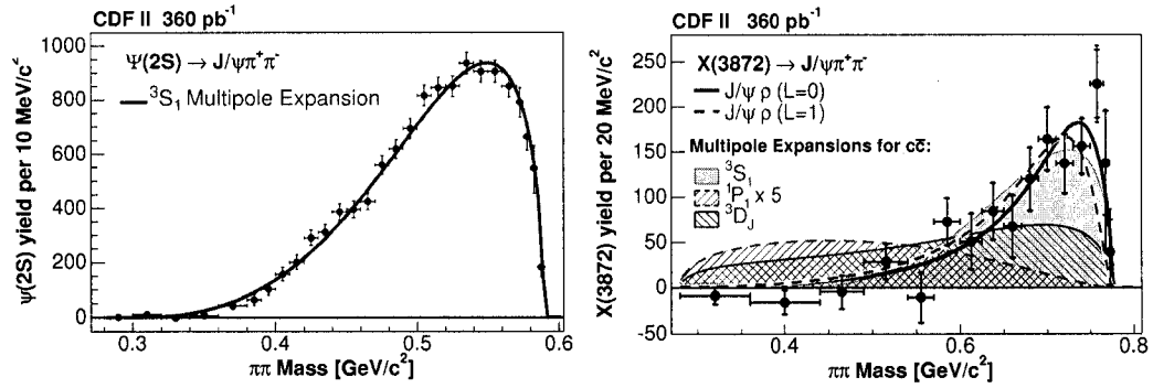
Figure 1.15: The dipion mass spectrum as observed by CDF II for the \psi(2S) (left) and X(3872) (right) together with fits to various hypothesis.
