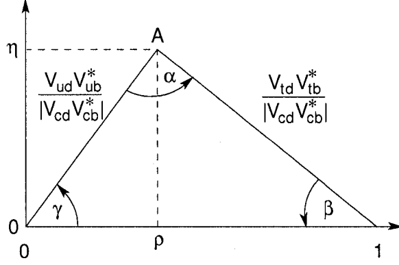
Figure 1.1: The rescaled Unitarity Triangle described by Eq. (1.12).
