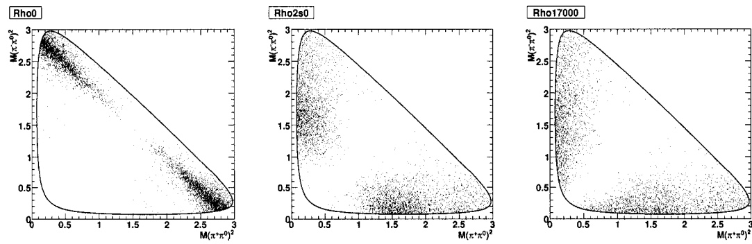
Figure 3.32: Dalitz plot distributions of \rho^0\pi^0 , \rho(1450)^0\pi^0 , and \rho(1700)^0\pi^0 toy MC events.
