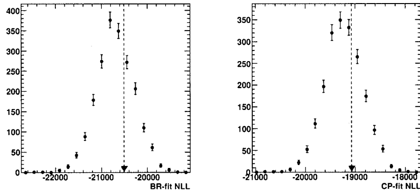
Figure 3.57: Minimum value of the NLL from the 2000 toy MC experiments for the yields step-1 fit (left) and the CP step-2 fit (right). The arrow indicates the NLL found in the data fit (section 3.10).
