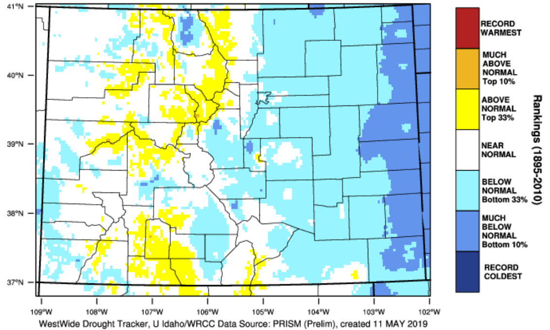
Colorado - Mean Temperature October-April 2019 Percentile
