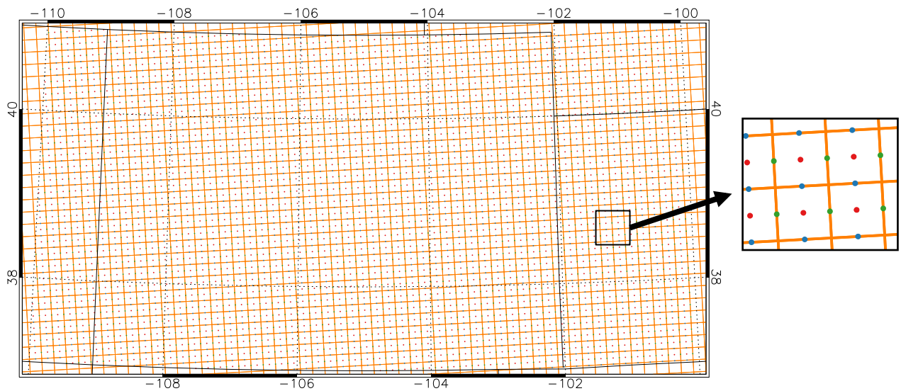
Figure 1. Kriging grid (in orange) with grid points (in red, blue, and green) zoomed in over Colorado with an insert to the right zoomed in over only a few grid cells to show detail.
