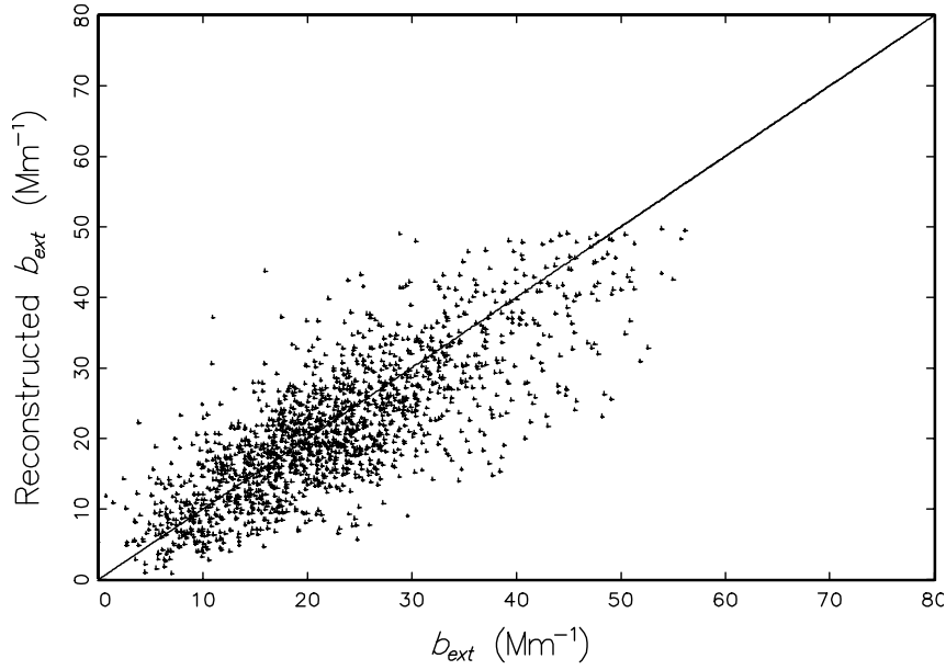
Figure 4.13 Reconstructed b_{ext} using b_{lac} and the sum of estimated aerosol scattering from the various aerosol species is plotted against measured b_{ext} for the IMPROVE data set. Units are in \text{Mm}^{-1} .
