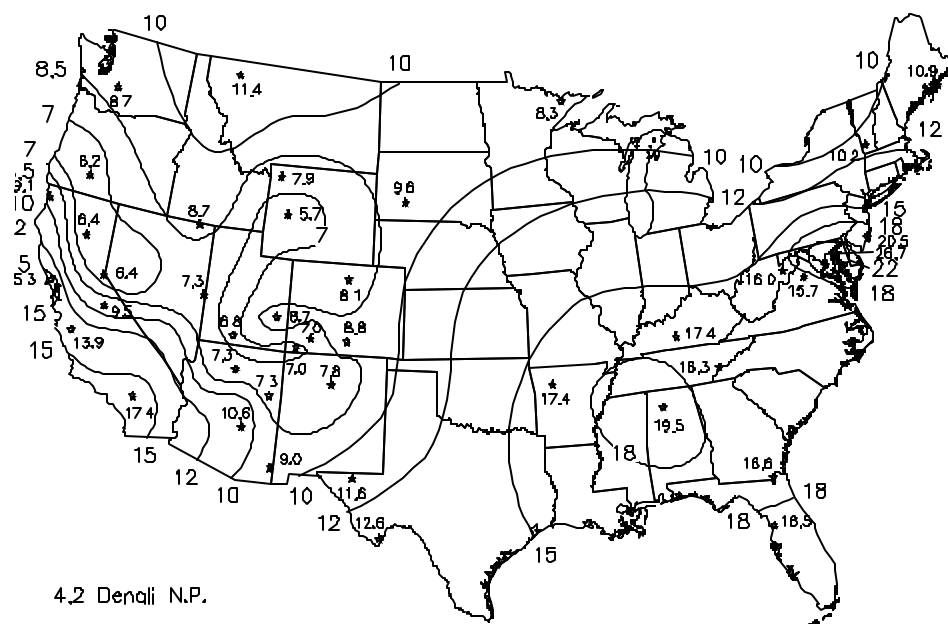
Figure 3.1 Average \text{PM}_{10} mass concentration (in \mu\text{g}/\text{m}^3 ) for each site in the IMPROVE network.
