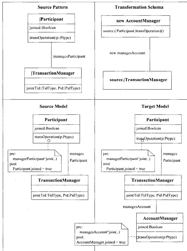
Figure 4.10: The source Directive Applied to Operation Templates.
