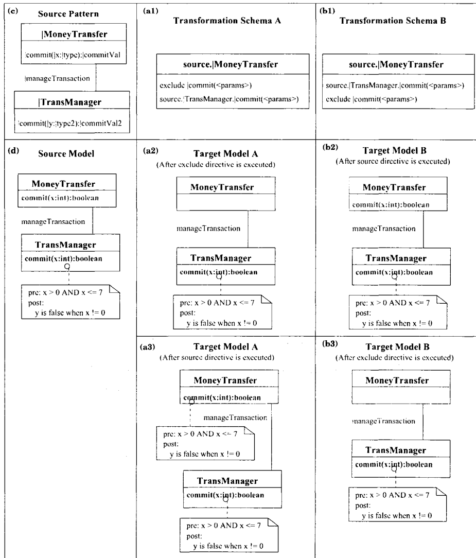
Figure 4.36: Ordering Transformation Directives - Example 1.
