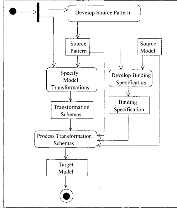
Figure 4.1: Model Transformation Process.
