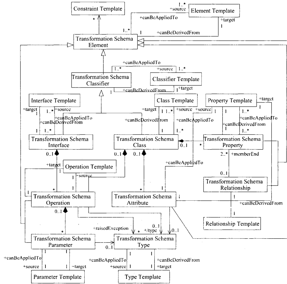
Figure 4.19: Transformation Implementation Metamodel Showing Relationships.
