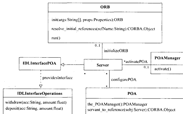
Figure 1.3: The Target Model.
