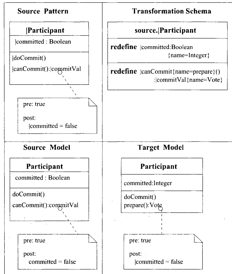
Figure 4.11: The redefine Directive.
