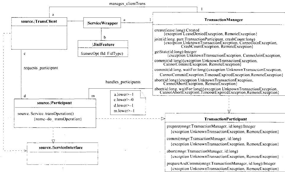
Figure 6.5: Jini Class Diagram Transaction Transformation Schema.
