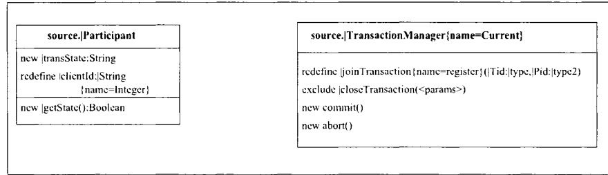
Figure 4.3: Transformation Schema.
