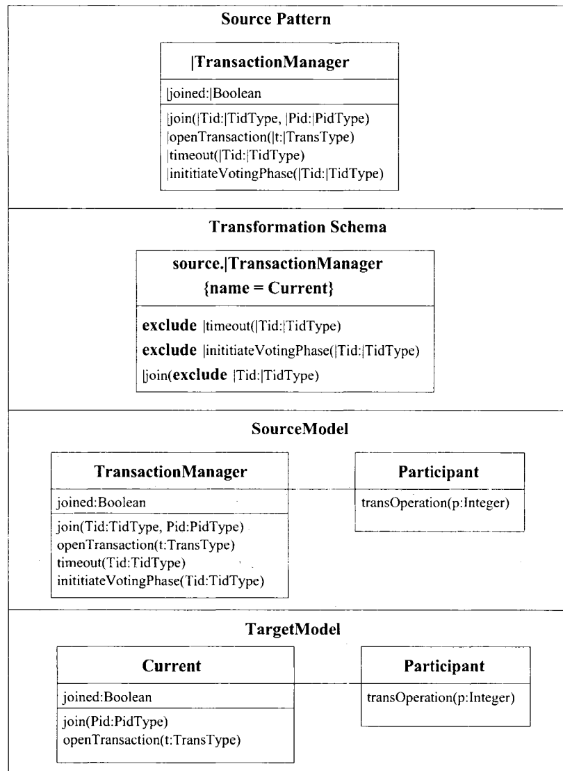
Figure 4.14: The exclude Directive.
