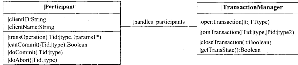
Figure 4.2: Source Pattern for Simple Transaction Service.
