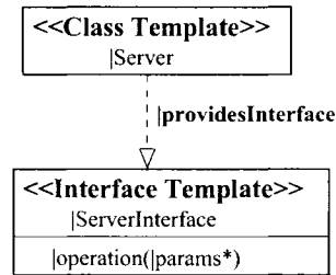
Figure 5.1: Source Pattern.
