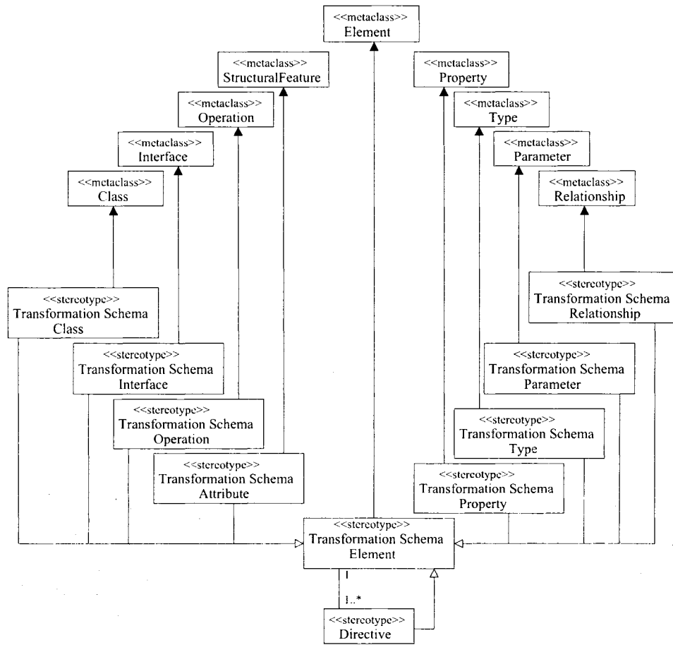
Figure 4.8: Transformation Schema Stereotypes.
