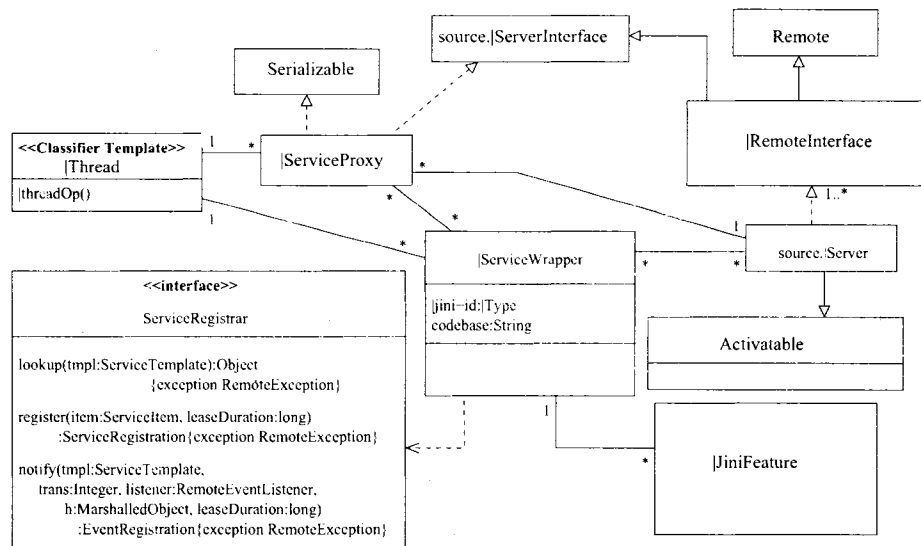
Figure 5.5: Class Transformation Schema.
