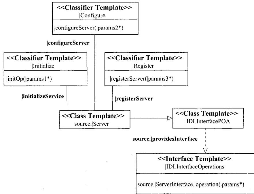
Figure 5.7: Target Class Pattern
