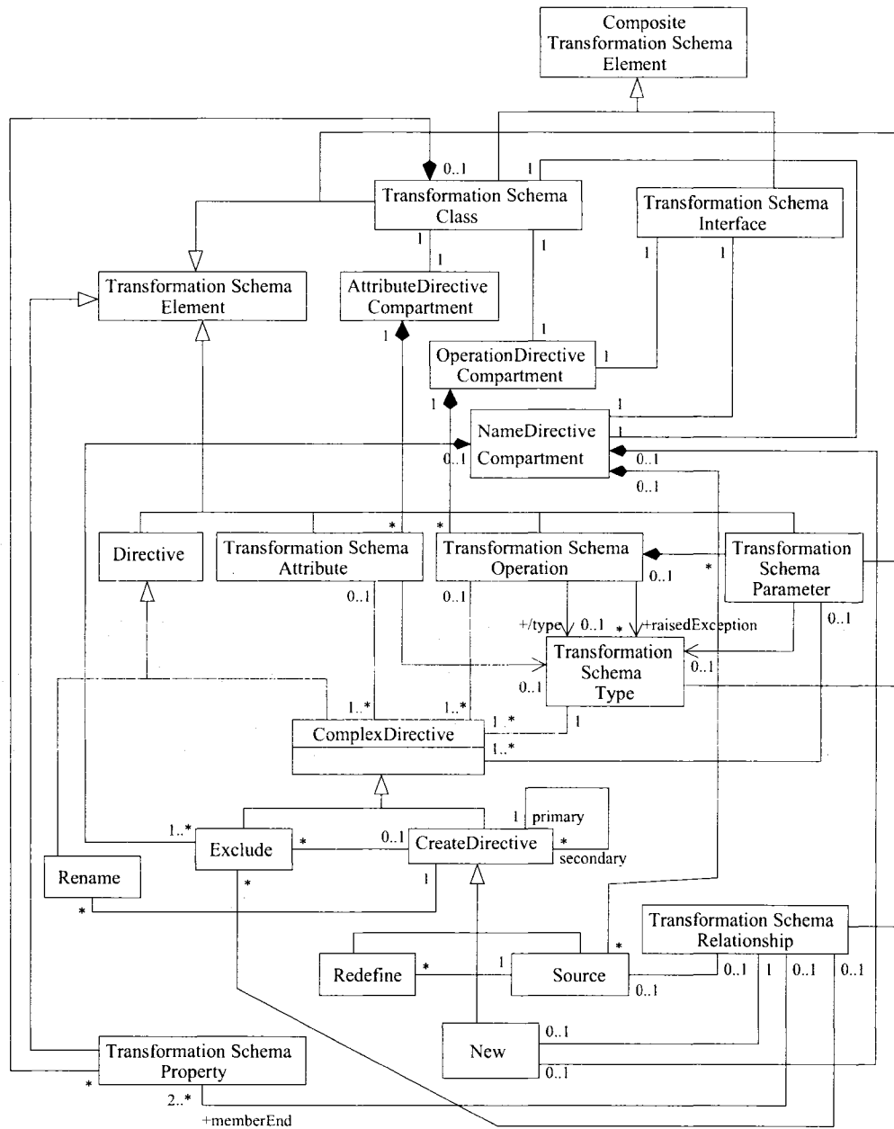
Figure 4.17: Transformation Schema Class Diagram Metamodel.
