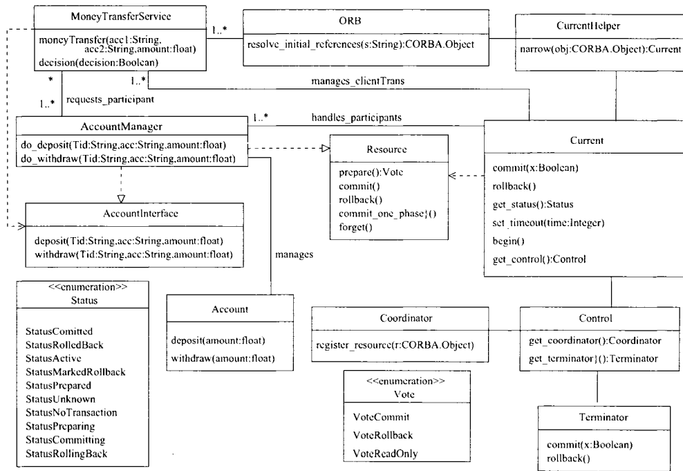
Figure 6.4: Target CORBA Transaction Class Model.
