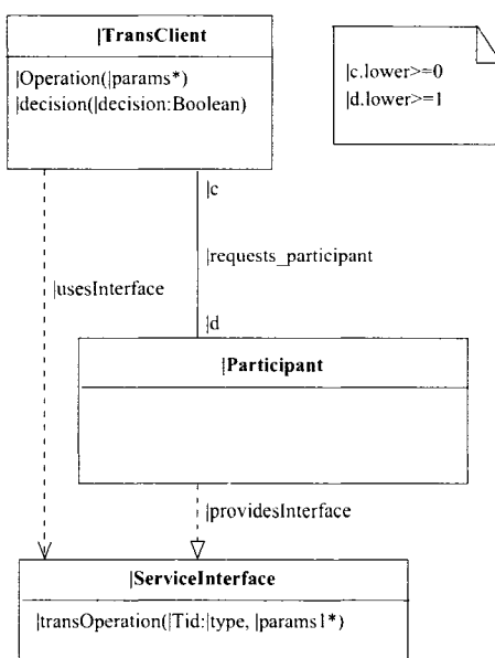
Figure 6.1: Source Class Pattern for Distributed Transactions.
