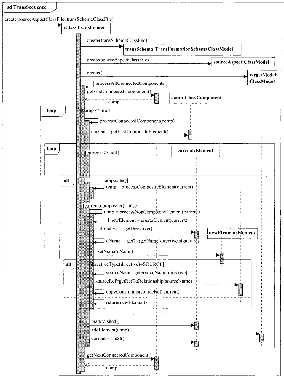
Figure 4.24: Sequence Diagram for Transformation Algorithm.
