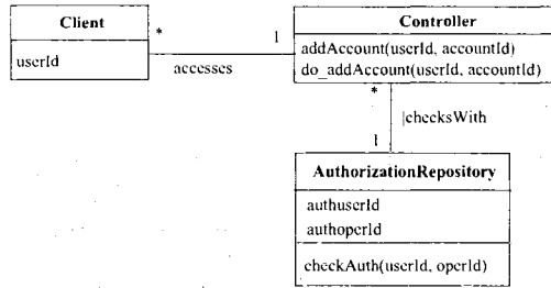
Figure 2.1: Example of A Class Diagram Template
