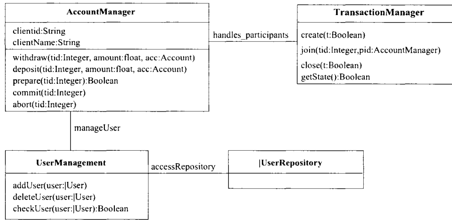
Figure 4.4: Source Model for Simple Transaction Service.
