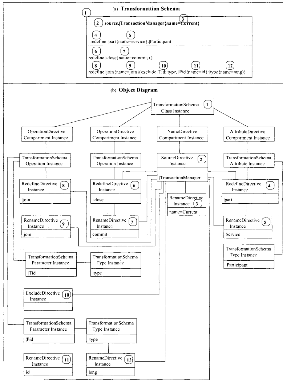
Figure 4.18: Transformation Schema Object Diagram.
