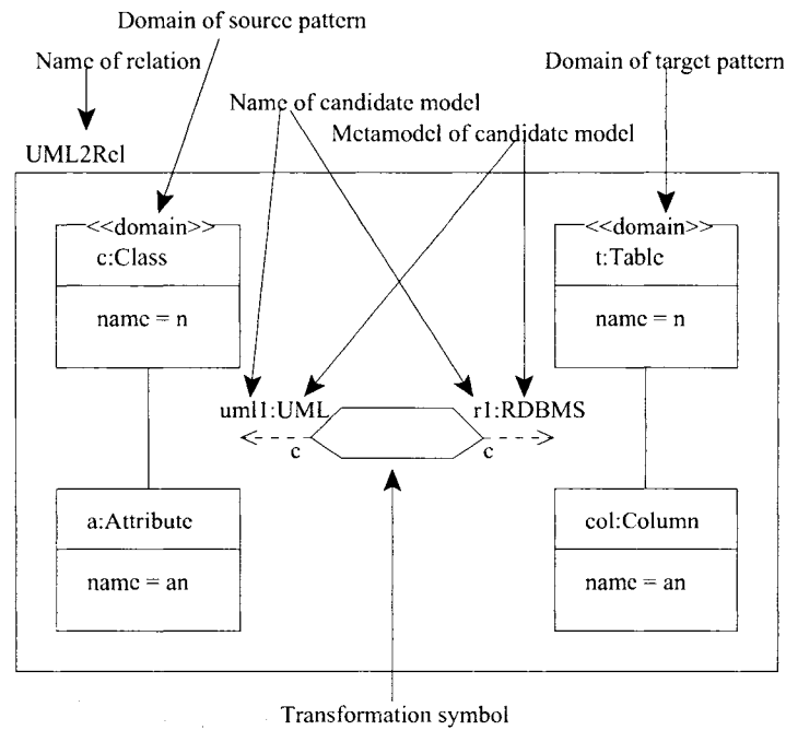
Figure 3.3: UML Class to Relational Table Relation [26].
