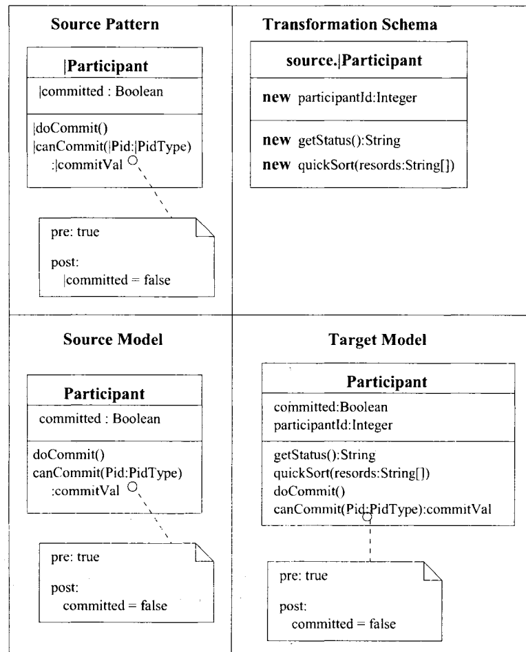
Figure 4.12: The new Directive.
