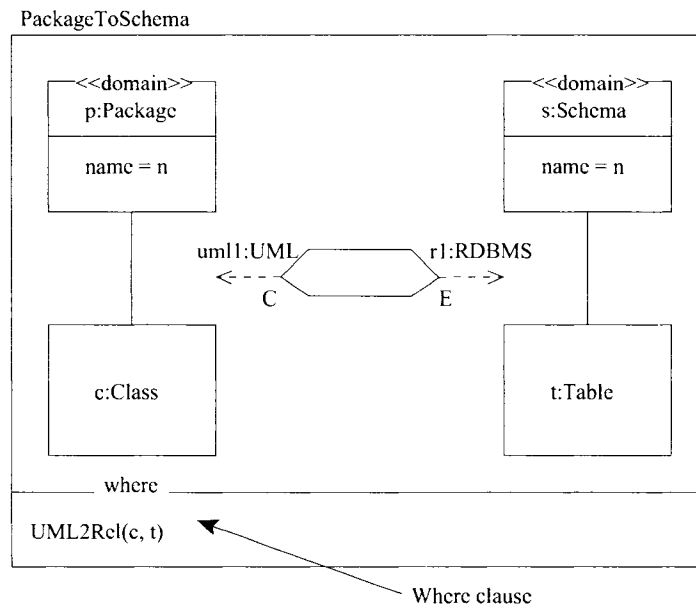
Figure 3.4: QVT Relation With where Clause [25].
