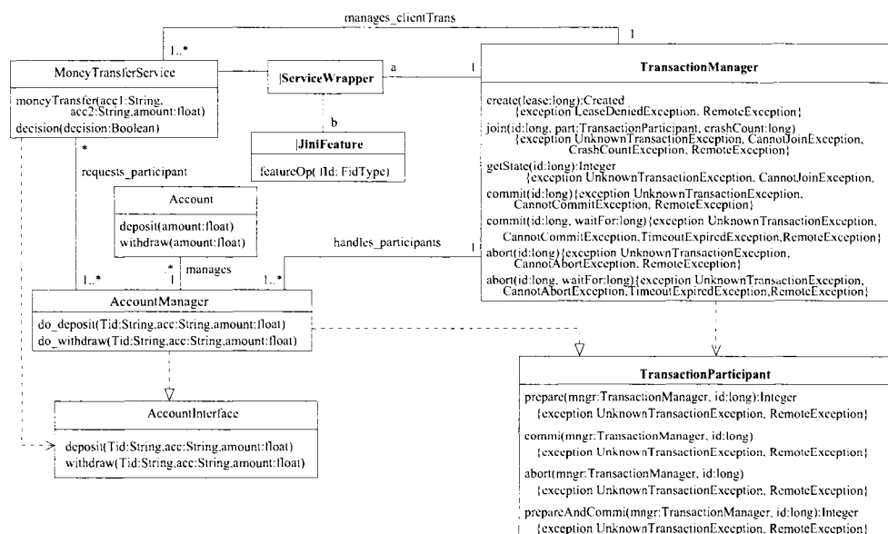
Figure 6.6: Target Jini Transaction Class Model.
