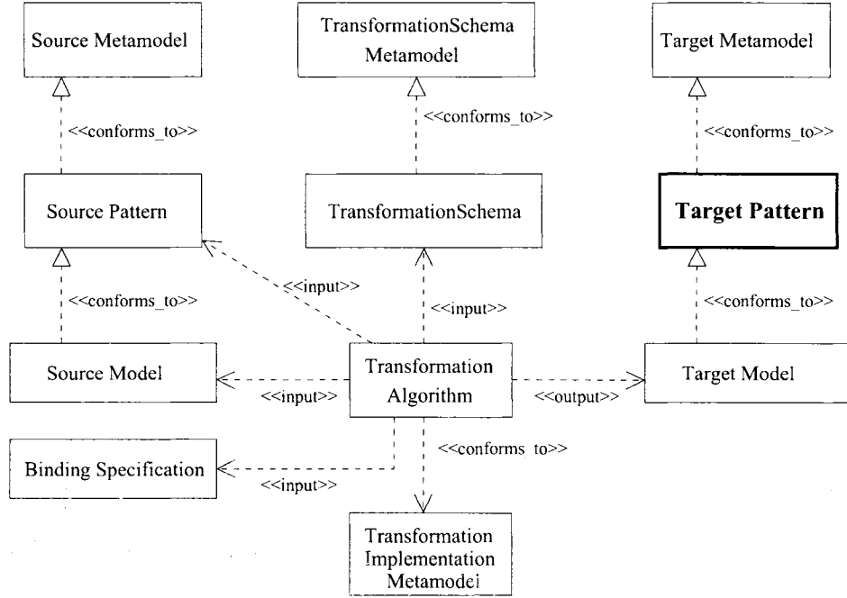
Figure 4.39: Transformation Conceptual Model With Target Pattern.
