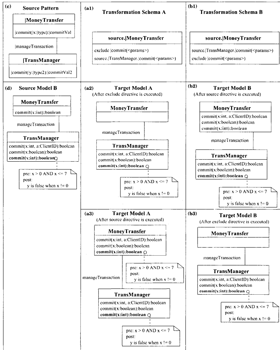
Figure 4.37: Ordering Transformation Directives - Example 2.
