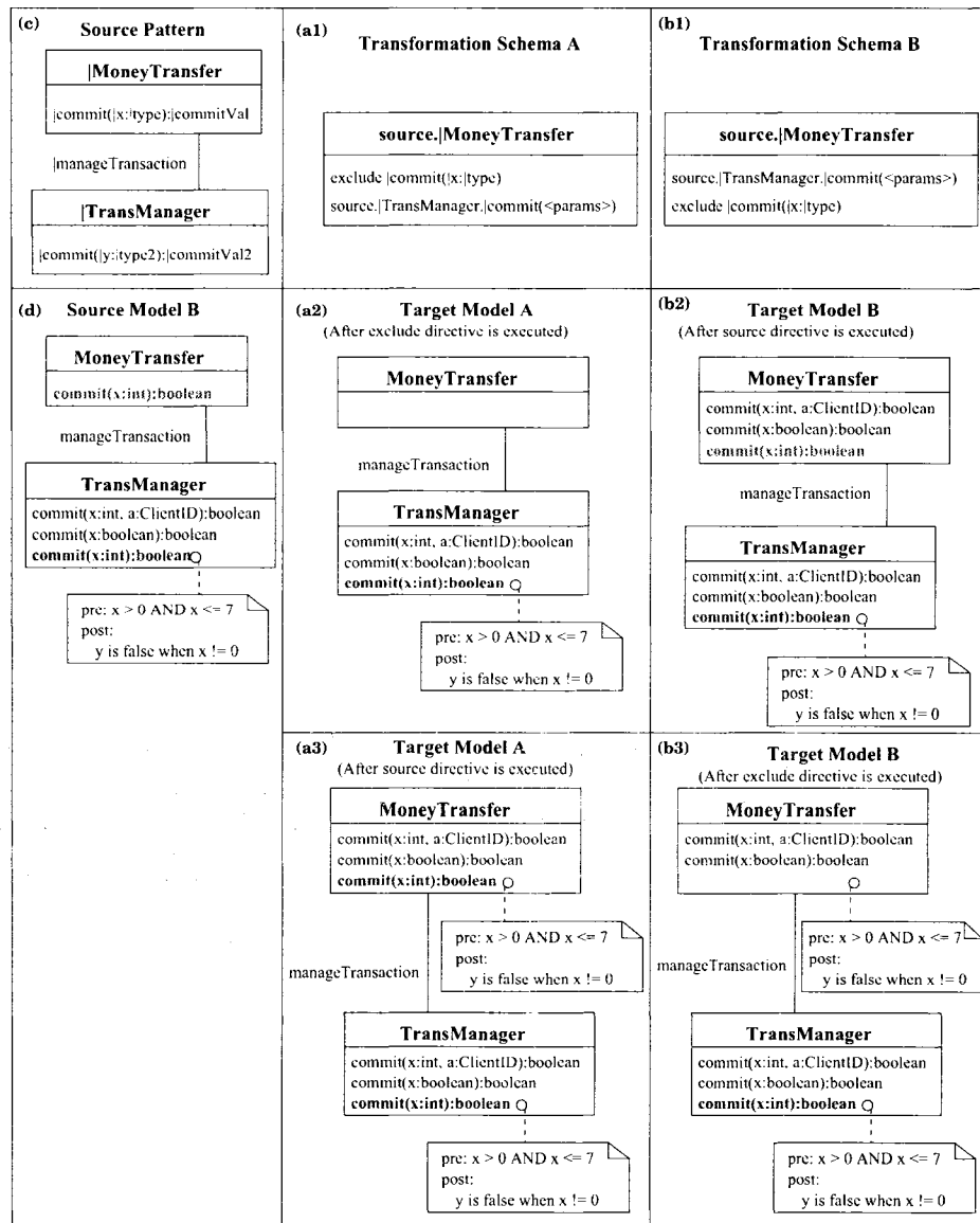
Figure 4.38: Ordering Transformation Directives - Example 3.
