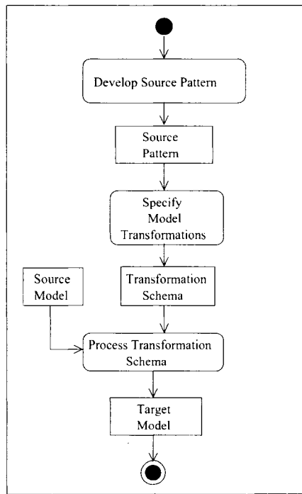
Figure 1.4: Model-to-model Transformation Process.
