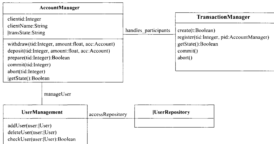
Figure 4.6: Target Model for Simple Transaction Service.
