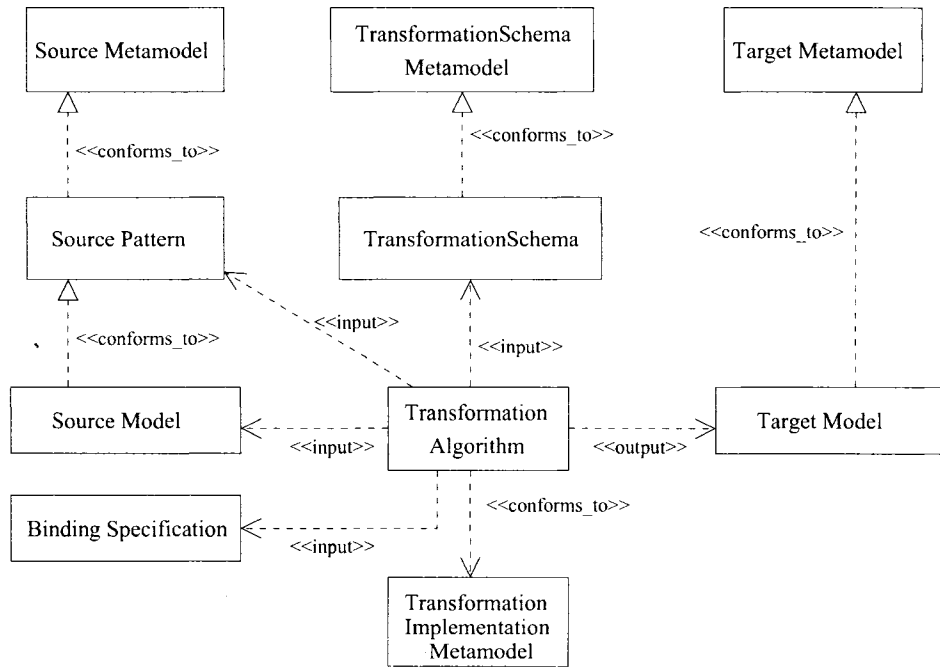
Figure 4.16: Model-to-model Transformation Conceptual Model.
