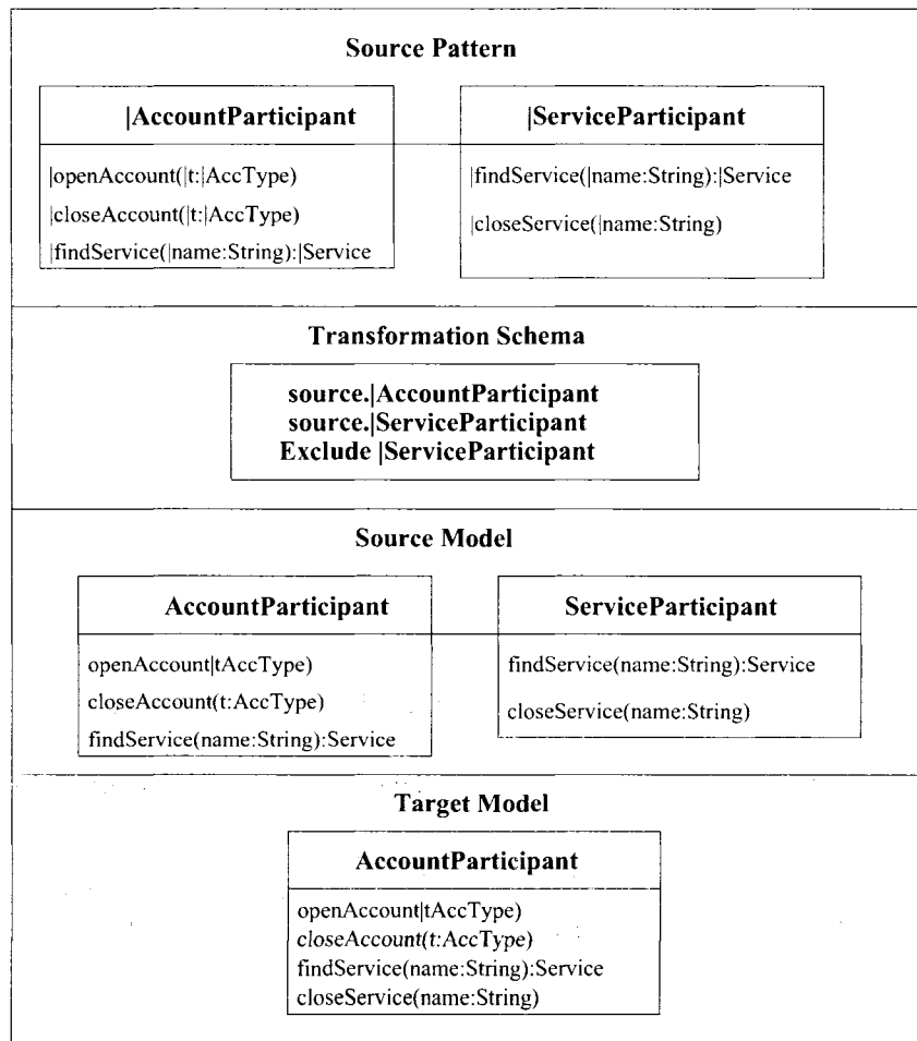
Figure 4.9: Merging Model Elements Using The source Directive.
