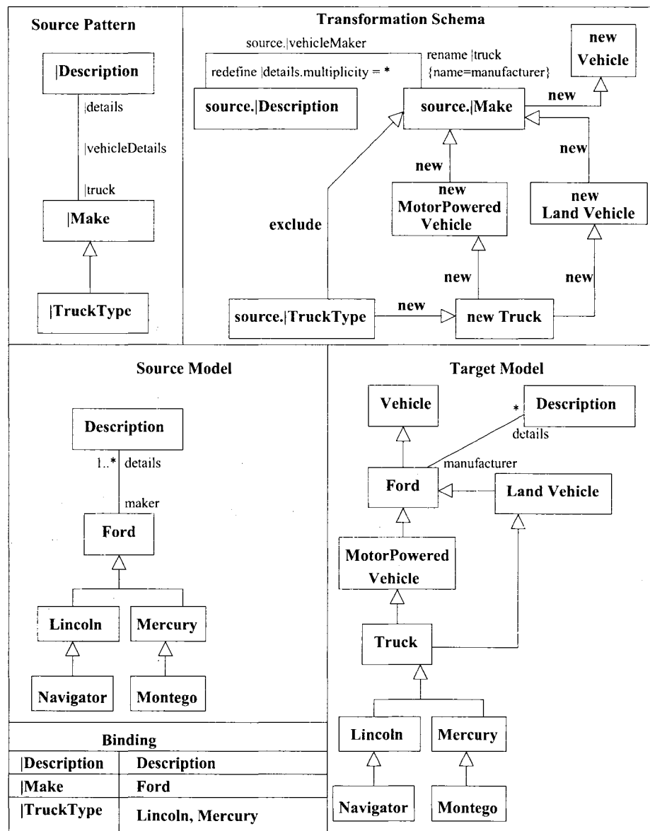
Figure 4.15: Applying Directives to UML Relationships.
