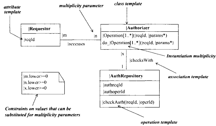
Figure 2.1: Example of A Class Diagram Template
