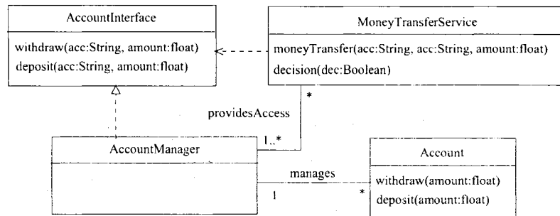
Figure 6.3: A Money Transfer Service Class Diagram.
