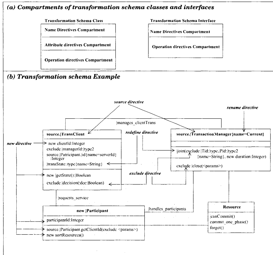
Figure 4.7: Transformation Schema Compartments.
