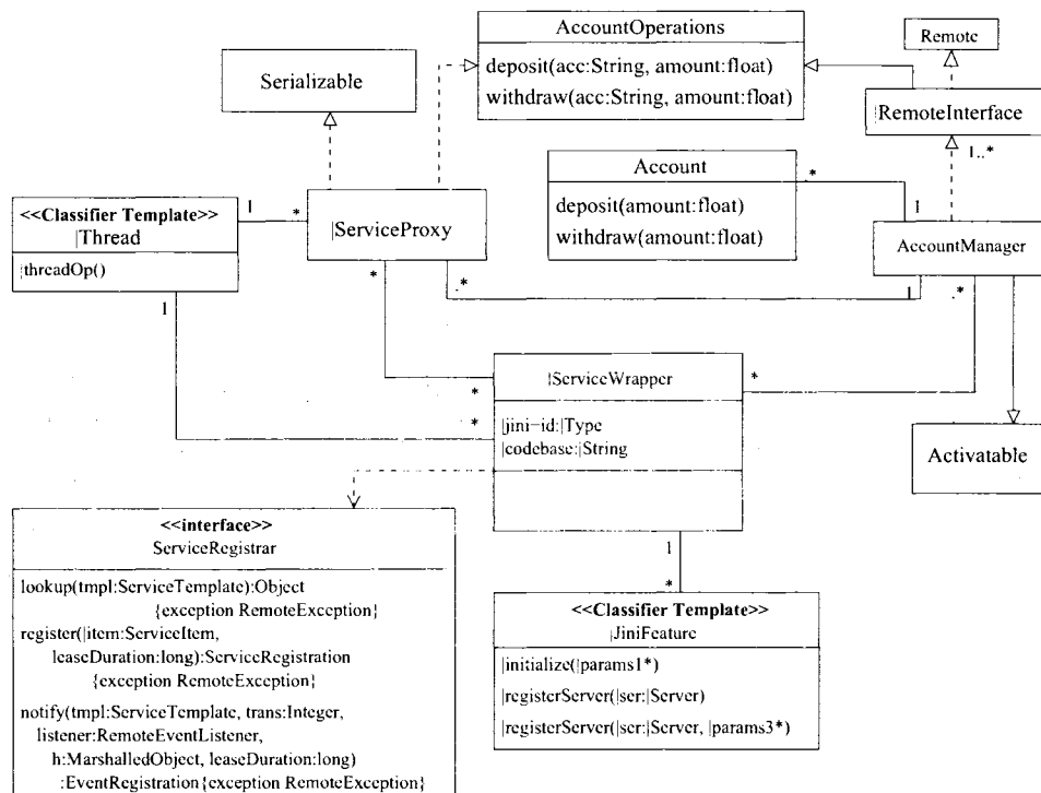
Figure 5.6: Jini Server Distribution Target Model.
