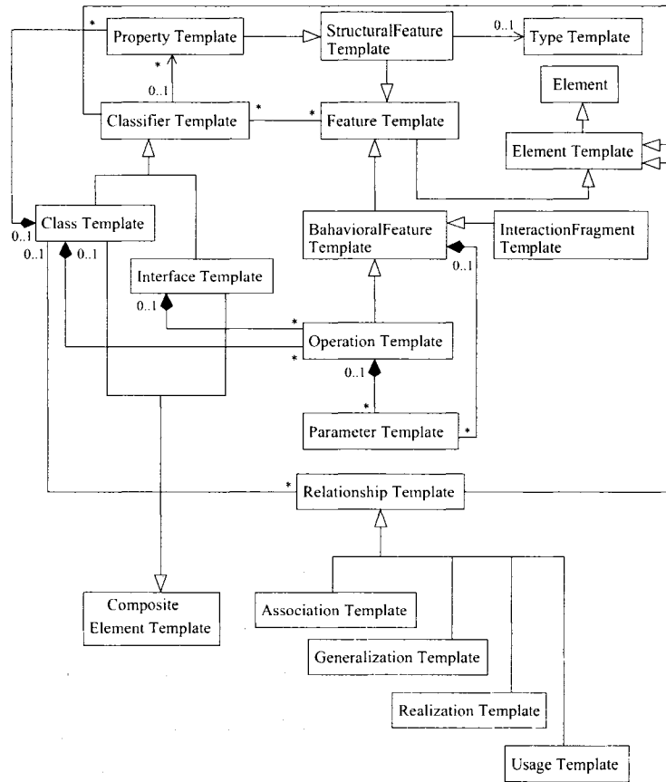
Figure 2.3: Class Template Metamodel.
