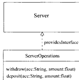
Figure 1.2: A Source Model.
