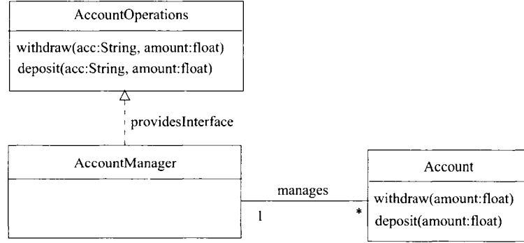
Figure 5.3: Source Model for Server Distribution.
