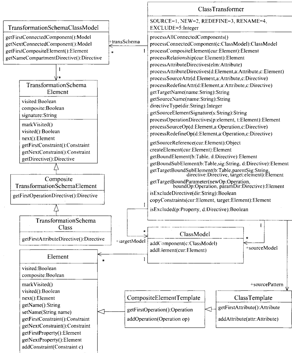
Figure 4.20: Transformation Implementation Metamodel Showing Behavioral Features.
