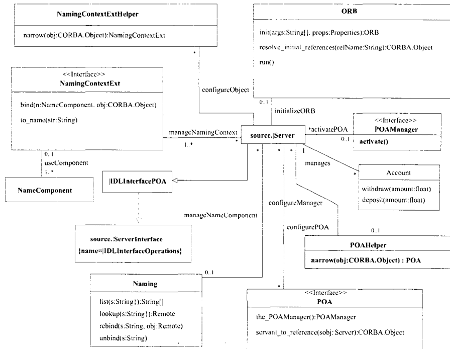
Figure 5.2: CORBA Class Transformation Schema.
