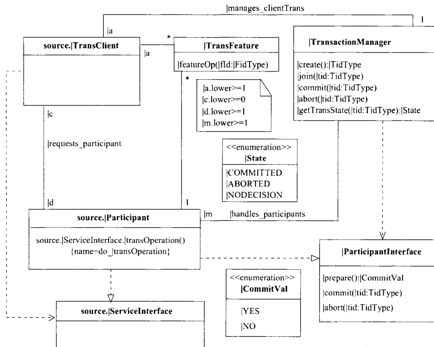
Figure 6.7: Target Pattern for Distributed Transactions.
