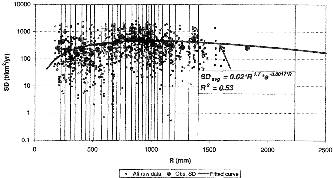
Figure 3.6: Weighted average SD as function of R
