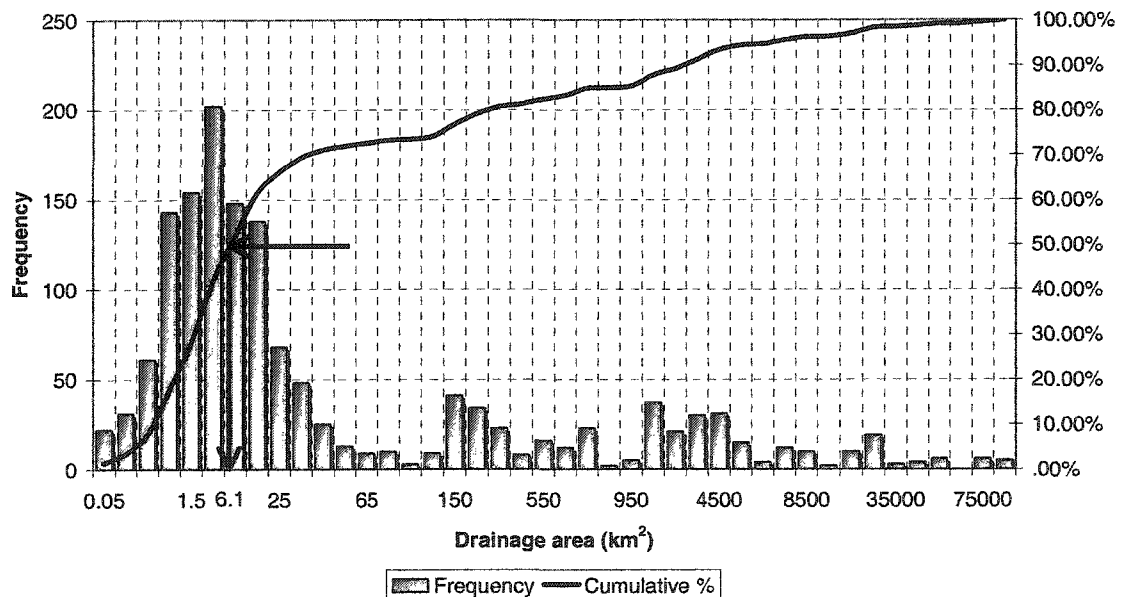
Figure 3.3: Distribution of A
