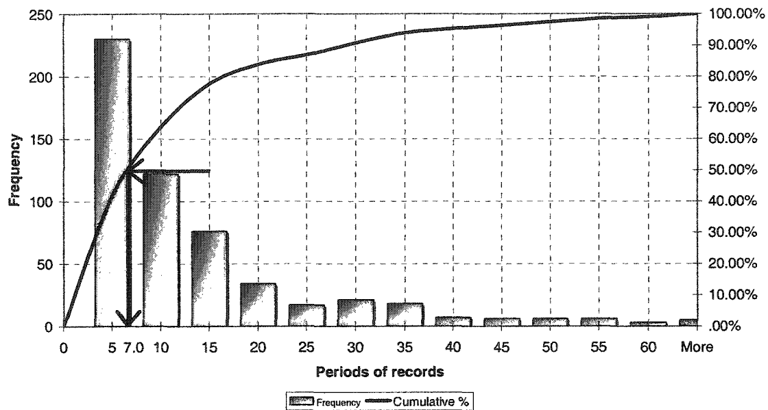
Figure 4.4: Distribution of the periods of records
