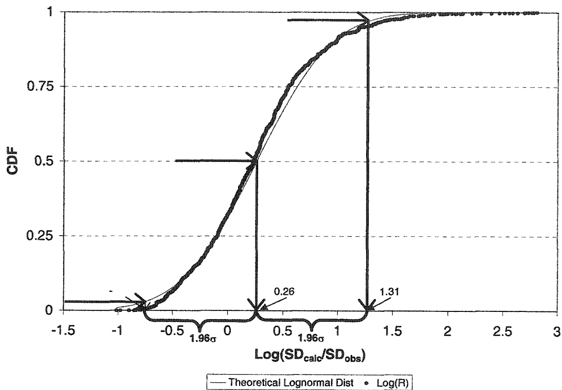
Figure 3.20: Distribution of the ratios of \text{Log}(SD_{calc}/SD_{obs}) using the equation with A
