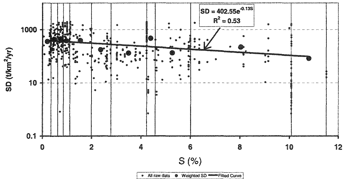
Figure 4.7: Weighted average SD as function of S
