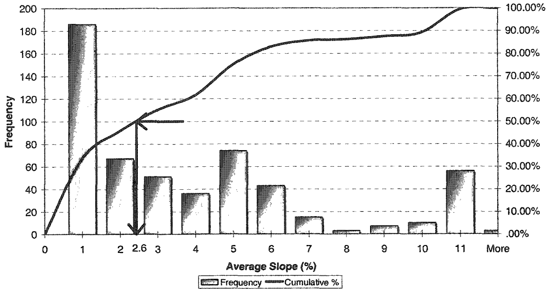
Figure 4.5: Distribution of the slopes
