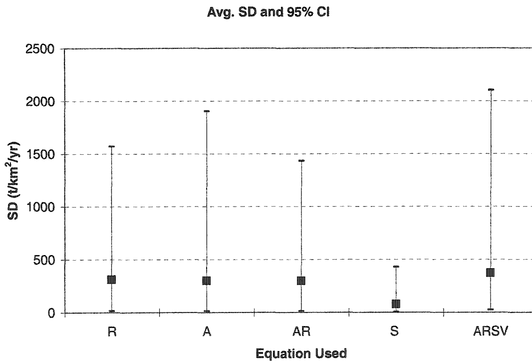
Figure 5.18: Average SD calculations and 95% confidence limits for California Gulch
