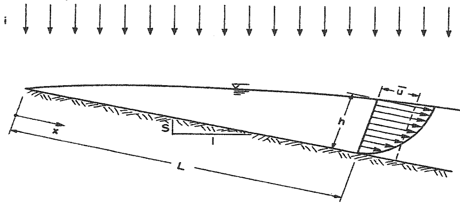
Fig. 2.1: Definition sketch of overland flow:
