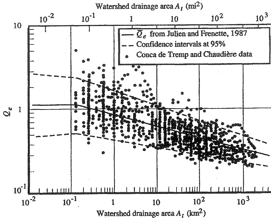
Fig. 2.4: Correction factor Q_e (after Julien and Frenette, 1986)
