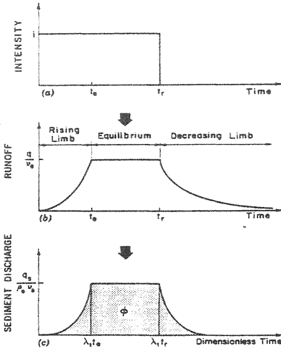
Figure 2.3: Soil erosion for a single event: a) hyetograph; b) hydrograph; c) sedimentograph
