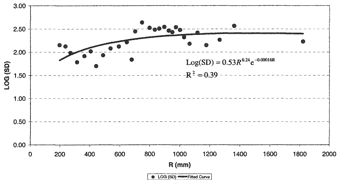
Figure 3.9: Log transformed SD with respect to R
