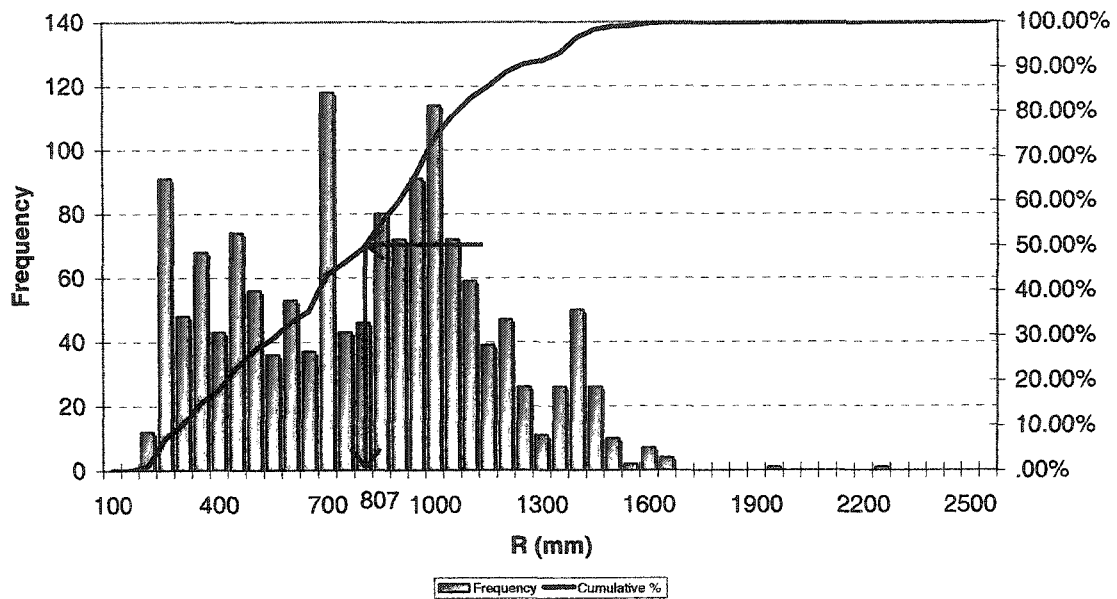
Figure 3.4: Distribution of R
