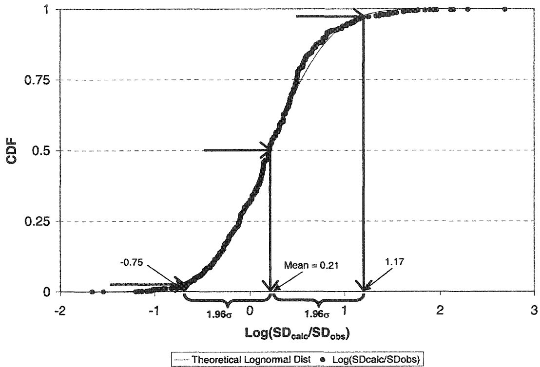
Figure 4.15: Distribution of ratio of \text{Log}(\text{SD}_{\text{calc}}/\text{SD}_{\text{obs}}) using Eq. 4.6
