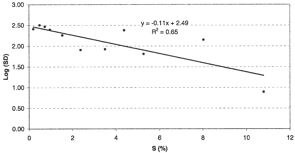
Figure 4.10: Log transformed SD with respect to S
