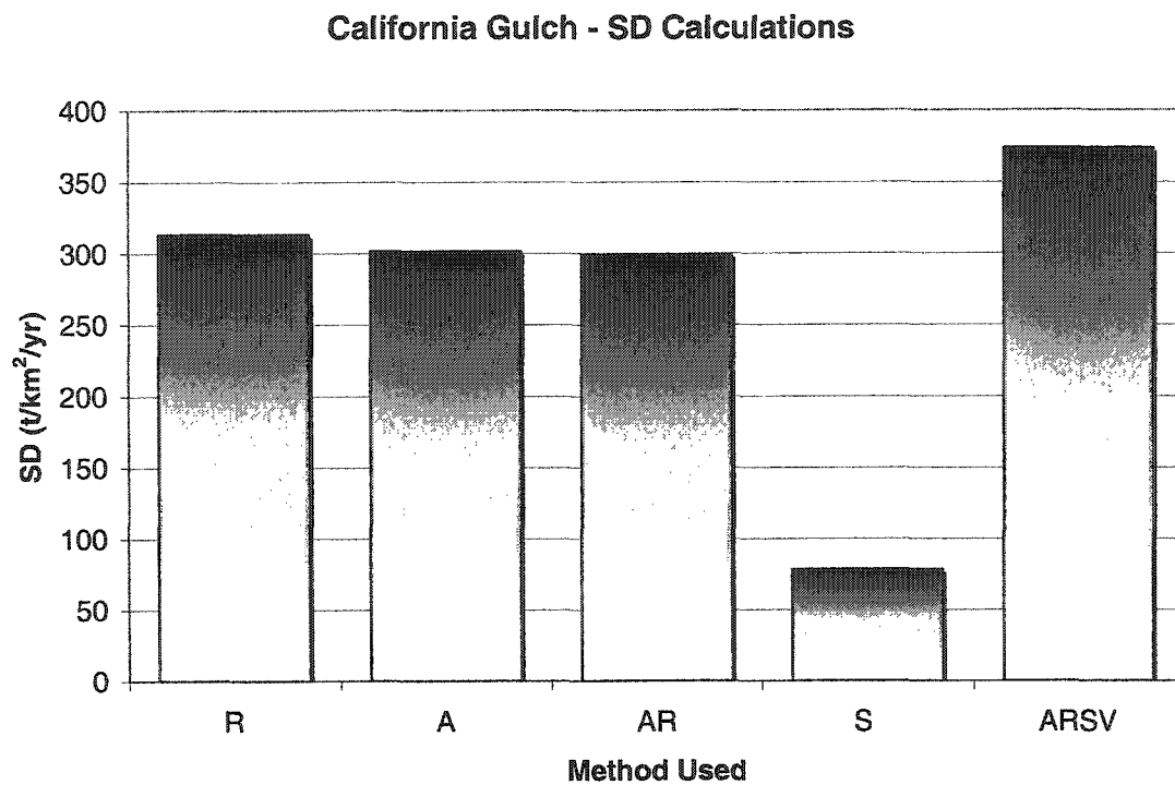
Figure 5.17: Average SD calculations for California Gulch
