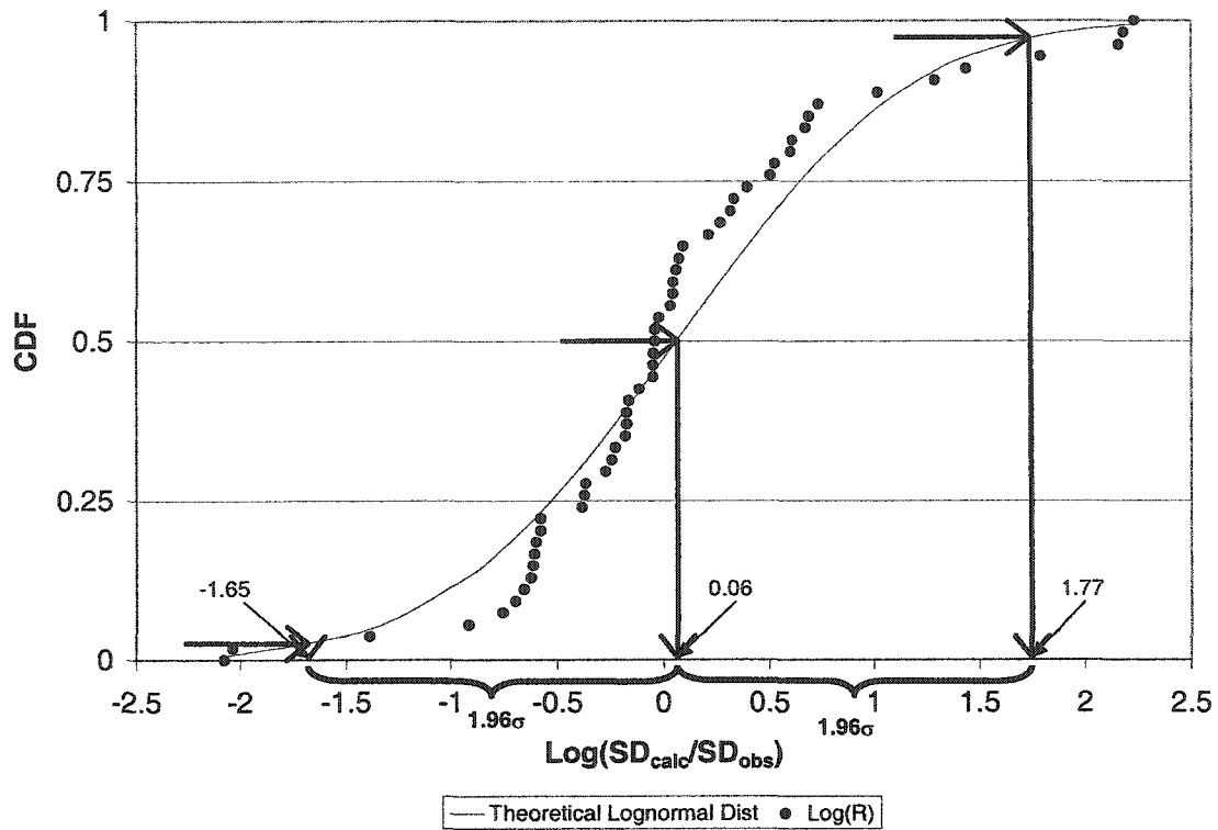
Figure 5.13: Distribution of \text{Log}(\text{SD}_{\text{calc}}/\text{SD}_{\text{obs}}) using the equation with A,R,S,V
