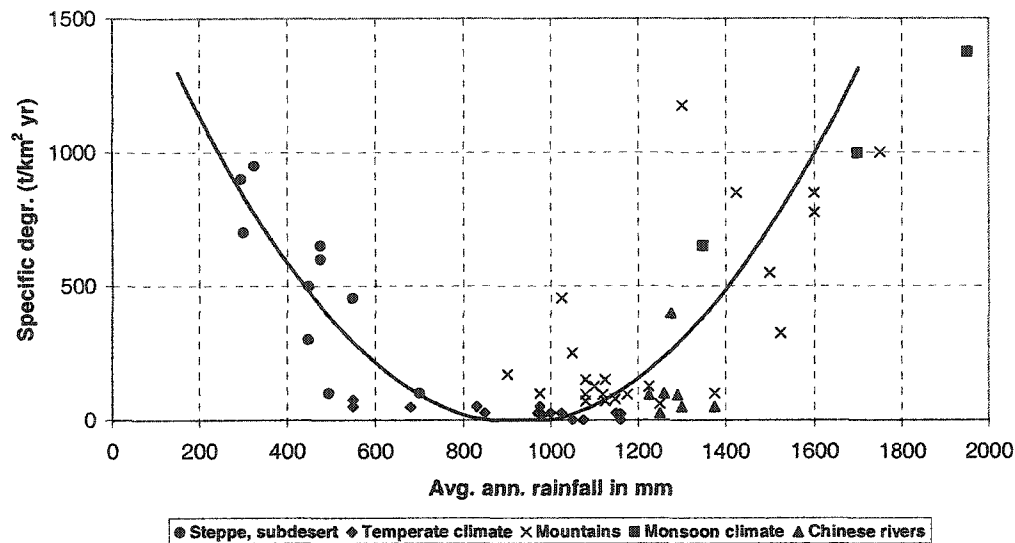
Figure 2.6: Mean SD vs. R (after Fournier, 1949)
