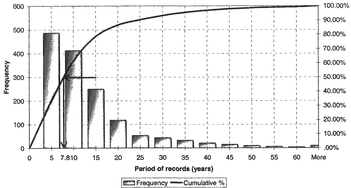
Figure 3.2: Distribution of the periods of records
