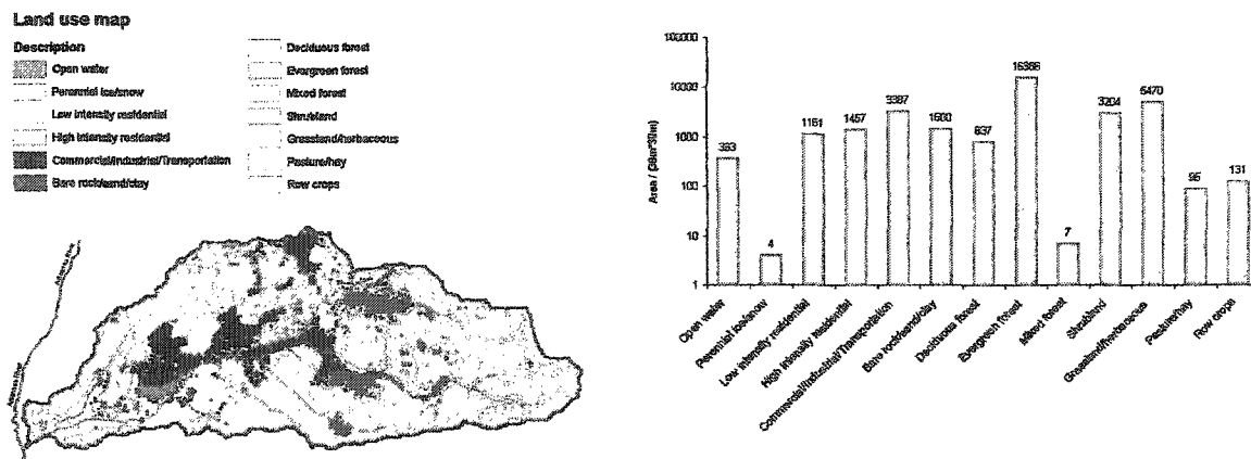
Figure 5.16: Land use/land cover data of the California Gulch
