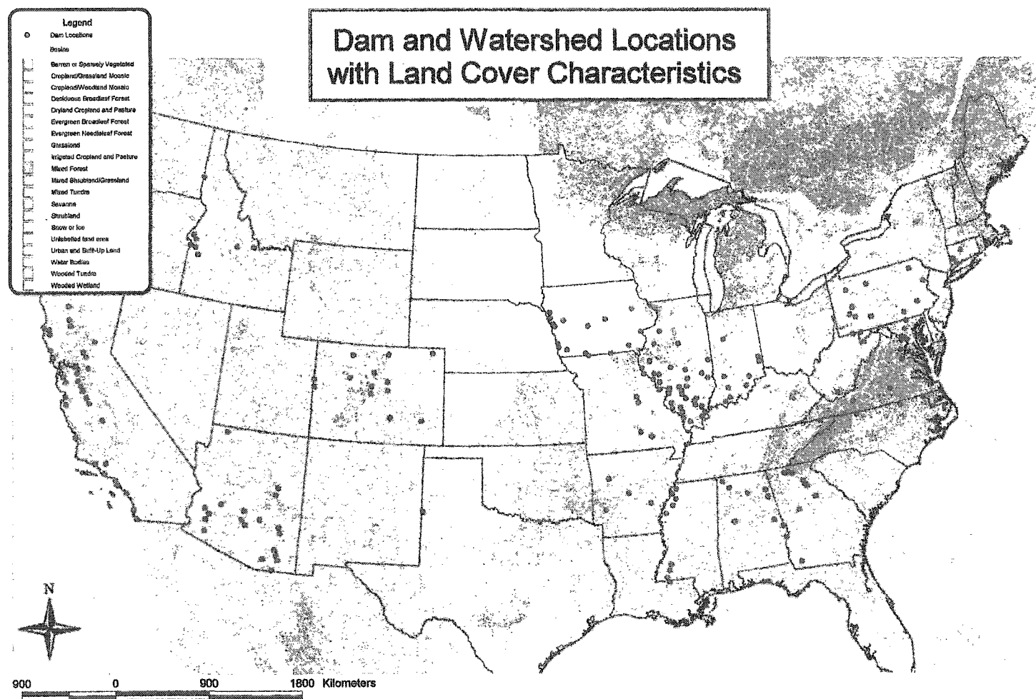
Fig. 4.2: Land cover characteristics of the basins
