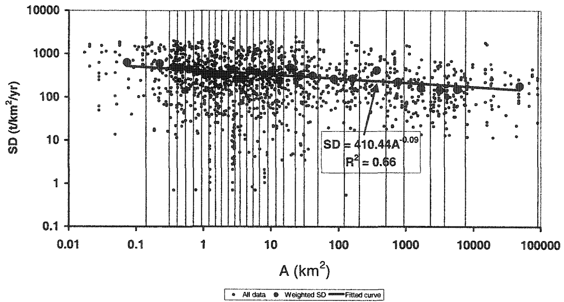
Figure 3.14: Weighted average SD as function of A
