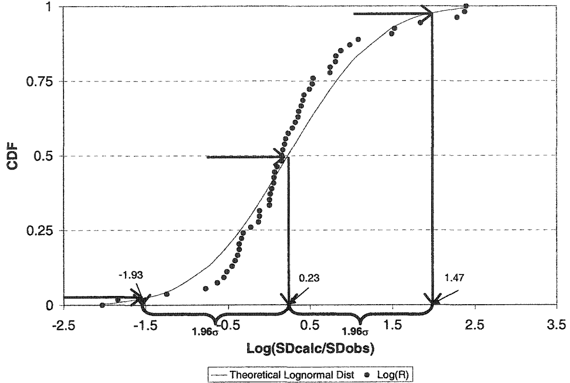
Figure 5.11: Distribution of \text{Log}(\text{SD}_{\text{calc}}/\text{SD}_{\text{obs}}) using the equation with R and A
