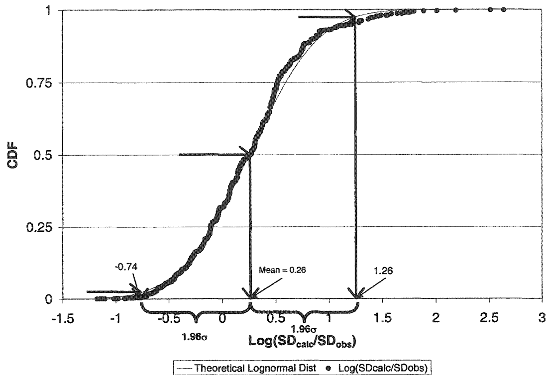
Figure 4.13: Distribution of \text{Log}(\text{SD}_{\text{calc}}/\text{SD}_{\text{obs}}) using the equation with S
