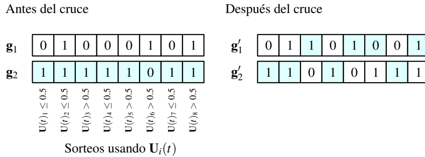
Figura 7.13: Crossover uniforme
