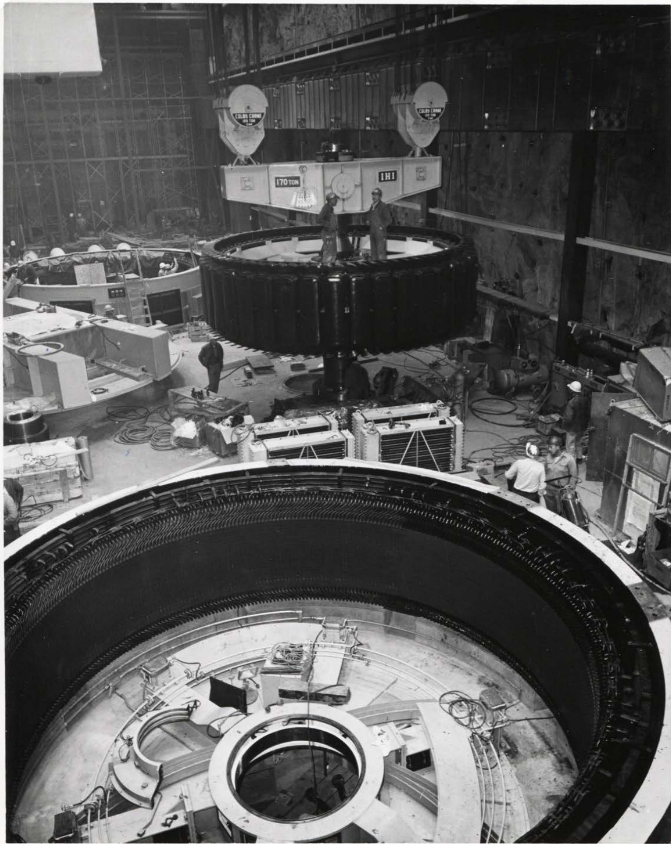
The 181 ton rotor for the first generating unit is being lifted from the rotor erection pedestal and will be placed in the stator in the foreground. April 14, 1970 Bureau of Reclamation Photo by V. Jetley.
