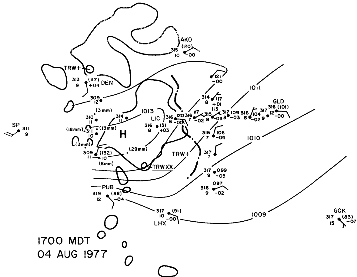
Figure 66. Similar to Fig. 64, for 1700 MDT, 04 August 1977. Bold dashed line is edge of Goodland radar echo.
