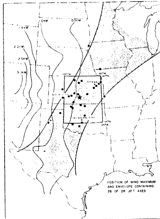
Figure 12. Location of core of the horizontal low-level jet, for 28 selected cases. The star represents the median location of all the jet cores. The envelope contains 26 of the 28 jet axes. Terrain contours in km are included. From Bonner (1968).
