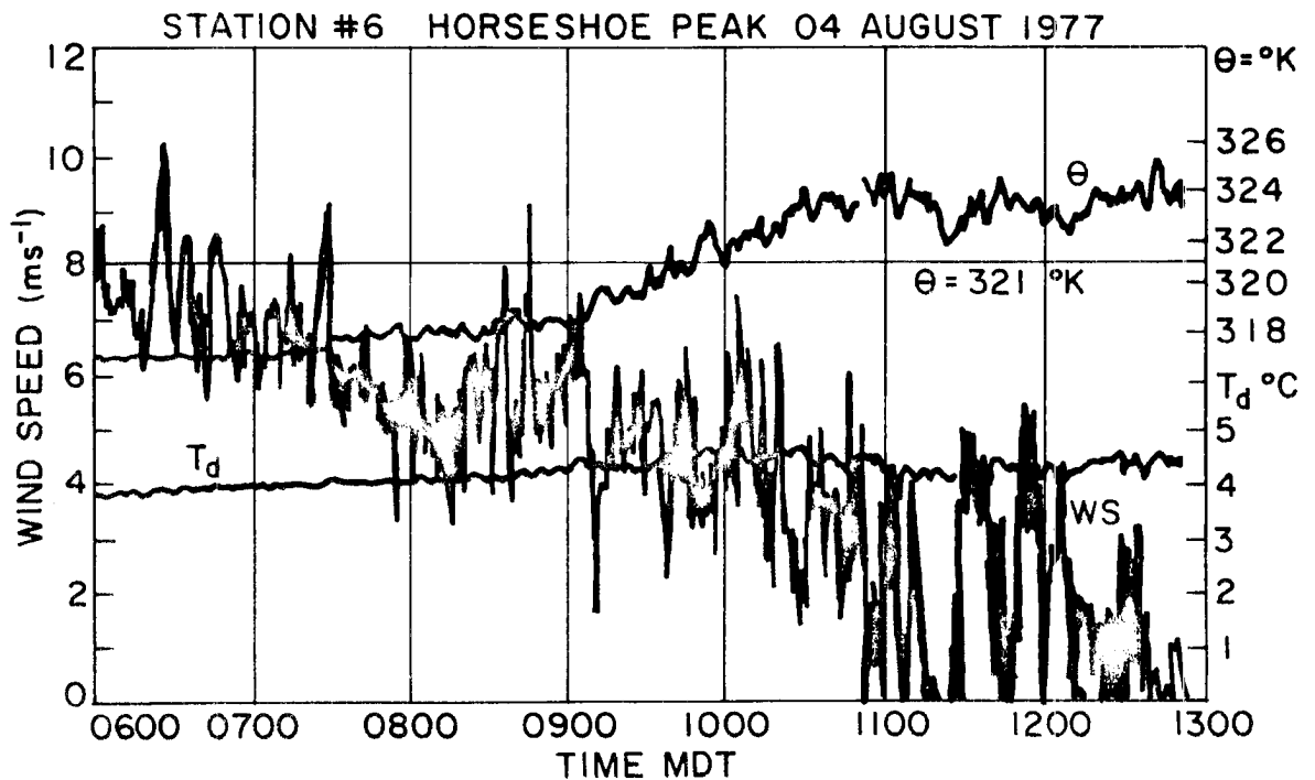
Figure 54. Temperature, dew-point, and wind speed plotted vs. time at PAM station #6 (Horseshoe Peak), for 0600-1300 MDT, 04 August 1977.
