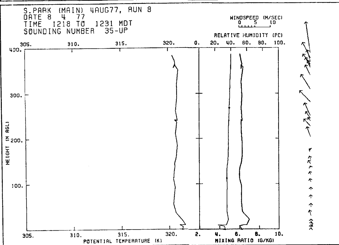
Figure 53. Same as Fig. 47, for a) 1054 MDT, and b) 1218 MDT, taken at Site #1 (CSU base).
