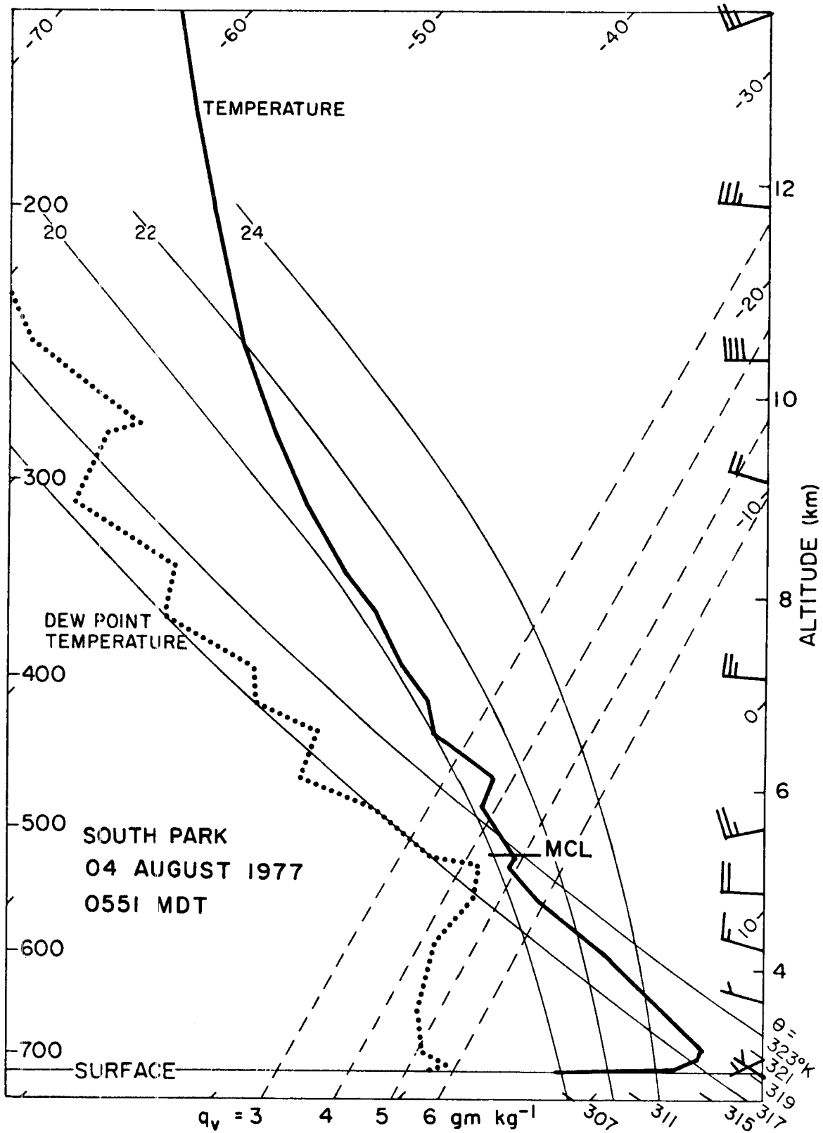
Figure 45. South Park sounding of 0551 MDT, 04 August 1977, plotted on skew-T log-P diagram.
