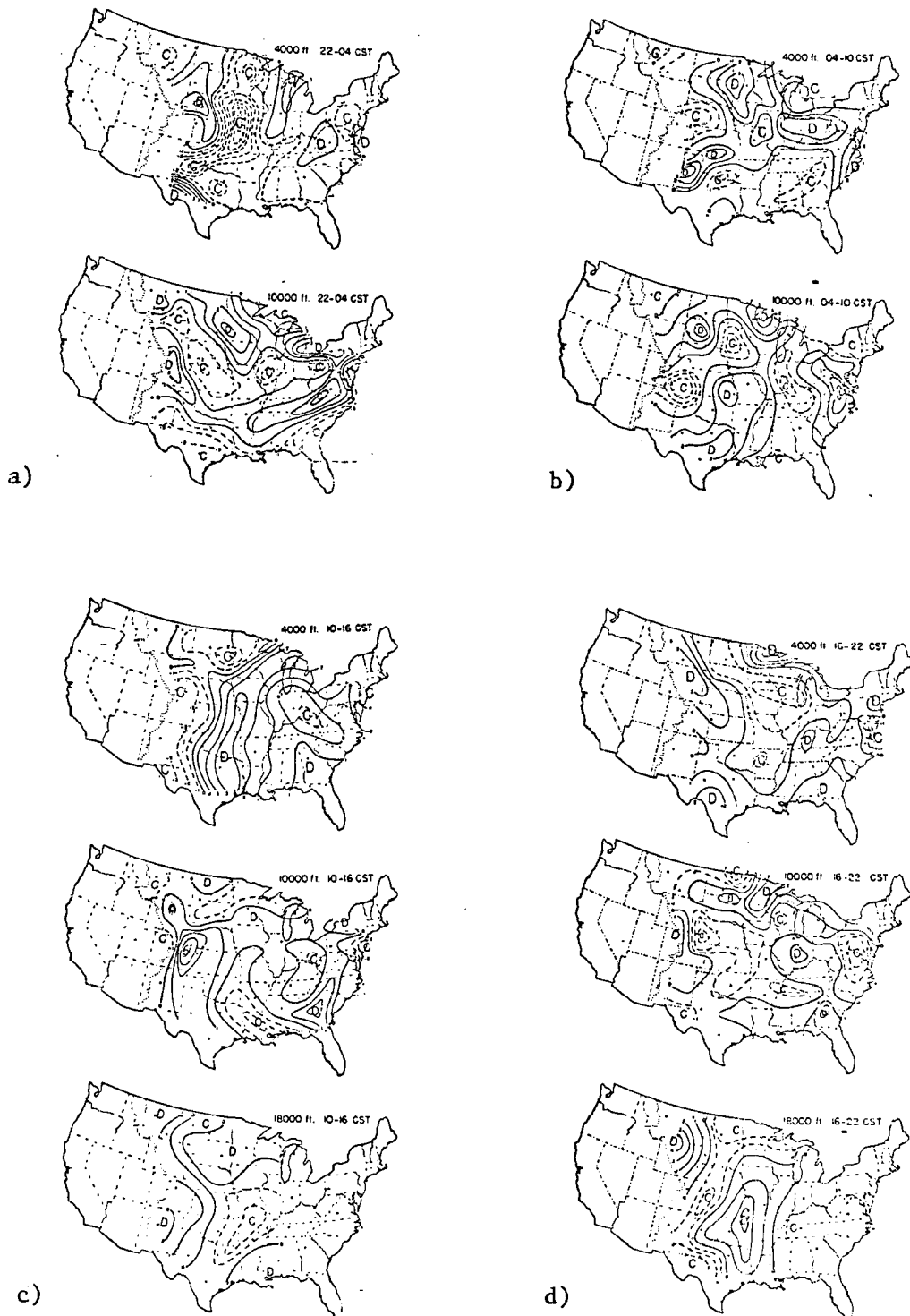
Figure 9. Change in divergence between two successive sets of balloon wind observations, for all days in August 1947 and August 1948. a) 2200-0400 CST (Central Standard Time; same as MDT, or Mountain Daylight Time) or nighttime. b) 0400-1000 CST, early morning. c) 1000-1600 CST, midday. D) 1600-2200 CST, evening. Levels are 1.2 km (4000 ft.), 3.0km (10,000 ft.) and 5.5km (18,000 ft.). From Bleeker and Andre (1951).
