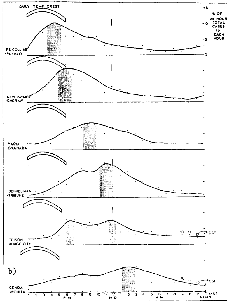
Figure 6. a) Six groups of stations with north-south orientations used in the timing analysis of convective shower activity. b) Timing of major convective activity for ten-year summary of hourly precipitation \geq .10 inch for the six groups of stations (from Crow, 1969).
