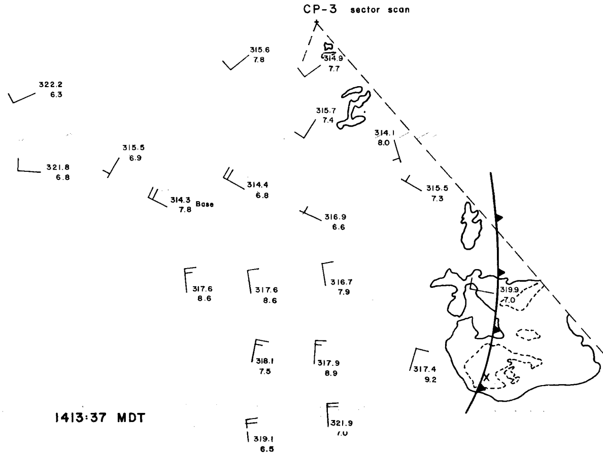
Figure 63. Same as Fig. 60, for 1413 MDT.
