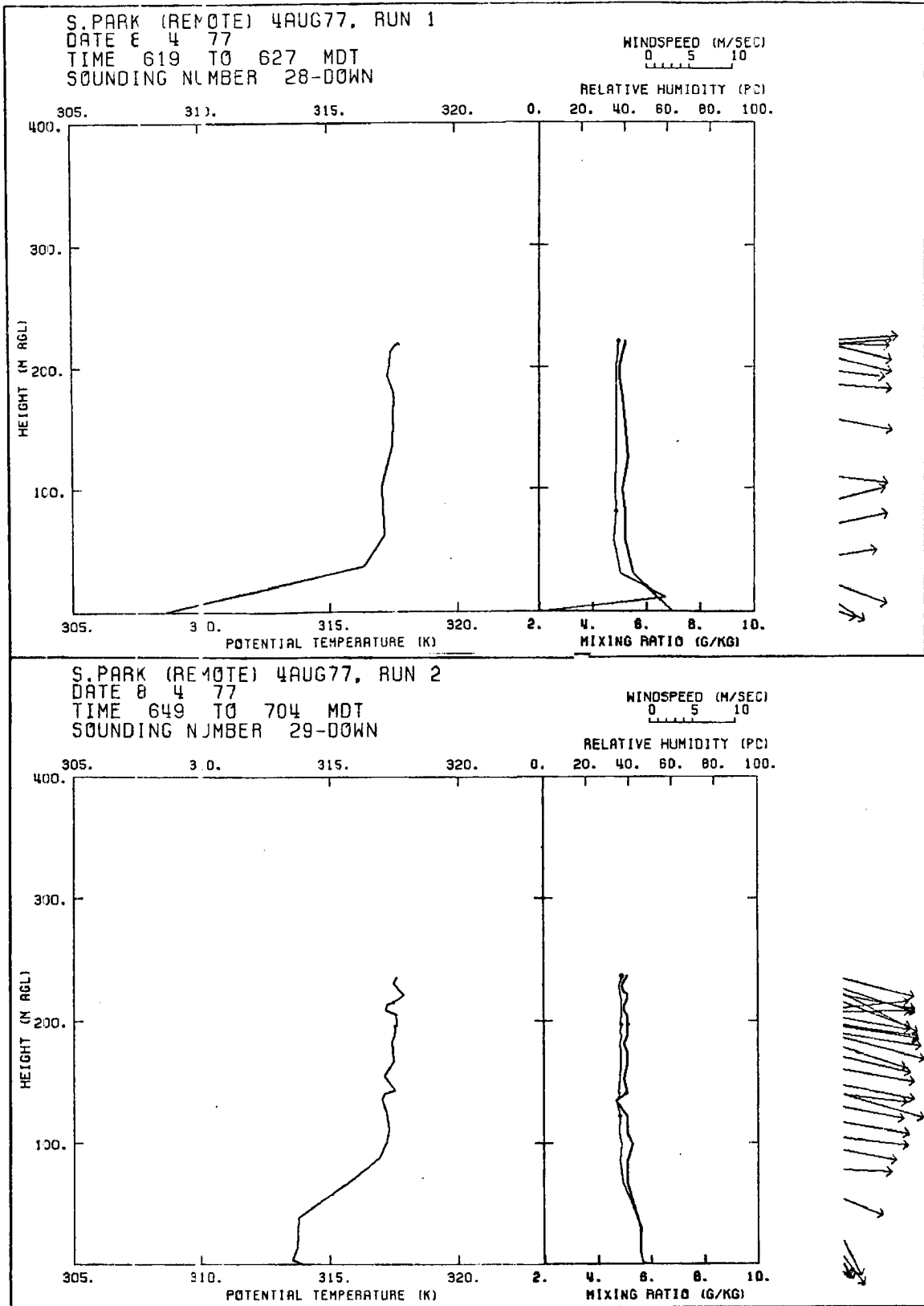
Figure 4'. Boundary Layer Profiler (BLP) tethered balloon soundings. Potential temperature, water vapor mixing ratio, and winds plotted against height in meters AGL. Soundings begun at a) 0619 MDT, and b) 0649 MDT, (04 August 1977, both at Site #2.
