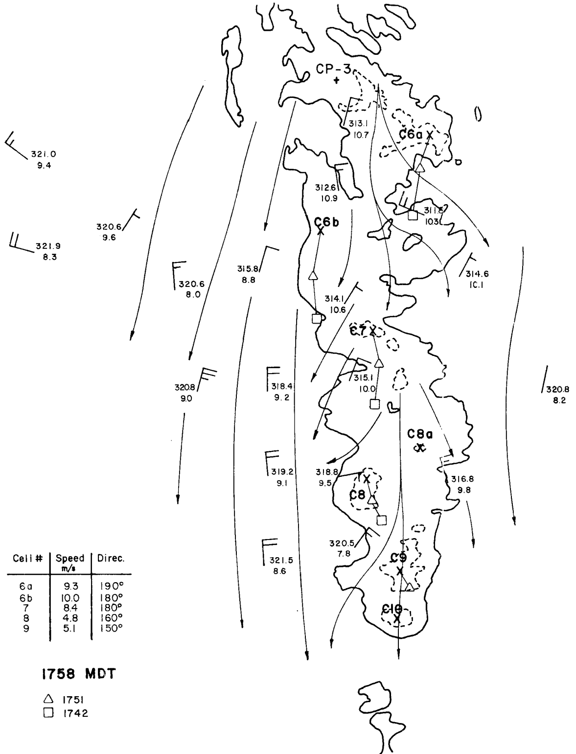
Figure 34. Same as Fig. 24, for 1758 MDT.
