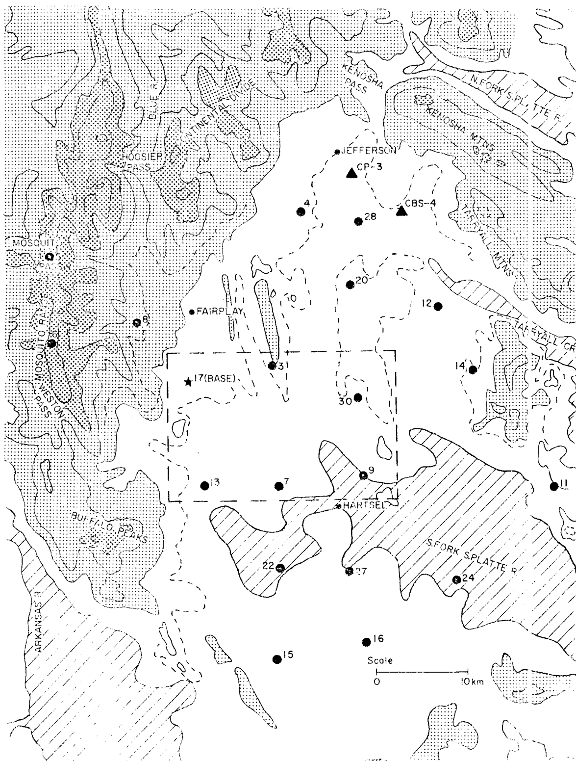
Figure 1. Map of terrain in South Park, Colorado. Regions below 9000 ft. (2744m) are hatched; regions above 10,000 ft. (3049m) are lightly shaded, and regions above 12,000 ft. (3659m) are heavily shaded. PAM remote stations are indicated with dark circles accompanied by the station number, with a star for the base site. CP-3 and CBS-4 radars are indicated with dark triangles.
