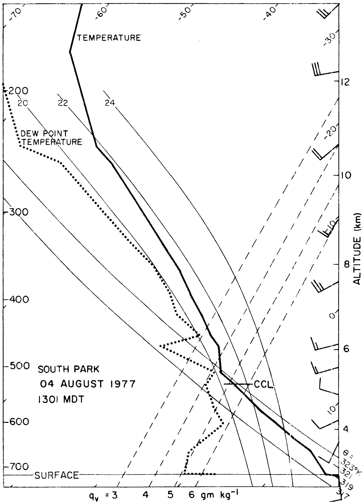
Figure 55. South Park sounding of 1301 MDT, 04 August 1977, plotted on skew-T log-P diagram. Cloud Condensation Level (CCL) marked.
