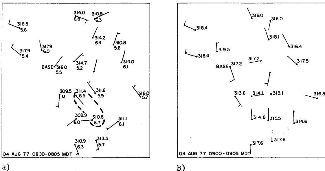
Figure 49. Same as Fig. 46, for a) 0800 MDT, and b) 0900 MDT, 04 August 1977 (water vapor mixing ratio data missing for 0900 MDT). Dashed line encloses region with mixing ratio >6.5 \text{ gm kg}^{-1} .
