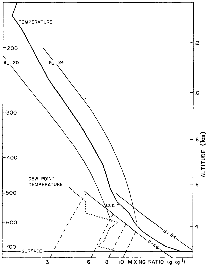
Figure 19. South Park sounding of 1000 MDT, 19 July, 1977, plotted on skew-T log-P diagram.
