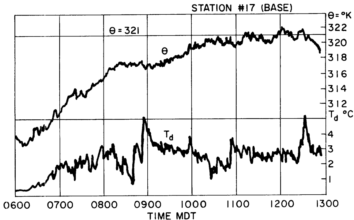
Figure 50. Plot of potential temperature and dew-point vs. time, at the CSU base, 0600-1300 MDT, 04 August 1977.
