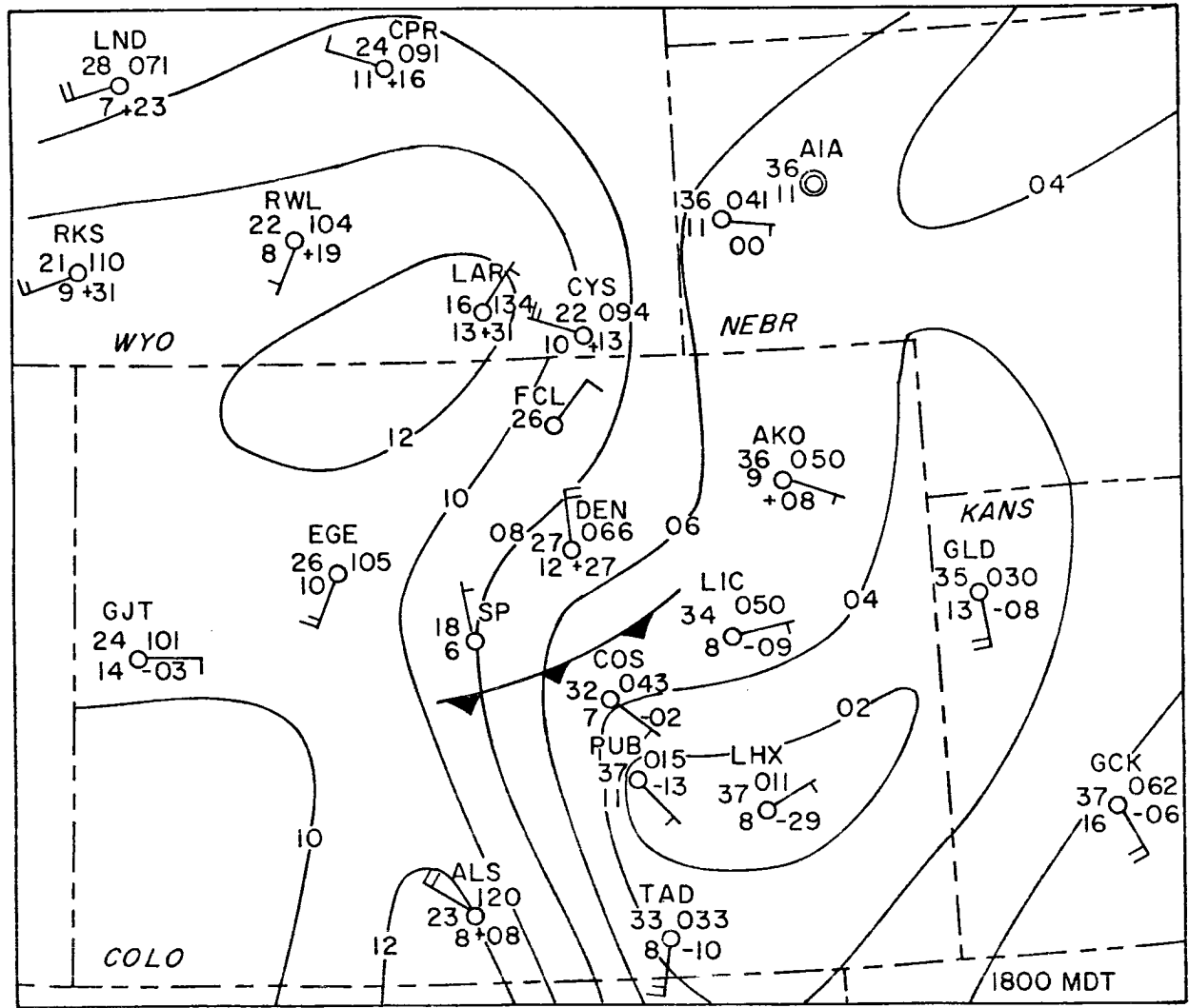
Figure 32. Mesoscale surface map, like Fig. 14, for 1800 MDT, 19 July, 1977.
