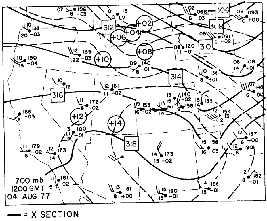
Figure 41. Upper air analyses as in Fig. 13, for a) 500 mb and b) 700 mb levels, 0600 MDT, 04 August, 1977.
