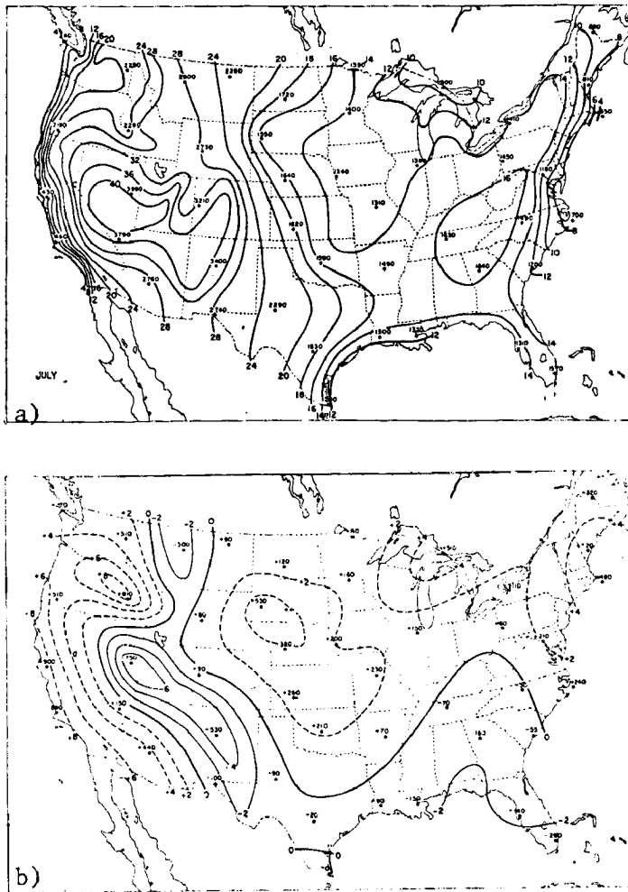
Figure 8. a) The mean maximum mixing depth (m) for July, from 10 years sounding data over the contiguous United States. b) Differences, in meters, between mean lifted condensation level and mean maximum mixing depth for July. A positive value (dashed contours) indicates that the condensation level is higher than the mixing depth. From Holzworth (1964).
