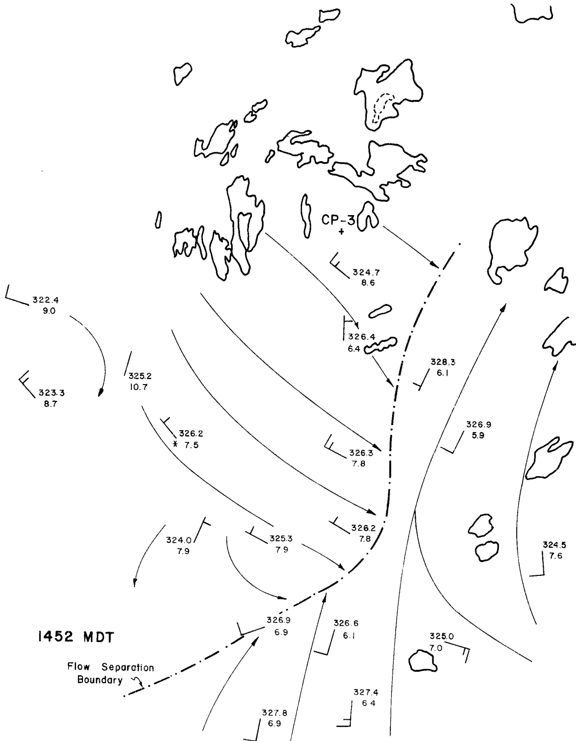
Figure 23. Same as Fig. 21, for 1452 MDT.
