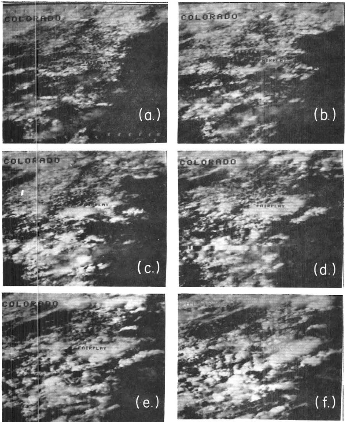
Figure 58. Visible satellite images, processed by video imaging techniques showing eastern 2/3 of Colorado and part of New Mexico. State borders in Fig. a) Town of Fairplay, about 10 km north of CSU base, is labeled. The town is located at the lower left corner of the label. The dark surface feature, lower right of each figure, is the Arkansas River east of Pueblo. The Palmer Lake Divide is marked by clouds, just north of the Arkansas River, especially in Fig. 58b. Picture times are a) 1200 MDT, b) 1245 MDT, c) 1315 MDT, d) 1345 MDT, e) 1415 MDT, and f) 1442 MDT.
