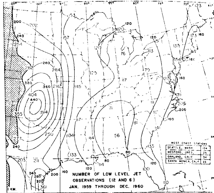
Figure 11. Number of low-level wind maxima, here defined as a wind speed of over 12 \text{ ms}^{-1} occurring below 1.5 km AGL, with a decrease of wind speed above the maximum of 6 \text{ ms}^{-1} or more, during two complete years, for soundings at 0600 MDT and 1800 MDT. (A total of 1462 soundings at each station). From Bonner (1968).
