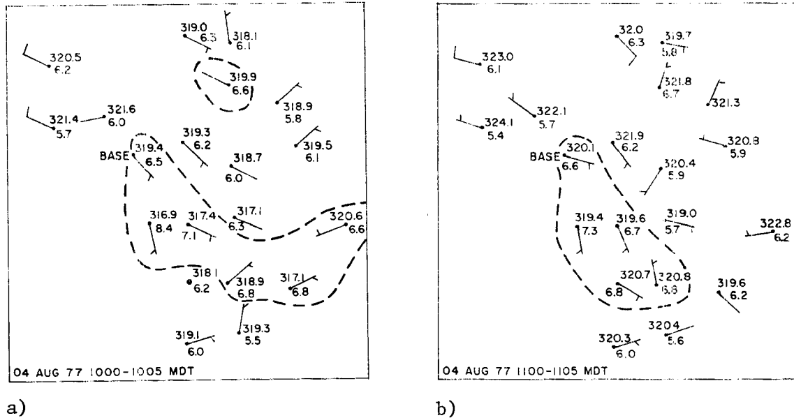
Figure 51. Same as Fig. 46, for a) 1000 MDT, and b) 1100 MDT, 04 August 1977.
