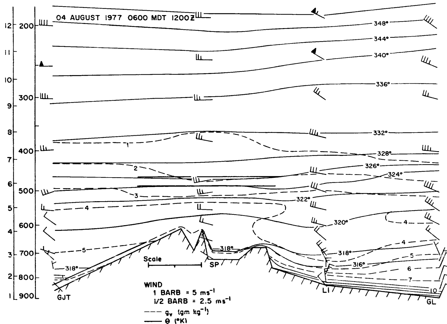
Figure 44. East-west cross-section, as in Fig. 21, for 0600 MDT, 04 August 1977.
