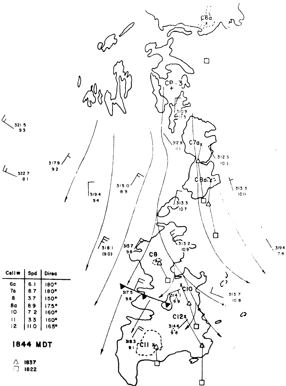
Figure 36. Same as Fig. 24, for 1844 MDT.
