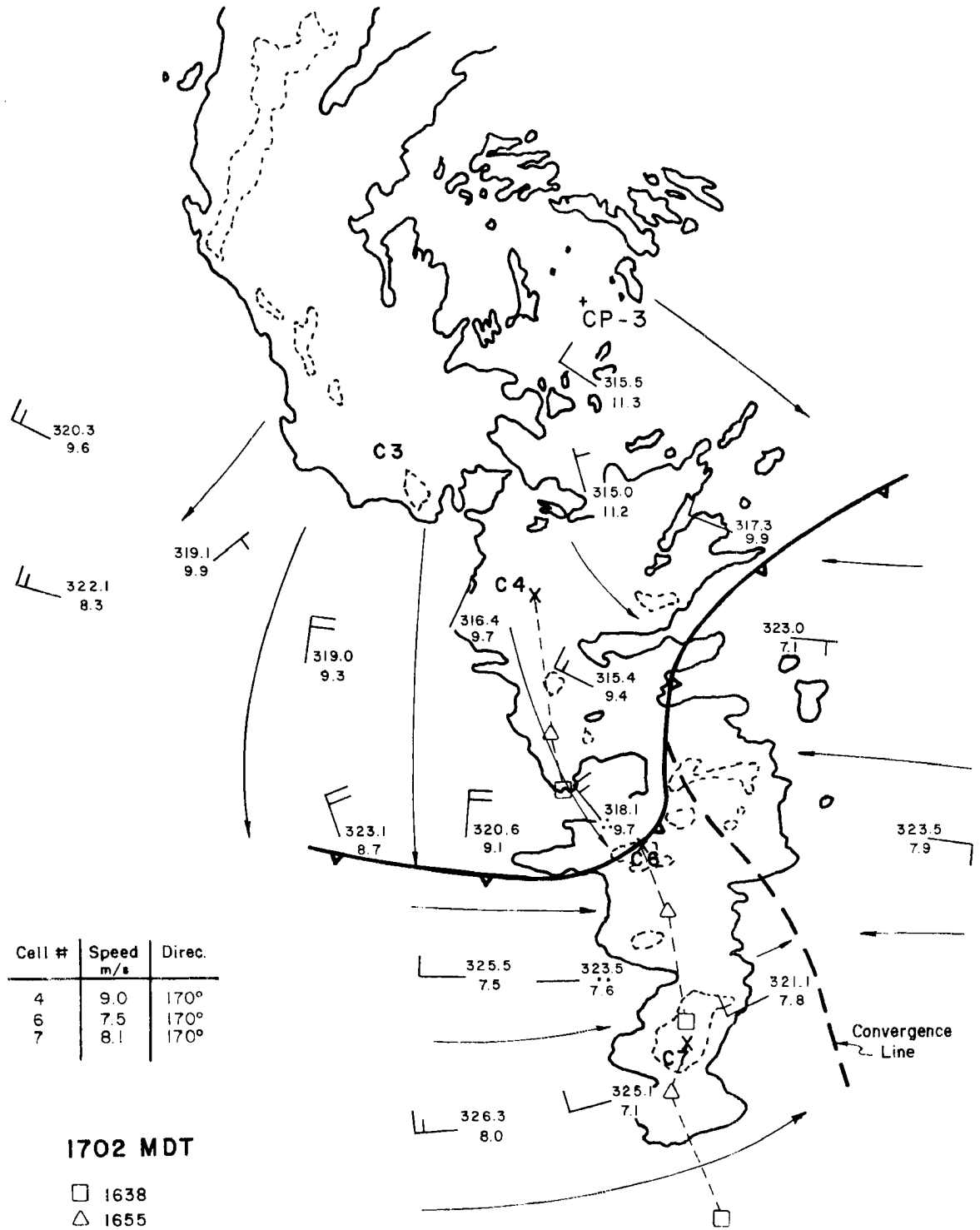
Figure 26. Same as Fig. 24, for 1702 MDT.
