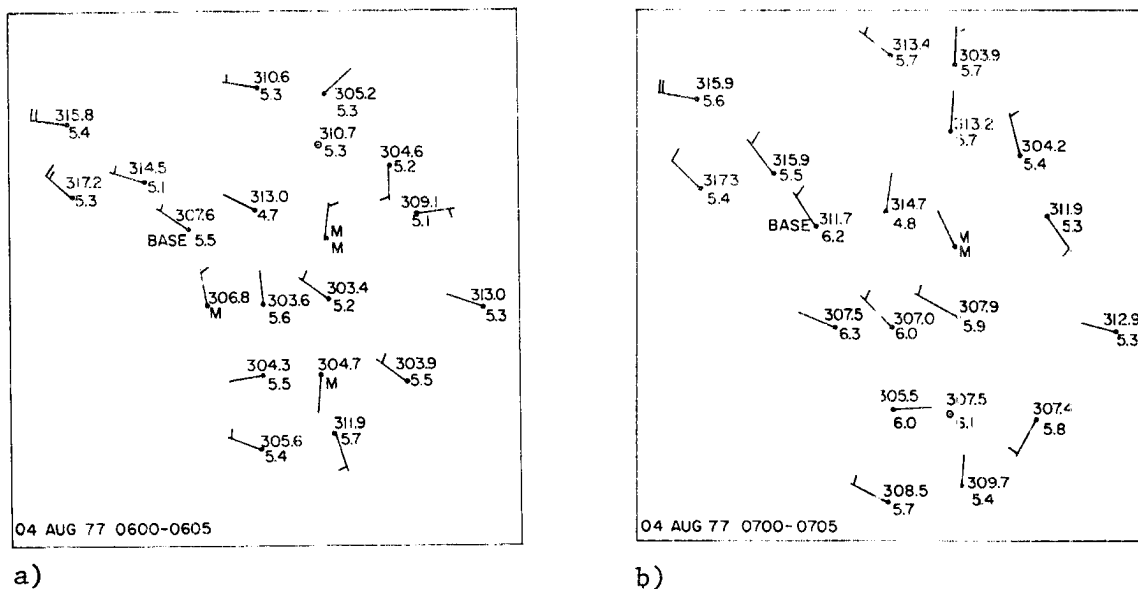
Figure 46. PAM surface data from South Park, as in Fig. 18, for a) 0600 MDT and b) 0700 MDT, 04 August 1977.
