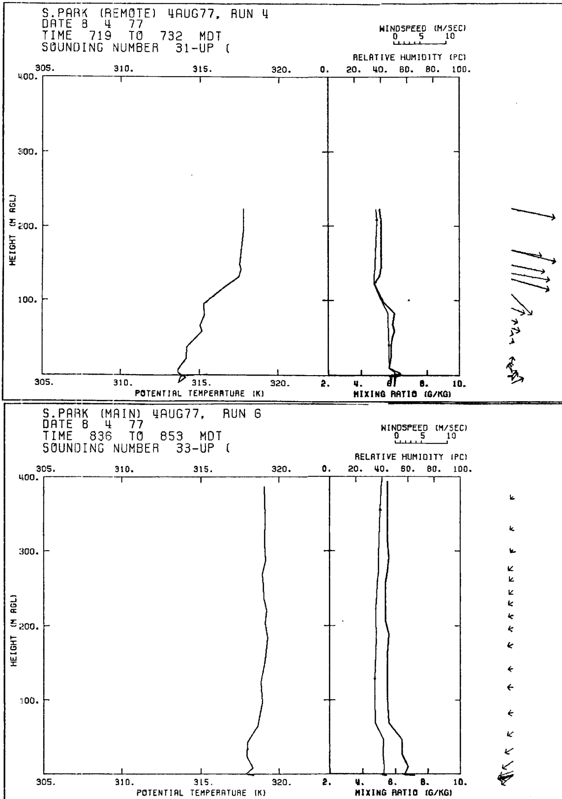
Figure 48. Same as Fig. 47, for a) 0720 MDT, Site #2, and b) 0836 MDT, Site #1 (CSU base site).
