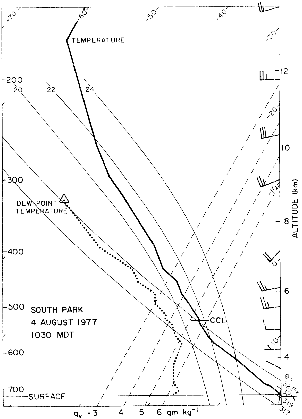
Figure 52. South Park sounding of 1030 MDT, 04 August 1977, plotted on skew-T log-P diagram.
