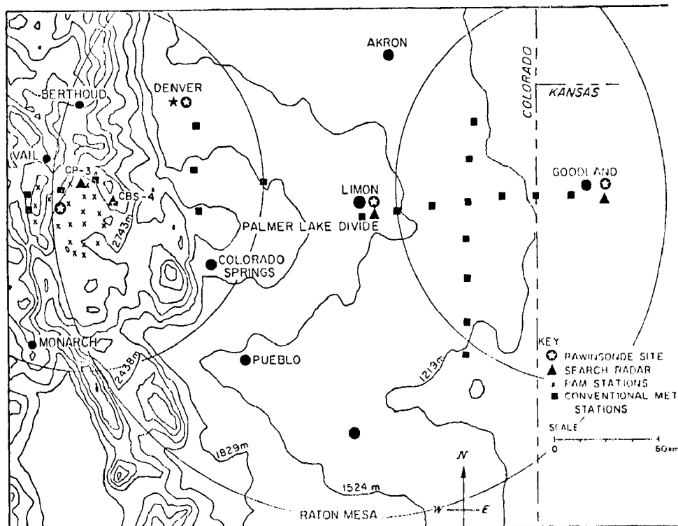
Figure 2. Map of extended SPACE/HIPLEX experimental area, with averaged terrain contours every 304.8m (1000 feet). The large circles represent radar effective coverage areas.
