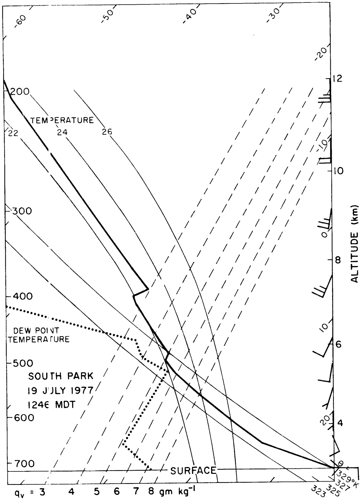
Figure 20. South Park sounding of 1240 MDT, 19 July 1977, plotted on skew-T log-P diagram.
