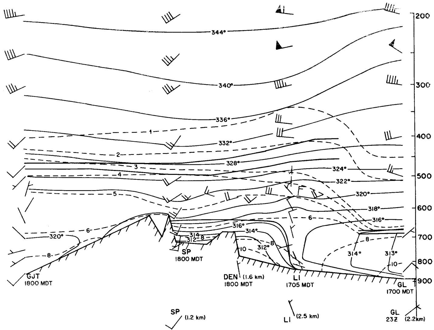
Figure 68. Same as Fig. 56, for 1700-1800 MDT, 04 August 1977. Aircraft flew east to west.
