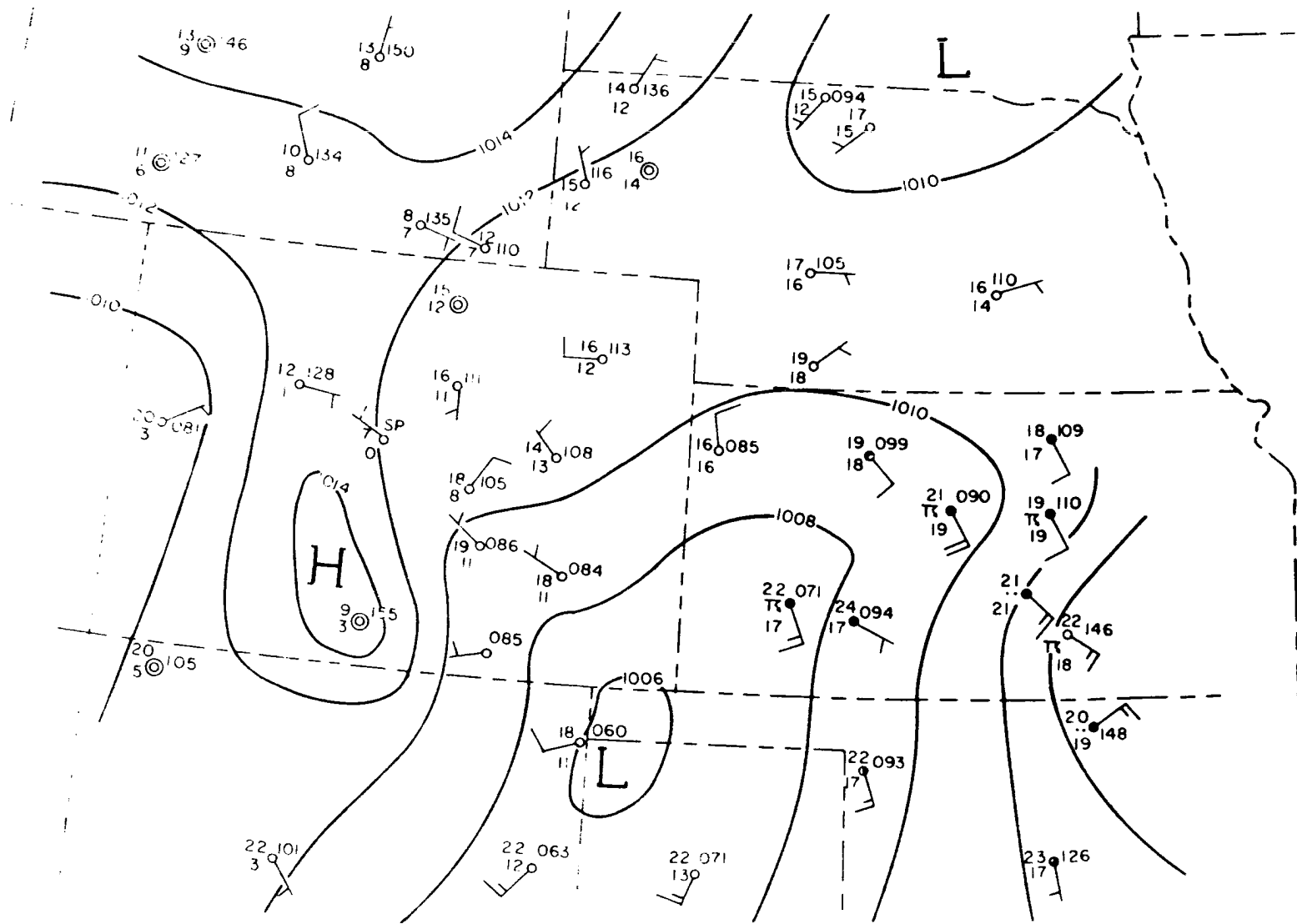
Figure 42. Extended area surface analysis, similar to Fig. 14, for 0600 MDT, 04 August 1977.
