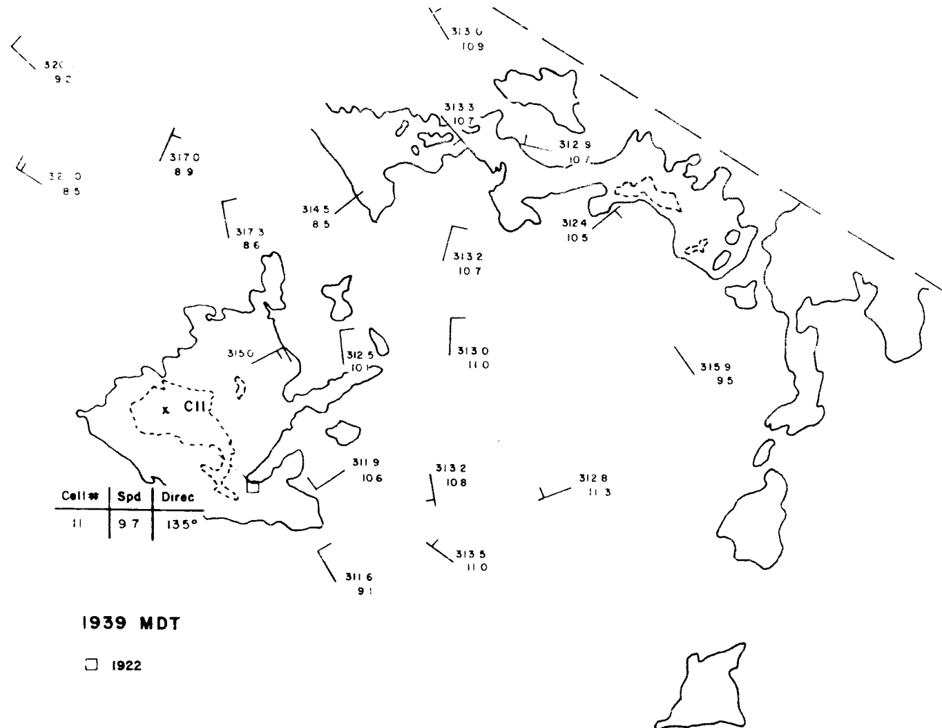
Figure 39. Same as Fig. 24, for 1939 MDT.
