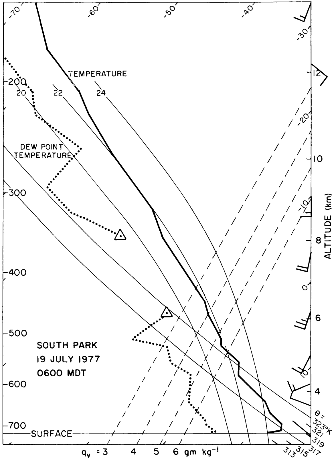
Figure 16. South Park sounding for 0600 MDT (1200 GMT), plotted on skew-T log-P diagram.
