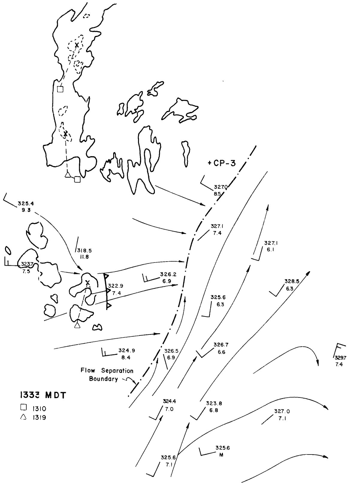
Figure 22. Same as Fig. 21, for 1333 MDT.
