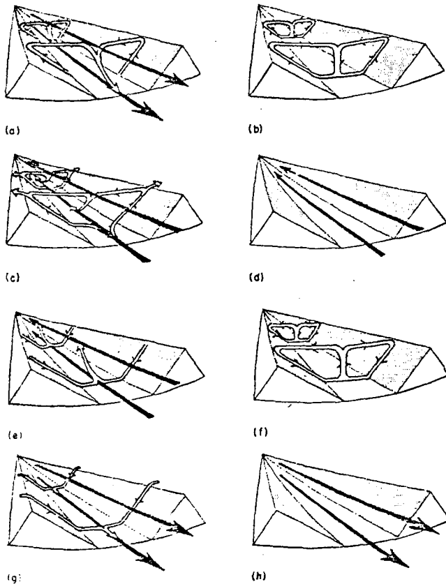
Figure 3. Schematic of the interactions between valley winds and slope winds for a complete 24 hour diurnal cycle. From Defant (1951).
