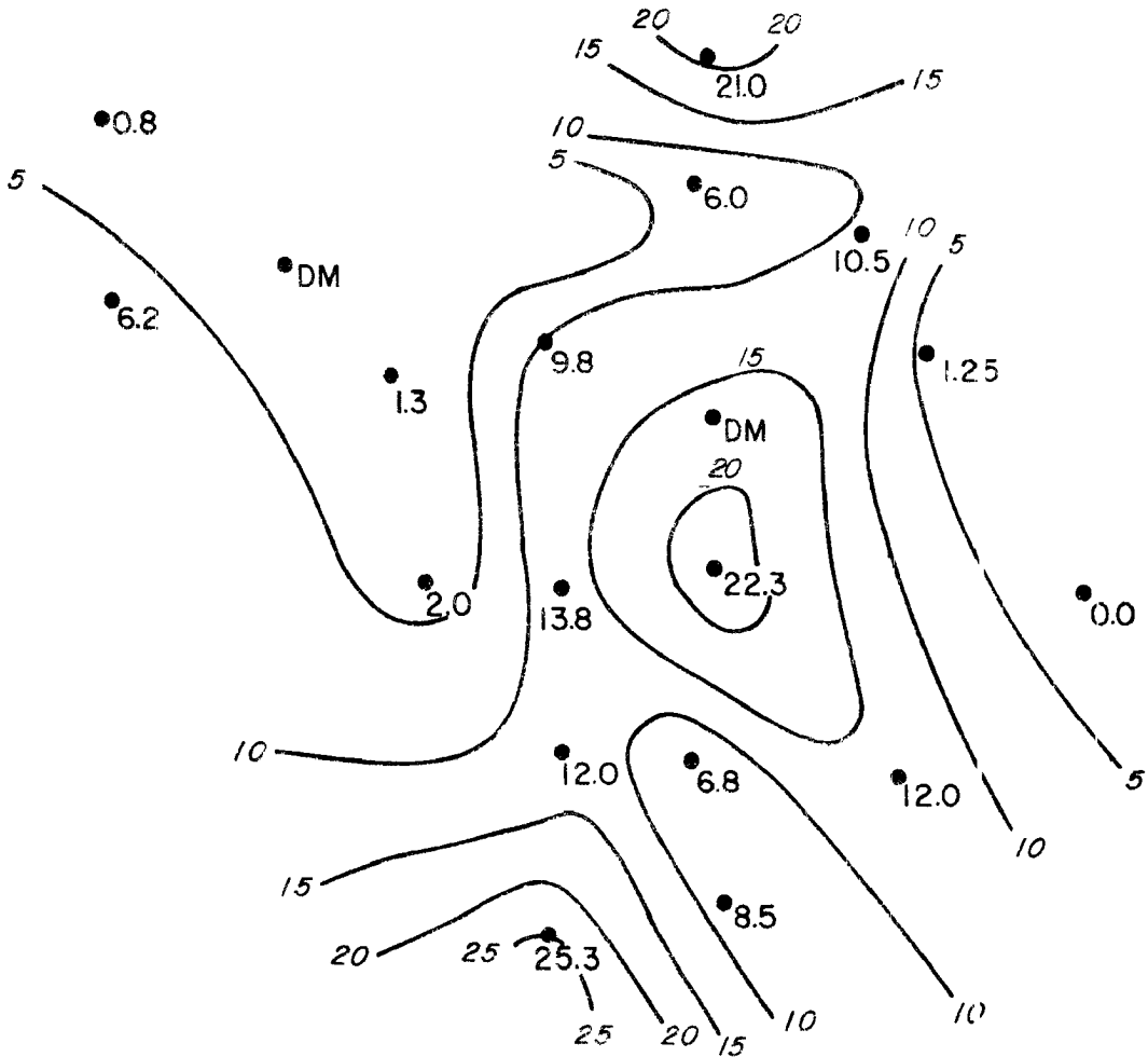
Figure 40. Total rainfall in mm observed at PAM stations, for the time period 1600-2400 MDT, 19 July 1977. Contour interval 5 mm.
