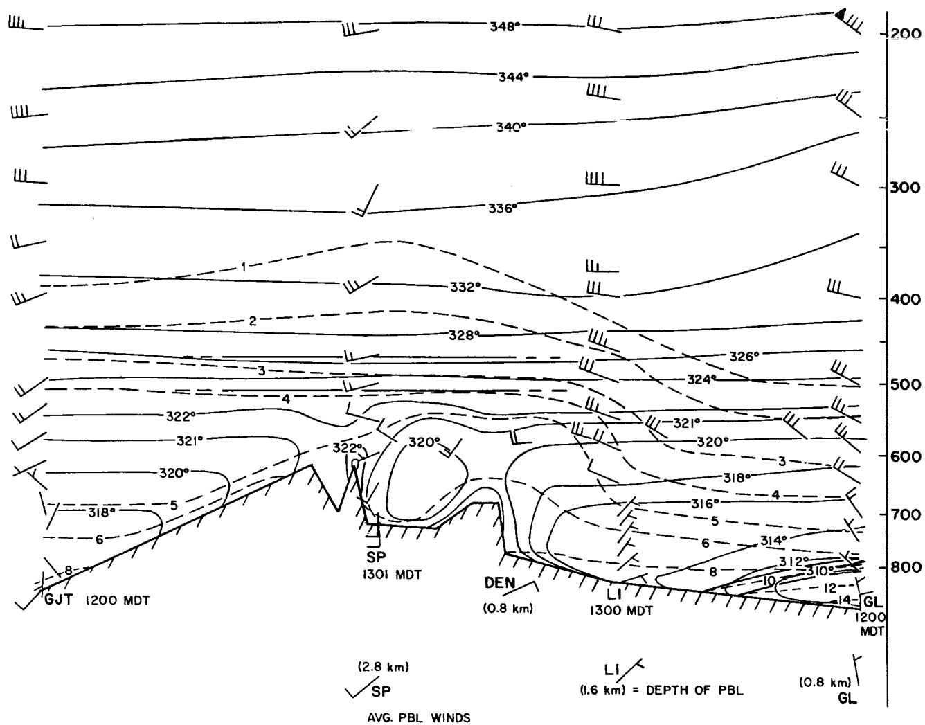
Figure 56. East-west cross-section, as in Fig. 17, for 1200-1300 MDT, 04 August 1977. Average winds in the PBL, along with PBL depth, are plotted for 4 stations (SP, LI, GL, and Denver) in the lower margin. Data from a west-to-east aircraft flight are included in analysis.
