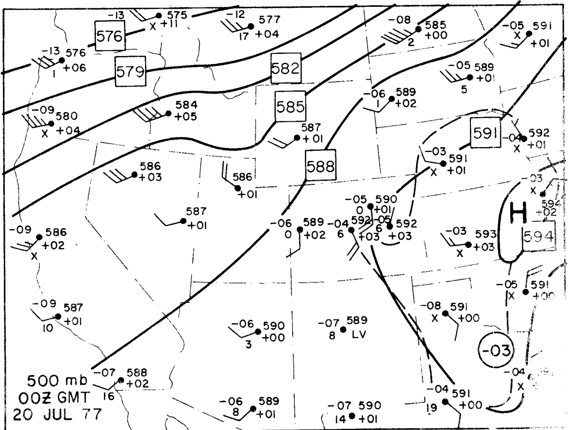
Figure 29. Same as Fig. 13, for 1800 MDT, 19 July, 1977 (0000 GMT, 20 July, 1977).
