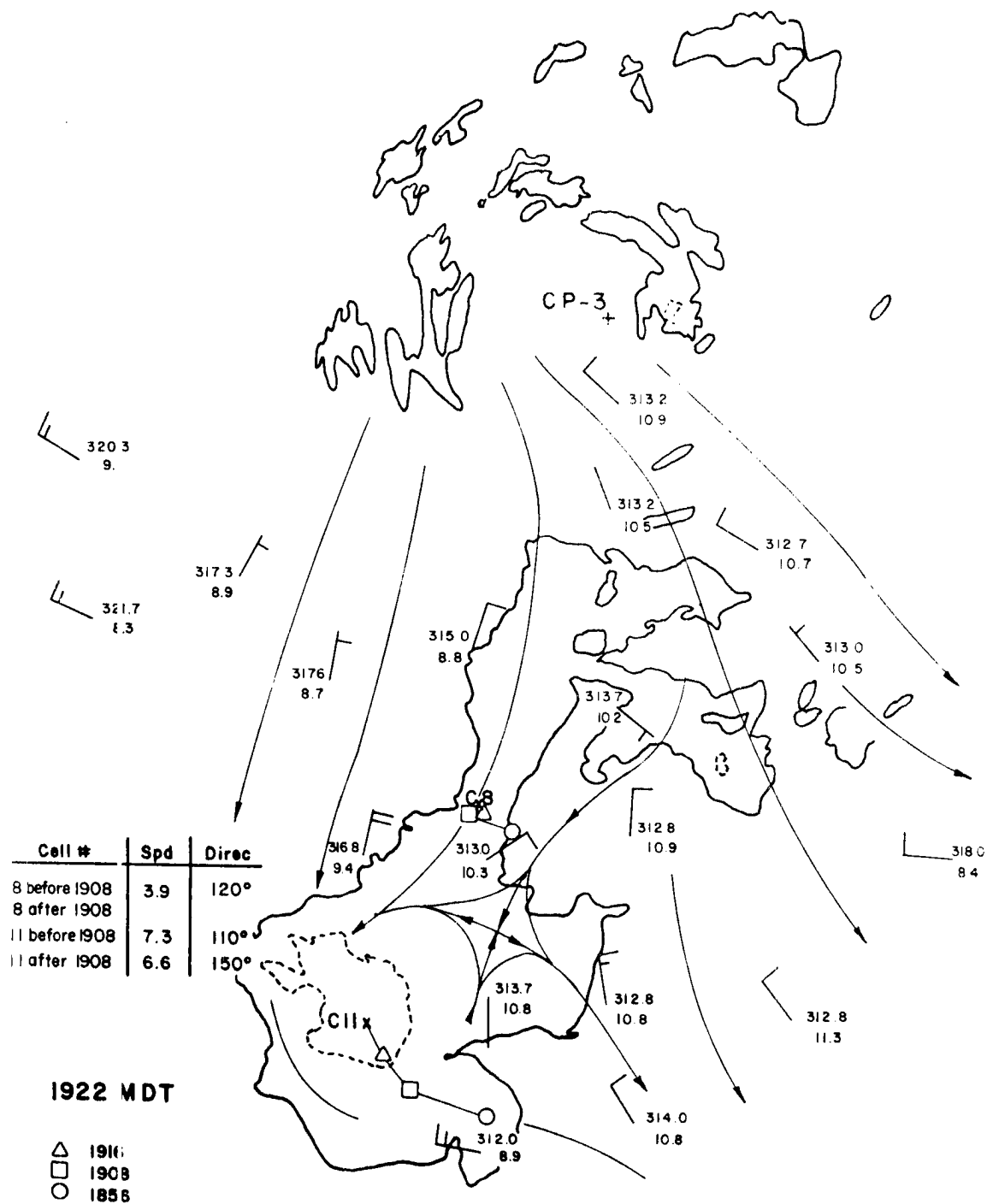
Figure 38. Same as Fig. 24, for 1922 MDT.
