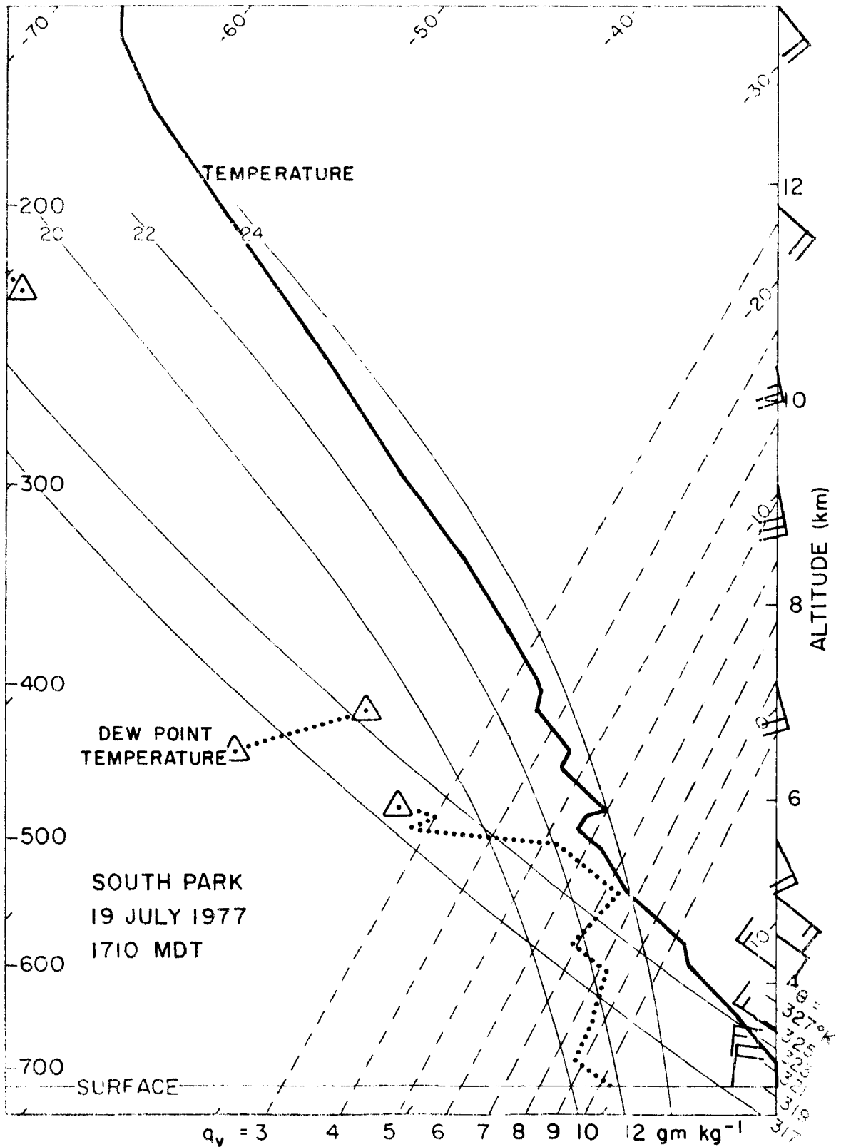
Figure 33. South Park sounding of 1710 MDT, 19 July 1977, plotted on skew-T log-P diagram. Winds between the surface (720 mb) and 500 mb are estimated.
