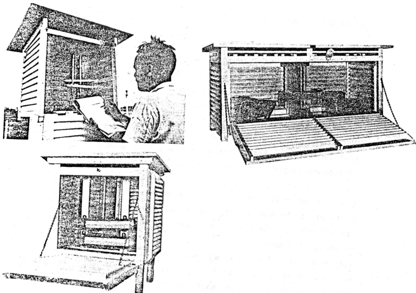
Figure 18. Examples of types of thermometer shelters which may also house hygrothermographs.
