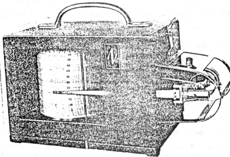
Figure 4. Bi-metallic recording thermograph.
