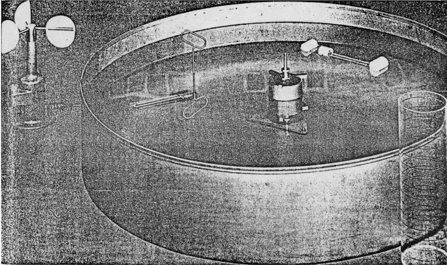
Figure 8. Class A evaporation pan shown with instruments for water temperature and wind speed at pan height.
