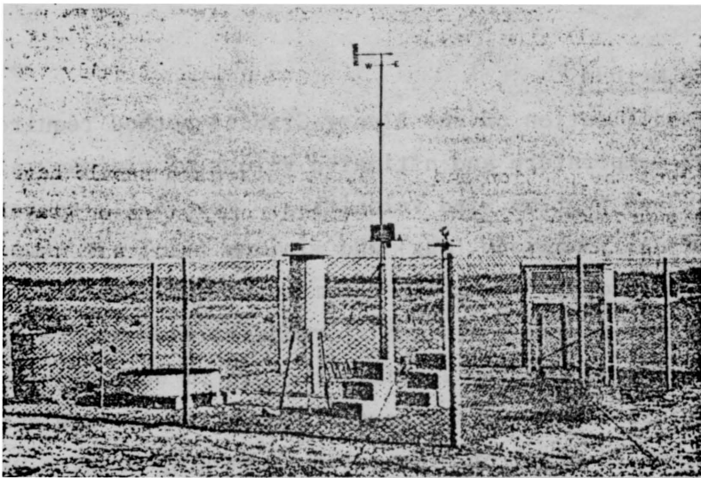
Figure 1. An example of an agrometeorological field station.
