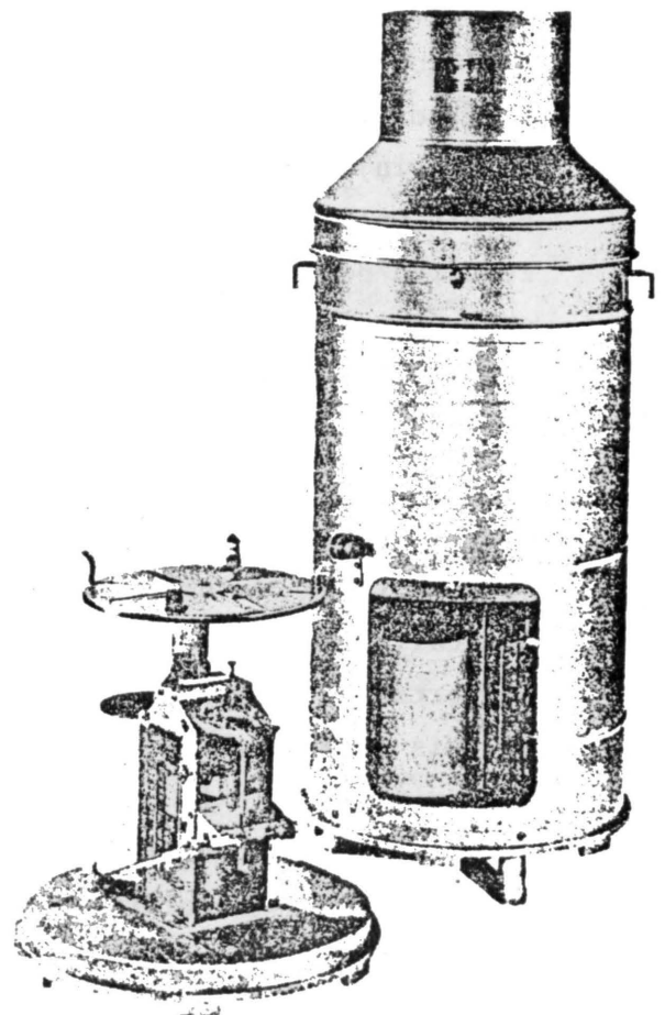
Figure 17. Example of weighing bucket rain gauge and recording device.
