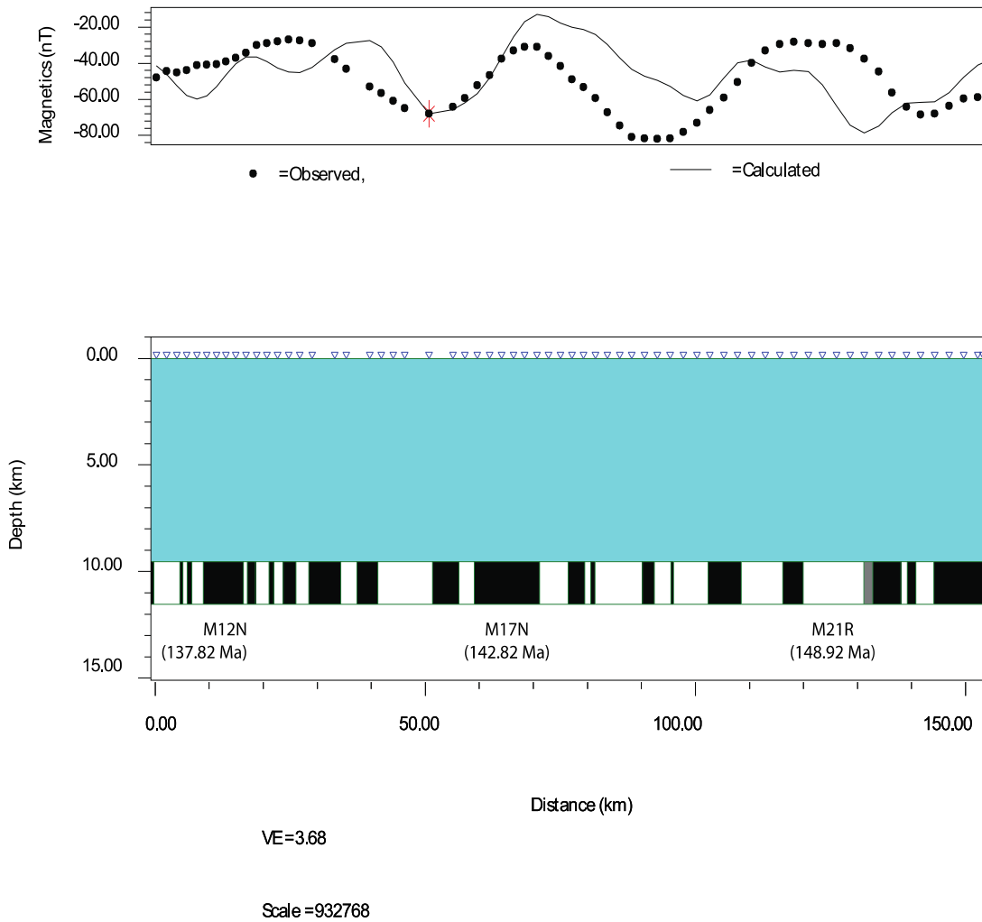
Figure 14: GM-SYS Model of Crust Profile West of the Inferred Spreading Ridge
