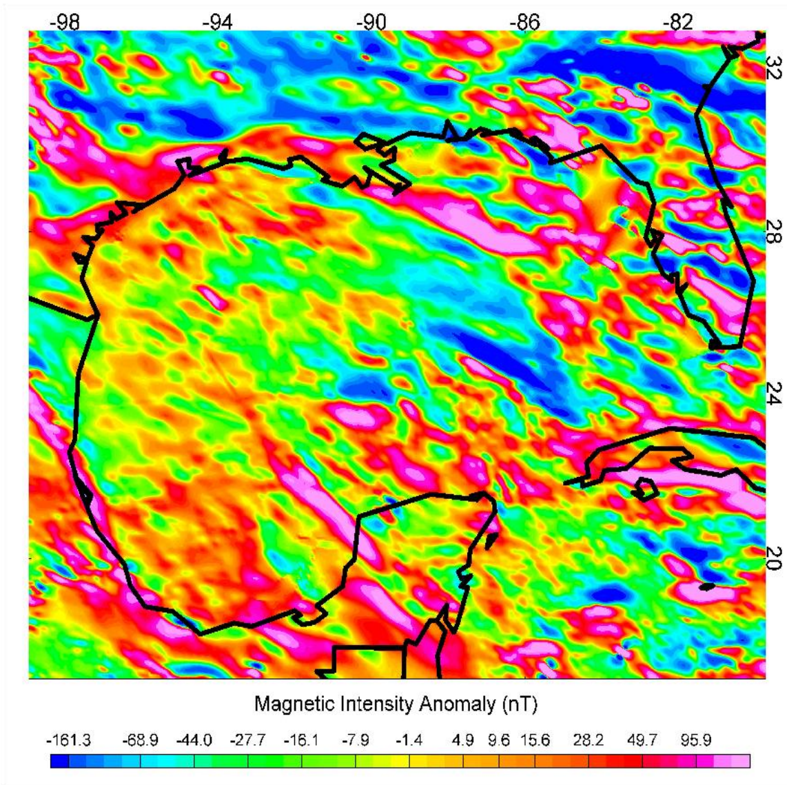
Figure 12c: Directional-Filtered Regional Magnetic Reduced to Pole Intensity Map: 120^\circ
