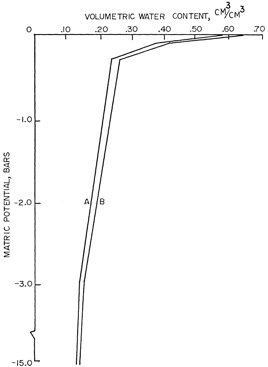
Figure 3.9. Desorption curve for Shingle-Renohill Complex.
