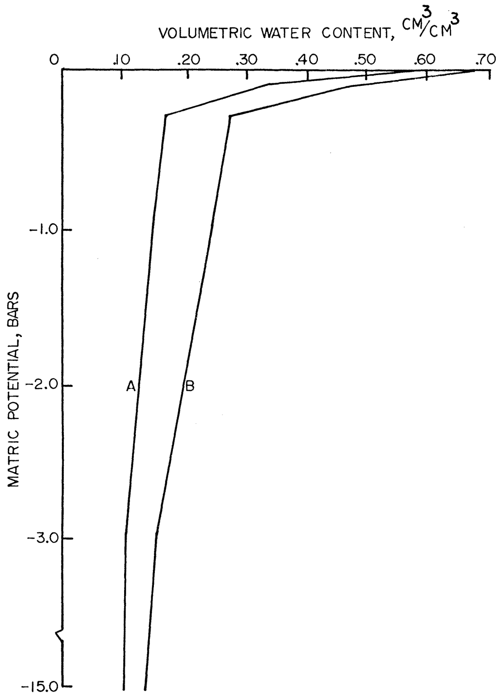
Figure 3.7. Desorption curve for Renohill sandy loam.
