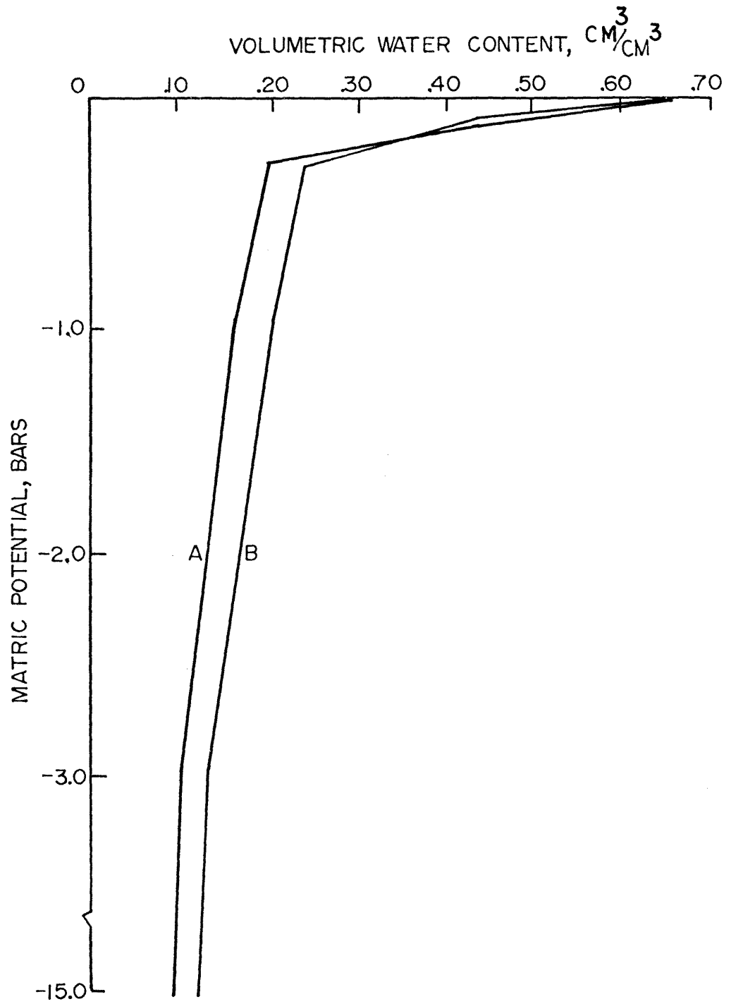
Figure 3.6. Desorption curve for Ascalon sandy loam.
