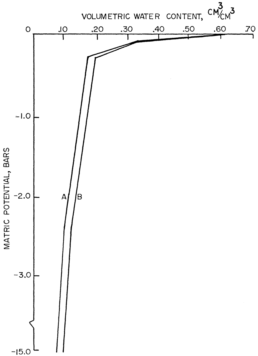
Figure 3.5. Desorption curve for Vona sandy loam.
