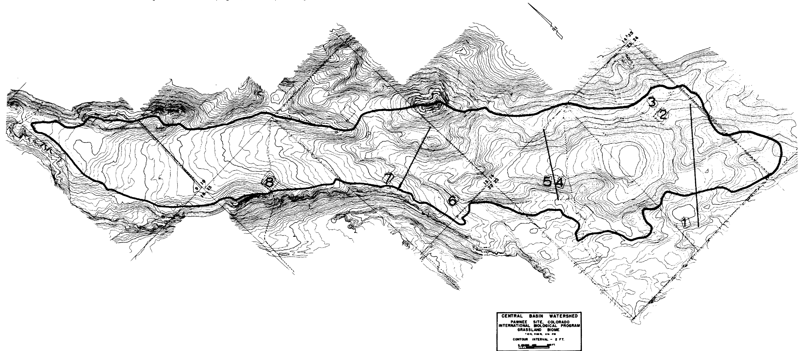
Figure 3.2. Topographic map of Lynn Lake watershed.
