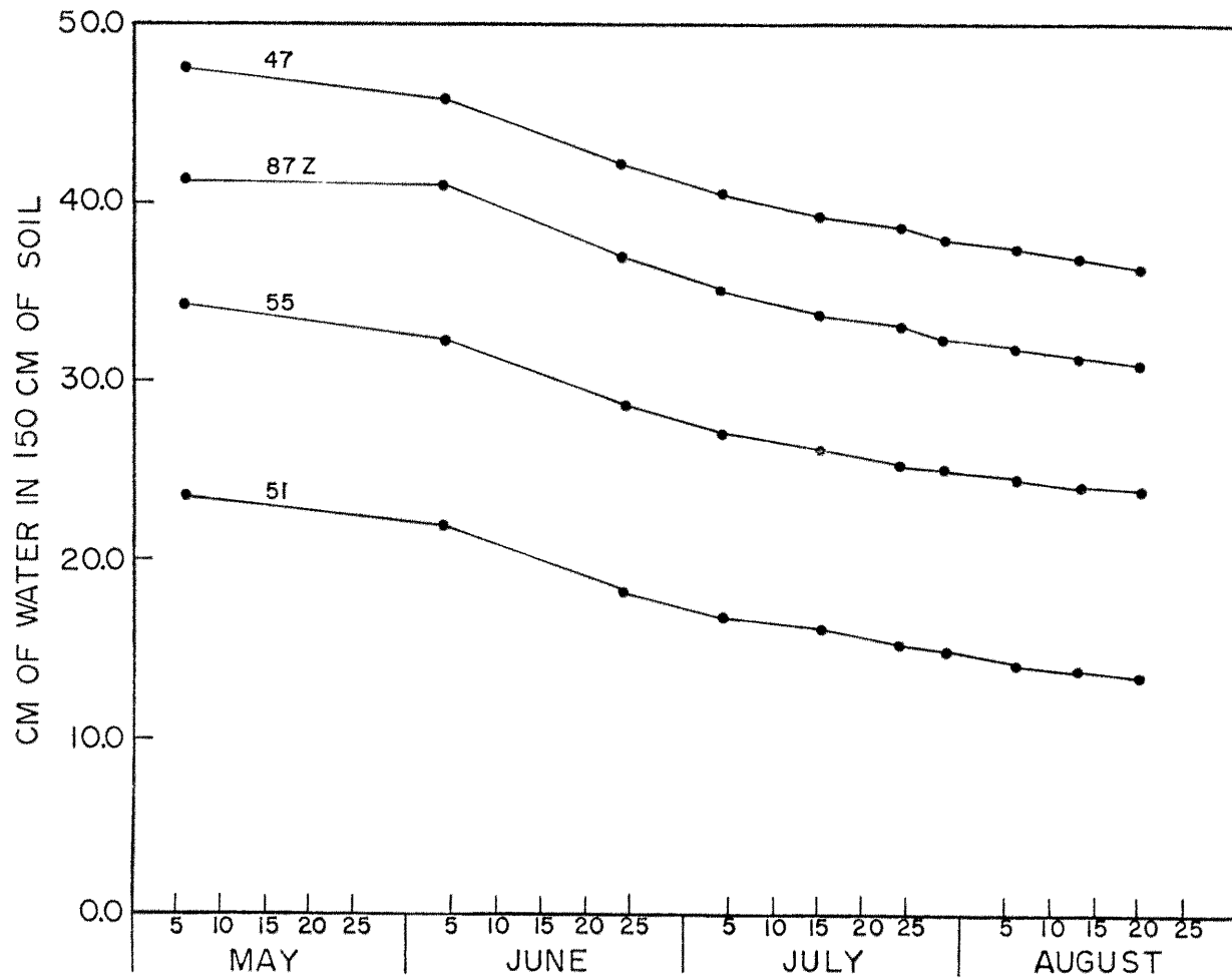
Figure 5.6. Seasonal distribution of soil water depletion by soil type for the heavily-grazed transect.
