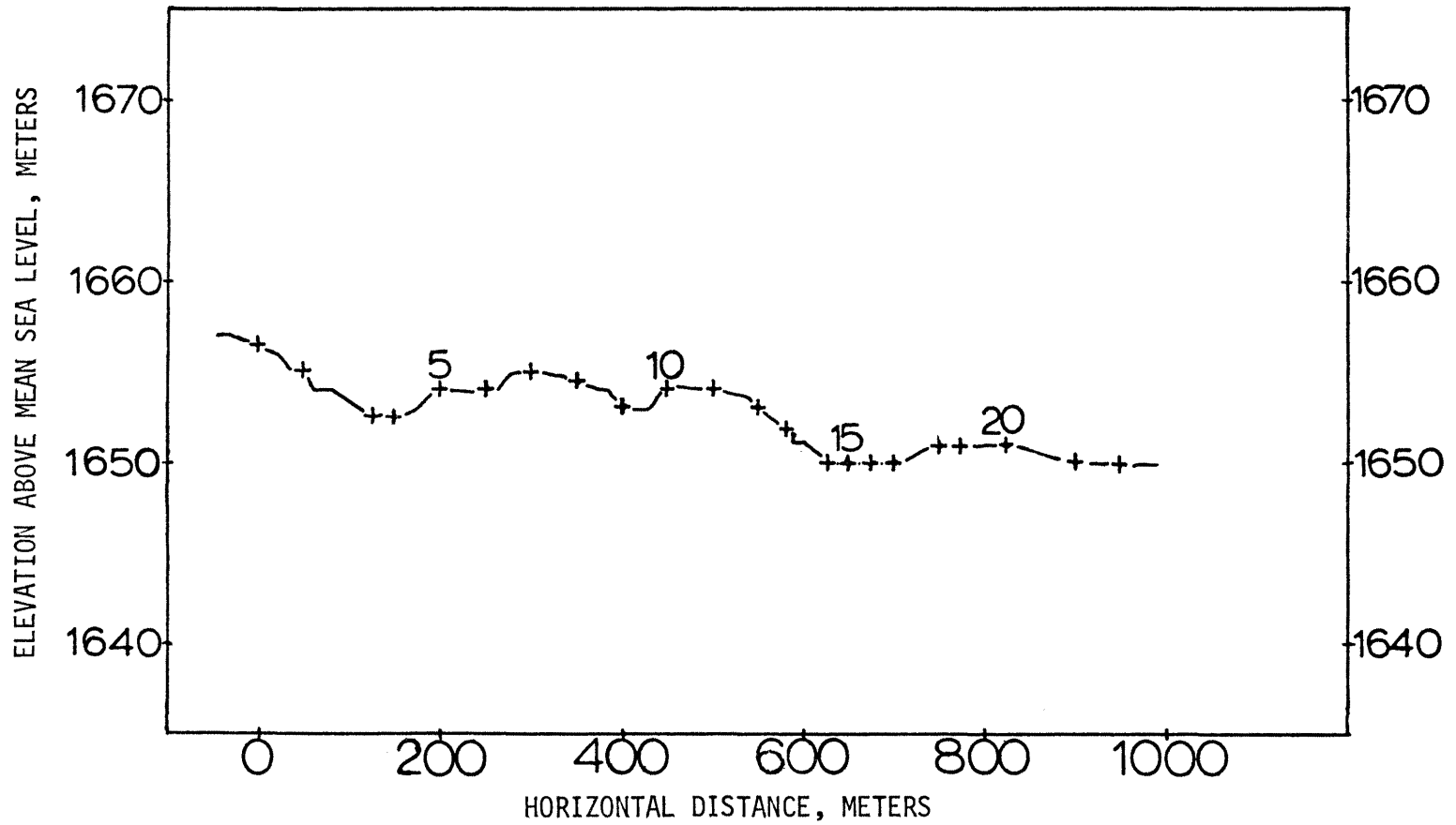
Figure A3. Topographic profile of the heavily-grazed transect, showing the 22 sampling points.
