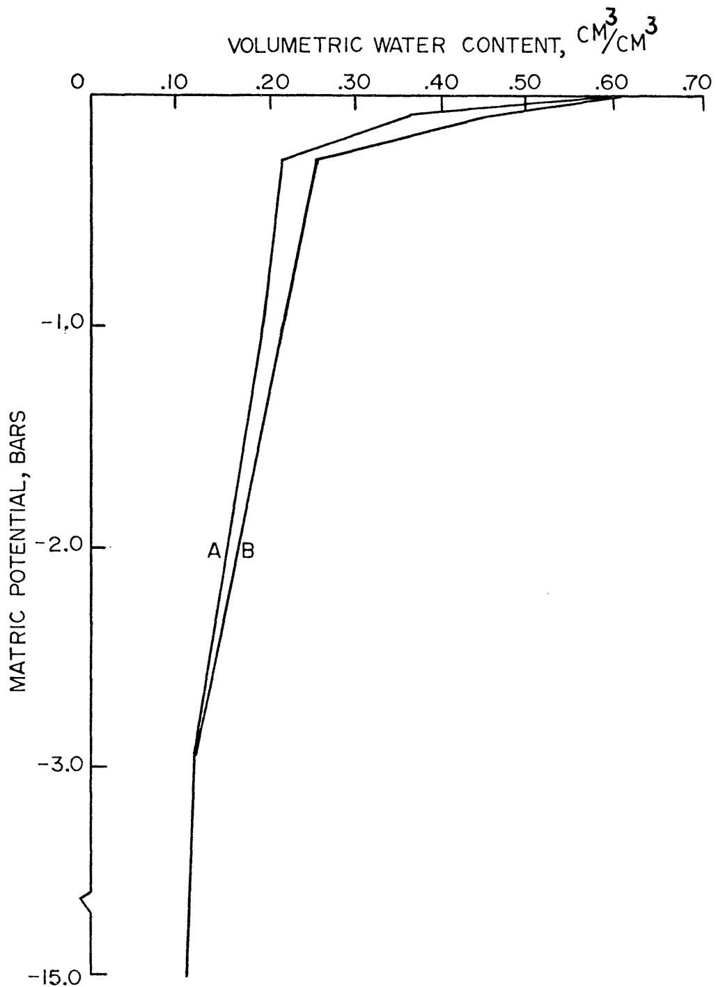
Figure 3.8. Desorption curve for Shingle loam.
