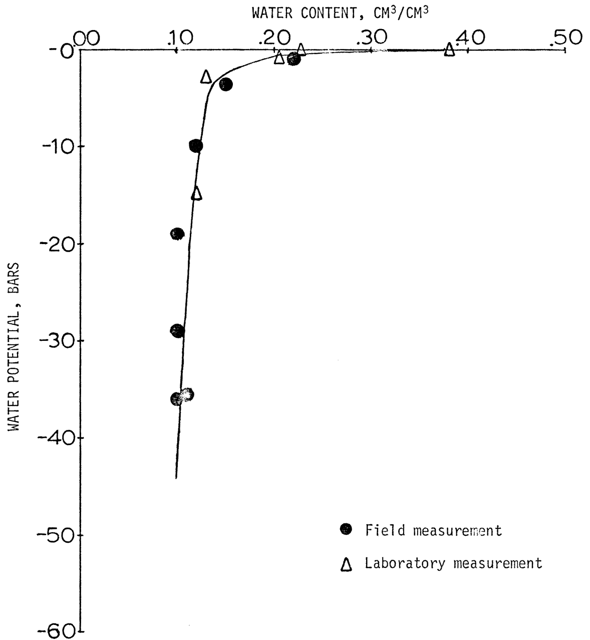
Figure 7.5. Comparison of field vs. laboratory soil water desorption curves for the 40 cm depth in Shingle loam soil.
