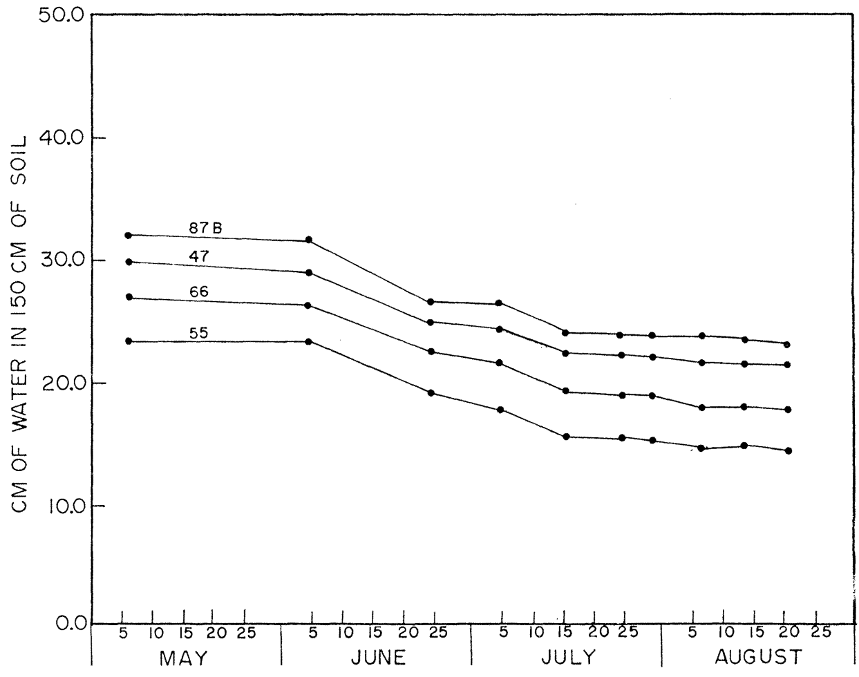
Figure 5.7. Seasonal distribution of soil water depletion by soil type for the moderately-grazed transect.
