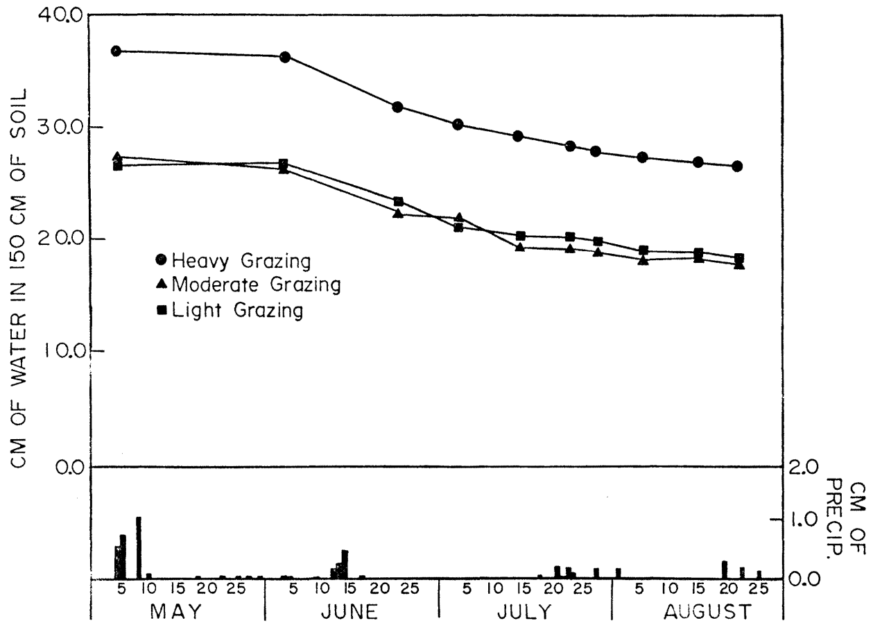
Figure 5.5. Seasonal distribution of soil water storage by grazing treatment.
