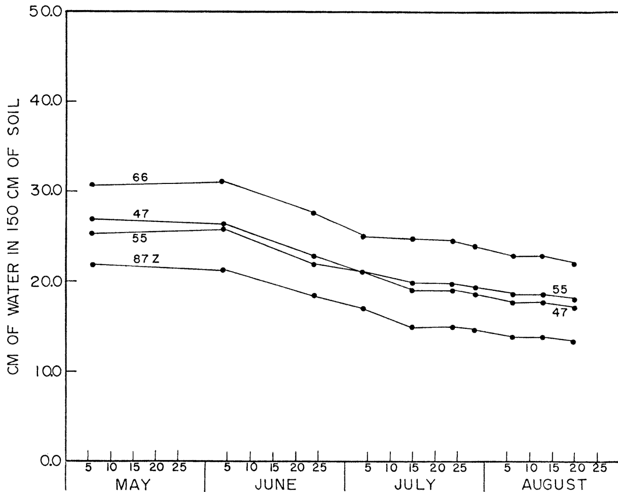
Figure 5.8. Seasonal distribution of soil water depletion by soil type for the lightly-grazed transect.
