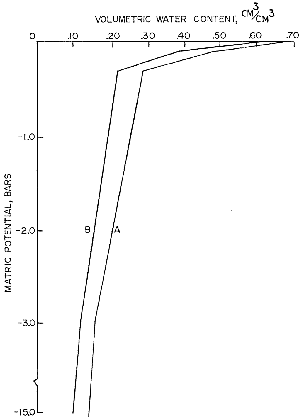
Figure 3.4. Desorption curve for undifferentiated soil.
