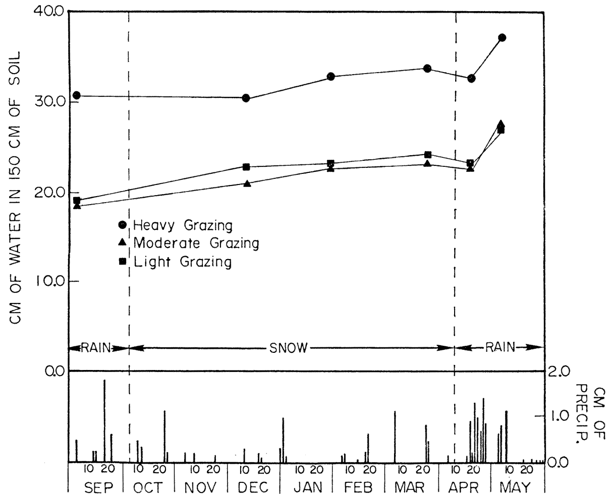
Figure 5.4. Seasonal distribution of soil water storage by grazing treatment.
