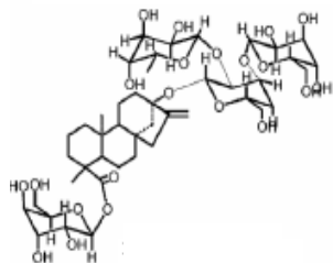
Rebaudioside C
