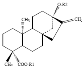
FIGURE 2.1: STEVIOL STRUCTURE
