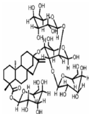
Rebaudioside-A
