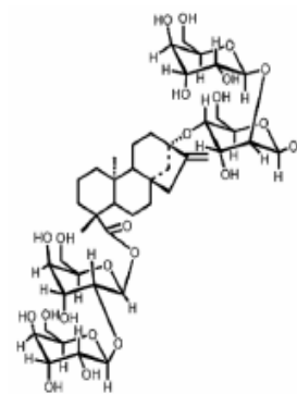
Rebaudioside E
