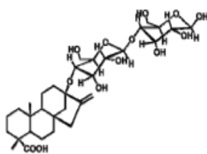
Steviolbioside
