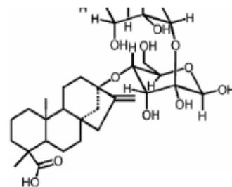
Dulcoside A
