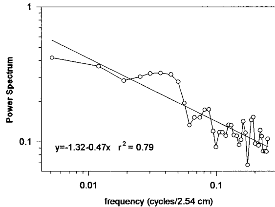
Fig. 4. Power spectrum of infiltration rate (data by Sisson and Wierenga, 1981). Slope of the fitted line \beta=0.47=2H-1 gives D=1.27 .
