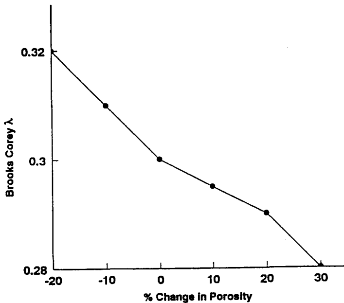
Fig. 1. Effect of changes in porosity on water retention.
