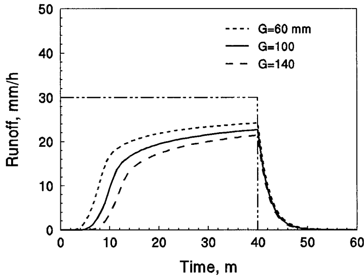
Fig. 3. Effect of G on plot runoff.
