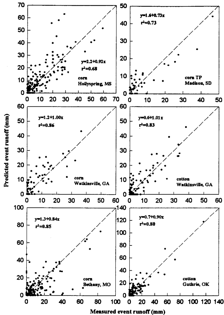
Fig. 4. Measured vs. predicted runoff for each individual storm on selected sites under row crop conditions.
