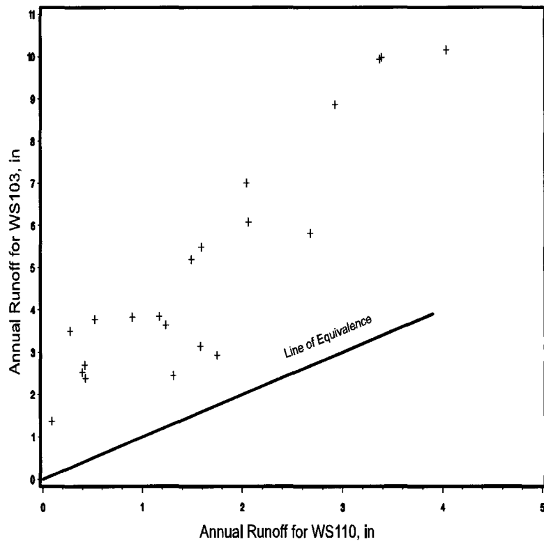
Fig. 1. Comparison of total annual runoff for Watersheds WS103 and WS110.
