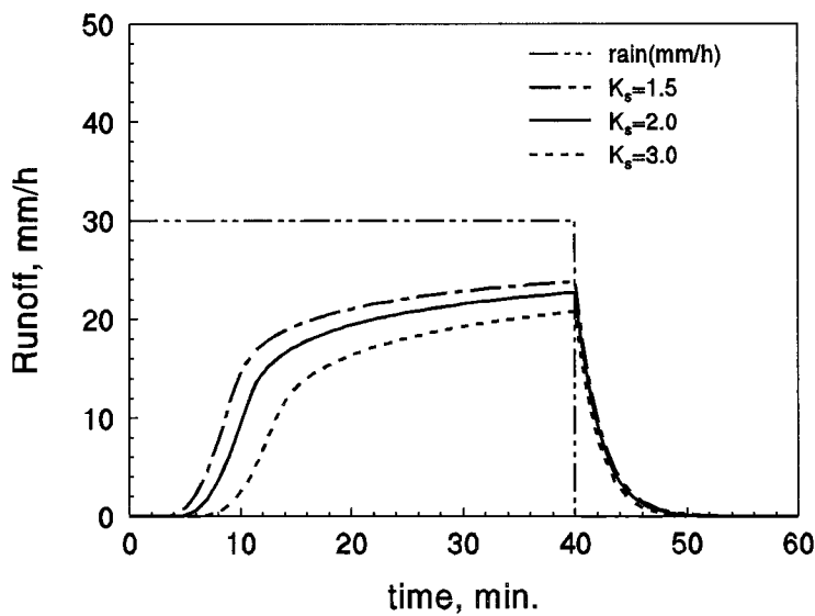
Fig. 4. Effect of K_s on longer hydrograph.
