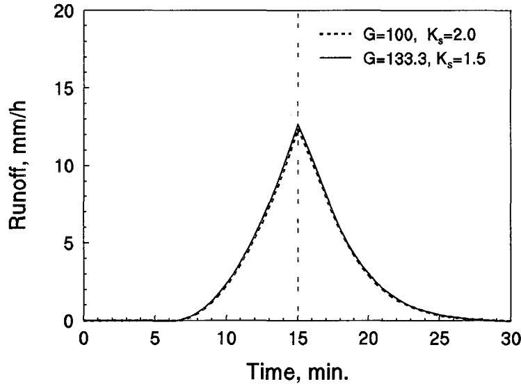
Fig. 5. Interaction of parameters G and K_s in short storms.
