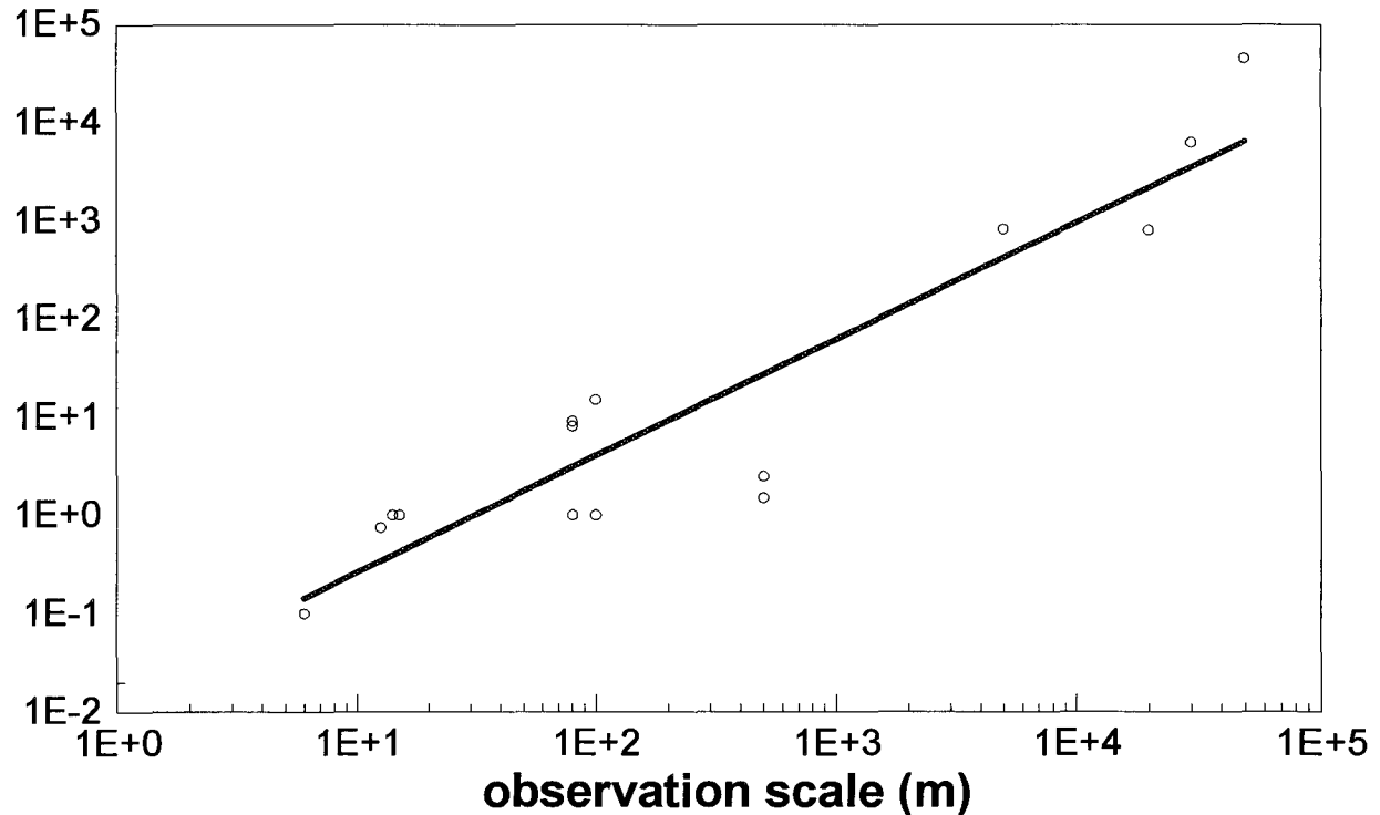
Fig. 1. Relationship between observation scale of the measurements and the calculated correlation scale for the Ks data of Table 1.
