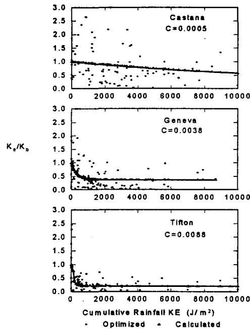
Fig. 3. Comparison of optimized effective conductivities to effective conductivities predicted by the proposed tillage adjustments at three sites.
