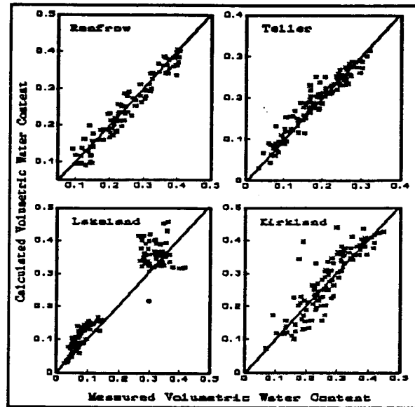
Fig. 2. Calculated versus measured soil water content resulting from the use of the GHM model.
