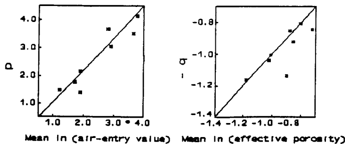
Fig. 3. Relationship between p and mean \ln(\theta_e) , and between q and mean \ln(\psi_e) for eight U.S. soils.
