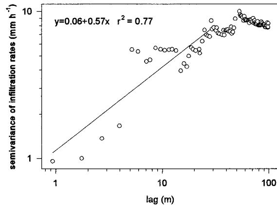
Fig. 3. Semivariogram of infiltration rates (data by Vieira et al., 1981). The slope of the fitted line gives 2H=0.57 and D=1.72 .
