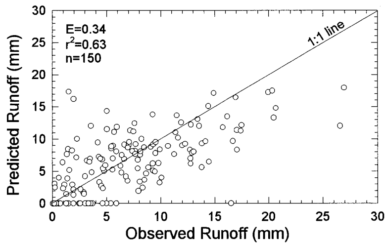
Fig. 3. Comparison of WEPP predicted runoff using K_e values estimated using equations 1 and 2 and observed runoff. The data set of observed runoff is from the same plots that equations 1 and 2 were developed from. E is the coefficient of efficiency (Nash and Sutcliff, 1970), r^2 is the coefficient of determination and n is the number of data points.
