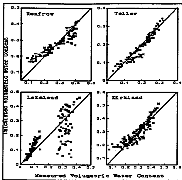
Fig. 1. Calculated versus measured soil water content resulting from the similar-media scaling technique.
