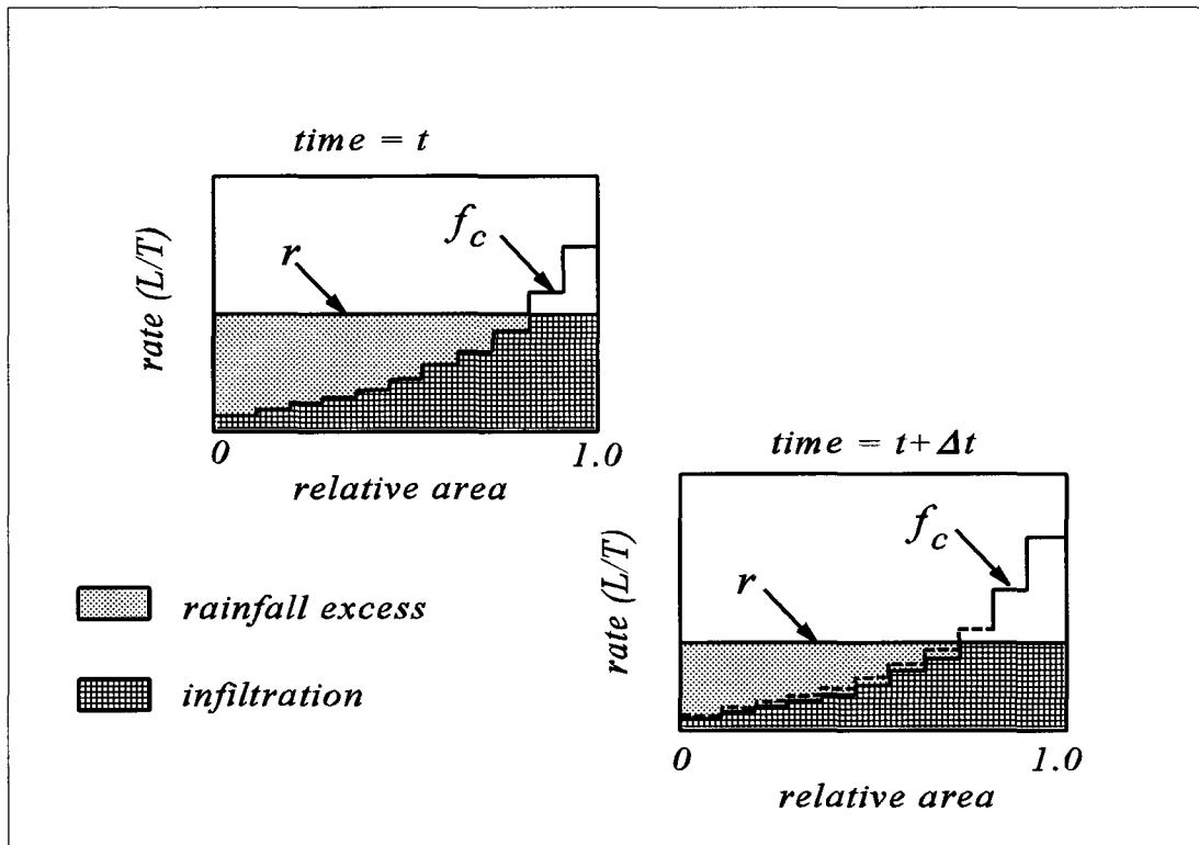
Fig. 1. Illustration of infiltration capacity and infiltration rate changes in space and time during a rainfall event of rate r . Note that infiltration is always limited by r , and f_c decreases in time when limited by soil rather than r . The dotted line indicates f_c at the previous time.
