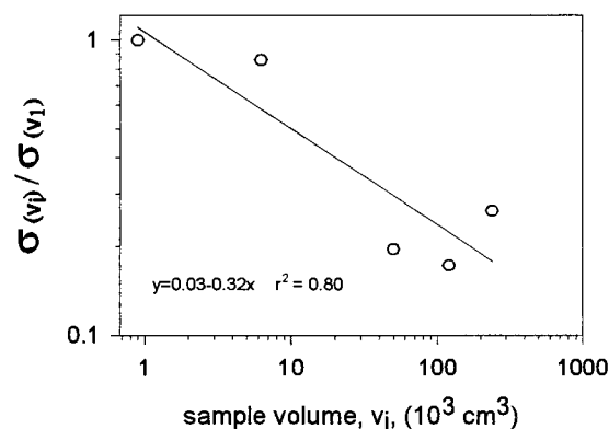
Fig. 2. Scaling of standard deviation, \sigma_i , of K_{sat} measurements as a function of soil volume v_i (data by Lauren et al., 1988). The slope of the fitted line is 2H=0.32 and D=1.84 .
