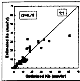
Fig. 1. Estimated values of baseline hydraulic conductivity for time-variable case plotted against those calibrated from curve number predictions.
