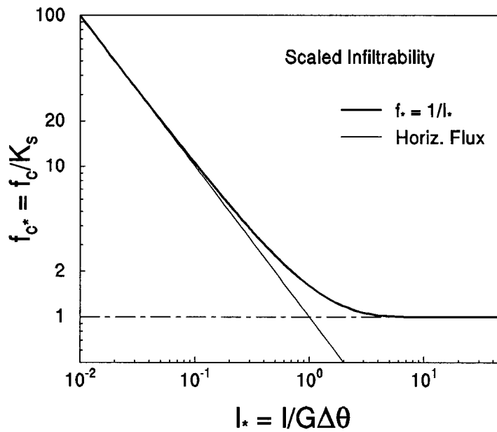
Fig. 2. Illustration of the scaled infiltration relation.
