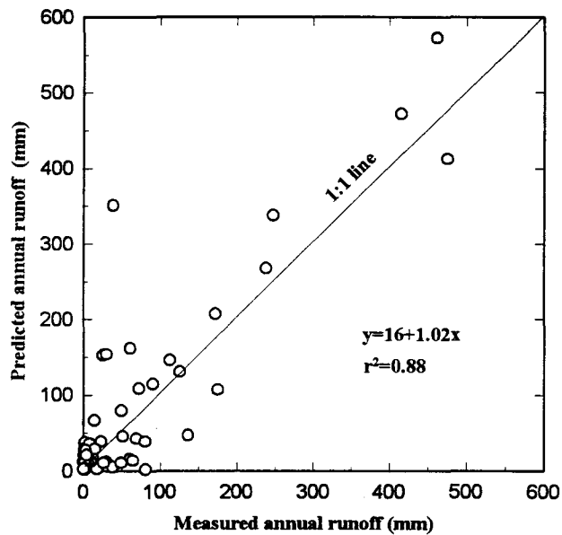
Fig. 5. Measured vs. predicted annual runoff for the data used under meadow conditions.
