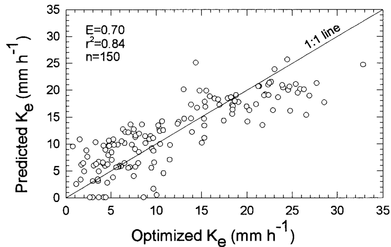
Fig. 1. Comparison of WEPP optimized and predicted effective hydraulic conductivity ( K_e , \text{mm h}^{-1} ) using equations 1 and 2. E is the coefficient of efficiency (Nash and Sutcliffe, 1970), r^2 is the coefficient of determination and n is the number of data points.
