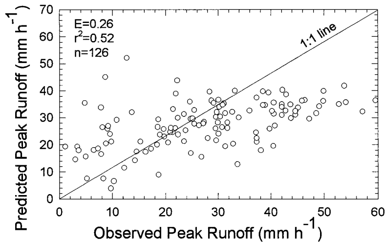
Fig. 4. Comparison of WEPP predicted peak runoff using K_e values estimated using equations 1 and 2 and observed runoff. The data set of observed peak runoff is from the same plots that equations 1 and 2 were developed from. E is the coefficient of efficiency (Nash and Sutcliff, 1970), r^2 is the coefficient of determination and n is the number of data points. The number of data points shown is 126 because 24 plots had zero predicted runoff.
