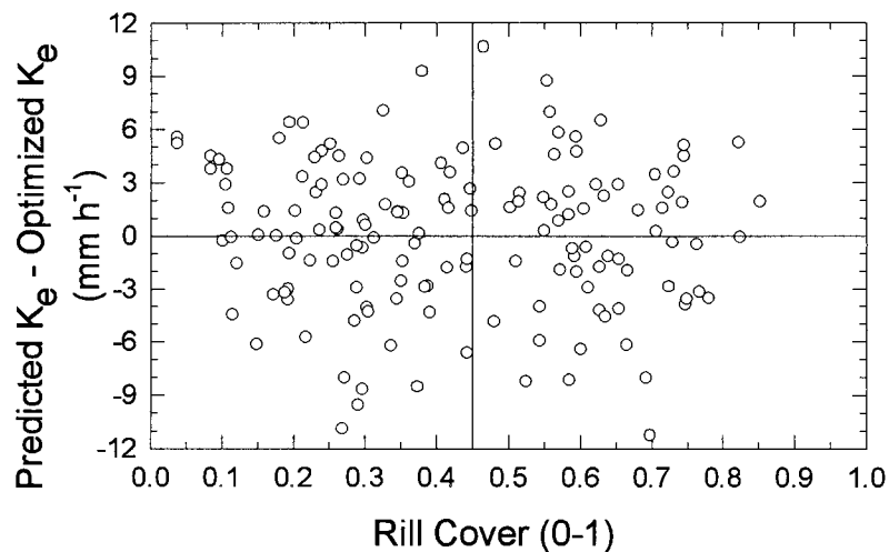
Fig. 2. Difference between WEPP optimized and predicted K_e using equations 1 and 2.
