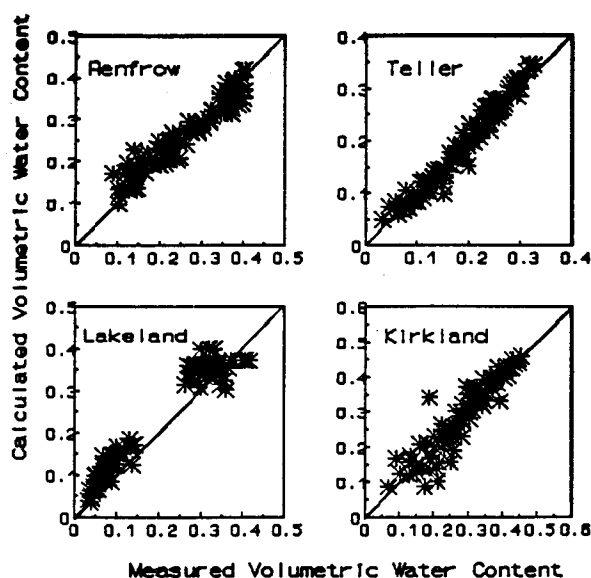
Fig. 4. Calculated versus measured soil water content using GHM with p and q values based on mean values of \ln(\theta_e) and \ln(\psi_e) , respectively.
