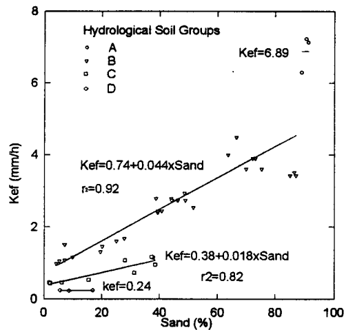
Fig. 6. Optimized effective conductivity values for fallow soil conditions, K_{ef} , plotted versus sand content of the soil. This is for the case of time-invariant conductivity.
