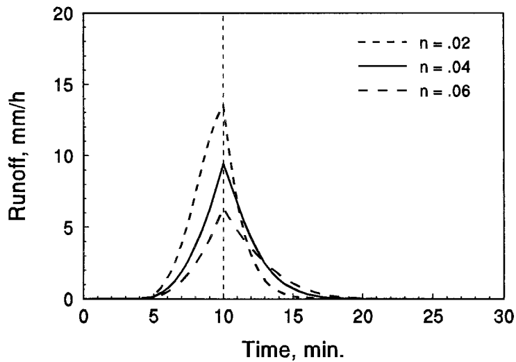
Fig. 7. Effect of roughness for short storm.
