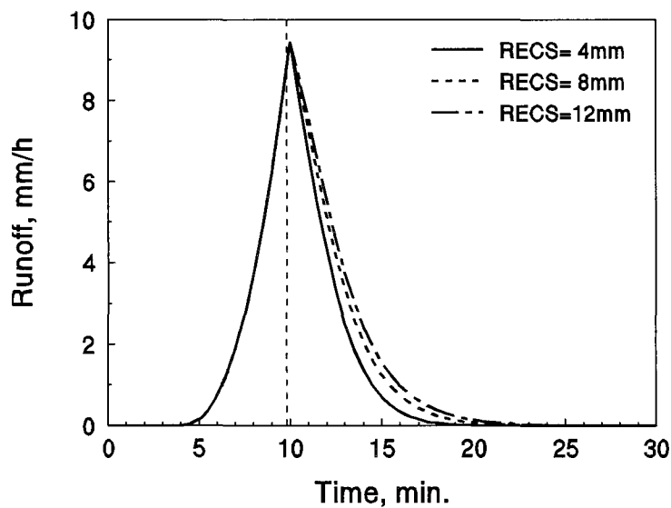
Fig. 8. Effect of microtopographic relief parameter on recession.
