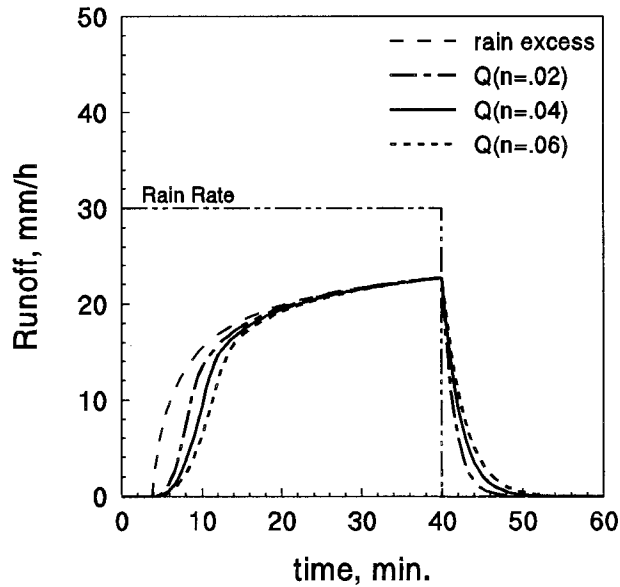
Fig. 6. Effect of roughness on surface storage.
