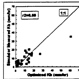
Fig. 2. Baseline hydraulic conductivity values for time-variable case measured under rainfall simulation compared to those calibrated from curve number predictions.
