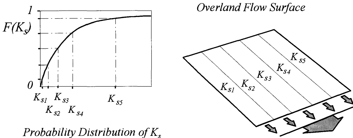
Fig. 3. Latin hypercube parallel strip method for simulating a distribution of infiltration parameters on a runoff surface. Each strip contains an equally likely value of K_s .
