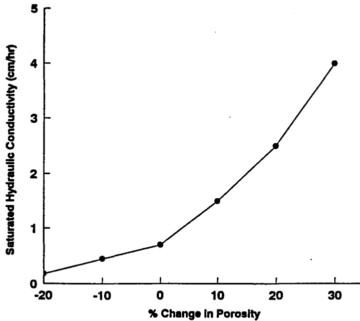
Fig. 3. Effect of changes in porosity on saturated hydraulic conductivity.
