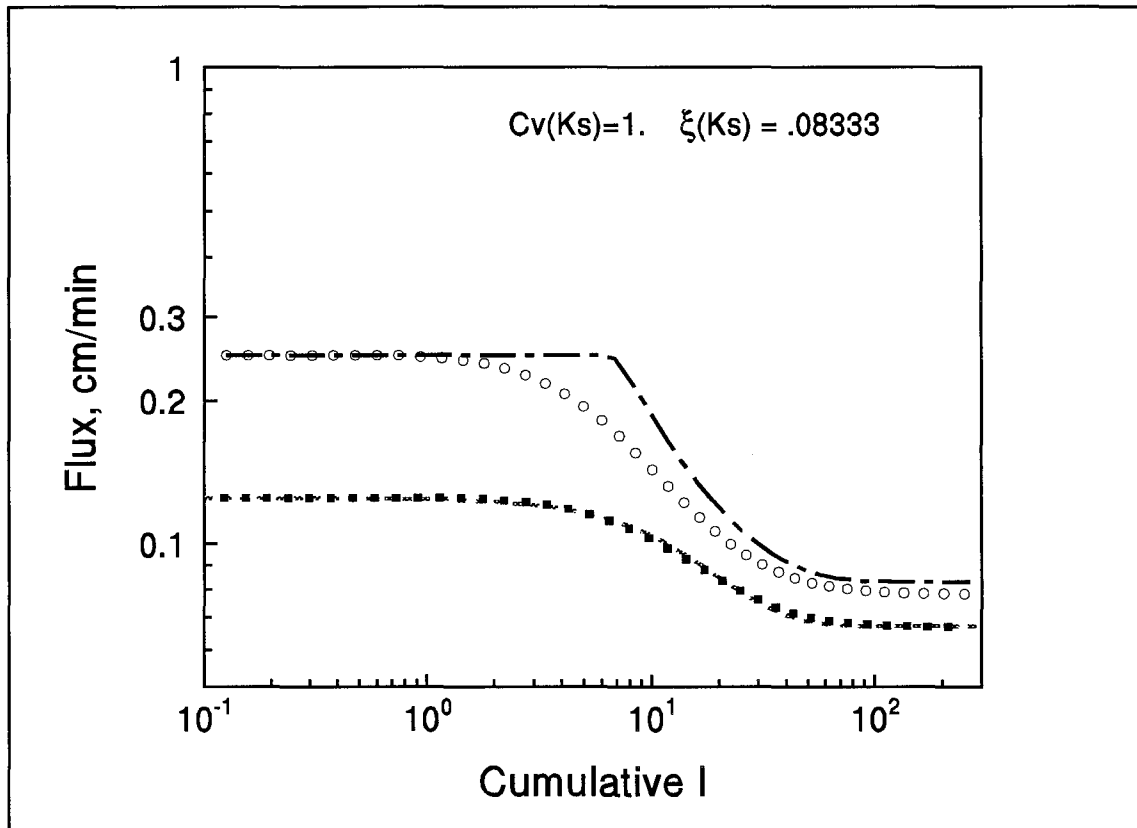
Fig. 2. Areal ensemble infiltration relations for two intensities, compared with the point infiltration function for the expected value of K_s (dot and dashed line), when the coefficient of variation of K_s is 1.
