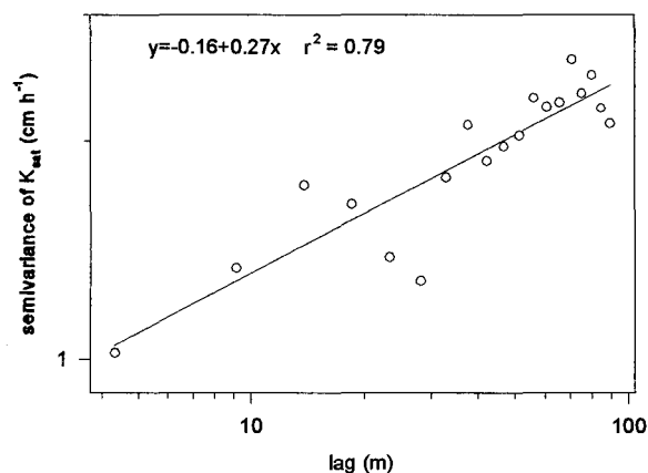
Fig. 1. Semivariogram of \ln K_{sat} measured in the field at 0.3 m depth (data by Mohanty et al., 1991). The slope of the fitted line gives 2H=0.27 and D=1.87 .
