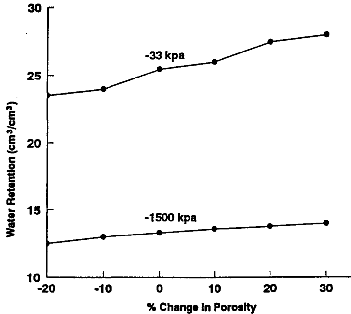
Fig. 1. Effect of changes in porosity on water retention.
