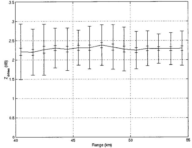
FIG. 6. Shown is Z_{DRbias} vs range based on 40 rays of CSU–CHILL data collected during the Fort Collins flood of 28–29 Jul 1997. Sample mean value and the 95% confidence interval for the mean are shown.
