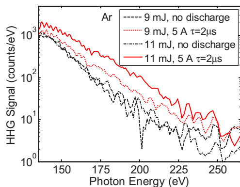
FIG. 4. (Color online) Laser intensity dependence of the highest observed photon energies obtained from 6 Torr of Ar using 9 and 11 mJ, 28 fs pulses, injected 2 \mu\text{s} after a current pulse of 5 A. The HHG spectra extend towards higher energies when laser intensity is increased in the case of a capillary discharge while the highest observed photon energies are intensity independent when a hollow waveguide is used.
