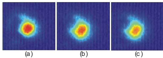
FIG. 12. (Color online) Comparison of near field images of low intensity ( <10^{14} W/cm 2 ) laser pulses exiting the discharge at (a) 200 ns before the onset of the current pulse, (b) 600 ns, and (c) 1200 ns after the onset of the current pulse. The discharge was operated under the same conditions as in Fig. 11.
