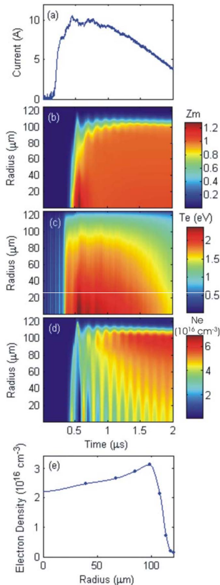
FIG. 6. (Color online) Calculated discharge plasma parameters for the measured 10 A current pulse (a) in a 250 \mu\text{m} inner diameter capillary initially filled with 3.0 Torr Xe. The mean ion charge (b) of the plasma is Z_m \sim 1 over most of the radius for most of the current pulse. The electron temperature (c) is highest on axis and decreases radially giving rise to a concave transverse electron density profile (d) through pressure equilibrium. The electron density profile at 2000 ns is plotted in (e). Please see the online version for an accurate color scale.
