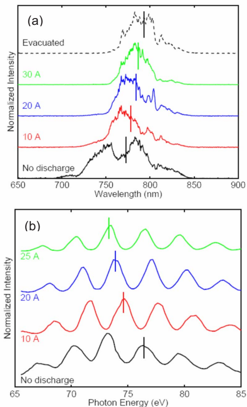
FIG. 9. (Color online) (a) Spectra showing the blueshift of 9 mJ laser pulses for various currents in the capillary discharge initially filled with 5.2 Torr Ar. The spectra for discharge currents of 0, 10, 20, and 30 A, and through an evacuated capillary are shown with central wavelengths (vertical bars) of 773, 778, 784, 787, and 793 nm, respectively. (b) High harmonic spectra, from a 9 mJ pulse propagating through 5.8 Torr Ar, with and without the discharge present, showing the effects of blueshifting of the fundamental spectrum. Spectra for 0, 10, 20, and 25 A are shown, as is the location of the center of the 47th harmonic (vertical bars).
