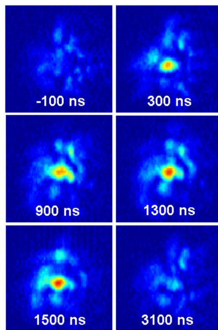
FIG. 11. (Color online) Near field images of intense laser pulses in the exit plane of the capillary at different time delays during the current pulse. The initial Ar pressure was 6.0 Torr and 10 A current pulses were used. The input laser pulses were 28 fs FWHM in duration and had energies of 8.5 mJ.
