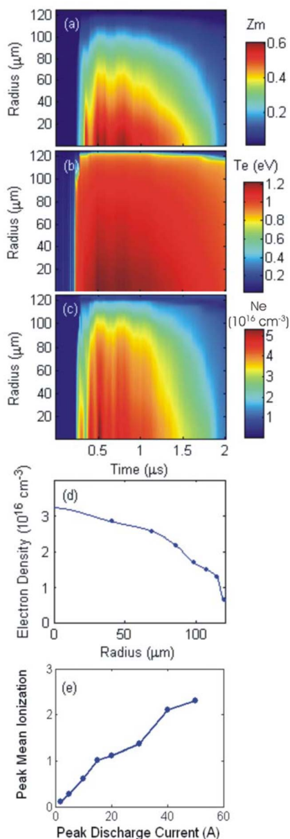
FIG. 7. (Color online) Calculated discharge plasma parameters for a 10 A current pulse in a 250 \mu\text{m} inner diameter capillary initially filled with 6.0 Torr Ar. The mean ionization (a) of the plasma peaks at Z_m=0.6 . The electron temperature (b) and the electron density profile (c) are significantly different than in the case of Xe. The electron density profile at 1500 ns (d) is essentially flat over the radius of the capillary. (e) Model prediction of peak mean ion charge vs discharge current for an initially 6.0 Torr Ar plasma in a 250 \mu\text{m} capillary. Please see the online version for an accurate color scale.
