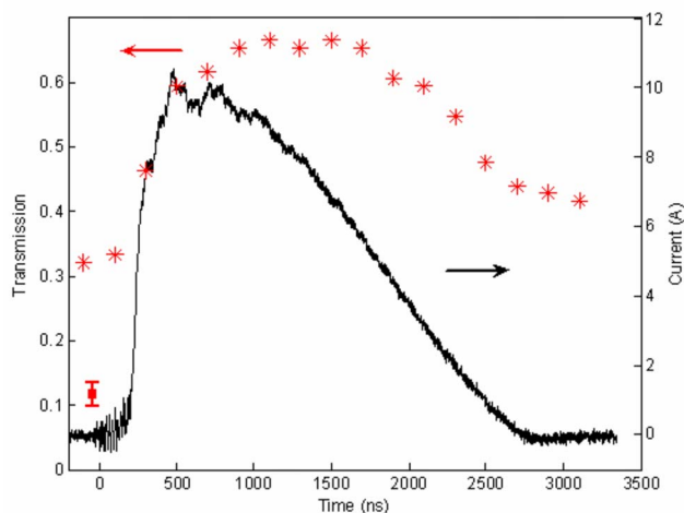
FIG. 10. (Color online). Measured transmission (stars) of 8.5 mJ, 28 fs FWHM pulses through the 5 cm capillary discharge waveguide with a 10 A peak current pulse and an initial Ar pressure of 6.0 Torr. The measured current pulse is shown.
