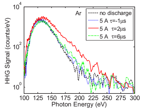
FIG. 3. (Color online) HHG signal for various delay times \tau between the onset of the discharge current pulse and the injection of the laser pulse (dotted blue \tau=-1 \mu\text{s} , laser pulse arrives before the current pulse; solid red \tau=2 \mu\text{s} , optimal time delay; and dash-dot green \tau=6 \mu\text{s} , laser pulse arrives after the current pulse). The spectra were obtained from 6 Torr of Ar using 9 mJ, 28 fs laser pulses in the capillary discharge with 5 A current pulses. A spectrum obtained under the same conditions in a hollow waveguide (dashed black) is shown for comparison.
