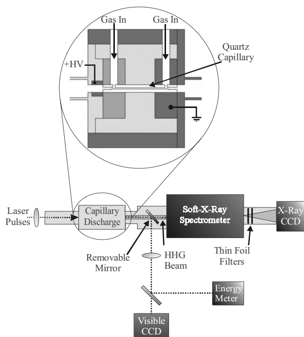
FIG. 1. Schematic of the experimental setup. The inset is a diagram of the capillary discharge.
