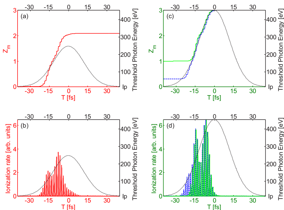
FIG. 8. (Color online) Calculated mean ionization Z_m and laser ionization rates of Ar species for 28 fs laser pulses with peak intensities of 1.3 \times 10^{15} \text{ W/cm}^2 [(a) and (b)] and 2.3 \times 10^{15} \text{ W/cm}^2 [(c) and (d)] using ADK rates for the conditions in Fig. 5 [without the discharge (solid red, initial Z_m=0 ); with a discharge current of 5 A (dashed blue, initial Z_m \sim 0.3 ) and 15 A (solid green, initial Z_m \sim 1 )]. The right axes show the predicted threshold photon energy for the laser intensity profile (dotted black) calculated from the cutoff rule h\nu_{\text{max}} = I_p + 3.17U_p .
