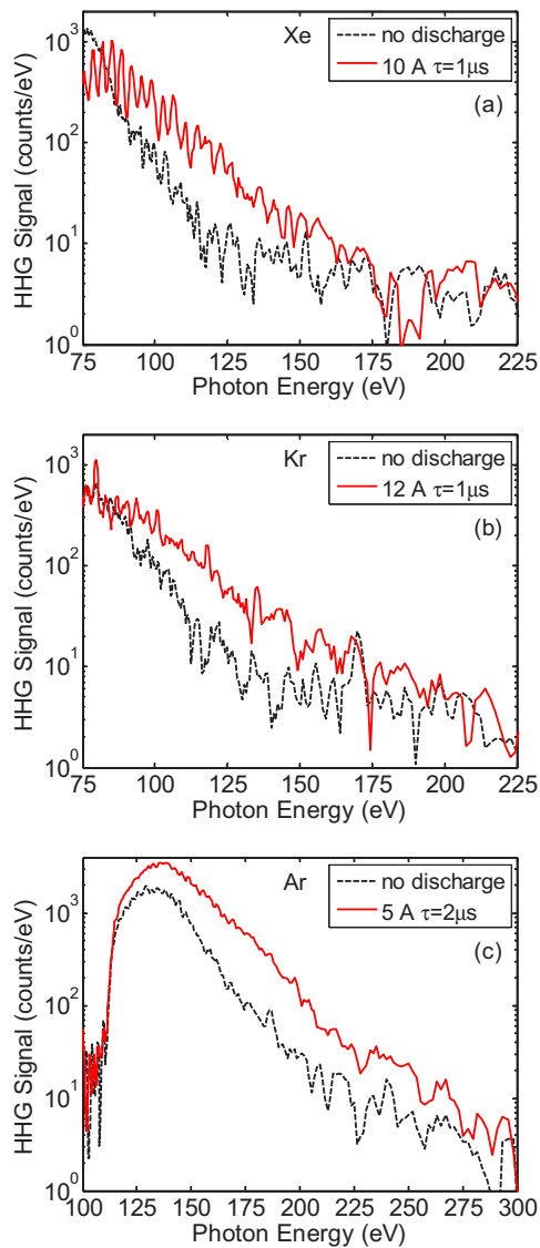
FIG. 2. (Color online) High-order harmonic spectra on a log scale with (solid red) and without (dashed black) the discharge showing an extension of the HHG cutoff to photon energies of (a) above 160 eV in 3 Torr of Xe using 10 mJ laser pulses; (b) above 170 eV in 6 Torr of Kr with 10 mJ laser pulses; and (c) above 275 eV in 6 Torr of Ar with 11 mJ laser pulses. A 250 \mu\text{m} diameter bore, hollow core fiber was used for all three gases. The discharge current and the time delay parameters are shown in the picture.
