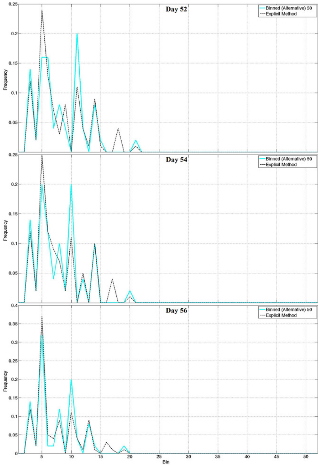
Figure 4.261. Total plant available water distribution plots for the explicit and alternative binned (50 bins) method, where precipitation events occur each day somewhere over the grid area as a result of the highly spatially varying precipitation distribution (bin wetness increases to the right).
