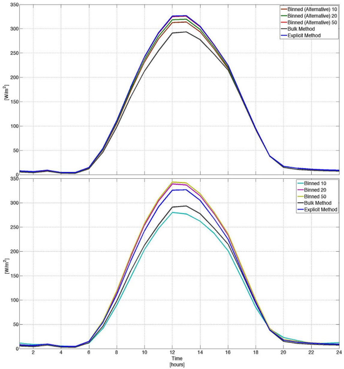
Figure 4.23b. Diurnal composites of the grid area averaged SH flux for all methods in biome 9.
