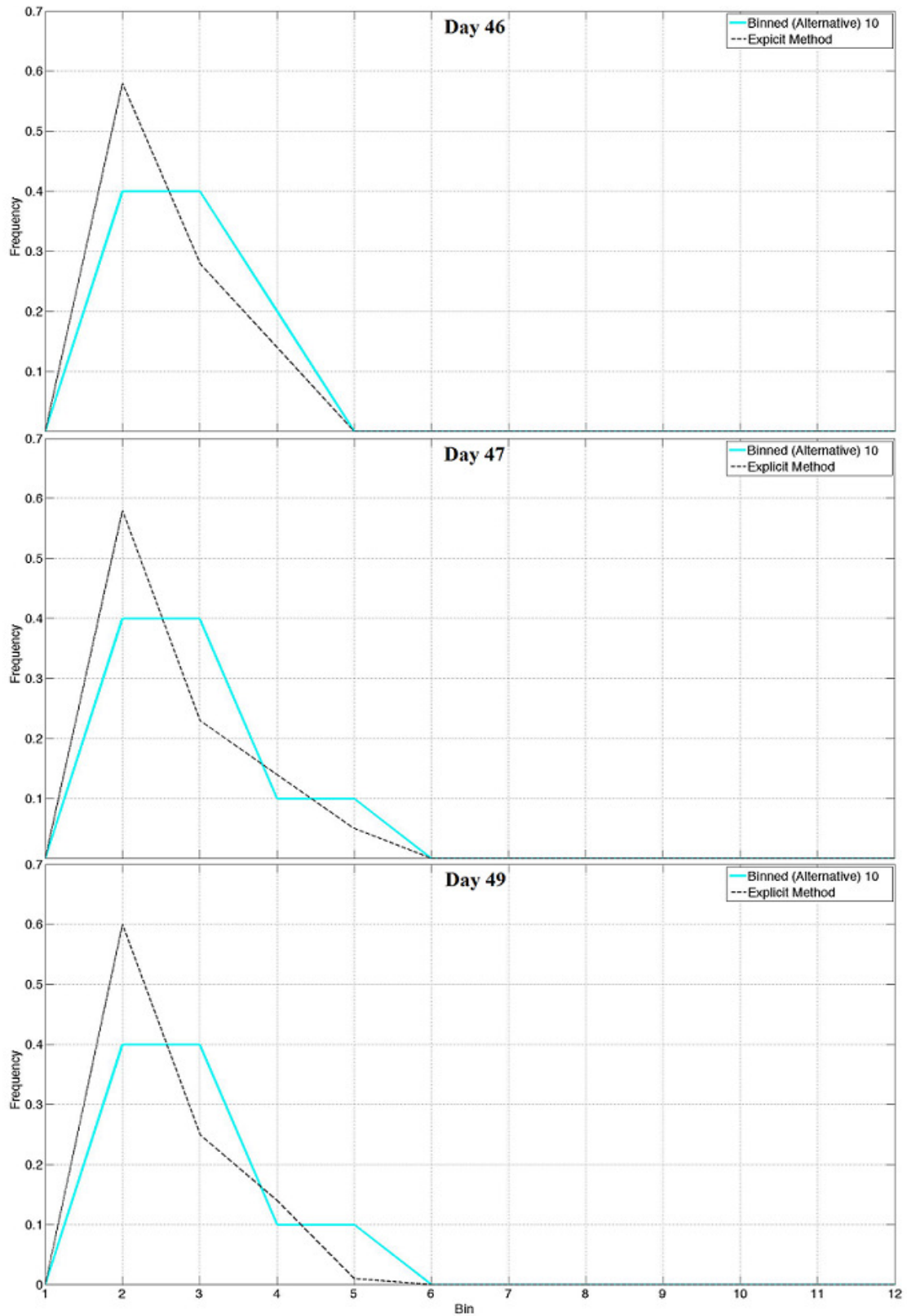
Figure 4.16j. Total plant available water distribution plots for the explicit and alternative binned (10 bins) method, where days 46 and 49 are dry and day 47 has a precipitation event (bin wetness increases to the right).
