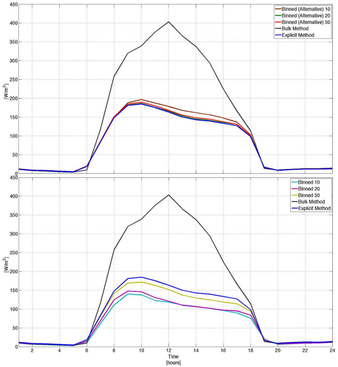
Figure 4.22d. Diurnal composites of the grid area averaged LH flux for all methods in biome 3.
