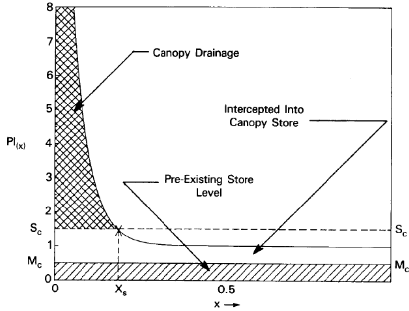
Figure 2.2b. Dynamics of precipitation intercepted by the vegetation canopy in SiB. M_c is water already stored on the canopy before precipitation interception and is uniformly distributed over the grid (hatched region). The integral of the water amount above M_c is the total amount of water intercepted by the canopy. X_s is the fraction of the grid area where intercepted rainfall added to the preexisting water storage ( M_c ) exceeds the canopy storage limit S_c . All water above S_c drains off the canopy and everything below S_c is added to the canopy interception store (Sato et al., 1989b).
