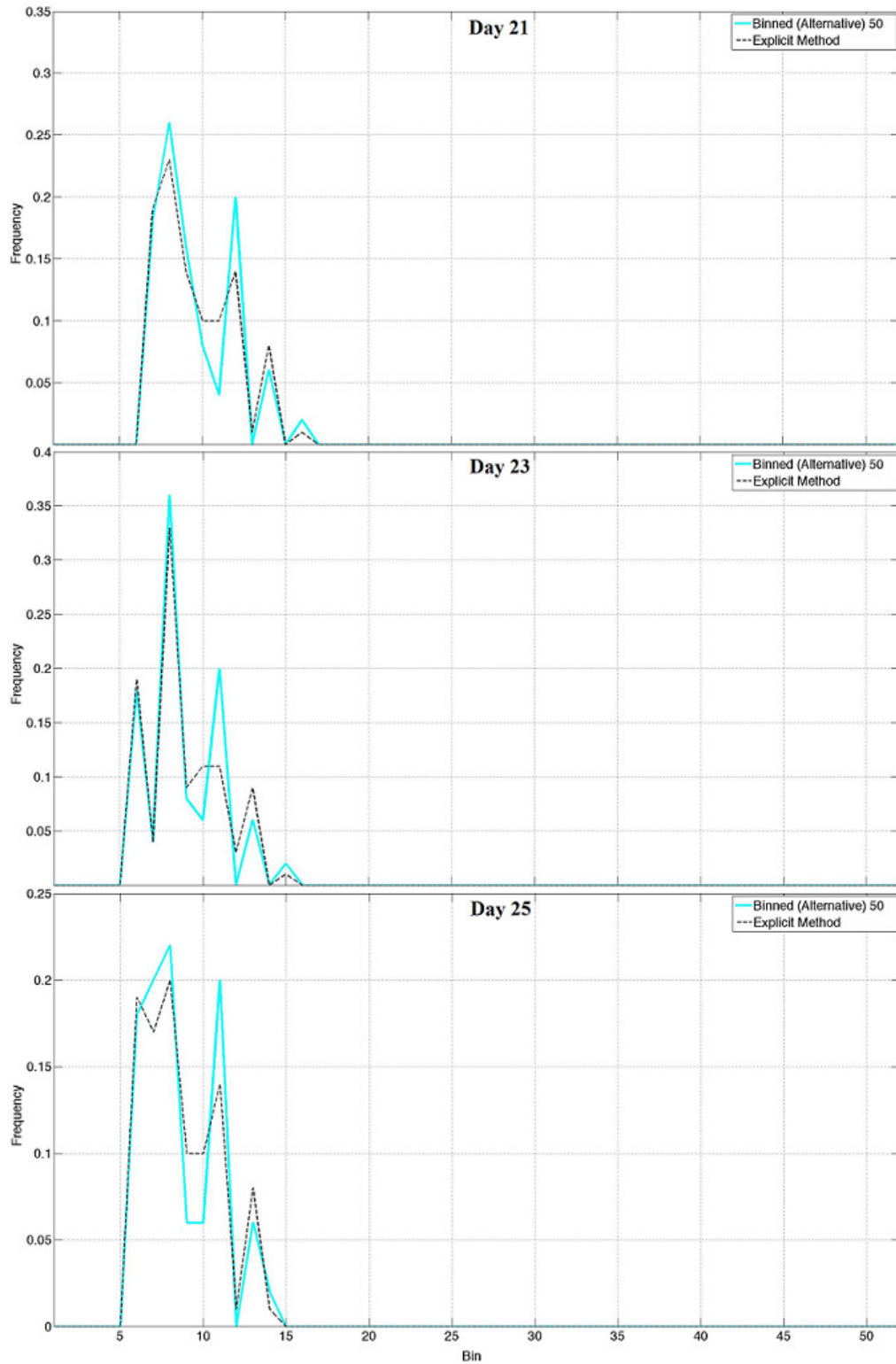
Figure 4.26f. Total plant available water distribution plots for the explicit and alternative binned (50 bins) method, where precipitation events occur each day somewhere over the grid area as a result of the highly spatially varying precipitation distribution (bin wetness increases to the right).
