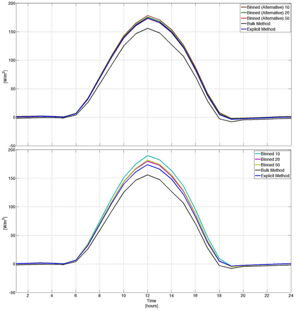
Figure 4.13c. Diurnal composites of the grid area averaged SH flux for all methods in biome 6.
