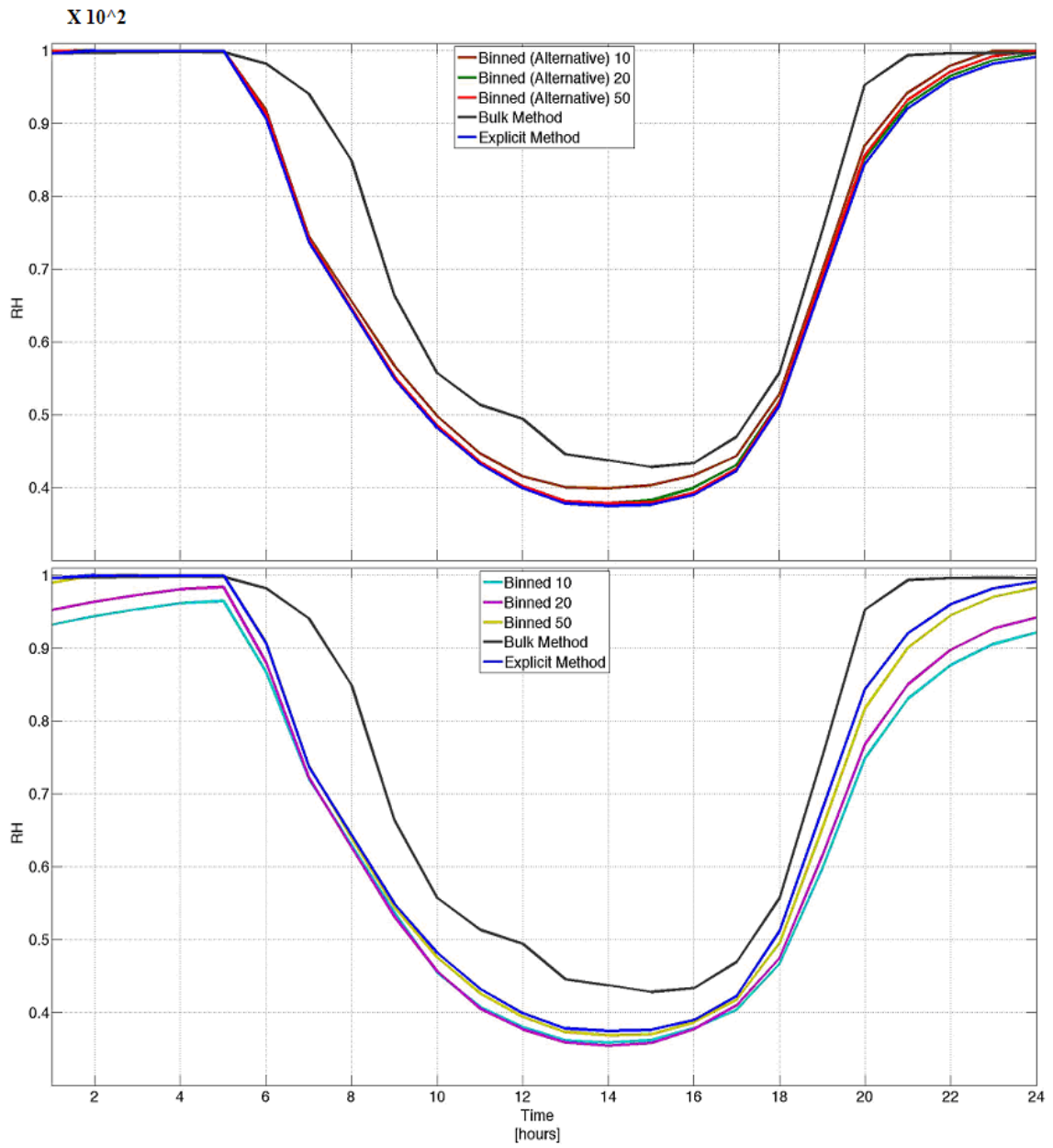
Figure 4.25f. Diurnal composites of the grid area averaged CAS relative humidity for all methods in biome 3.
