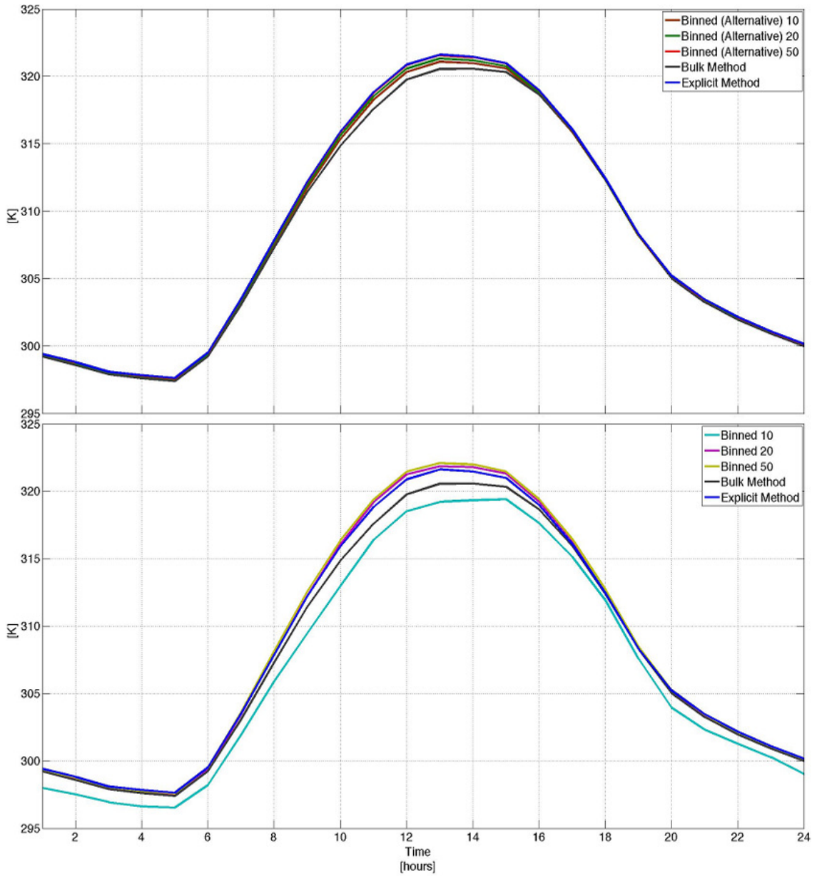
Figure 4.25a. Diurnal composites of the grid area averaged CAS temperature for all methods in biome 9.
