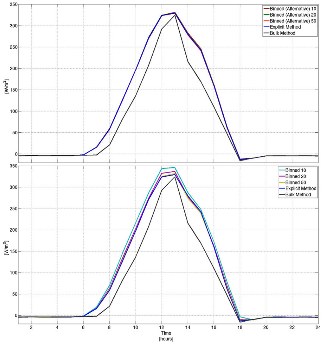
Figure 4.13d. Diurnal composites of the grid area averaged SH flux for all methods in biome 3.
