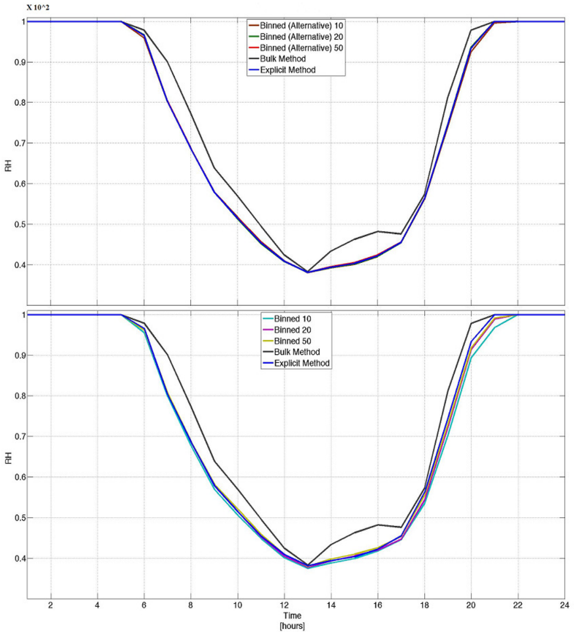
Figure 4.15f. Diurnal composites of the grid area averaged CAS relative humidity for all methods in biome 3.
