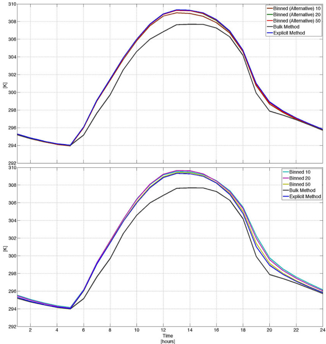
Figure 4.25c. Diurnal composites of the grid area averaged CAS temperature for all methods in biome 3.
