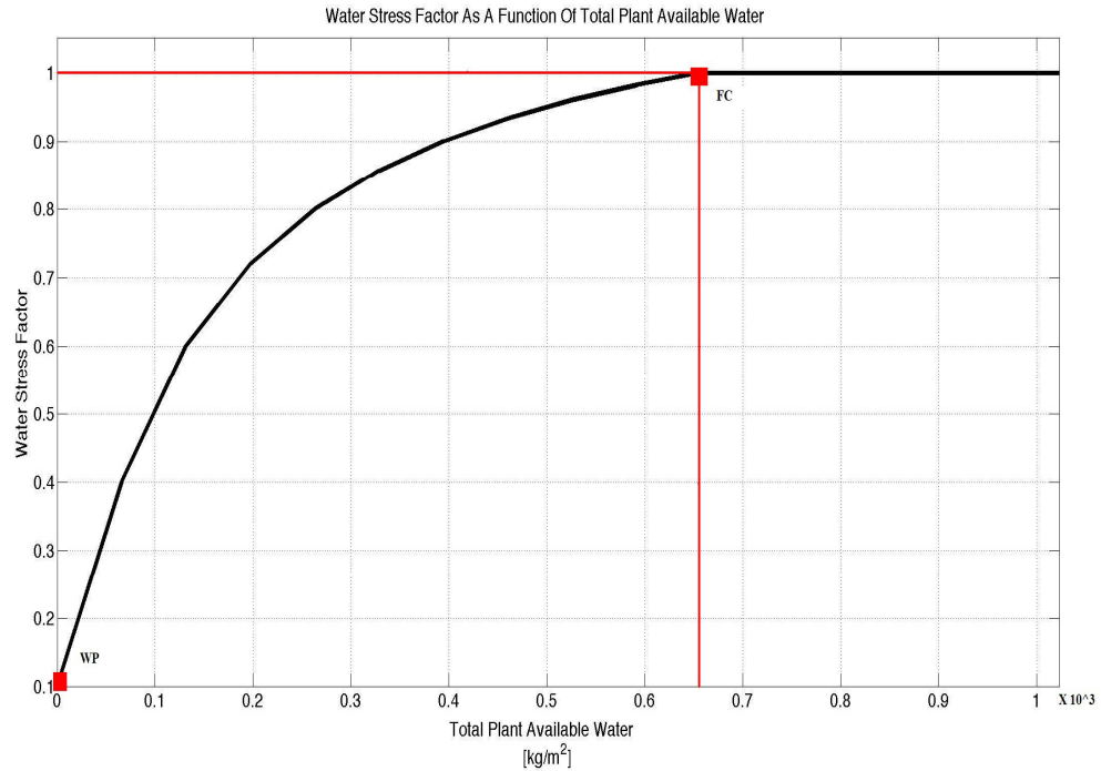
Figure 3.31a. Water stress factor as a function of PawTot for SiB-biome 6 (Oklahoma City, OK).
