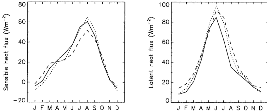
Figure 1.5b. HadAM3 GCM and MOSES 2 simulated surface energy fluxes for the tiled method (solid line), coupled aggregate model (dashed line) and off-line aggregate model (dotted line) for a grid box in Colorado (Essery et al., 2003).
