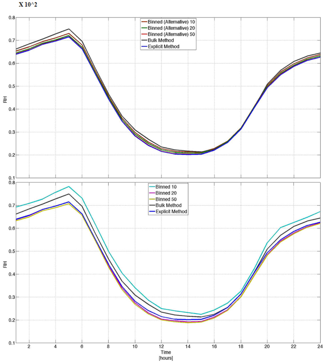
Figure 4.25d. Diurnal composites of the grid area averaged CAS relative humidity for all methods in biome 9.
