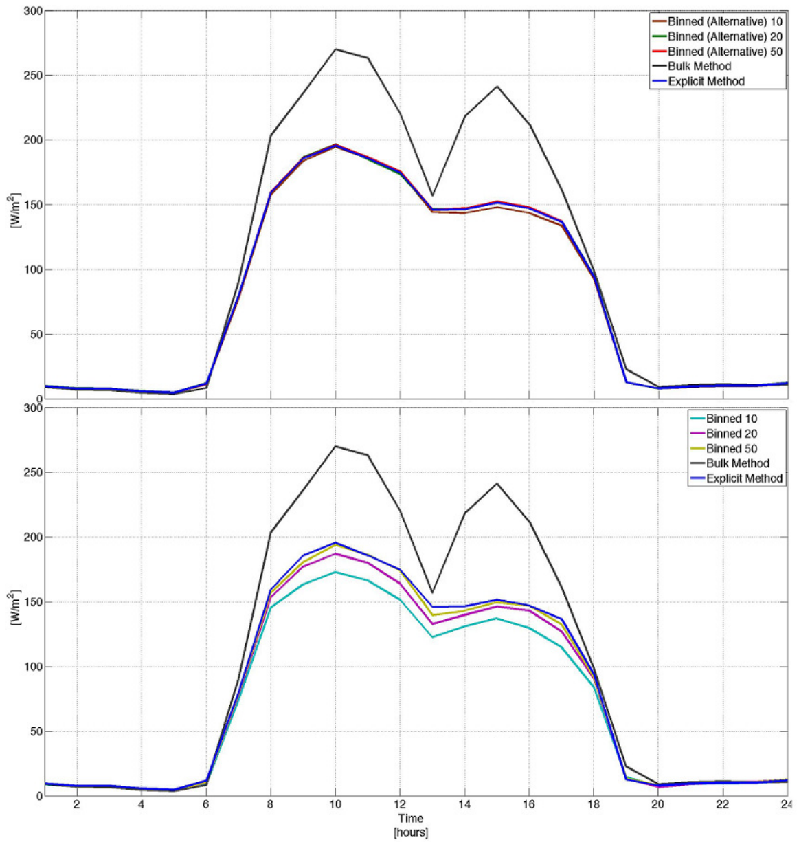
Figure 4.12d. Diurnal composites of the grid area averaged LH flux for all methods in biome 3.
