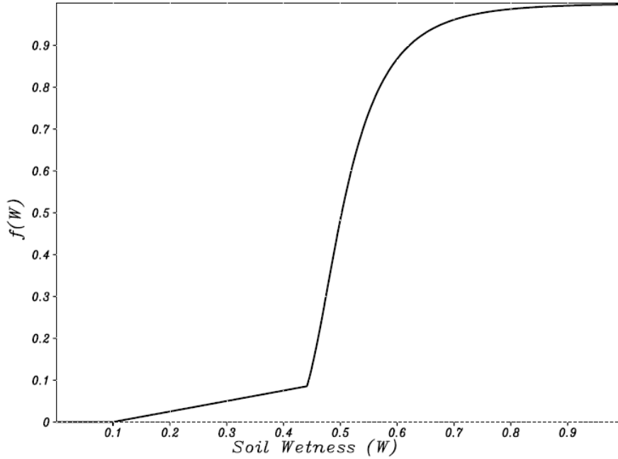
Figure 3.1a. Soil moisture stress function based on data from Colello et al. (1998) (Sellers et al., 2007).
