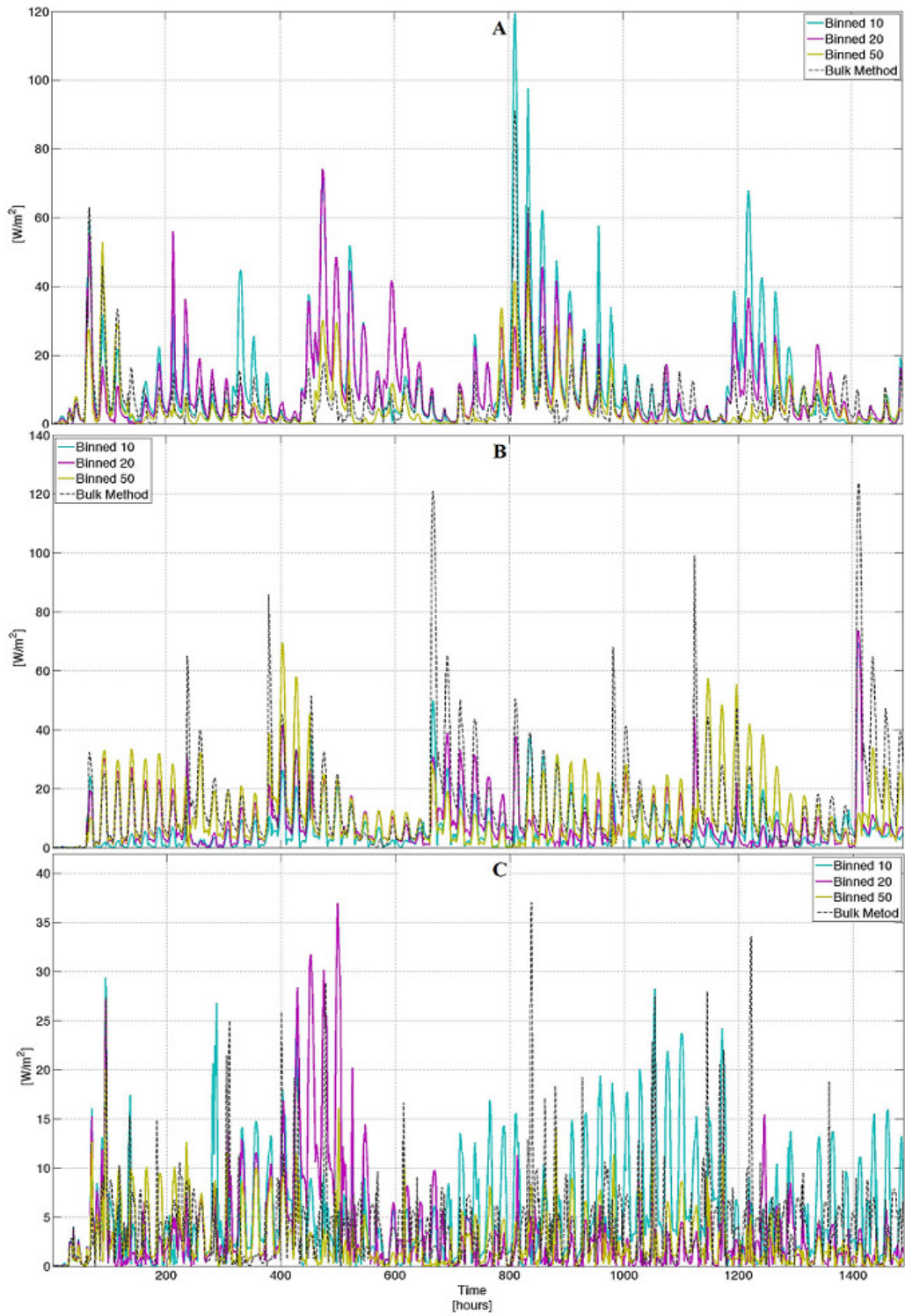
Figure 4.12f. Time series of absolute errors for the grid area averaged ground LH flux for the binned and bulk method, where panel A is biome 9, panel B is biome 6, and panel C is biome 3.
