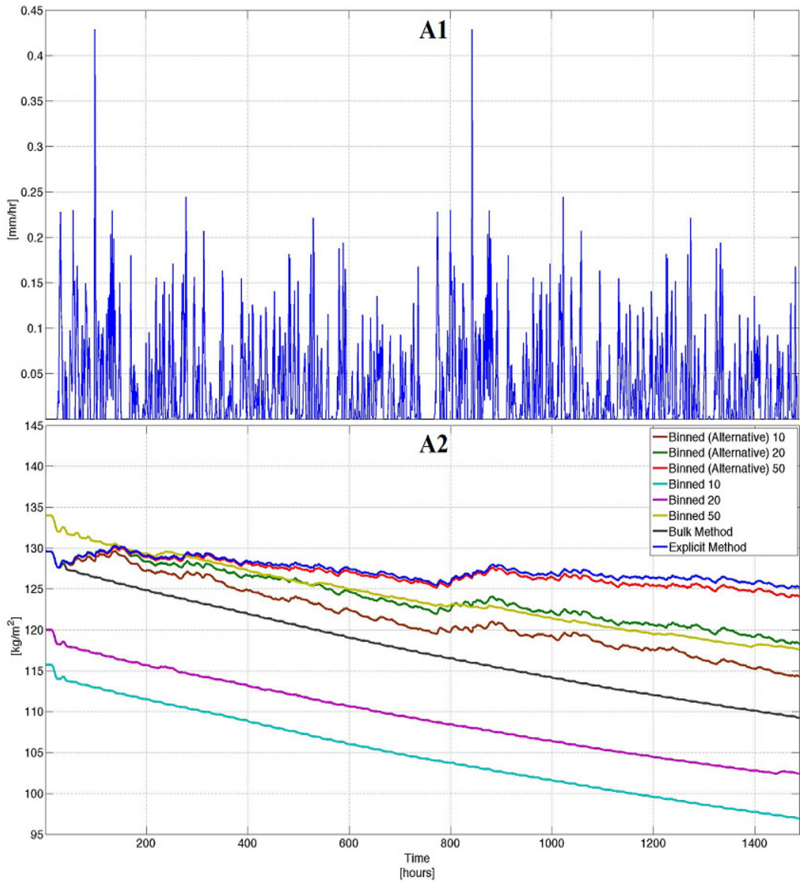
Figure 4.21a. Time series of the grid area averaged rainfall and total plant available water for biome 9, where panel A1 shows the grid area averaged rainfall rate and panel A2 is the grid area averaged total plant available water for the various methods.
