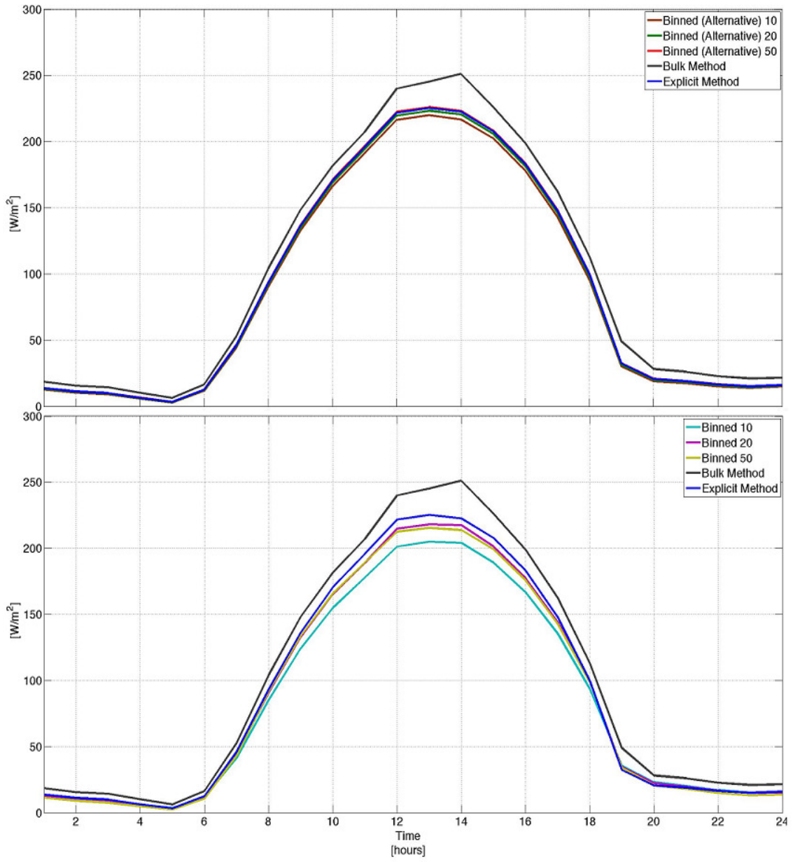
Figure 4.12c. Diurnal composites of the grid area averaged LH flux for all methods in biome 6.
