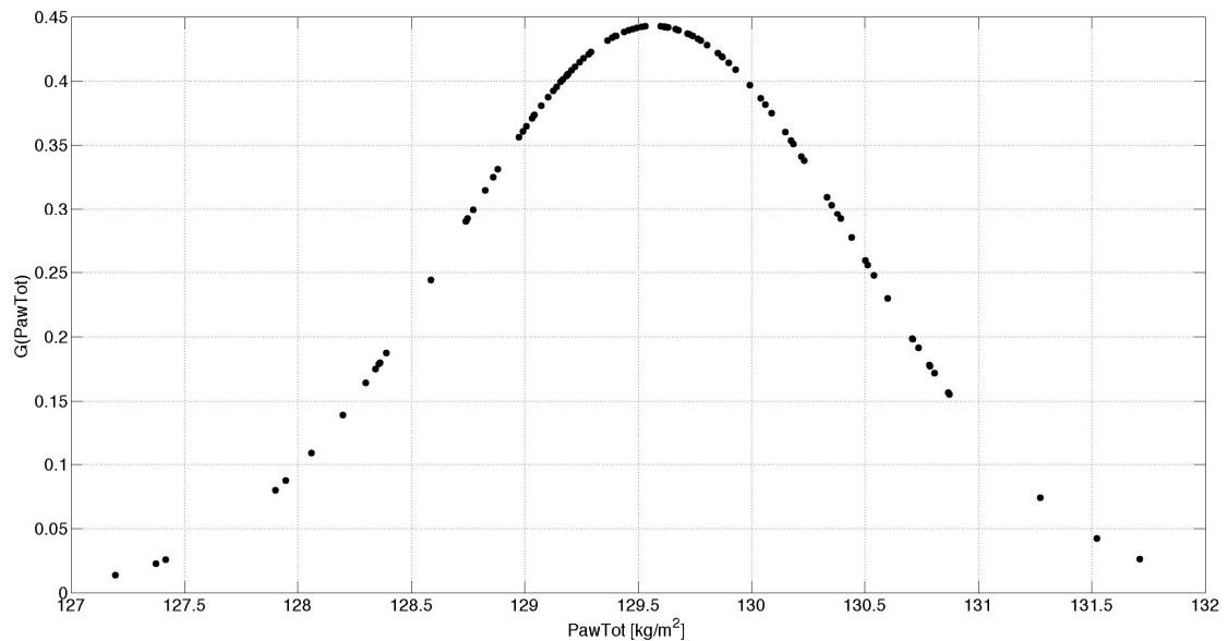
Figure 3.32a. Initial Gaussian distribution of PawTot centered on a mean value of 129.5693 \text{ kg/m}^2 for SiB-biome 6 (Oklahoma City, OK).
