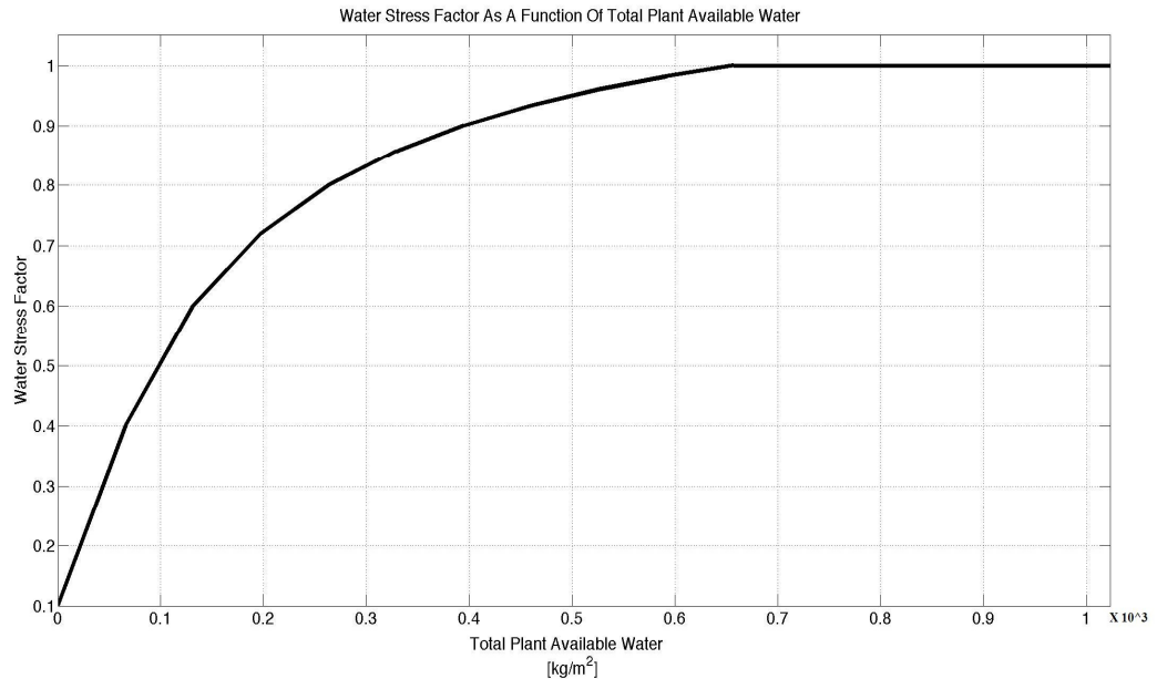
Figure 1.6a. Water stress factor as a function of PawTot for Oklahoma City, OK (SiB, biome 6).
