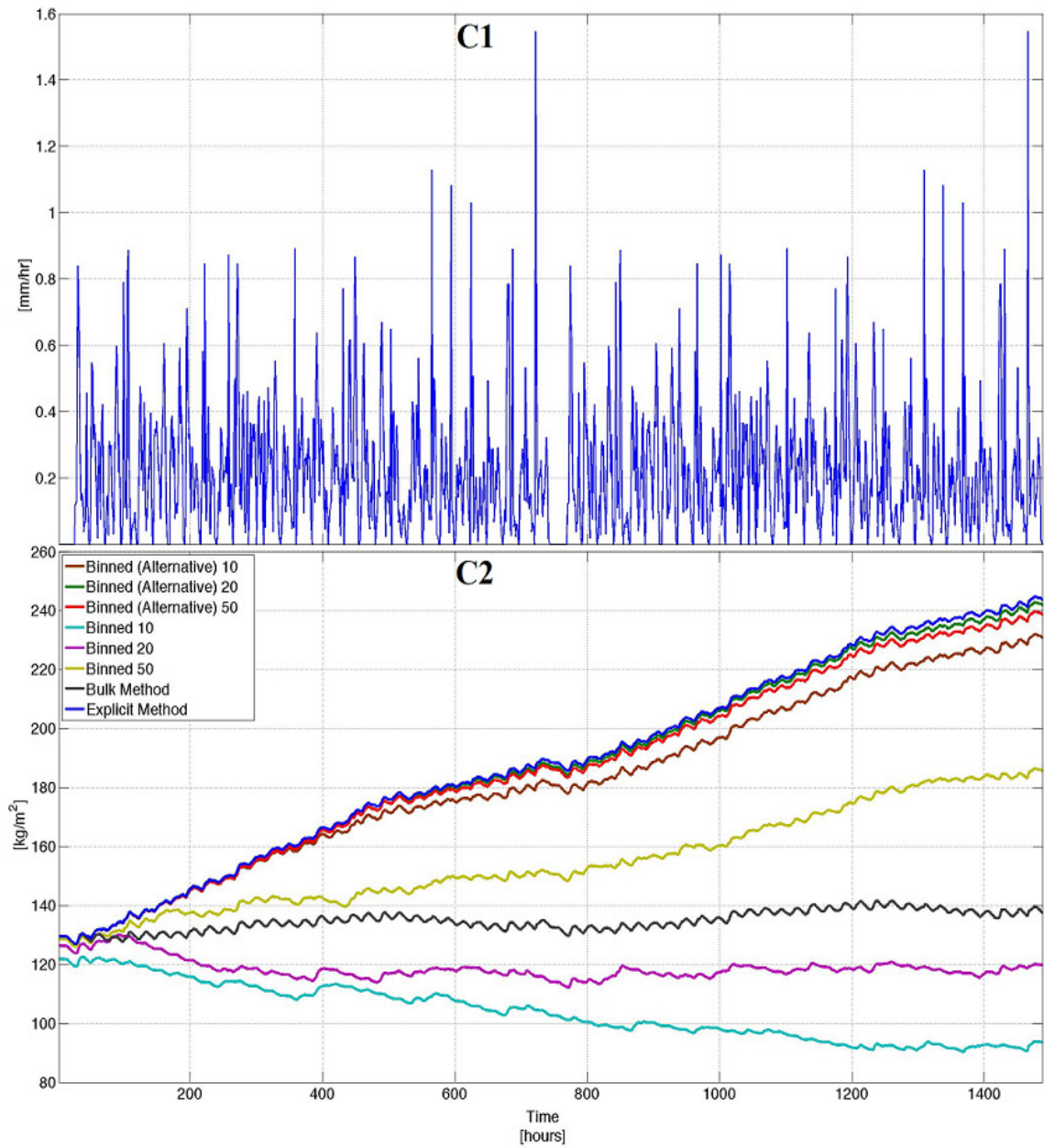
Figure 4.21c. Time series of the grid area averaged rainfall and total plant available water for biome 3, where panel C1 shows the grid area averaged rainfall rate and panel C2 is the grid area averaged total plant available water for the various methods.
