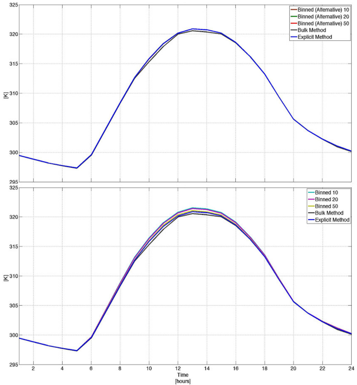
Figure 4.15a. Diurnal composites of the grid area averaged CAS temperature for all methods in biome 9.
