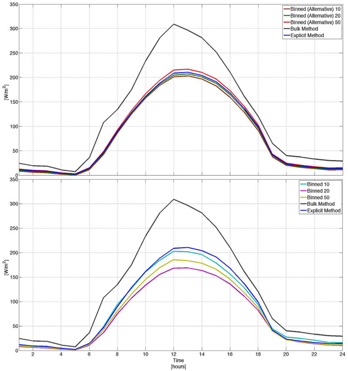
Figure 4.22c. Diurnal composites of the grid area averaged LH flux for all methods in biome 6.
