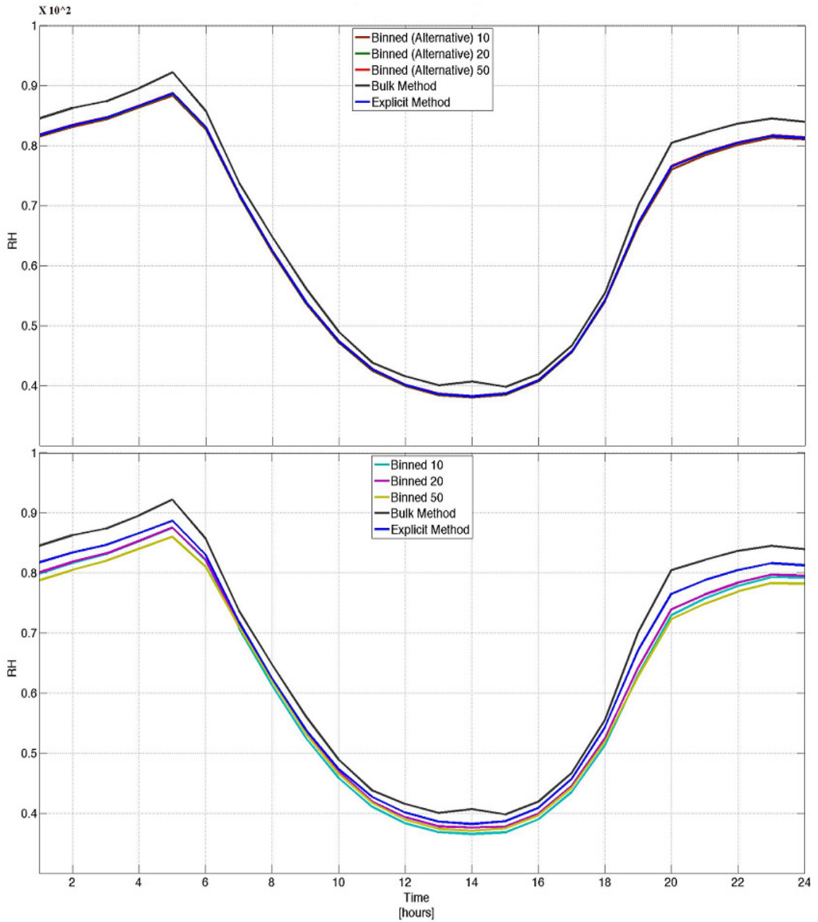
Figure 4.15e. Diurnal composites of the grid area averaged CAS relative humidity for all methods in biome 6.
