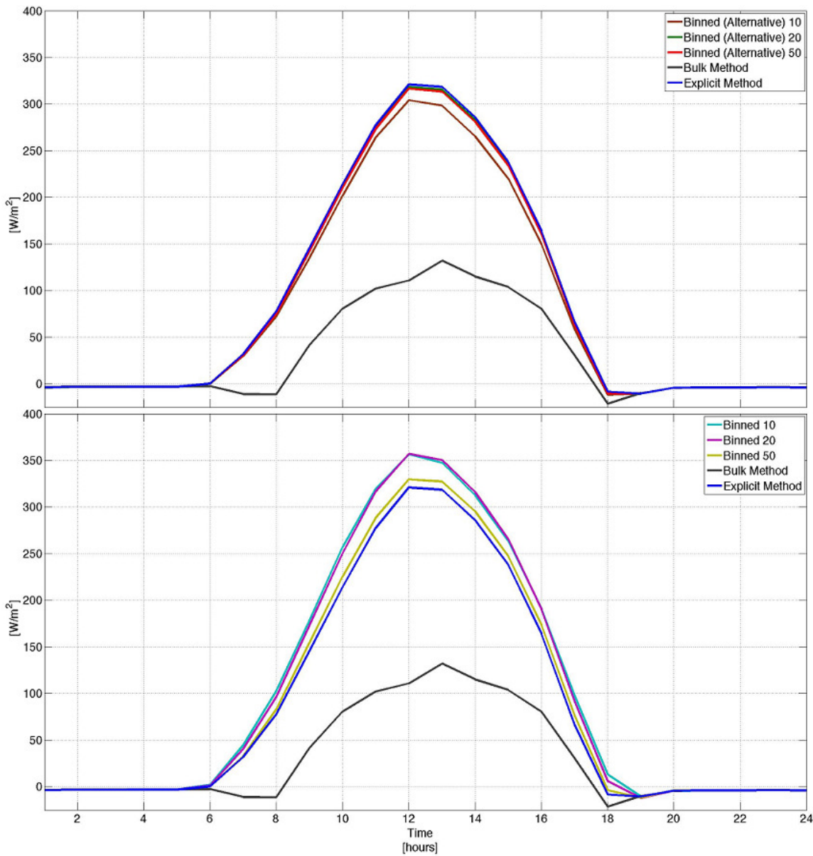
Figure 4.23d. Diurnal composites of the grid area averaged SH flux for all methods in biome 3.
