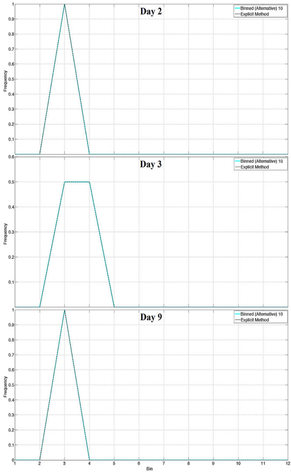
Figure 4.16d. Total plant available water distribution plots for the explicit and alternative binned (10 bins) method, where days 2 and 9 are dry and day 3 has a precipitation event (bin wetness increases to the right).
