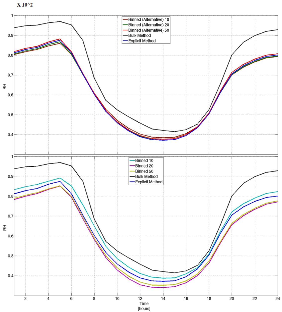
Figure 4.25e. Diurnal composites of the grid area averaged CAS relative humidity for all methods in biome 6.
