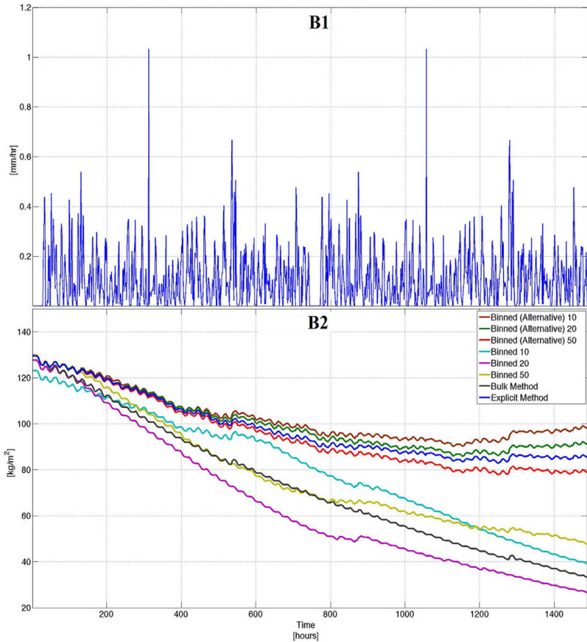
Figure 4.21b. Time series of the grid area averaged rainfall and total plant available water for biome 6, where panel B1 shows the grid area averaged rainfall rate and panel B2 is the grid area averaged total plant available water for the various methods.
