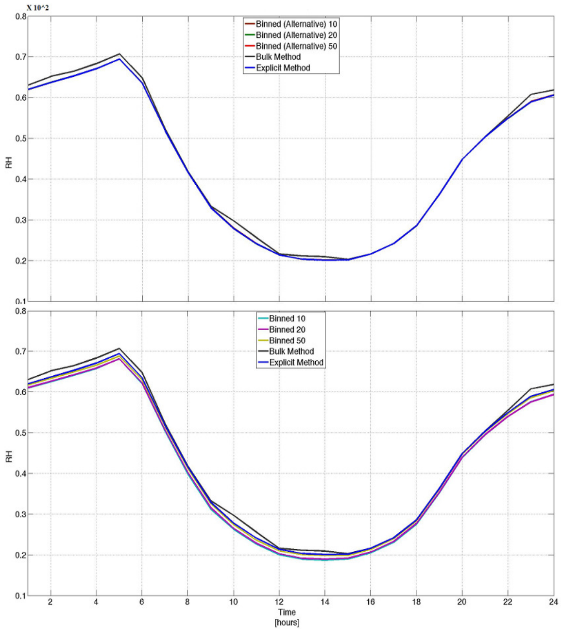
Figure 4.15d. Diurnal composites of the grid area averaged CAS relative humidity for all methods in biome 9.
