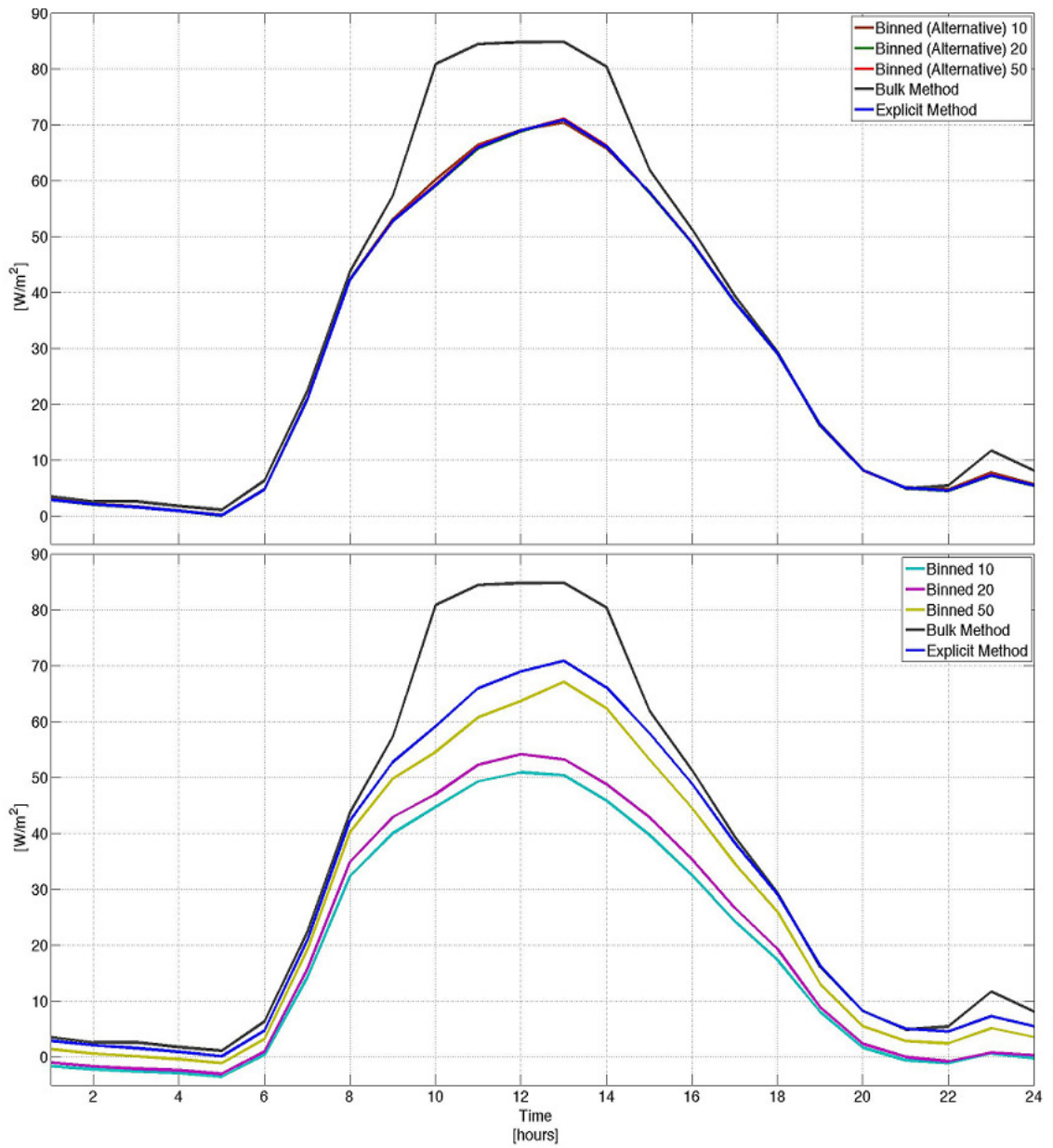
Figure 4.12b. Diurnal composites of the grid area averaged LH flux for all methods in biome 9.
