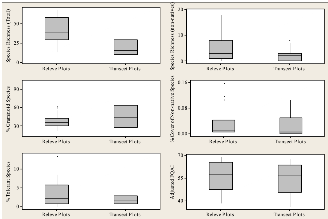
Figure 16. Boxplots of Selected Metrics for Relève and Transect Plot Methods
