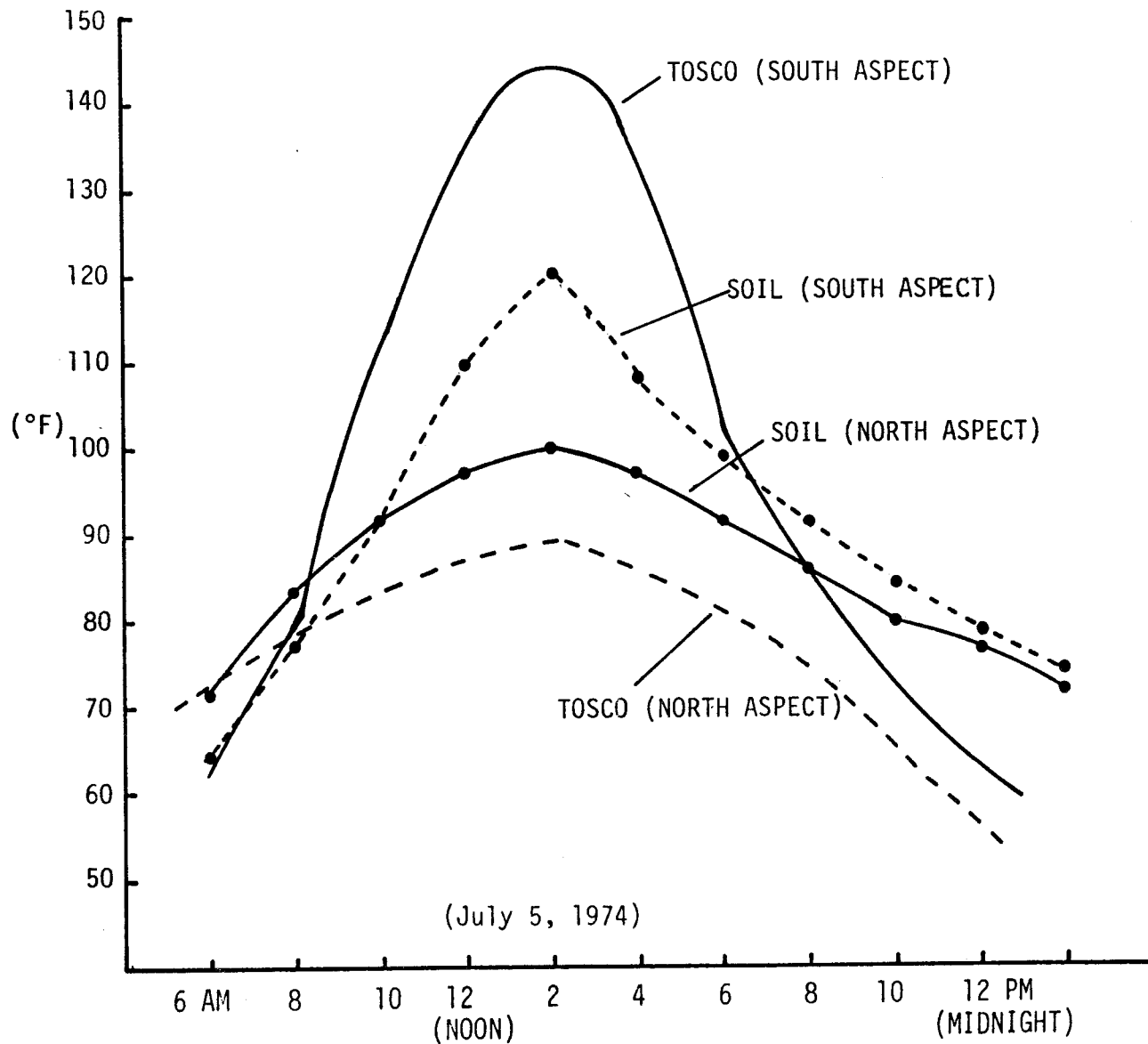
Figure 10. Surface temperatures of TOSCO spent shale and 6" of soil cover over TOSCO spent shale, north and south aspects (Anvil Points study site, July 5, 1974).
