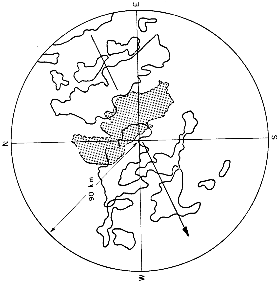
1.1 Composite radar echo of squall-line number 47 July 24, 1972.
