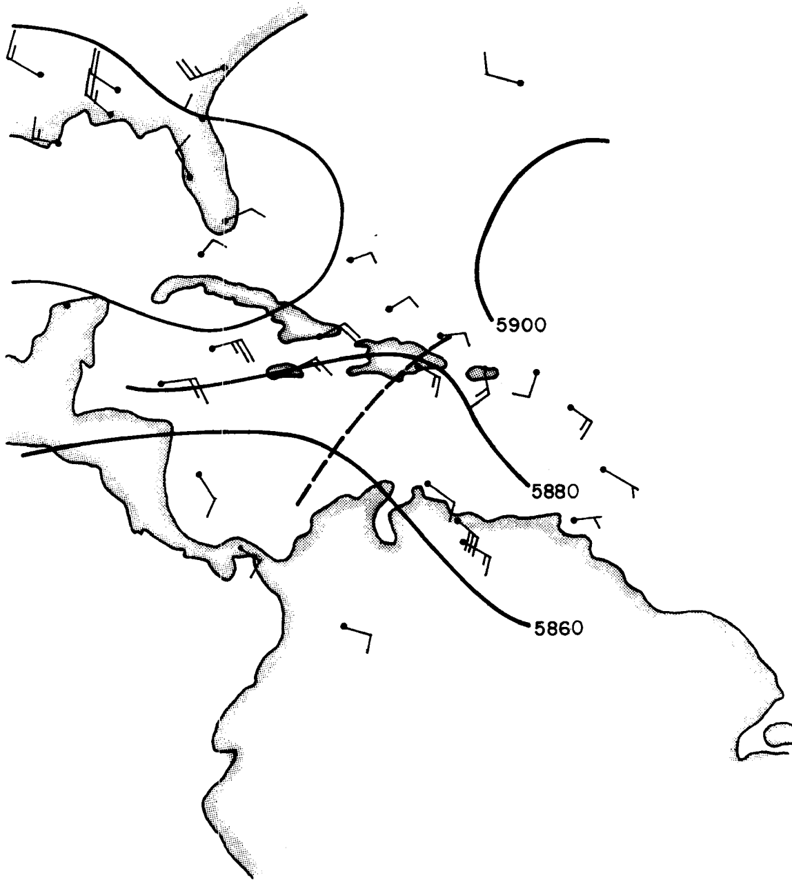
Figure 4.5 - Height pattern on 500 mb surface at 1200 Z, August 12, 1972.
