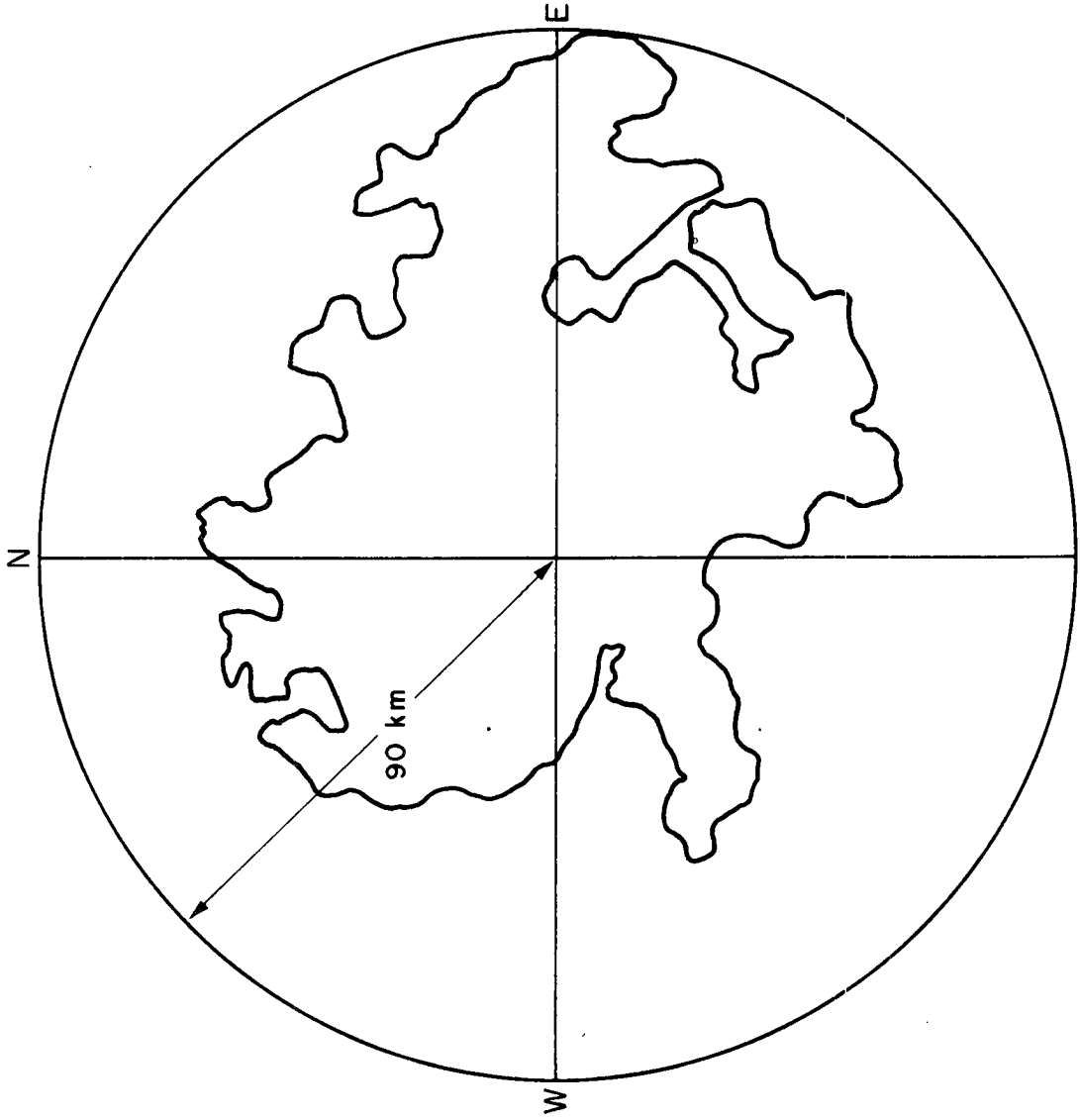
Figure 4.7 - Storm 109 at 0800 LST on September 2nd.
