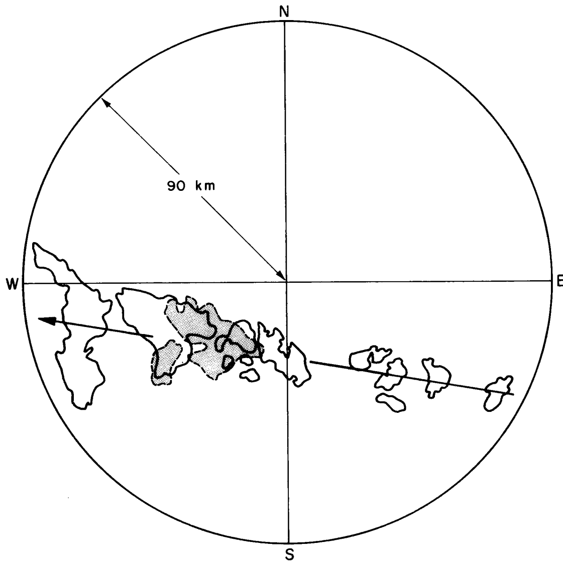
Figure 4.12 - Storm 68 at 1/2 hour intervals from 1400 LST on August 12, 1972 as seen by radar.
