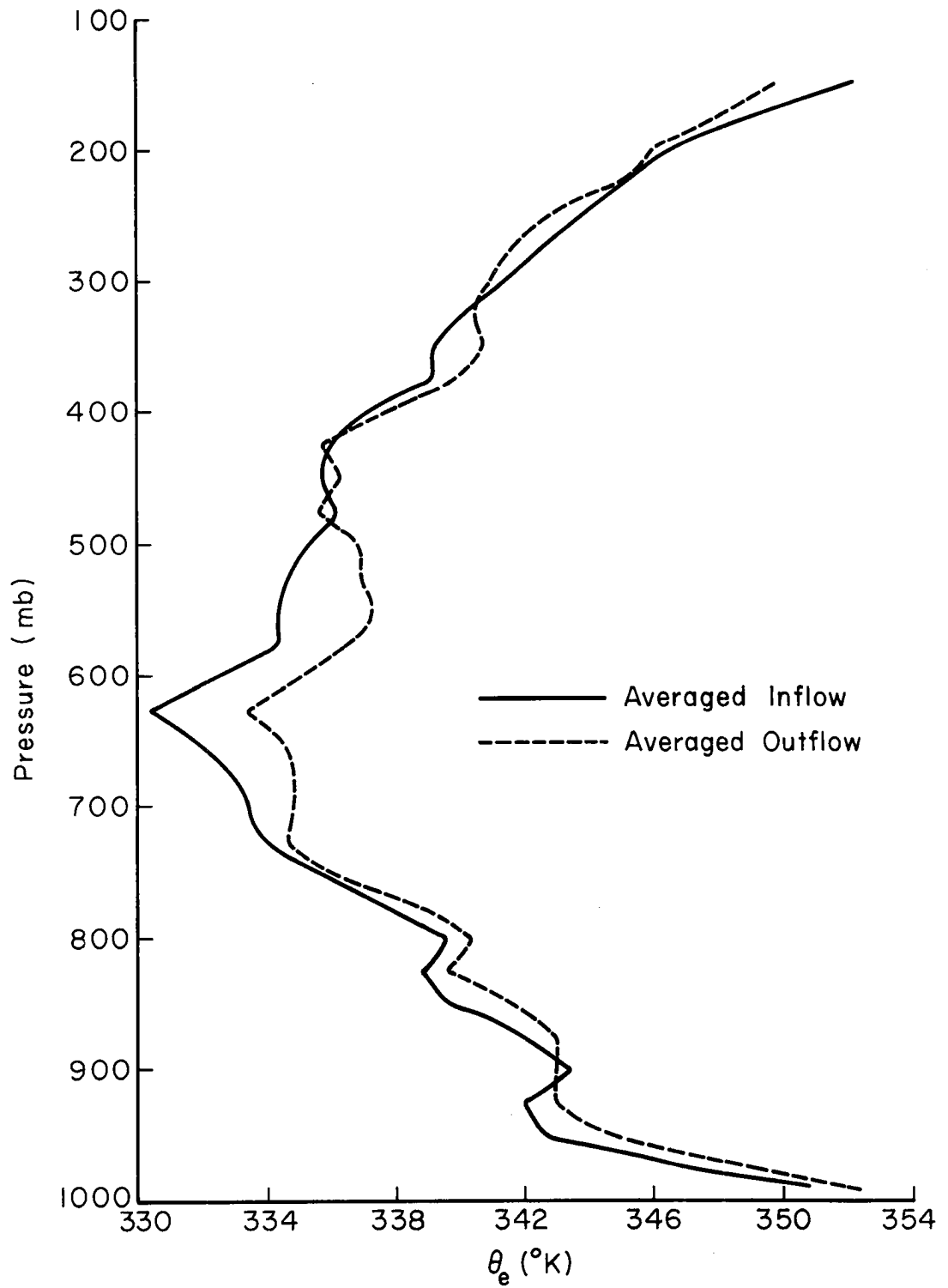
Figure 4.24 - Composite non-squall-line \theta_e profiles.
